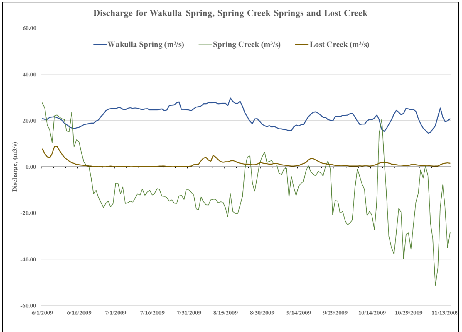
Figure 6.7: Discharge for Wakulla Spring, Spring Creek Springs and Lost Creek swallet for duration of the 2009 Lost Creek swallet trace.
