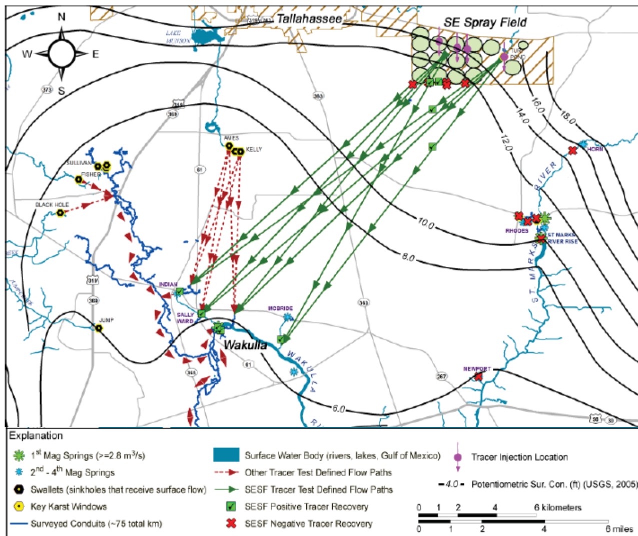
Figure 3.15: Combined results of the 2002-2006 dye traces in the Woodville Karst Plain. (Modified from Kincaid et al., 2012).
