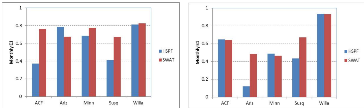
Figure 28. Comparison of baseline adjusted model fit efficiency for total suspended solids monthly loads for calibration site (left) and downstream site (right).
