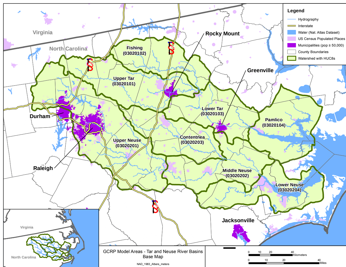
Figure 15. Tar/Neuse River basin model area.
