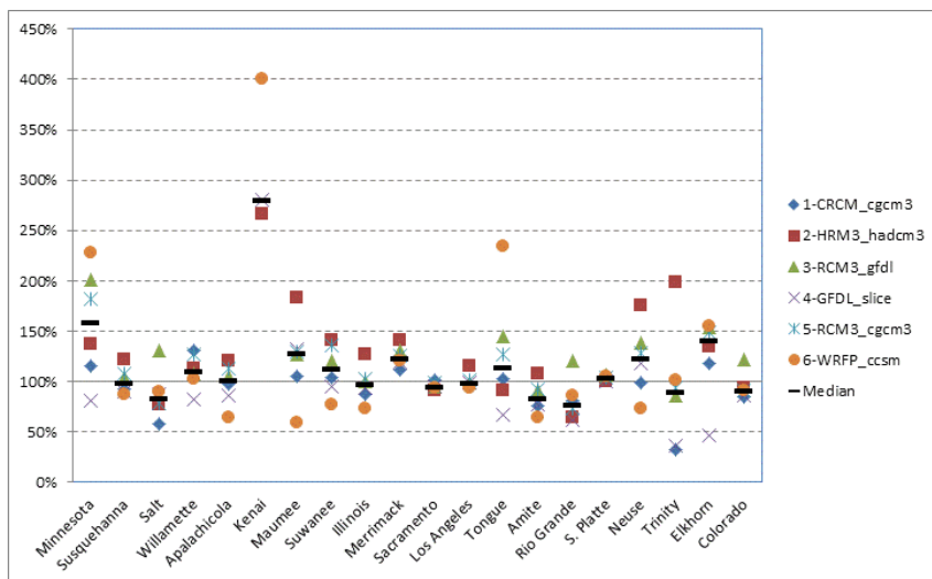
Figure 40. Simulated 7-day low flow relative to current conditions (NARCCAP climate scenarios with urban development) for selected downstream stations
