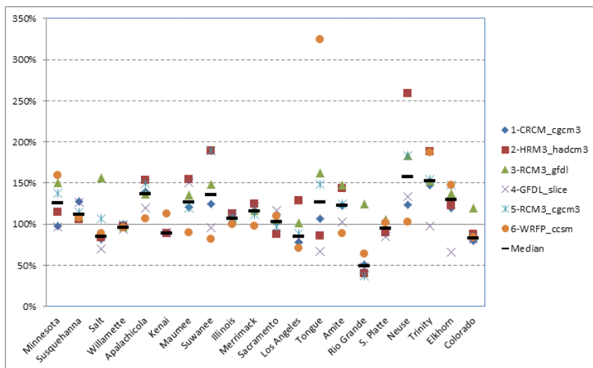
Figure 50. Simulated total phosphorus load relative to current conditions (NARCCAP climate scenarios with urban development) for selected downstream stations.
