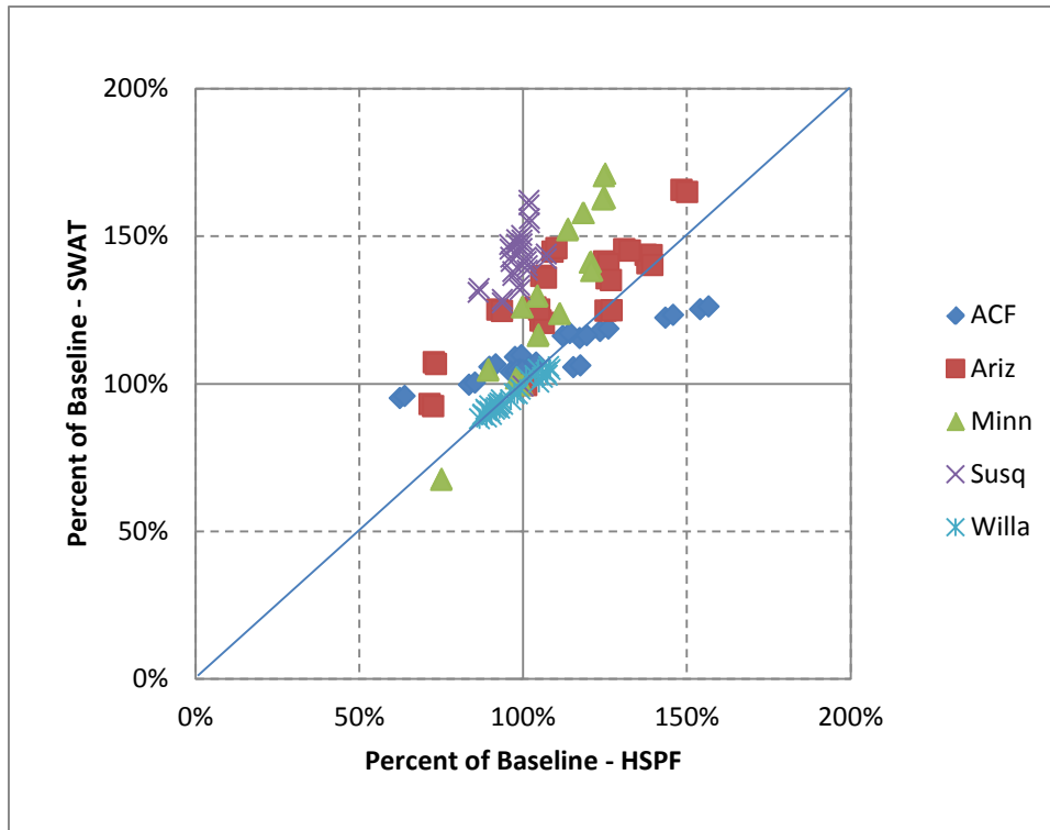
Figure 33. SWAT and HSPF simulated changes in total nitrogen load in pilot watersheds (expressed relative to current conditions).
