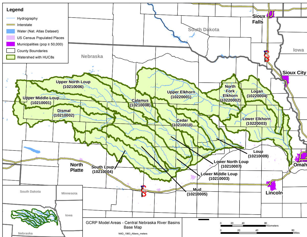
Figure 14. Loup and Elkhorn River basins model area.
