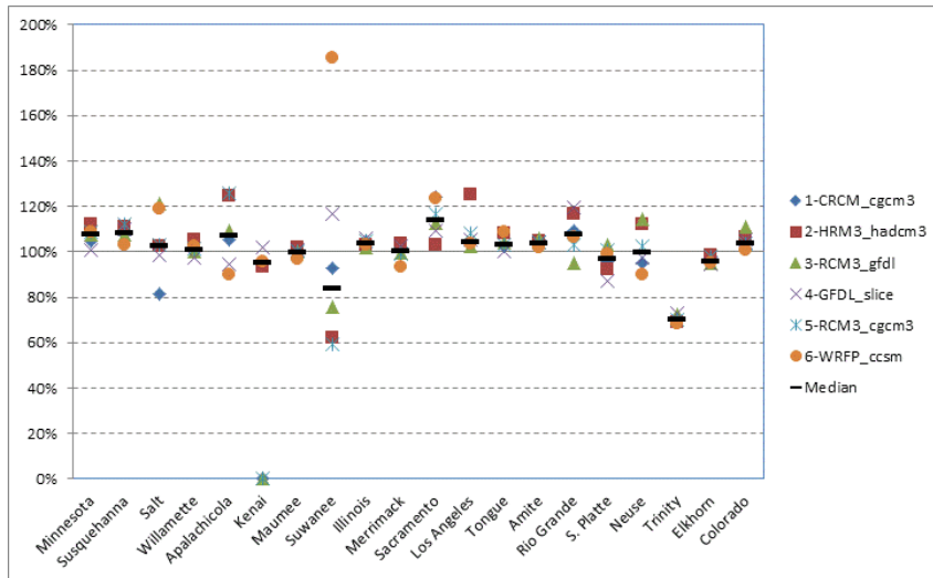
Figure 46. Simulated Richards-Baker flashiness index relative to current conditions (NARCCAP climate scenarios with urban development) for selected downstream stations
