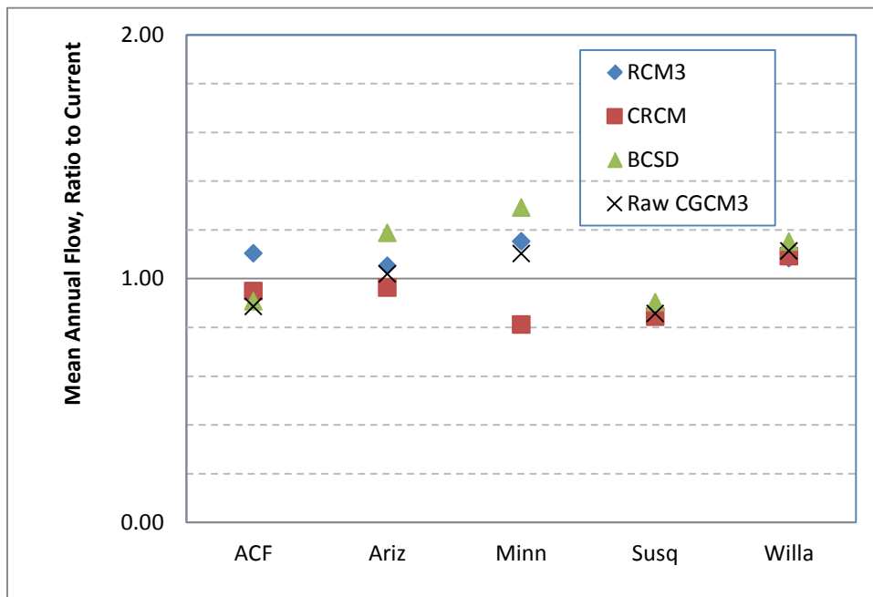
Figure 36. Consistency in SWAT model predictions of mean annual flow with downscaled (NARCCAP, BCSD) and GCM projections of the CGCM3 GCM
