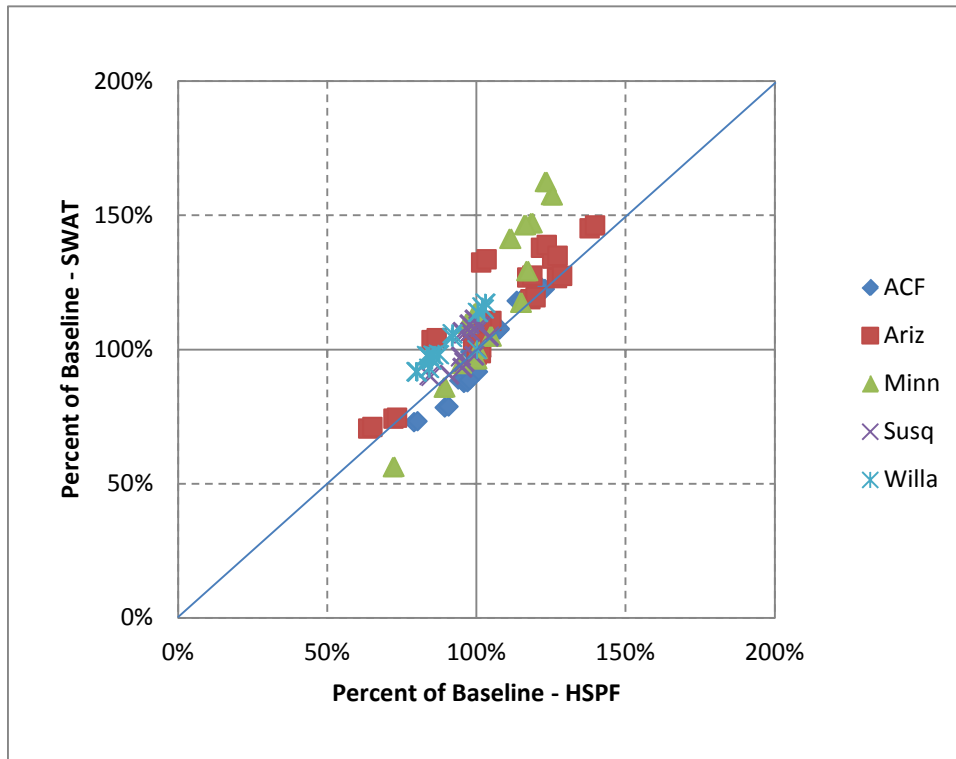
Figure 31. SWAT and HSPF simulated changes in total flow in pilot watersheds (expressed relative to current conditions).
