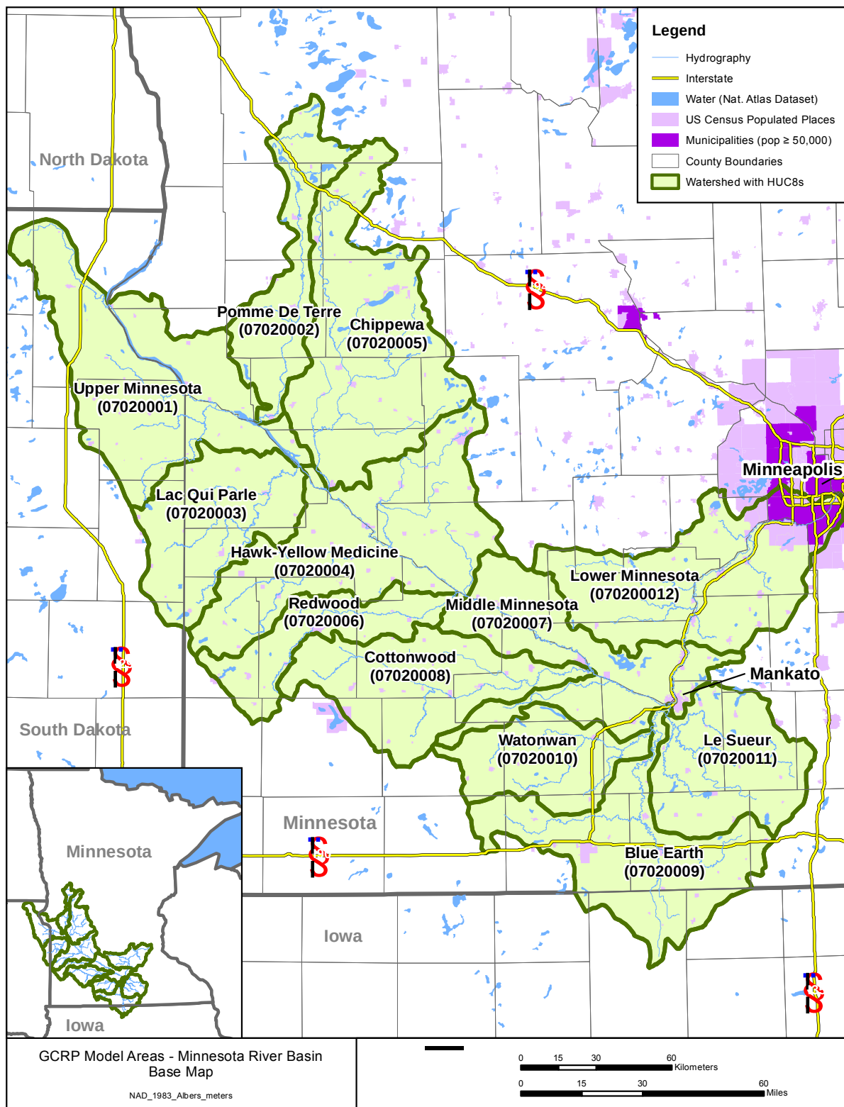
1 2 Figure 3. Minnesota River watershed.
