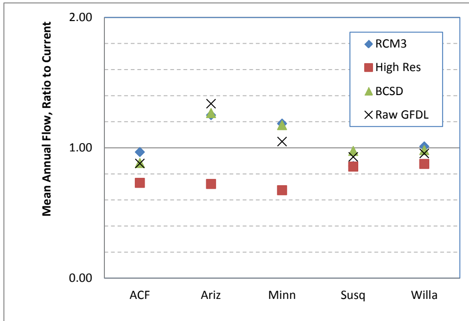
Figure 35. Consistency in SWAT model predictions of mean annual flow with downscaled (NARCCAP, BCSD) and GCM projections of the GFDL GCM
