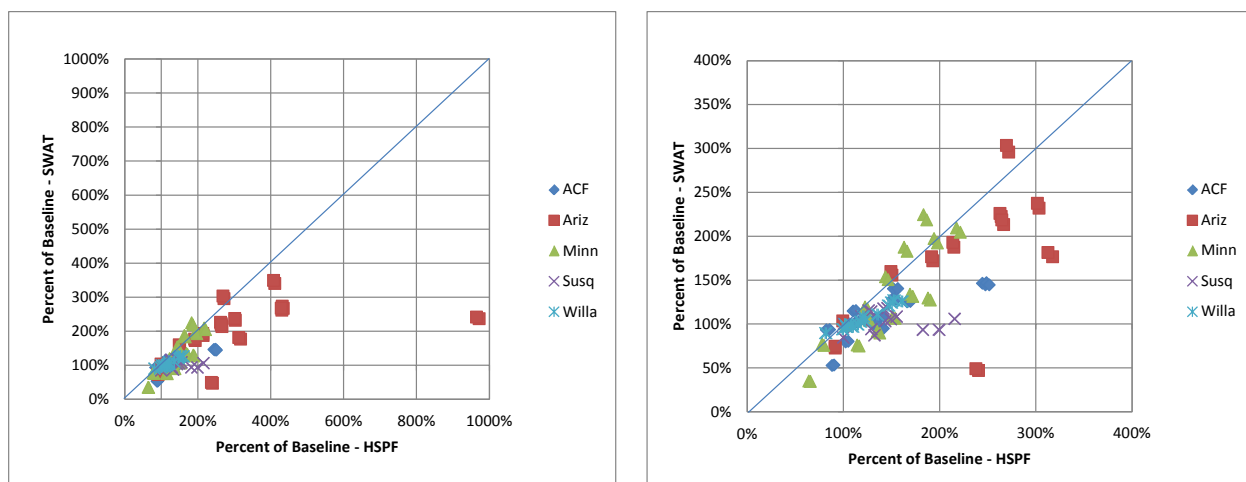
Figure 32. SWAT and HSPF simulated changes in TSS in pilot watersheds (expressed relative to current conditions).
