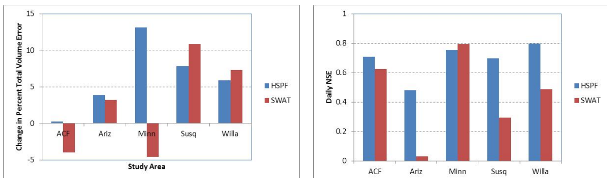
Figure 26. Sensitivity of model fit for total flow volume to temporal change.
