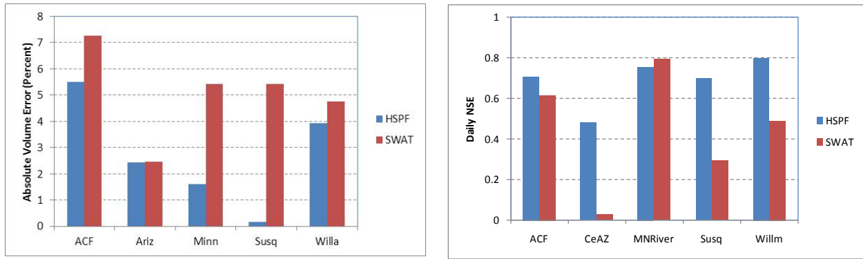
Figure 25. Comparison of model calibration fit to flow for the calibration initial site.
