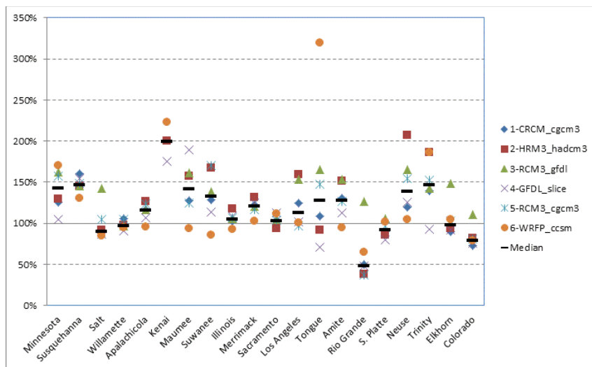
Figure 52. Simulated total nitrogen load relative to current conditions (NARCCAP climate scenarios with urban development) for selected downstream stations.
