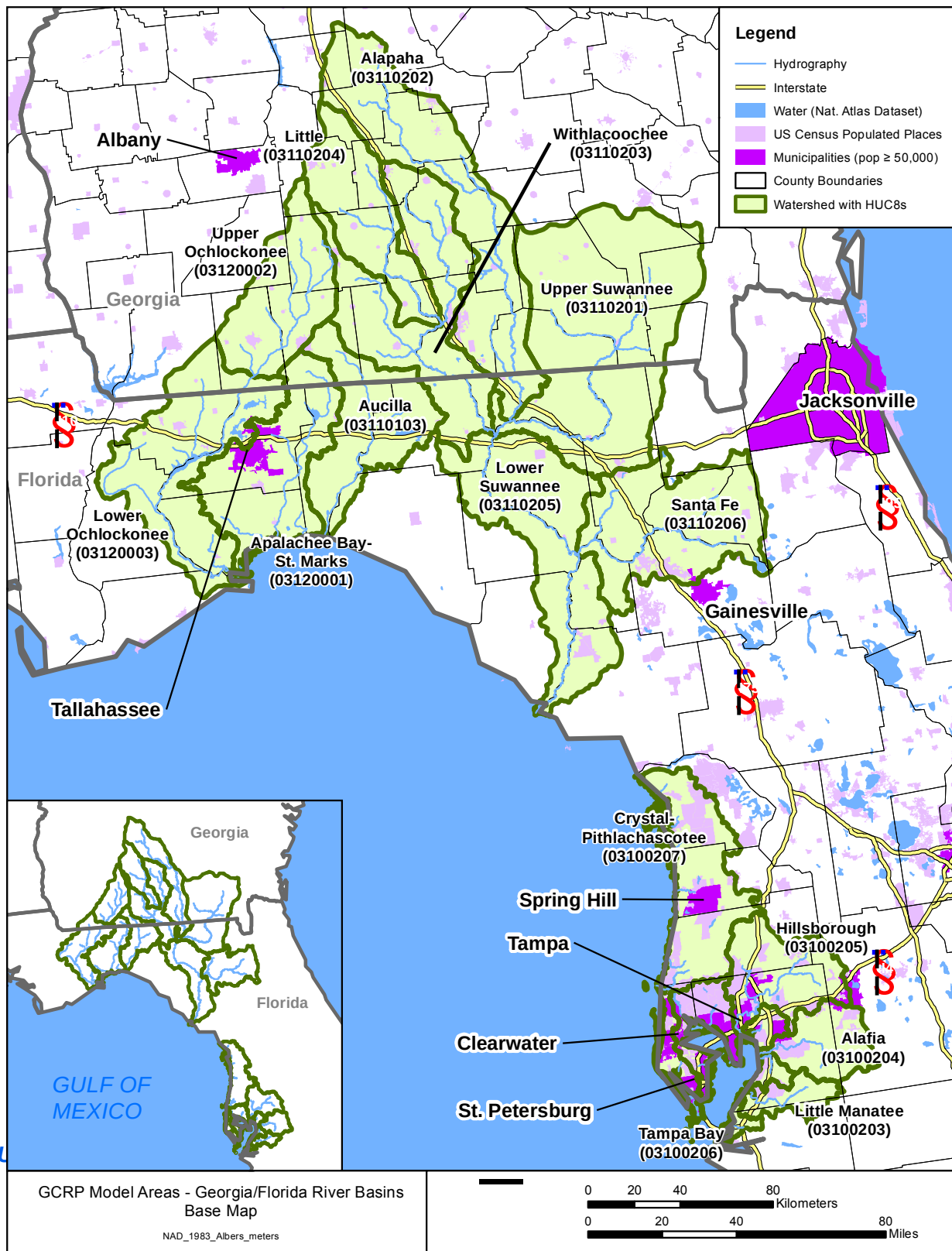
Figure 10. Georgia-Florida Coastal Plain basins model area.
