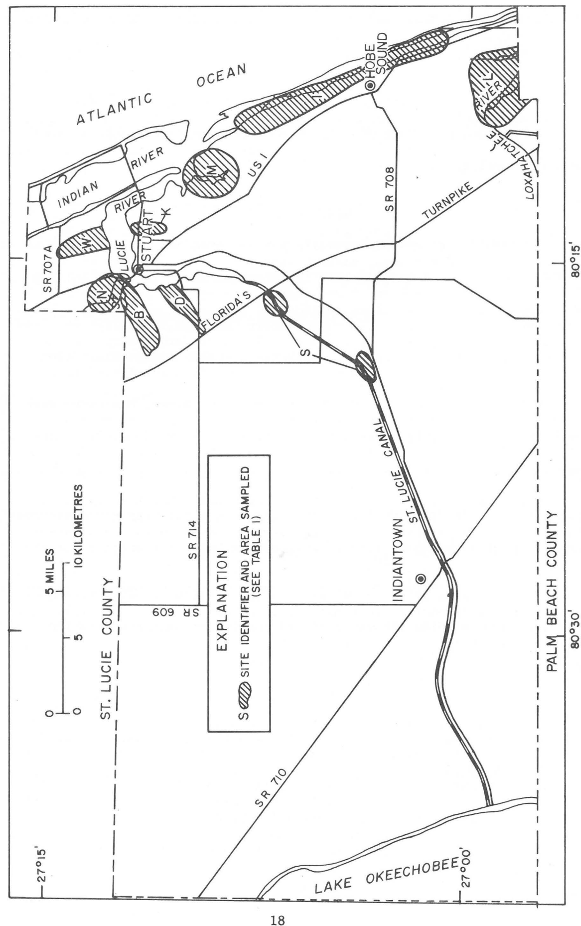
Figure 10. Location of water-quality sampling sites.
