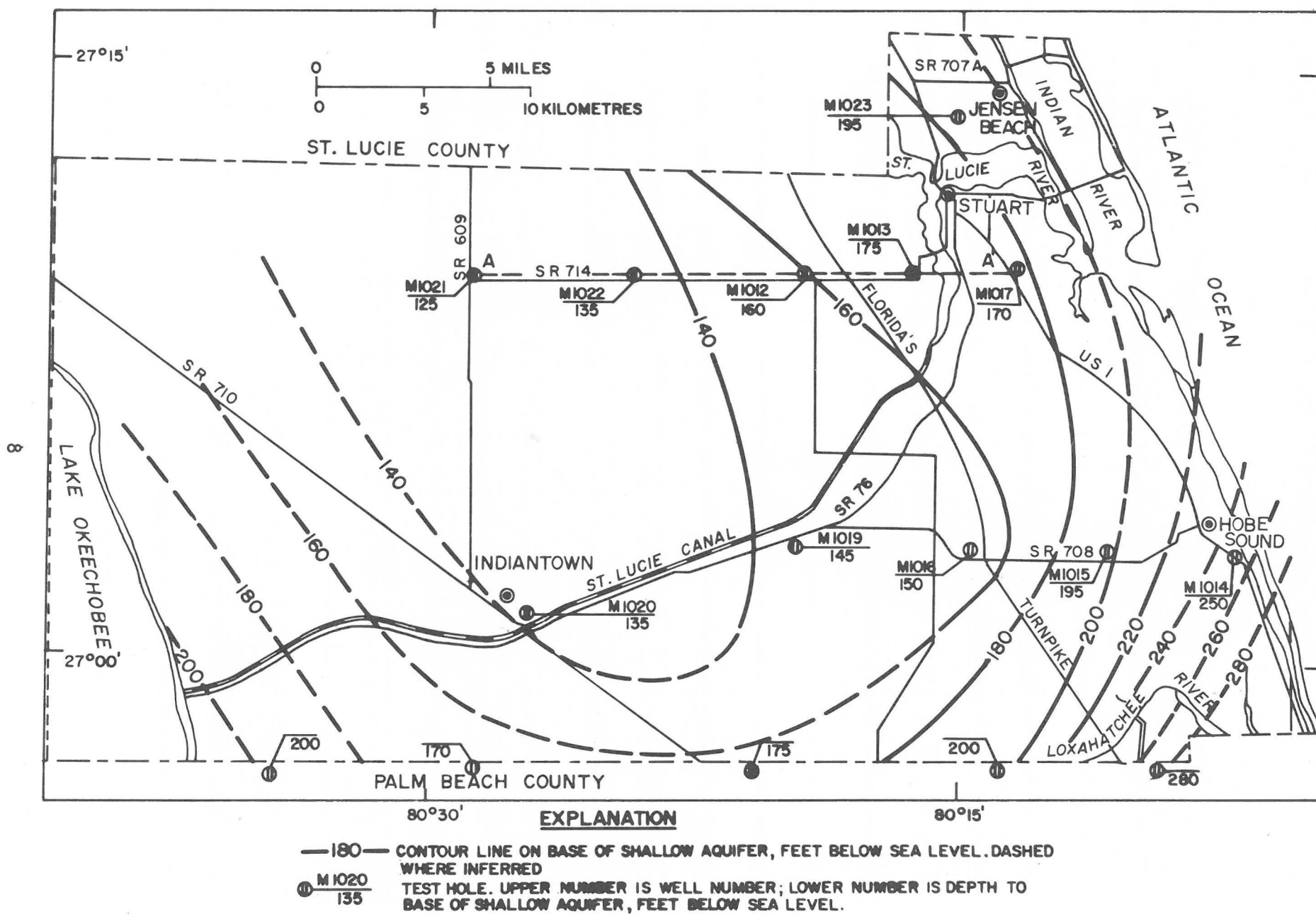
Figure 2. Location of test holes, and contours of the base of the shallow aquifer.
