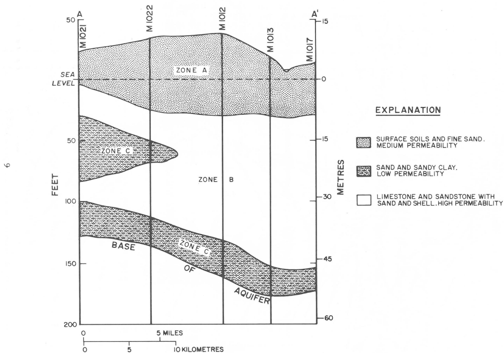
Figure 3. Geologic section showing zones of high and low permeability.
