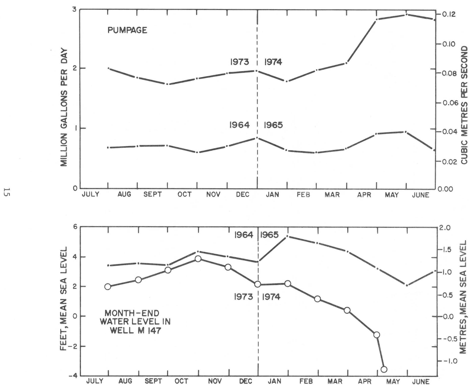
Figure 8. Pumpage from municipal supply wells at Stuart, and the water level in well M 147 for July 1964 - June 1965 and July 1973 - June 1974.
