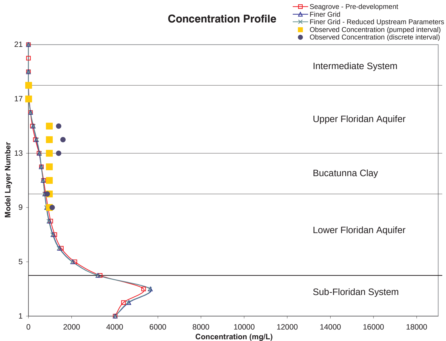
Figure 4.24 Concentration Profiles at Seagrove for Pre-Development and Grid Sensitivity Simulations
