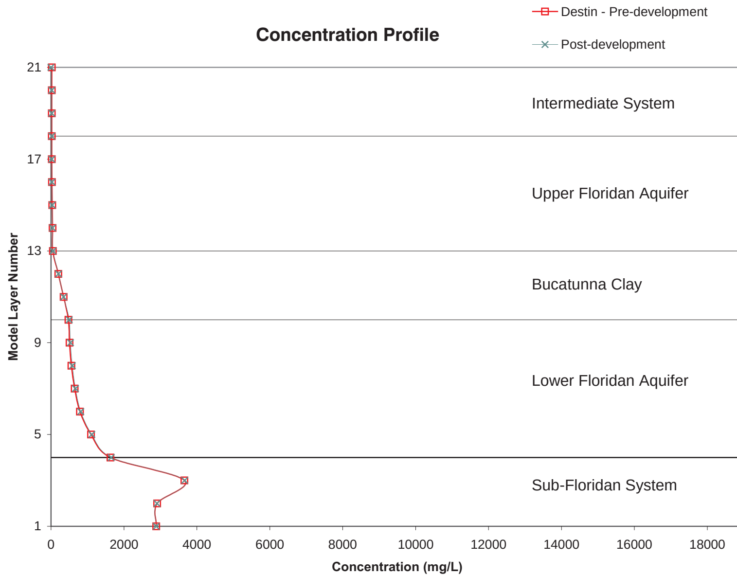
Figure 4.53 Concentration Profiles at Destin for Pre-Development and 2004 Simulations
