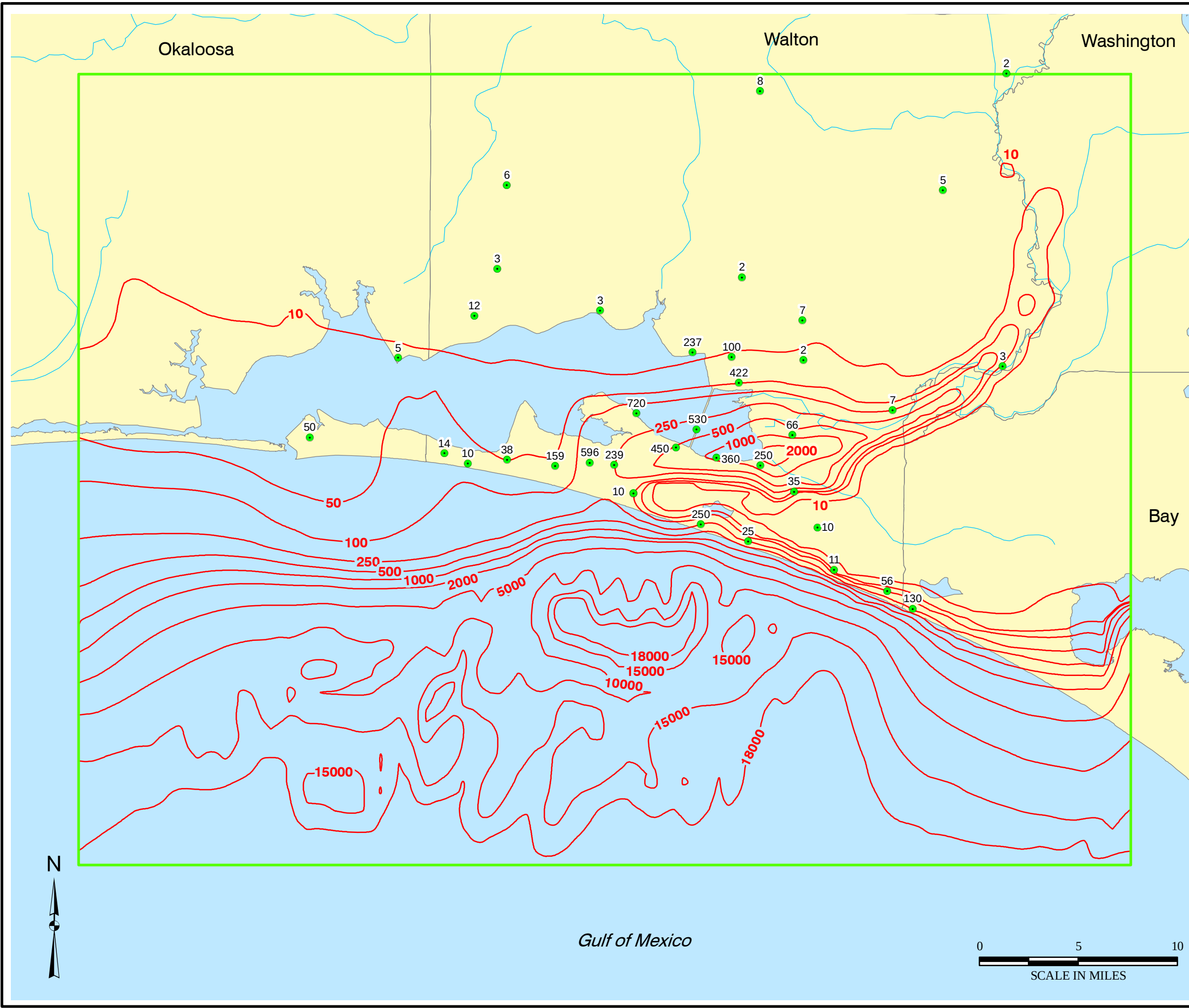
Figure 4.51d Simulated Concentration Contours vs. Observed Chloride Concentrations in the Upper Floridan Aquifer (or the Upper Portion of the Undifferentiated Floridan Aquifer) 1951 – 2003
