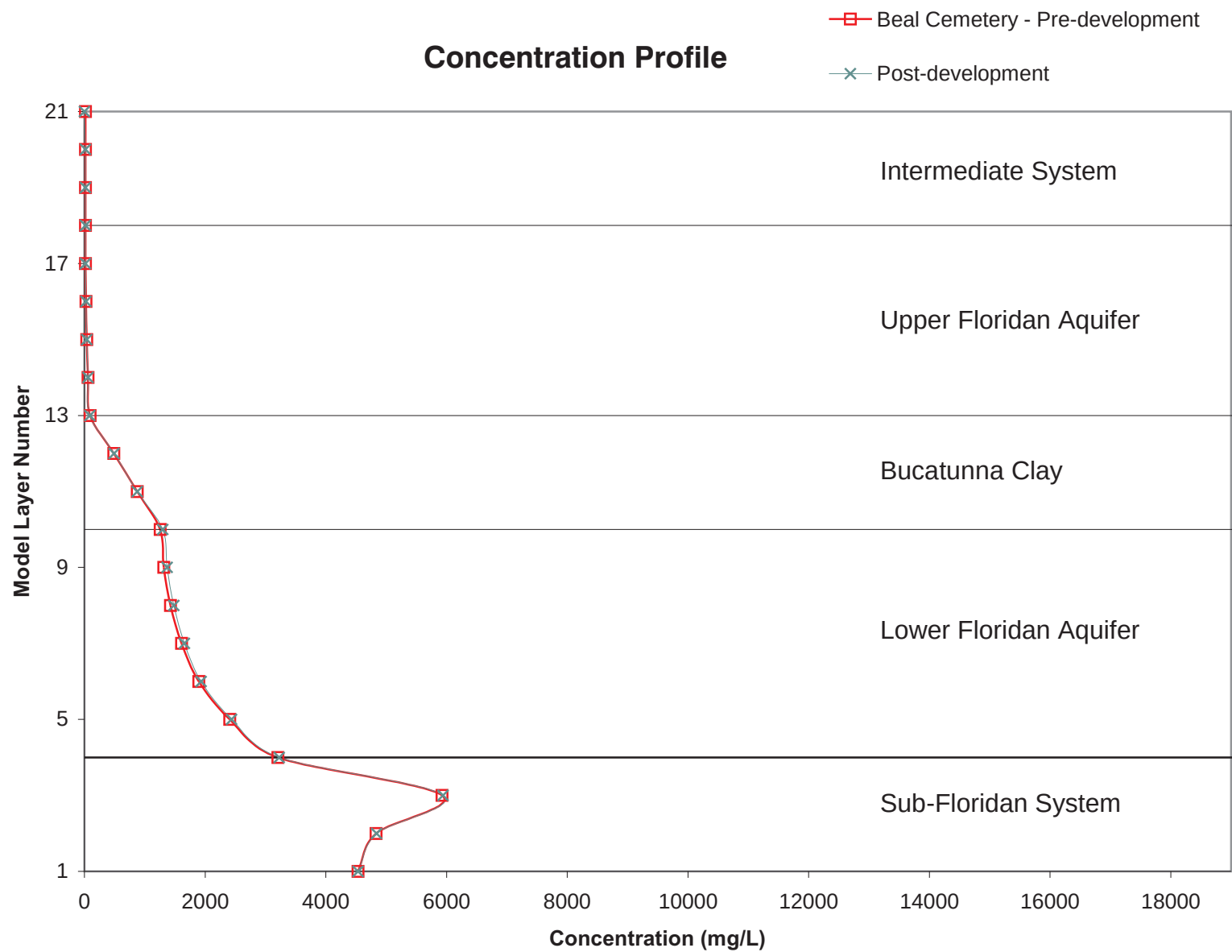
Figure 4.55 Concentration Profiles at Beal Cemetery for Pre-Development and 2004 Simulations
