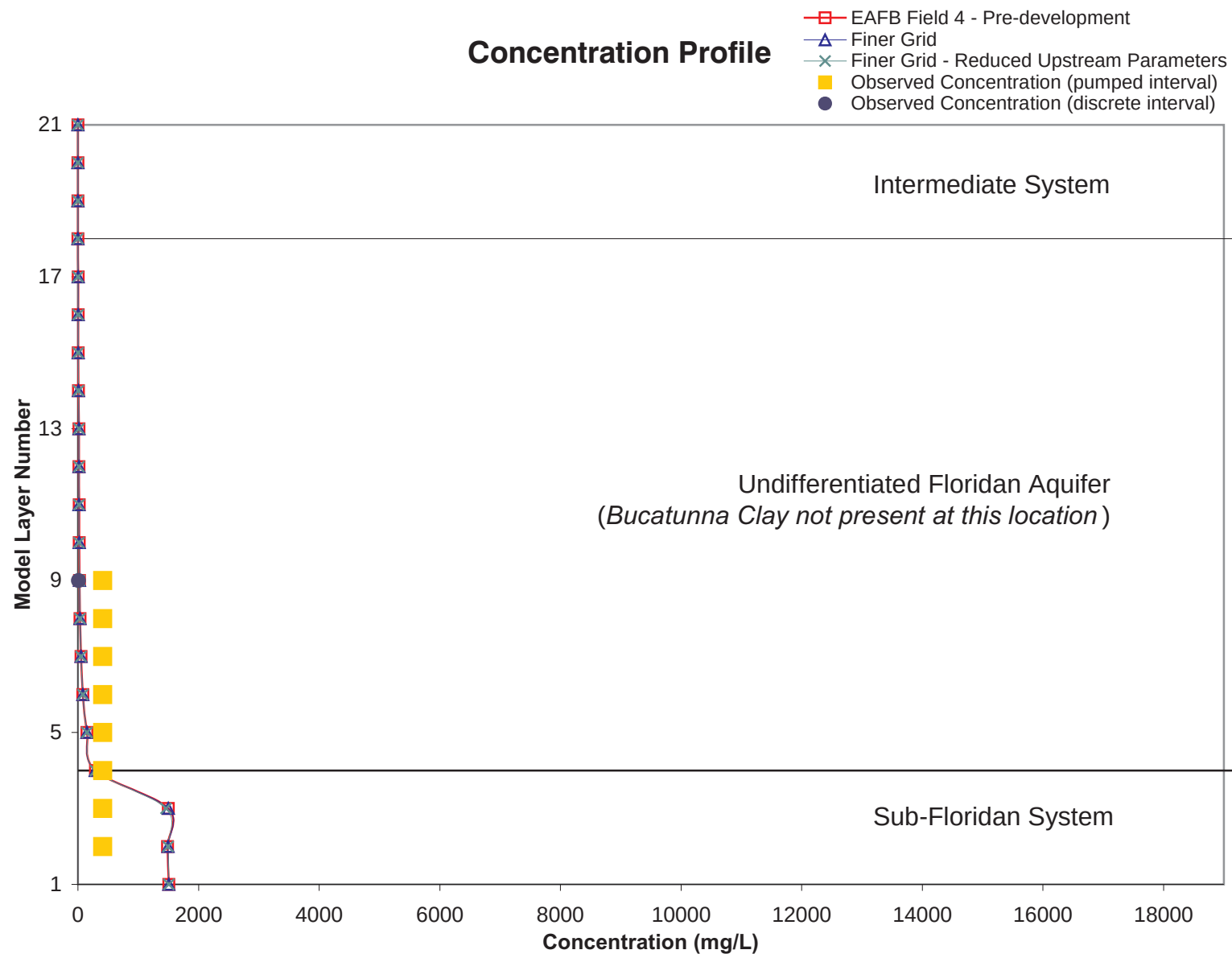
Figure 4.29 Concentration Profiles at EAFB Field 4 for Pre-Development and Grid Sensitivity Simulations
