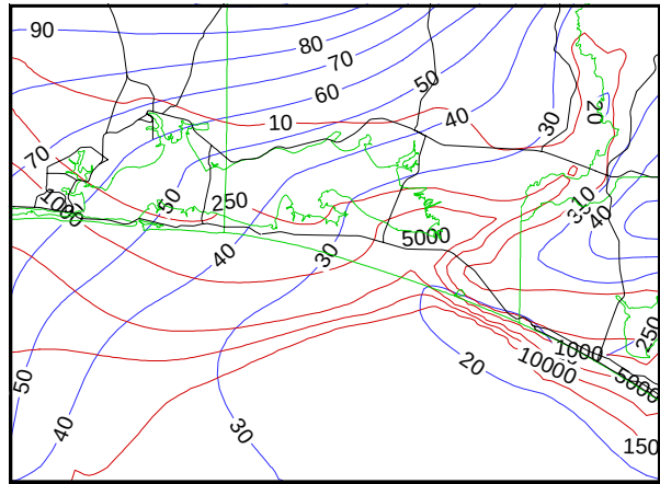
LOWER FLORIDAN AQUIFER
