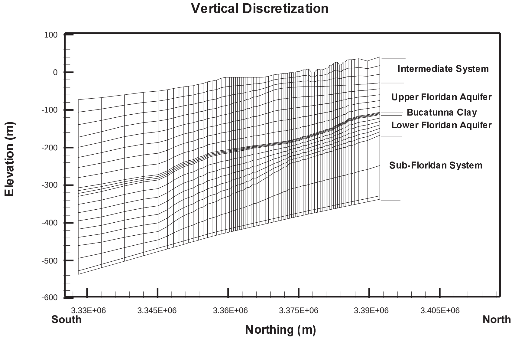
Figure 3.3 Vertical Discretization Along y-z Cross-Section at x=569764m
