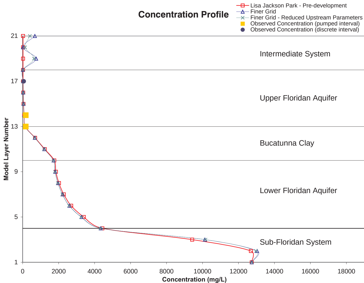
Figure 4.26 Concentration Profiles at Lisa Jackson Park for Pre-Development and Grid Sensitivity Simulations
