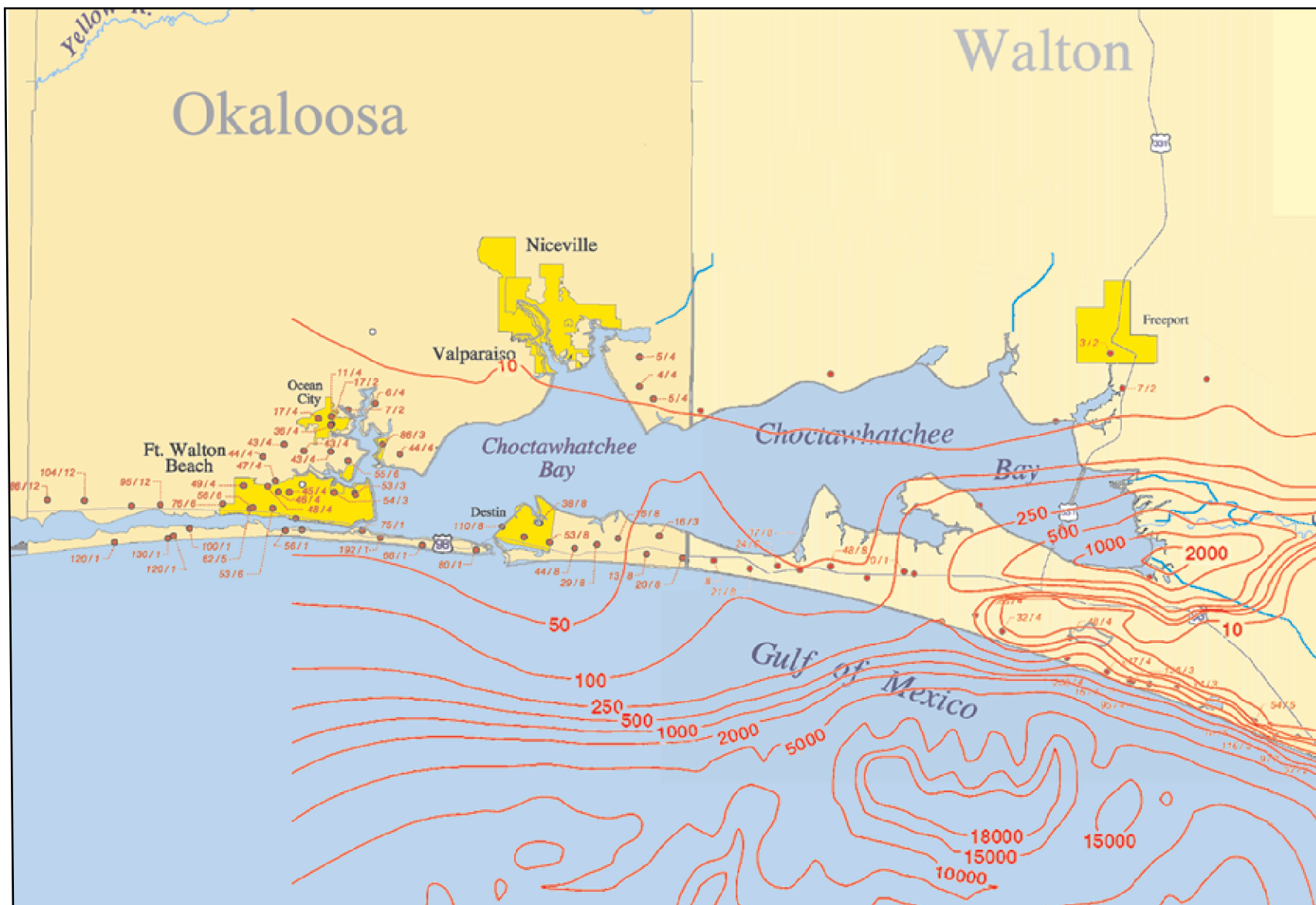
Figure 4.51c Simulated Concentration Contours vs. Mean Chloride Concentrations in the Upper Floridan Aquifer (or the Upper Portion of the Undifferentiated Floridan Aquifer) 1998 – 2000
