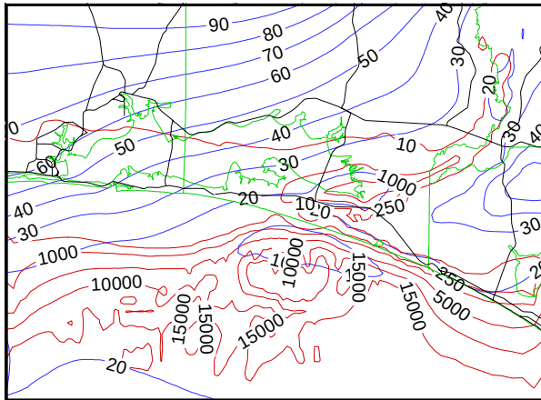
UPPER FLORIDAN AQUIFER
