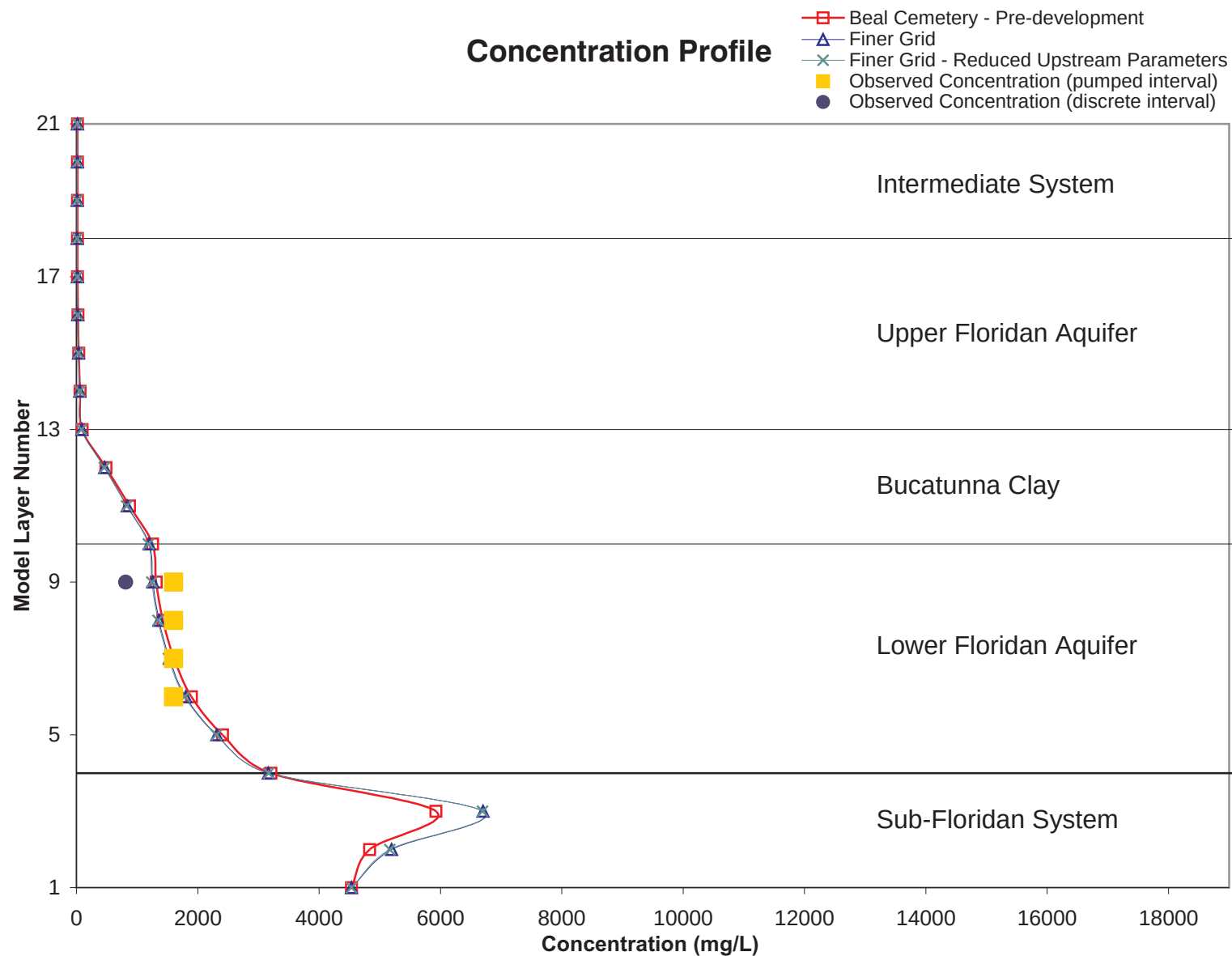
Figure 4.27 Concentration Profiles at Beal Cemetery for Pre-Development and Grid Sensitivity Simulations
