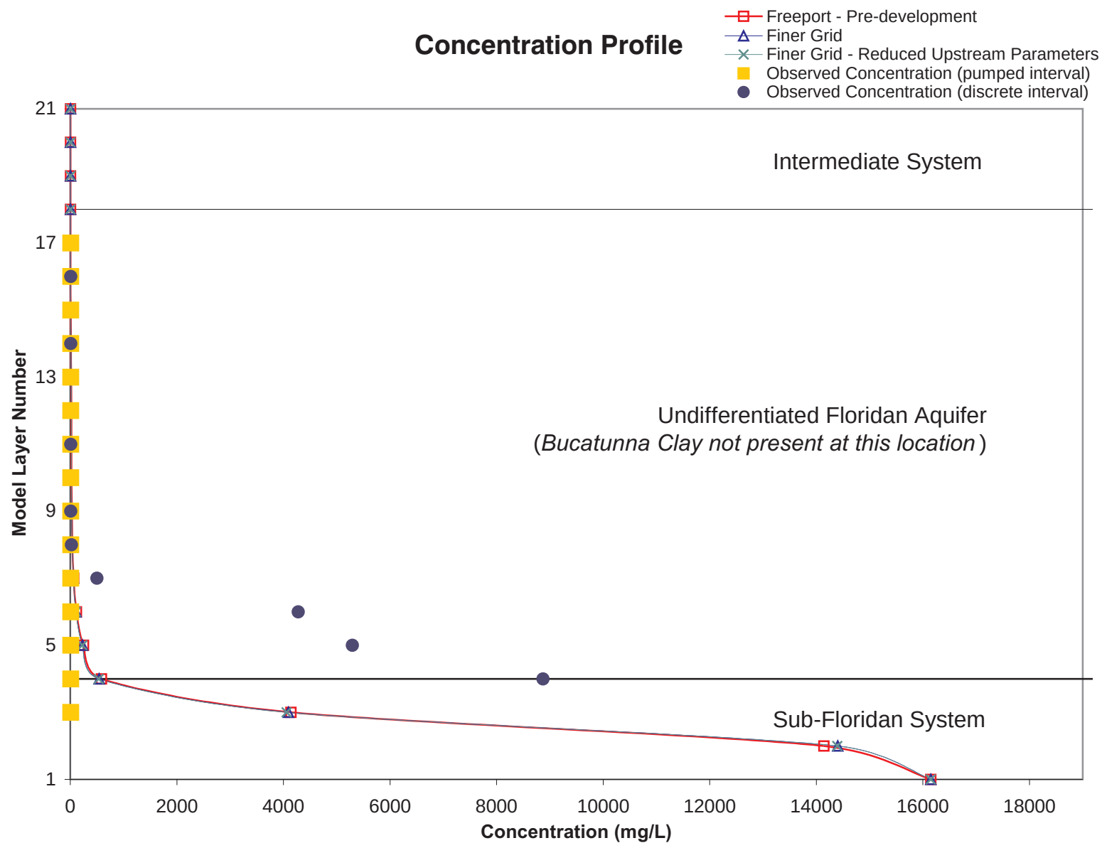
Figure 4.28 Concentration Profiles at Freeport for Pre-Development and Grid Sensitivity Simulations
