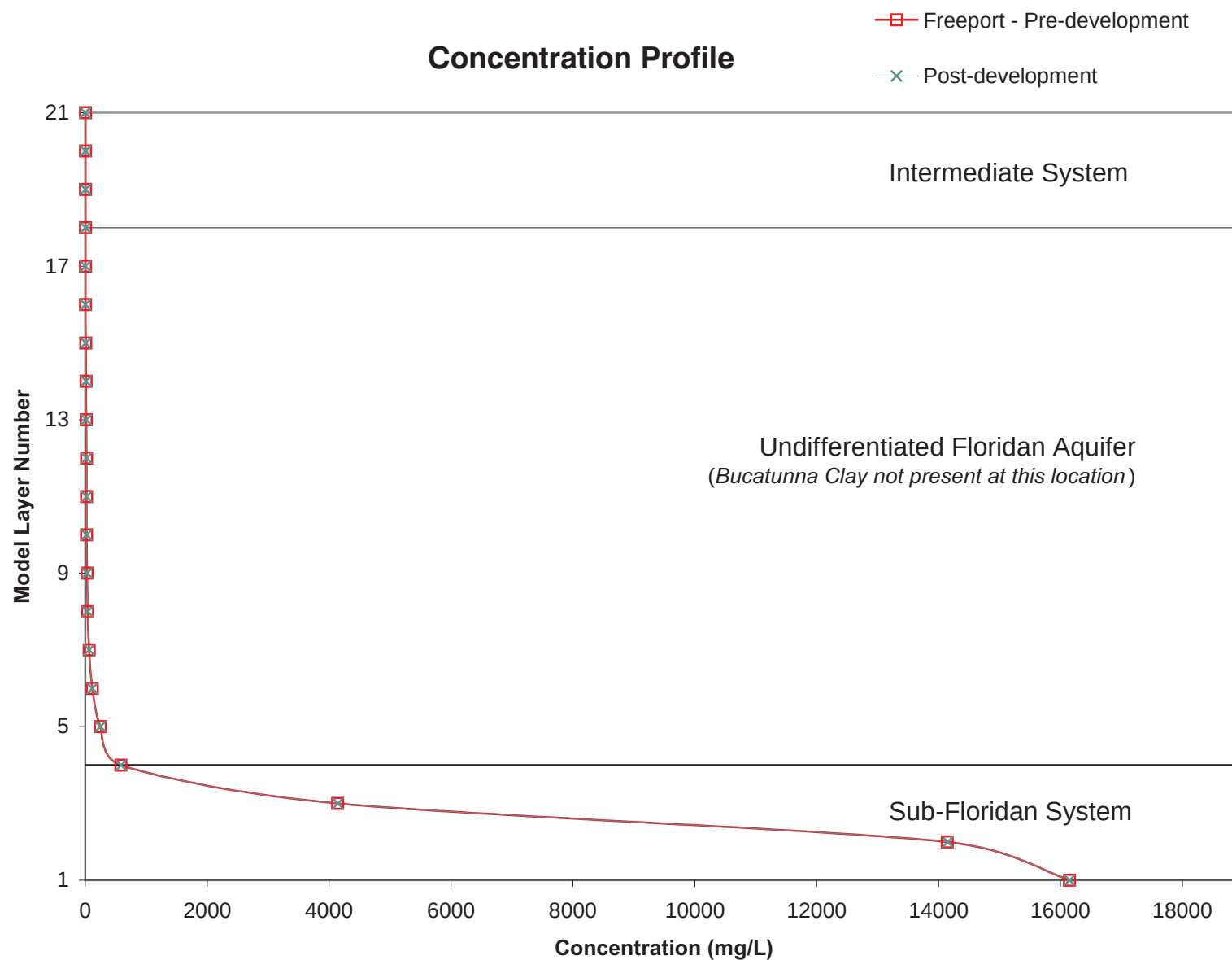
Figure 4.56 Concentration Profiles at Freeport for Pre-Development and 2004 Simulations
