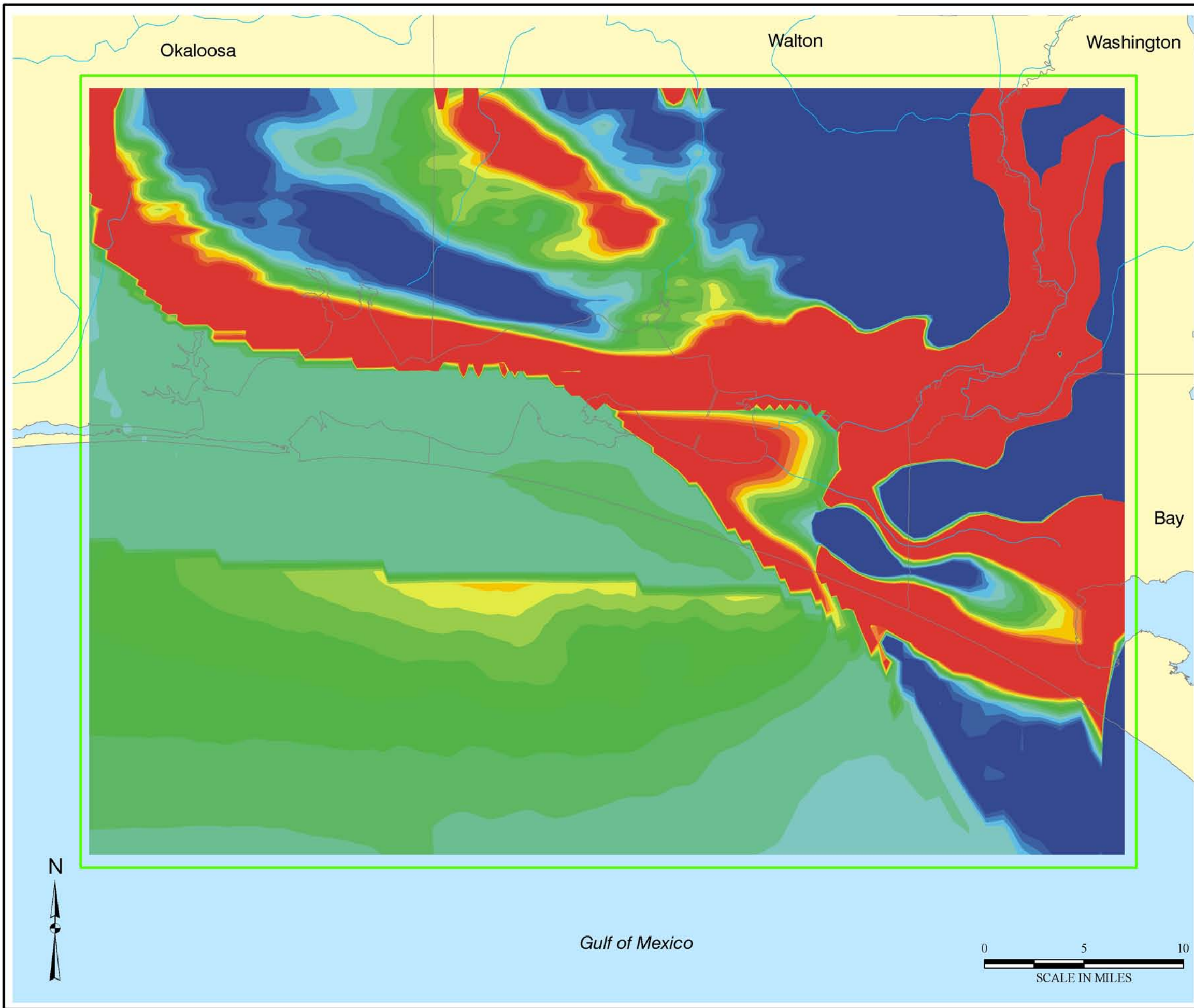
Figure 4.15 Pre-Development Vertical Darcy Velocities for the Bucatunna Clay Confining Unit and Middle Portion of the Undifferentiated Floridan Aquifer System (Elemental Layer 11)
