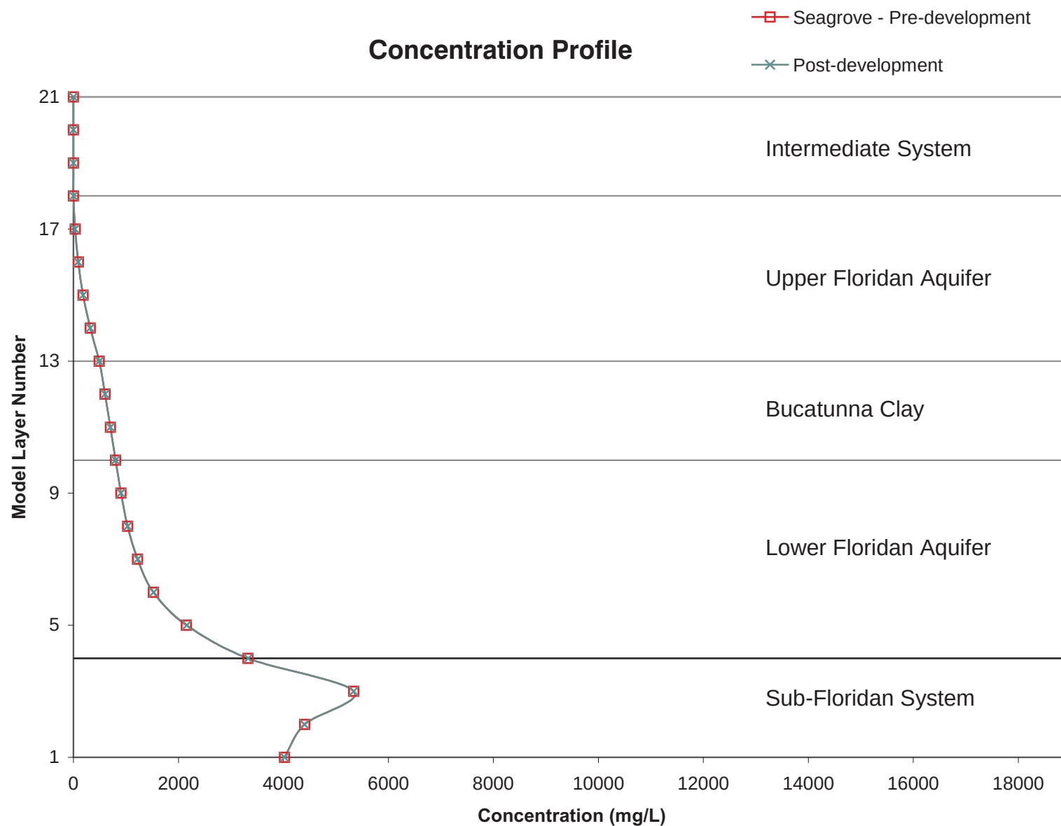
Figure 4.52 Concentration Profiles at Seagrove for Pre-Development and 2004 Simulations
