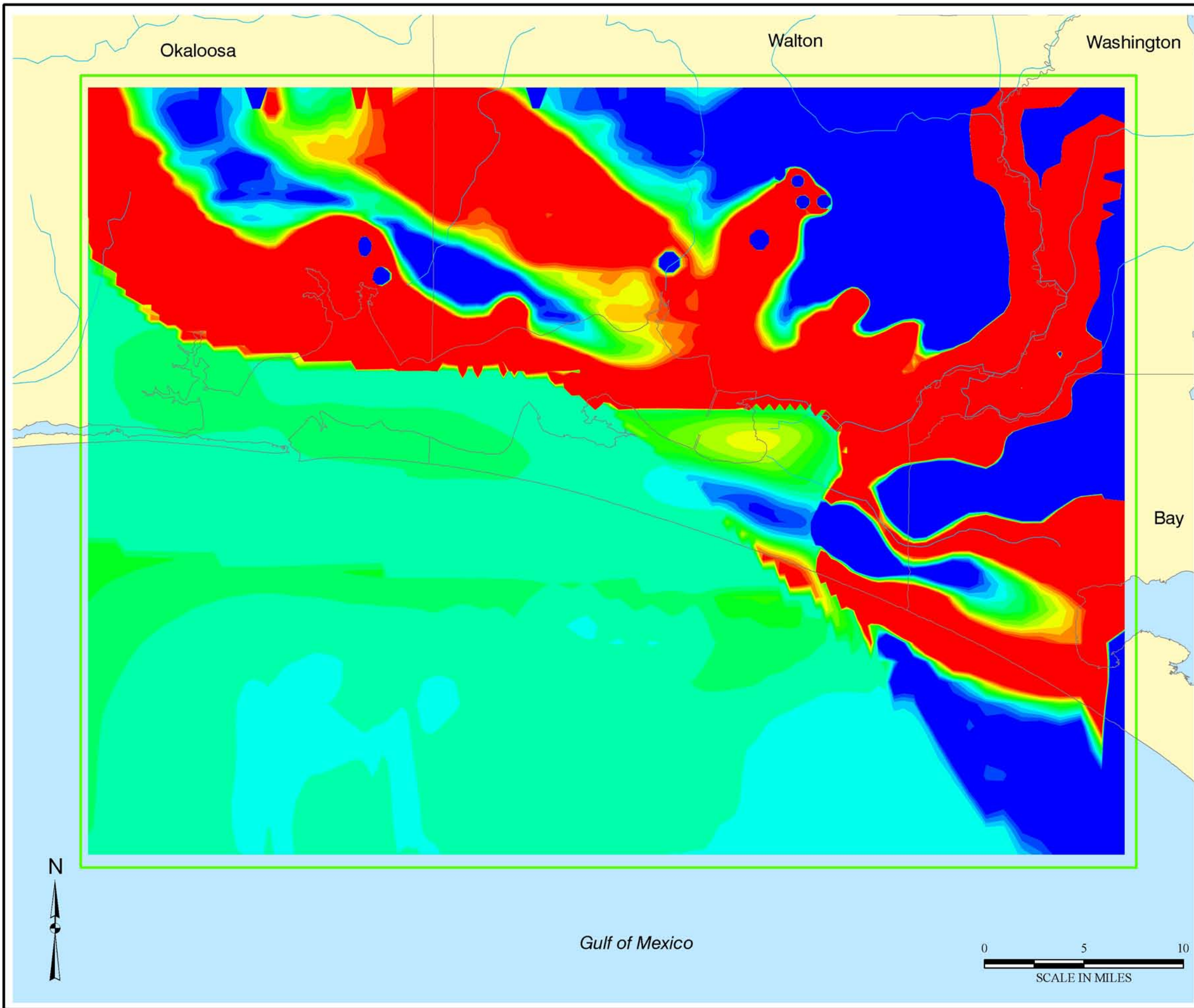
Figure 4.39 2004 Vertical Darcy Velocities for the Bucatunna Clay Confining Unit and Middle Portion of the Undifferentiated Floridan Aquifer System (Elemental Layer 11)
