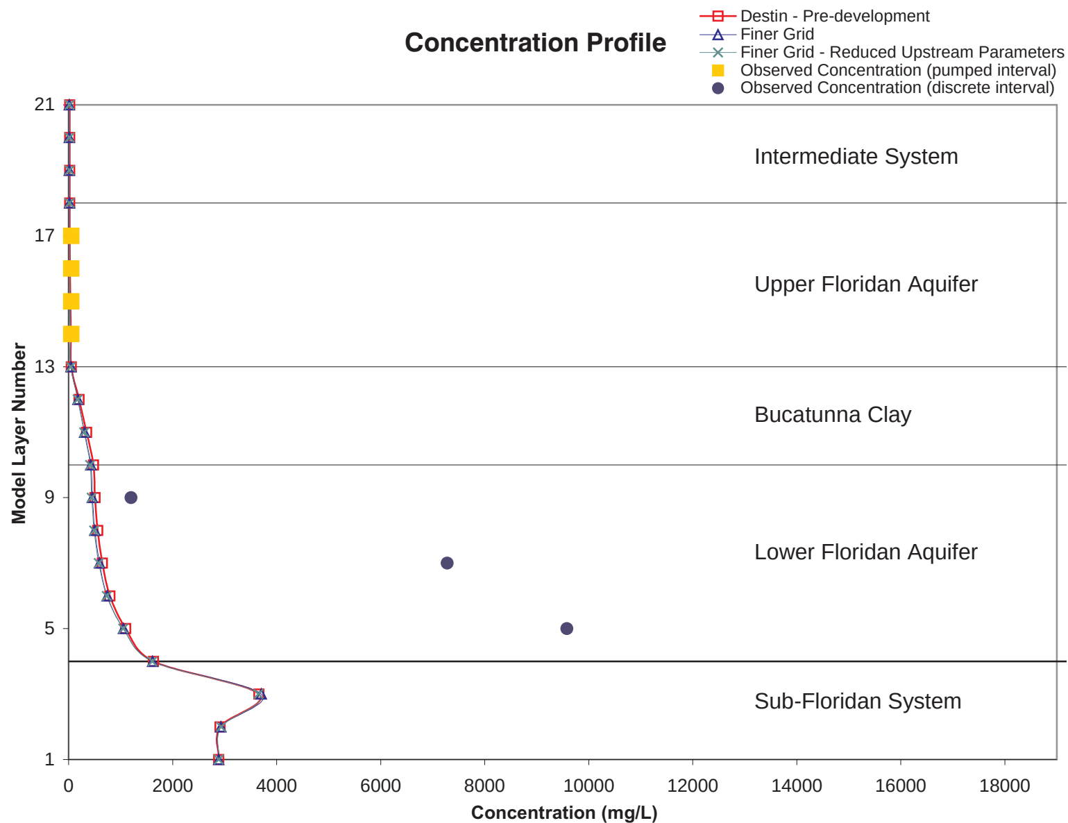
Figure 4.25 Concentration Profiles at Destin for Pre-Development and Grid Sensitivity Simulations
