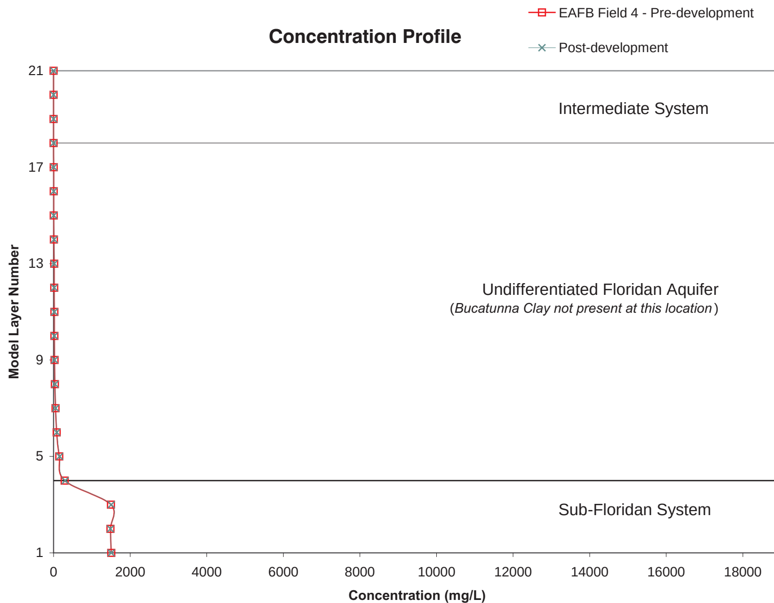
Figure 4.57 Concentration Profiles at EAFB Field 4 for Pre-Development and 2004 Simulations
