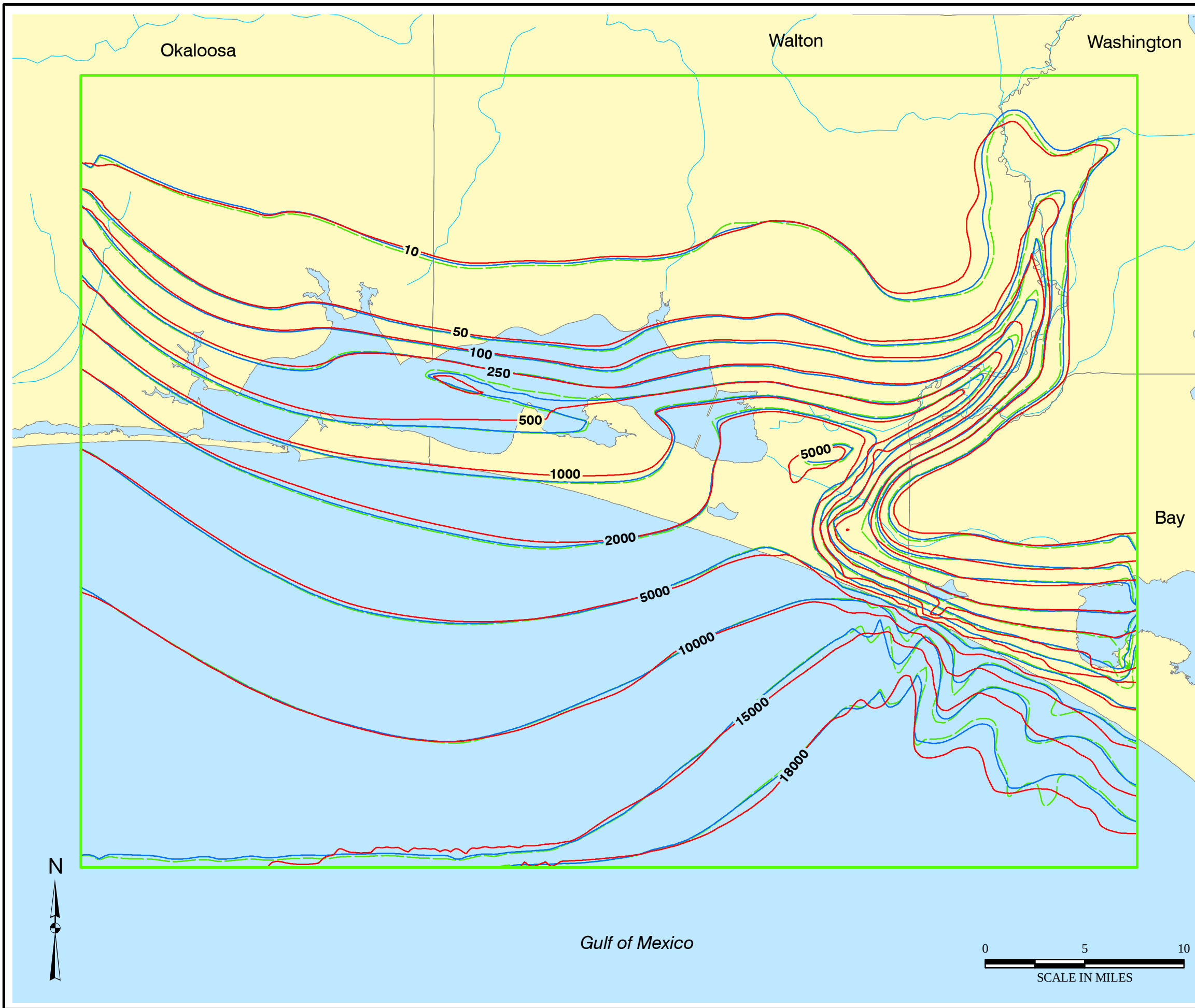
Figure 4.23 Pre-Development Chloride Concentrations for the Lower Floridan Aquifer Grid Sensitivities (Nodal Layer 7, mid-aquifer)
