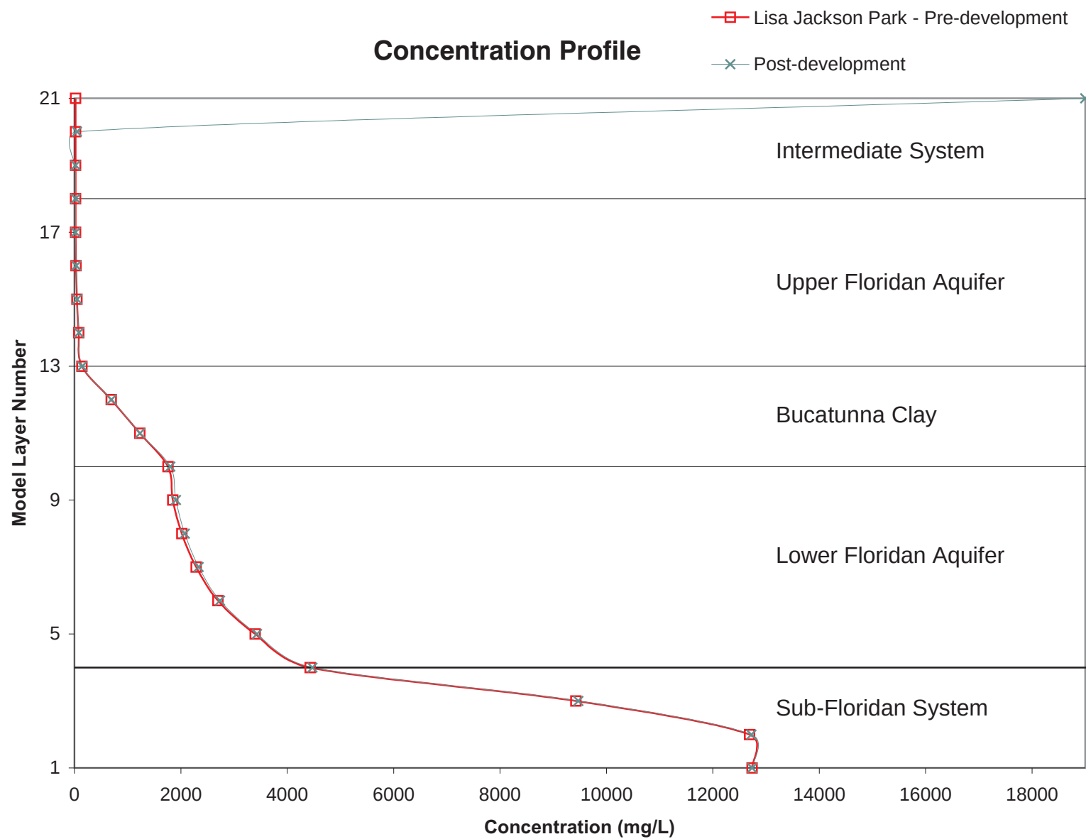
Figure 4.54 Concentration Profiles at Lisa Jackson Park for Pre-Development and 2004 Simulations
