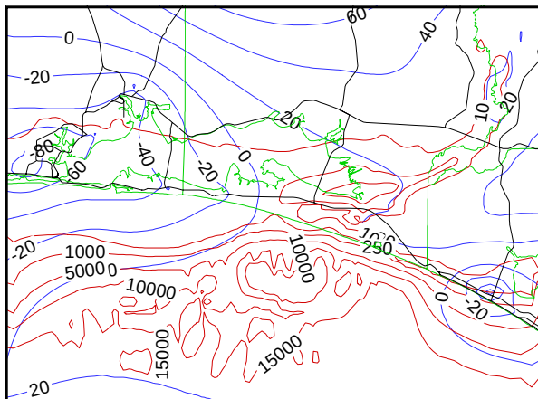
UPPER FLORIDAN AQUIFER
