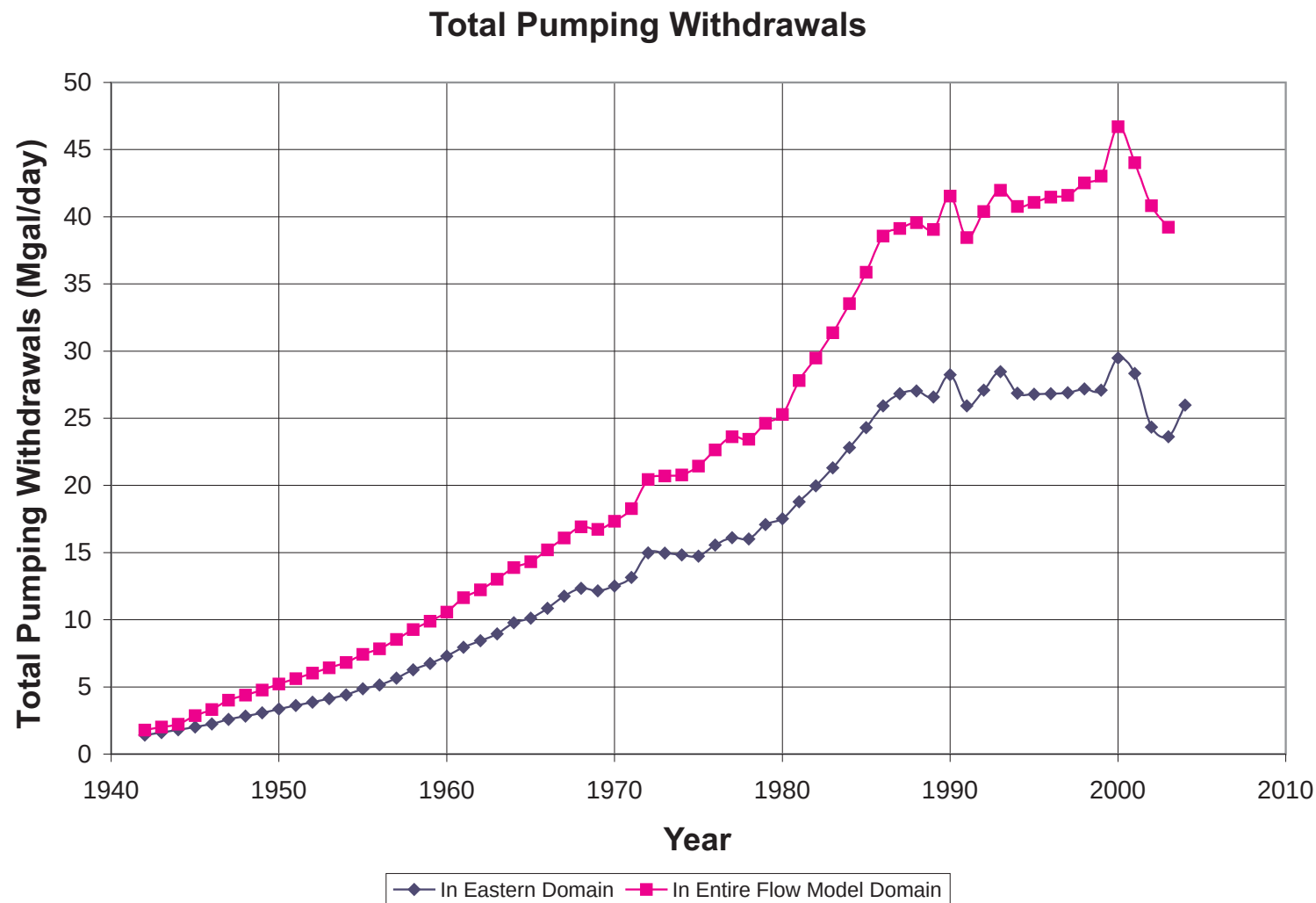
Figure 4.30 Total Withdrawals Applied to the Post-development Simulations in the Eastern Model Domain and the Entire Flow Model Domain
