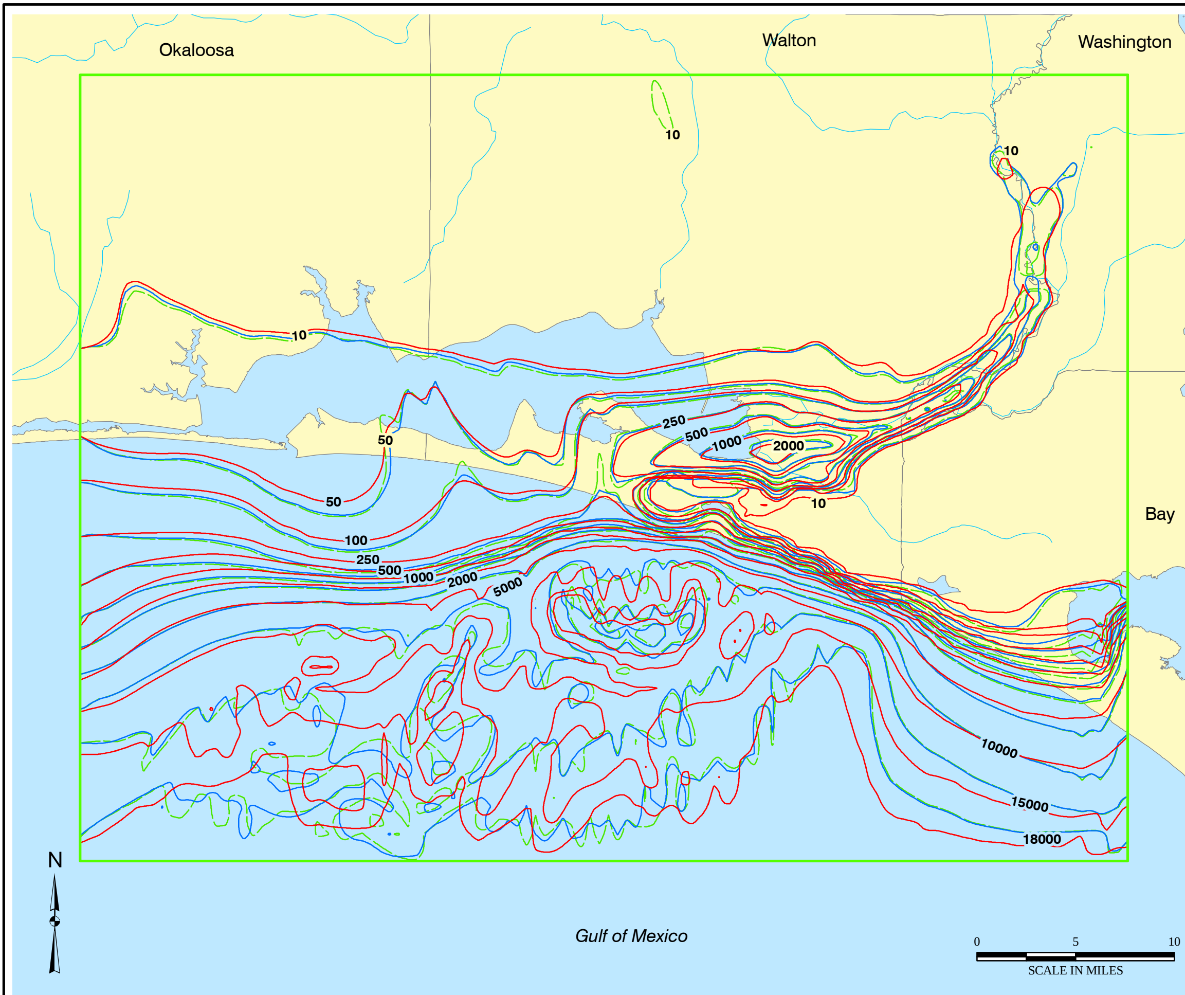
Figure 4.22 Pre-Development Chloride Concentrations for the Upper Floridan Aquifer Grid Sensitivities (Nodal Layer 16, mid-aquifer)
