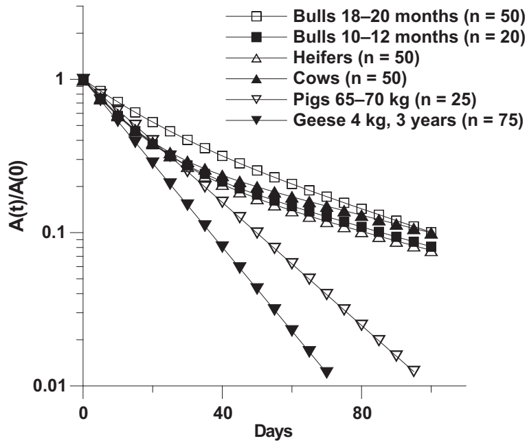
FIG. 4. Change with time in 137 Cs activity concentrations in muscle of various livestock ( A ( t )) normalized to initial concentration ( A (0)) [158, 159].
