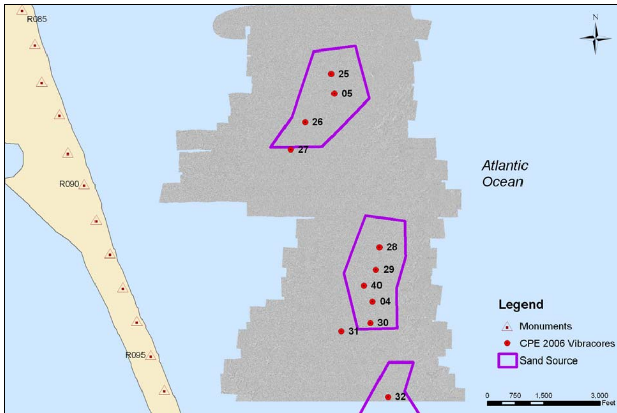
Figure 22. Geo-referenced sidescan mosaic, nearshore study area
