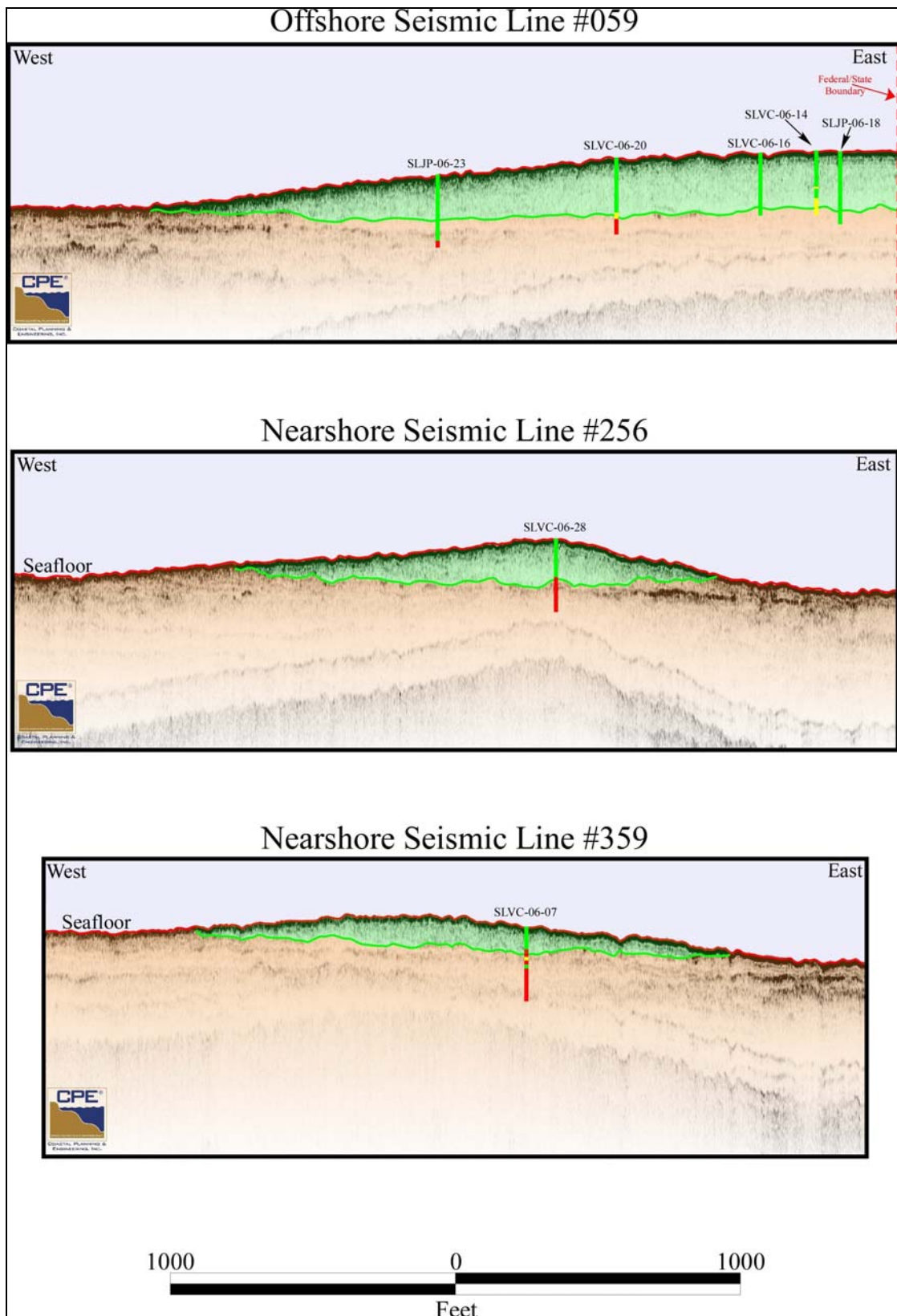
Figure 14. Seismic images showing correlation between seismic reflectors and vibracores layers. The thickness of the clean sand deposits correlate with sand ridge relief, but deposit thickness decreases away from ridge crests. The location of the seismic lines in plan view is shown in Figure 13.
