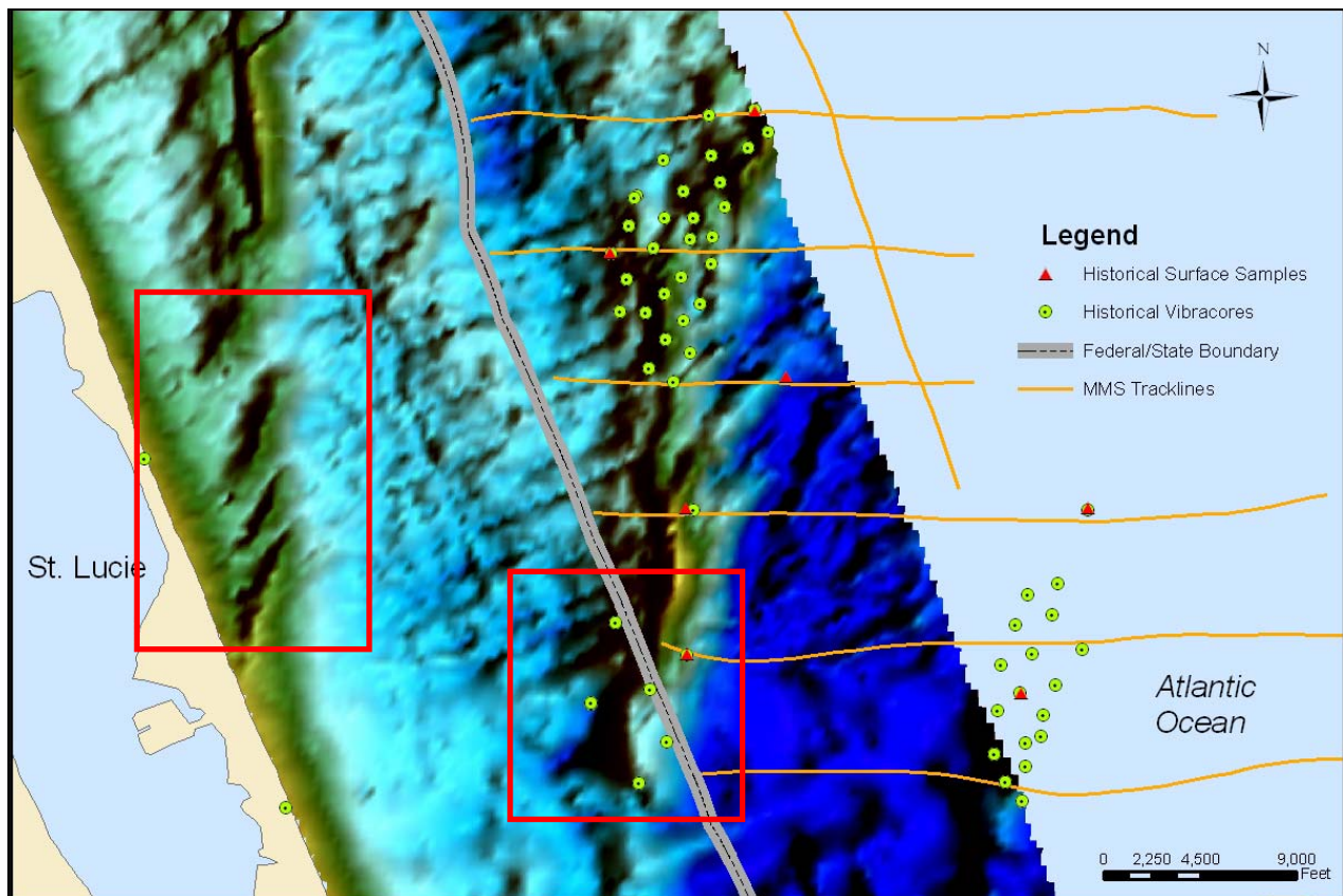
Figure 10. Location of historic geotechnical and geophysical data overlaid on top of a 3D bathymetric model created using NOAA-GEODAS bathymetry data. Sand ridge features identified offshore of the project area (see red rectangles) were selected for reconnaissance investigations.
