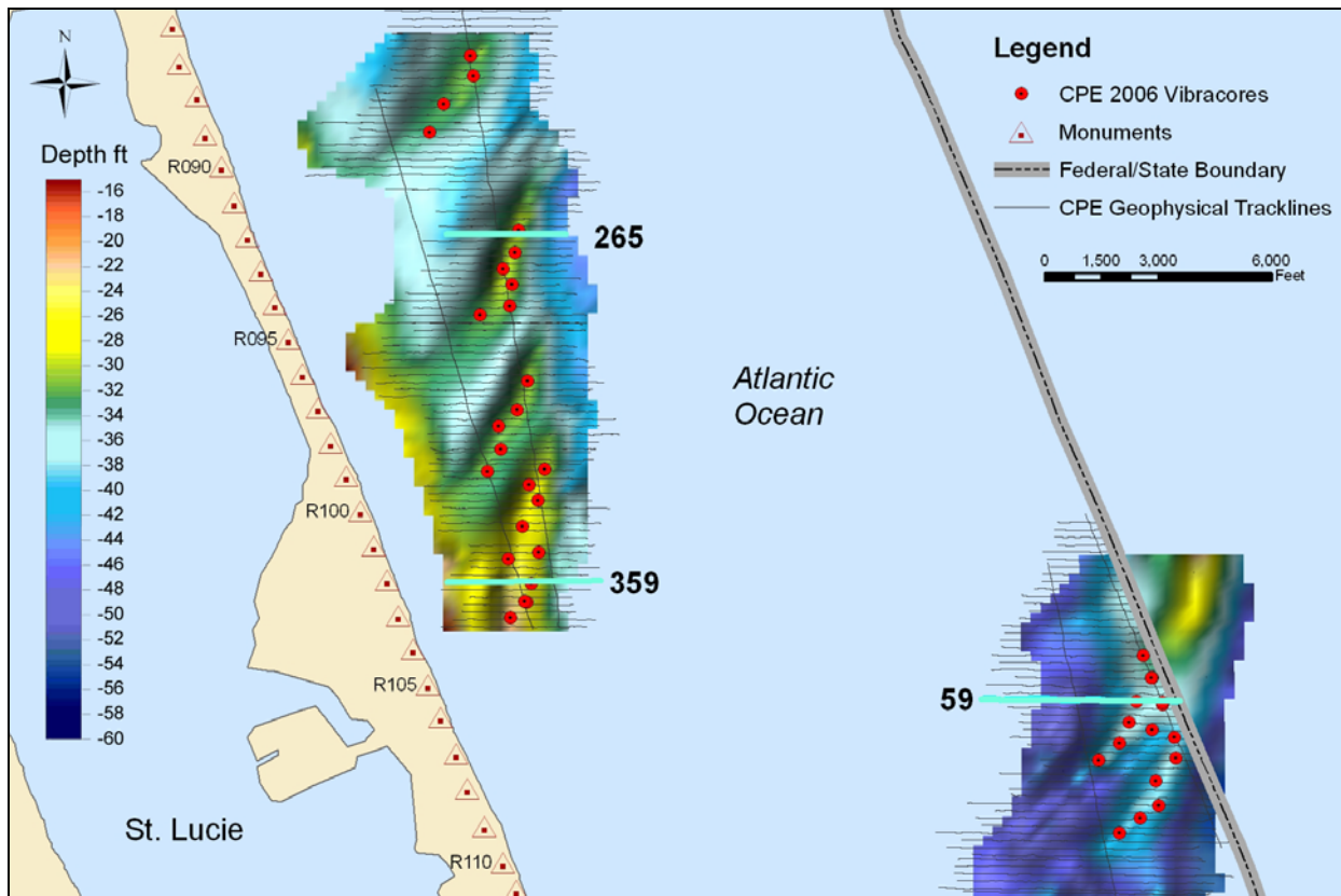
Figure 13. Location of seismic tracklines, vibracores and selected seismic cross-sections shown in Figures 9 and 10. Cross-sectional seismic profiles for the highlighted blue tracklines are shown in Figure 14.
