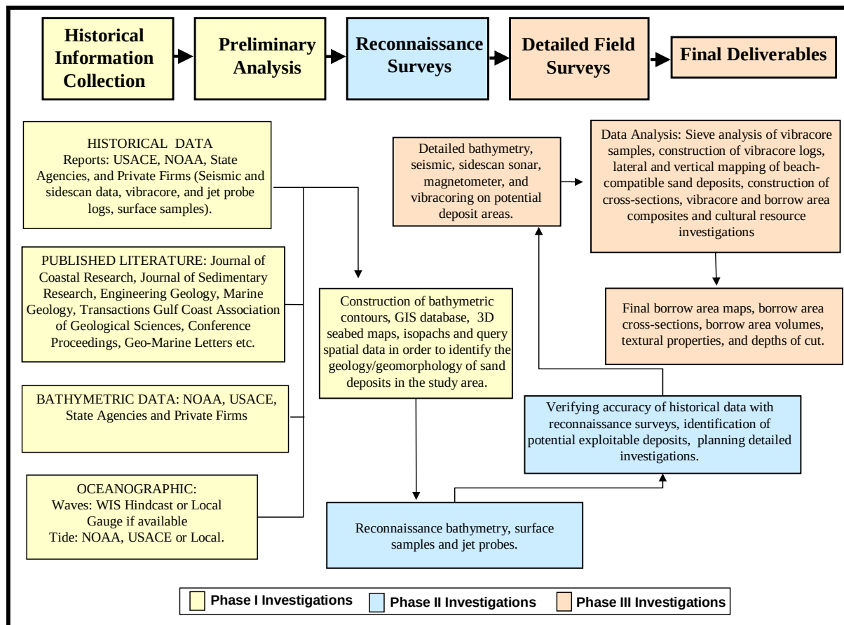
Figure 9. This flow diagram summarizes the main phases of sand searches that are comprised by strategic geotechnical and geophysical studies.
