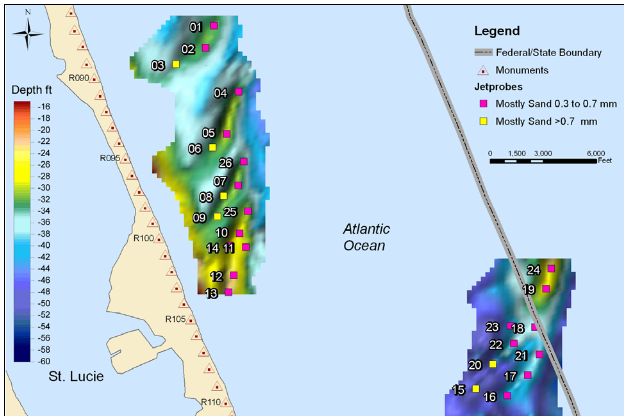
Figure 12. Location of CPE jet probes on top of bathymetric image. Jet probes are classified based on grain size intervals indicated in the legend.
