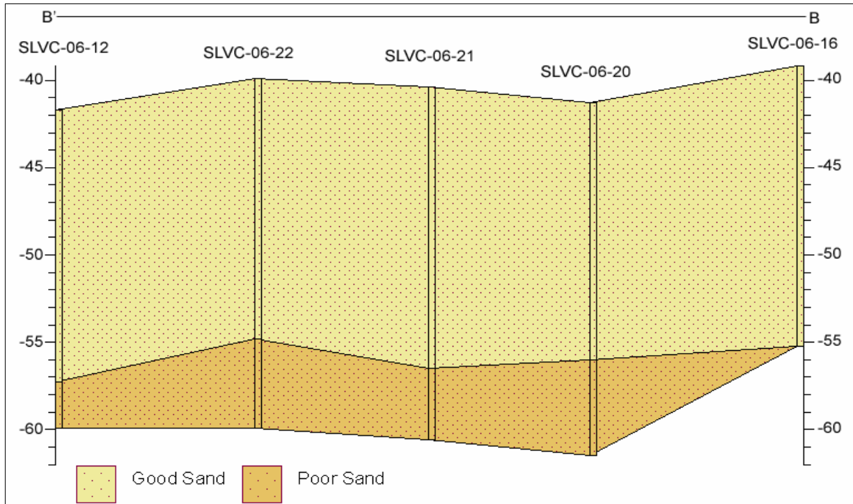
Figure 18. Schematic cross section based on interpretation of vibracore data (see Figure 17 for location). Sediments in the vibracores were divided into two main categories: (1) good sand, (2) poor sand, and (3) clay. The “good sand” layer contains clean sandy sediments (fine to medium sand less than 5% silt, generally less than 5% shell, moderately to moderately well sorted). “Poor sands” contain sandy layers mixed with more than 5% fines (silt or clay) and shell/rock fragments.
