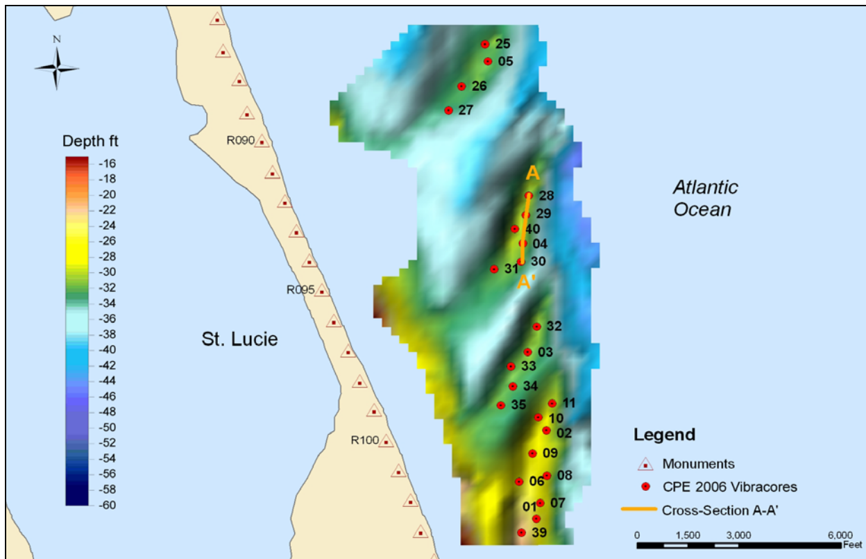
Figure 15. Zoom view of the nearshore study area showing vibracores and location of vibracore cross-section A-A' (Figure 16).
