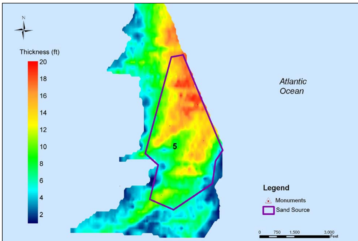
Figure 21. Sediment isopachs for the offshore sand-source. Sediment thickness increases to the NE, towards the main ridge crest. This study area is the terminus (W-SW corner) of a very large sediment ridge that lies seaward of the study area (to the E-NE) (see Figure 10). Only the corner of the ridge was surveyed because the seaward section lies in Federal waters under MMS jurisdiction. It is anticipated, however, that the seaward continuation of this sand body represents a significant sand reserve for future renourishments in St. Lucie County.
