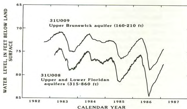
Figure 10.--Daily mean water levels in the upper Brunswick and Upper and Lower Floridan aquifers, Hopeulikit site, Bulloch County, 1983-87.
