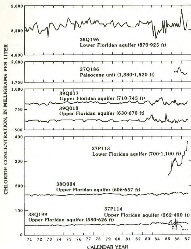
Figure 22.--Chloride concentration in the Upper and Lower Floridan aquifers and the Paleocene unit in the Savannah area, 1971-87.
