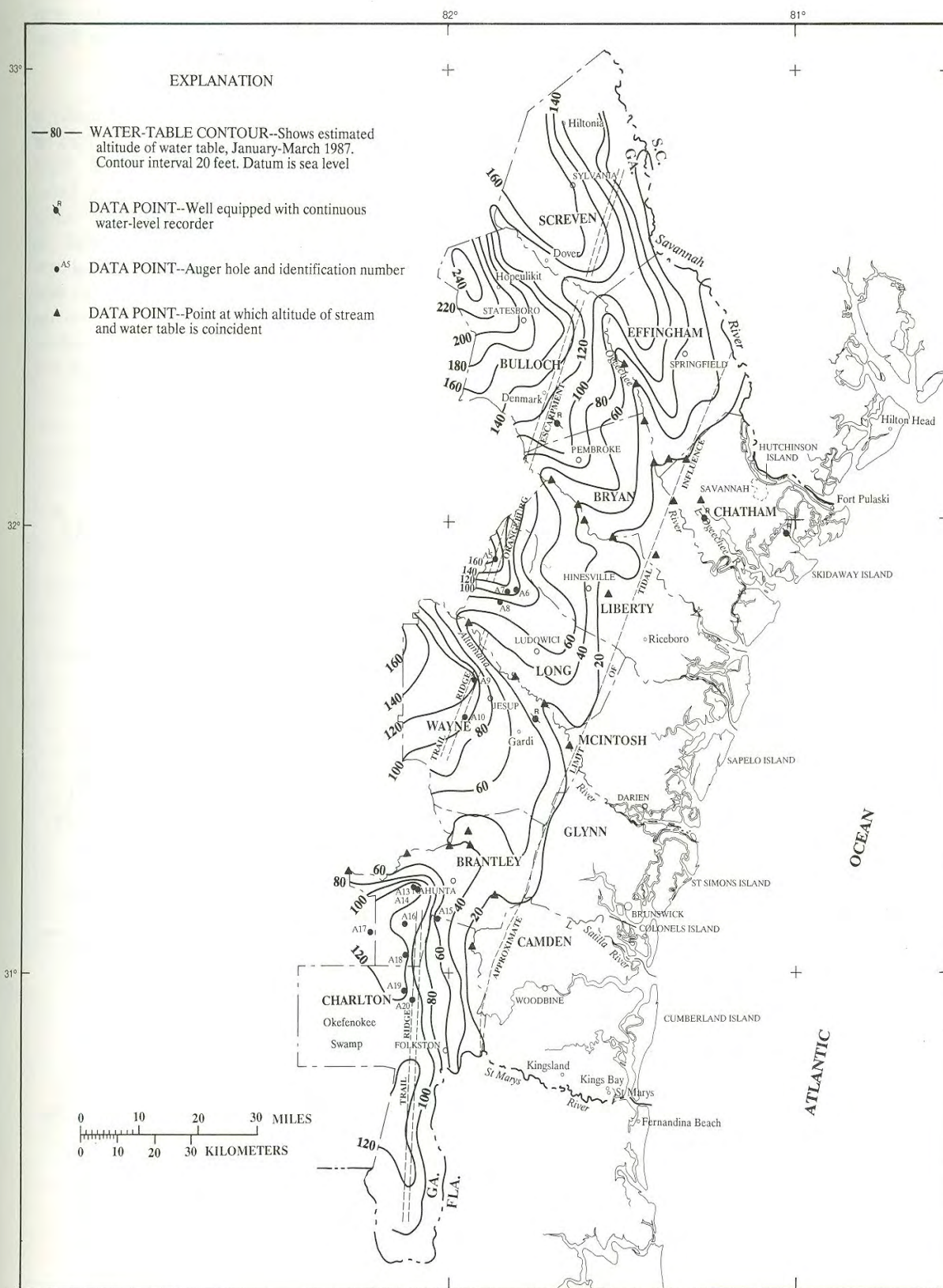
Figure 4.--Estimated water-table surface of the surficial aquifer in the coastal area.
