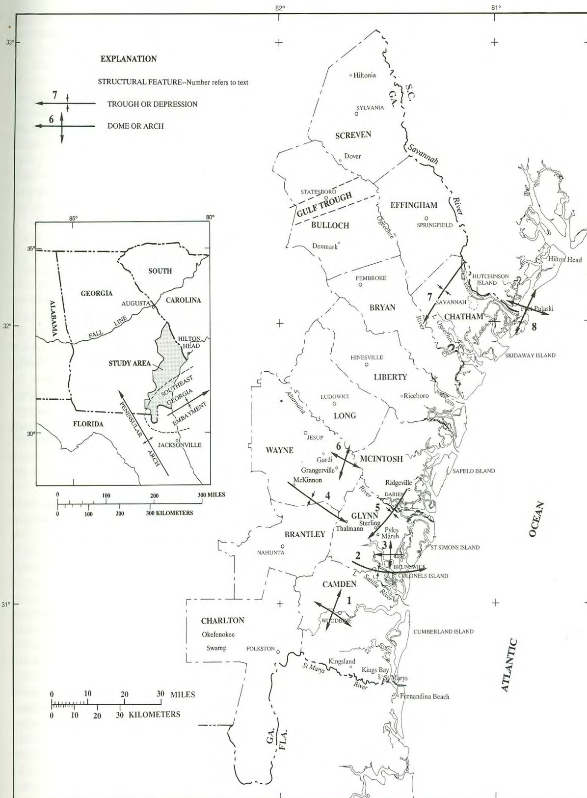
Figure 2.--Structural features in the coastal area of Georgia and adjacent parts of Florida and South Carolina.
