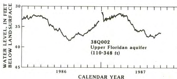
Figure 16.--Daily mean water levels in the Upper Floridan aquifer at well 38Q002 and in the Paleocene unit and late Cretaceous-age rocks at well 38Q201, Fort Pulaski, Chatham County, 1986-87.
