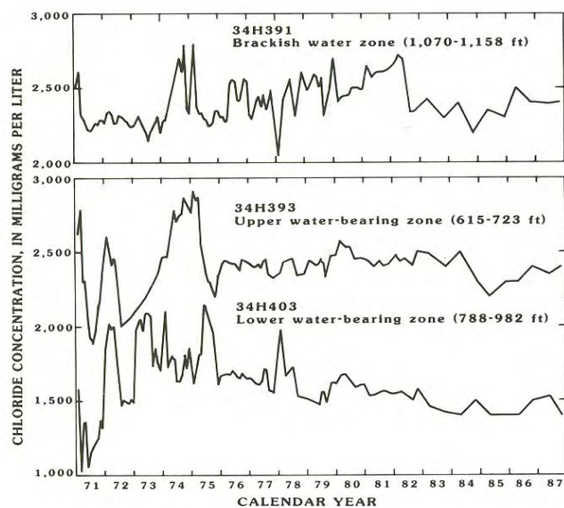
Figure 24.--Chloride concentration in the brackish-water zone of the Lower Floridan aquifer, and in the upper and lower water-bearing zones of the Upper Floridan aquifer in the Bay Street area of Brunswick, 1971-87.
