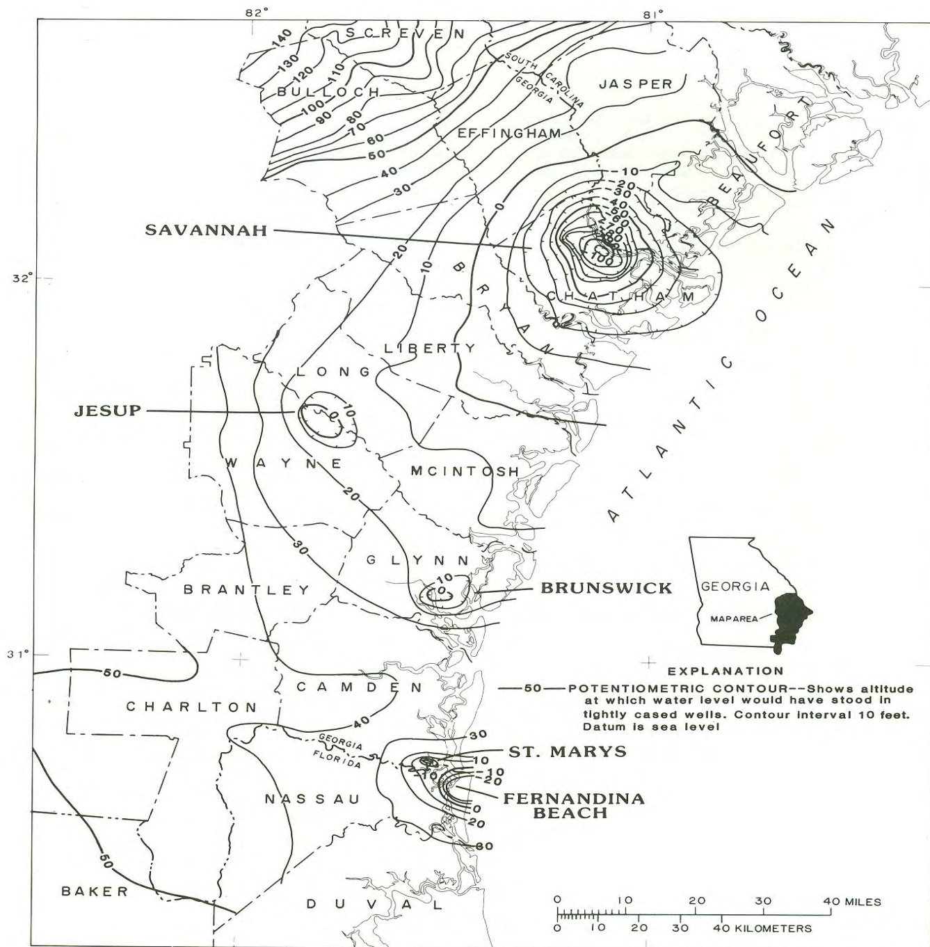
Figure 12.--Potentiometric surface of the Upper Floridan aquifer in the coastal area, May 1985.
