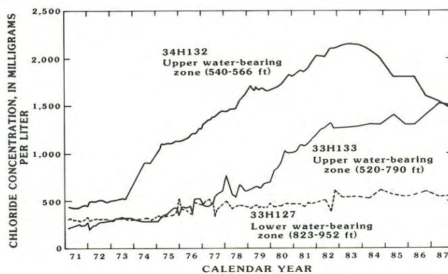
Figure 25.--Chloride concentration in the upper and lower water-bearing zones of the Upper Floridan aquifer in the north Brunswick area, 1971-87.
