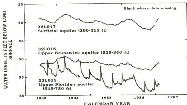
Figure 9.--Daily mean water levels in the surficial, upper Brunswick, and Upper Floridan aquifers at the Gardi site, Wayne County, 1983-87.
