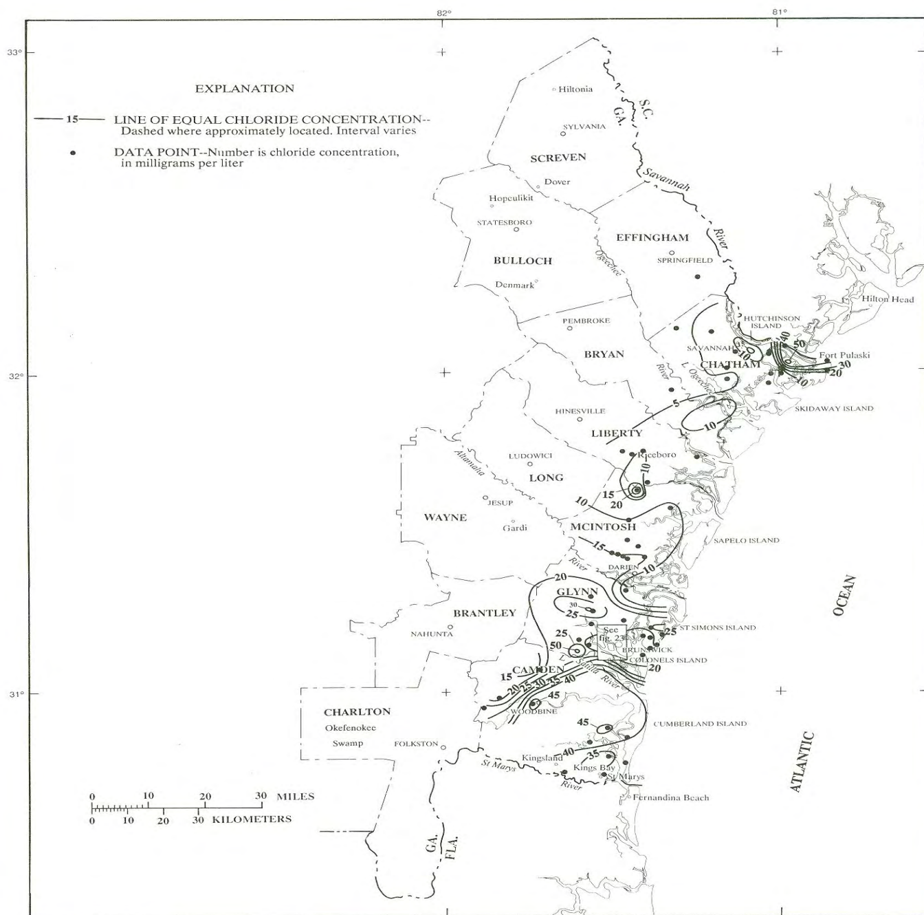
Figure 20.--Chloride concentrations in the Upper Floridan aquifer in the coastal area, October-November 1984.
