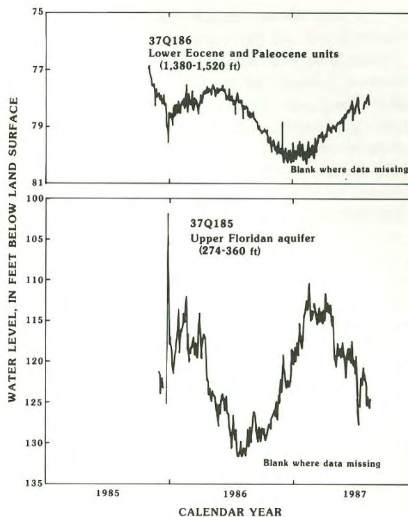
Figure 15.--Daily mean water levels in the Paleocene unit in well 37Q186 and in the Upper Floridan aquifer in well 37Q185, Hutchinson Island, Chatham County, 1985-87.
