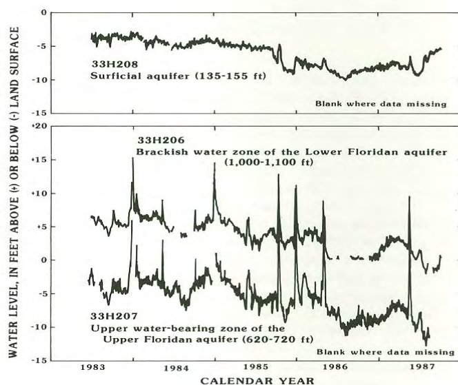
Figure 7.--Daily mean water levels in the surficial aquifer and the upper water-bearing zone and brackish-water zone of the Floridan aquifer system, Brunswick Pulp and Paper Company site, Glynn County, 1983-1987.
