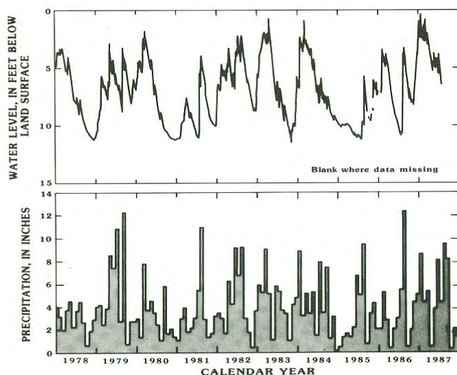
Figure 5.--Daily mean water levels in the surficial aquifer at well 35P094, and total monthly rainfall at National Weather Service Station, Savannah WSO AP Chatham County, 1978-87.
