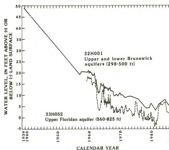
Figure 11.--Periodic water levels in the upper and lower Brunswick aquifers at well 32H001, and in the Upper Floridan aquifer at well 33H052, Glynn County, 1939-86.
