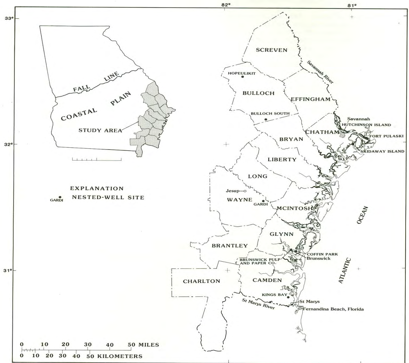
Figure 1.--Location of study area and nested-well sites.
