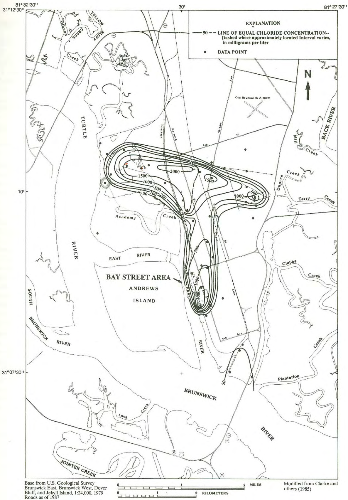
Figure 23.--Chloride concentrations in the upper water-bearing zone of the Upper Floridan aquifer in the Brunswick area, October-November 1984.
