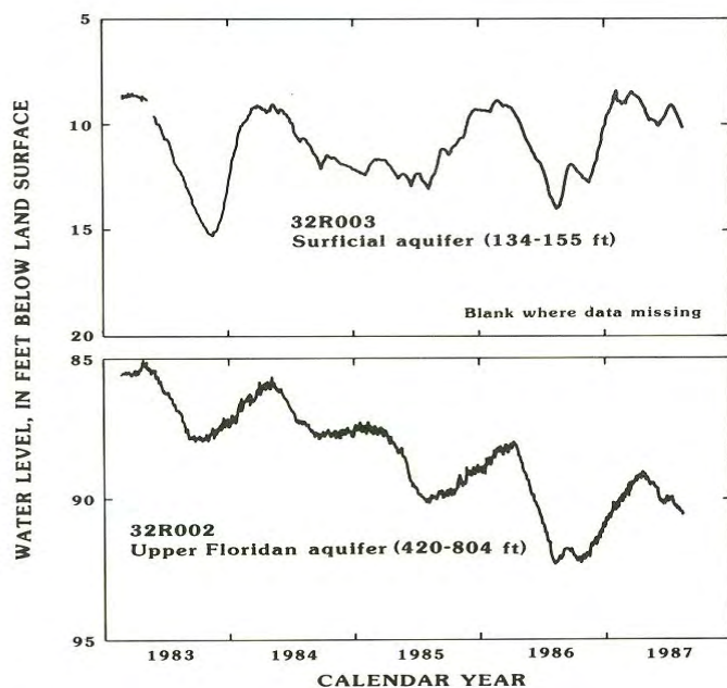
Figure 6.--Daily mean water levels in the surficial and Upper Floridan aquifers, Bulloch South site, Bulloch County, 1983-87.
