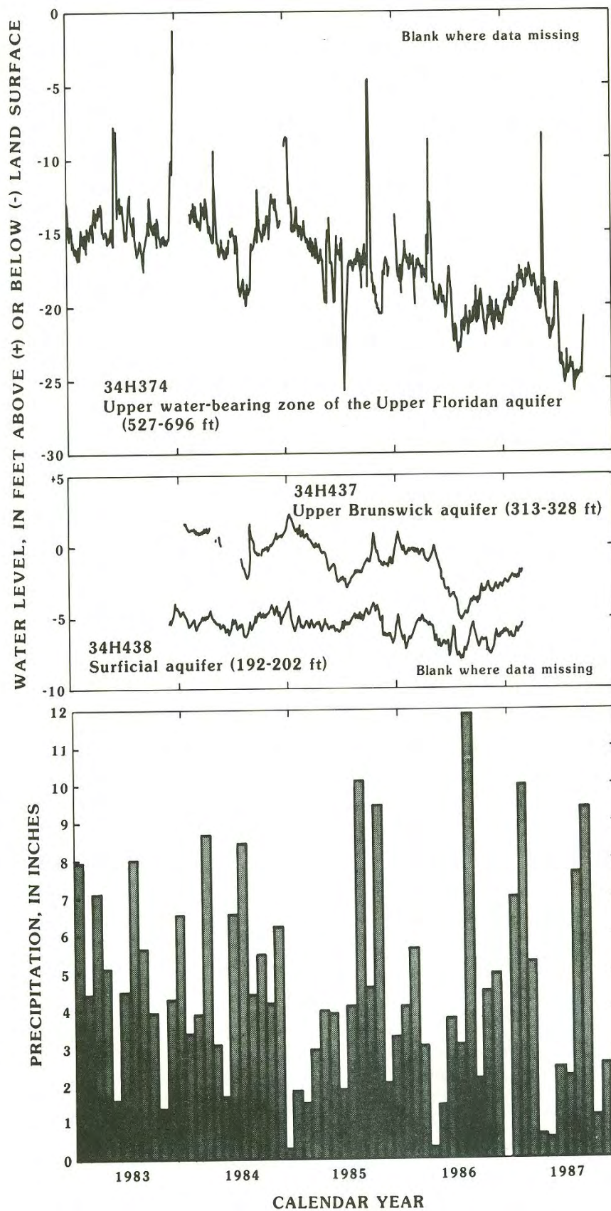
Figure 8.--Daily mean water levels in the upper water-bearing zone of the Upper Floridan aquifer and the surficial and upper Brunswick aquifers, Coffin Park site, and total monthly rainfall at the National Weather Service station at Brunswick, 1983-87.
