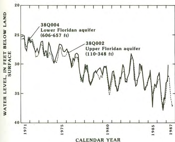
Figure 13.--Monthly mean water levels in the Upper Floridan aquifer at well 38Q002 and in the Lower Floridan aquifer at well 38Q004, Fort Pulaski, Chatham County, 1971-87.
