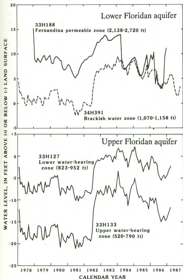
Figure 14.--Monthly mean water levels in the brackish-water zone and Fernandina permeable zone of the Lower Floridan aquifer, and in the upper and lower water-bearing zones of the Upper Floridan aquifer, Glynn County, 1978-87.
