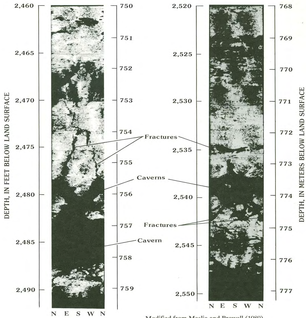
Figure 3.--Acoustic televiwer log at well 33H188, Colonels Island, Glynn County.
