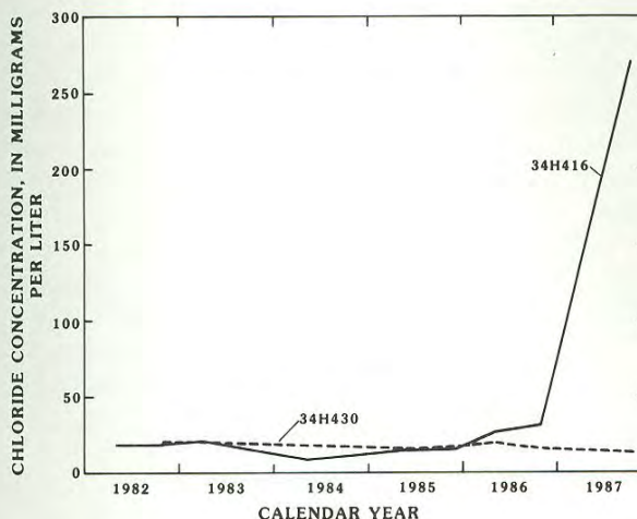
Figure 19.--Graph showing chloride concentration in the surficial aquifer at wells 34H416 and 34H430, Glynn County, 1982-87.
