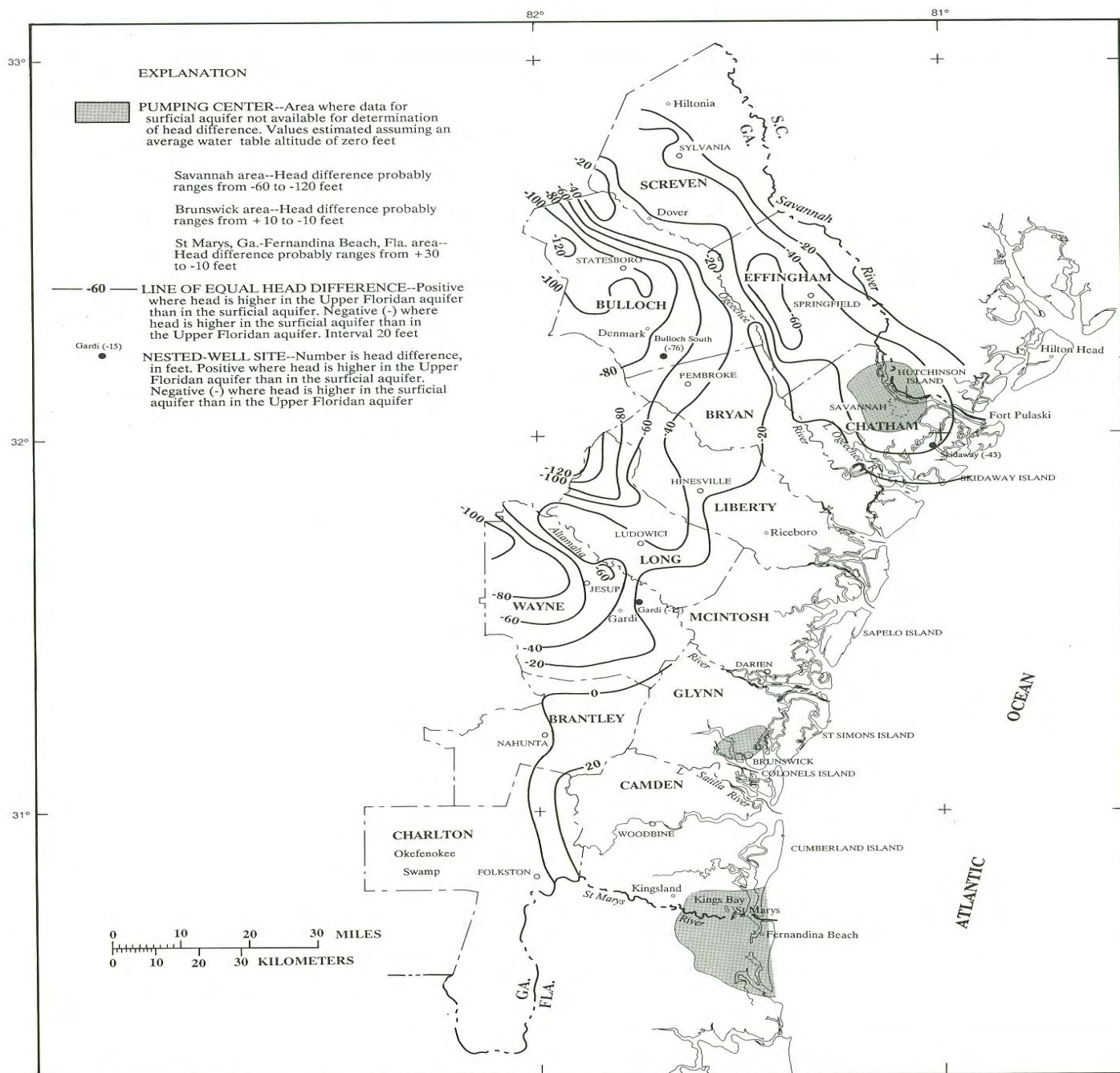
Figure 17.--Estimated difference in head between the Upper Floridan aquifer and the surficial aquifer.
