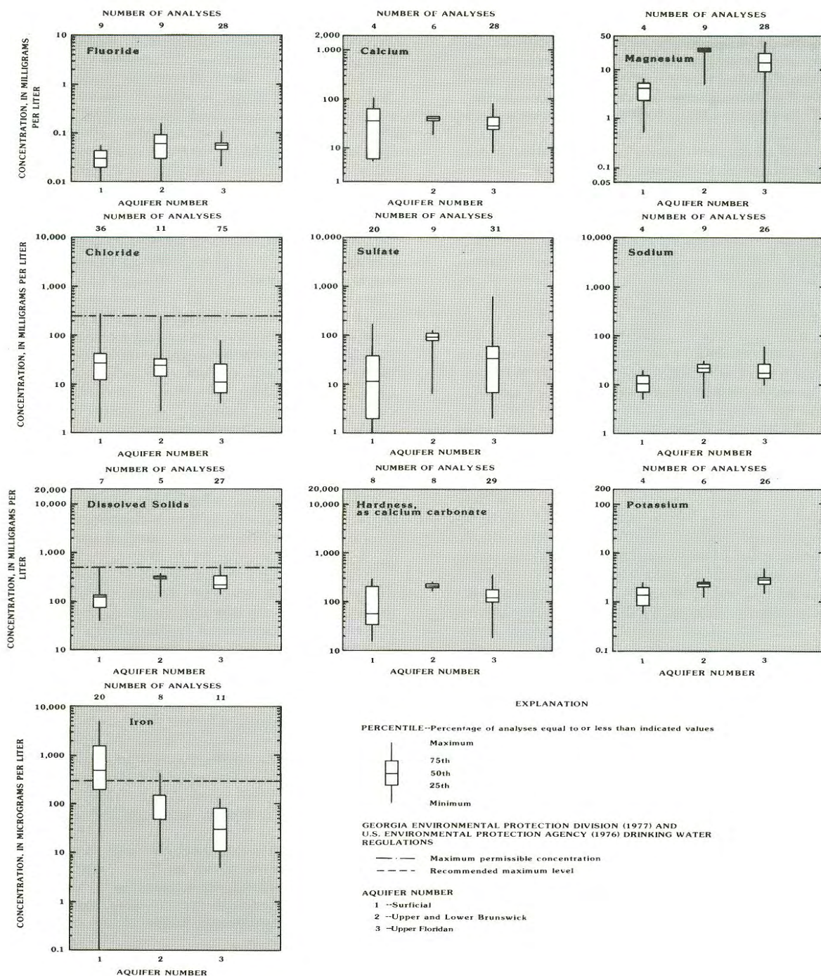
Figure 18.--Boxplots of selected chemical constituents.
