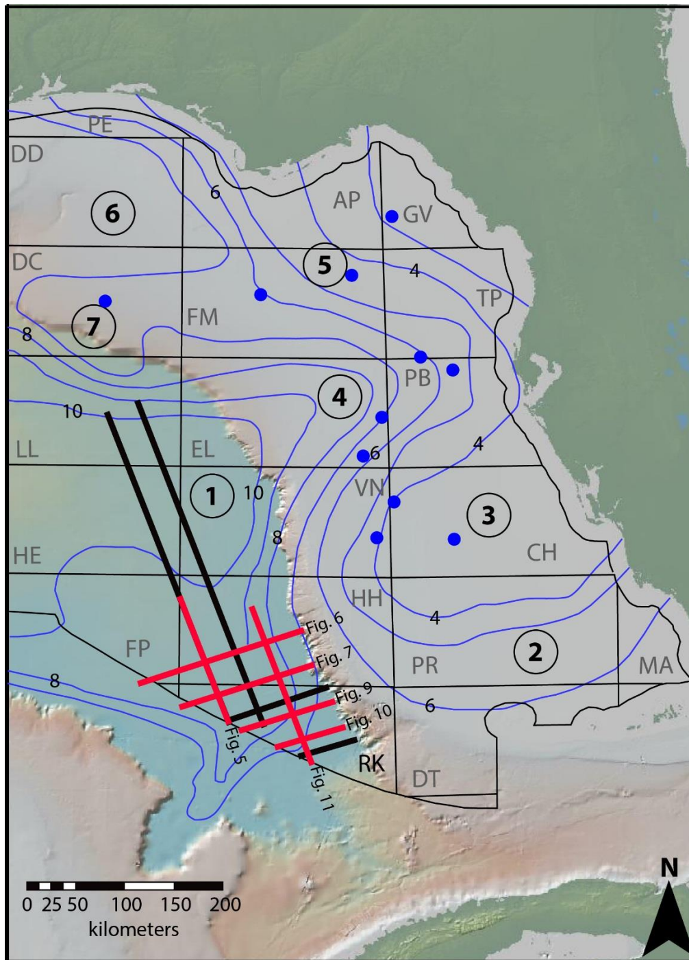
Figure 1. Basement contour map showing locations of major rift related structures in the EGoM that are discussed in text: 1) West Florida Basin; 2) South Florida Basin; 3) Sarasota Arch; 4) Tampa Embayment; 5) Middle Ground Arch; 6) DeSoto Canyon Salt Basin; 7) Southern Platform. Thick black lines are seismic reflection profiles used in this study with figure locations marked. Depth to basement (in blue) is in kilometers from Sawyer et al. (1991). Thin black lines denote protraction areas in the EGoM. Blue dots indicate well locations.
