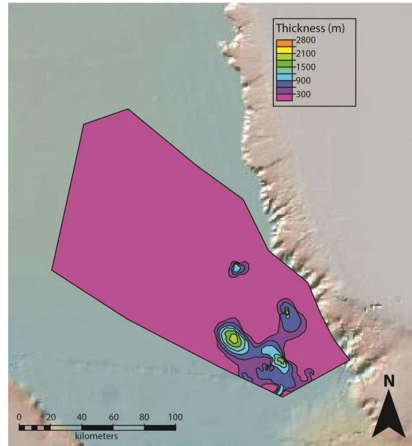
Figure 13. Isochore map for carbonate buildups. Carbonate buildups are present on basement highs towards the southeast.
