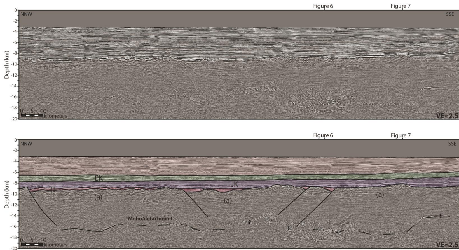
Figure 5. Strike Line. Crust (a) appears more linear and is overall devoid of brittle faults. Moho/detachment surface is present along the entire profile beneath an approximate depth of 16 km. This interpretation is used to infer that crust (a) may be oceanic/proto oceanic crust. TJ is thin or absent along the profile. JK and EK are widely distributed and are generally not influenced by basement topography.
