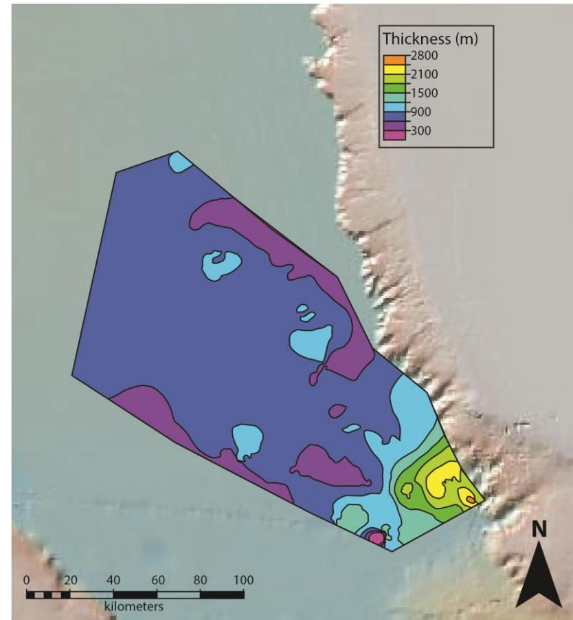
Figure 15. Isochore map for EK. EK has a wider distribution within the study area as sedimentation overcomes basement topography.
