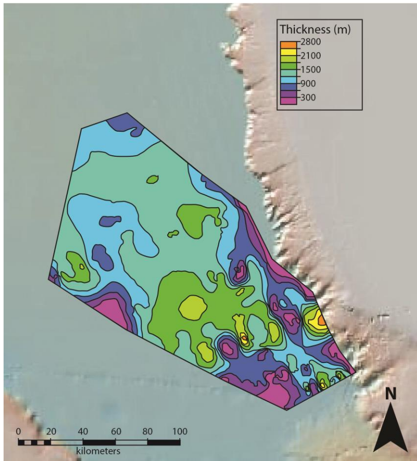
Figure 14. Isochore map for JK. JK thickness varies from north to south depending on basement topography following extension.
