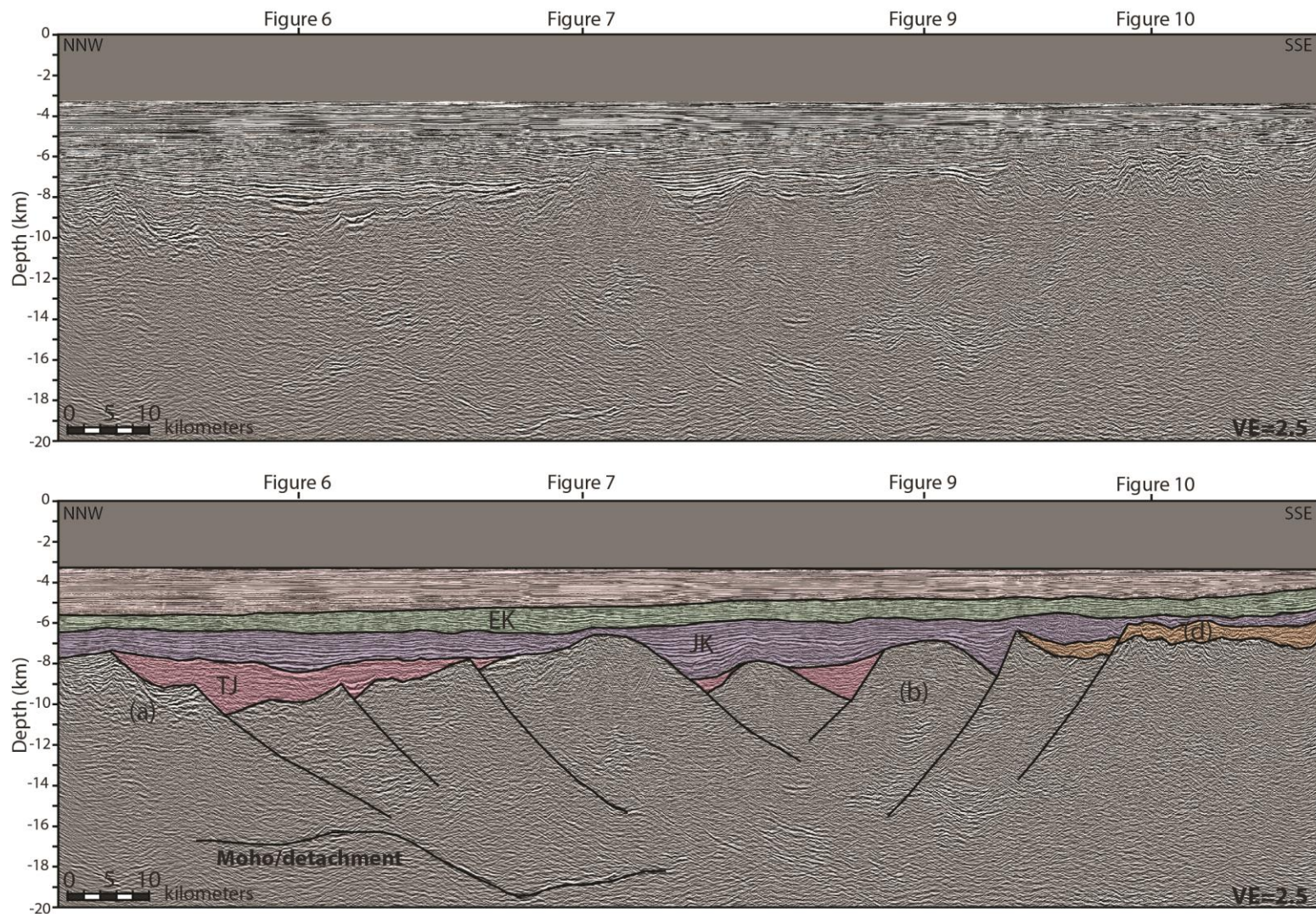
Figure 11. Strike Line. Basement topography increases towards the southeast. Carbonate buildups (d) cap basement highs in the south. TJ is absent in the southeast but present in basement lows to the northwest. A Moho/detachment shallows towards the northwest and crust type changes from continental to oceanic/proto oceanic in the north.
