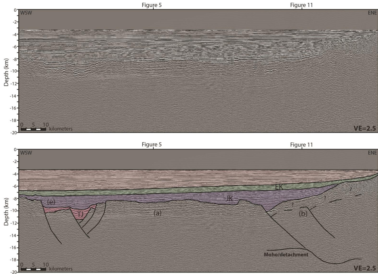
Figure 6. Dip Line. The oceanic/ proto oceanic crust (a) appears more linear, while the continental crust (b) has a chaotic seismic character. Moho/detachment reflector shallows basinward. TJ distribution is highly controlled by basement topography. JK and TJ exhibit fanning (e) off basement structures due to syn-rift sedimentation.
