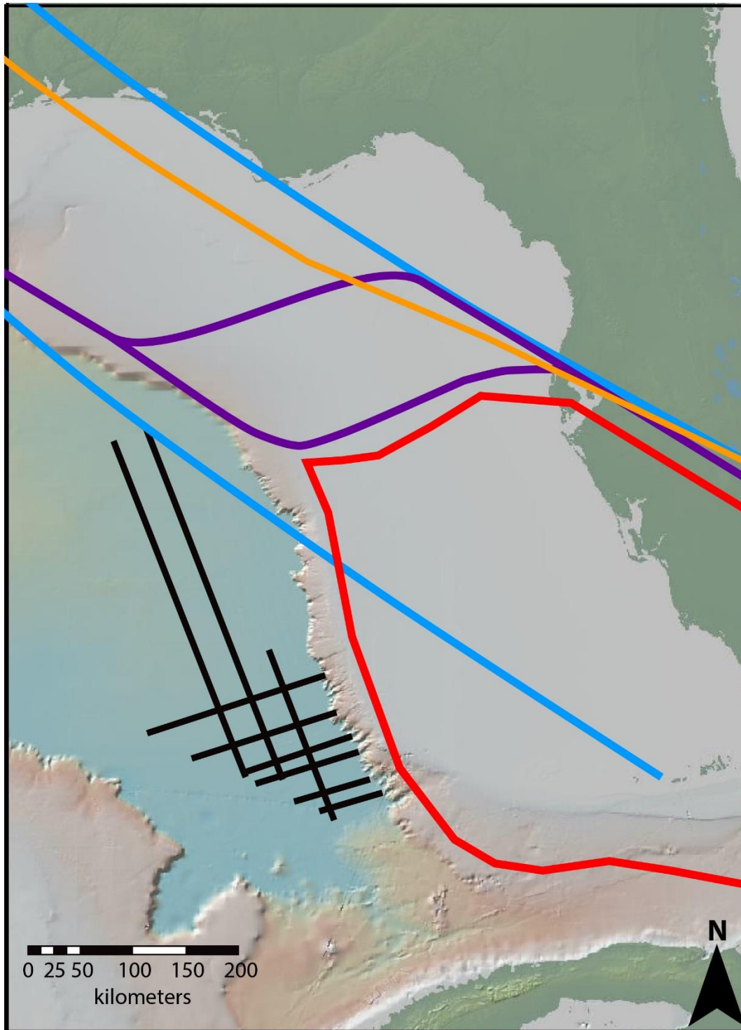
Figure 16. Location of proposed transfer faults during Late Triassic rifting in the EGoM. Orange: Marton and Buffler, 1994; Blue: MacRae and Watkins, 1996; Purple: Pindell and Kennan, 2001. Red indicates the Florida Continental Block by Pindell and Kennan, 2001
