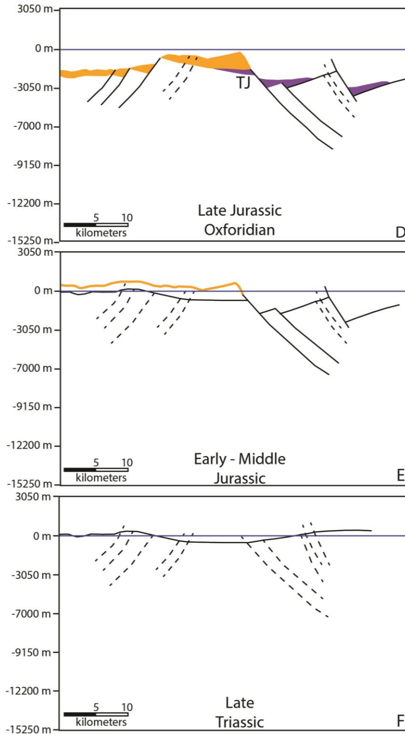
Figure 17. Restoration of Figure 10. A-F are time slices in the evolution of the West Florida Basin. In each frame, the youngest layer is removed and the layers underneath are decompacted. Faults (in black) are restored at the appropriate time intervals. This seismic dip line trends over transitional continental crust in the southeastern GoM. Blue line represents modern day sea level. Dashed lines indicate location of future fault planes. Faults represent apparent dip.
