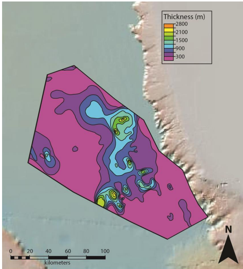
Figure 12. Isochore map for TJ. Distribution is limited to the south by basement topography, while to the northwest TJ is thin over oceanic/proto-oceanic crust.
