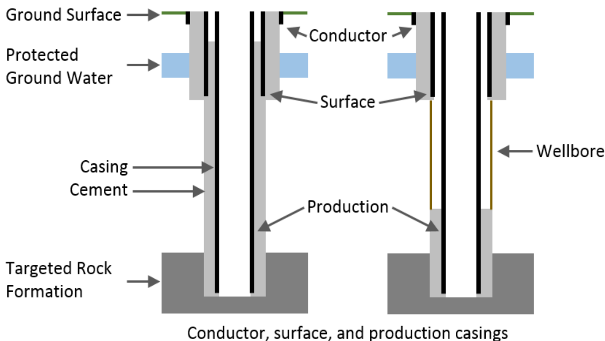
Figure 3-7. Illustration of well construction showing different types of casing and cement.
