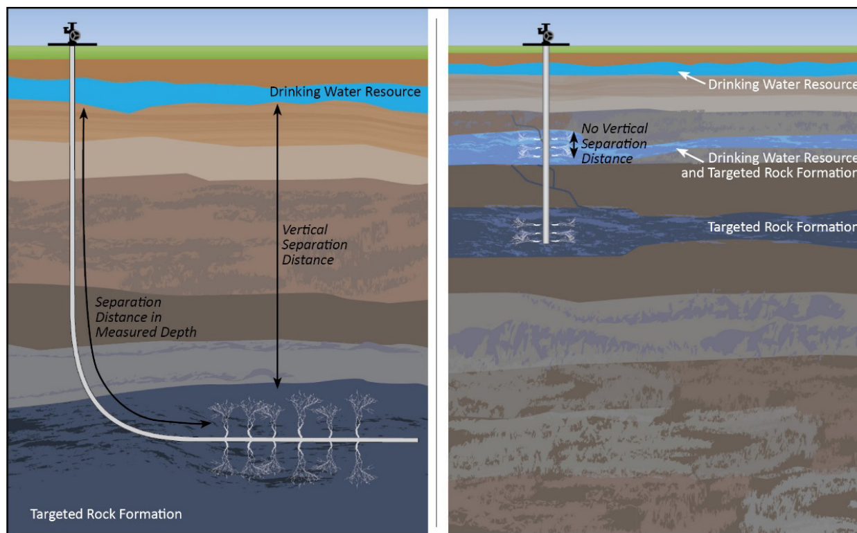
Figure 6-6. Vertical distances in the subsurface separating drinking water resources and hydraulic fracturing depths.
