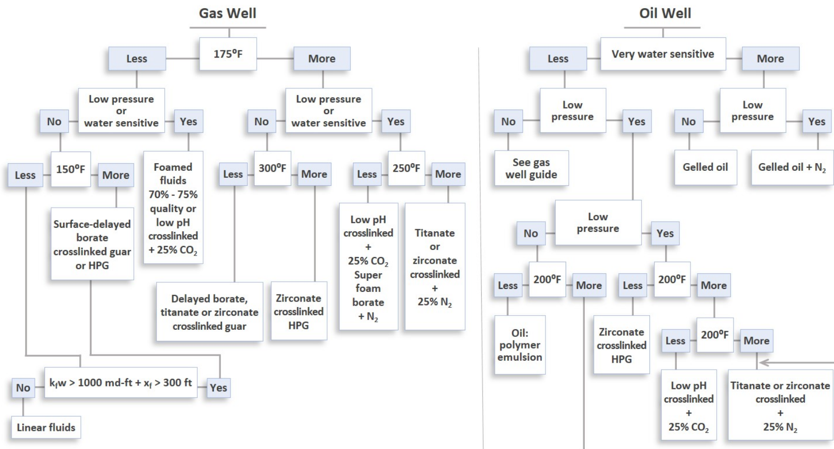
Figure 5-3. Example hydraulic fracturing fluid decision tree for gas and oil wells.
