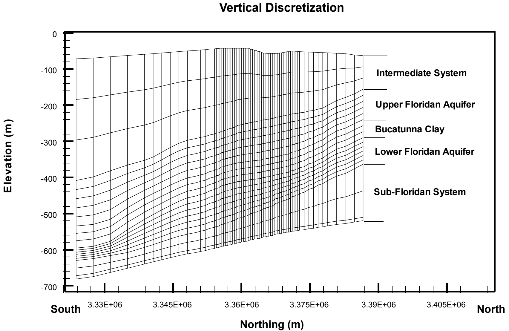
Figure 3.3 Vertical Discretization Along y-z Cross-Section at x=505327m
