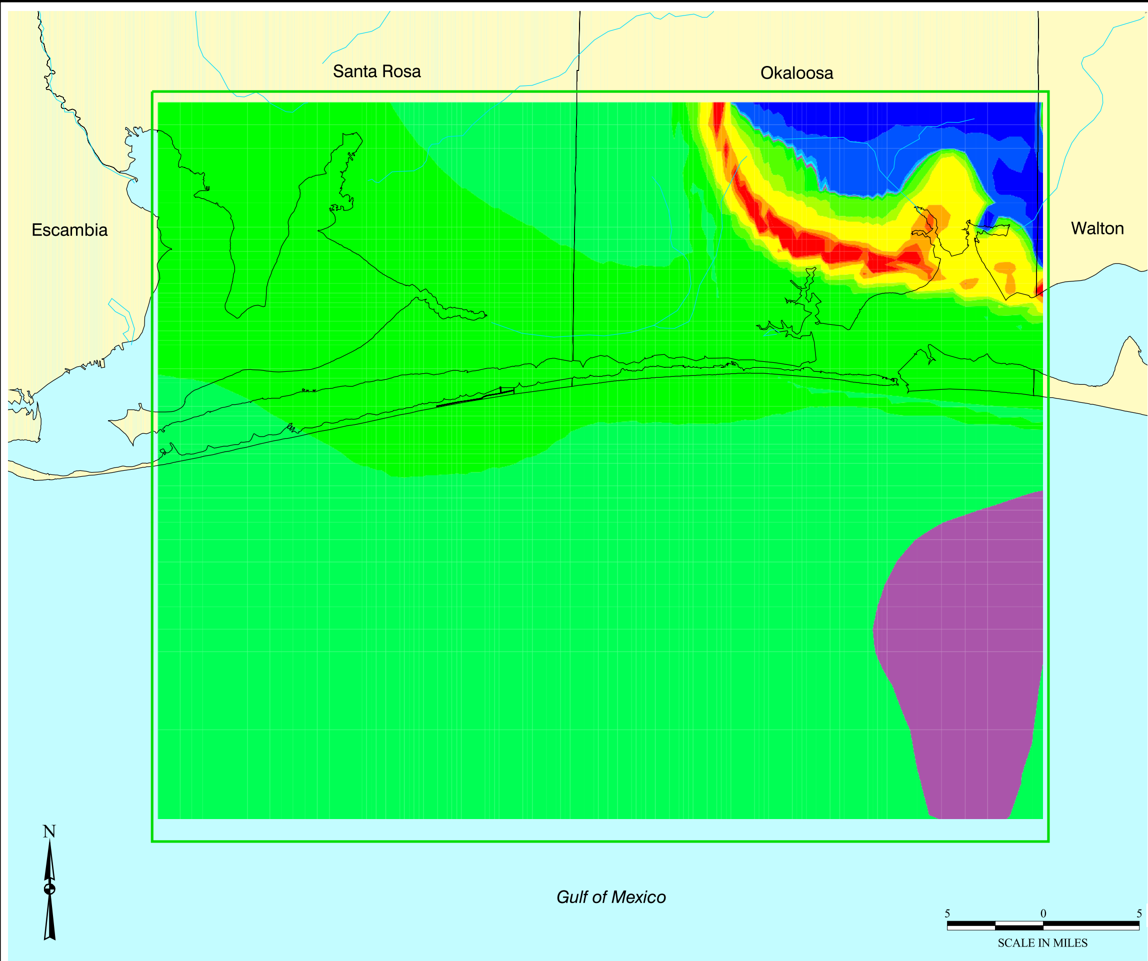
Figure 4.32 1998 Vertical Darcy Velocities for the Bucatunna Clay Confining Unit and Middle Portion of the Undifferentiated Floridan Aquifer System (Elemental Layer 11)
