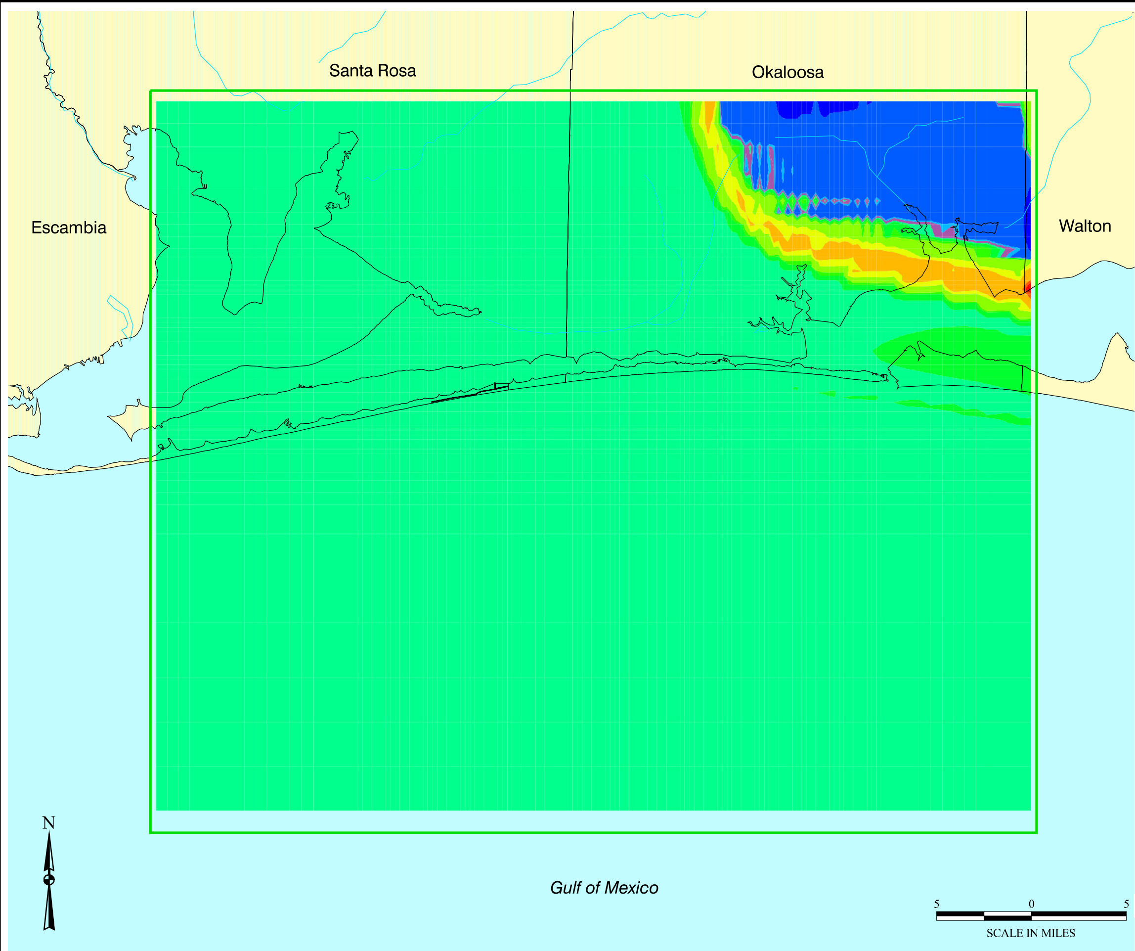
Figure 4.14 Pre-Development Vertical Darcy Velocities for the Bucatunna Clay Confining Unit and Middle Portion of the Undifferentiated Floridan Aquifer System (Elemental Layer 11)
