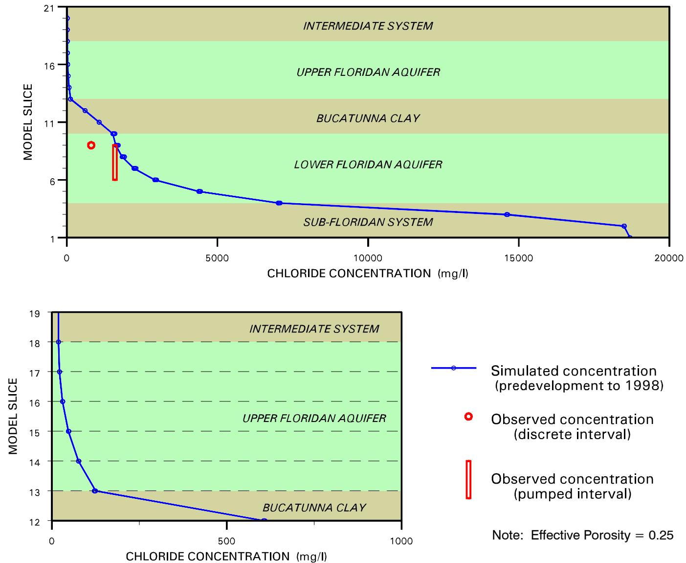
Figure 4.61 Beal Cemetery Concentration Profile
