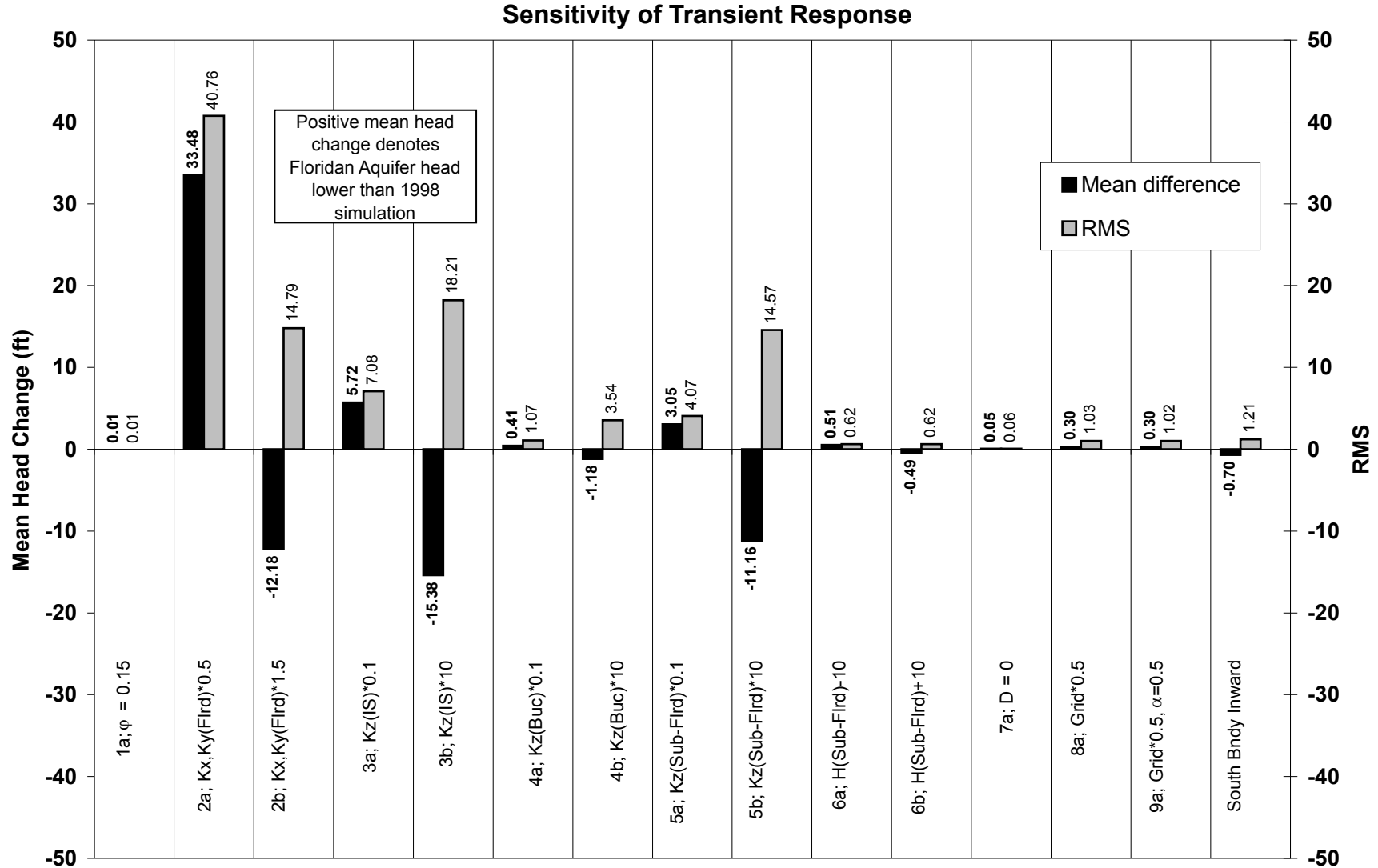
Figure 5.7 RMS and Mean Head Change from Post-Development Base Case for the Upper and Lower Floridan Aquifers Combined
