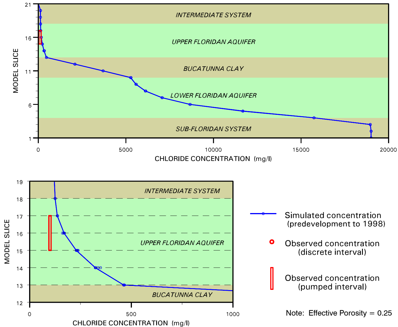
Figure 4.59 Navarre Beach Concentration Profile
