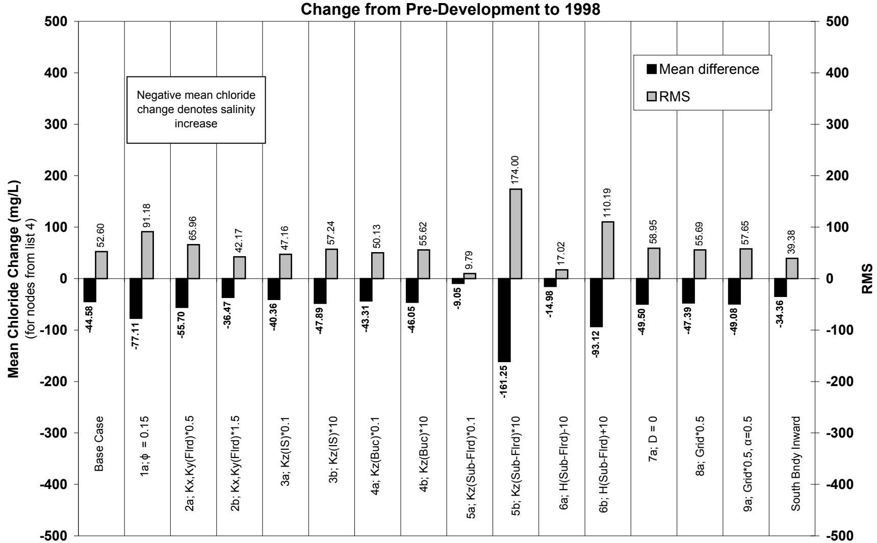
Figure 5.14 RMS and Mean Chloride Change from Pre-Development to 1998 for the Lower Floridan Aquifer
