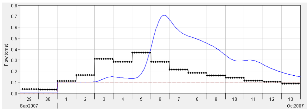
Figure 2-30. Wolf Creek Validation Results USGS Gauge 02231458
