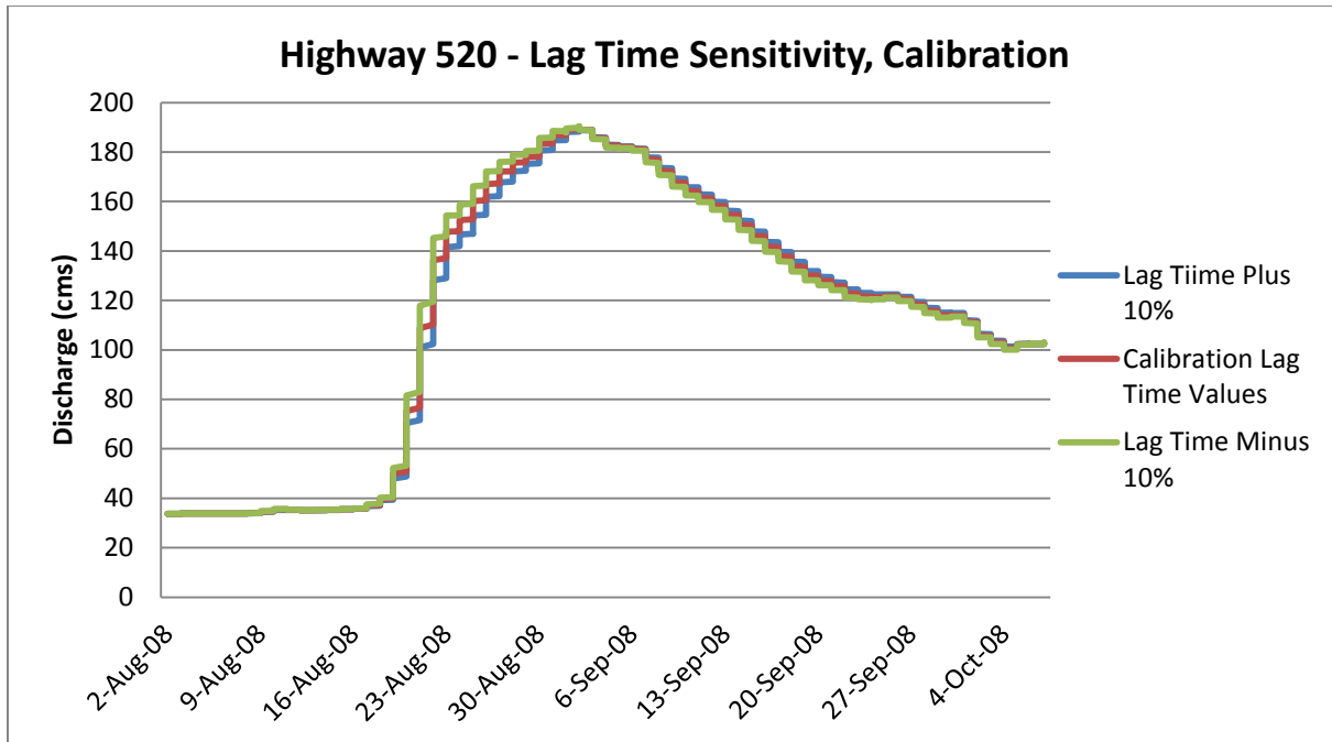
Figure 2-55. Highway 520, Lag Time Sensitivity Analysis for Calibration
