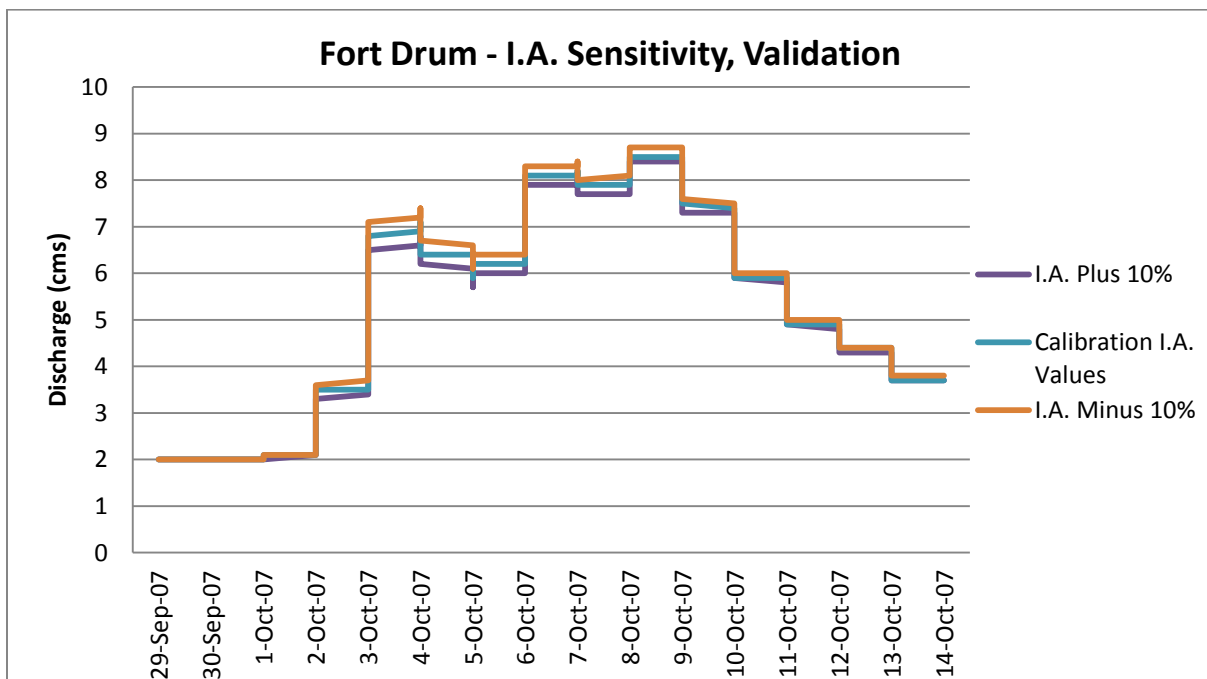
Figure 2-62. Fort Drum, Initial Abstraction Sensitivity Analysis for Validation
