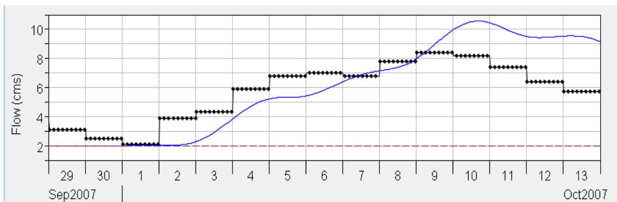
Figure 2-29. Blue Cypress Creek Validation Results USGS Gauge 02231396
