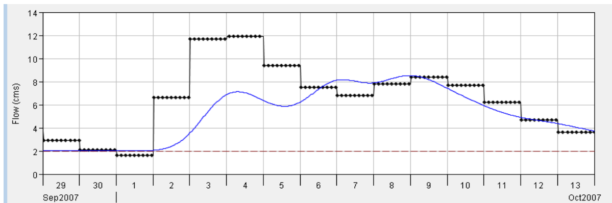
Figure 2-28. Ft. Drum Creek Validation Results, USGS Gauge 02231342
