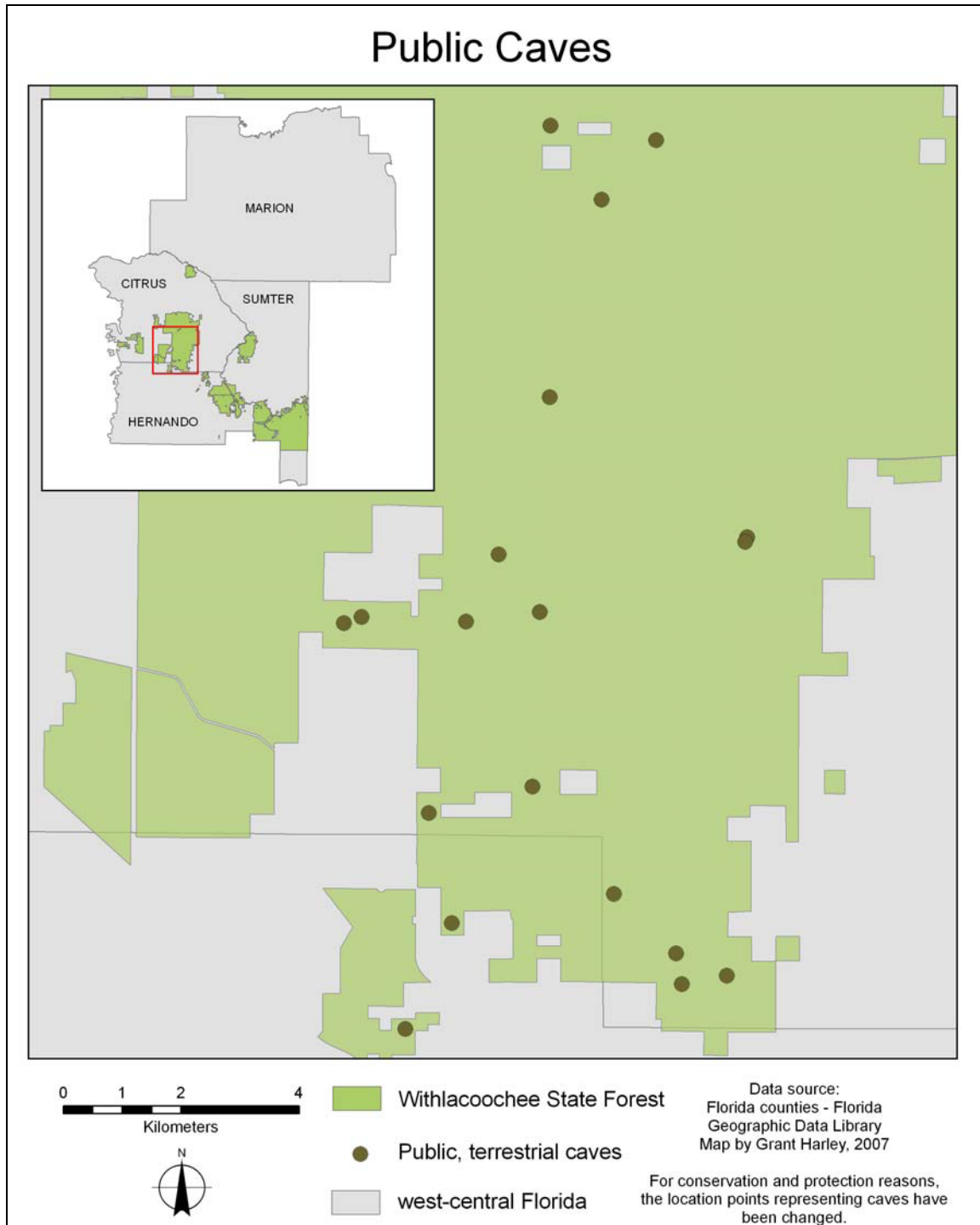
Figure 22. Locations of public caves inventoried during this project. Of the 36 caves, 19 were located on the public, state-owned land of the Withlacoochee State Forest, west-central, Florida.
