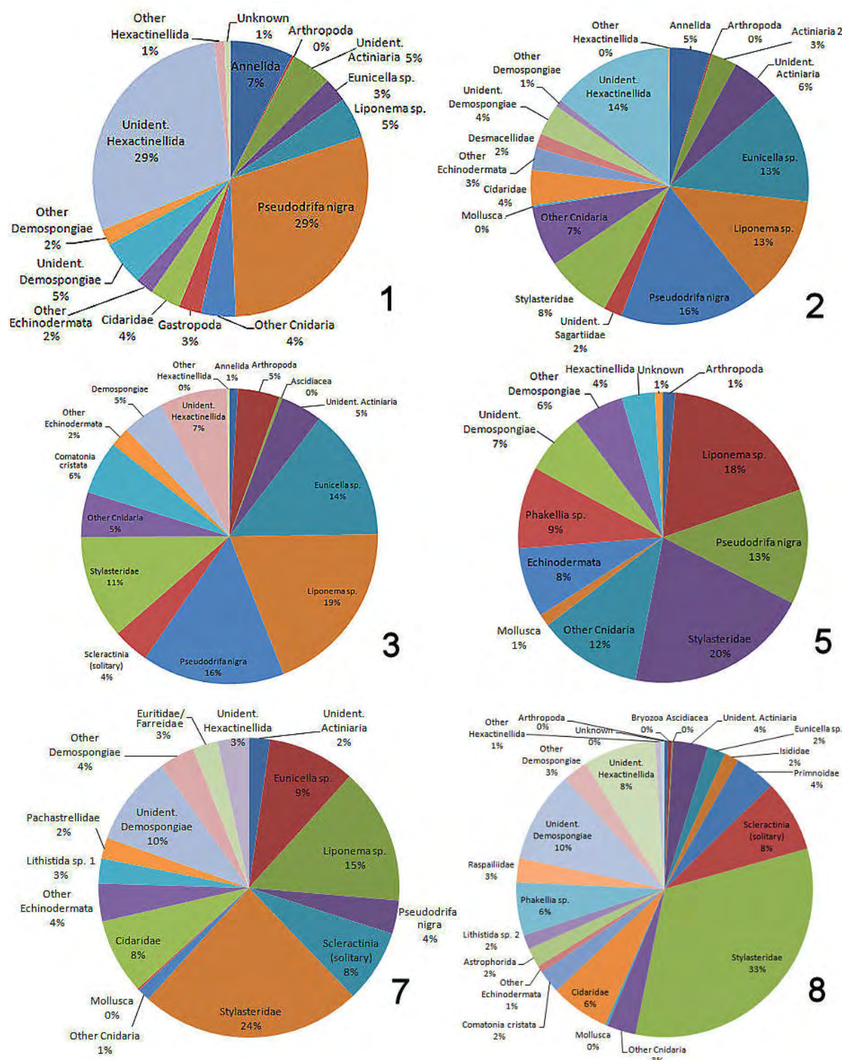
Figure 6-29. Priority Area 3 primary transect low-slope quantitative photostations 1, 2, 3, 5, 7 and 8. Macrofaunal organism densities (in m^{-2} ) expressed as percentages of total organism abundance (data from Table 6-18). Font in this and Figures 6-30 and 6-31 size varied among pie diagrams to keep labels from overlapping.
