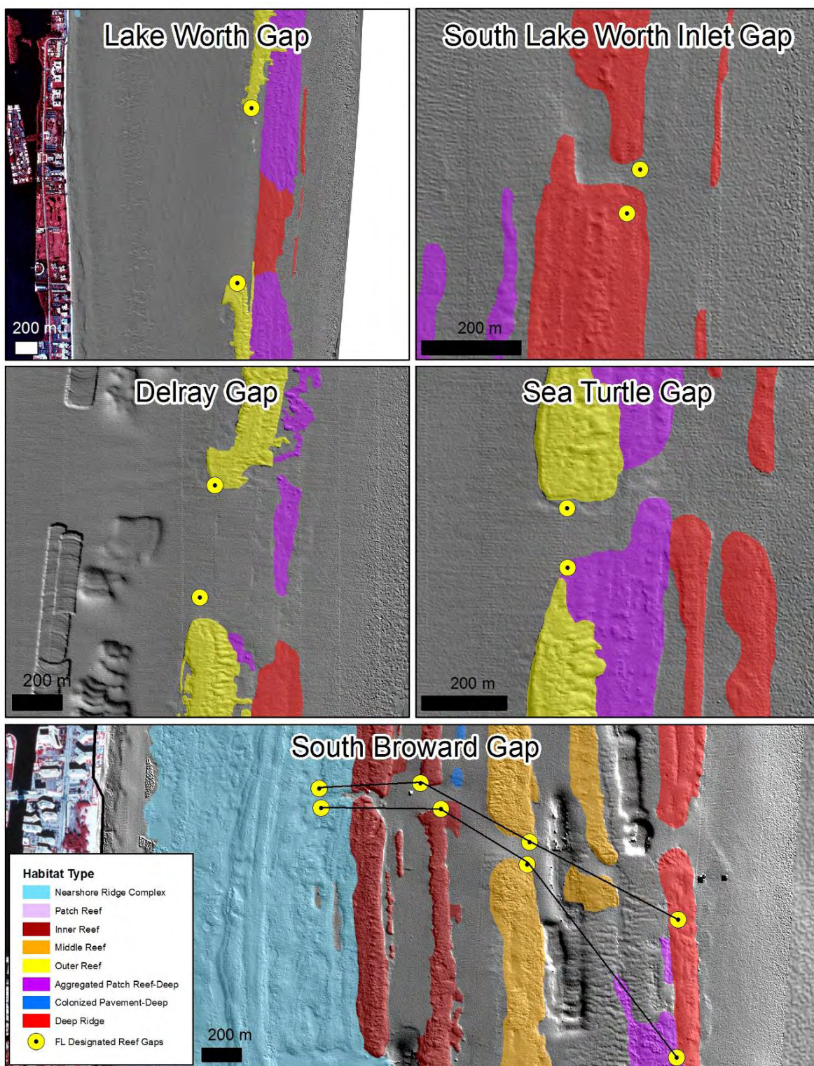
Figure 4-2. Map of the State of Florida (Chapter 18-21.004(2) (l), FAC) designated shallow-water reef gaps in southeastern Florida. Yellow dots are the locations listed in Table 4-1. The underlying image is hillshaded topography derived from bathymetric lidar data color coded by the southeastern Florida benthic habitats (Walker, 2012).
