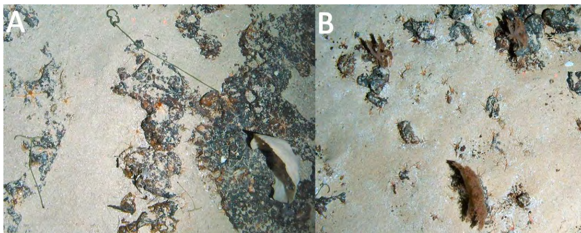
Figure 6-21. Inner Terrace Platform. A. Several echiuran worms Ochetostoma sp., fan sponge Phakellia sp. and numerous ophiuroids on low-relief, sediment-veneered pavement. B. Several soft corals Pseudodrifa nigra on phosphoritic rubble.
