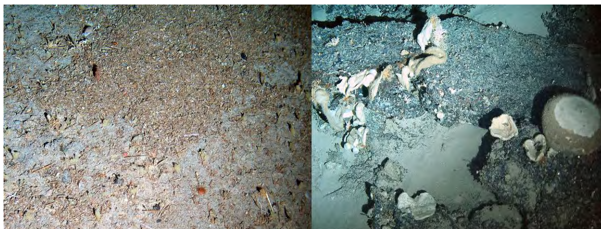
Figure 6-22. Priority Area 3 northeast transect. A. Coarse shelly hash including echinoid spines on low-relief pavement with a gastropod (possibly Sconsia sp.), solitary corals and ophiuroids. B. High-relief tilted phosphoritic slabs with a variety of sponges including lithistids (fluted plates) and a spherical astrophorid.
