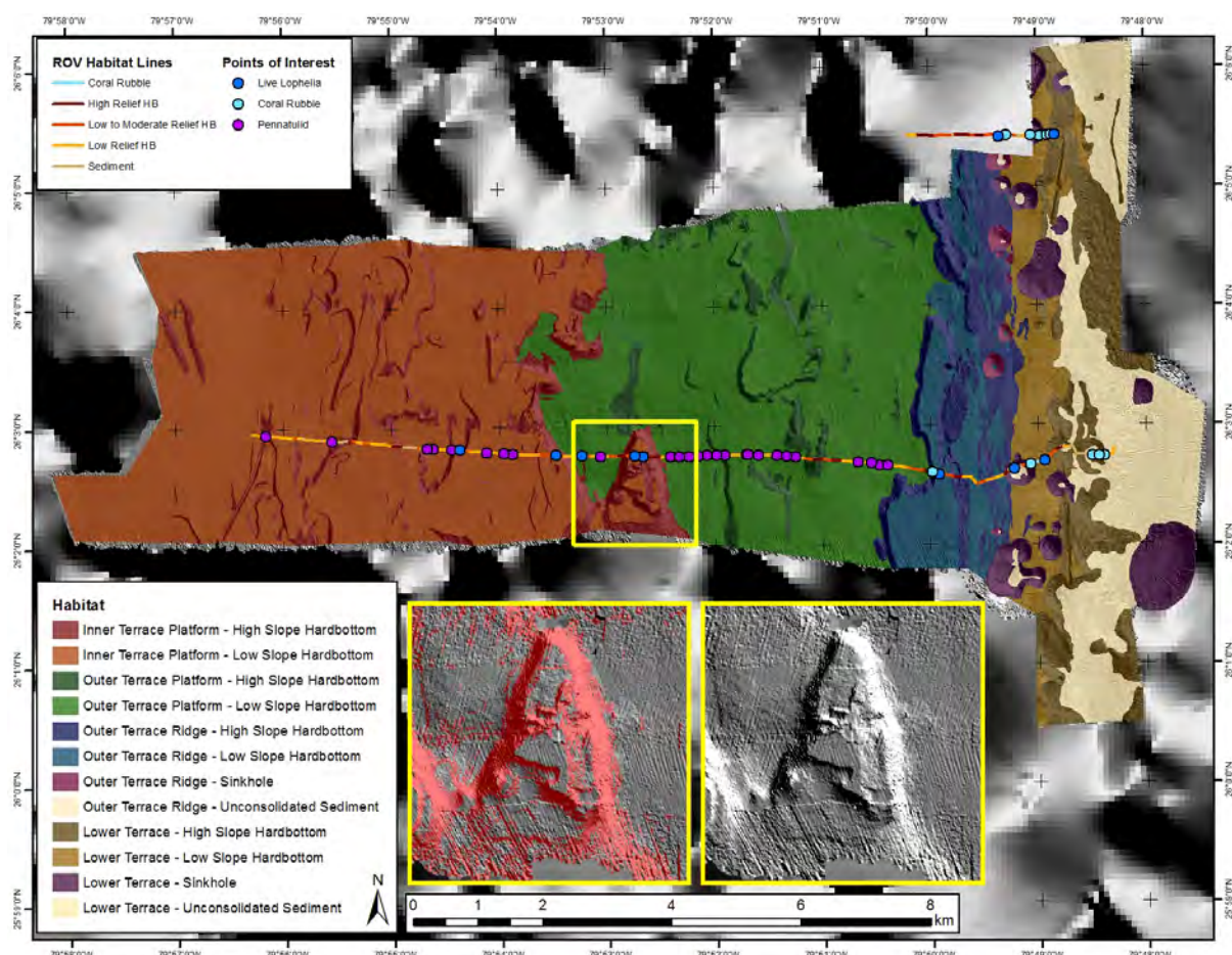
Figure 6-17. Priority Area 3 Benthic Habitat Map showing transect lines and the four major zones. Left insert: Red and pink areas illustrate high-slope ( >5^{\circ} ) seafloor areas from geophysical data. Right insert: shows detail of the multibeam topography on which the distinction between low- and high-slope areas was made.
