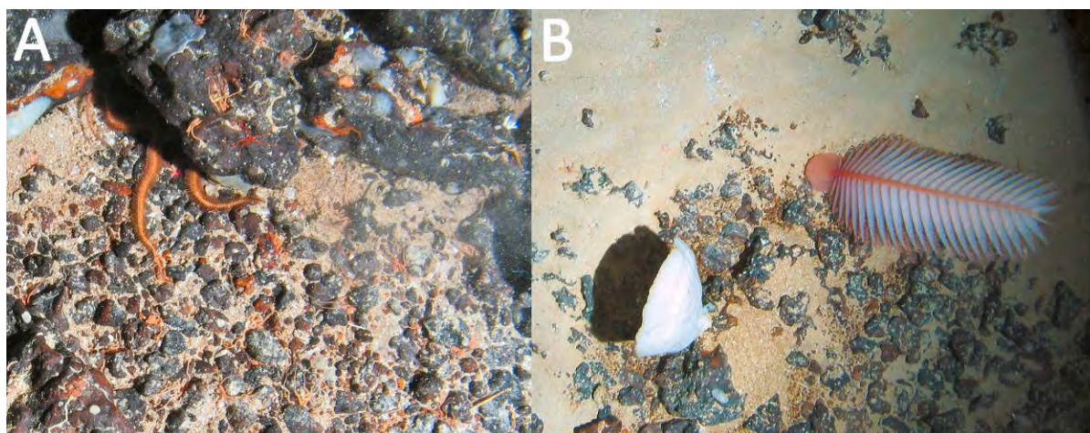
Figure 6-20. Outer Terrace Platform. A. Abundant ophiuroids belonging to three species. B. Sea pen ( Pennatula or Ptilosarcus sp.) apparently on sediment-veneered hard bottom, accompanied by the fan sponge Phakellia sp.
