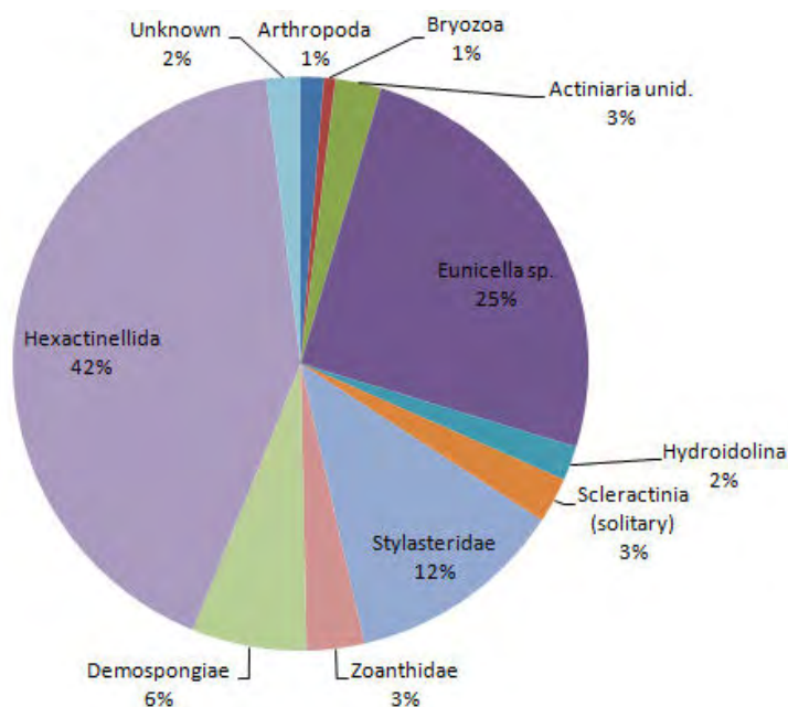
Figure 6-28. Macrofaunal organism densities (in m^{-2} ) at the Priority Area 1 quantitative photostation expressed as percentages of total benthic density (data from Table 6-16).
