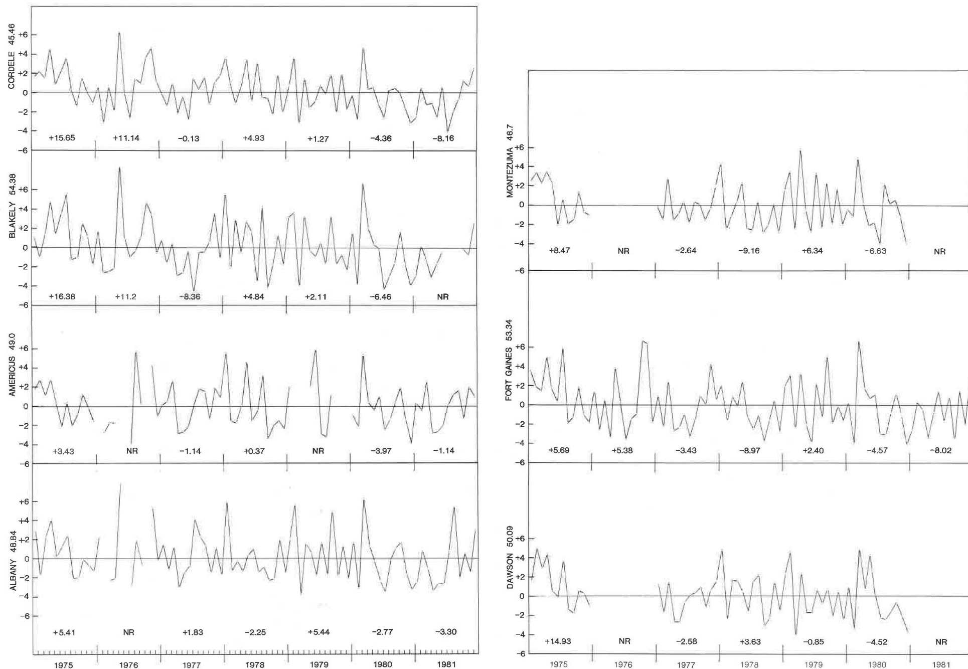
Figure 4. Rainfall Departure Curves - Cities In Study Area. Plotted are the monthly rainfall departures from the 30-year norm. Annual departures are shown below the curve for each city.
