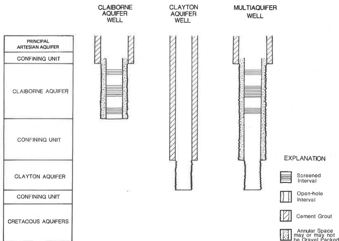
Figure 13. Typical Well construction in the Study Area.
