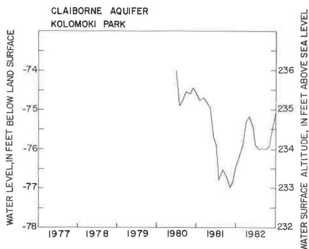
Figure 26. Hydrographs of Claiborne Aquifer Wells. a). U.S. Geological Survey TW 2, located south of Albany, Dougherty County. b). Georgia Geologic Survey test well located in Kolomoki Park, Early County.
