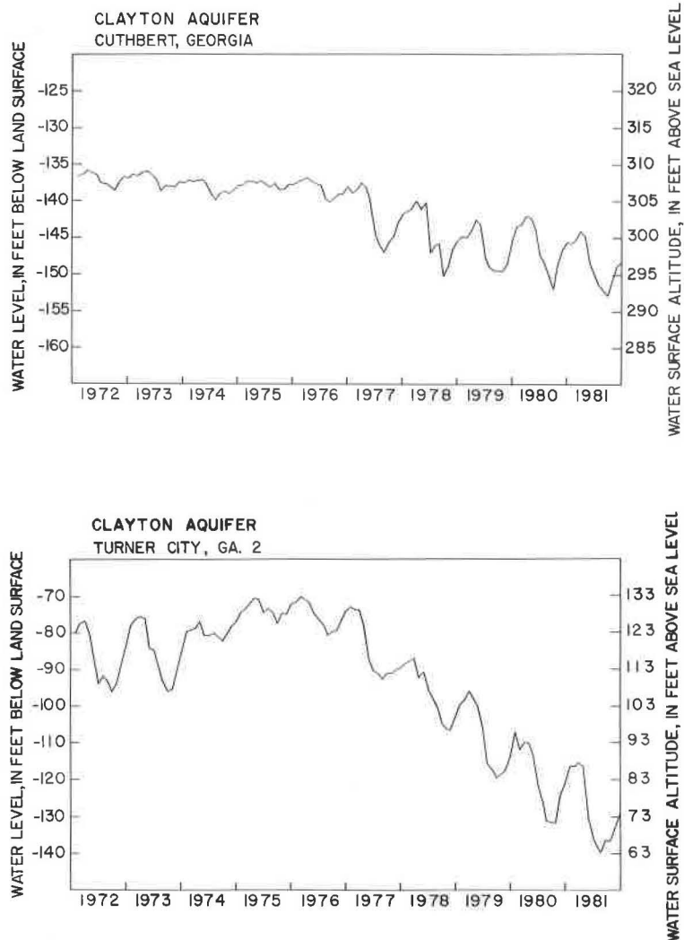
Figure 25. Hydrographs of Clayton Aquifer Wells. a). City of Cuthbert, Randolph County. b). Turner City, Dougherty County. (Source of data U.S. Geological Survey).
