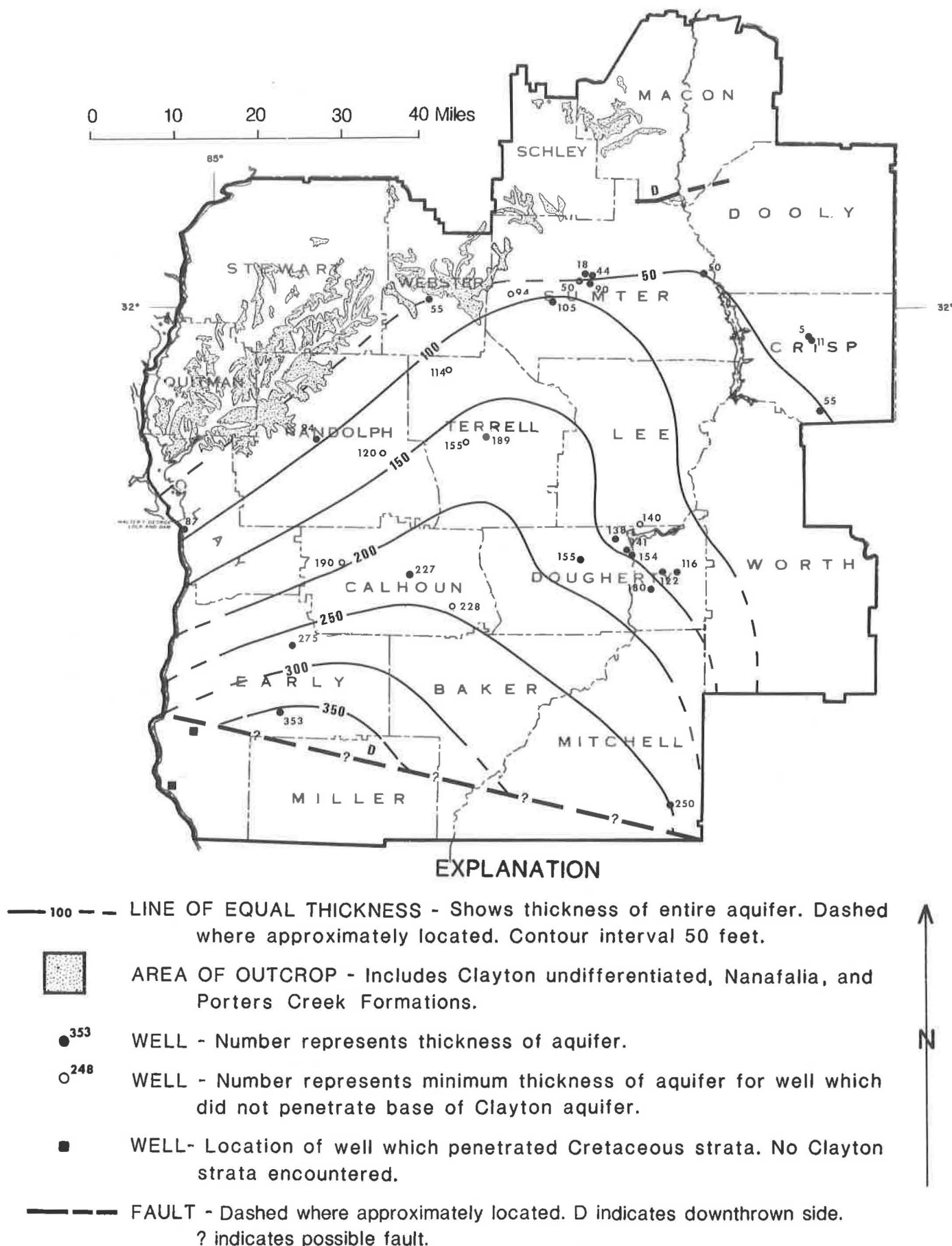
Figure 6. Isopach Map of the Clayton Aquifer (from Tuohy, M.A., 1983c).
