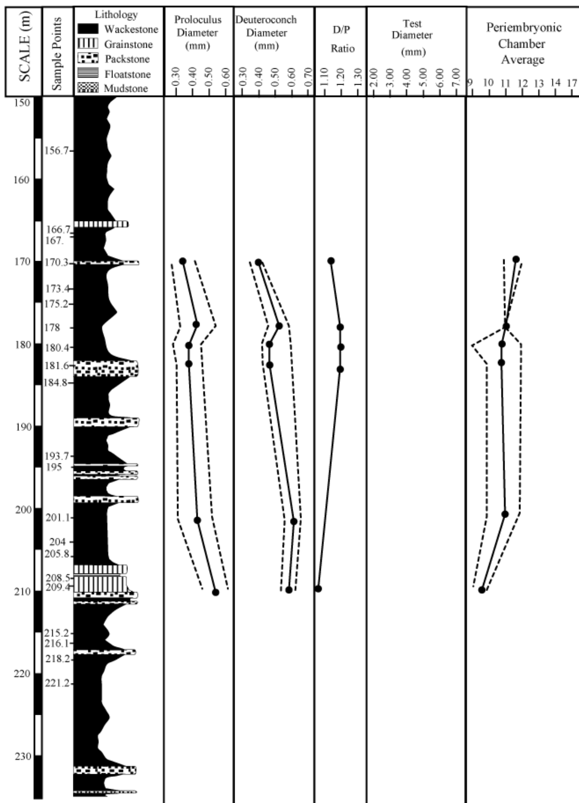
Figure 4.13 Lepidocyclus ocalana var. B measurements compared to stratigraphy of ROMP 29A core. Solid lines represent averages of measurements. Dashed lines indicate the range of the measured feature.
