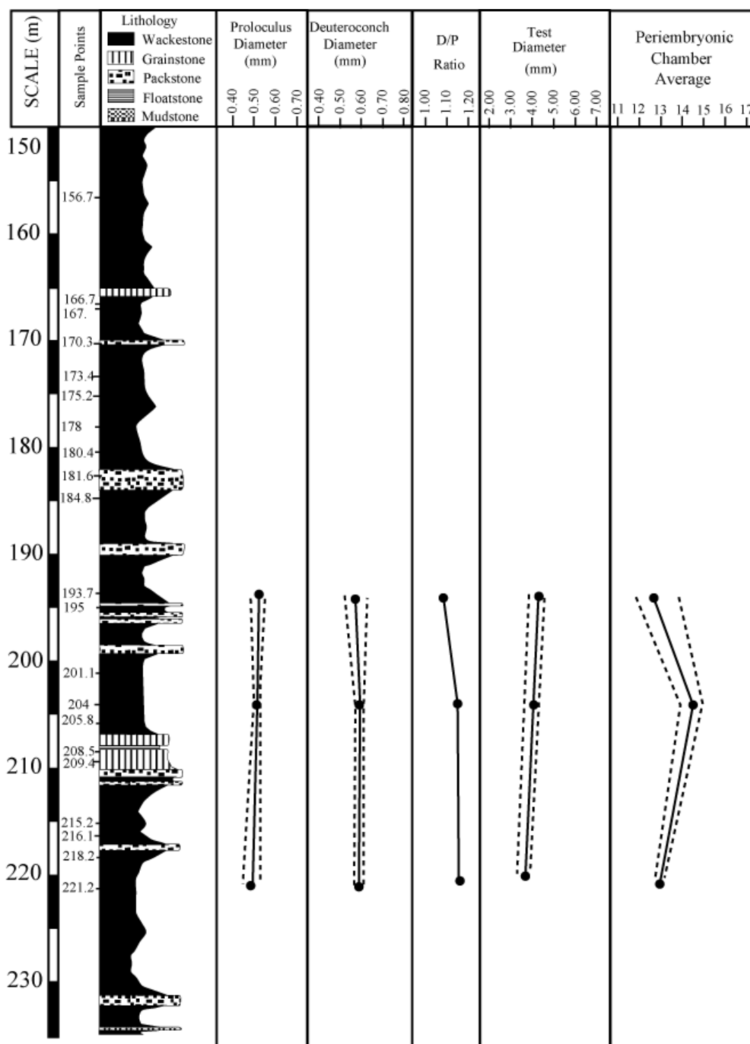
Figure 4.12 Lepidocyclina ocalana var. A measurements compared to stratigraphy of ROMP 29A core. Solid lines represent averages of measurements. Dashed lines indicate the range of the measured feature.
