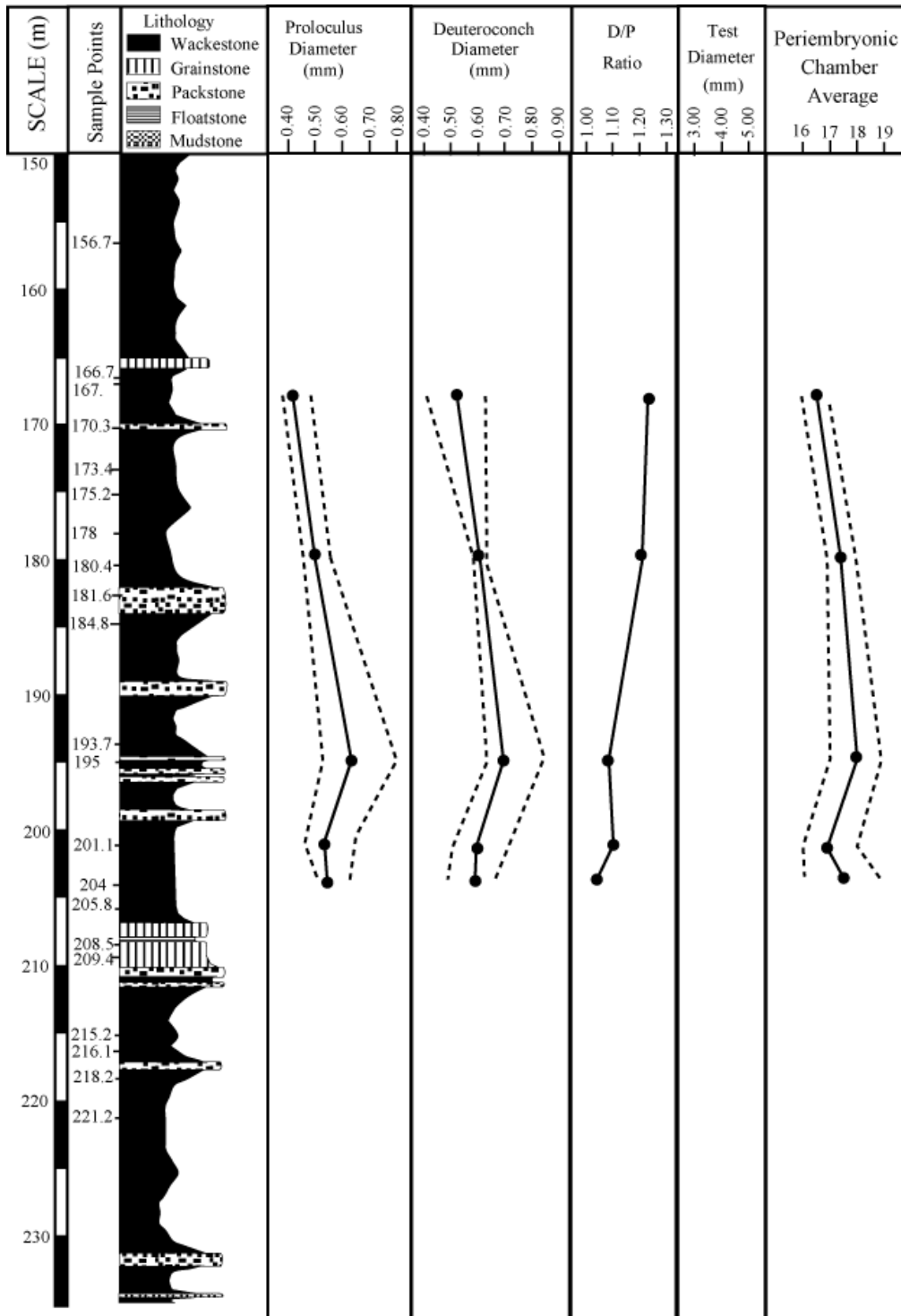
Figure 4.15 Lepidocyclus ocalana var. D measurements compared to stratigraphy of the ROMP 29A core. Solid lines represent averaged measurements. Dashed lines indicate the range of the measured feature.
