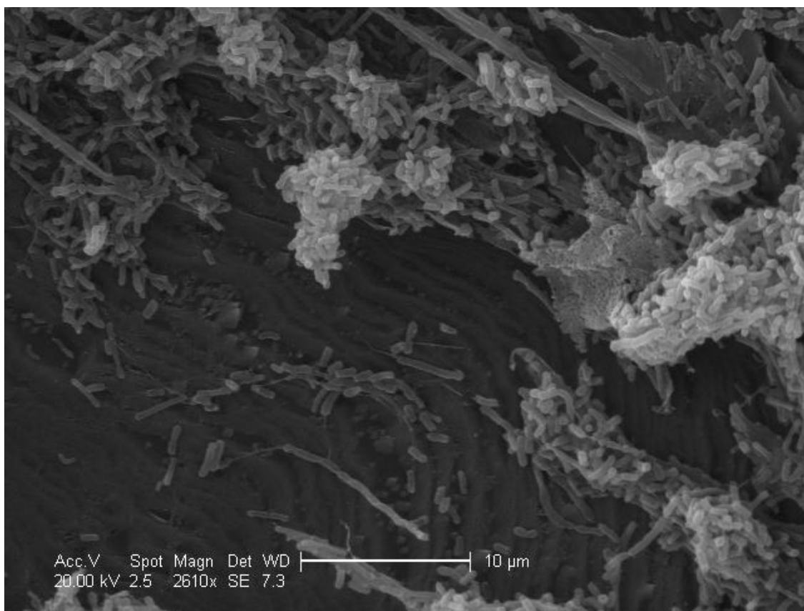
Figure 21. SEM image of Iceland Spar coupon retrieved from Biotic CDC 4 reactor inoculated with a LKC microbial mat performed at pH = 8.3 after 3 weeks in reactor. Scale bar 10 \mu m. Bulk media was at equilibrium w.r.t. calcite which resulted in corrosive textures that resemble filamentous morphologies.
