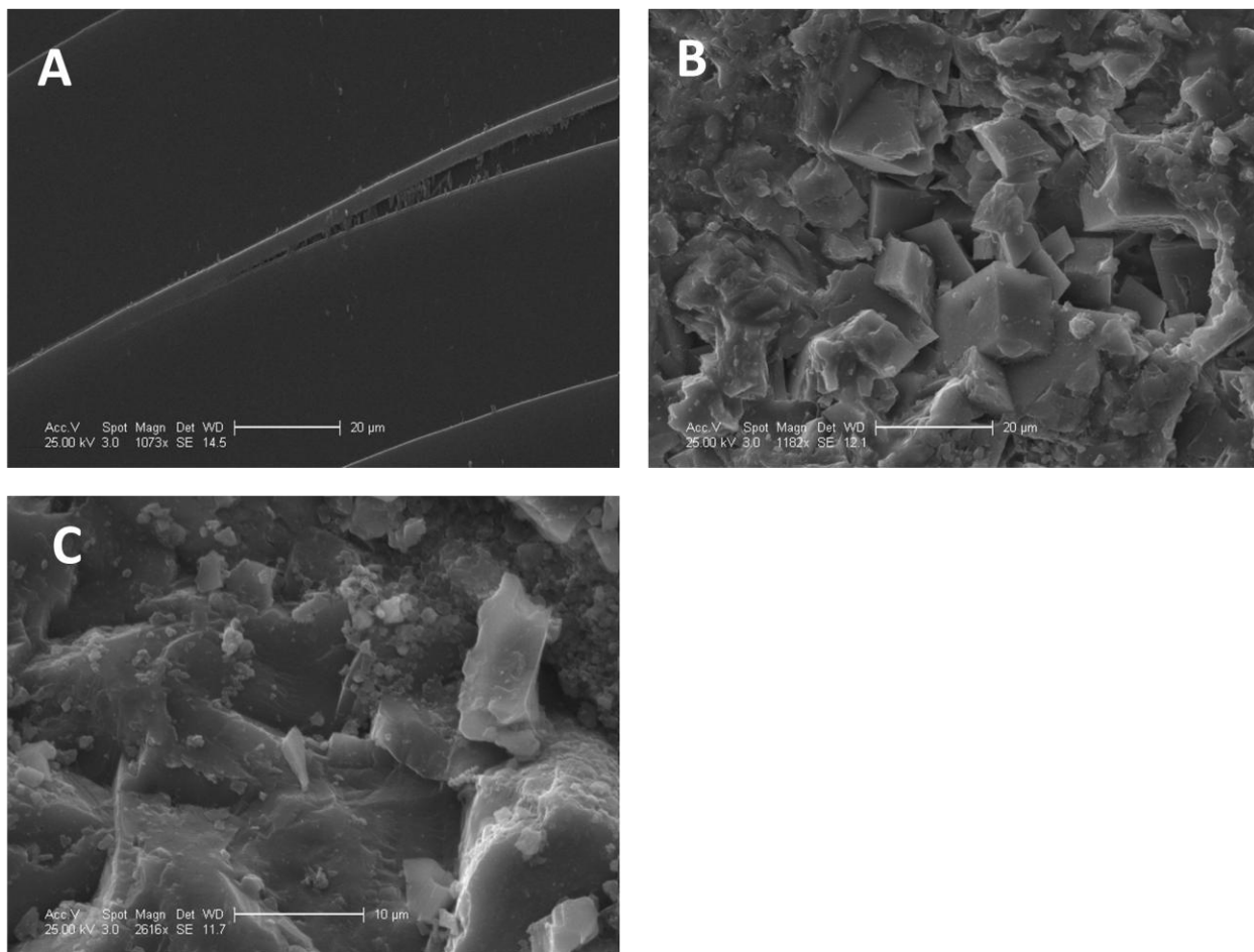
Figure 13. SEM images of carbonate coupons that were not run in the CDC reactor. A is Iceland Spar, B is Limestone, C is Dolostone. Scale bar is 20 \mu\text{m} on A and B, 10 \mu\text{m} on C. Coupons surfaces are free of corrosive textures.
