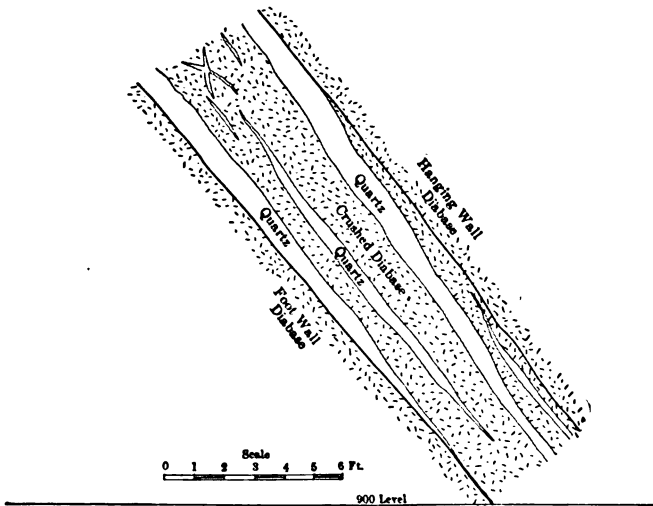
FIG. 145.—Section of the Pittsburg vein, ninth level, Nevada City district, Cal. XVII. Ann. Rep. U. S. Geol. Survey, Part II., p. 204, reduced one half.
