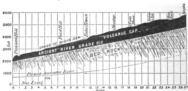
FIG. 141.—Section of Forest Hill Divide, Placer County, California, to illustrate the relations of old and modern lines of drainage. After R. E. Broune, Rep. Cal. State Mineralogist , 1890, p. 444.
