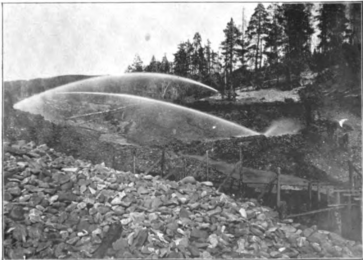
FIG. 137. — The Stevens Hydraulic placer mine, Auro City, Colorado. From a photograph.
