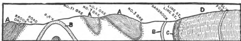
FIG. 11.—Geological Section of the Low Moor, Va., Iron-ore Bed. After B. S. Lyman, Trans. Amer. Inst. Min. Eng. , XIV., 801. A—Marcellus Shale; B—Oriskany Sandstone; C—Lower Helderberg Limestone; D—Clinton Shales.
