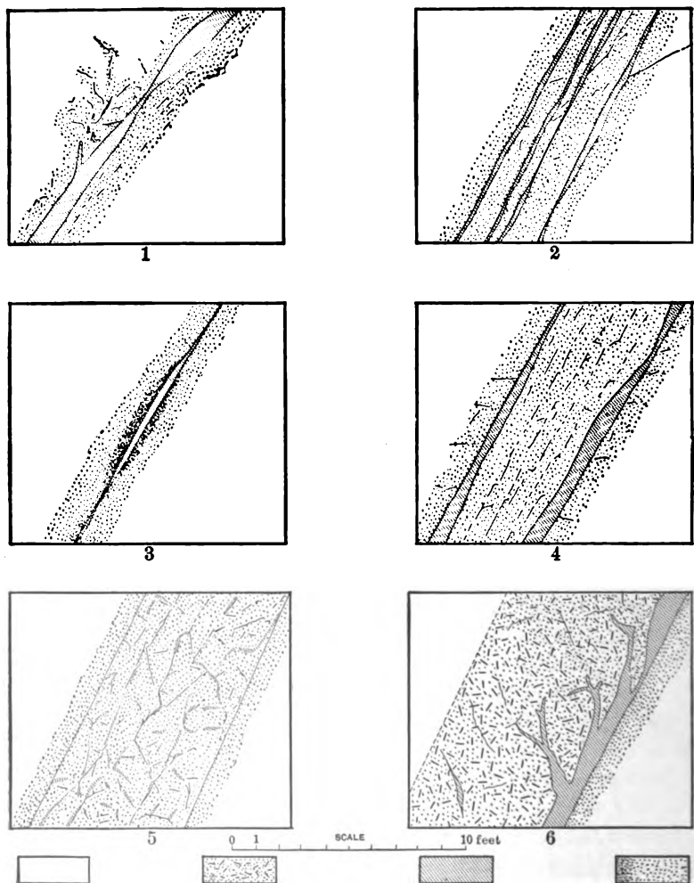
FIG. 137. —Sections to illustrate typical gold veins in the Boise granite region, Idaho. After W. Lindgren, XVIII. Ann. Rep. U. S. Geol. Survey, Part III., Plate XC.
