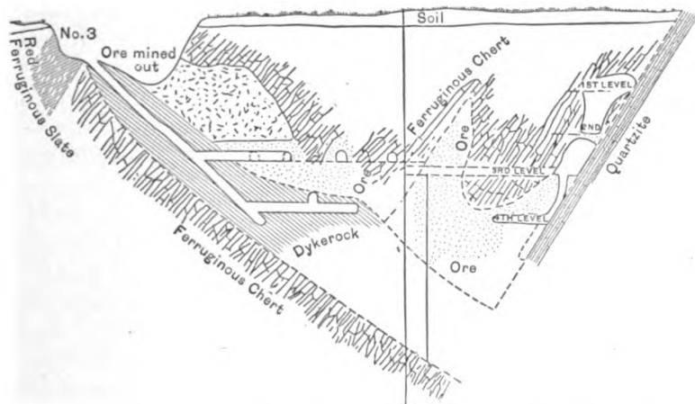
FIG. 33.—Cross-section of the Colby mine, Penokee-Gogebic district, Michigan, to illustrate occurrences and origin of the ore. After C. R.
