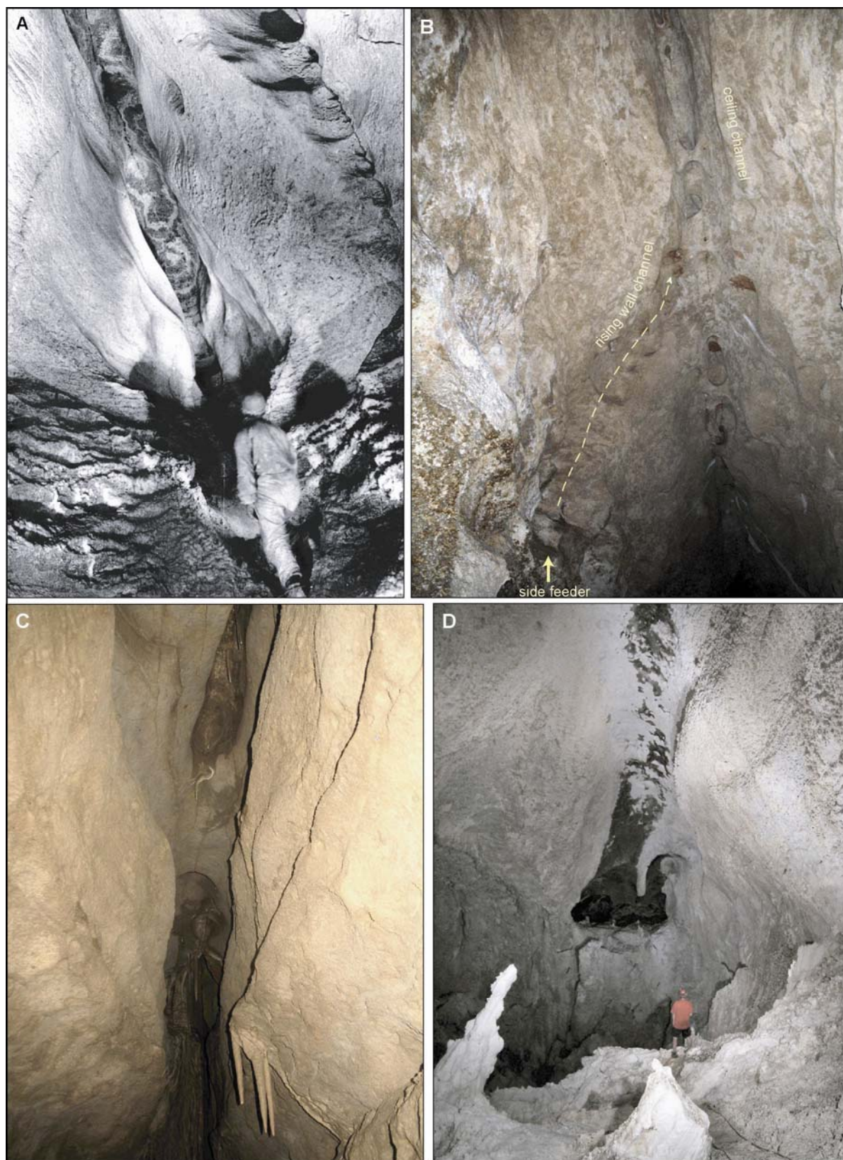
Plate 7. Ceiling channels and cupolas in linear series. A = Atlantida Cave, western Ukraine (Miocene gypsum); B = Carlsbad Cavern, Guadalupe Mountains, NM, USA (Permian limestone); C = Mystery Cave, MN, USA (Ordovician limestone); D = Lechuguilla Cave, NM, USA (Permian limestone). Photo D by S.Allison, other photos by A.Klimchouk.
