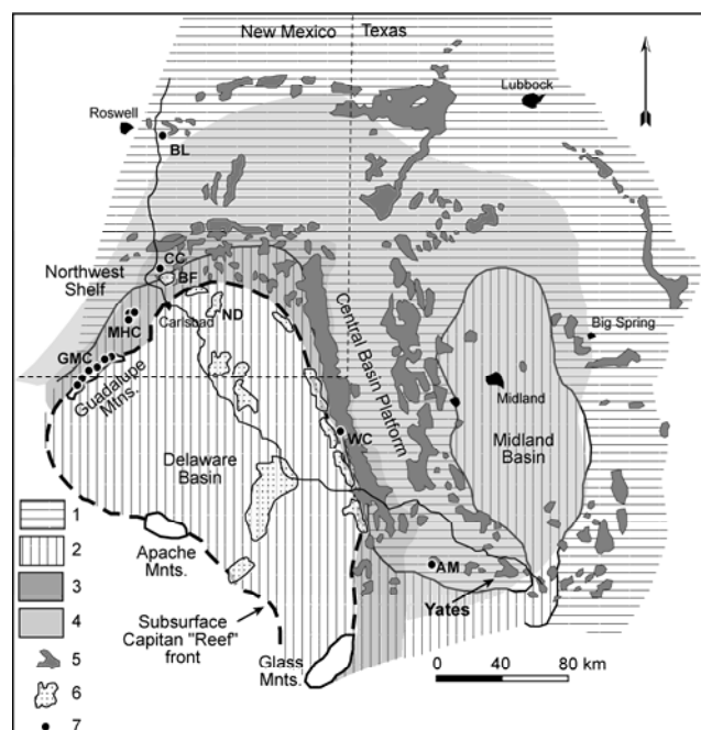
Figure 61. Distribution of oil and gas fields of west Texas and southeast New Mexico in relation to major features of regional geology and hypogenic karst. Compiled using data about regional geology features from Scholle et al. (2004) and oil and gas field distribution from Craig (1988) and Ward et al. (1986). Shading indicates distribution of Permian, lower Guadalupian depositional facies: 1 = San Andres limestone and dolomite; 2 = Lower Cherry Canyon & Brushy Canyon formations (basinal sandstone, siltstone & shale); 3 = Backreef dolomites and sandstones of Yates, Seven Rivers, & Queen formations; 4 = Evaporite facies. 5 = Oil and gas fields; 6 = Dissolution troughs in evaporites; 7 = Major features of hypogenic karst: BL = Bottomless Lakes; CC = Coffee Cave; BF = Burton Flat; ND = Nash Draw; MHC = McKittrick Hill caves; GMC = Guadalupe Mountains caves; WC = Wink Sink; AM = Amazing Maze Cave.
