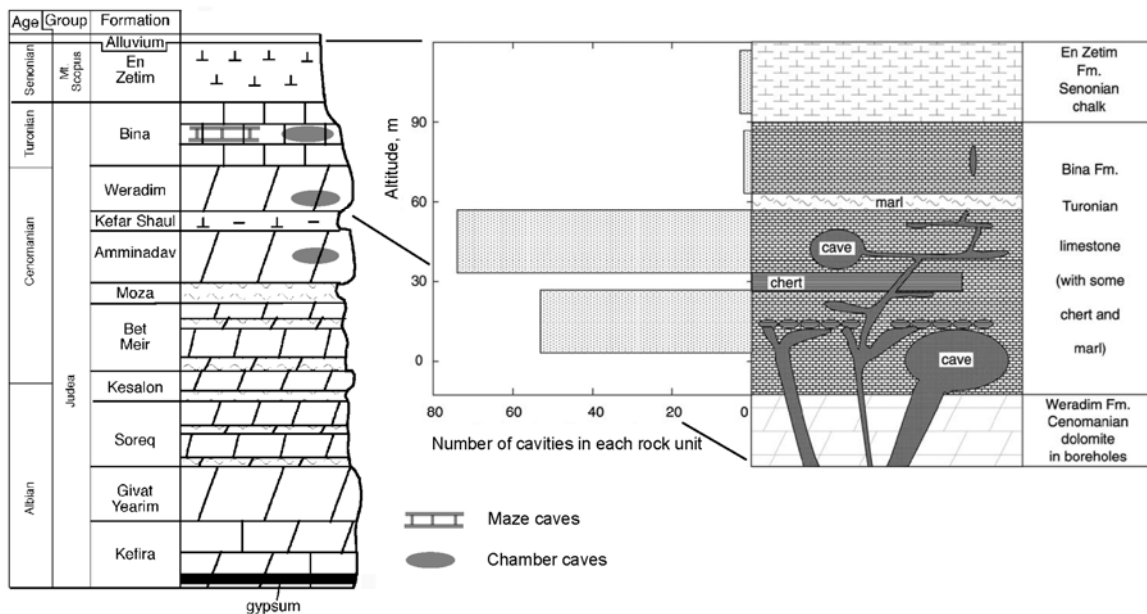
Figure 35. Stratigraphic section of Cretaceous formations in the Samaria Mountains, Israel (left) and a quarry in the confined zone (right) showing distribution of caves. The Judea Group consists of karstified dolomite and limestone with thin-bedded marl intercalations; Menuha Formation, composed of chalk and marl, is a confining unit. The histogram with the quarry section represents an arbitrary sample of voids encountered by the quarry from 1997 to 1999, the best available approximation of actual void frequency in the ASA zone in the confined flow area. Combined from Frumkin and Fischhendler (2005) and Frumkin and Gvirtzman (2006).
