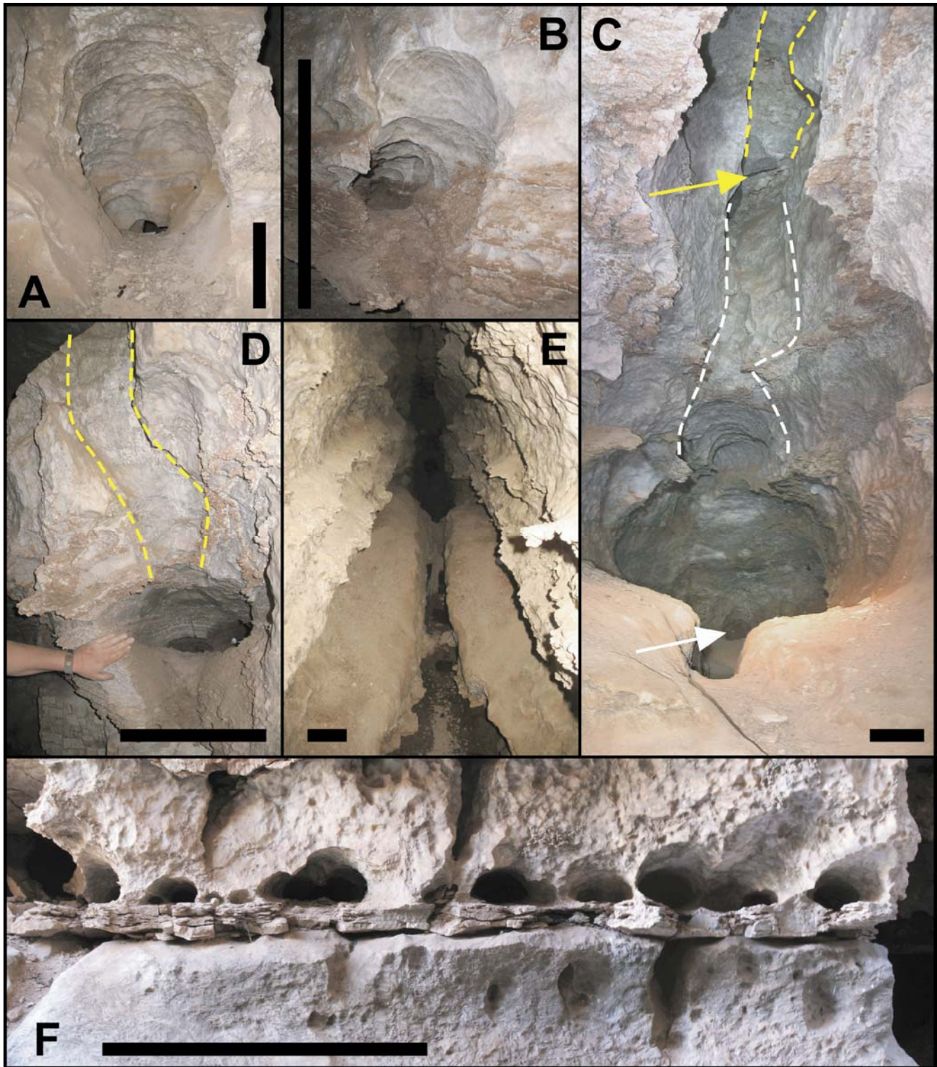
Plate 17. Hypogenic morphology in Coffee Cave, NM, USA (Permian gypsum): Feeder features (photos and compilation by K. Stafford, from Stafford et al., 2008). Black scale bars in figures are all approximately 0.5 m and camera angle is near-horizontal in all feeder features photos. A = point source feeder showing prominent doming morphology proximal to master passage; B = typical feeder showing development at the top of a dolomitic interbed; C = complete hypogenic morphologic suite showing riser (white arrow), wall channel (dashed white lines), ceiling channel (solid yellow lines) and outlet (yellow arrow); D = well developed wall riser with associated wall channel (dashed yellow lines); E = linear riser developed along axis of master passage; F) dense cluster of small feeders above dolomite interbed with minor vadose overprinting below dolomite interbed.
