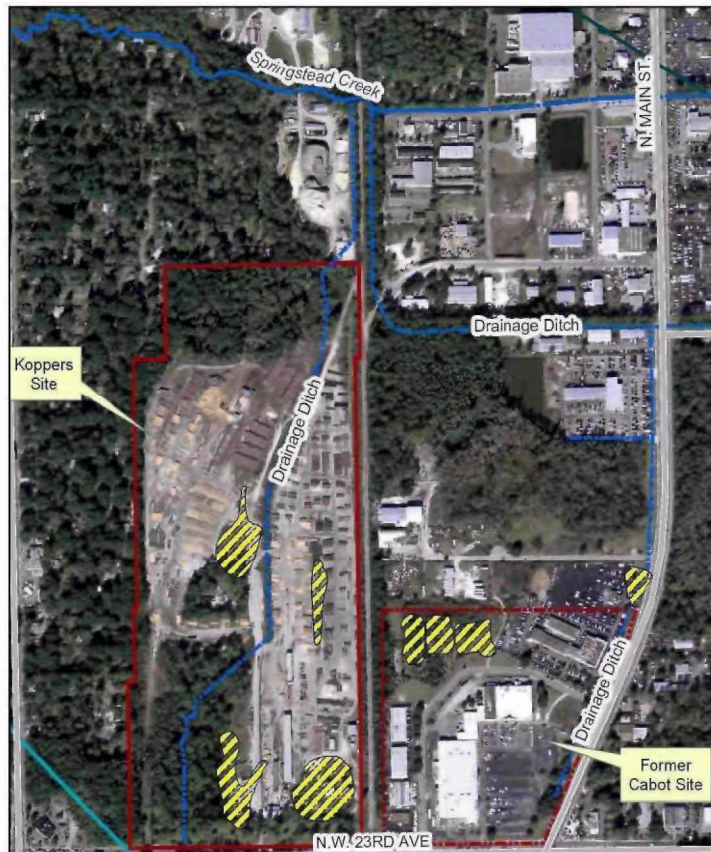
Figure 2.1 Site Layout
