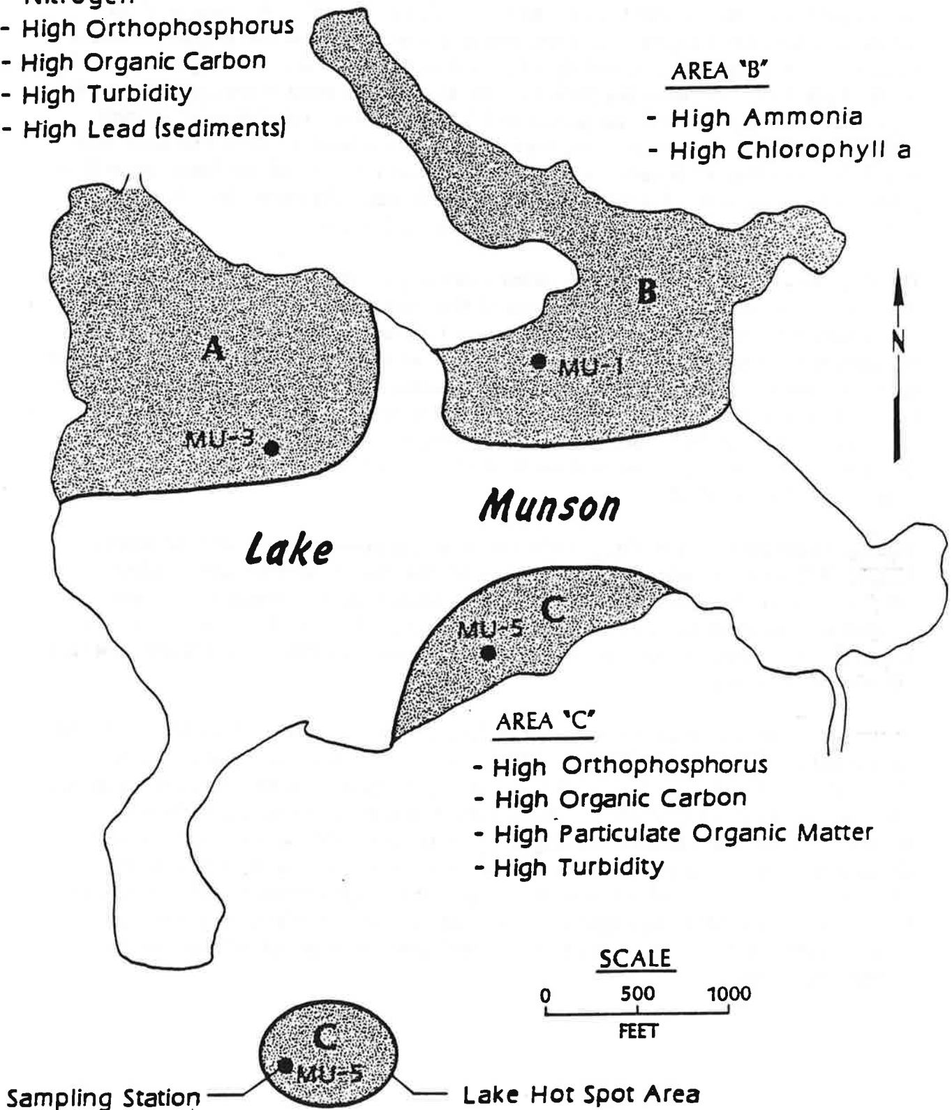
Figure 4. Lake Munson 'Hot Spots' Based on Extent and Nature of Adverse Environmental Indicators.
