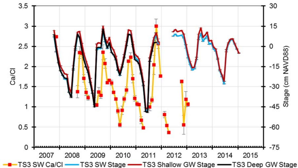
Figure 59: Monthly mean surface water (SW) stage, groundwater (GW) stages, and SW Ca/Cl ratio over time at TS3 with standard errors.
