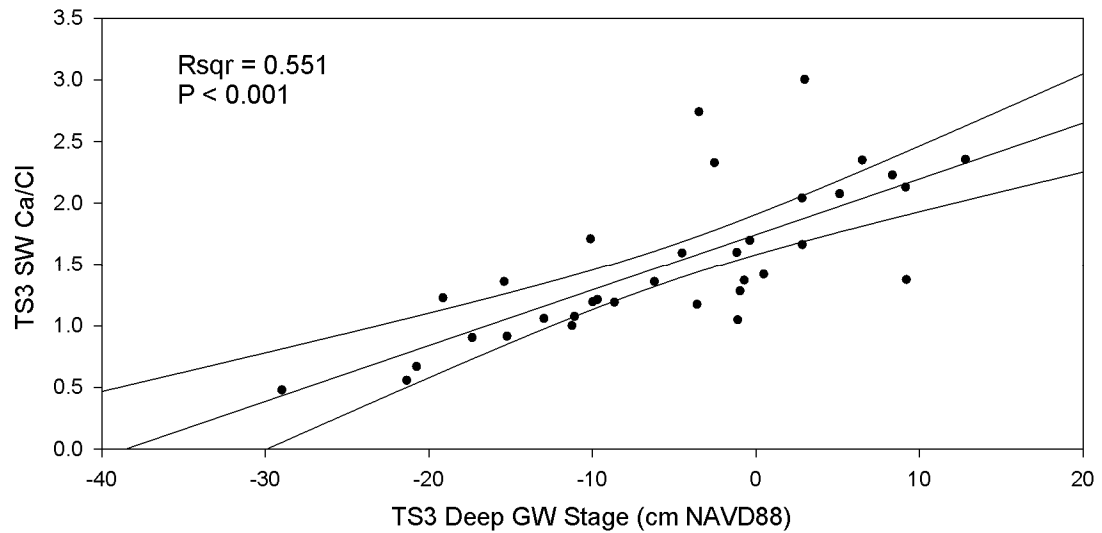
Figure 62: Linear regression with monthly mean deep groundwater (GW) stage and surface water (SW) Ca/Cl ratio over time at TS3. 95% confidence interval shown.
