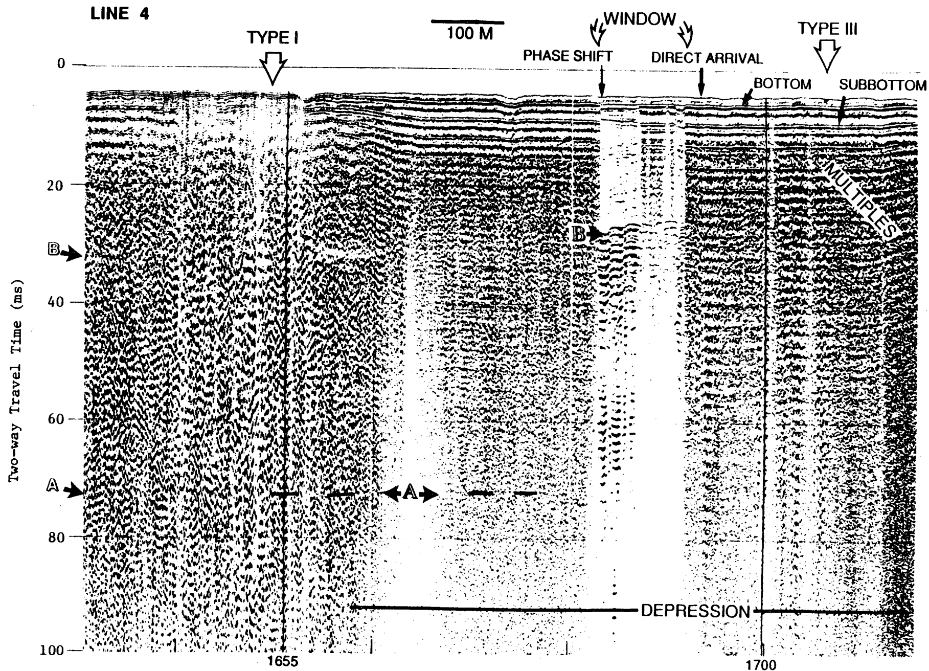
Figure 9. Section of seismic line 4 showing examples of reflection character types, a "window", and deep seismic horizons A and B. A clear phase shift in the reflected pulse is observed at the edge of the window. See Figure 2 for location.
