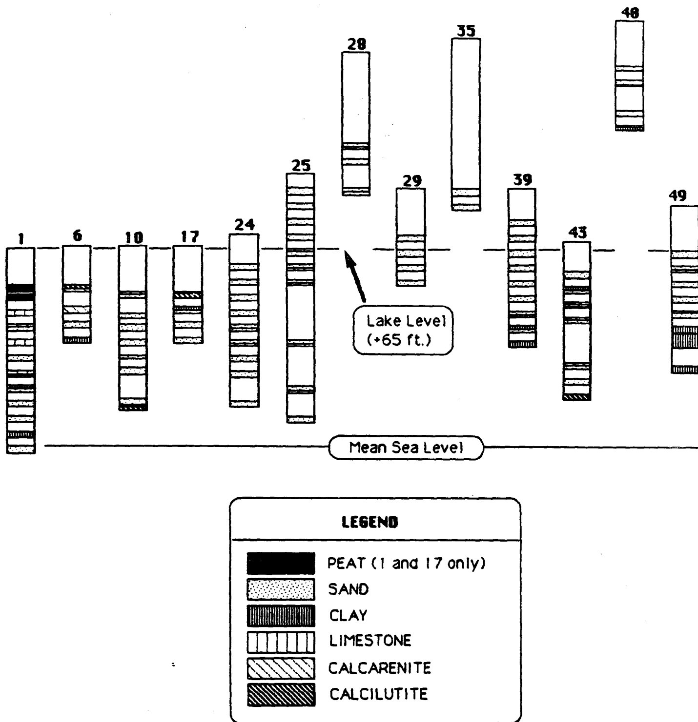
Figure 3. Shallow well data from sites around the perimeter of lake. These wells primarily sampled the upper zone of undifferentiated clastics and possibly the Hawthorn Formation.
