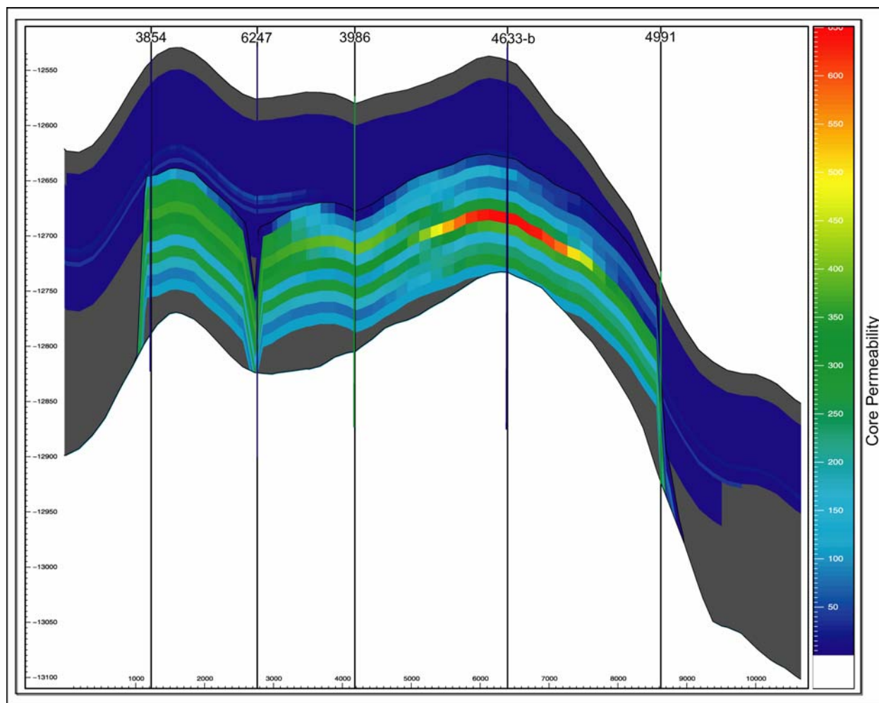
Figure 257 –Cross section showing permeability at Appleton Field.
