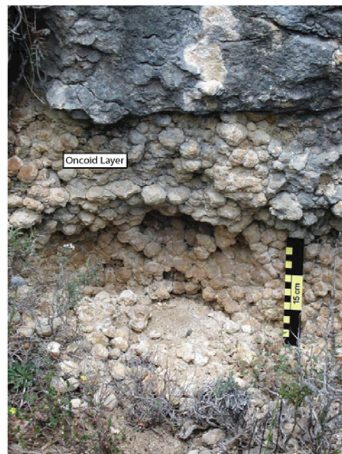
Figure 333. Outcrop photographs showing: (A) encrusted and cemented surface on which reef growth initiated, Arroyo Cerezo (AC), (B) close-up of the encrusted and cemented surface, Arroyo Cerezo (AC), (C) post-reef facies of grainstone and packstone, Barranco de las Balsillas (BB), and (D) oncolite layer, part of the post-reef facies, Tormón (TO).
