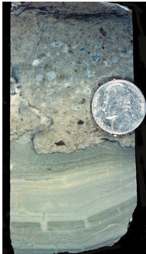
Figure 326. Core photographs of Smackover microbolite mesostructure: (A) chaotic thrombolite, well Permit #2935, depth 4.308 m (14,135 ft), Vocation Field, (B) stromatolite, well Permit #3739, depth 4,287 m (14,066 ft), Vocation Field.
