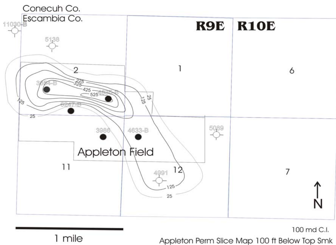
Figure 94. Appleton Permeability Slice Map 100 ft below Top of Smackover.
