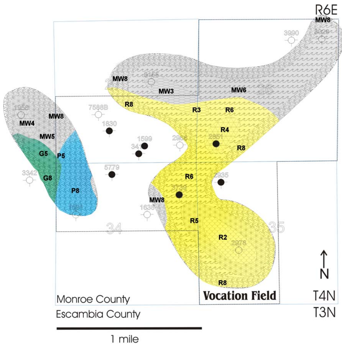
Vocation Flow Unit Slice Map 100 ft Below Top of Smackover
