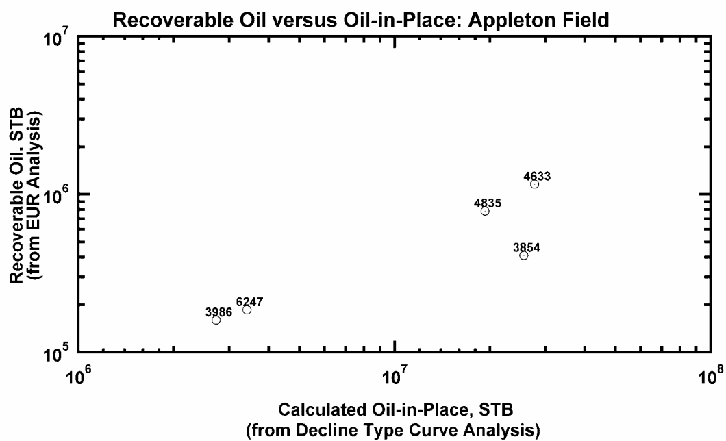
Fig. 163 — Recoverable Oil ( EUR Analysis) versus Computed Original Oil-in-Place (Decline Type Curve Analysis), Appleton Oil Field.
