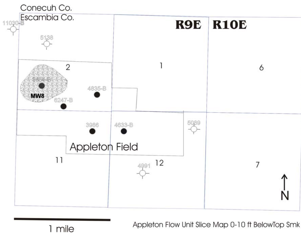
Figure 105. Appleton Flow Unit Slice Map 0-10 ft below Top of Smackover.
