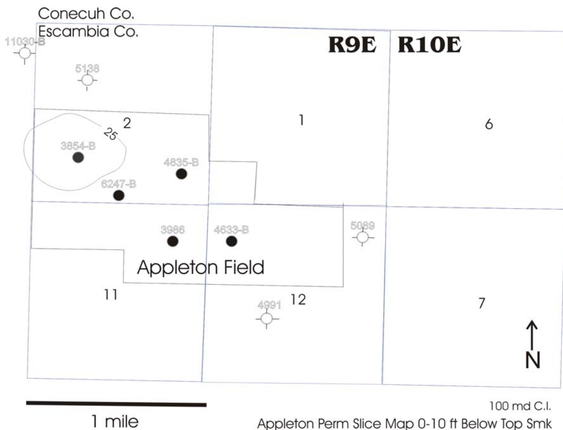
Figure 92. Appleton Permeability Slice Map 0-10 ft below Top of Smackover.
