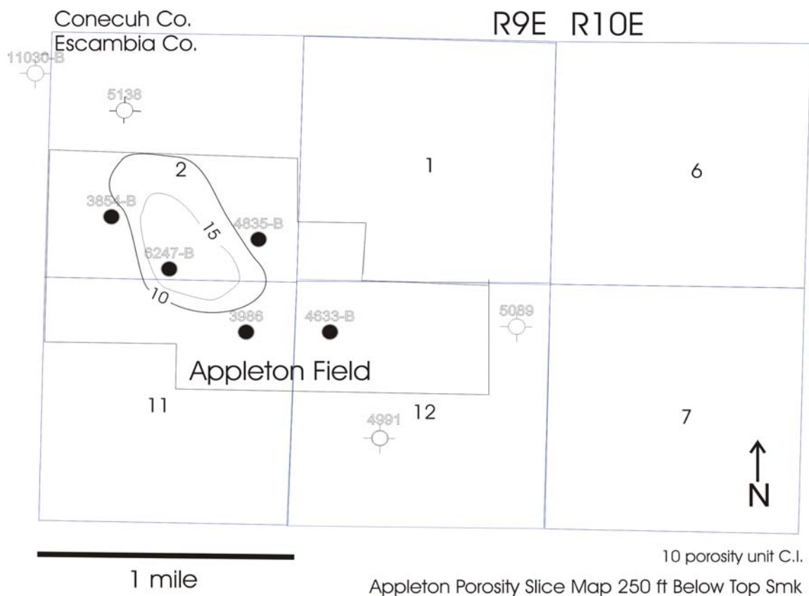
Figure 85. Appleton Porosity Slice Map 250 ft below Top of Smackover.
