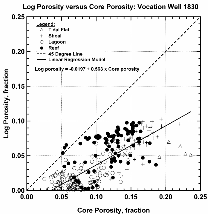
Figure 201 — Log Porosity versus Core Porosity, Vocation Well 1830.
