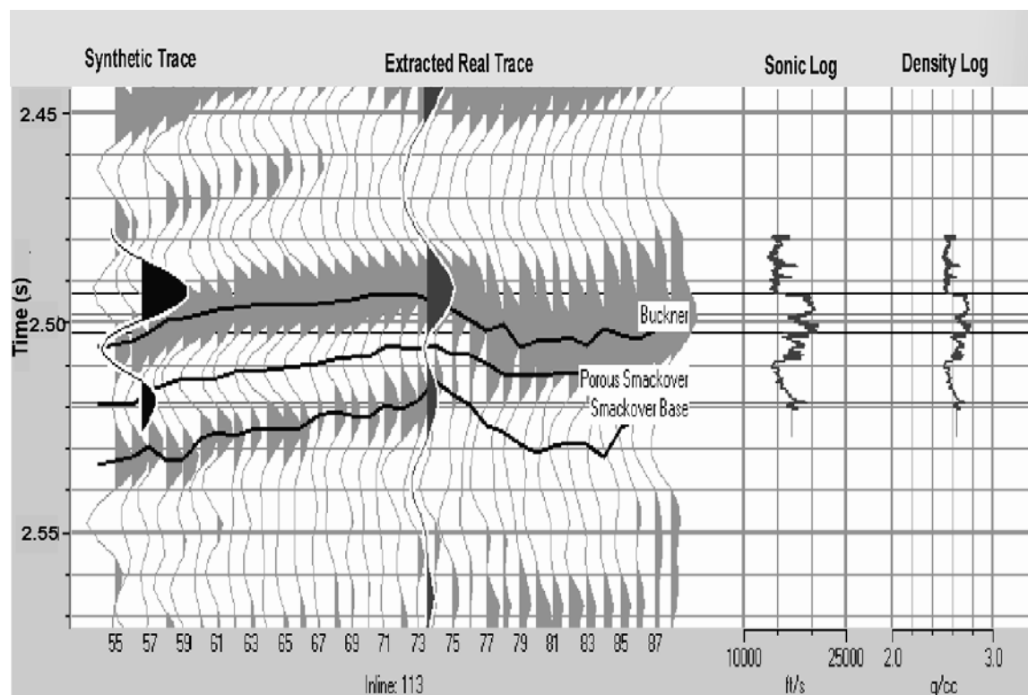
Figure 45: Example of synthetic seismogram (well 4633-B) used for tying well data to seismic. Black curve = log synthetic, grey = seismic trace extracted along wellbore at well location.
