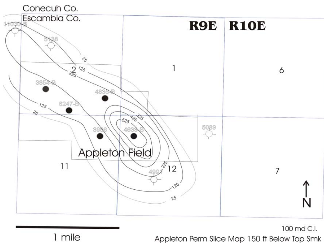
Figure 95. Appleton Permeability Slice Map 150 ft below Top of Smackover.
