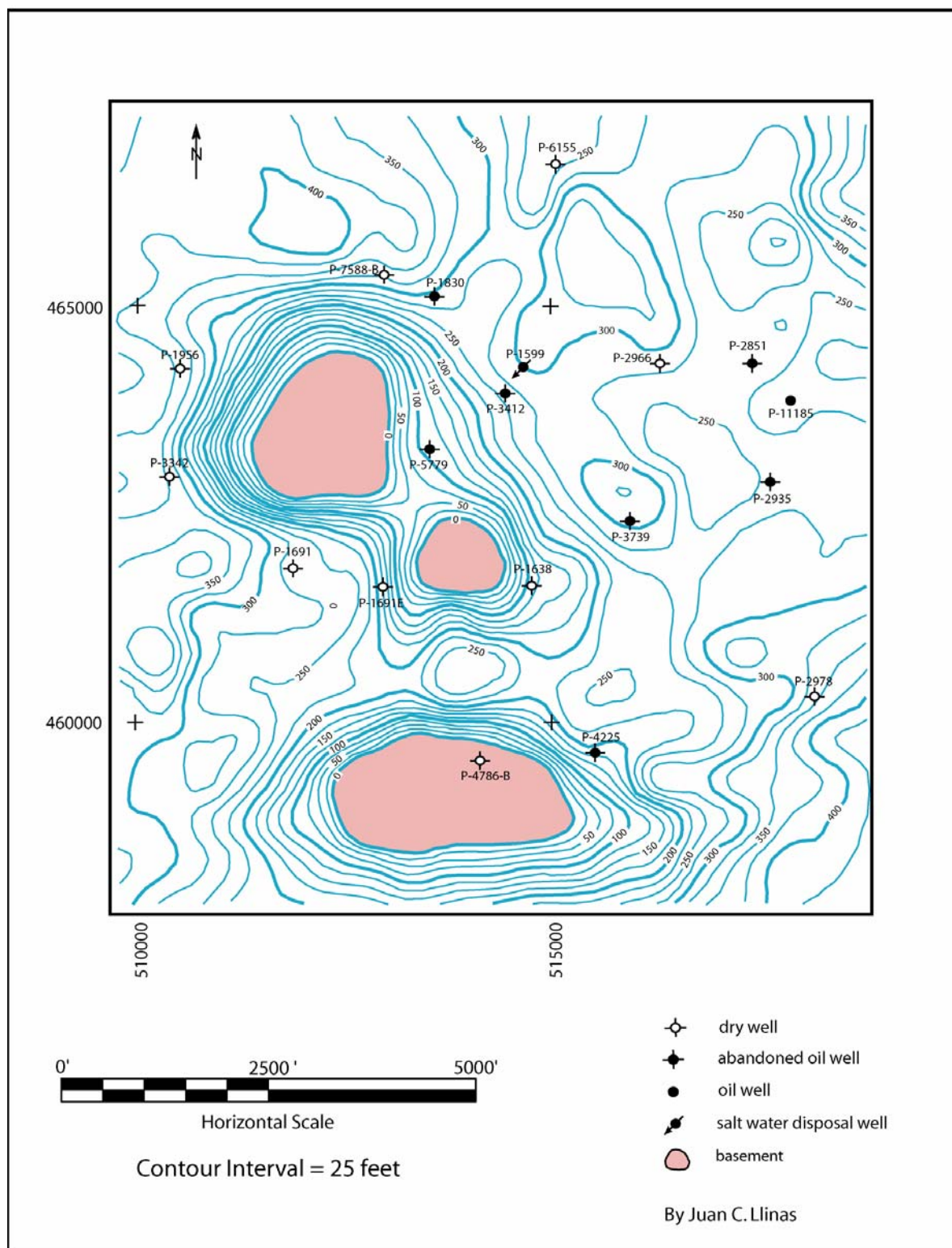
Figure 40. Isopach map of the Smackover Formation.
