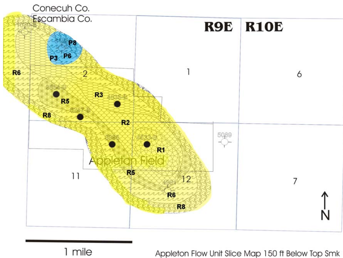
Figure 108. Appleton Flow Unit Slice Map 150 ft below Top of Smackover.
