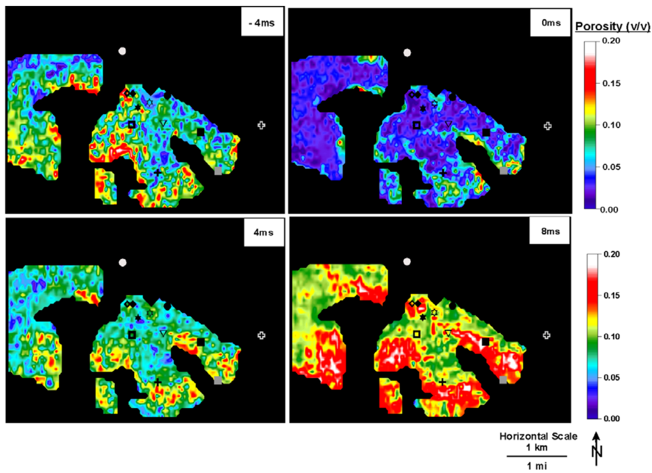
Figure 54: Slices through the porosity volume (porosity values are in decimals (v/v) i.e., volume of voids/total volume of rock, and not percentages), starting 4 ms above the porous Smackover pick. Porosity at -4ms above this pick was attributed to shoal grainstone facies, which constitute the other major reservoir facies in the Appleton Field. Note the overall association of higher porosities (hot colors) with the southern (paleoseaward) flanks of structure, which we attribute primarily to changes in facies type and growth form. Well symbols are indicated in Figure 43 and 48.
