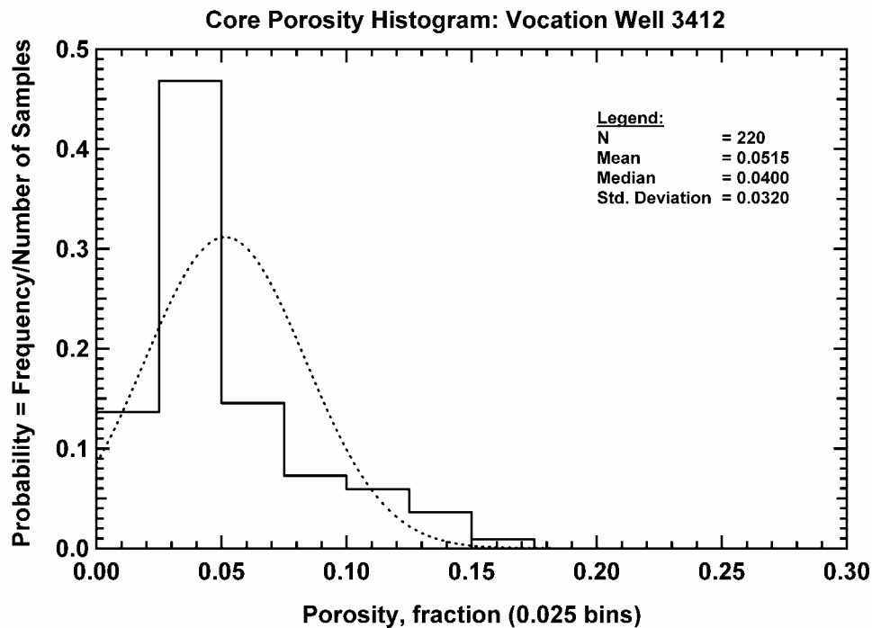
Figure 177 — Core Porosity Histogram, Vocation Well 3412.
