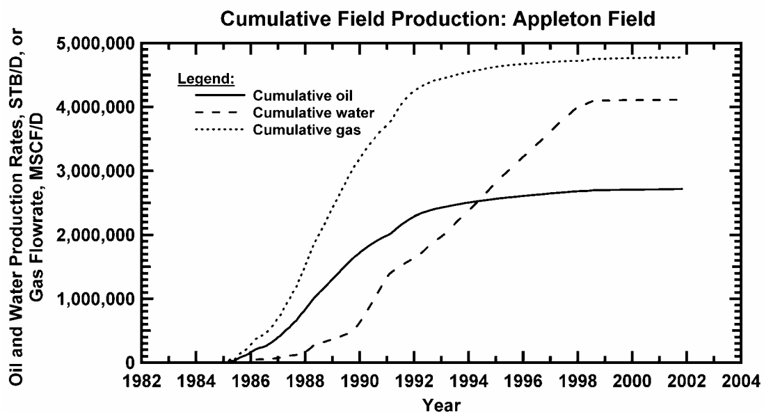
Figure 271 — Cumulative Production Profiles, Appleton Field.
