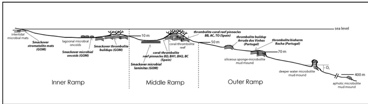
Figure 336. Generalized diagram illustrating the distribution of microbial buildups on a carbonate ramp (modified from Leinfelder, 1993b and Leinfelder and Schmid, 2000). Note inner to middle ramp settings for Upper Jurassic Smackover microbial growth in the northeastern Gulf of Mexico (GOM), middle ramp setting for the Upper Jurassic pinnacle reef development in northeastern Spain, and outer ramp setting for Upper Jurassic thrombolite buildups in Portugal.
