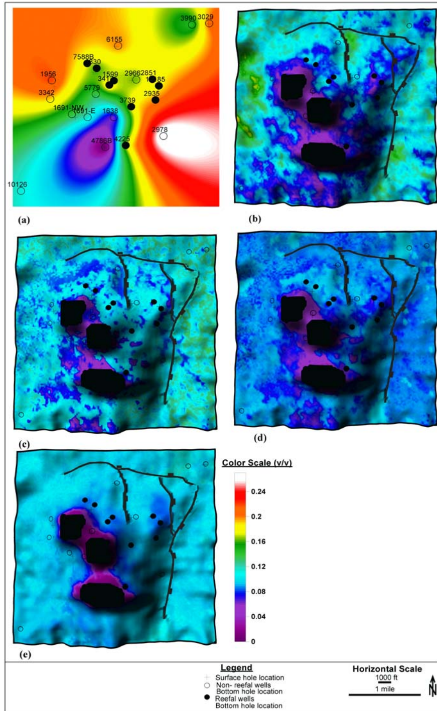
Figure 71: Maps showing the maximum porosity for the Smackover Formation. a) based only on contouring of well data, b) MLR result, c) MLR trend-cascaded PNN result, d) conventional PNN result, e) MLFN result. Note how low these are compared to actual porosity values at well locations.
