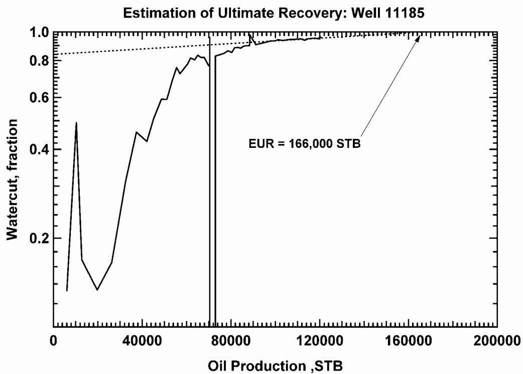
Figure 241 — Alternative Calculation of Recoverable Oil, Vocation Well 11185.
