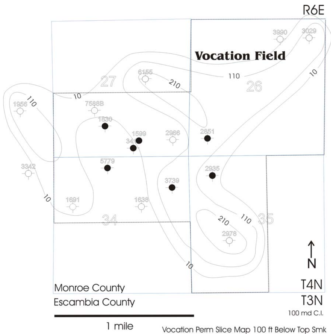
Figure 100. Vocation Permeability Slice Map 100 ft below Top of Smackover.
