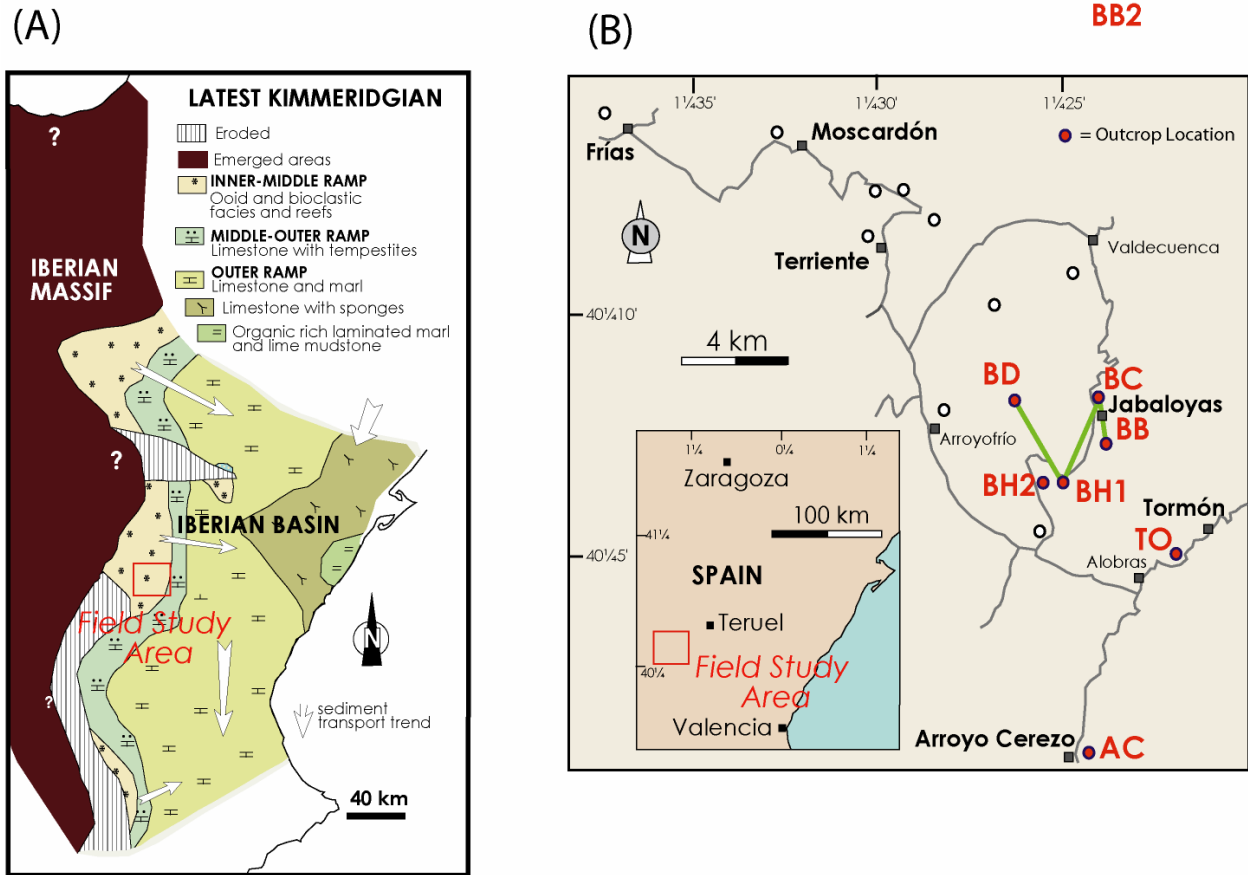
Figure 329. (A) Paleographic map of the Iberian Basin during the latest Kimmeridgian, and location of the field study area, and (B) location of the key pinnacle reef outcrops studied in the Sierra de Albarracín. BD=Barranco del Diablo, BC=Barranco del la Canaleja, BB=Barranco de las Balsillas, BH1 and BH2=Barranco de la Hoz, TO=Tormón, AC=Arroyo Cerezo (modified from Aurell and Bádenas, 1997).
