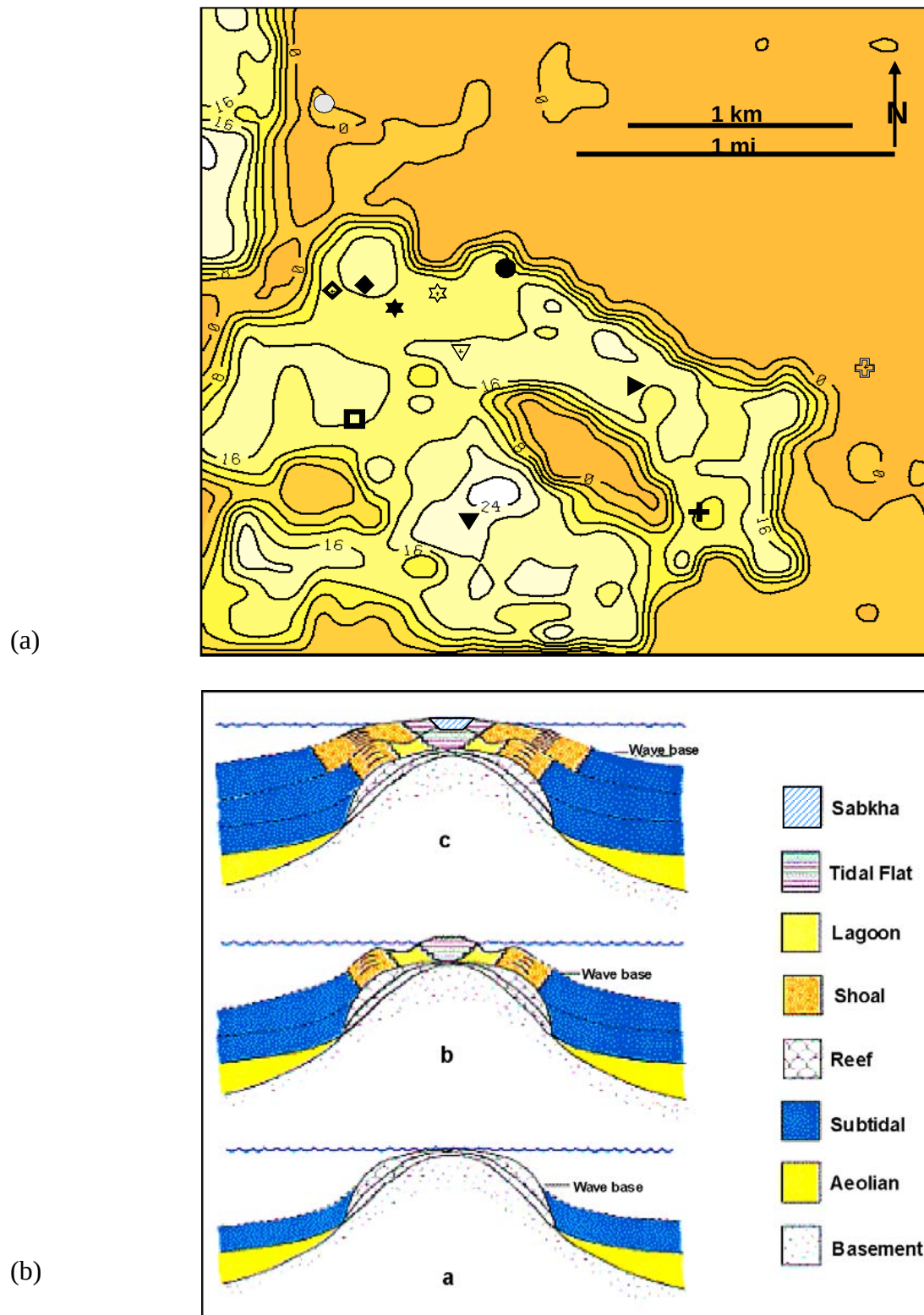
Figure 56: Existing models for the Appleton field. (a) Model of Hart and Balch (2000) depicting porosity distribution in the porous unit of the Smackover Formation, Appleton Field. Map created using a horizon-based seismic attribute study. (b) Model by Mancini et al , 1999. This illustrates facies distribution as a function of water depth on the basement paleohigh.
