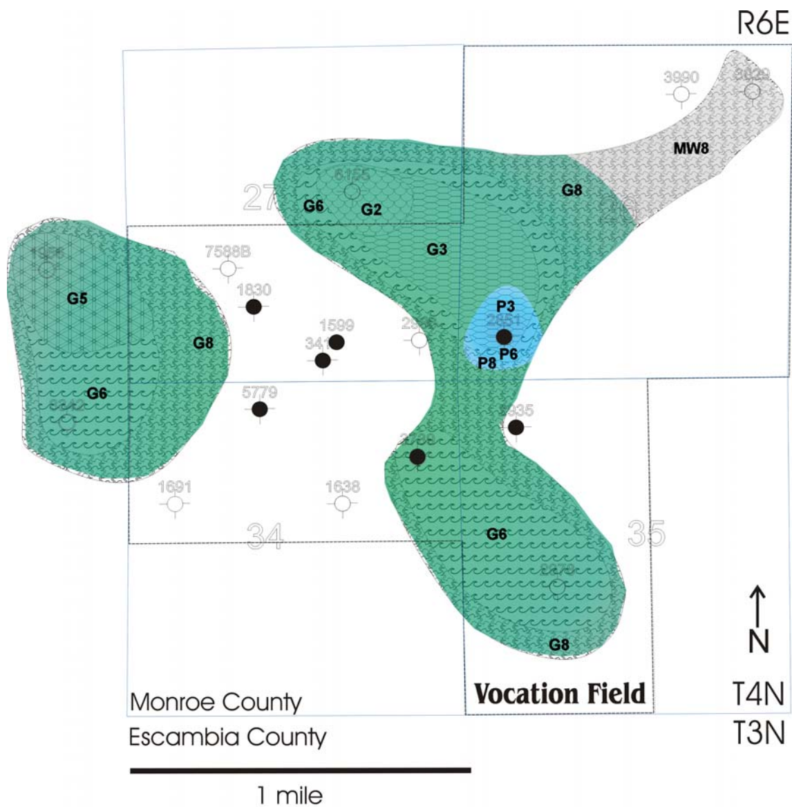
Vocation Flow Unit Slice Map 50 ft Below Top Smk
