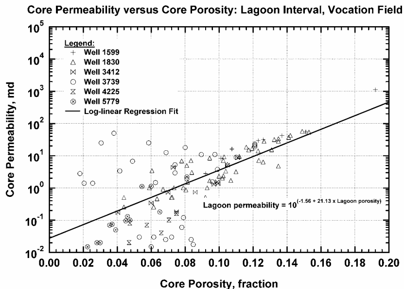
Figure 219 — Core Permeability versus Core Porosity, Lagoon.
