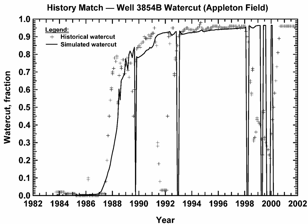
Figure 277 — Watercut history match, Well 3854B (Appleton Field).
