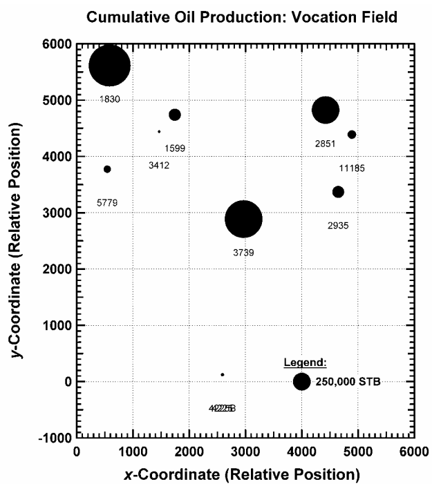
Figure 289 — Oil Production as a Function of Well Location, Vocation Field.
