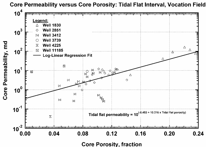
Figure 217 — Core Permeability versus Core Porosity, Tidal Flat.
