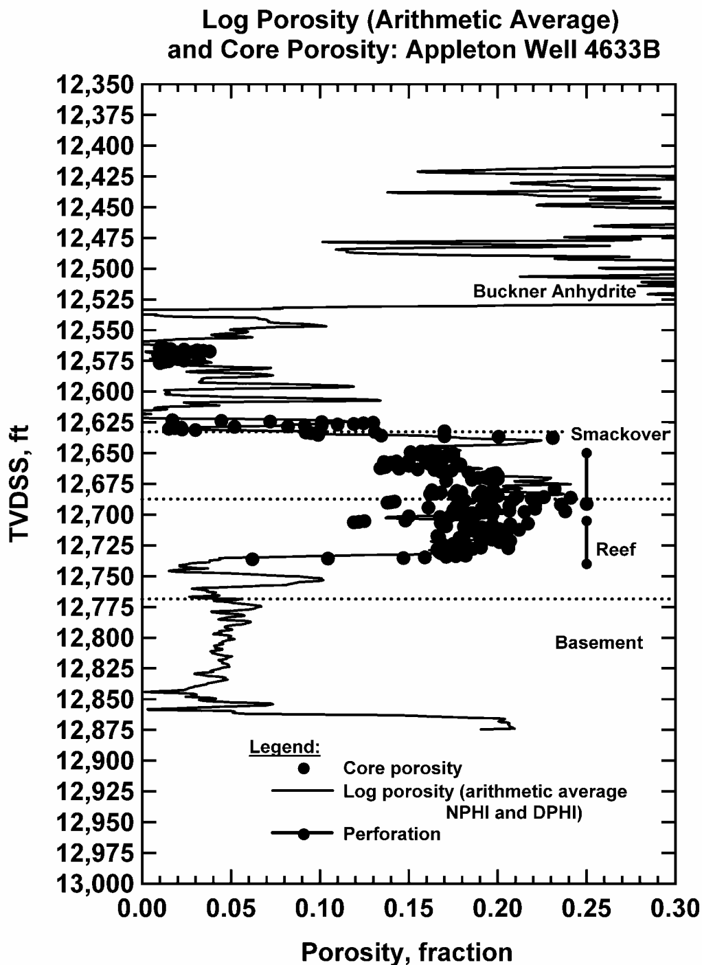
Fig. 140 — Porosity Variation with Depth, Appleton Well 4633B
