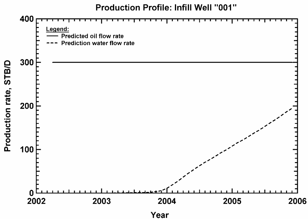
Figure 316 — Oil and water production rates, proposed infill well 001, Vocation Field.
