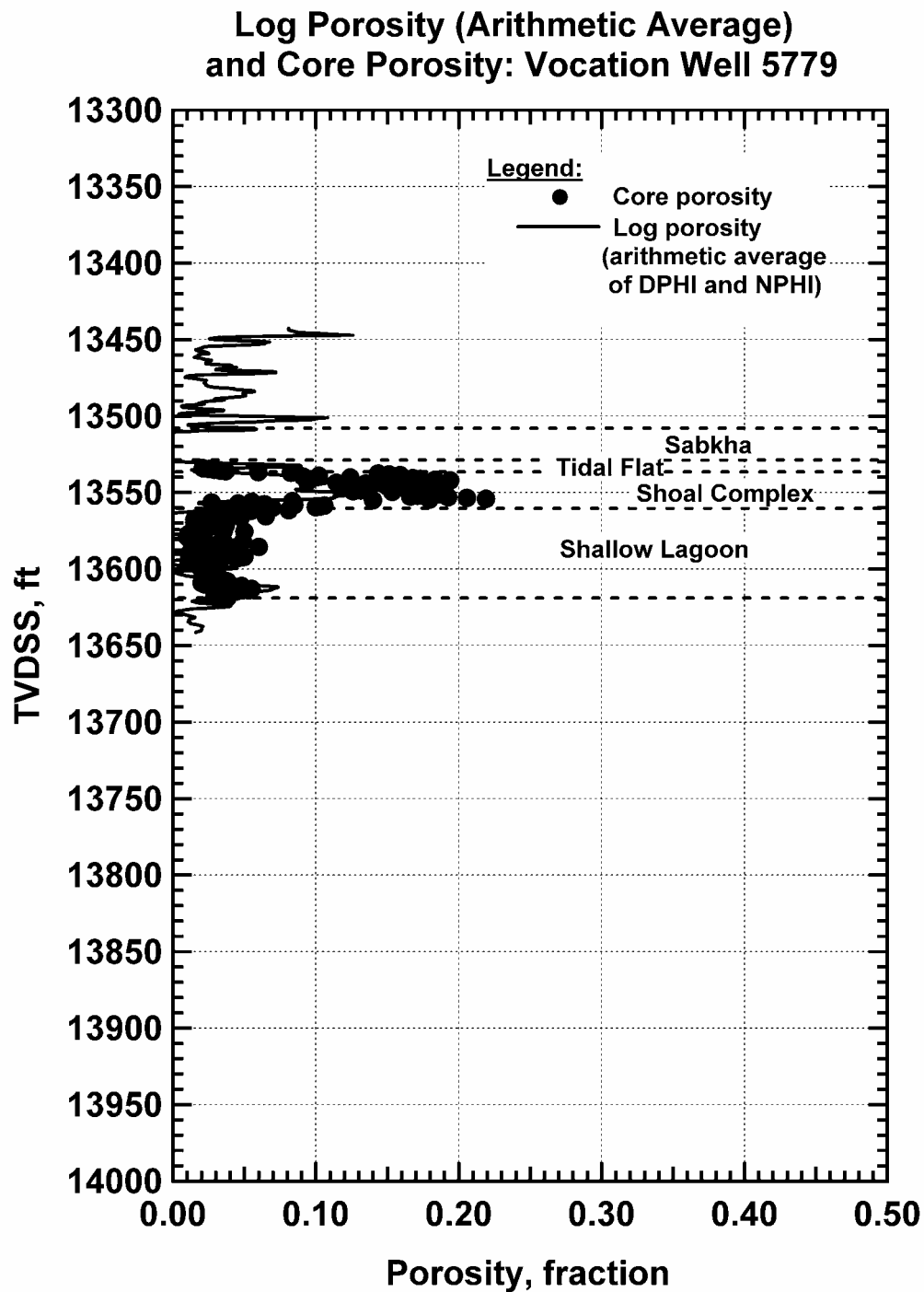
Figure 198 — Porosity Variation with Depth, Vocation Well 5779.
