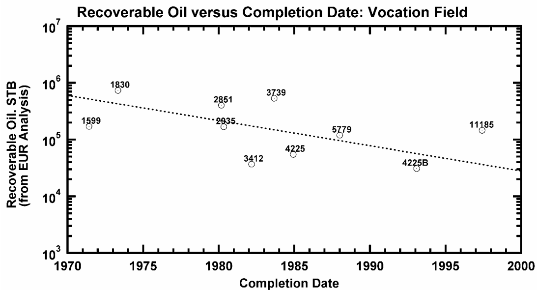
Figure 244 — Recoverable Oil versus Completion Date, Vocation Oil Field.
