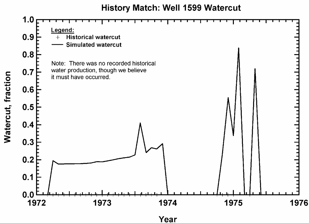
Figure 299 — Watercut history match, Vocation Well 1599.
