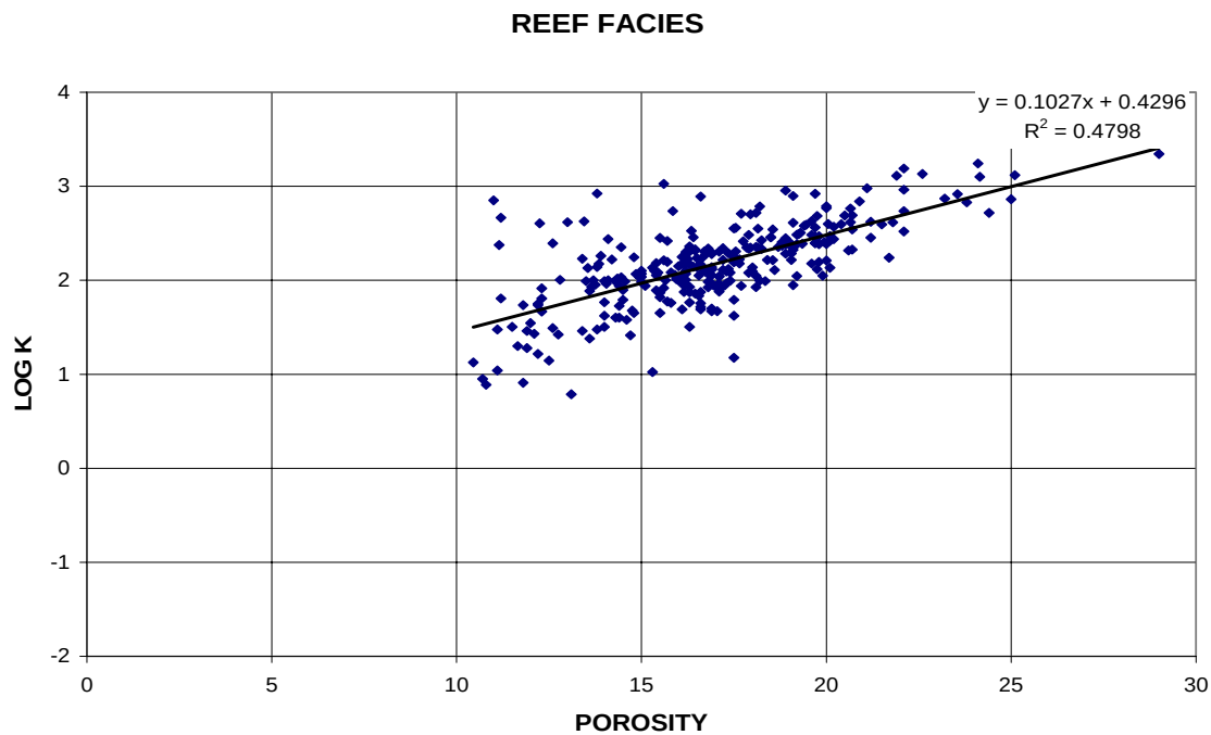
Figure 123. Porosity-permeability plot showing correlation to rock type in Appleton field.
