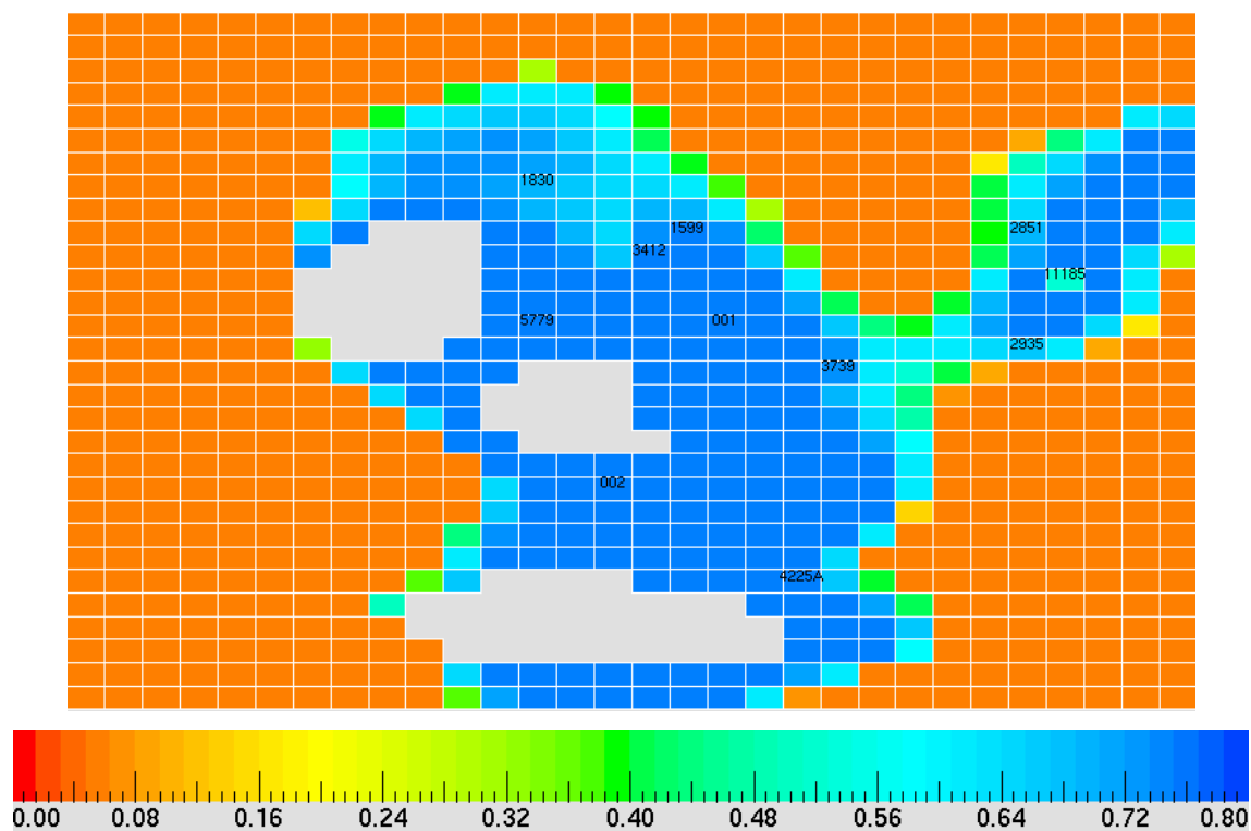
Figure 313 — Oil saturation in top simulation layer 2001, Vocation Field.
