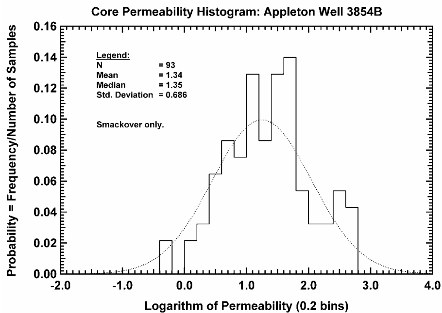
Fig. 133 — Core Permeability Histogram, Appleton Well 3854B
