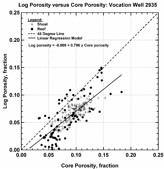
Figure 203 — Log Porosity versus Core Porosity, Vocation Well 2935.
