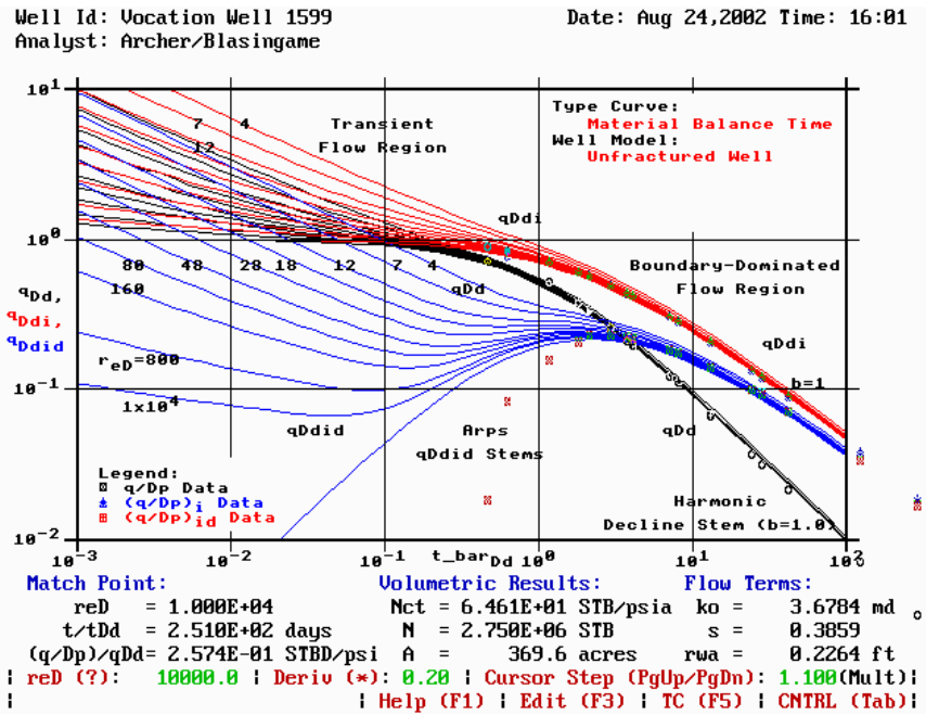
Figure 221 — Type Curve Match, Vocation Well 1599.
