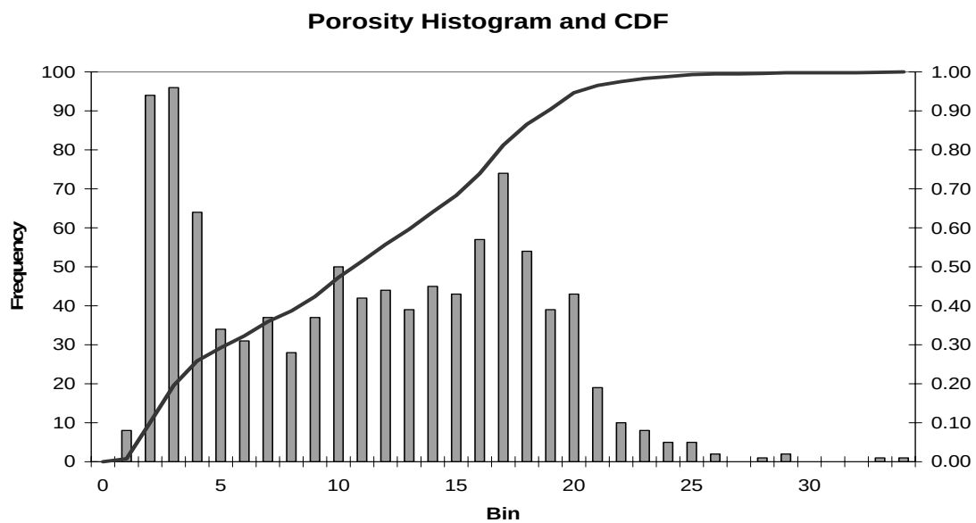
Figure 117. Histogram of porosity distribution and cumulative distribution frequency (CDF) in Appleton and Vocation fields.
