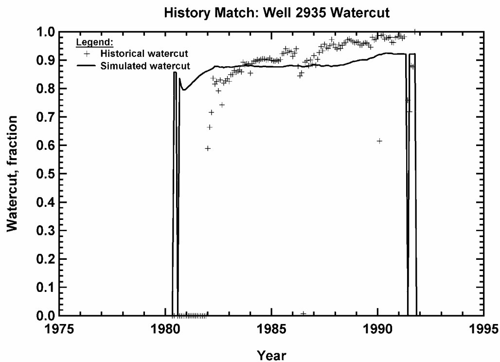
Figure 302 — Watercut history match, Vocation Well 2935.
