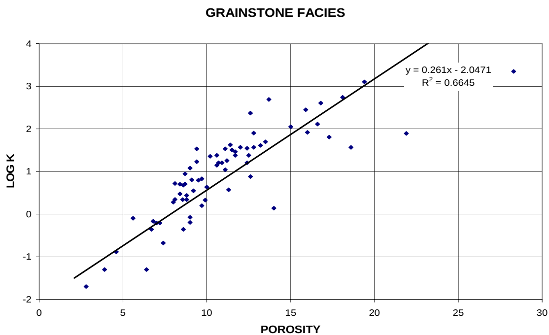
Figure 126. Porosity-permeability plot showing correlation to rock type in Vocation field.
