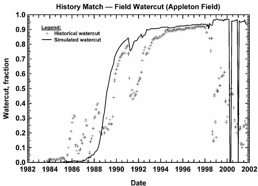
Figure 273 — Fieldwide watercut history match, Appleton Field
