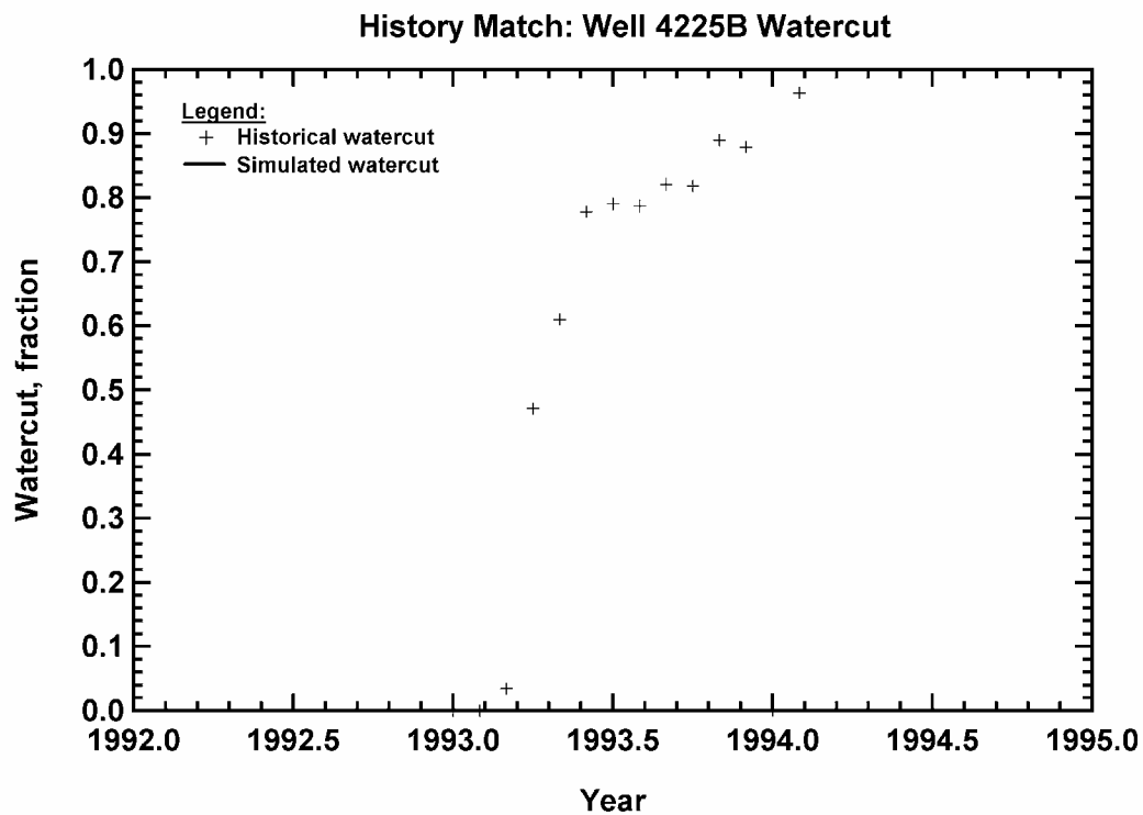
Figure 306 — Watercut history match, Vocation Well 4225B.
