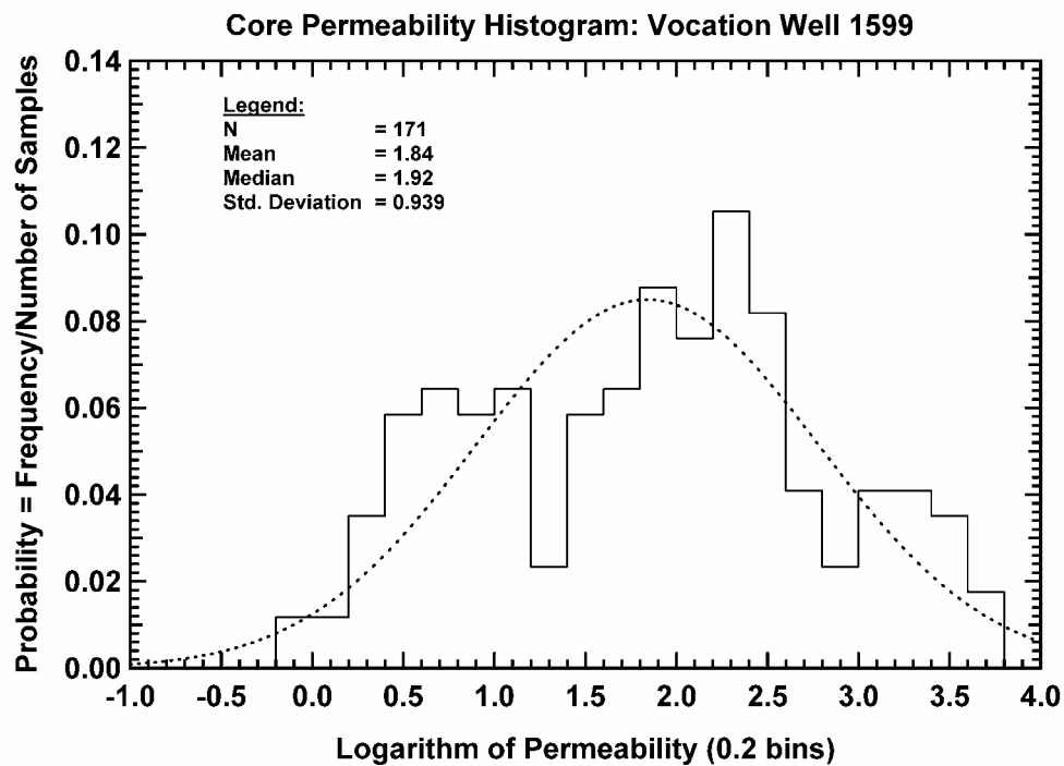
Figure 182 — Core Permeability Histogram, Vocation Well 1599.
