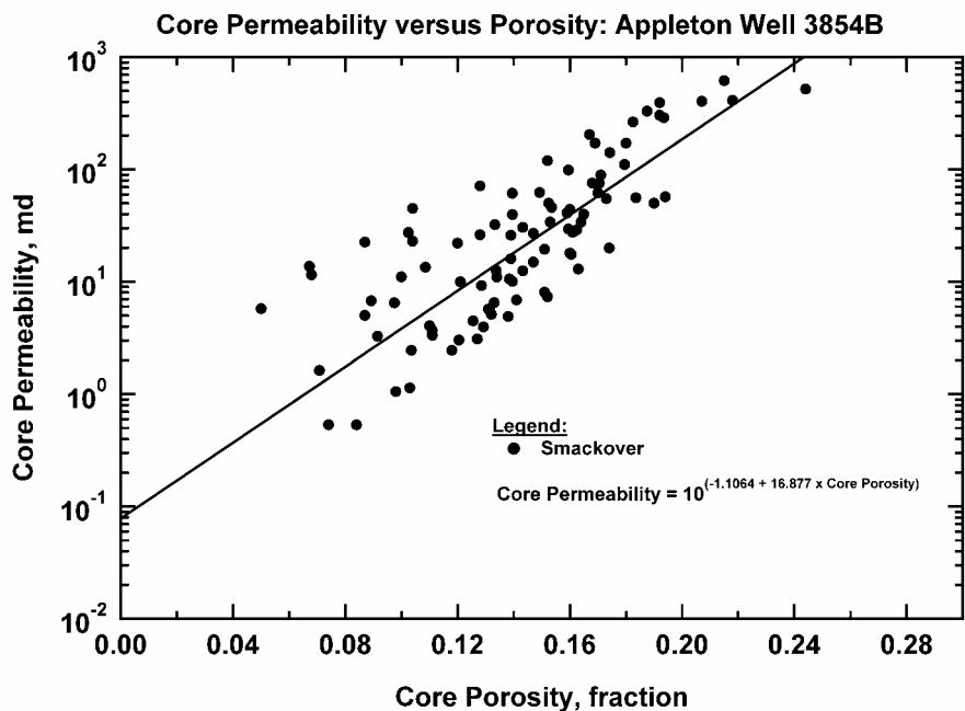
Fig. 148 — Core Permeability versus Core Porosity, Appleton Well 3854B.
