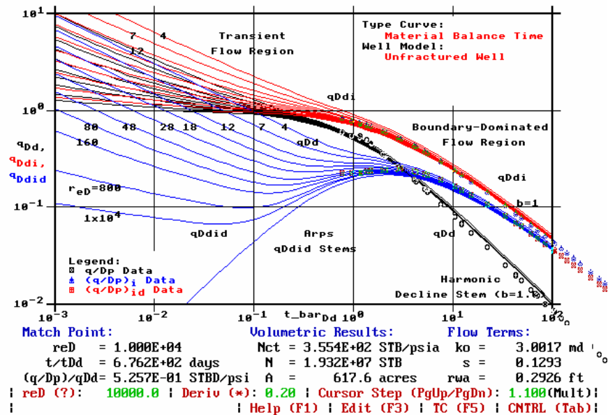
Fig. 156 — Type Curve Match, Appleton Well 4835B.
