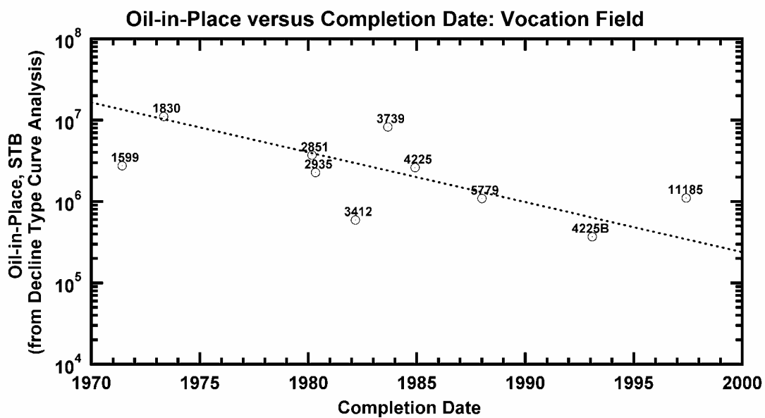
Figure 243 — Computed Original Oil-in-Place versus Completion Date, Vocation Oil Field.
