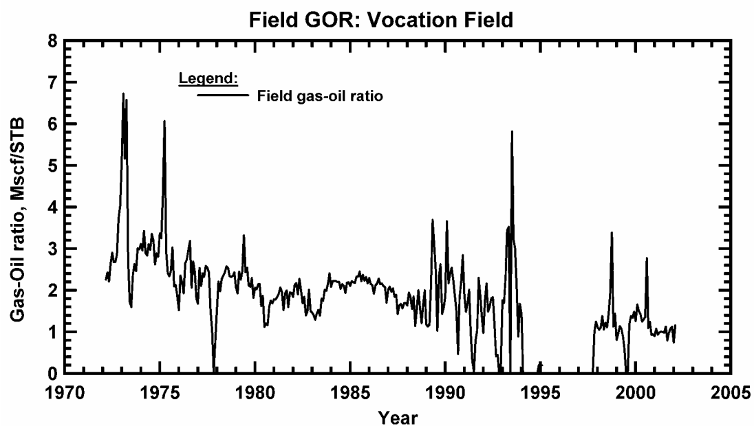
Figure 294 — Gas-Oil Ratio Profile, Vocation Field.
