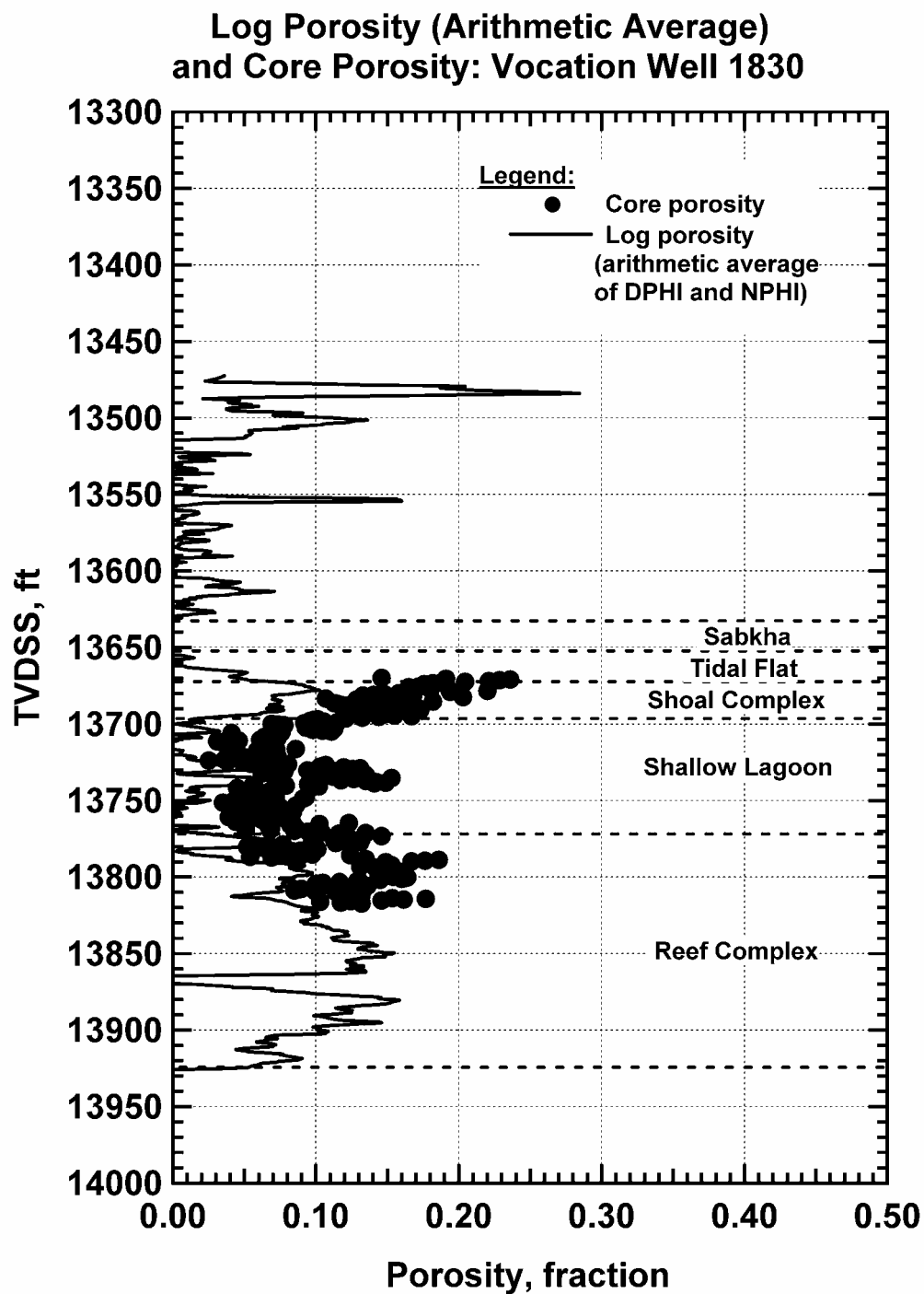
Figure 192 — Porosity Variation with Depth, Vocation Well 1830.
