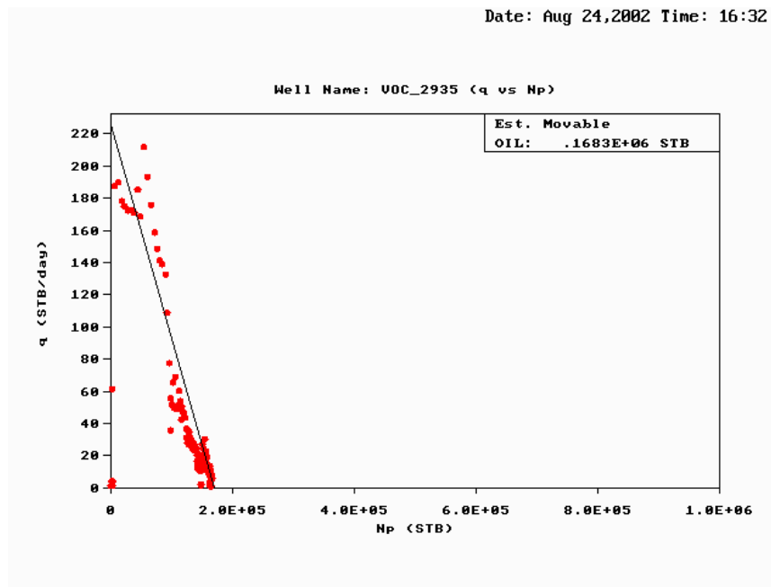
Figure 234 — Calculation of Recoverable Oil, Vocation Well 2935.
