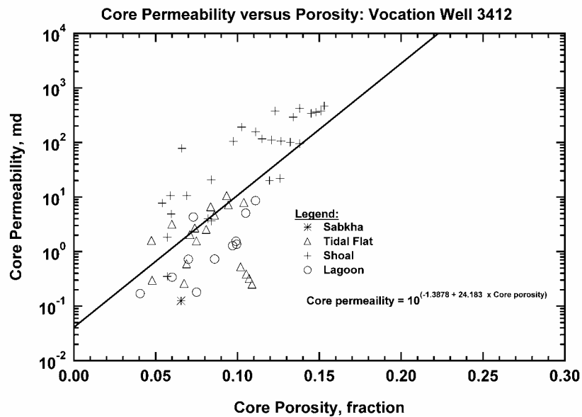
Figure 213 — Core Permeability versus Core Porosity, Vocation Well 3412.
