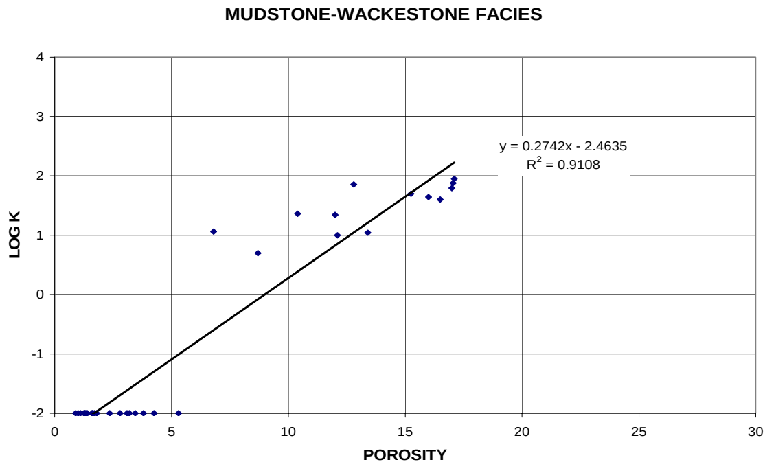
Figure 120. Porosity-permeability plot showing correlation to rock type in Appleton field.
