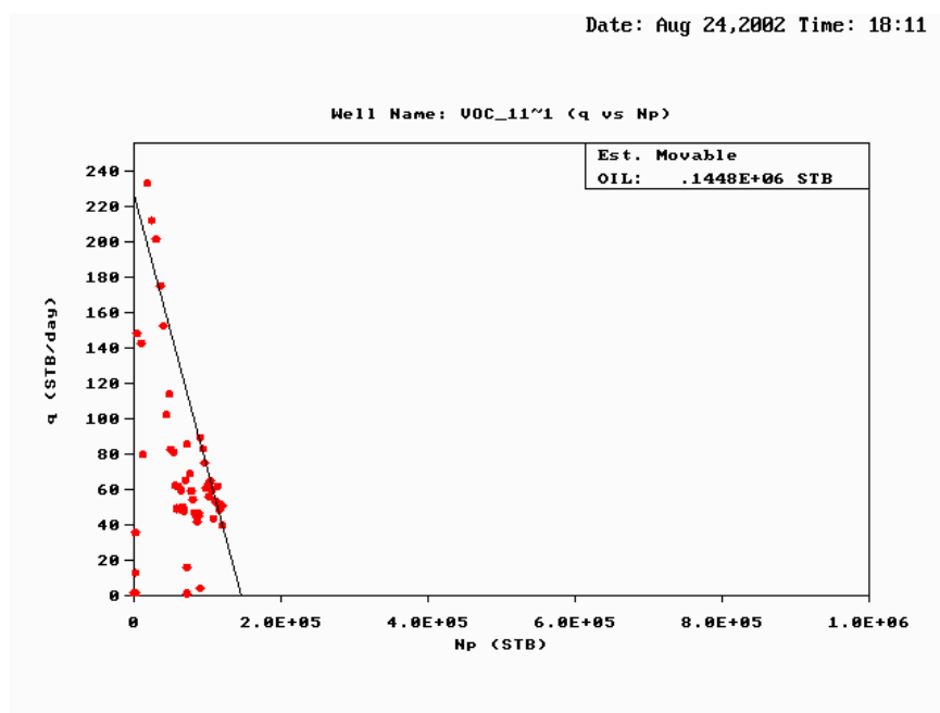
Figure 240 — Calculation of Recoverable Oil, Vocation Well 11185.
