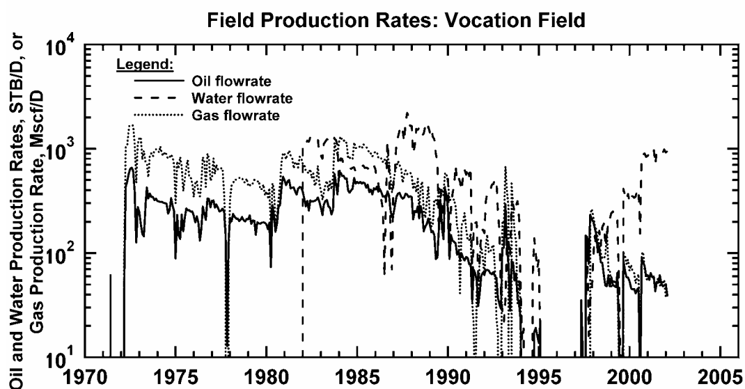
Figure 292 — Individual Phase Flowrates, Vocation Field (Semilog Format).
