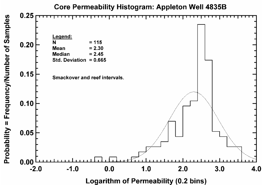
Fig. 136 — Core Permeability Histogram, Appleton Well 4835B
