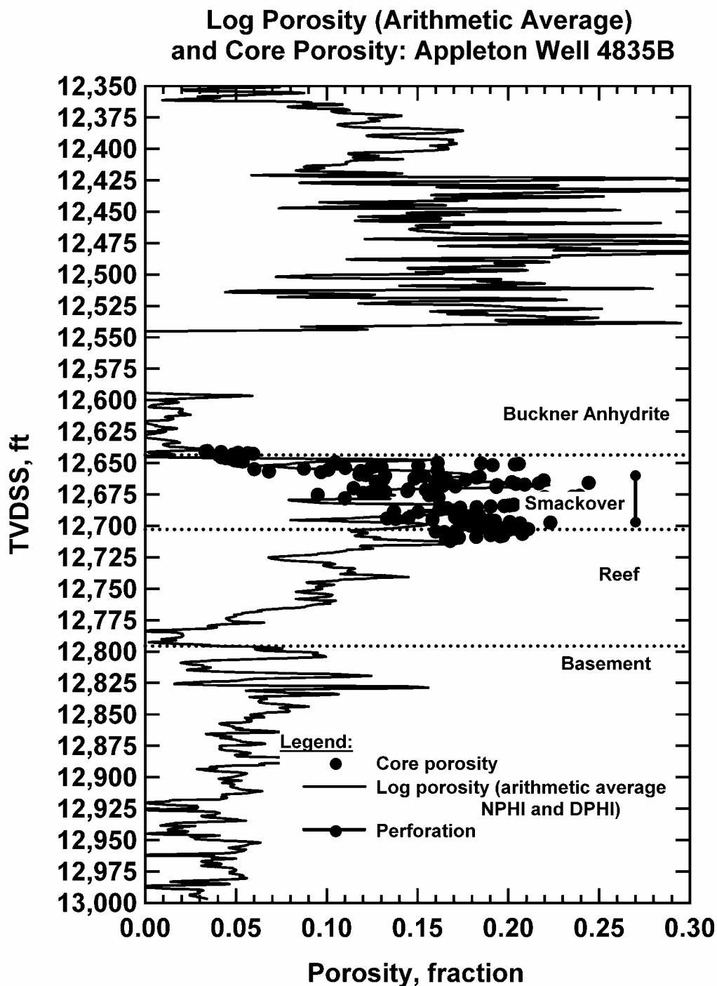
Fig. 141 — Porosity Variation with Depth, Appleton Well 4835B
