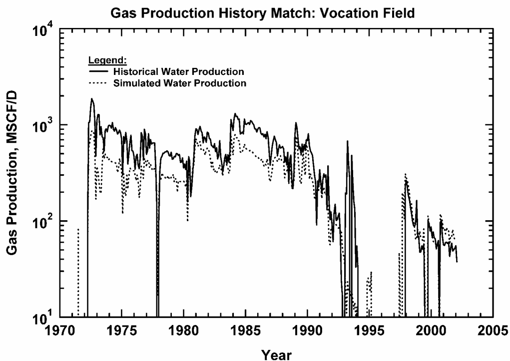
Figure 298 — Gas Production Rate History Match, Vocation Field.
