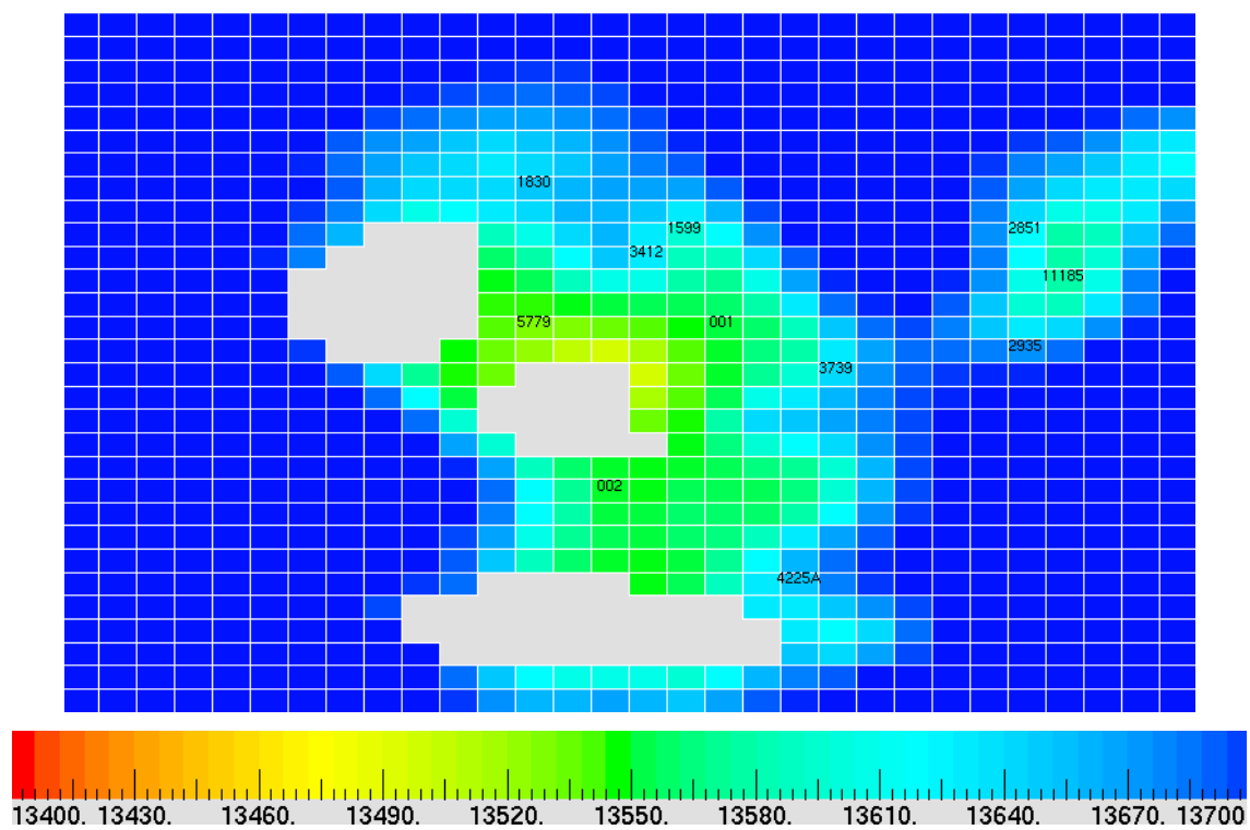
Figure 315 — Map showing well locations and depth to reservoir top, Vocation Field.
