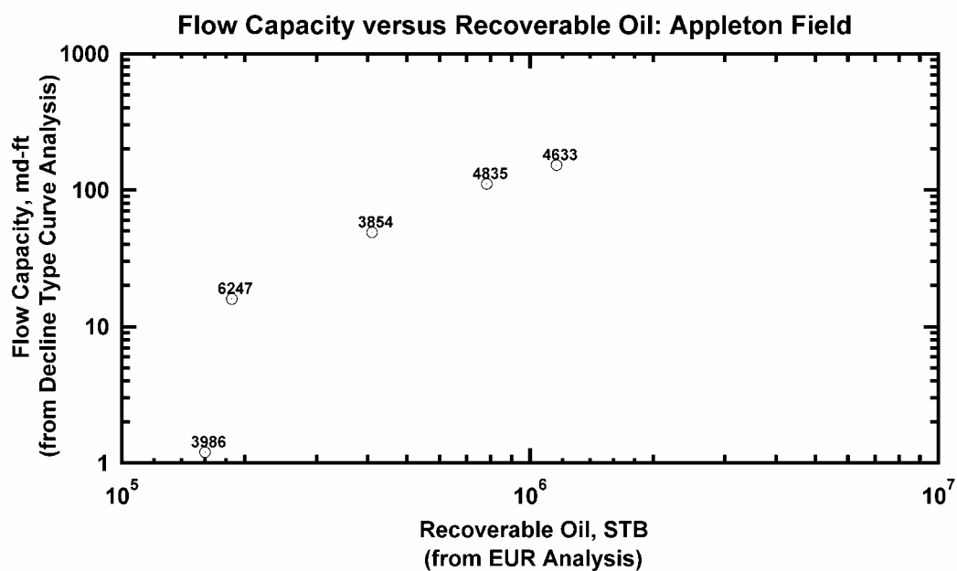
Fig. 167 — Flow Capacity versus Recoverable Oil, Appleton Oil Field.
