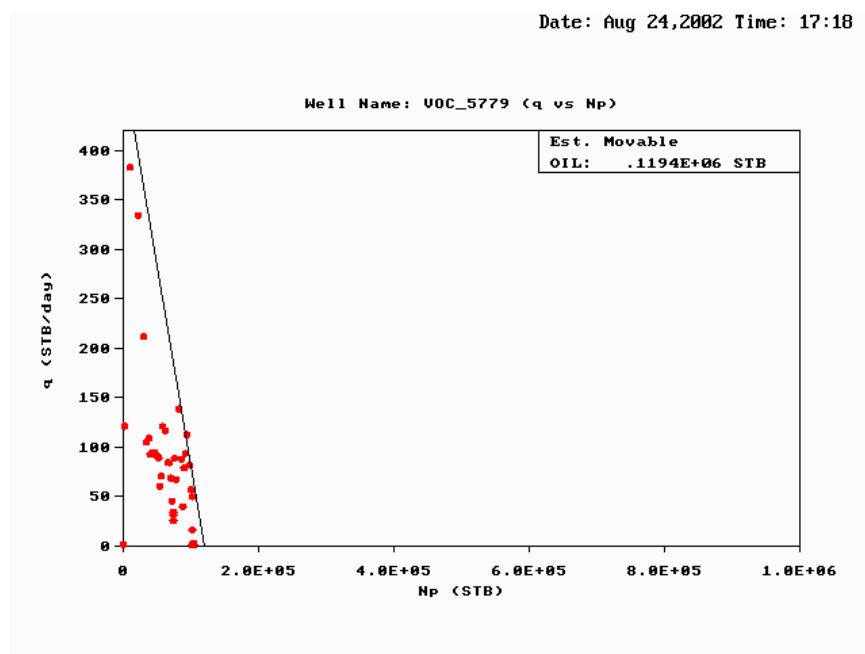
Figure 239 — Calculation of Recoverable Oil, Vocation Well 5779.
