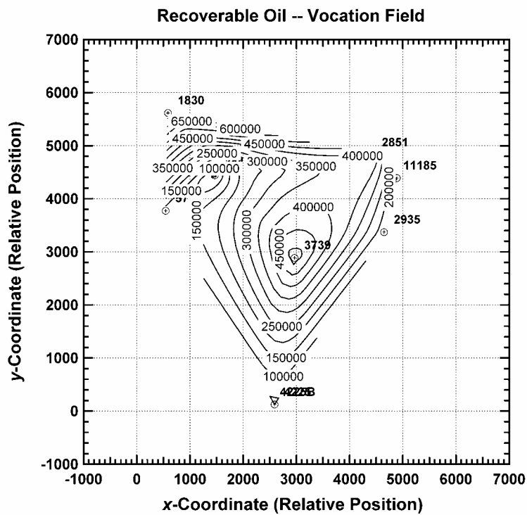
Figure 249 — Contour Map of Recoverable Oil, Vocation Oil Field.
