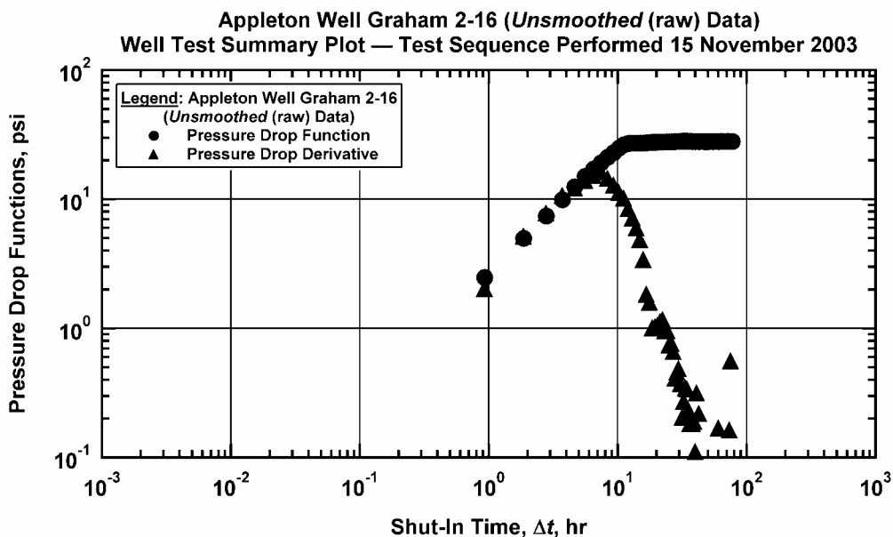
Figure 171b — Log-log Summary Plot (No Analysis) for Graham Well 2-16 (testing sequence of November 2003) — raw pressure buildup data case. Appleton Field (Alabama, USA)
