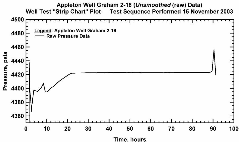
Figure 171a — "Strip Chart" Data Summary Plot (No Analysis) for Graham Well 2-16 (testing sequence of November 2003). Appleton Field (Alabama, USA)
