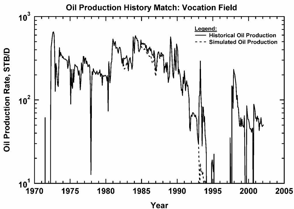
Figure 296 — Oil Production Rate History Match, Vocation Field.
