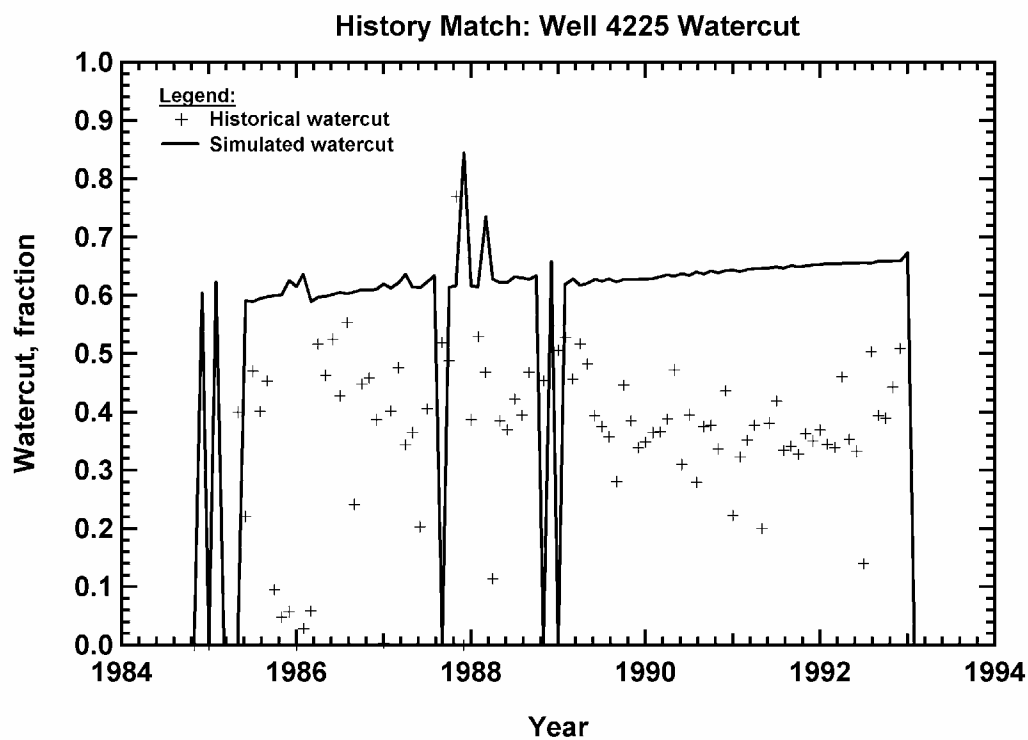
Figure 305 — Watercut history match, Vocation Well 4225.
