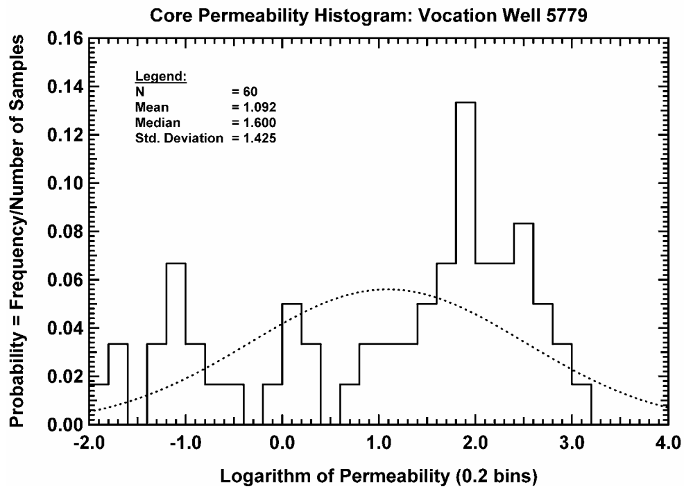
Figure 189 — Core Permeability Histogram, Vocation Well 5779.
