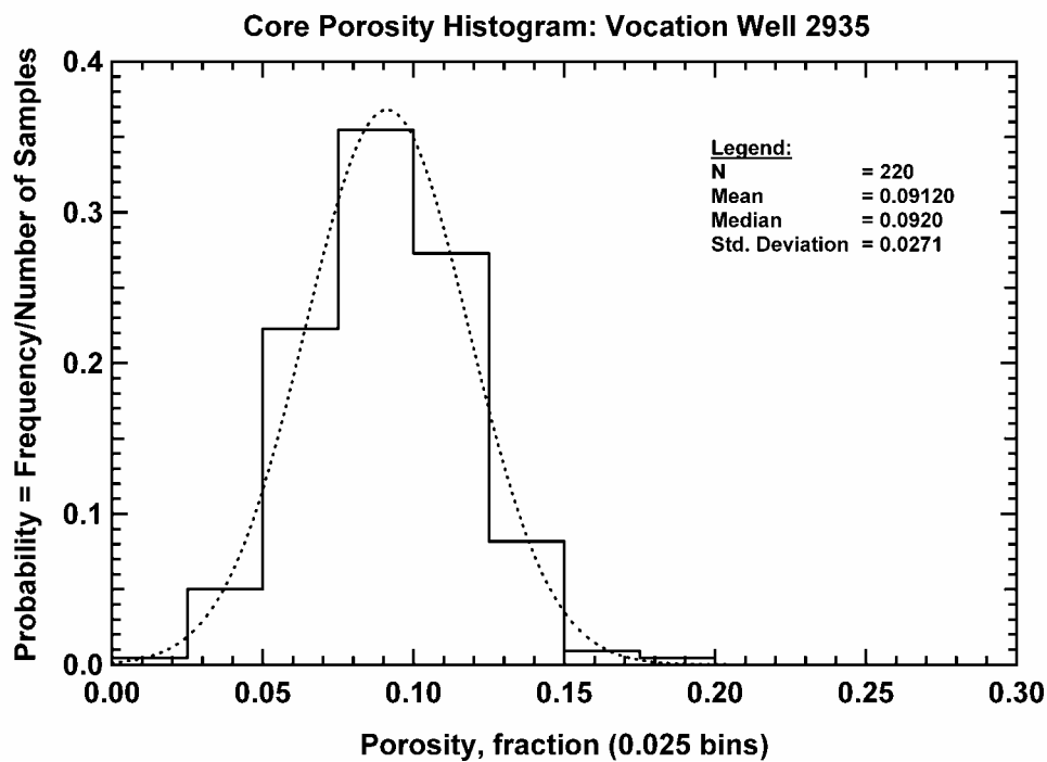
Figure 176 — Core Porosity Histogram, Vocation Well 2935.
