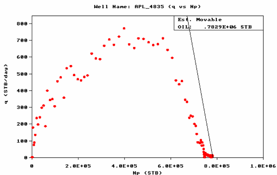
Fig. 161 — Estimate of Recoverable Oil, Appleton Well 4835B.
