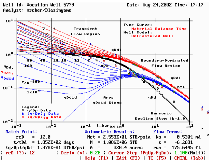
Figure 229 — Type Curve Match, Vocation Well 5779.
