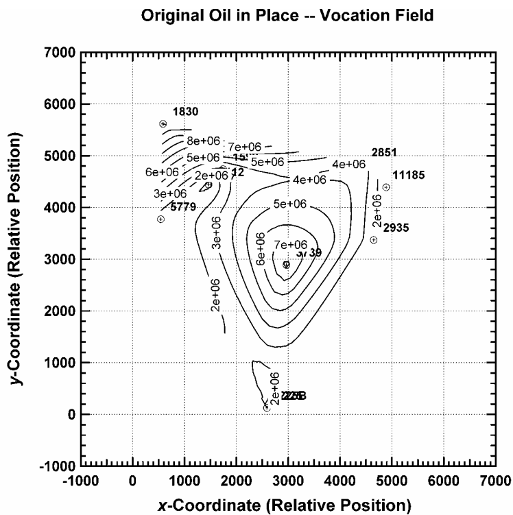
Figure 248 — Contour Map of Original Oil-in-Place, Vocation Oil Field.
