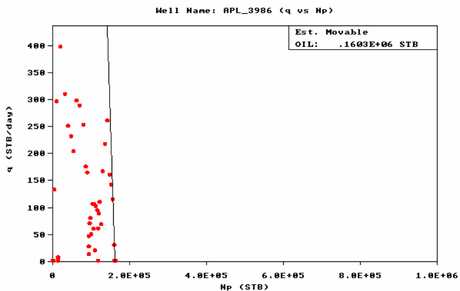
Fig. 159 — Estimate of Recoverable Oil, Appleton Well 3986.
