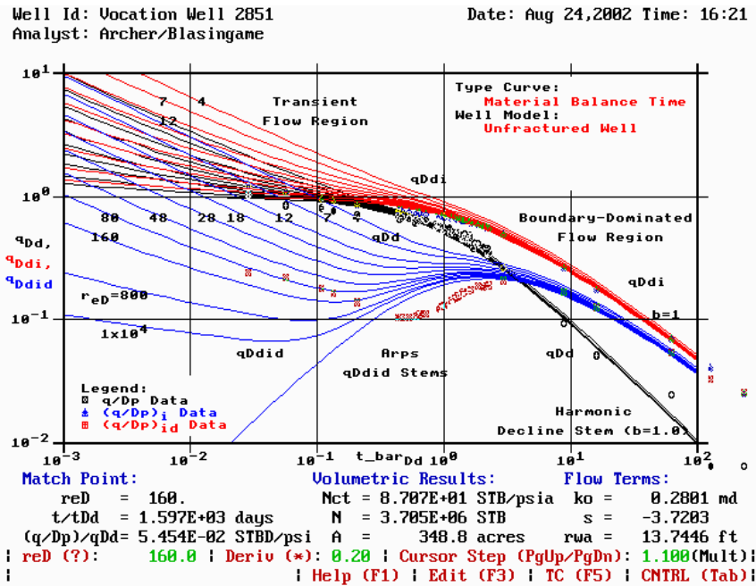
Figure 223 — Type Curve Match, Vocation Well 2851.
