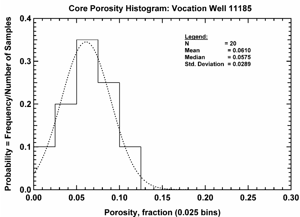
Figure 181 — Core Porosity Histogram, Vocation Well 11185.
