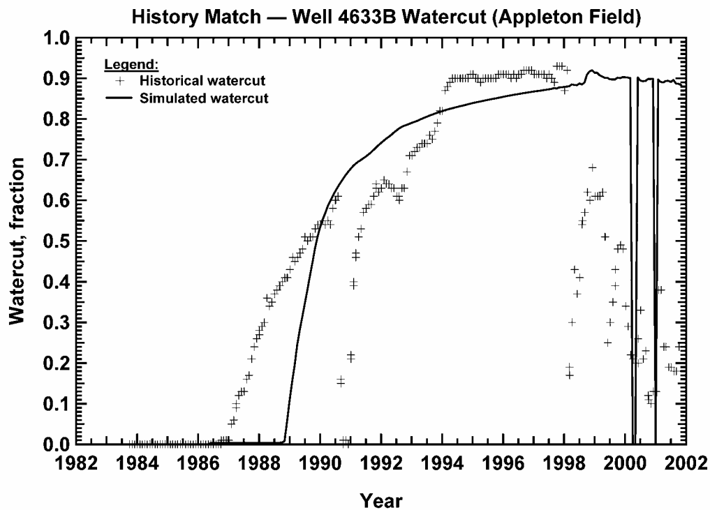
Figure 279 — Watercut history match, Well 4633B (Appleton Field).
