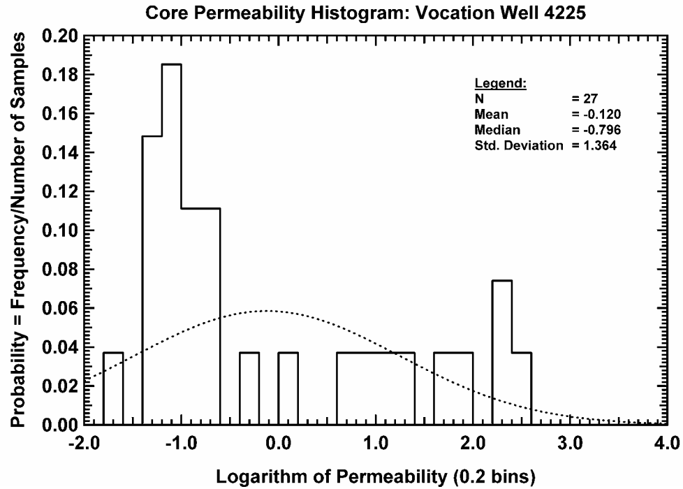
Figure 188 — Core Permeability Histogram, Vocation Well 4225.
