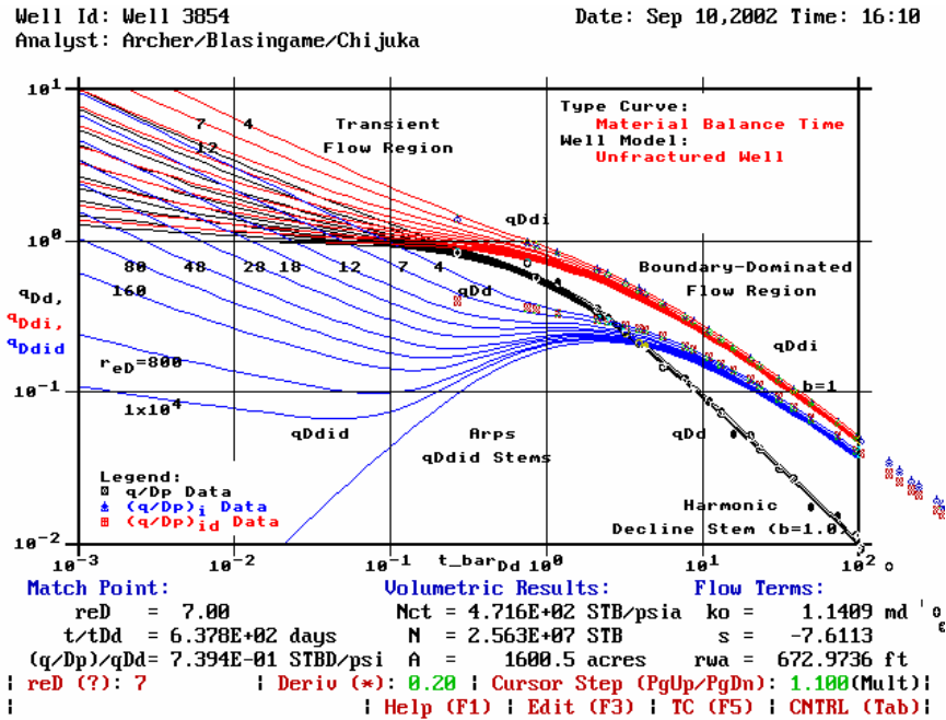
Fig. 153 — Type Curve Match, Appleton Well 3854.
