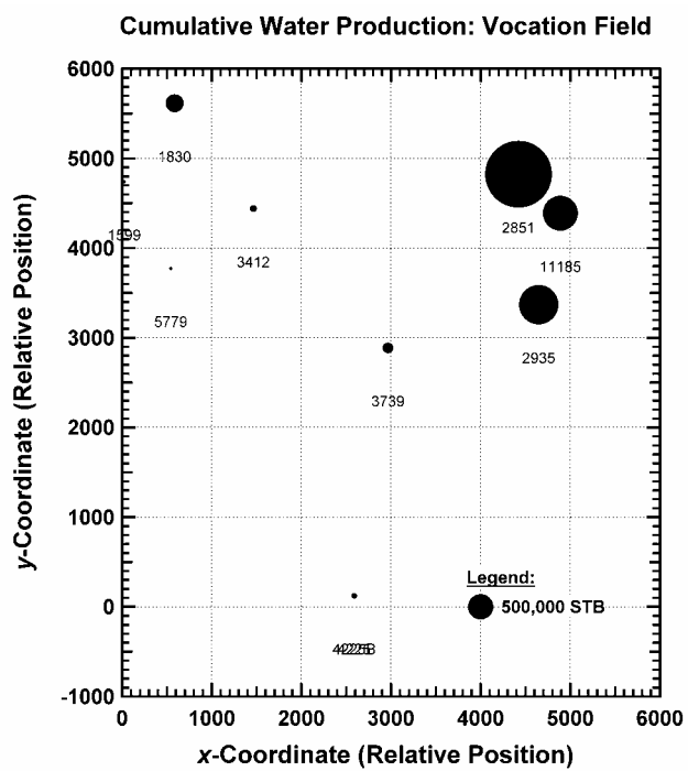
Figure 290 — Water Production as a Function of Well Location, Vocation Field.
