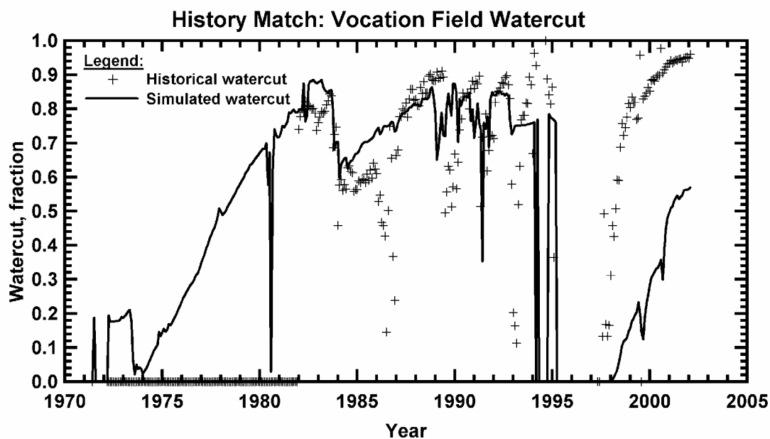
Figure 295 — Watercut history match, Vocation Field.
