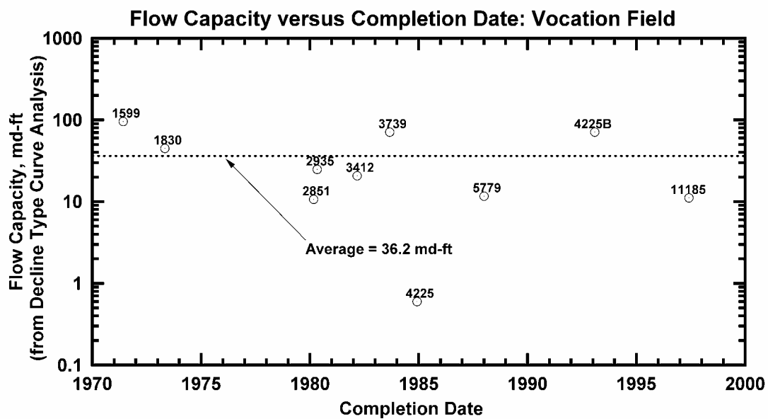
Figure 245 — Flow Capacity versus Completion Date, Vocation Oil Field.
