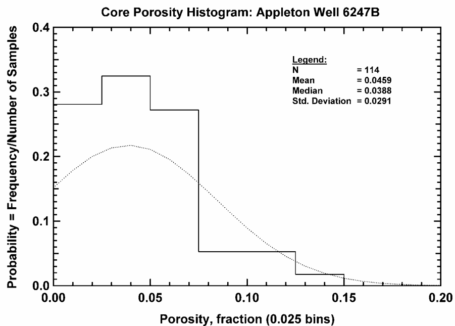
Fig. 132 — Core Porosity Histogram, Appleton Well 6247B
