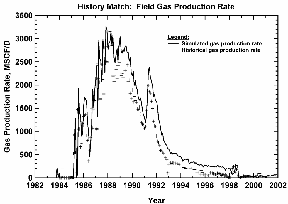
Figure 276 — Gas Production Rate History Match, Appleton Field.
