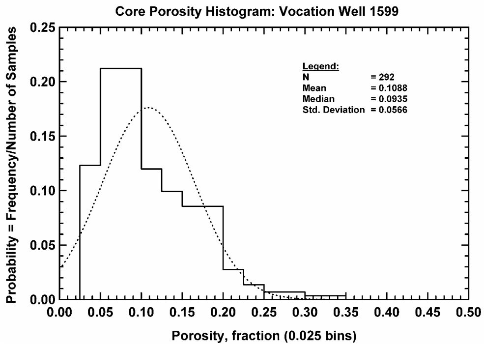
Figure 173 — Core Porosity Histogram, Vocation Well 1599.
