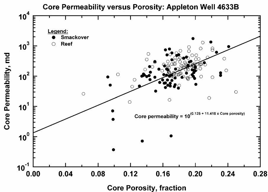
Fig. 150 — Core Permeability versus Core Porosity, Appleton Well 4633B.
