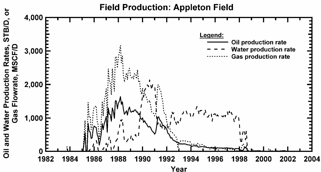
Figure 269 — Individual Phase Flowrates, Appleton Field (Cartesian Format).
