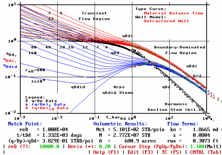
Fig. 155 — Type Curve Match, Appleton Well 4633B.
