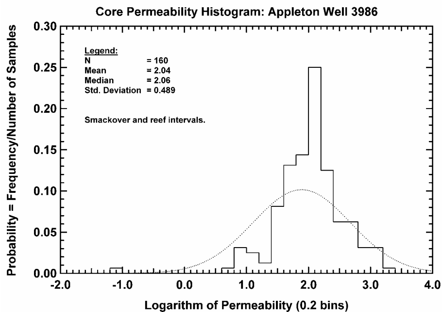
Fig. 134 — Core Permeability Histogram, Appleton Well 3986
