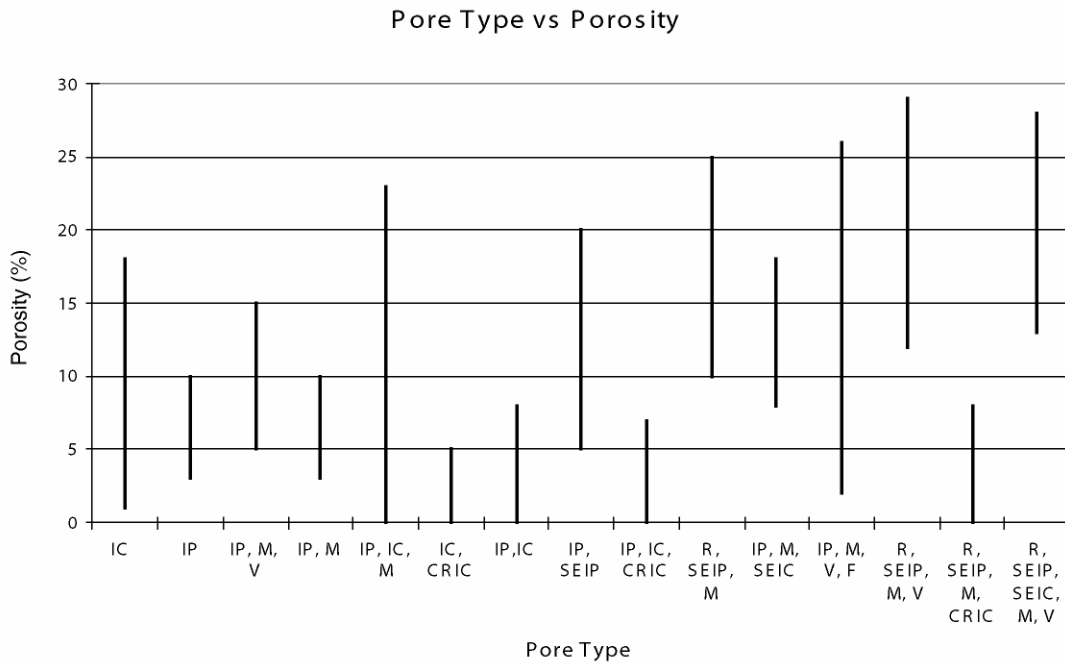
Figure 78. Graph of pore type versus porosity. It should be noted that no one pore type has a porosity range which is distinctive.
