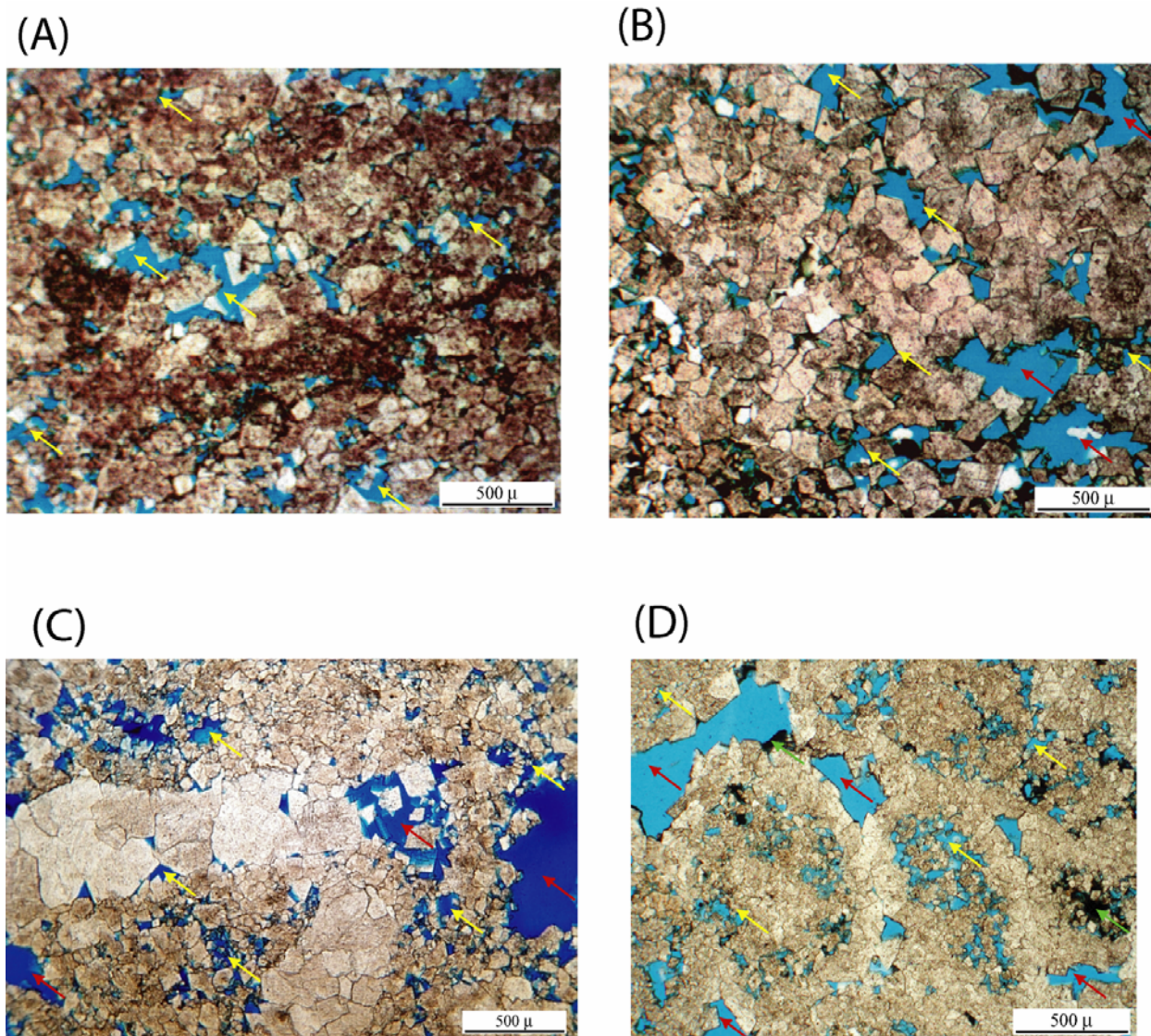
Figure 339. Photomicrographs of Smackover thrombolite facies from Appleton, Vocation and Northwest Appleton Fields showing the intense degree of dolomitization and the resulting development of effective dolomite intercrystalline (yellow arrows) and vuggy (red arrows) porosity, that acted to improve reservoir connectivity of: (A) layered thrombolite, well Permit #4633-B, depth 3,969 m (13,022 ft), Appleton Field, (B) dendroidal thrombolite, well Permit #3986, depth 3,953 m (12,970 ft), Appleton Field, (C) chaotic thrombolite, well Permit #2935, depth 4,305 m (14,124 ft), Vocation Field, and (D) chaotic thrombolite, well Permit #11030-B, depth 4,005 m (13,139 ft), Northwest Appleton Field. Notice in the last photomicrograph the presence of dead oil residue that is partially filling pore space (green arrows).
