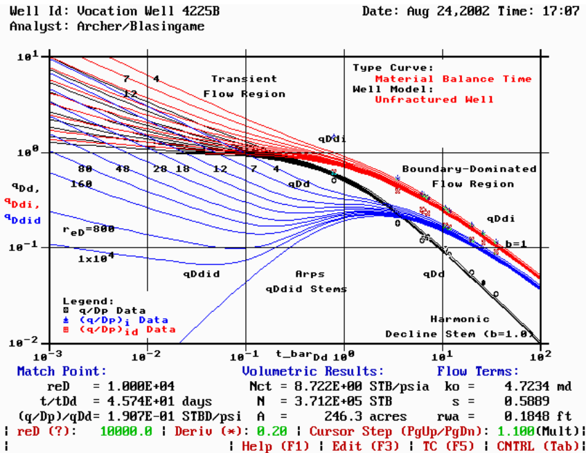
Figure 228 — Type Curve Match, Vocation Well 4225B.
