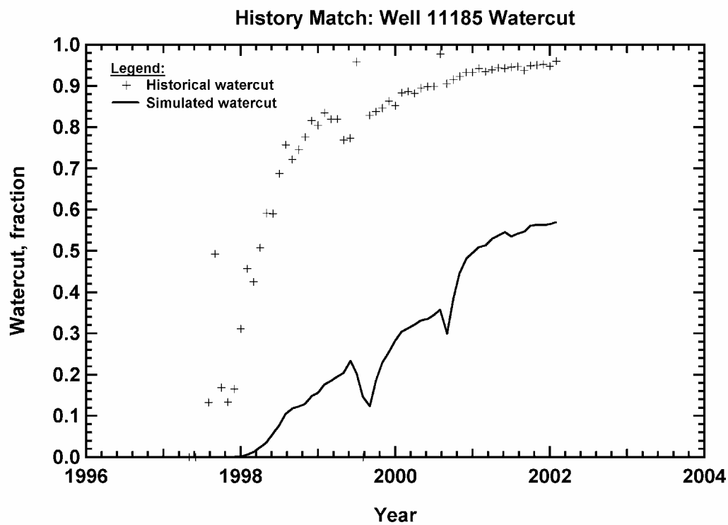
Figure 308 — Watercut history match, Vocation Well 11185.
