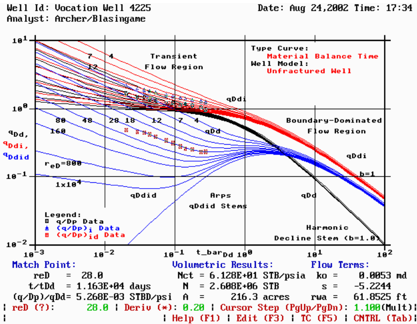
Figure 227 — Type Curve Match, Vocation Well 4225.
