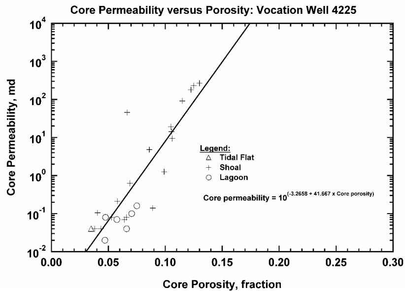
Figure 215 — Core Permeability versus Core Porosity, Vocation Well 4225.
