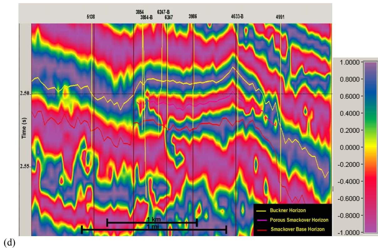
Figure 50: NW-SE transects through attribute volumes corresponding to Figure 47a. These show the physical relationship between the predicting attributes and porosity within the porous interval. (a) Derivative (b) Derivative of reflection strength (c) Reflection strength (this attribute is shown to illustrate the importance of its derivative (b) in imaging vertical changes) (d) Cosine instantaneous phase. See Figure 43 for location of transects.
