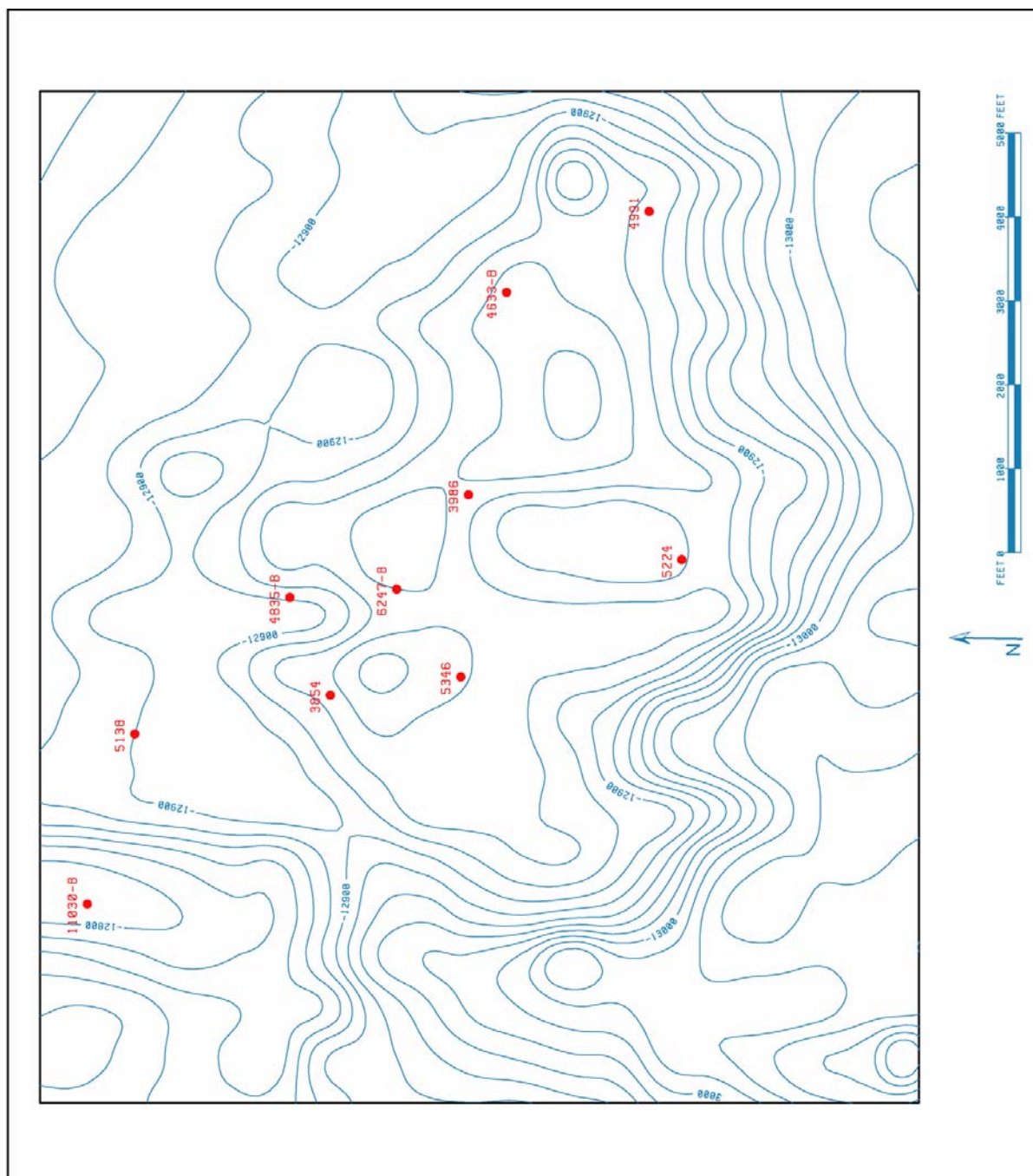
Figure 17. Structure on top of basement (from seismic data).
