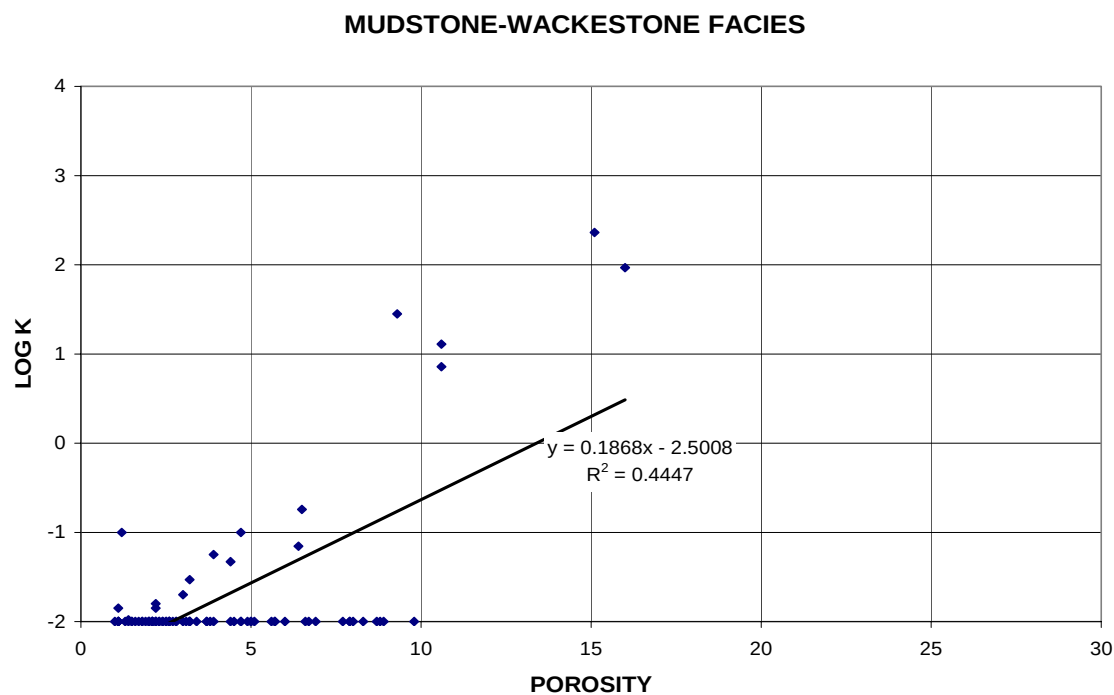
Figure 124. Porosity-permeability plot showing correlation to rock type in Vocation field.
