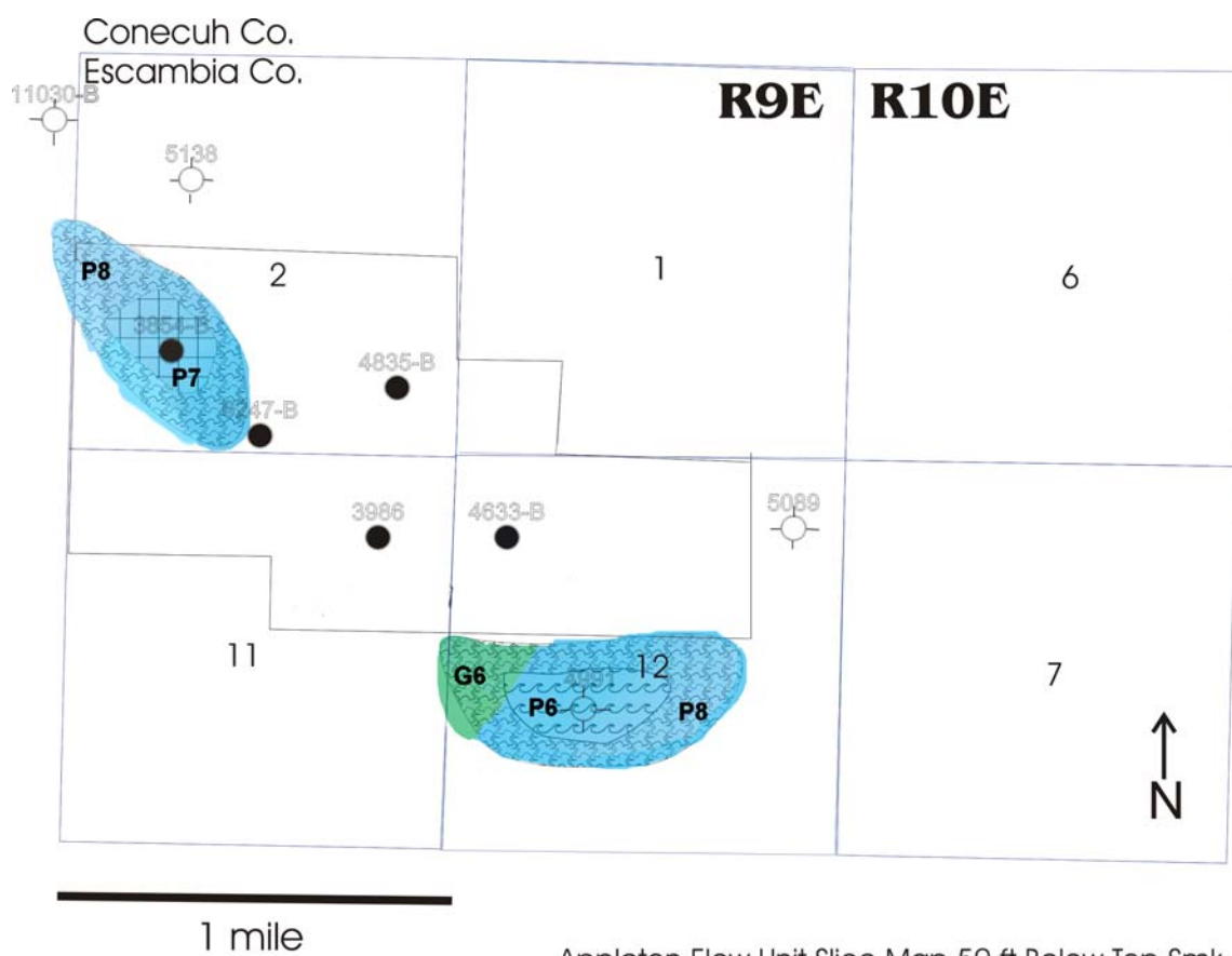
Figure 106. Appleton Flow Unit Slice Map 50 ft below Top of Smackover.
