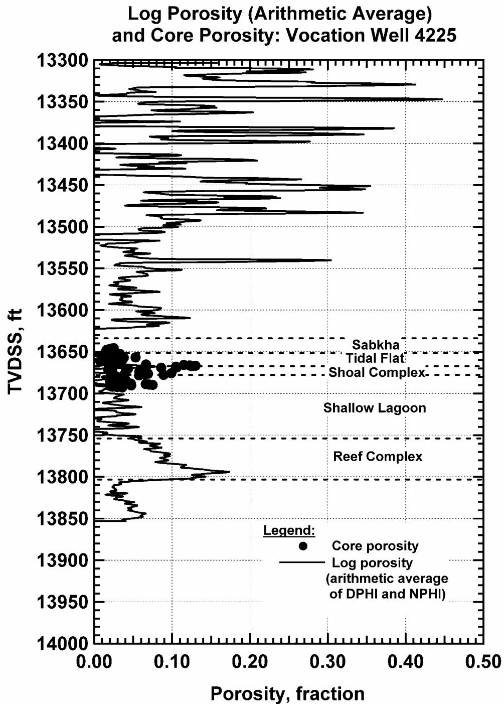
Figure 197 — Porosity Variation with Depth, Vocation Well 4225.
