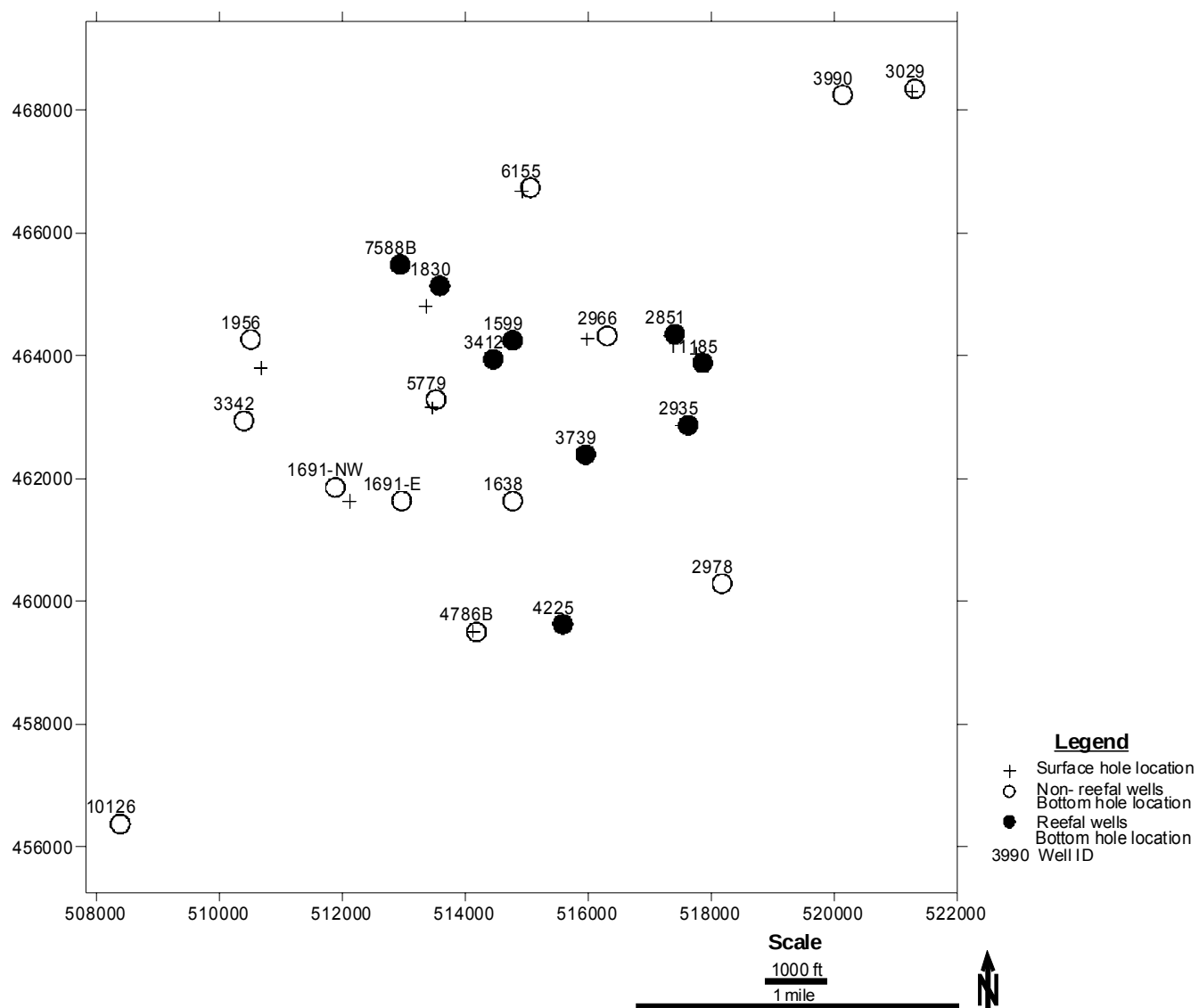
Figure 57: Well locations at Vocation Field. Wells classified based on presence or absence of reef facies.
