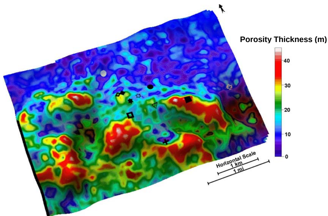
Figure 55: Porosity thickness map of the Smackover Formation overlain on the Buckner/Smackover structure map for better display. Note the overall porosity thickness (hot colors) on the southern flanks of structure. Observed differences in the distribution of porosity are mainly a result of the non-linear relationship between the predicting attributes and the seismic data. Well symbols are indicated in Figures 43 and 48.
