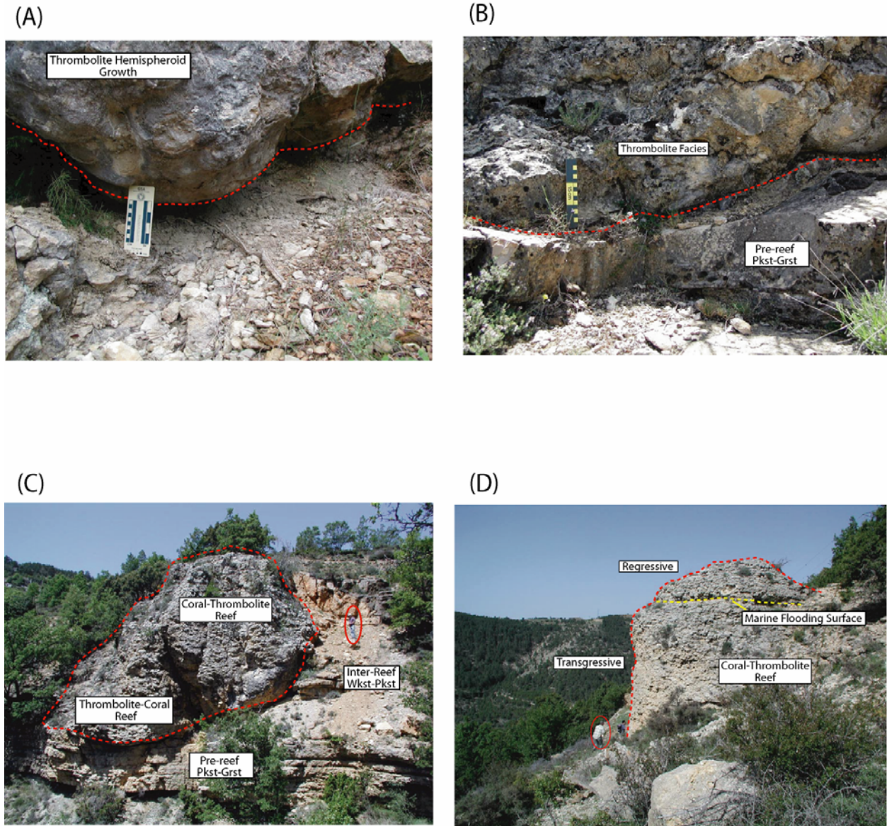
Figure 332. Outcrop photographs of pinnacle reefs and associated facies of the Torrecilla Formation : (A) thrombolite hemispheroid growth form of Leinfelder et al. (1993b), Tormón (TO), (B) pre-reef facies of packstone and grainstone, Barranco de Diablo (BD), (C) inter-reef facies of wackestone and packstone, Barranco de la Hoz (BH2), and (D) marine flooding surface affecting pinnacle reef faunal composition and growth, Barranco de la Hoz (BH1).
