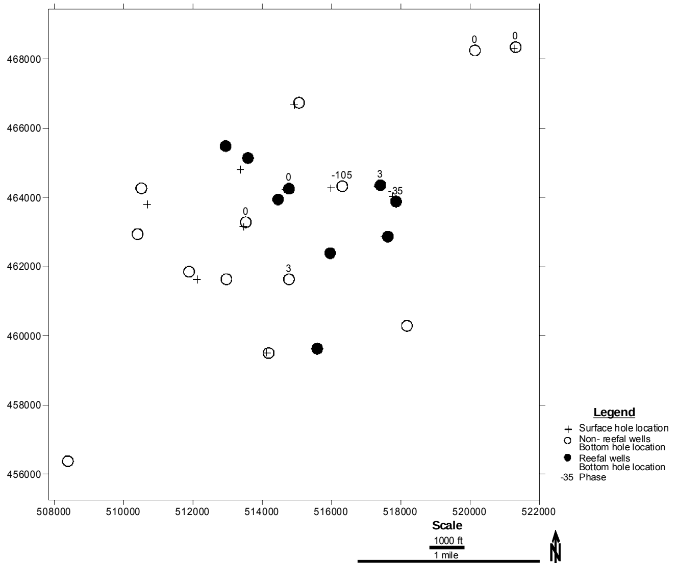
Figure 59: Seismic grid showing phase rotation necessary to obtain a statistically significant synthetic tie. Note phase variation in the east, which could be attributed to structural changes in that area. Wells with excessive phase rotations were not included in subsequent attribute analyses.
