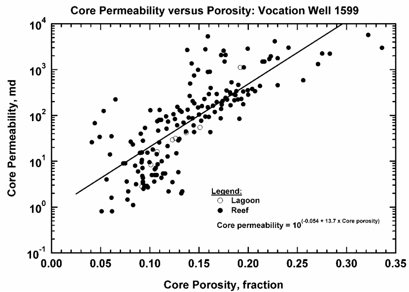
Figure 209 — Core Permeability versus Core Porosity, Vocation Well 1599.
