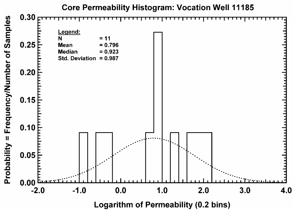
Figure 190 — Core Permeability Histogram, Vocation Well 11185.
