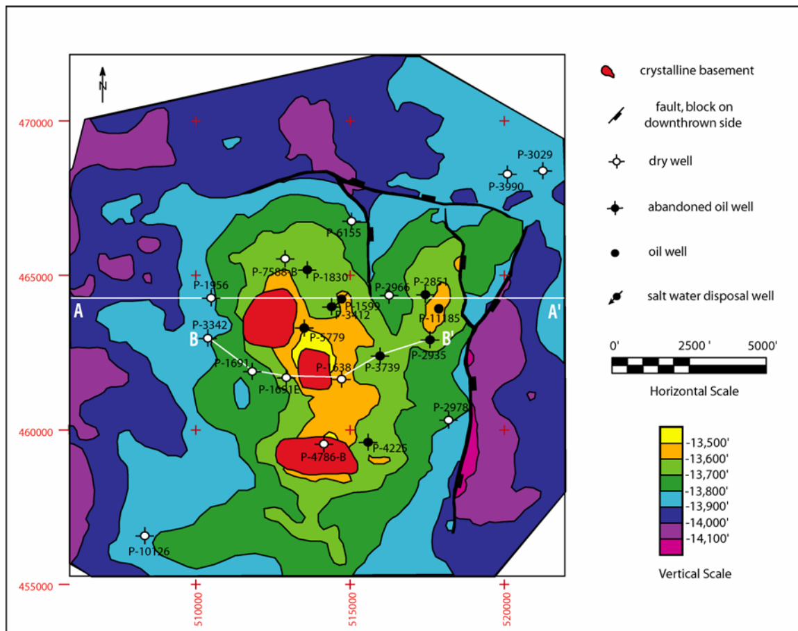
Figure 258: Structure contour map in depth based on 3-D seismic interpretation of the top of the Buckner-Smackover Formation at Vocation Field.
