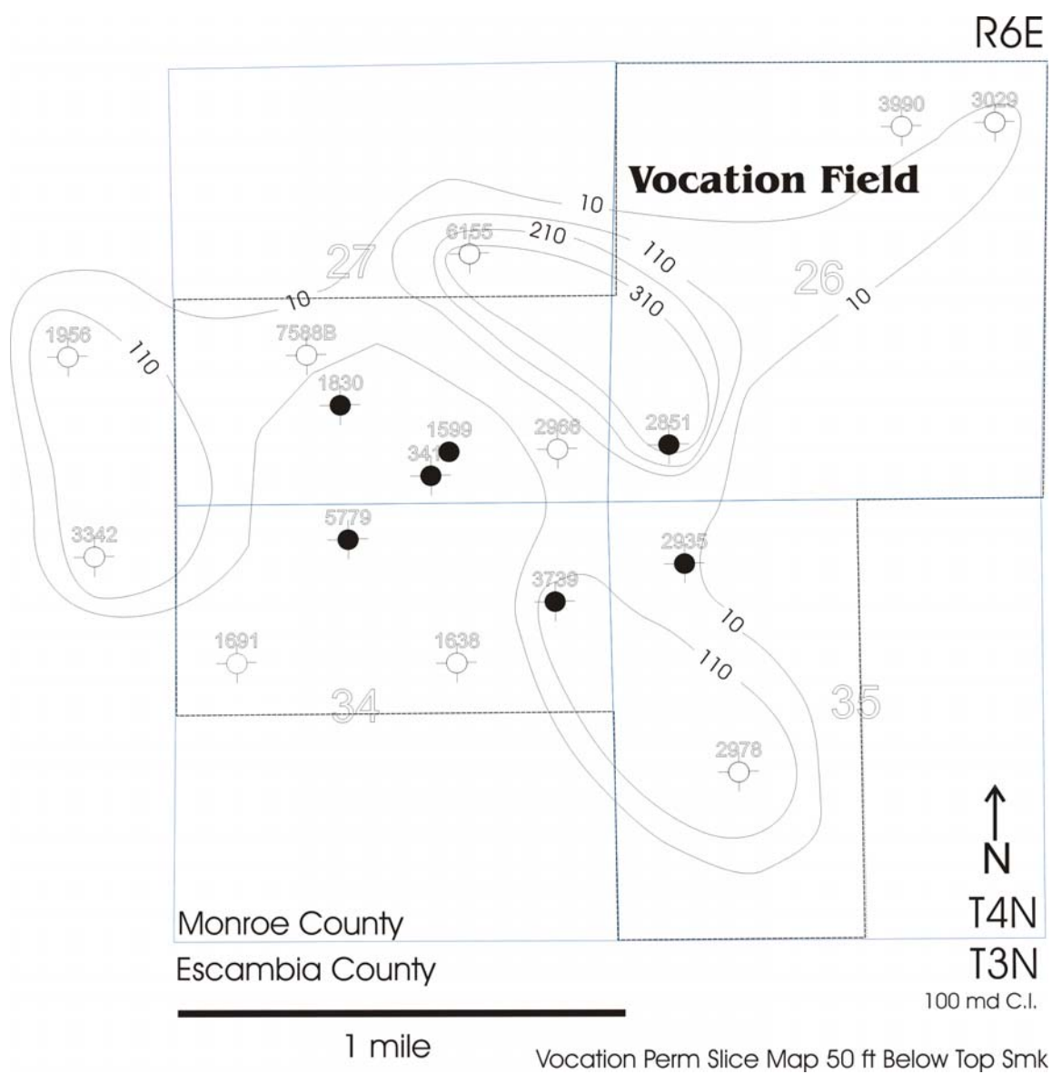
Figure 99. Vocation Permeability Slice Map 50 ft below Top of Smackover.
