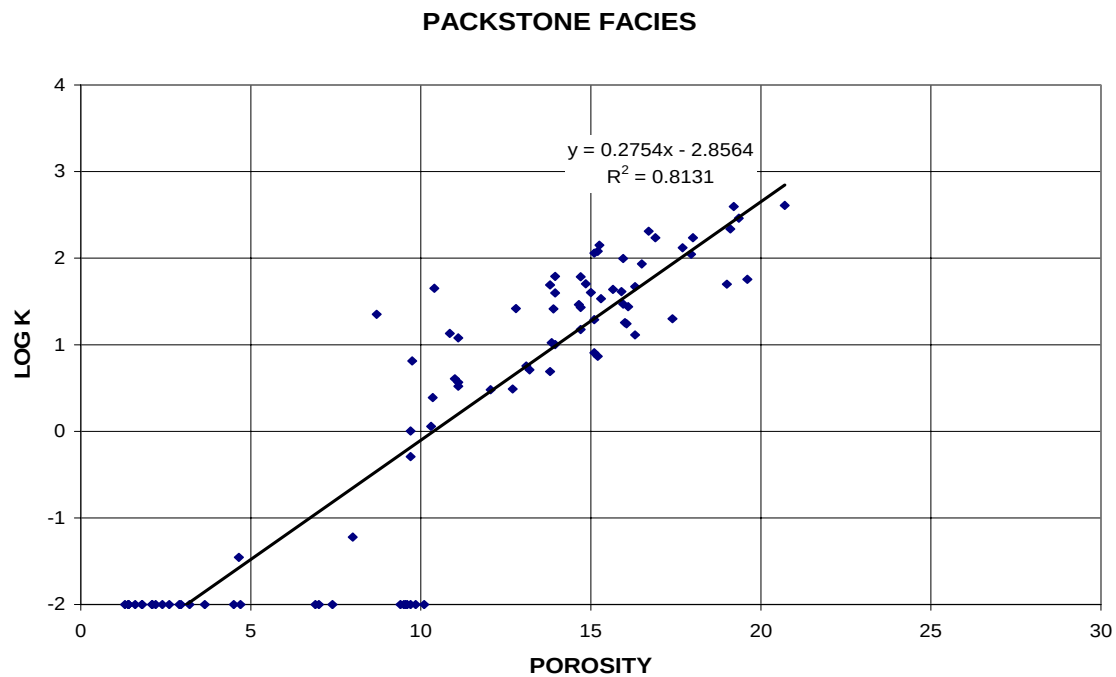
Figure 121. Porosity-permeability plot showing correlation to rock type in Appleton field.
