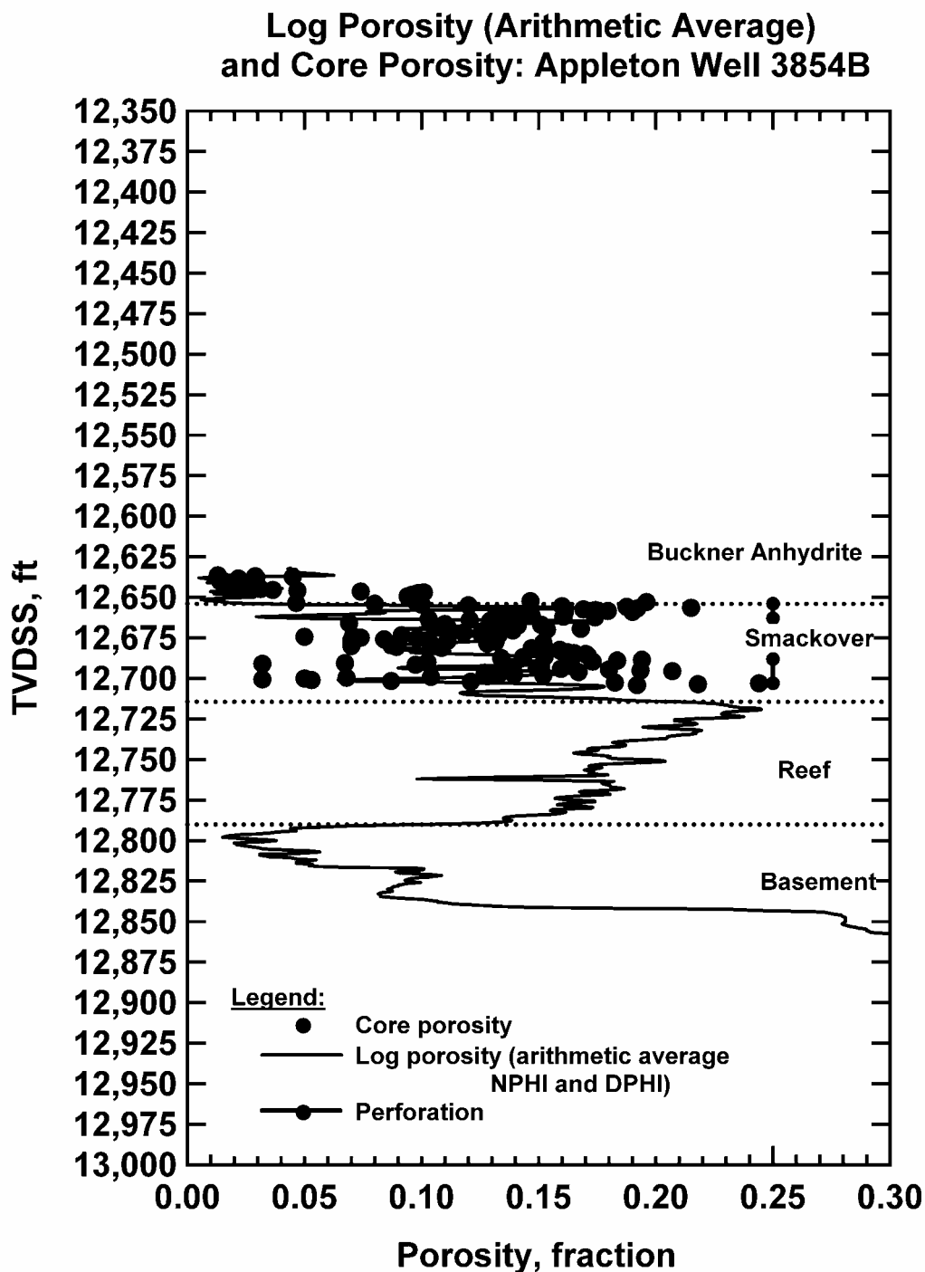
Fig. 138 — Porosity Variation with Depth, Appleton Well 3854B
