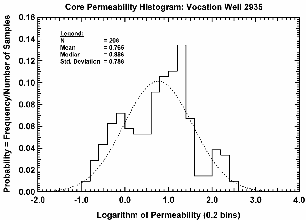
Figure 185 — Core Permeability Histogram, Vocation Well 2935.
