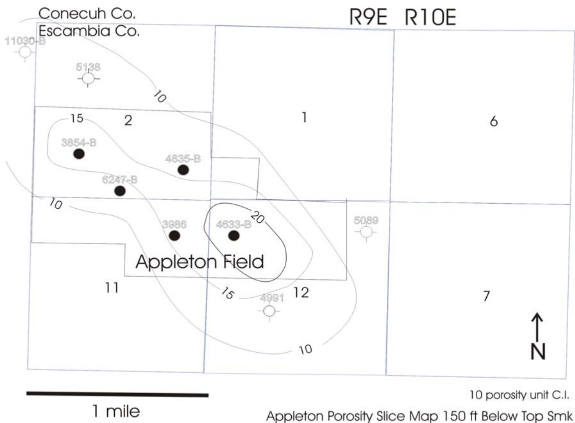
Figure 83. Appleton Porosity Slice Map 150 ft below Top of Smackover.
