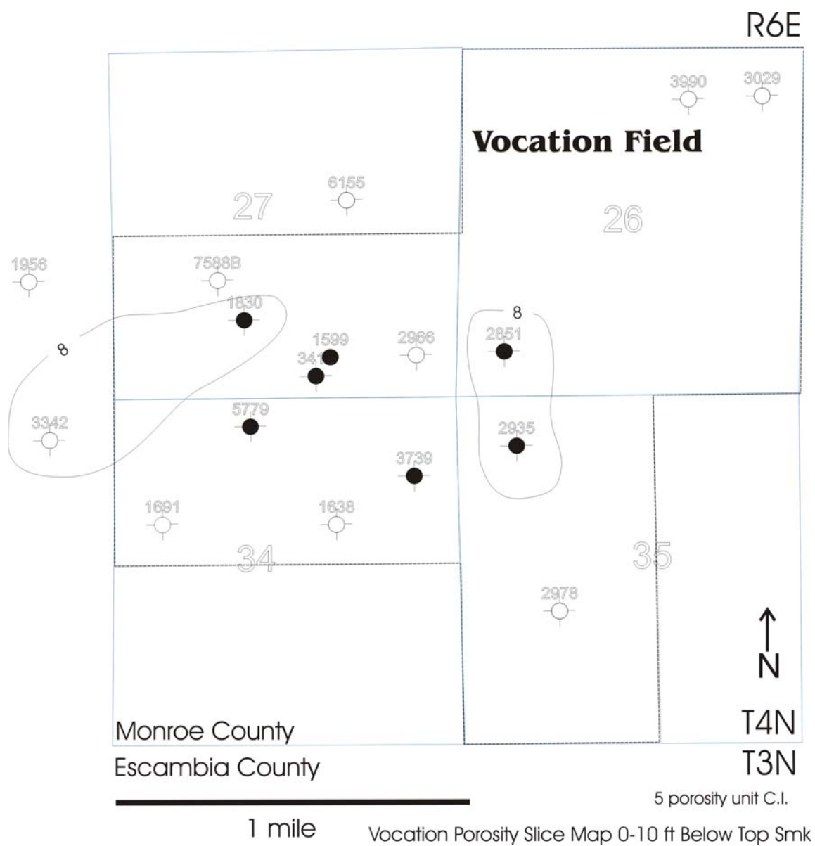
Figure 86. Vocation Porosity Slice Map 0-10 ft below Top of Smackover.
