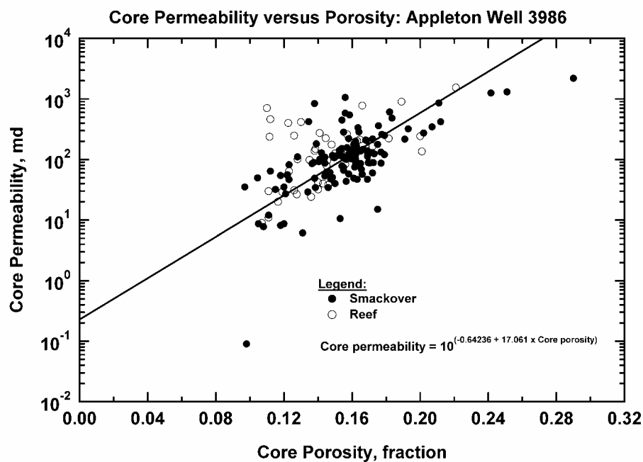
Fig. 149 — Core Permeability versus Core Porosity, Appleton Well 3986.
