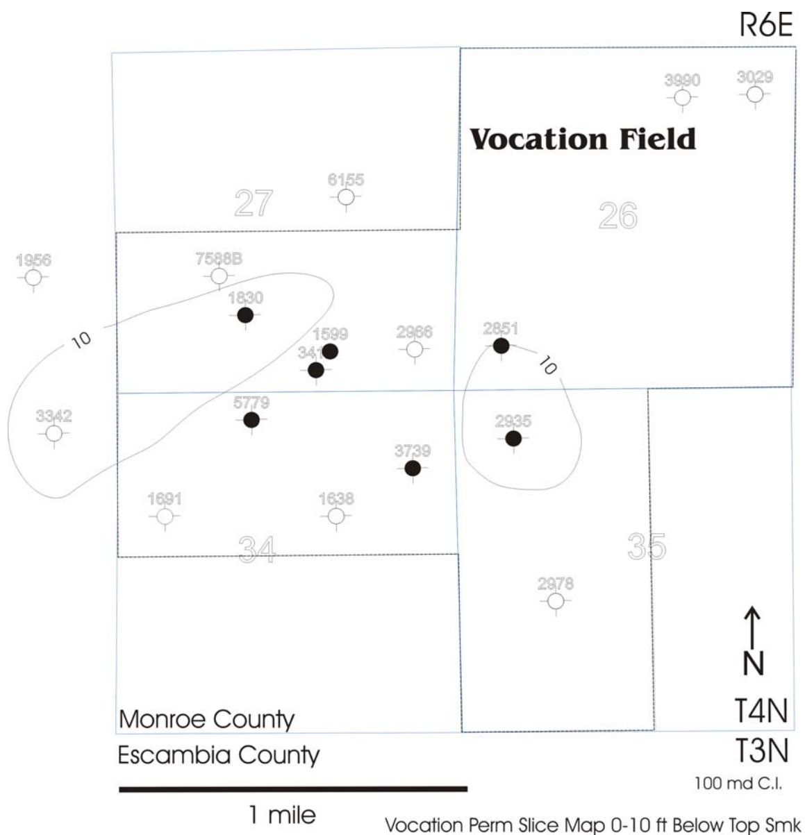
Figure 98. Vocation Permeability Slice Map 0-10 ft below Top of Smackover.
