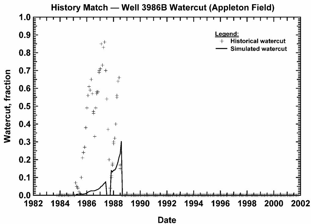
Figure 278 — Watercut history match, Well 3986B (Appleton Field).
