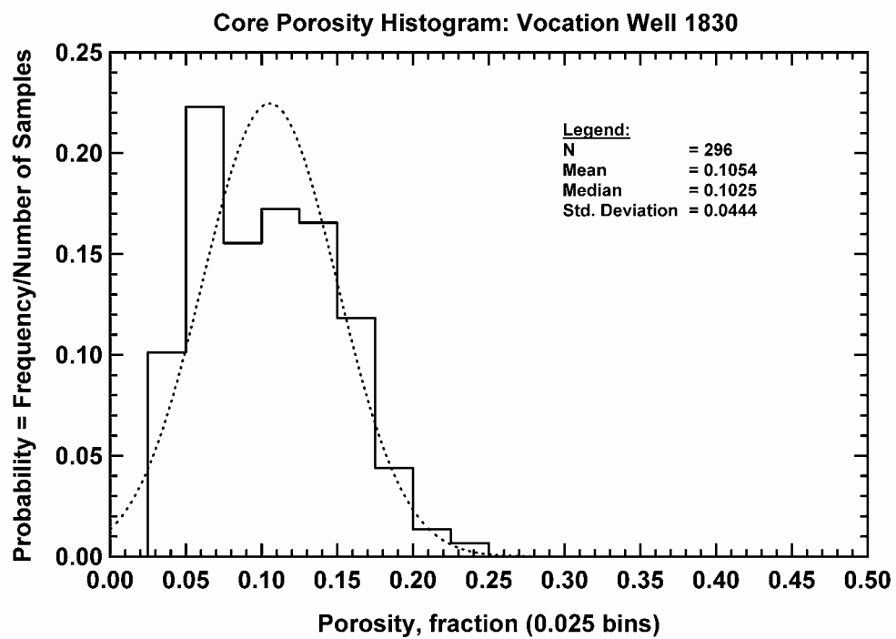
Figure 174 — Core Porosity Histogram, Vocation Well 1830.
