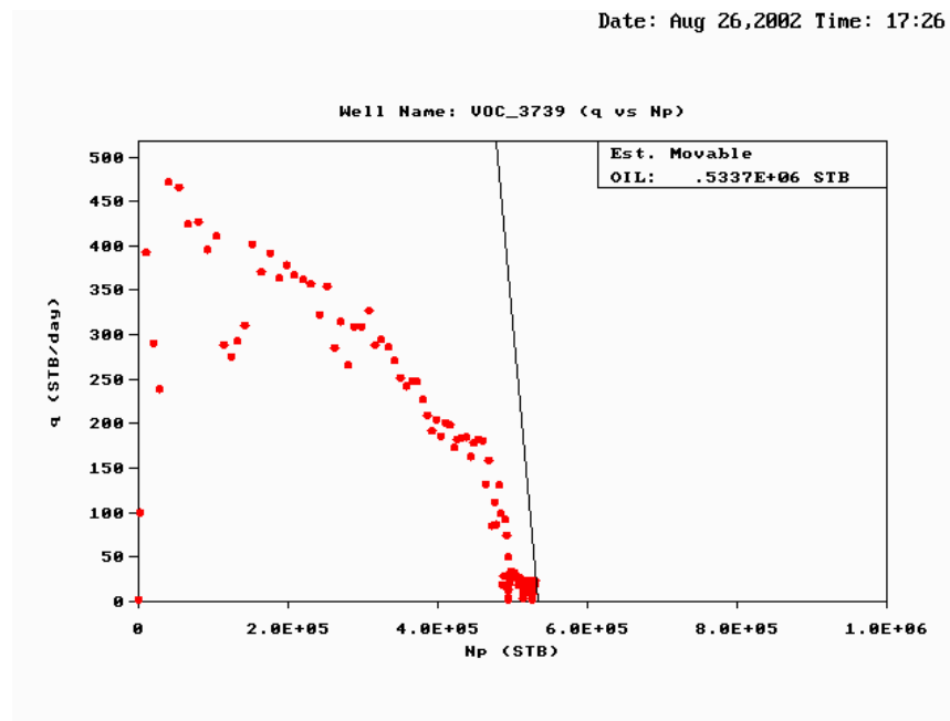
Figure 236 — Calculation of Recoverable Oil, Vocation Well 3739.
