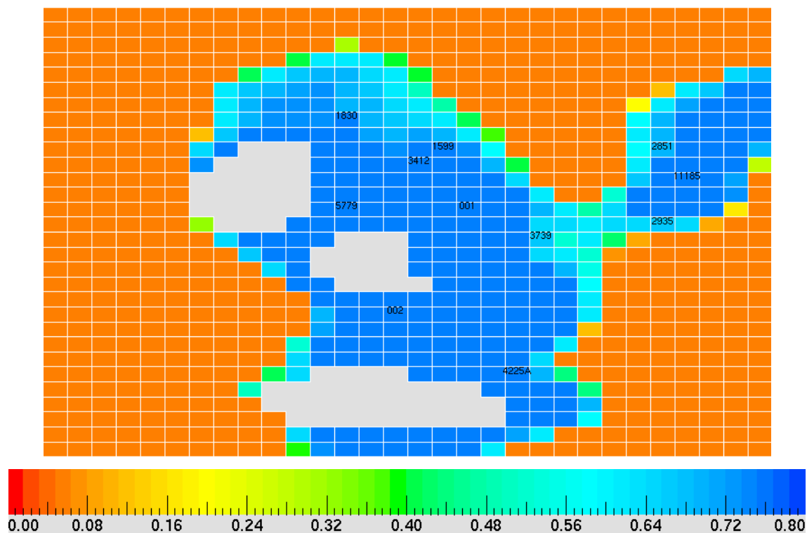
Figure 311 — Oil saturation in top simulation layer 1986, Vocation Field.
