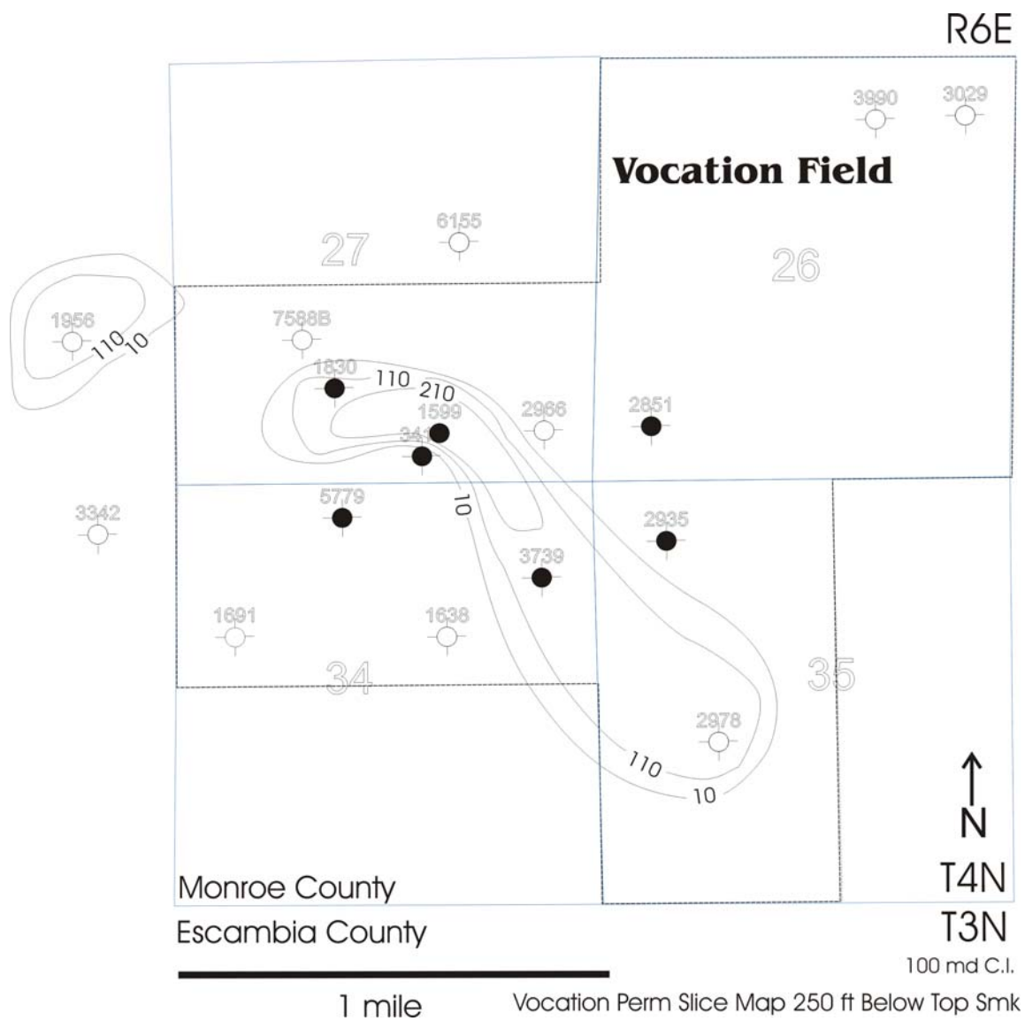
Figure 103. Vocation Permeability Slice Map 250 ft below Top of Smackover.
