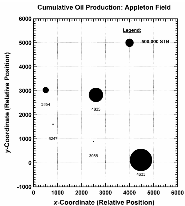
Figure 267 — Oil Production as a Function of Well Location, Appleton Field.
