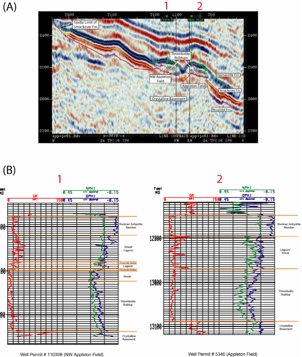
Figure 320. (A) Seismic profile oriented in an approximate dip direction showing the thrombolite buildups on the Appleton and Northwest Appleton paleohighs. Note the termination of Smackover and the underlying Norphlet strata against basement (updip depositional limit of these formations). (B) representative well logs from wells in these fields illustrating the characteristic regular pattern of lower gamma ray (GR) values coupled with relative high neutron (NPHI) and density (DPHI) porosity values for the thrombolite facies (well Permits #11030B and #5346).
