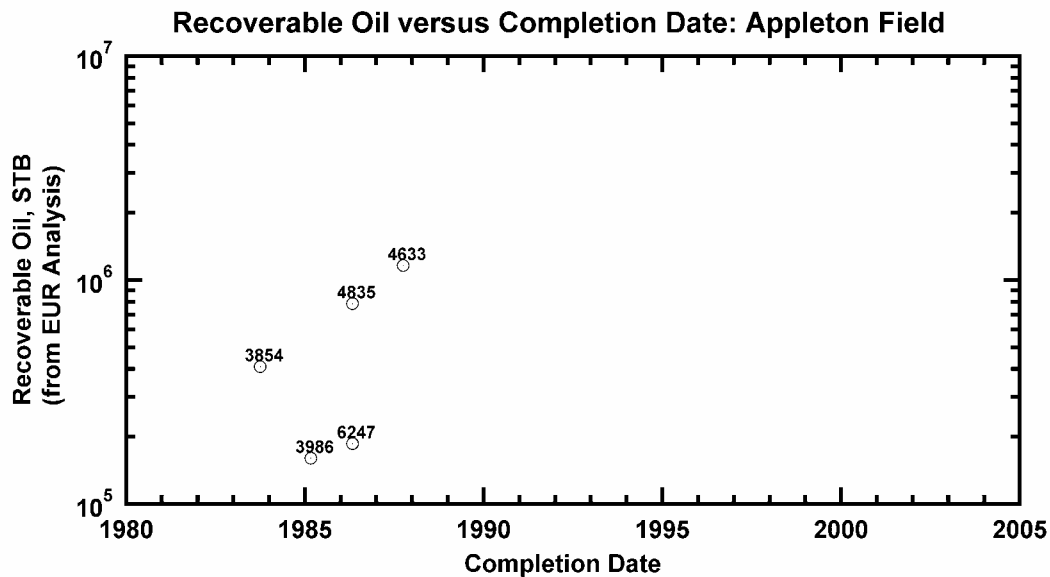
Fig. 165 — Recoverable Oil versus Completion Date, Appleton Oil Field.
