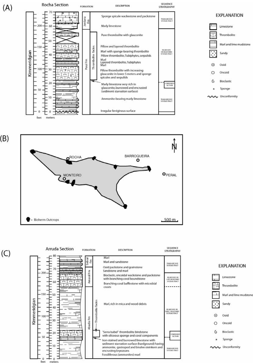
Figure 337. (A) Measured stratigraphic section of the Rocha thrombolite bioherm, Algarve Basin, (B) areal coverage of the thrombolite bioherm at Rocha, and (C) measured stratigraphic section of the Arruda dos Vinhas thrombolite buildup, Lusitanian Basin.
