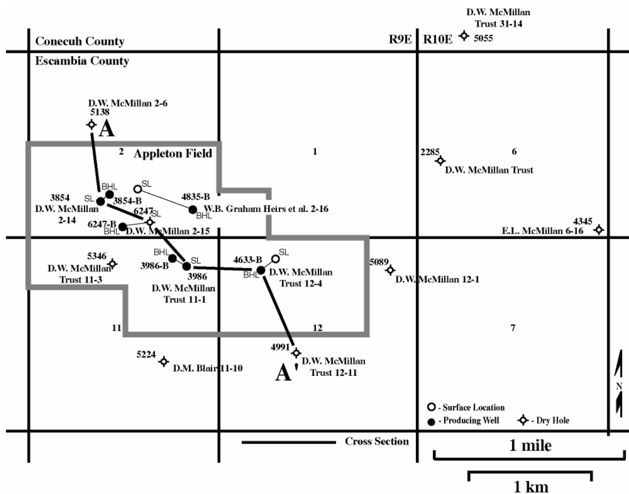
Figure 4. Appleton Field Unit area.
