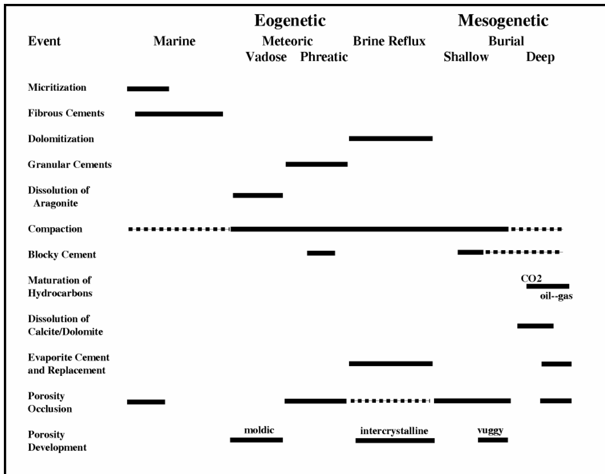
Figure 250 – Diagenetic sequence of the Smackover Formation at Appleton Field.
