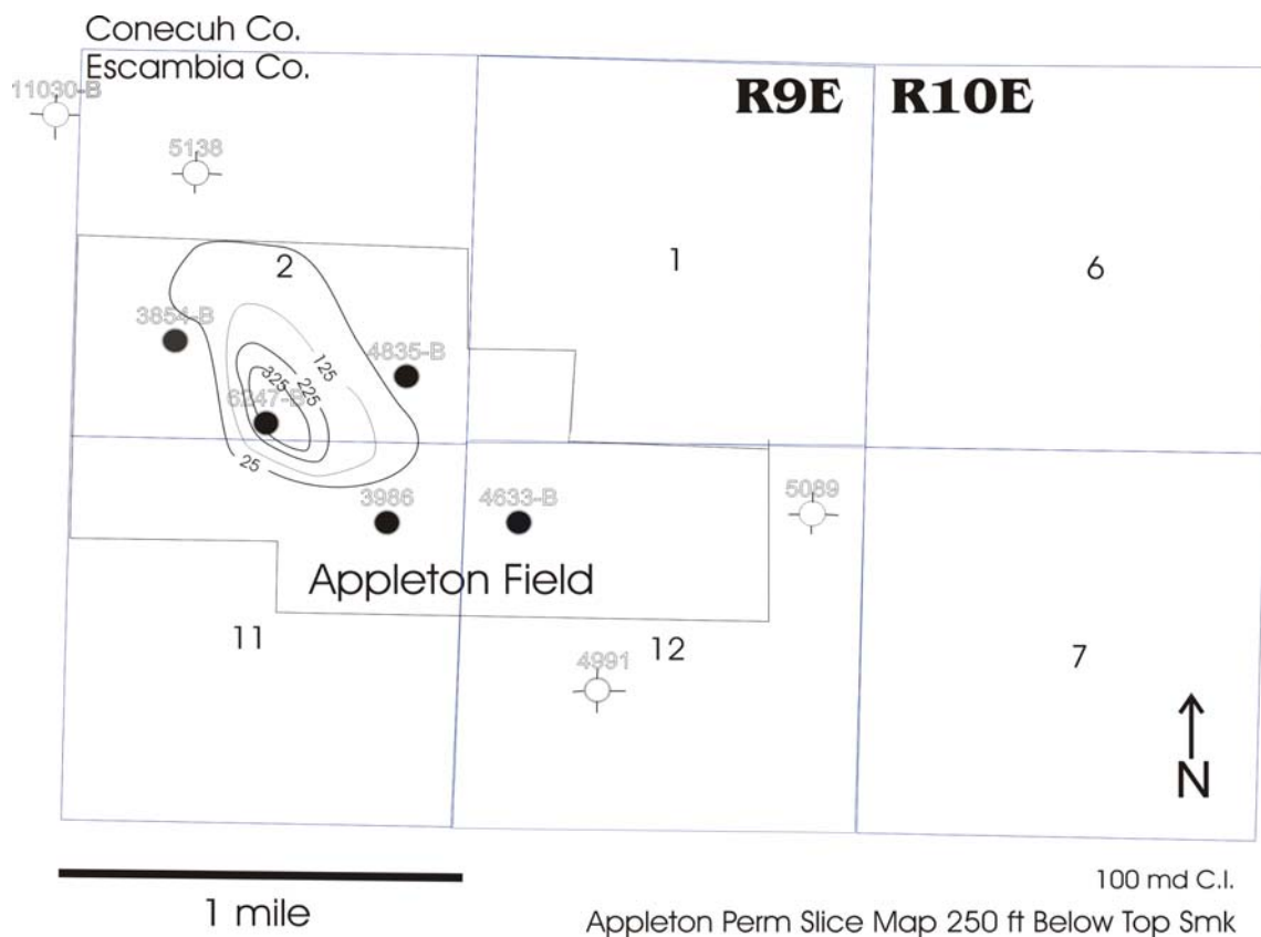
Figure 97. Appleton Permeability Slice Map 250 ft below Top of Smackover.
