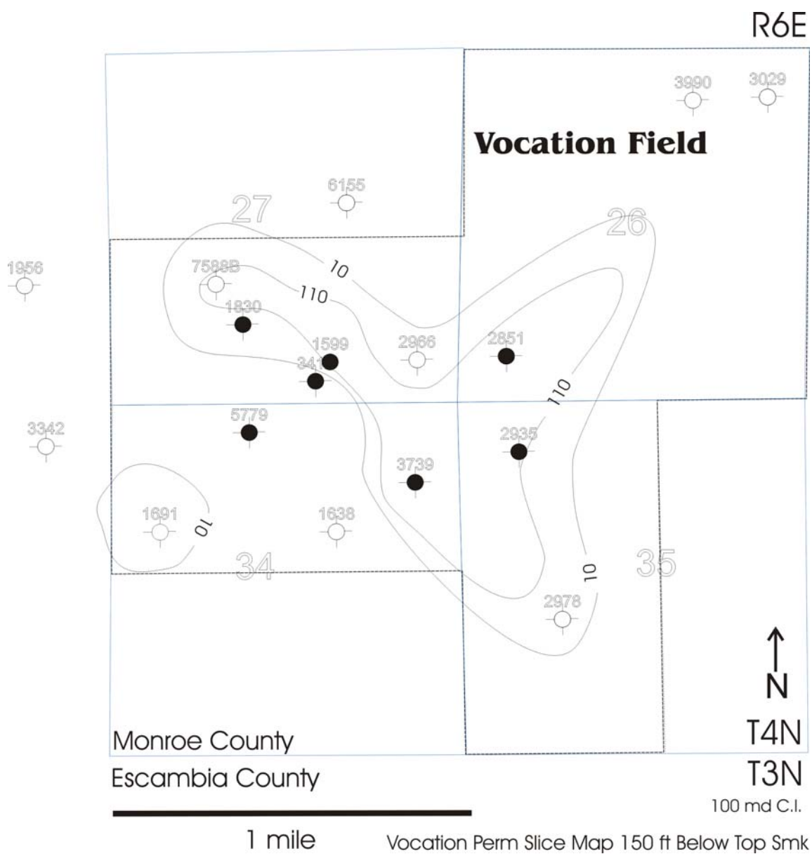
Figure 101. Vocation Permeability Slice Map 150 ft below Top of Smackover.
