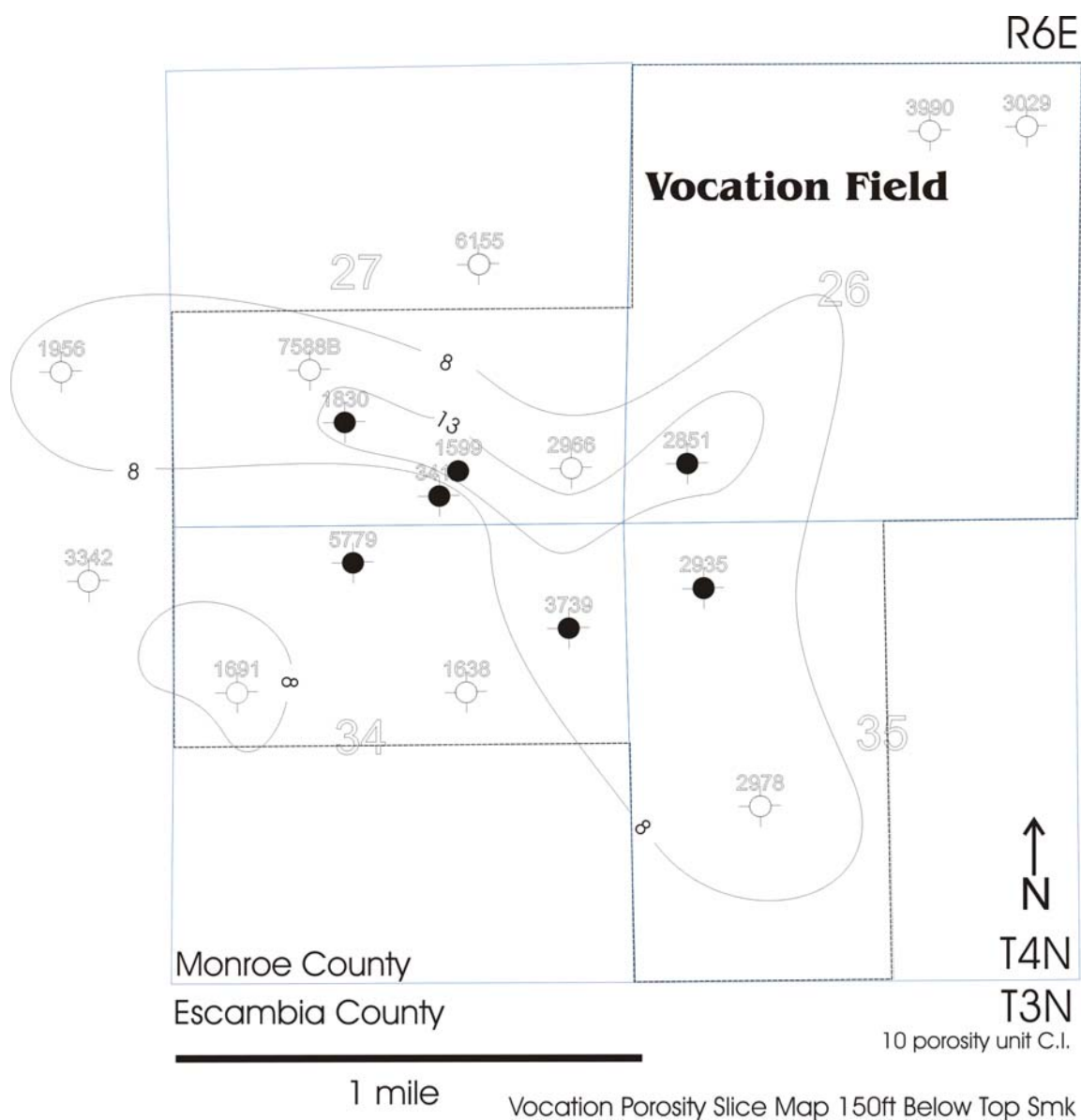
Figure 89. Vocation Porosity Slice Map 150 ft below Top of Smackover.
