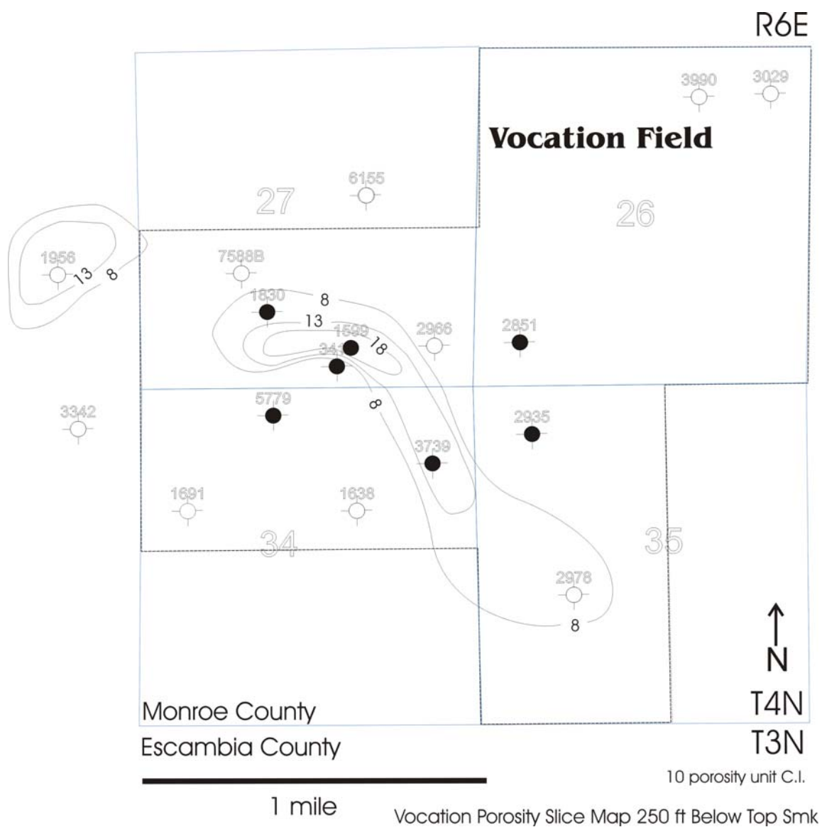
Figure 91. Vocation Porosity Slice Map 250 ft below Top of Smackover.
