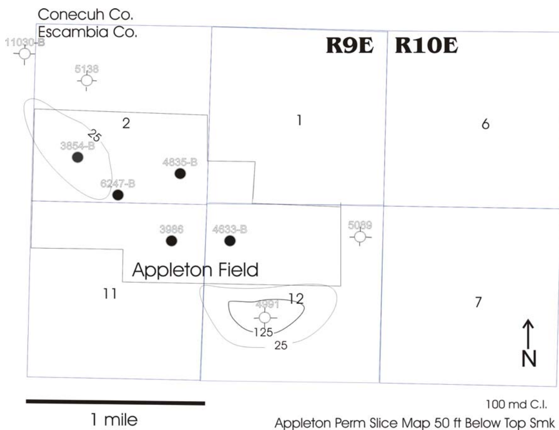
Figure 93. Appleton Permeability Slice Map 50 ft below Top of Smackover.
