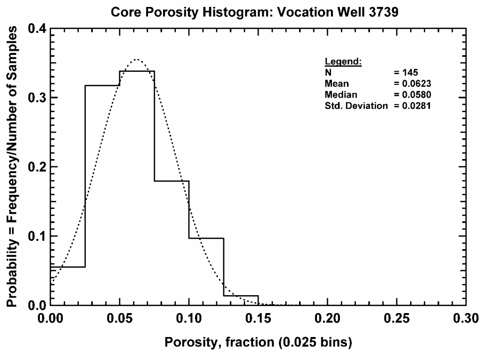
Figure 178 — Core Porosity Histogram, Vocation Well 3739.
