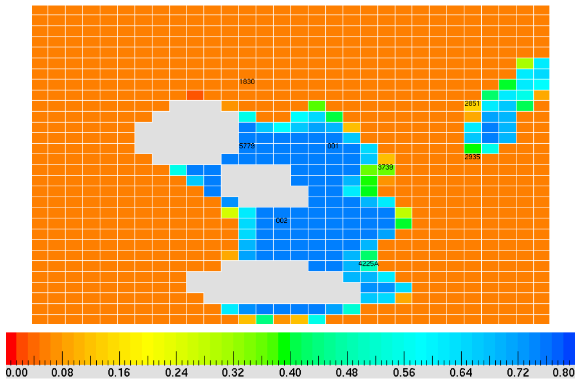
Figure 312 — Oil saturation in intermediate simulation layer (50ft from reservoir top) 1986, Vocation Field.
