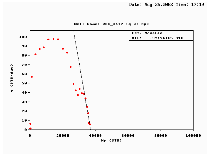
Figure 235 — Calculation of Recoverable Oil, Vocation Well 3412.
