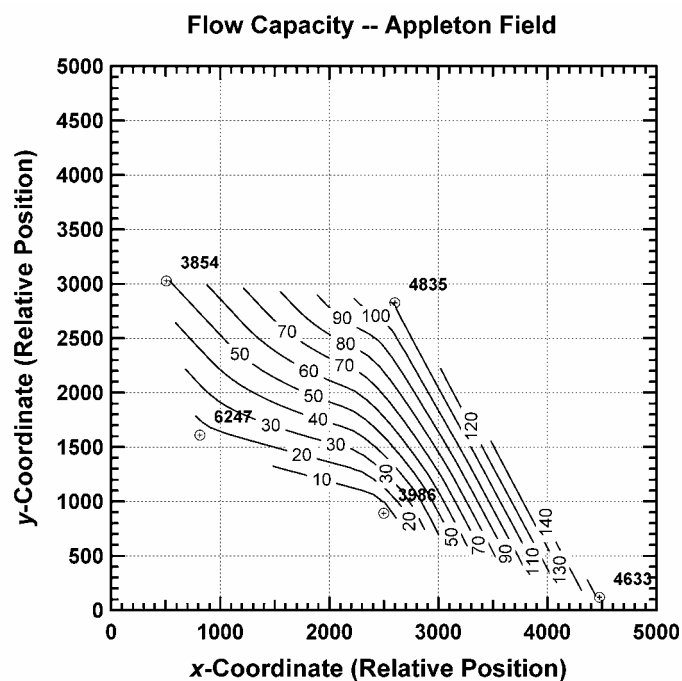
Fig. 168 — Contour Map of Flow Capacity, Appleton Oil Field.
