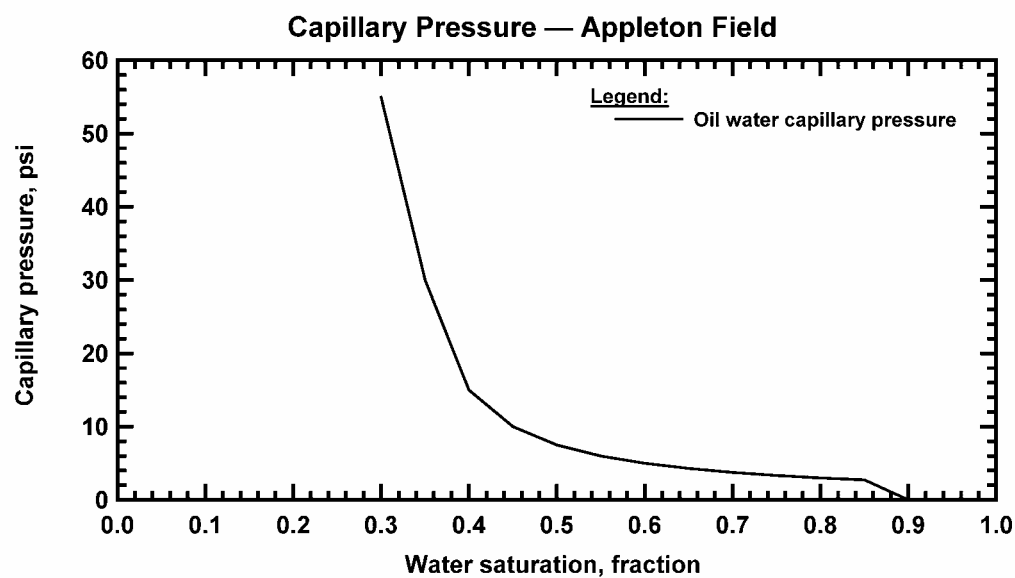
Figure 266 — History matched capillary pressure curve, Appleton Field.
