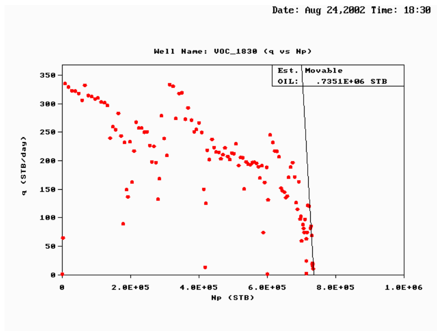
Figure 232 — Calculation of Recoverable Oil, Vocation Well 1830.
