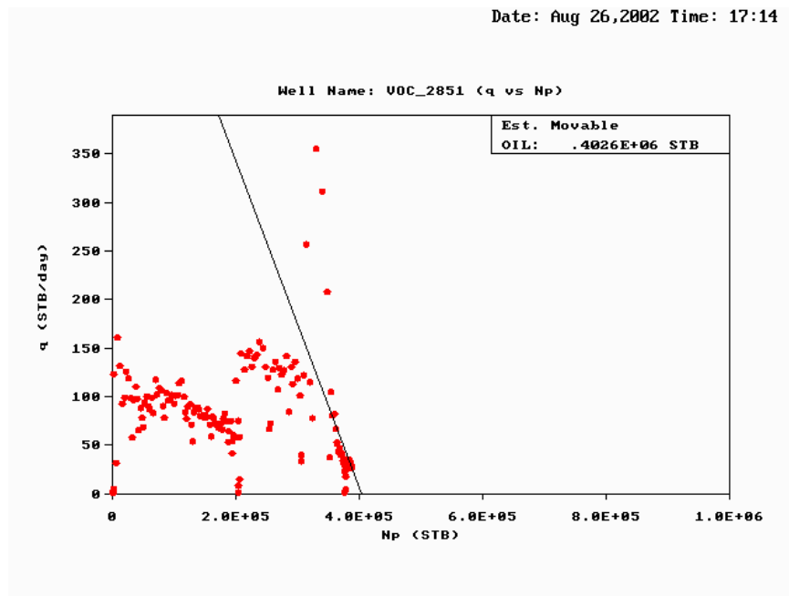
Figure 233 — Calculation of Recoverable Oil, Vocation Well 2851.
