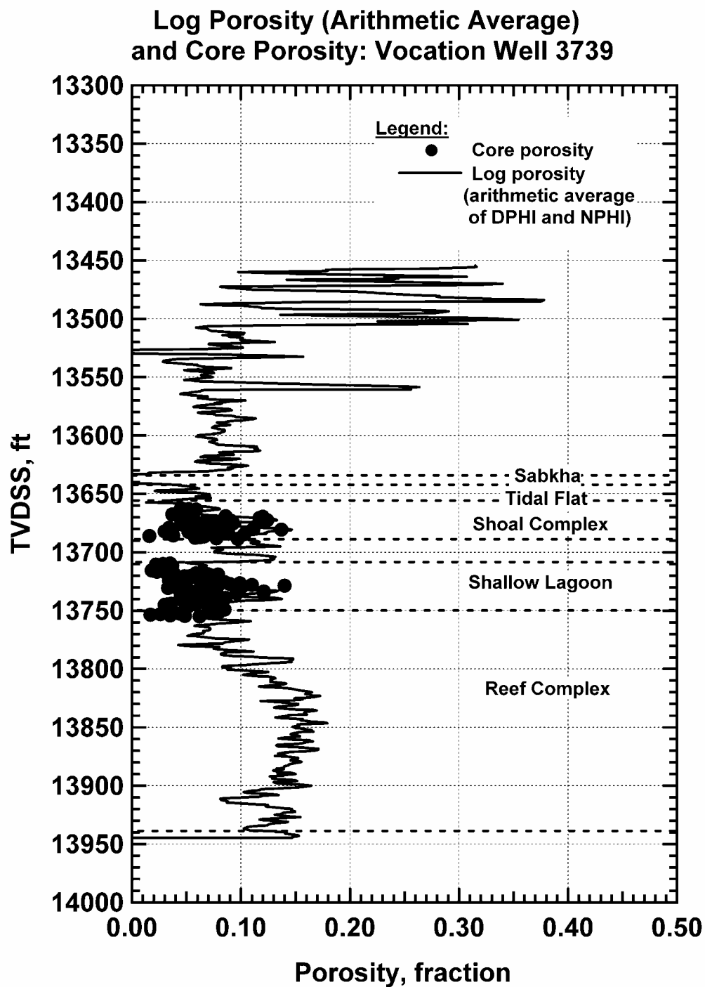
Figure 196 — Porosity Variation with Depth, Vocation Well 3739.
