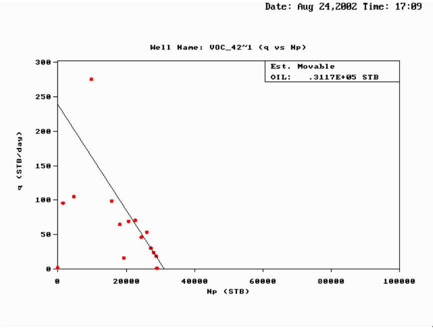
Figure 238 — Calculation of Recoverable Oil, Vocation Well 4225B.
