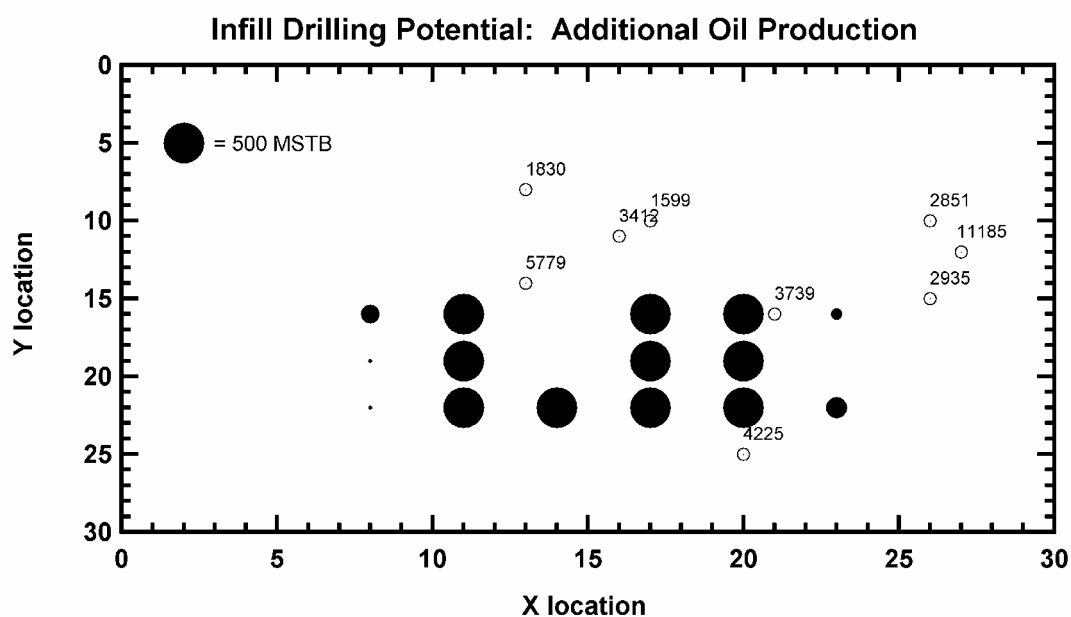
Figure 318 — Incremental oil production via an infill well at various locations, Vocation Field.
