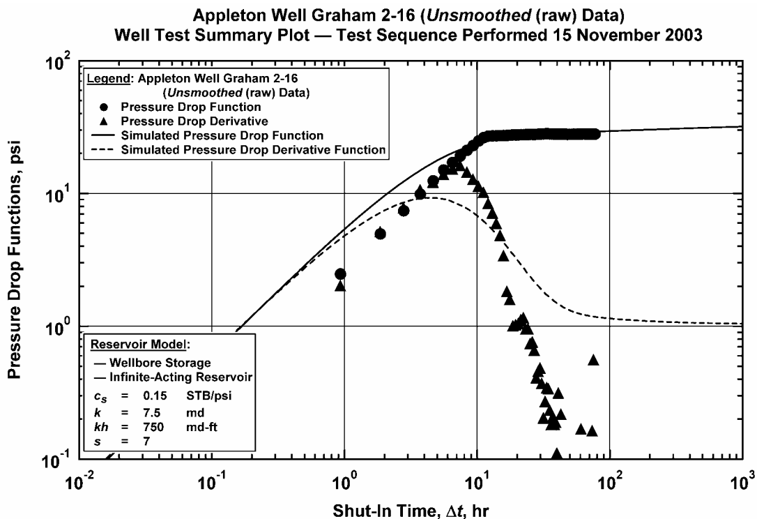
Figure 171d — Log-log Summary Plot (with Analysis) for Graham Well 2-16 (testing sequence of November 2003) — raw pressure buildup data case.
