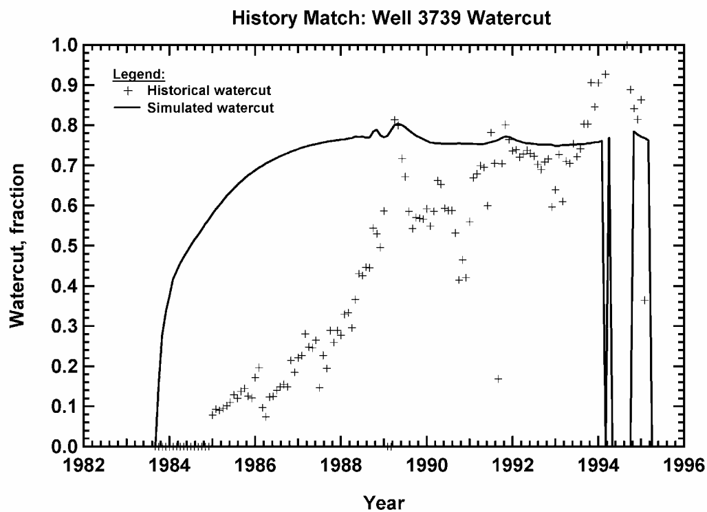
Figure 304 — Watercut history match, Vocation Well 3739.
