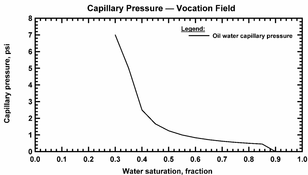
Figure 288 — History matched capillary pressure, Vocation Field.
