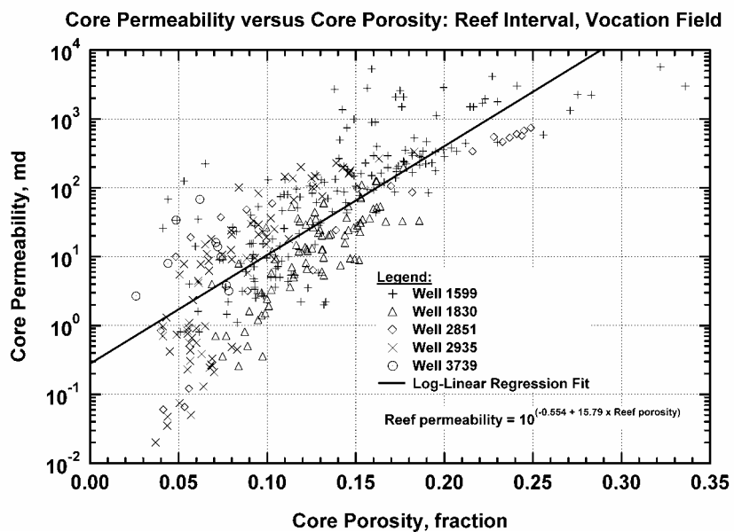
Figure 220 — Core Permeability versus Core Porosity, Reef.
