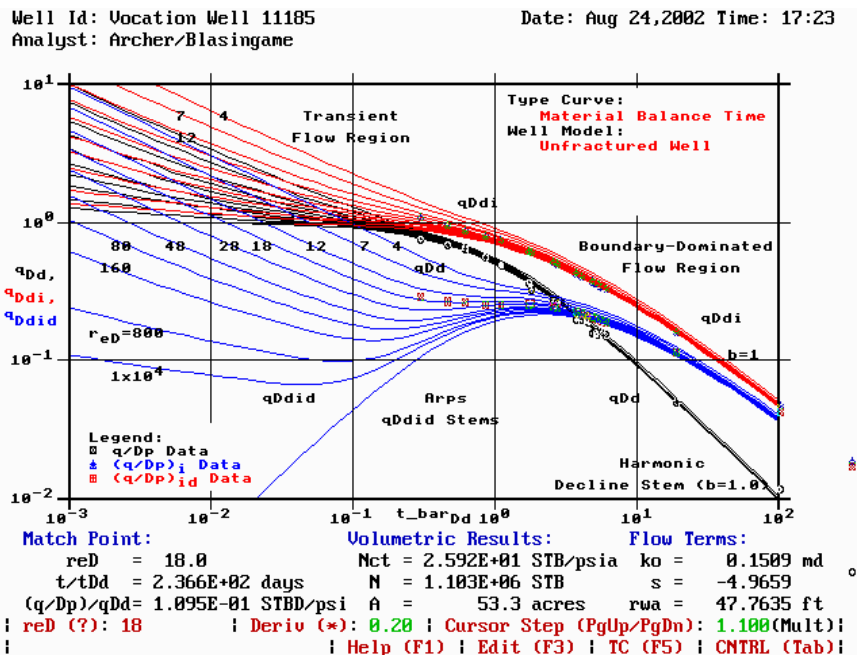
Figure 230 — Type Curve Match, Vocation Well 11185.
