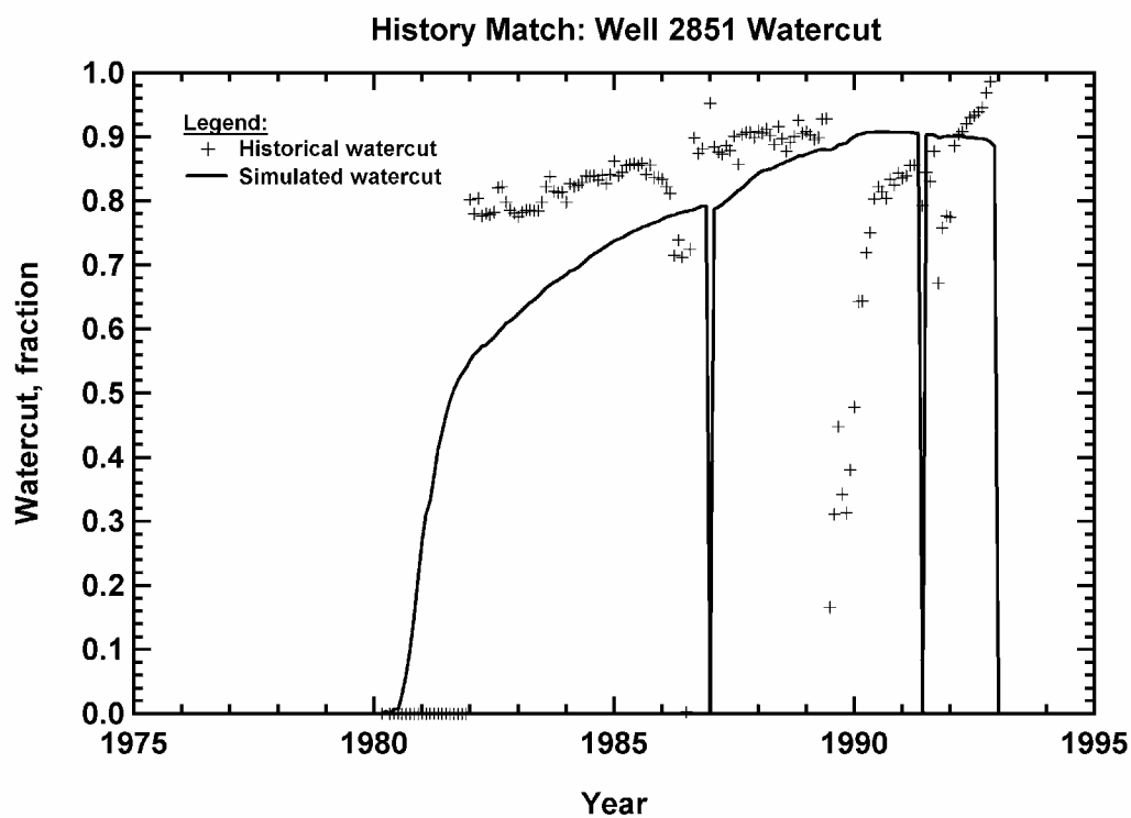
Figure 301 — Watercut history match, Vocation Well 2851.
