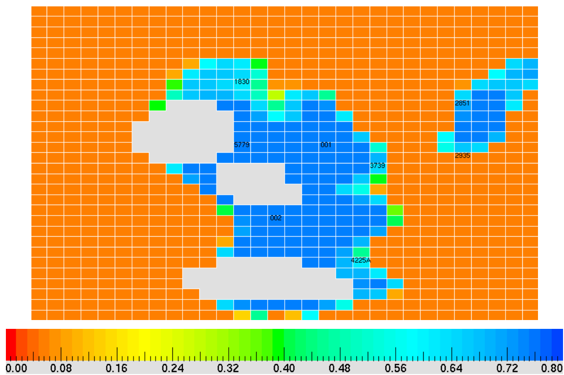
Figure 310 — Oil saturation in intermediate simulation layer (50ft from reservoir top) 1971, Vocation Field.
