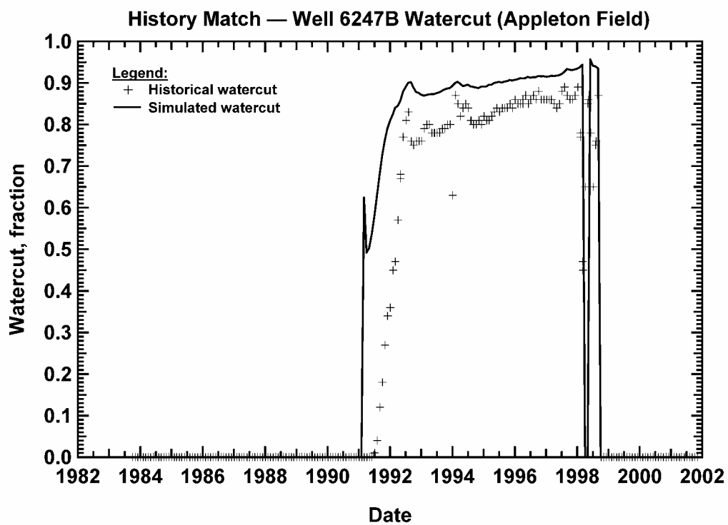
Figure 281 — Watercut history match, Well 6247B (Appleton Field).
