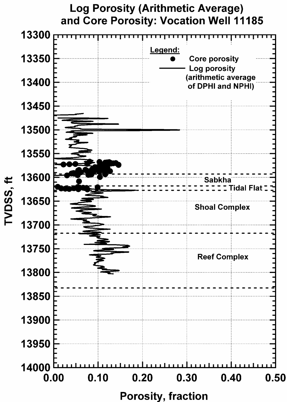
Figure 199 — Porosity Variation with Depth, Vocation Well 11185.
