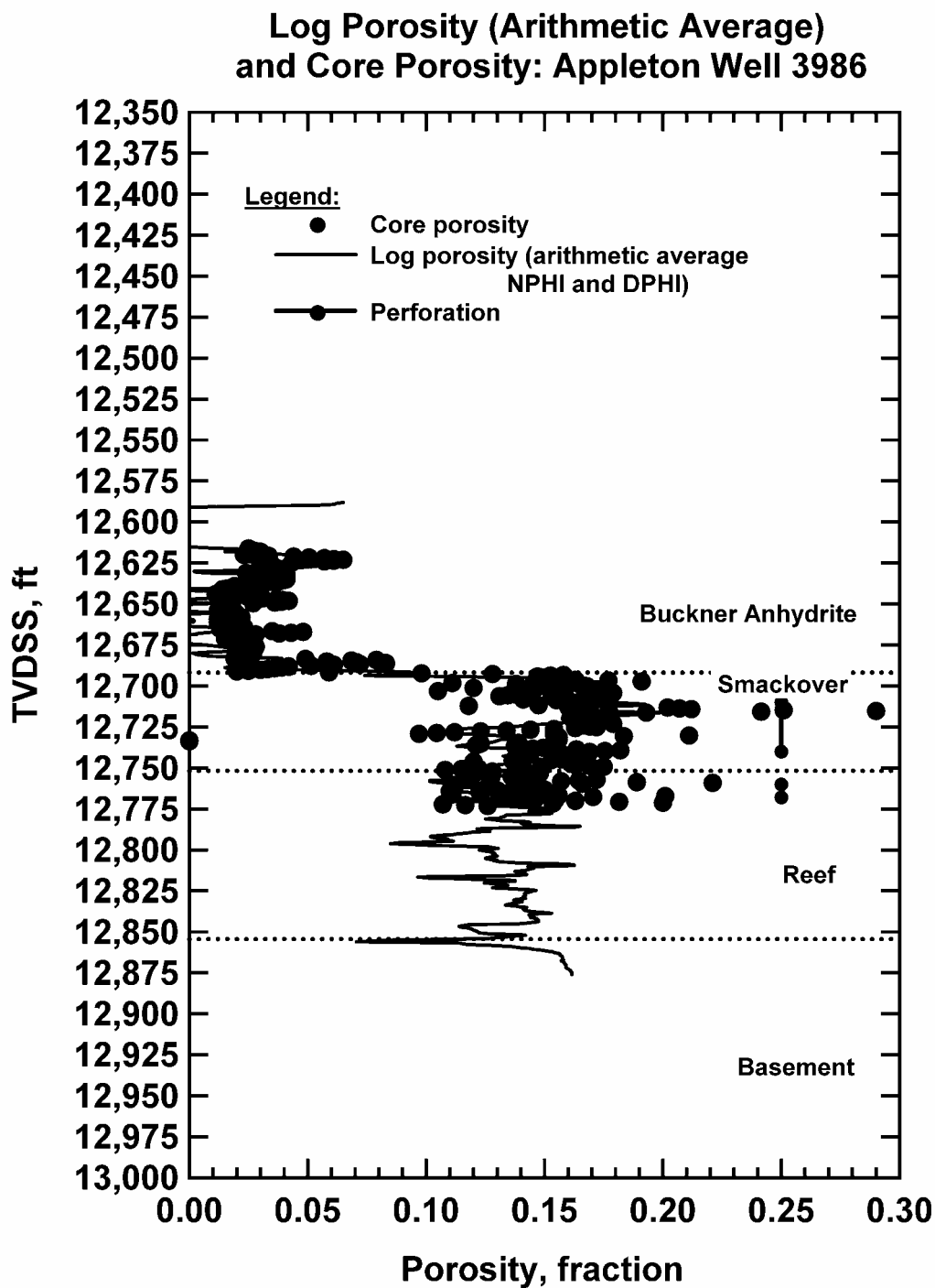
Fig. 139 — Porosity Variation with Depth, Appleton Well 3986
