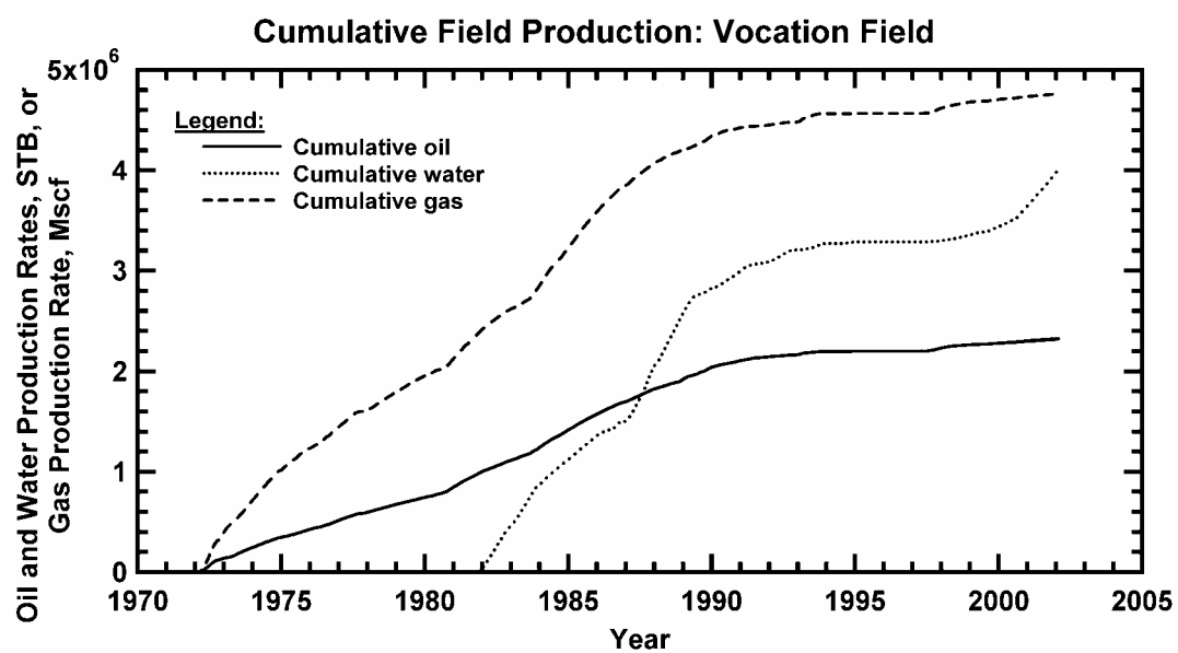
Figure 293 — Cumulative Production Profiles, Vocation Field.
