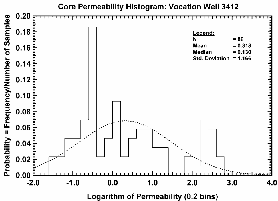
Figure 186 — Core Permeability Histogram, Vocation Well 3412.
