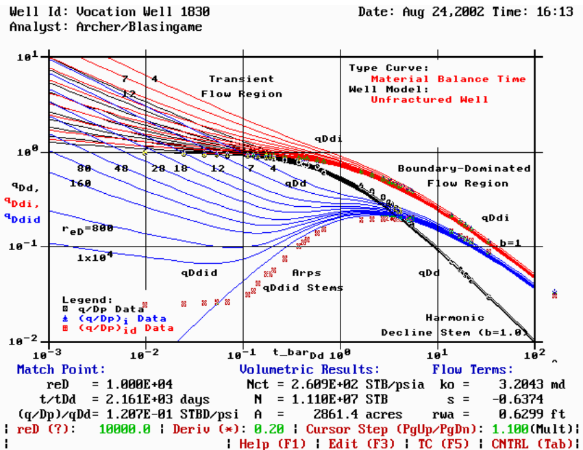
Figure 222 — Type Curve Match, Vocation Well 1830.
