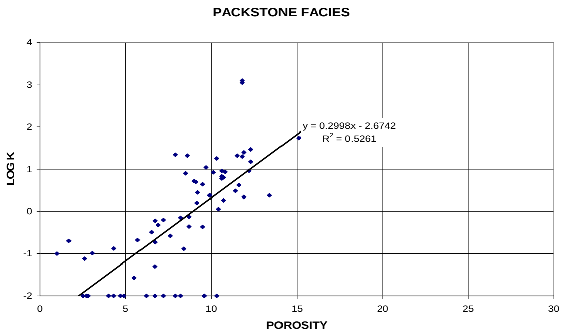
Figure 125. Porosity-permeability plot showing correlation to rock type in Vocation field.
