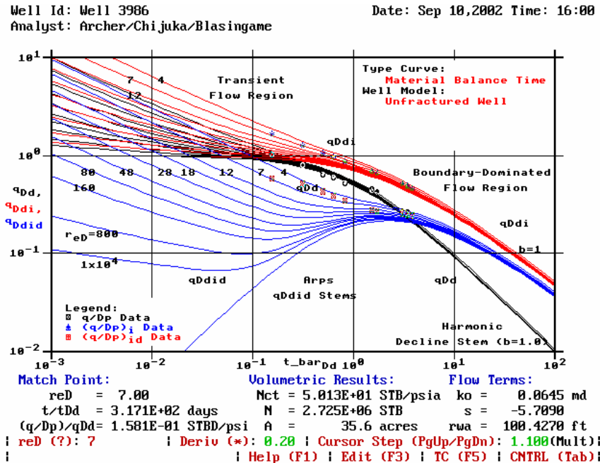
Fig. 154 — Type Curve Match, Appleton Well 3986.
