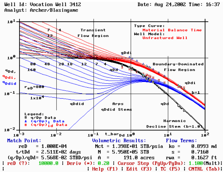
Figure 225 — Type Curve Match, Vocation Well 3412.
