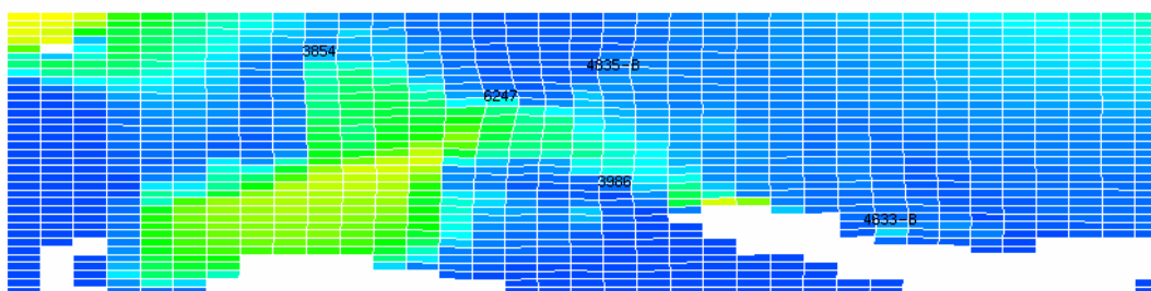
Figure 284 — Water saturations in 1993 at the top of the reef
