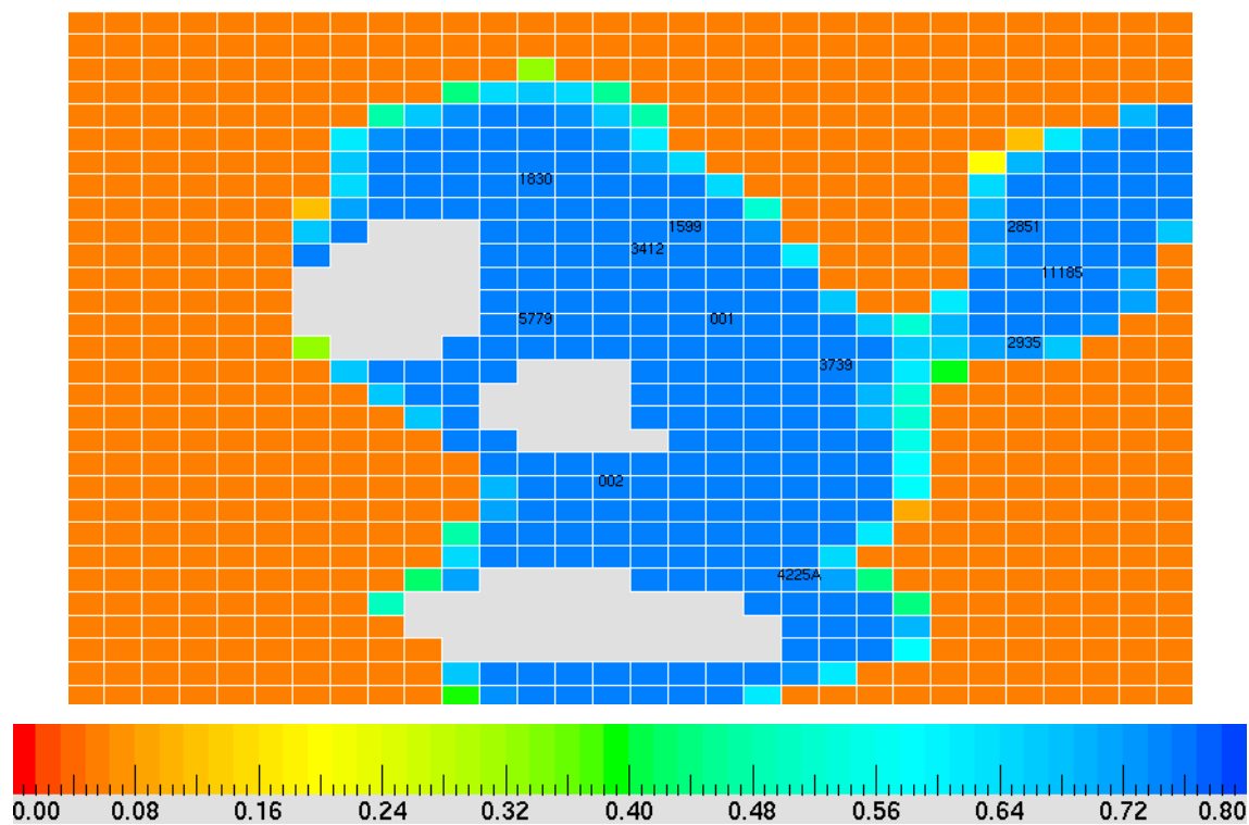
Figure 309 — Oil saturation in top simulation layer 1971, Vocation Field.
