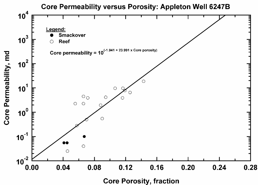
Fig. 152 — Core Permeability versus Core Porosity, Appleton Well 6247B.
