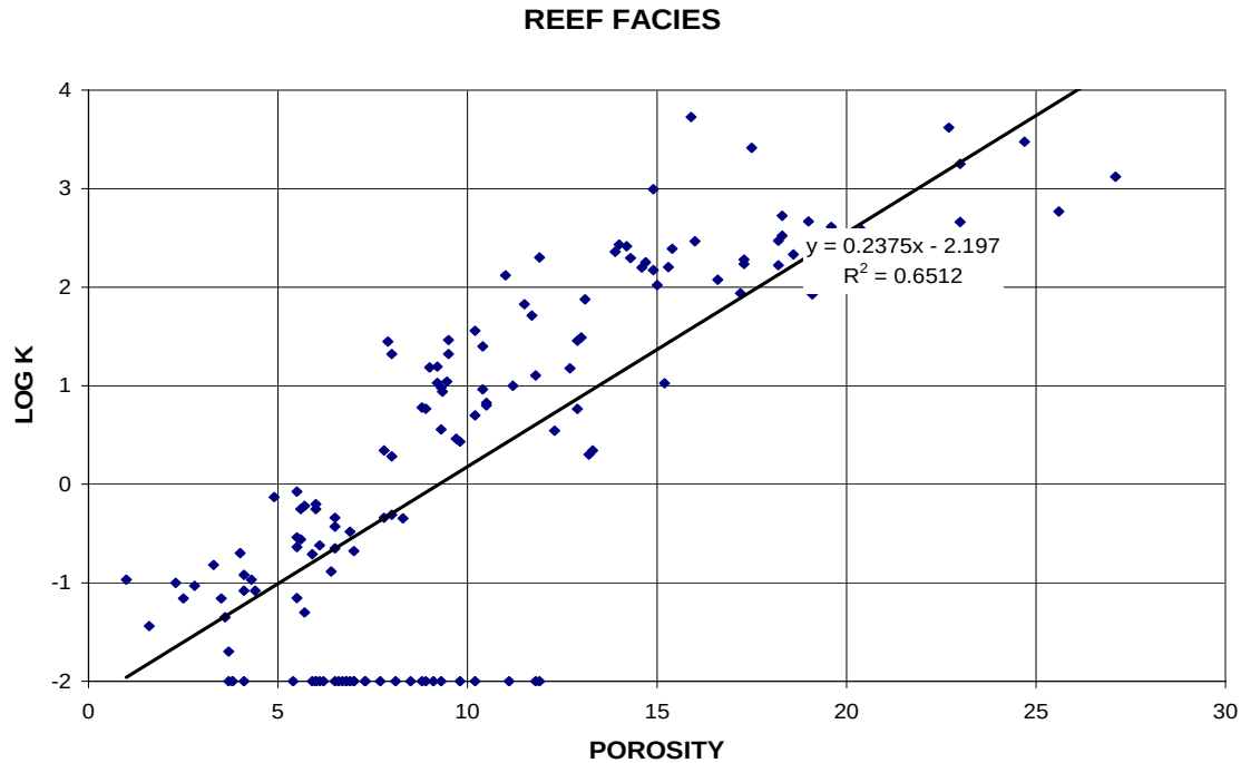
Figure 127. Porosity-permeability plot showing correlation to rock type in Vocation field.
