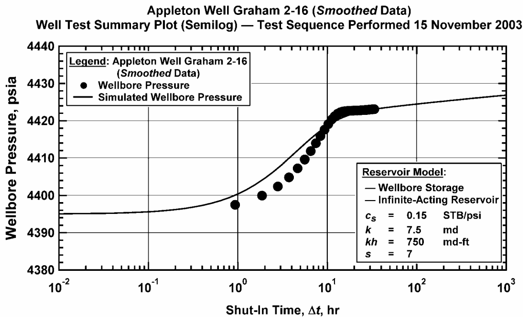
Figure 171f — Semilog Summary Plot (with Analysis) for Graham Well 2-16 (testing sequence of November 2003) — smoothed pressure buildup data case. Appleton Field (Alabama, USA)
