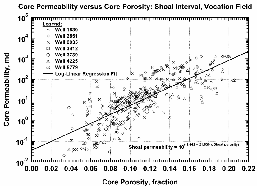
Figure 218 — Core Permeability versus Core Porosity, Shoal.
