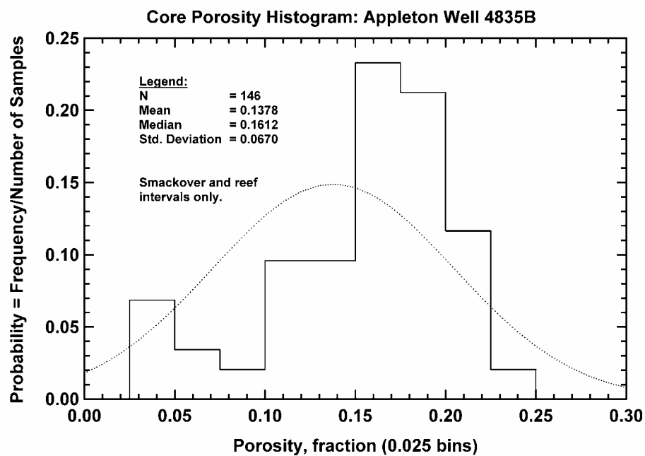
Fig. 131 — Core Porosity Histogram, Appleton Well 4835B
