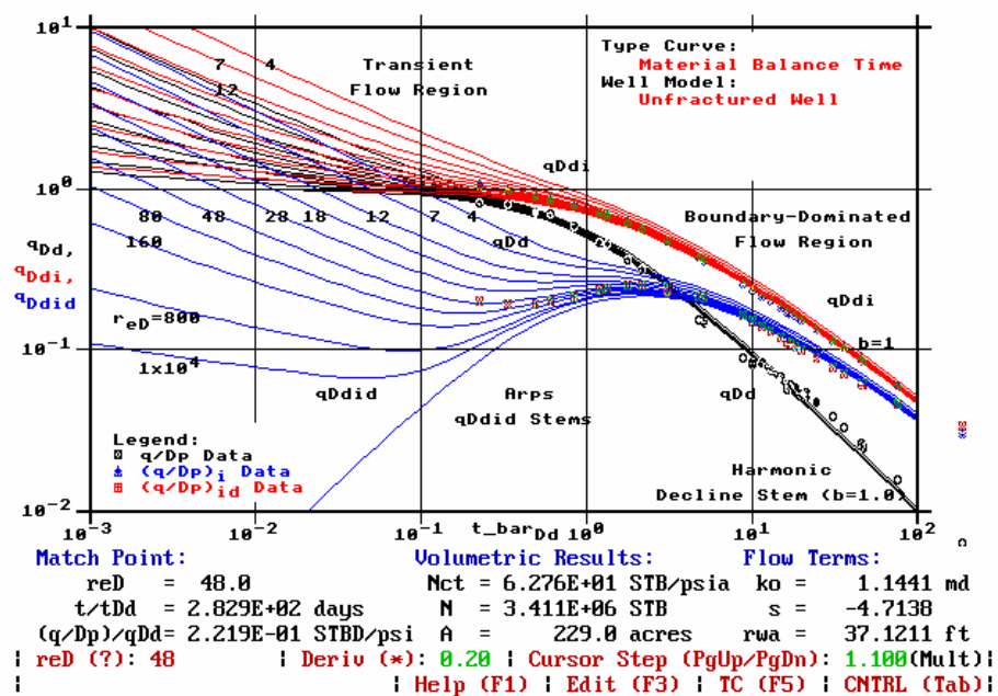
Fig. 157 — Type Curve Match, Appleton Well 6247B.
