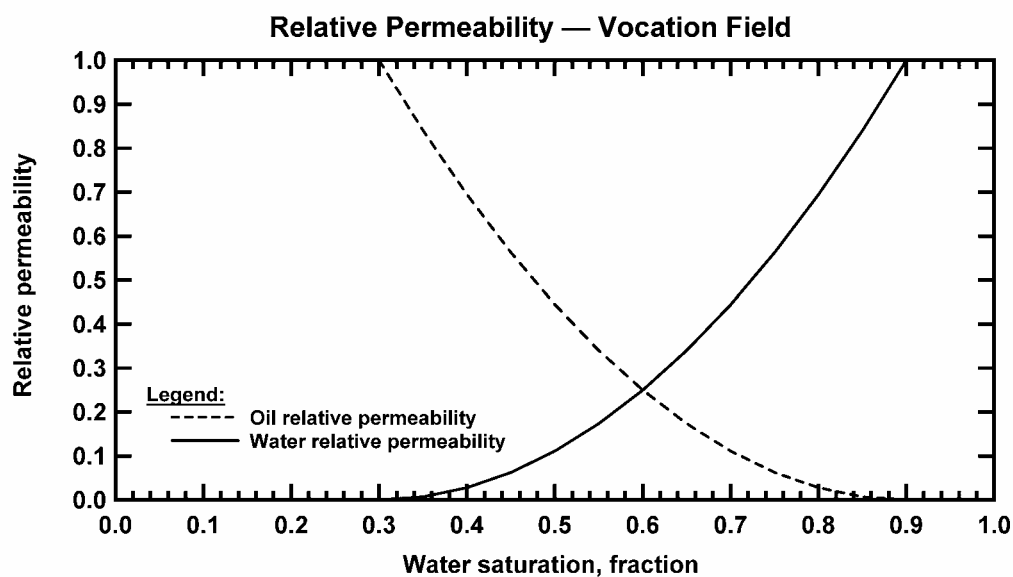
Figure 287 — History matched relative permeability curves, Vocation Field.
