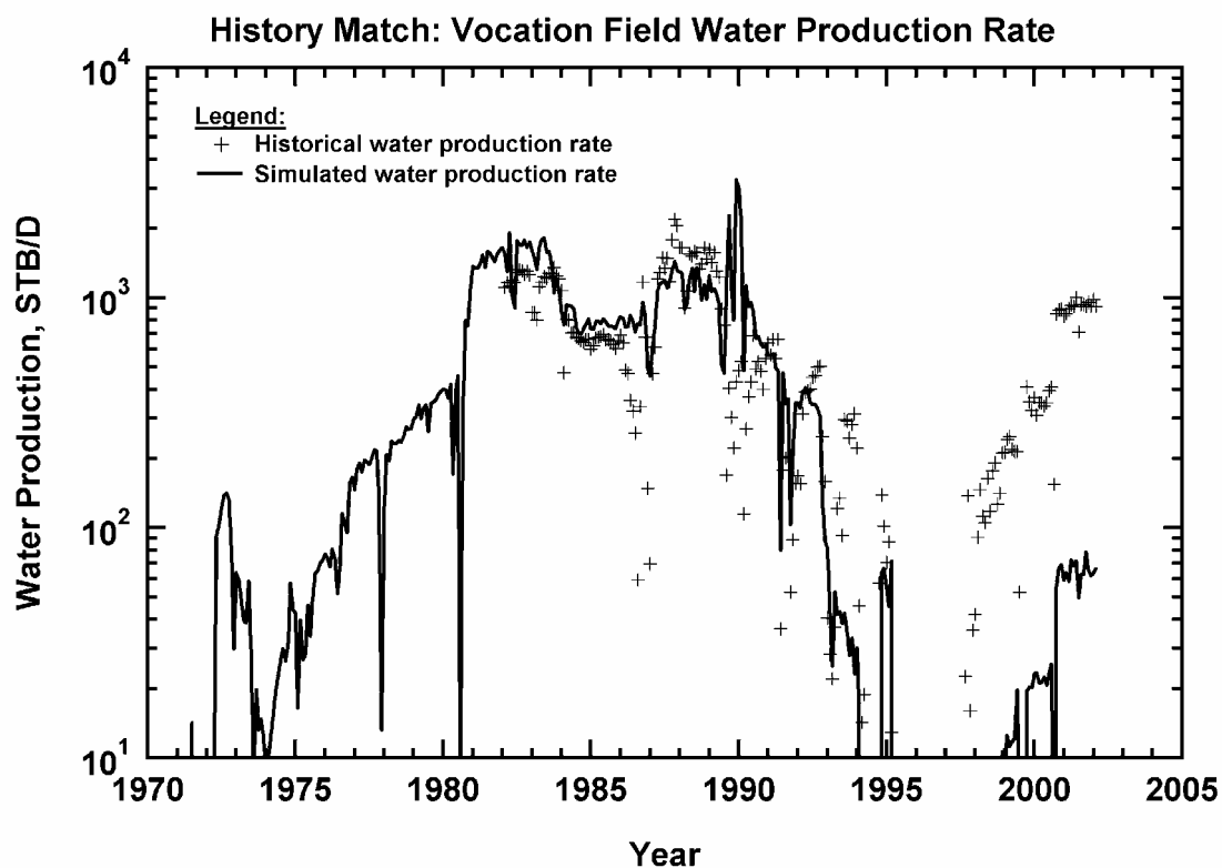
Figure 297 — Water production rate history match, Vocation Field.
