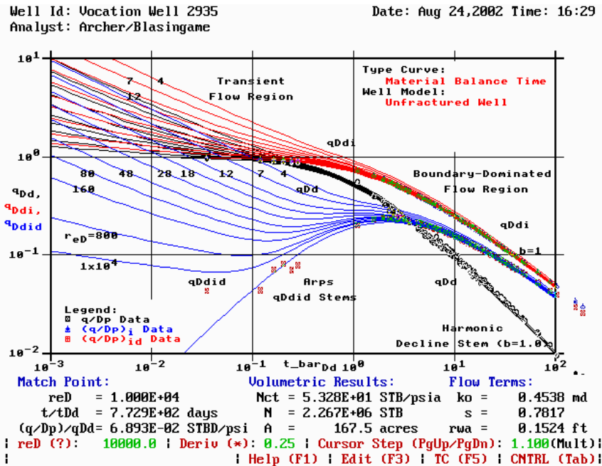
Figure 224 — Type Curve Match, Vocation Well 2935.
