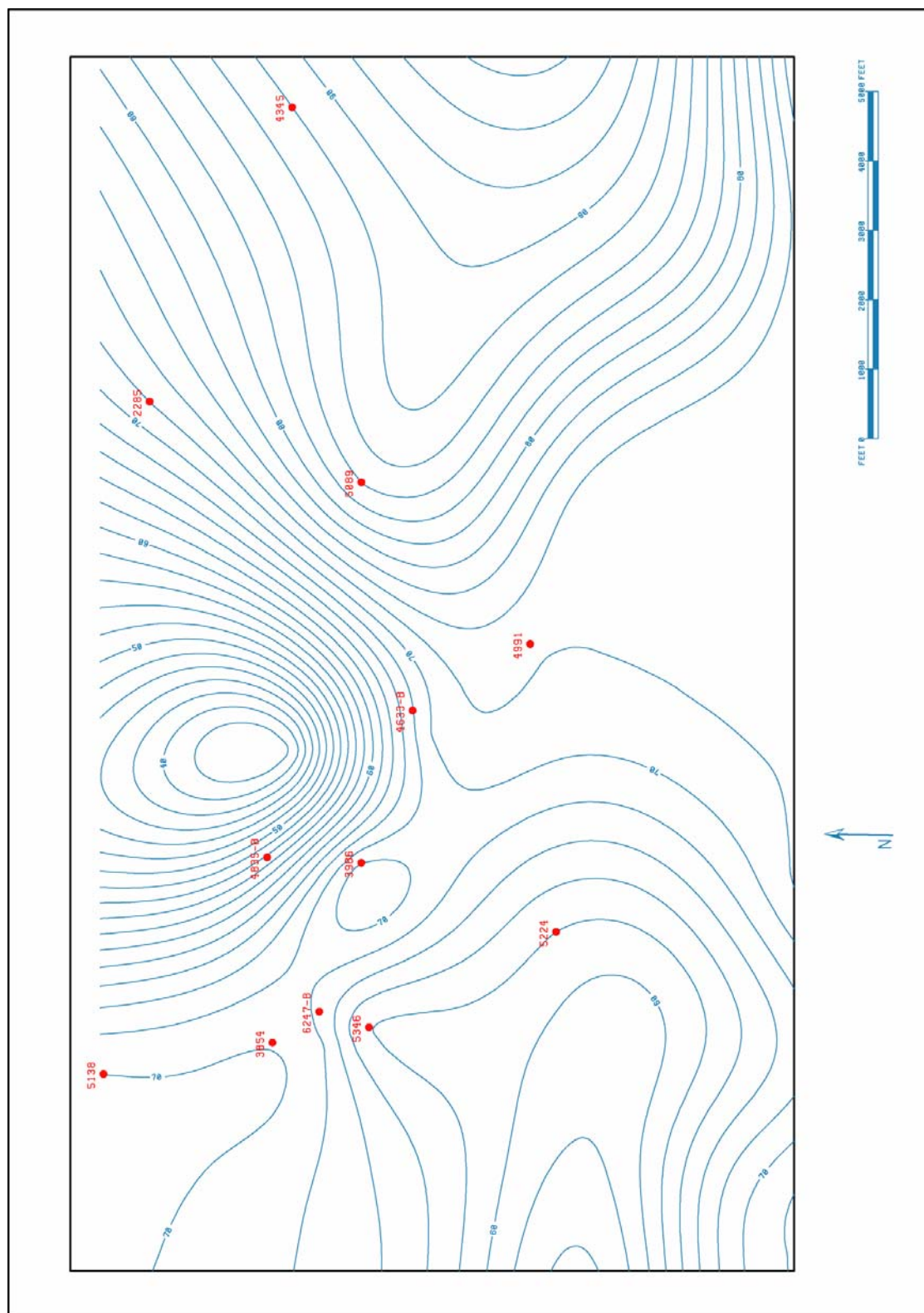
Figure 23. Thickness map of shoal facies (from log data).
