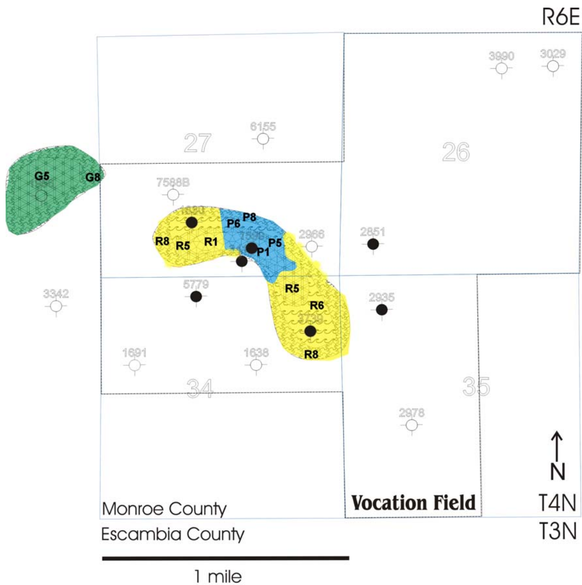
Figure 116. Vocation Flow Unit Slice Map 250 ft below Top of Smackover.
