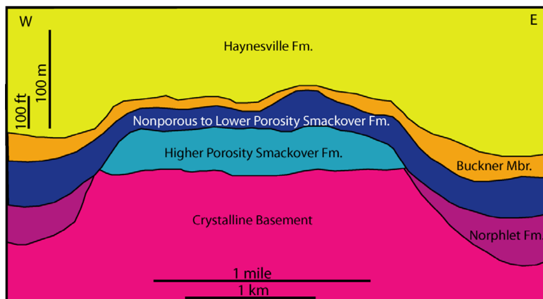
Figure 252. (A) Interpreted seismic project in the Appleton Field area, and (B) geologic model based on the seismic interpretation of Appleton Field. The seismic data show the distribution of the thrombolite buildup on the crystalline basement paleohigh in the Appleton Field area.
