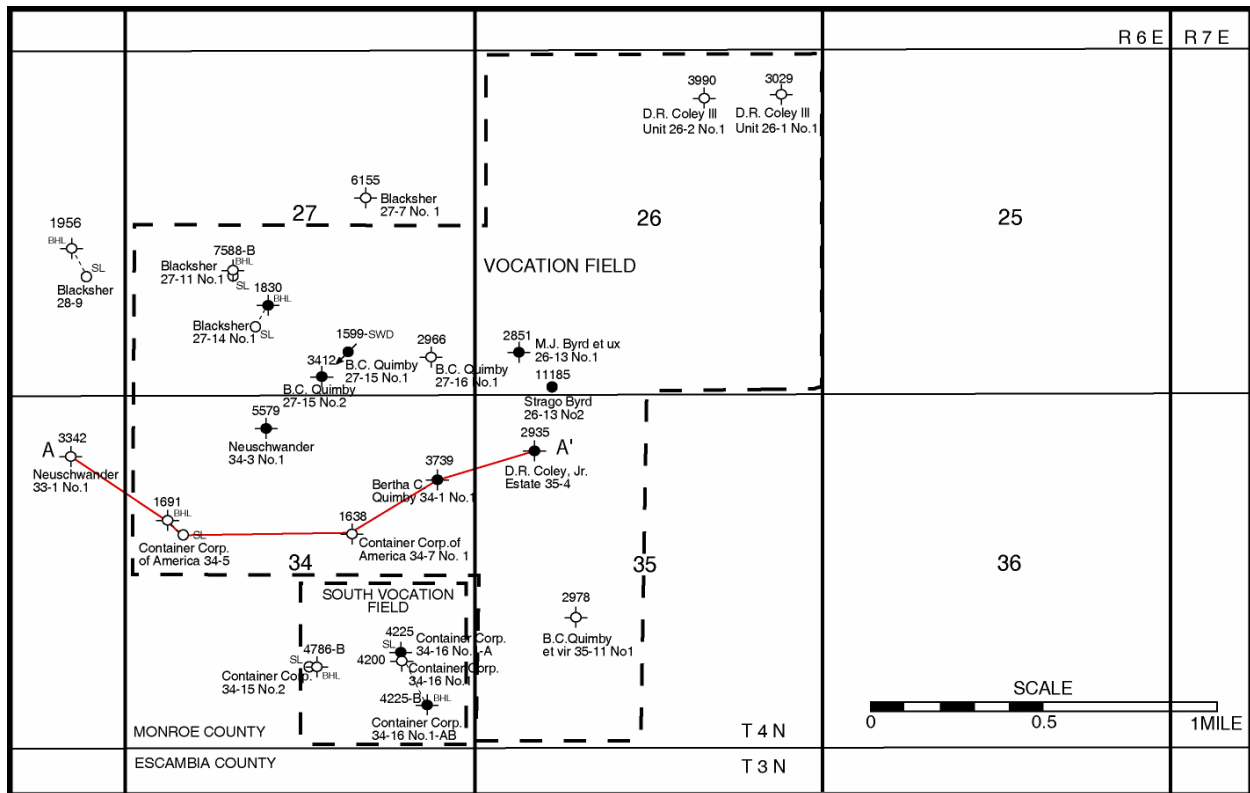
Figure 5. Vocation Field area.
