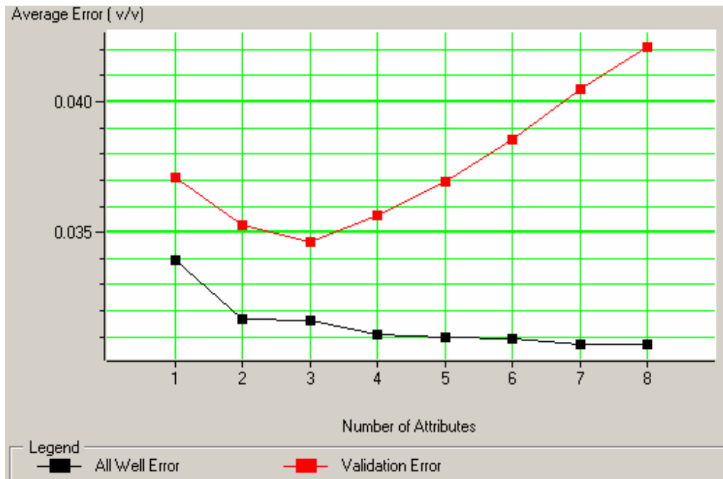
Figure 63: Validation plot, showing variation in all-well error and validation error in predicting porosity from apparent porosity logs using stepwise linear regression. The increase in validation error after the third attribute indicates that the optimum number of attributes to use is three. See Hampson et al. (2001) for a full description and justification of the method.
