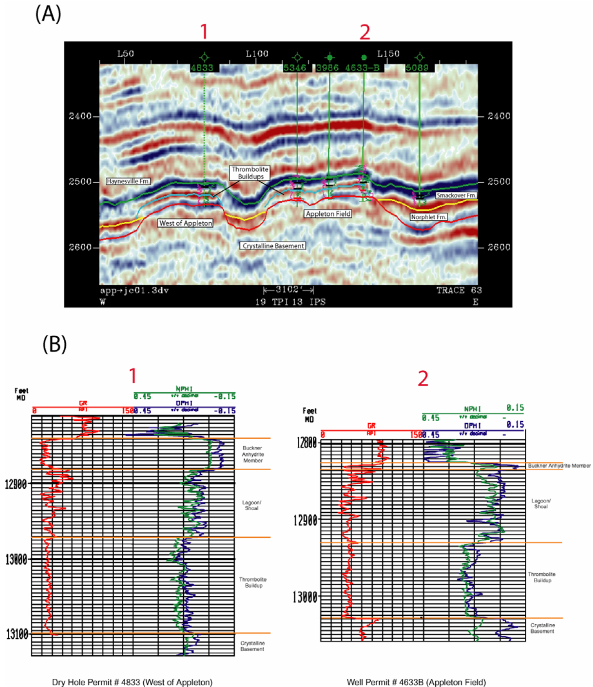
Figure 321. (A) Seismic profile oriented in an approximate strike direction showing the thrombolite buildups on the Appleton paleohigh and on a paleohigh west of Appleton Field, and (B) representative logs from wells for these areas illustrating the characteristic regular pattern of lower gamma ray (GR) values coupled with relative high density (DPHI) and neutron (NPHI) porosity values for the thrombolite facies (dry hole Permit #4833 and well Permit #4633B).
