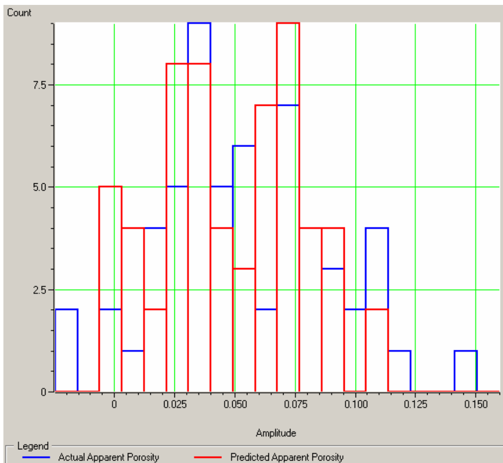
Figure 70: Histogram comparing the actual range of porosity values and those predicted using the MLR trend-cascaded PNN method (statistically and geologically preferred method).
