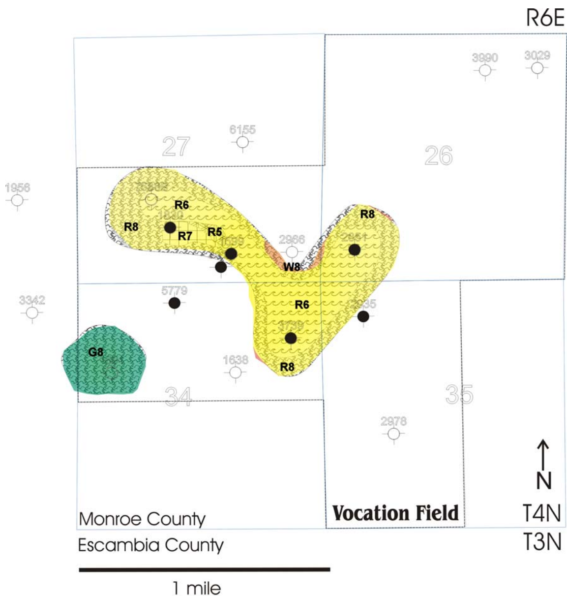
Vocation Flow Unit Slice Map 150 ft Below Top Smk
