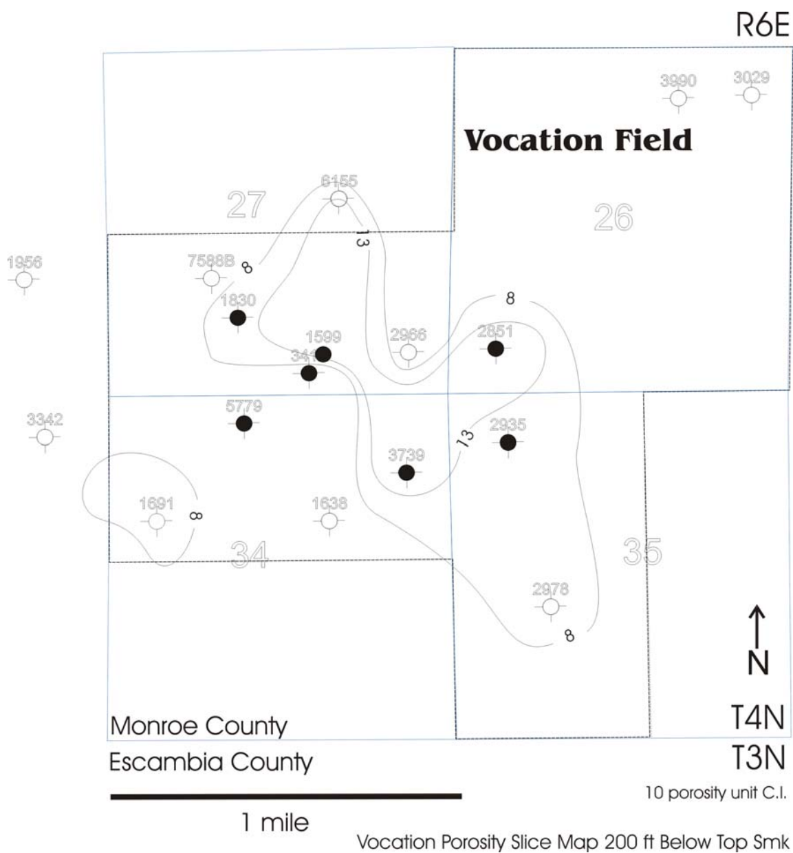
Figure 90. Vocation Porosity Slice Map 200 ft below Top of Smackover.
