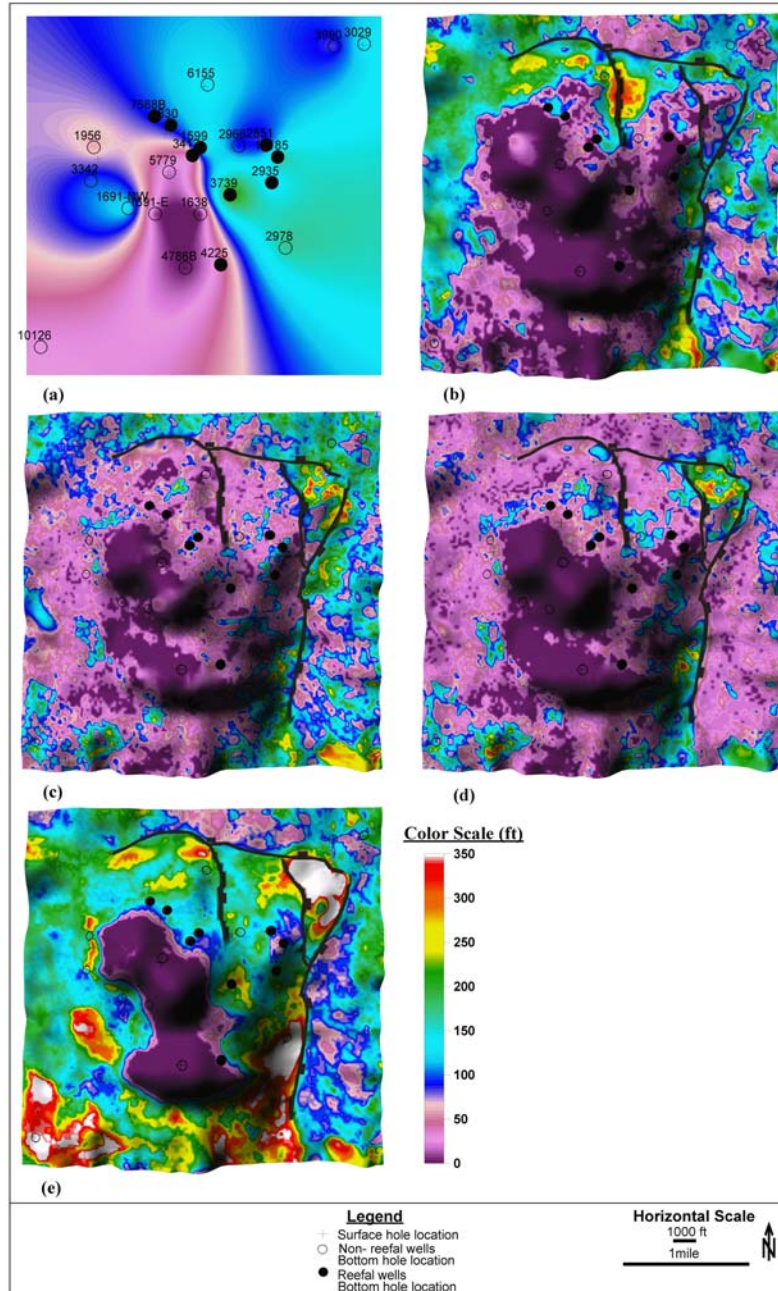
Figure 69: Porosity thickness map of the Smackover Formation overlain on the Buckner/Smackover depth-structure map for better display; a) based on contouring of wells only, b) MLR result, c) MLR trend-cascading PNN result, d) no trend cascaded PNN, and e) MLFN. Note the overall lack of porosity at the crests of structure, and thicker porosity to the flanks of structure and along faults. Also note the prediction of high/thick porosity zones associated with faults in eastern part of the study area. Observed differences in the distribution of porosity are mainly a result of the method used.
