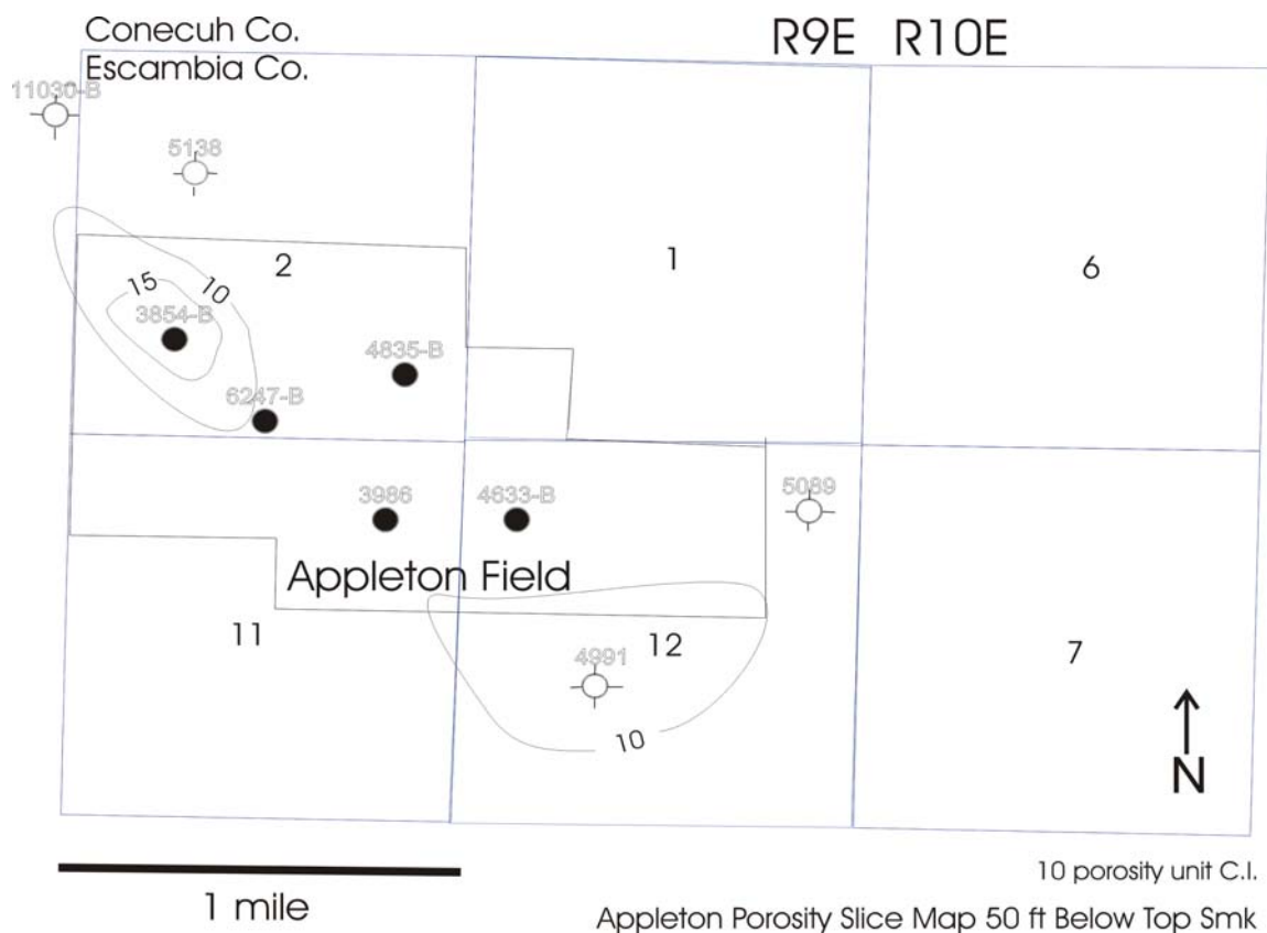
Figure 81. Appleton Porosity Slice Map 50 ft below Top of Smackover.
