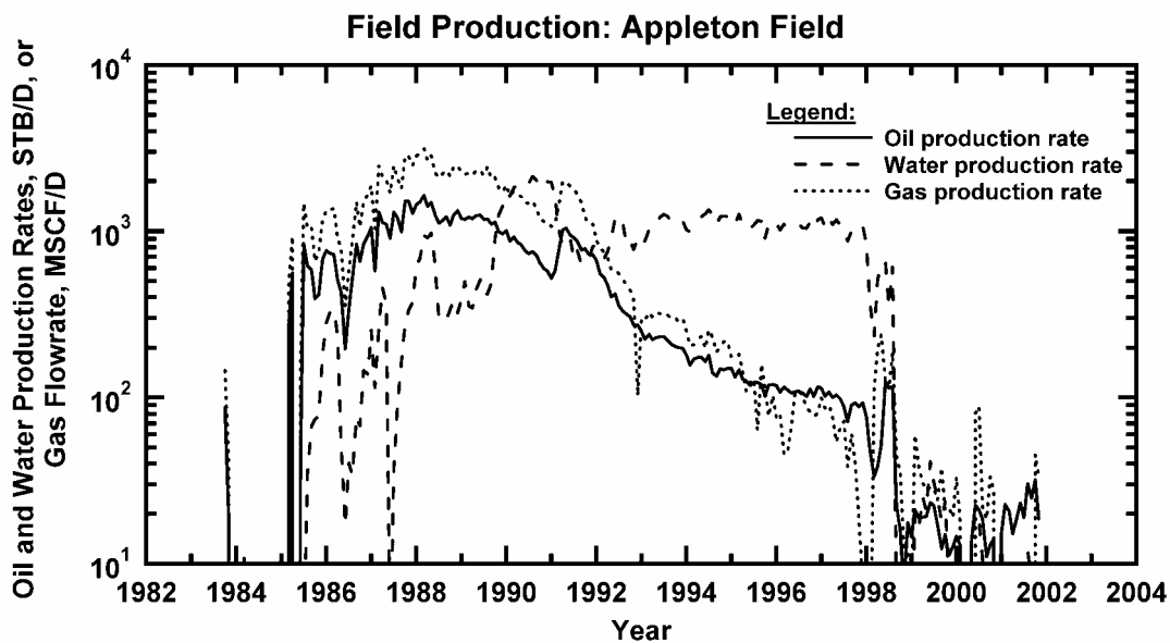
Figure 270 — Individual Phase Flowrates, Appleton Field (Semilog Format).
