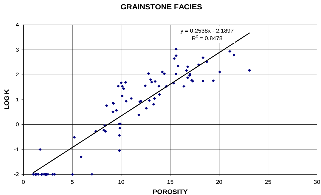
Figure 122. Porosity-permeability plot showing correlation to rock type in Appleton field.
