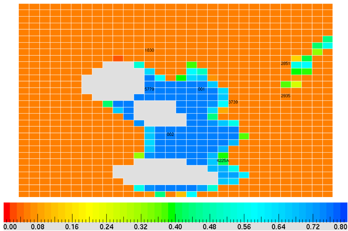
Figure 314 — Oil saturation in intermediate simulation layer (50ft from reservoir top) 2001, Vocation Field.
