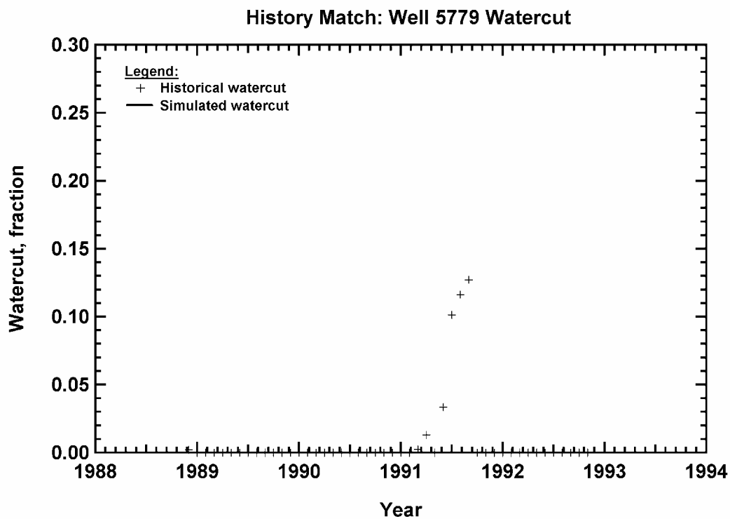
Figure 307 — Watercut history match, Vocation Well 5779.
