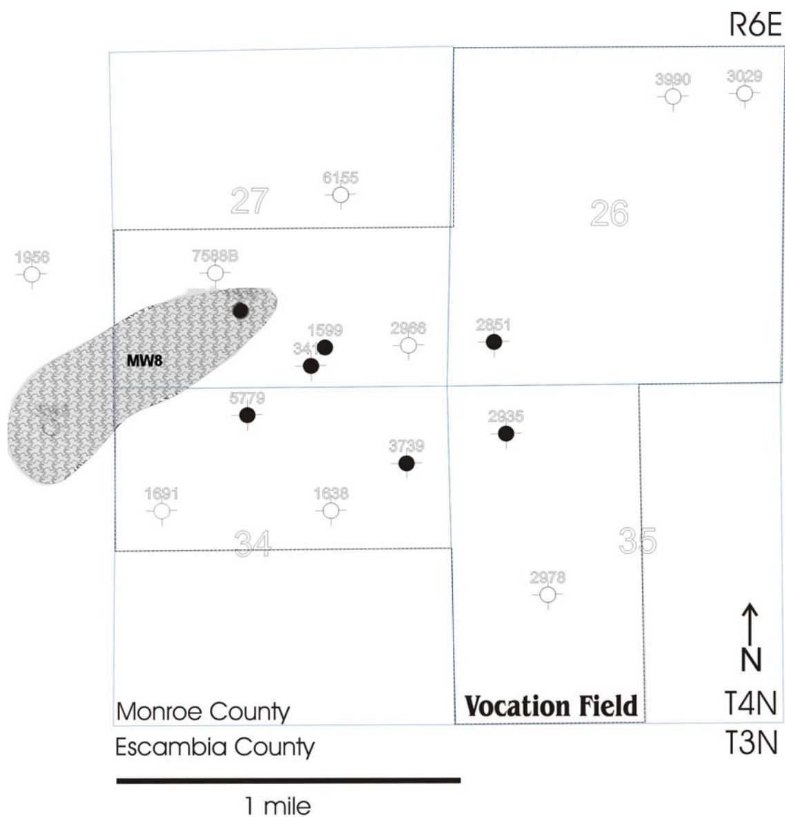
Vocation Flow Unit Slice Map 0-10 ft Below Top Smk
