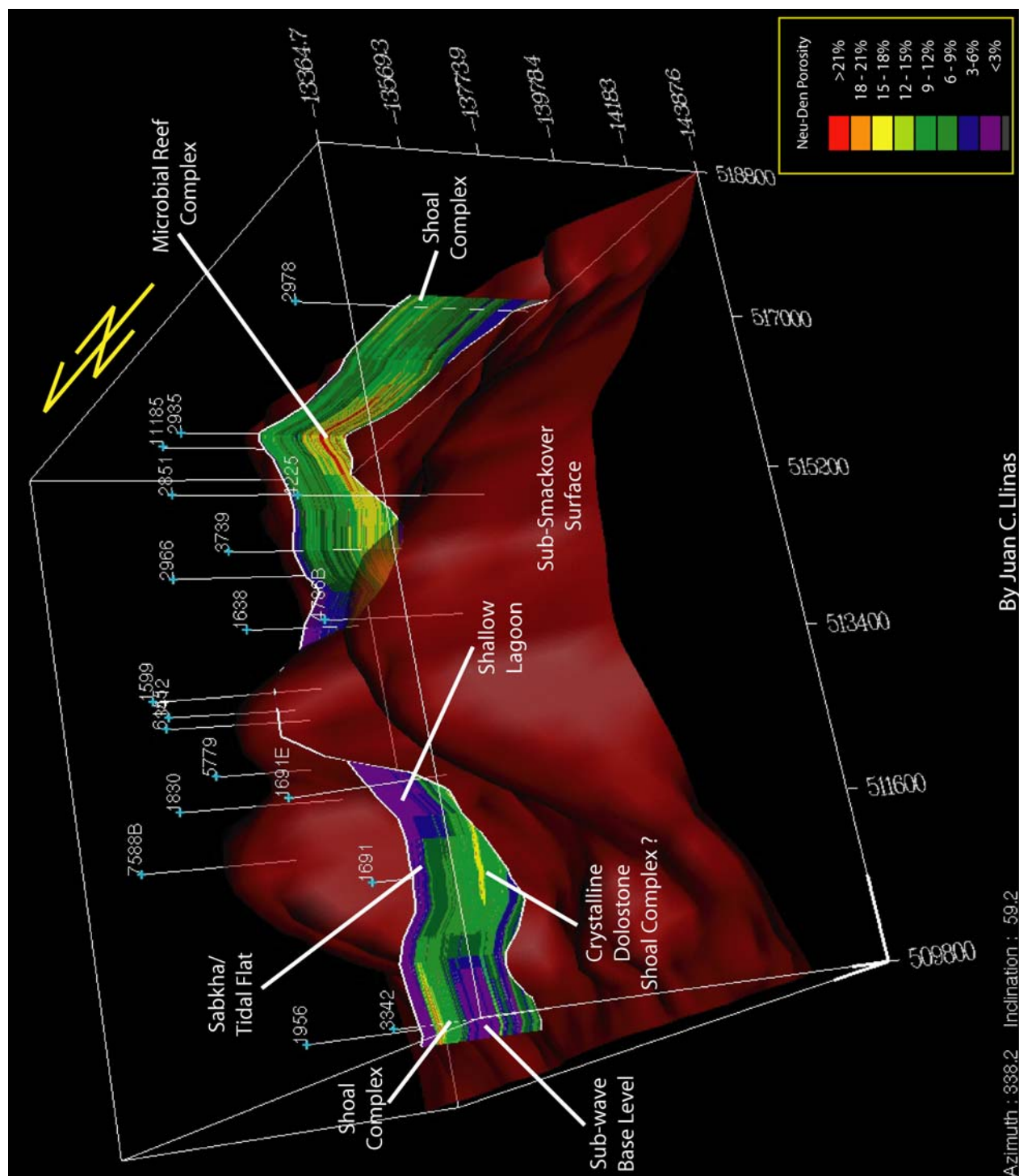
Figure 261. Depositional facies of the Smackover Formation in Vocation Field.
