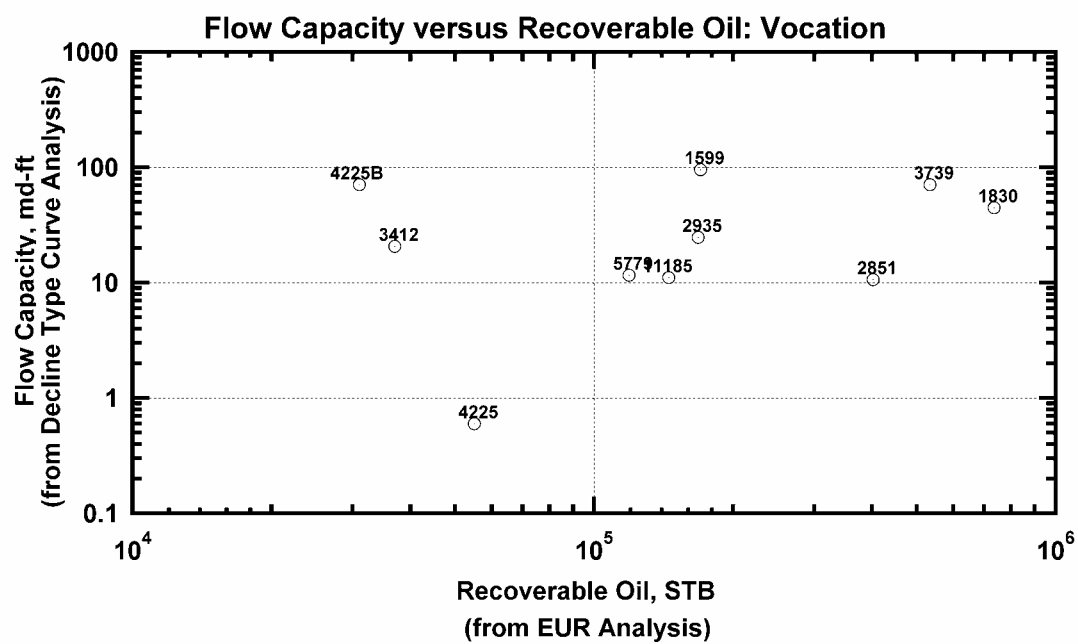
Figure 246 — Flow Capacity versus Recoverable Oil, Vocation Oil Field.
