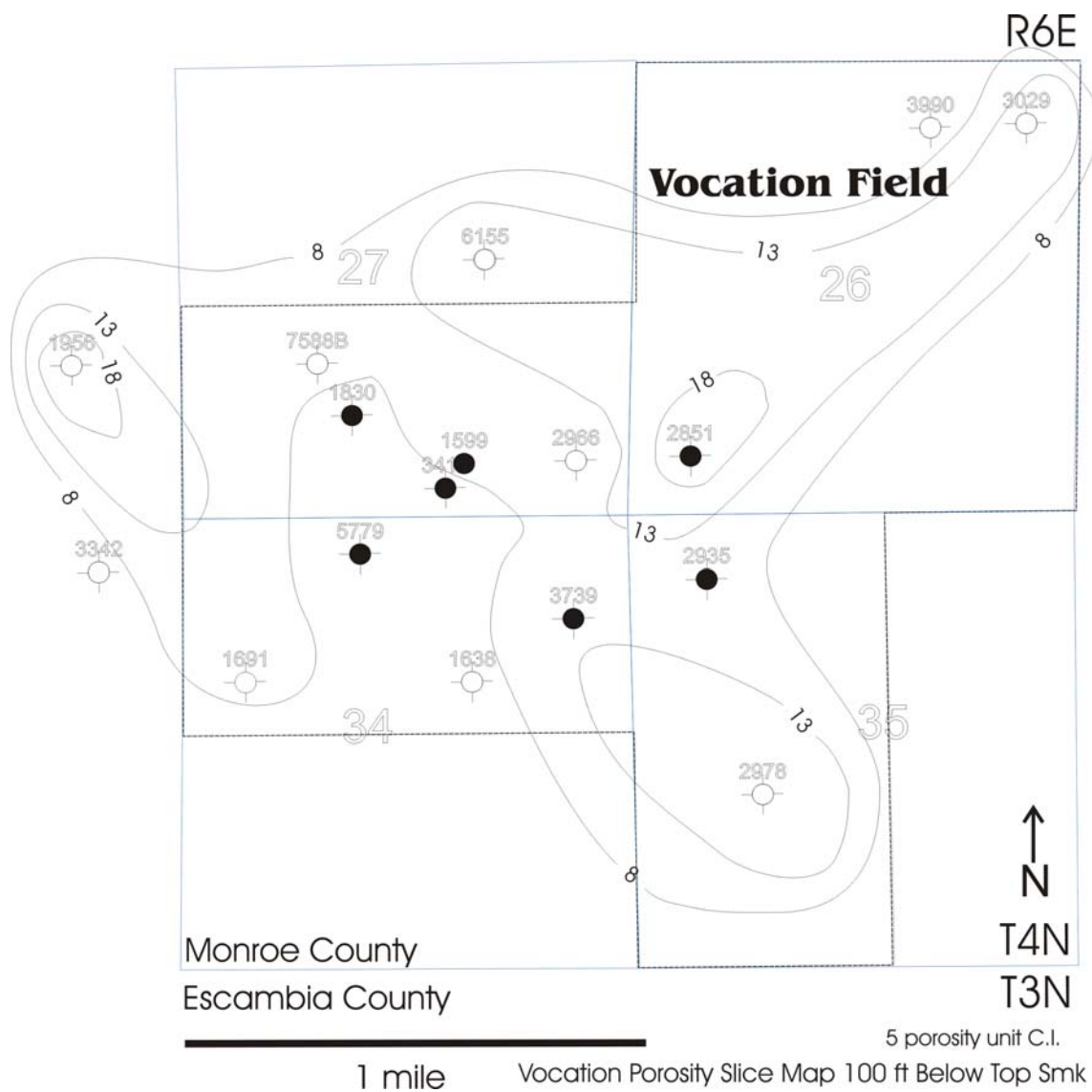
Figure 88. Vocation Porosity Slice Map 100 ft below Top of Smackover.
