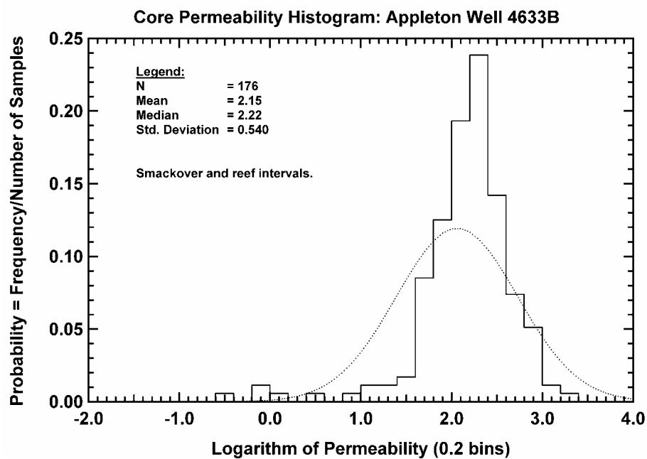
Fig. 135 — Core Permeability Histogram, Appleton Well 4633B
