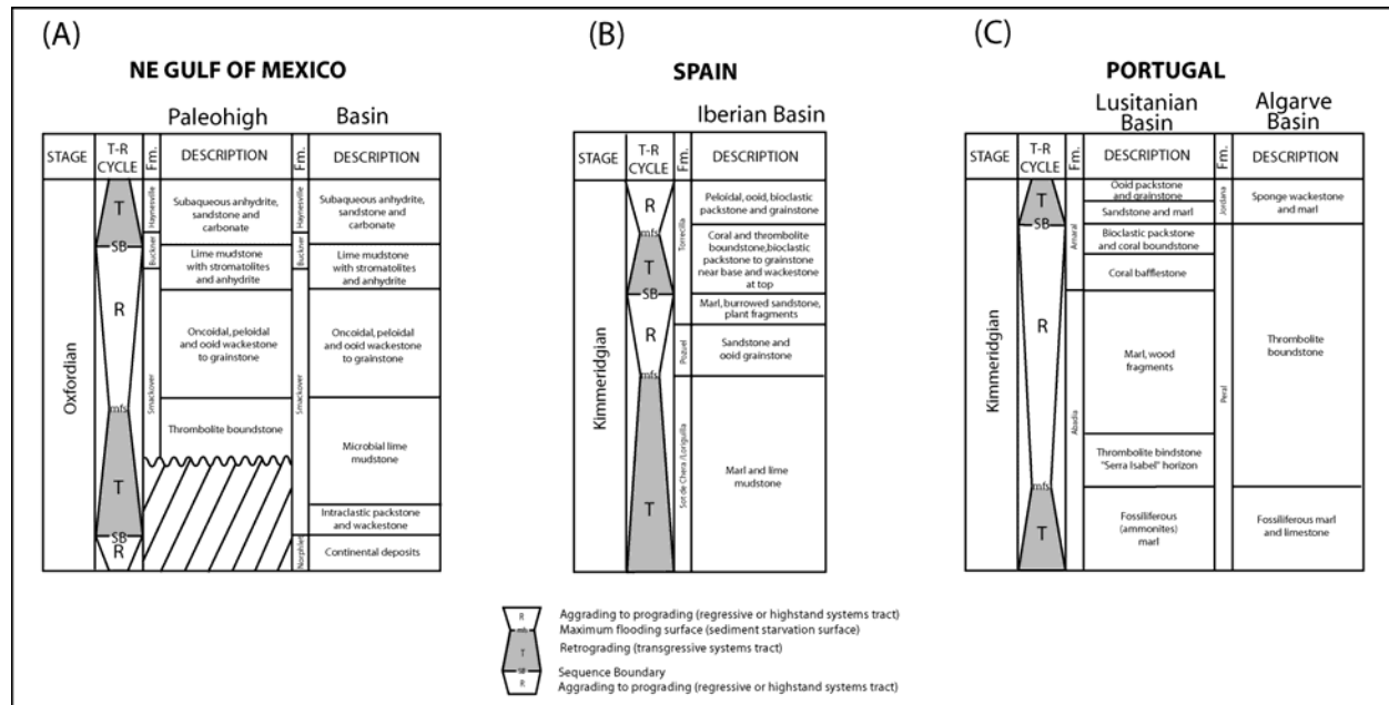
Figure. 324. Comparison of Upper Jurassic stratigraphy for: (A) the northeastern Gulf of Mexico, (B) Iberian Basin, Spain, and (C) Lusitanian and Algarve Basins, Portugal (modified from Leinfelder et al., 1993a; Aurell and Bádenas, 1997; Mancini and Parcell, 2001).
