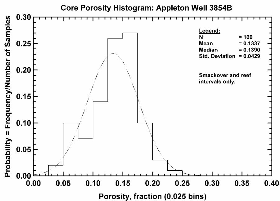
Fig. 128 — Core Porosity Histogram, Appleton Well 3854B
