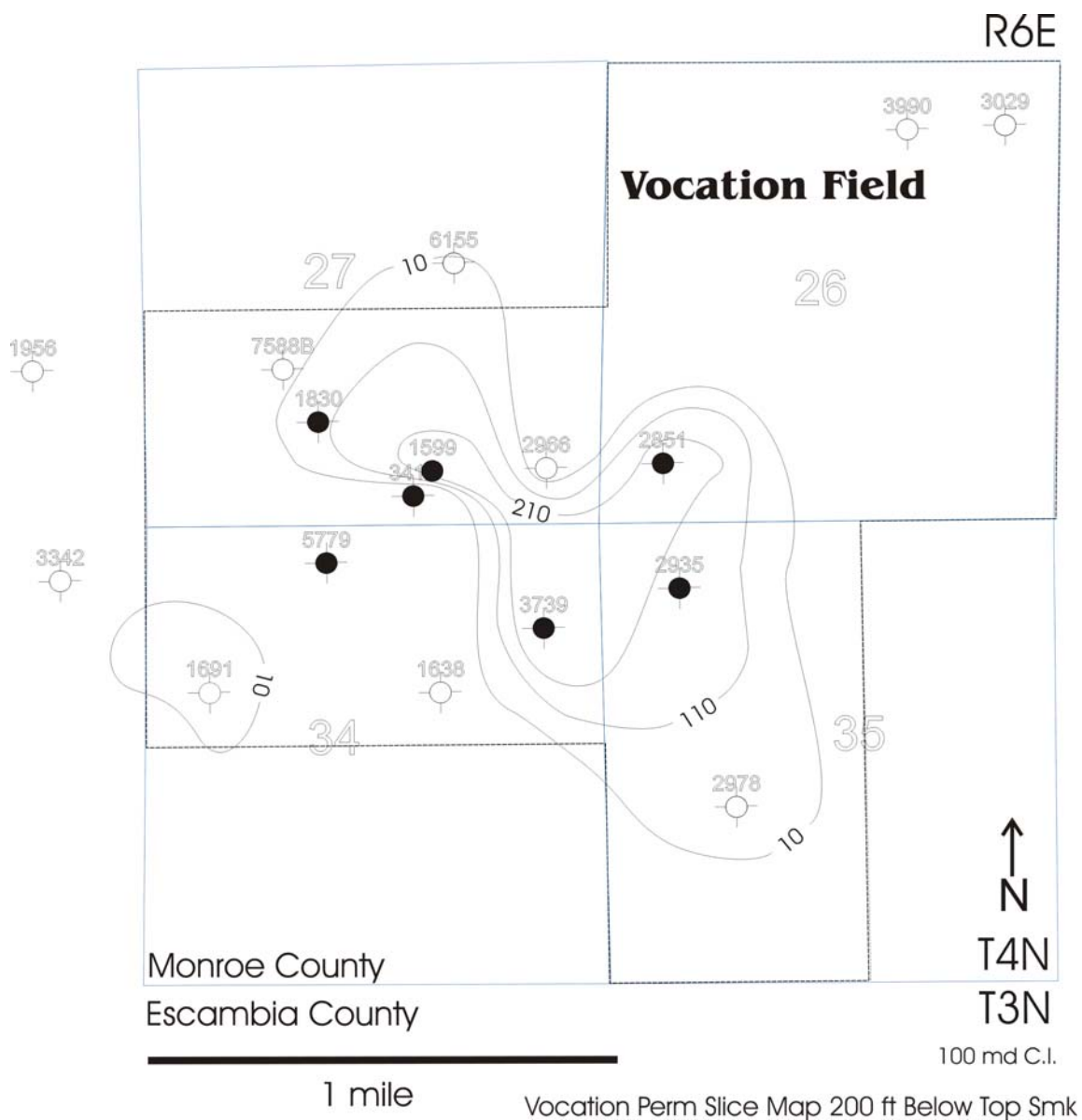
Figure 102. Vocation Permeability Slice Map 200 ft below Top of Smackover.
