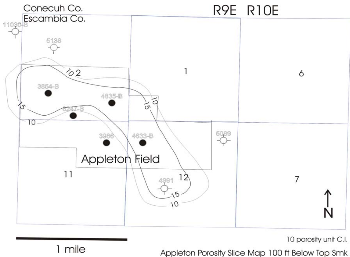
Figure 82. Appleton Porosity Slice Map 100 ft below Top of Smackover.
