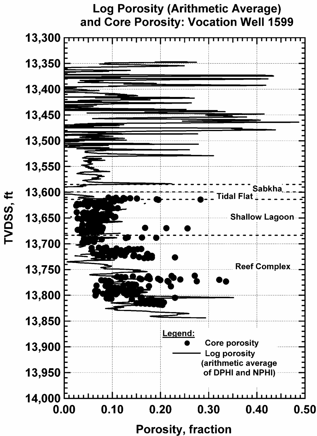
Figure 191 — Porosity Variation with Depth, Vocation Well 1599.
