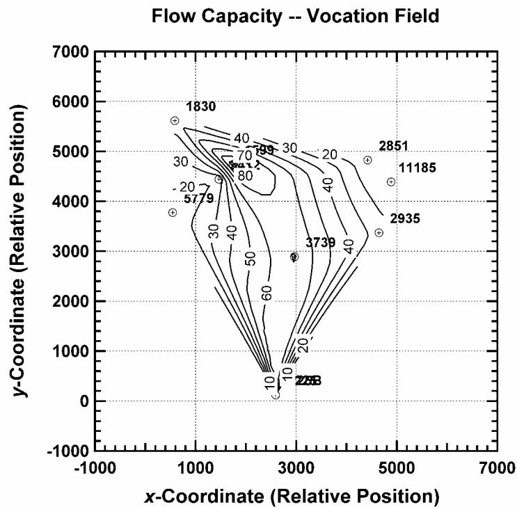
Figure 247 — Contour Map of Flow Capacity, Vocation Oil Field.
