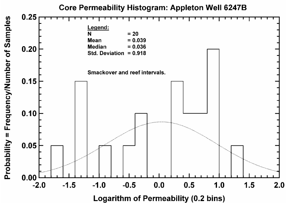
Fig. 137 — Core Permeability Histogram, Appleton Well 6247B
