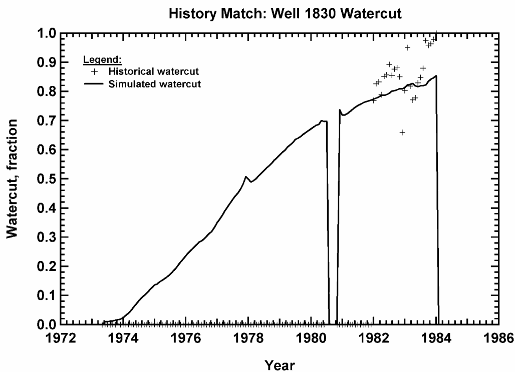
Figure 300 — Watercut history match, Vocation Well 1830.
