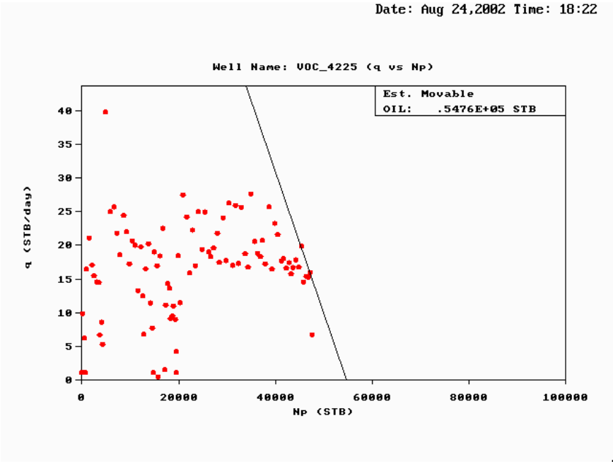
Figure 237 — Calculation of Recoverable Oil, Vocation Well 4225.
