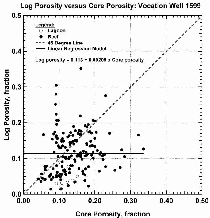
Figure 200 — Log Porosity versus Core Porosity, Vocation Well 1599.
