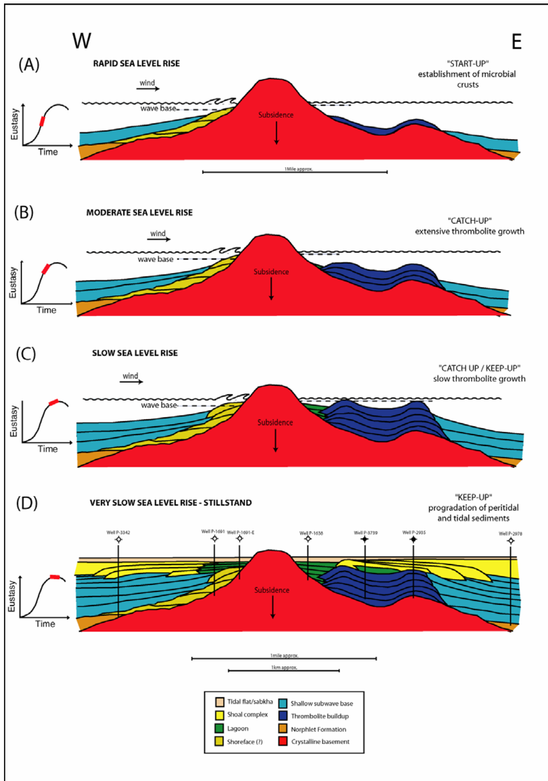
Figure 338. Evolution of thrombolite growth and associated facies on the high-relief structure at Vocation Field (modified from Llinás, 2002b).
