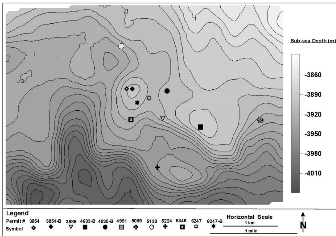
Figure 48: Structure map (depth sub-sea) of the base of the Smackover Formation. This shows main pre-existing structural culminations that controlled facies deposition, three at the Appleton Field in the east, and one to the NW. The structural high to the SW had no closure prior to Smackover deposition.
