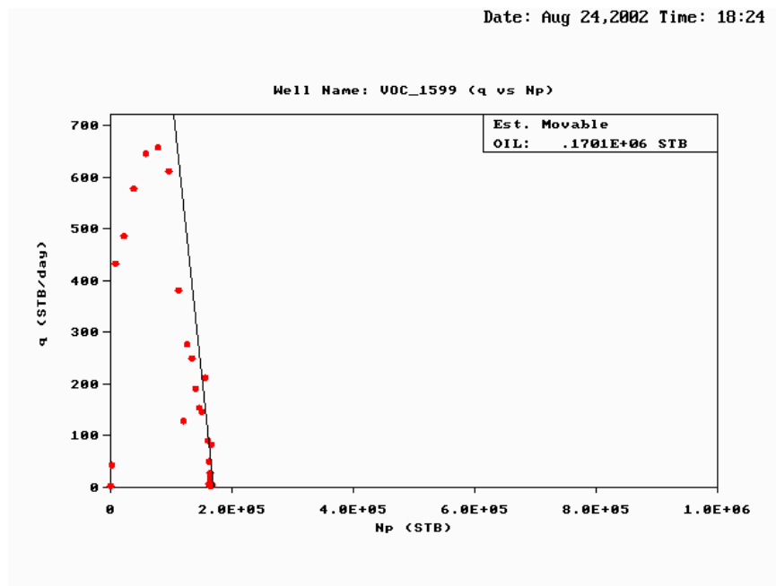
Figure 231 — Calculation of Recoverable Oil, Vocation Well 1599.
