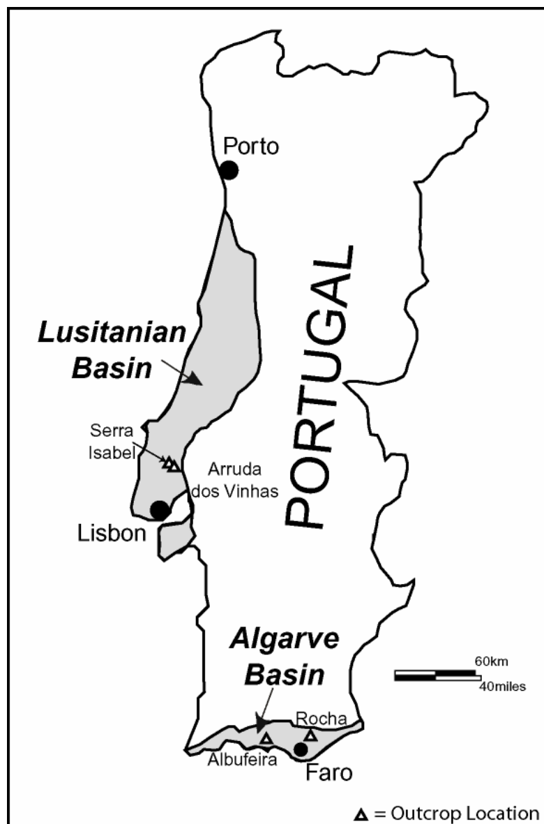
Figure 334. Map showing the location of key thrombolite outcrops studied in western Portugal, near Arruda dos Vinhas, Lusitanian Basin, and in southern Portugal, near Albufeira and Rocha, Algarve Basin.
