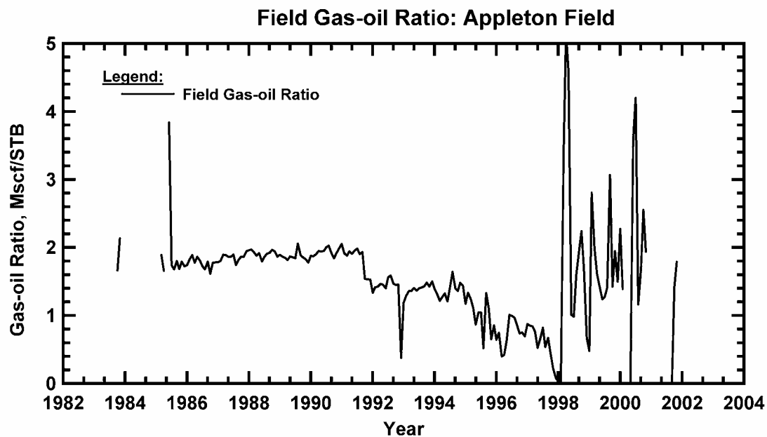
Figure 272 — Gas-Oil Ratio Profile, Appleton Field.
