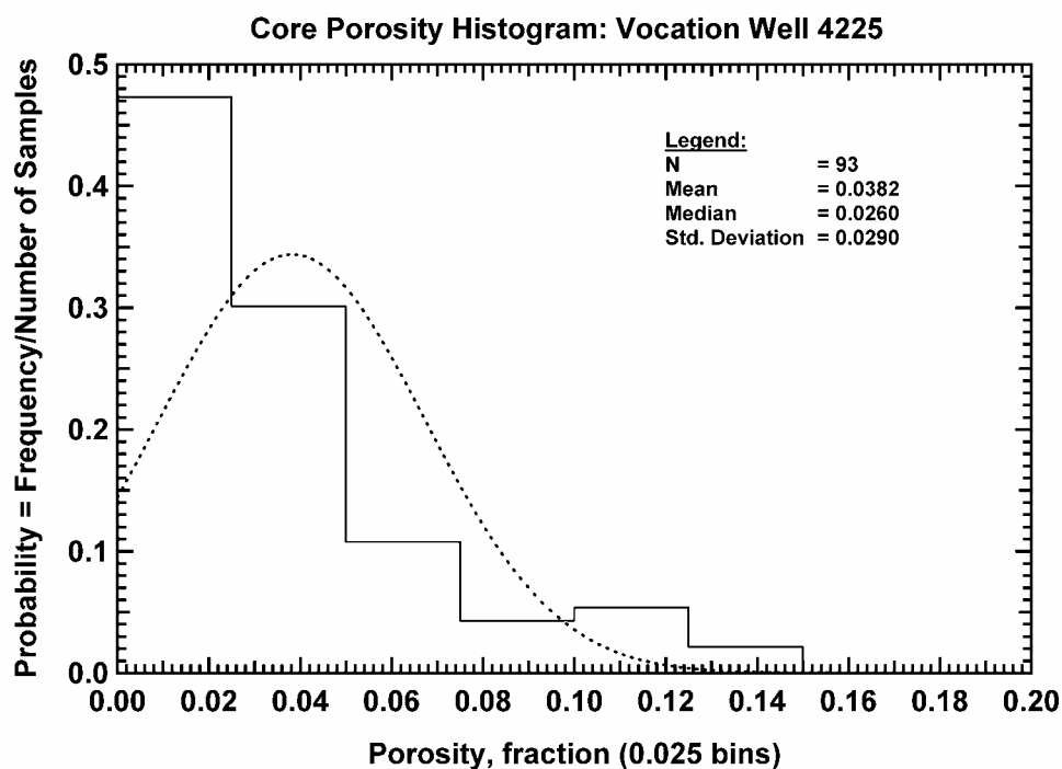
Figure 179 — Core Porosity Histogram, Vocation Well 4225.
