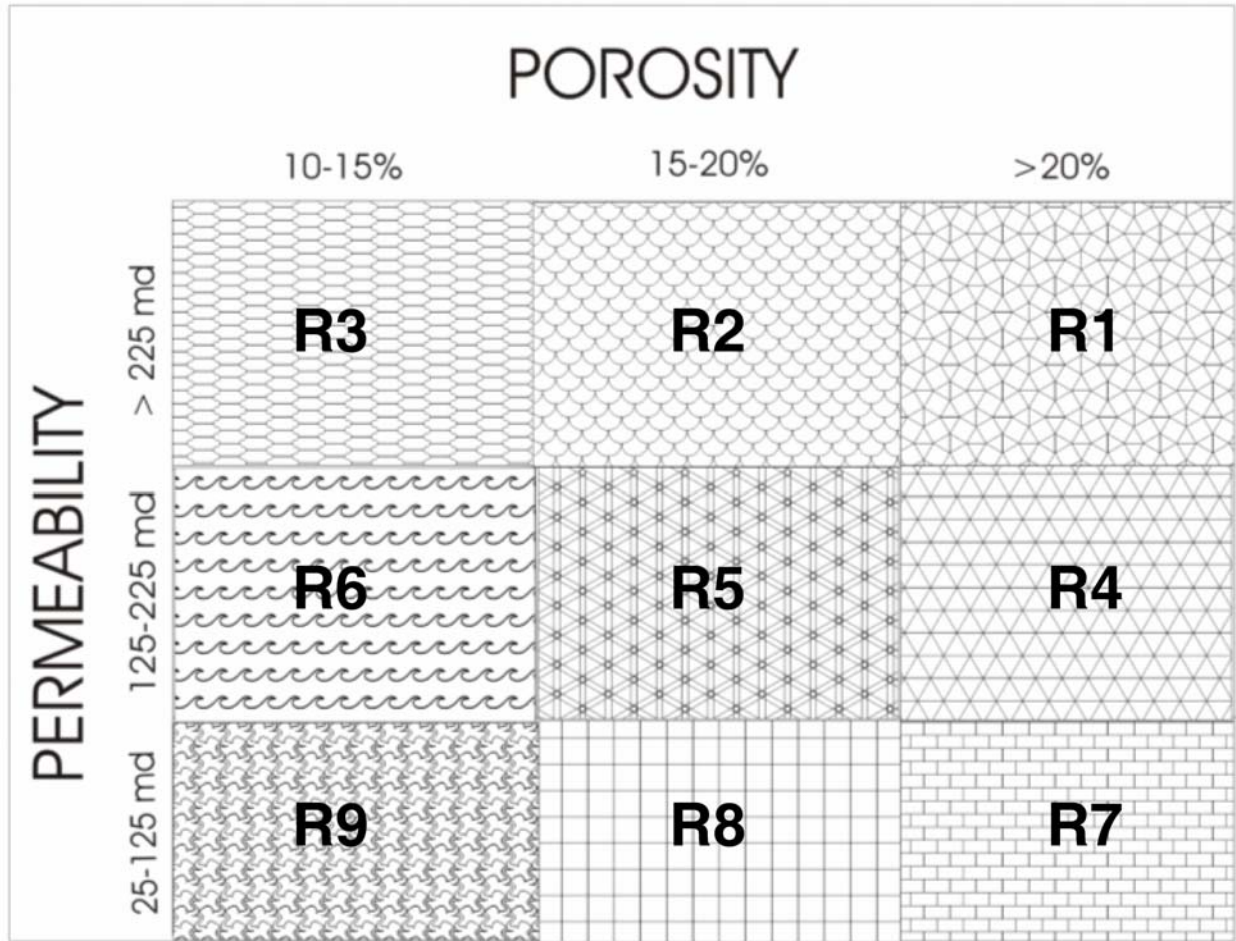
Figure 104. Vocation Reservoir Quality Map Key.
