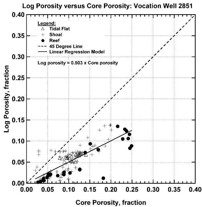
Figure 202 — Log Porosity versus Core Porosity, Vocation Well 2851.
