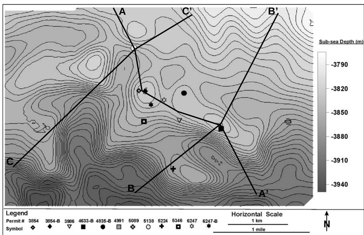
Figure 43: Seismic grid showing the aerial coverage of current survey area and well locations.
