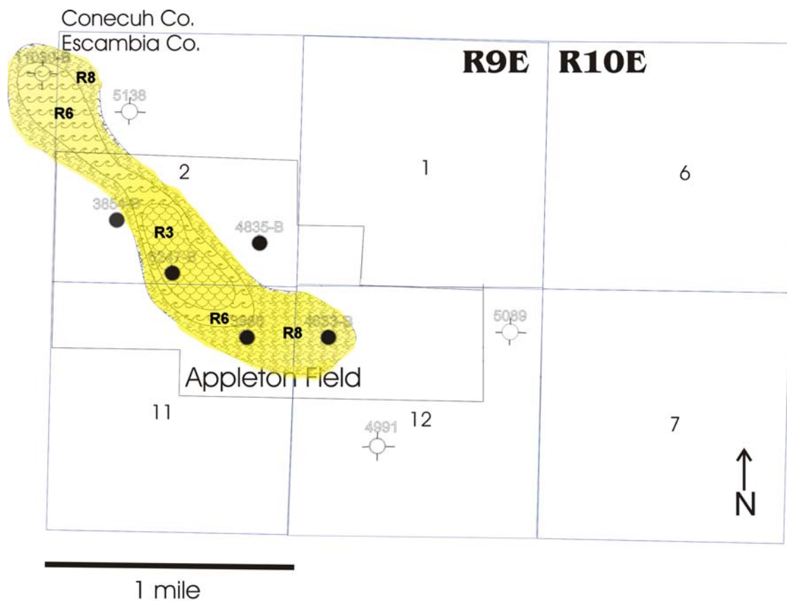
Appleton Flow Unit Slice Map 200 ft Below Top Smk
