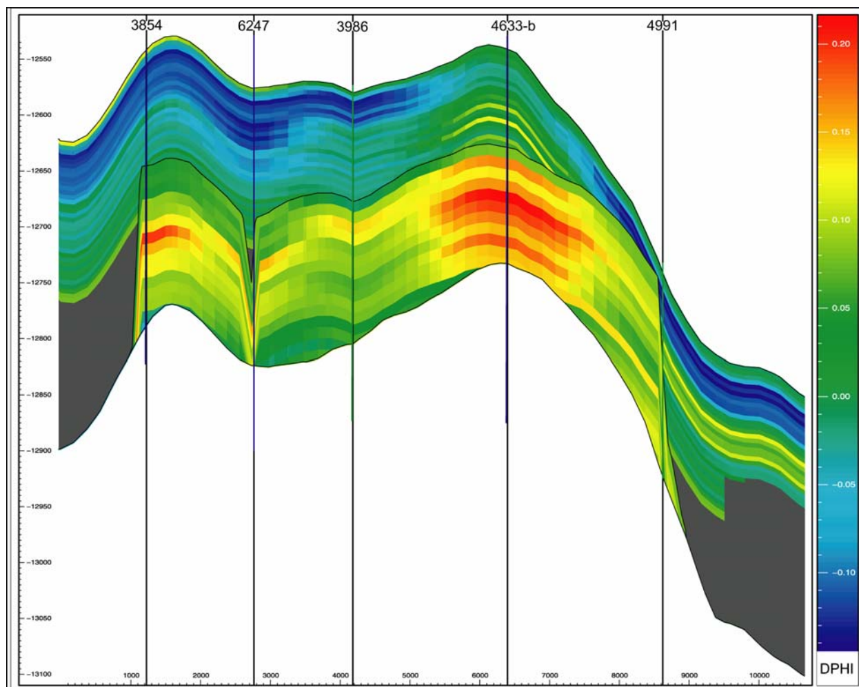
Figure 256 –Cross section showing reservoir porosity at Appleton Field.
