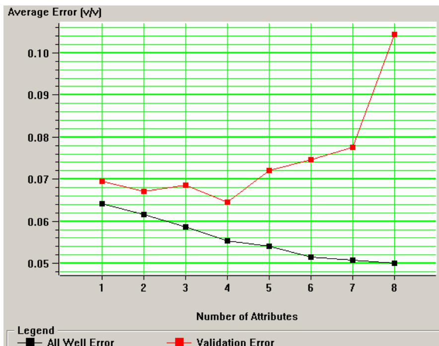
Figure 49: Validation plot, showing the optimum number of attributes to use in predicting porosity from density porosity logs using stepwise multilinear regression. This optimum number of attributes is reached when the validation error (red curve) associated with adding a new attribute to the predicting relationship fails to decrease convincingly. The black curve shows the training error. The training error generally decreases with an increase in number of attributes. See Hampton et al. (2001) for a full description and justification of this method.
