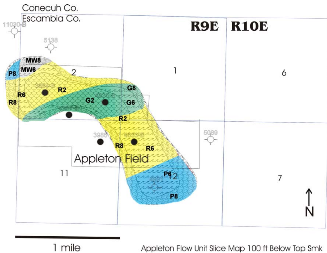
Figure 107. Appleton Flow Unit Slice Map 100 ft below Top of Smackover.
