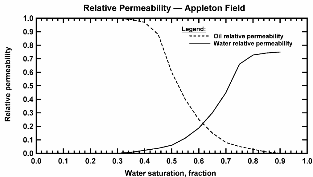
Figure 265 — History matched relative permeability curves, Appleton Field.
