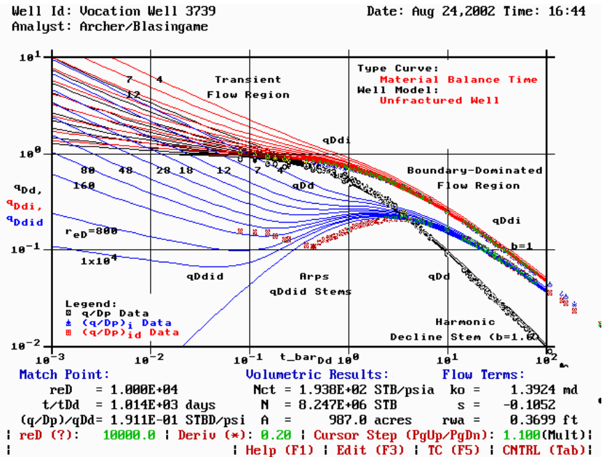
Figure 226 — Type Curve Match, Vocation Well 3739.
