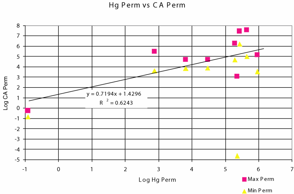
Figure 76. Comparison of mercury derived (Hg) permeability and core analysis (CA) derived permeability. It should be noted that there are two core analysis data points per mercury derived point to account for variability encountered in the interval sampled.
