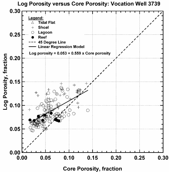
Figure 205 — Log Porosity versus Core Porosity, Vocation Well 3739.
