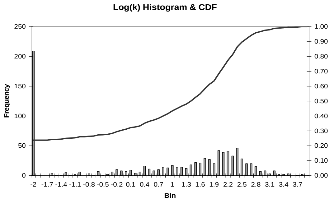
Figure 118. Histogram of permeability distribution and cumulative distribution frequency (CDF) in Appleton and Vocation fields.
