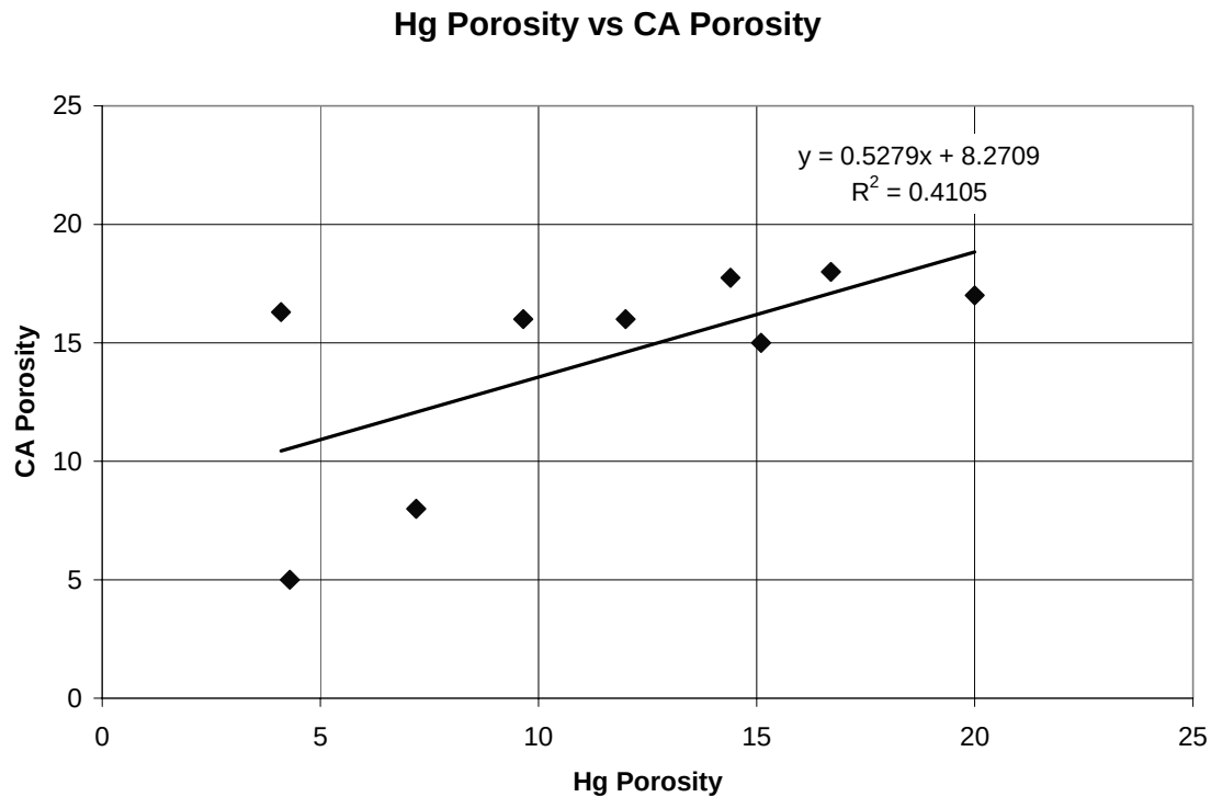
Figure 77. Comparison of mercury (Hg) derived porosity and core analysis (CA) derived porosity.
