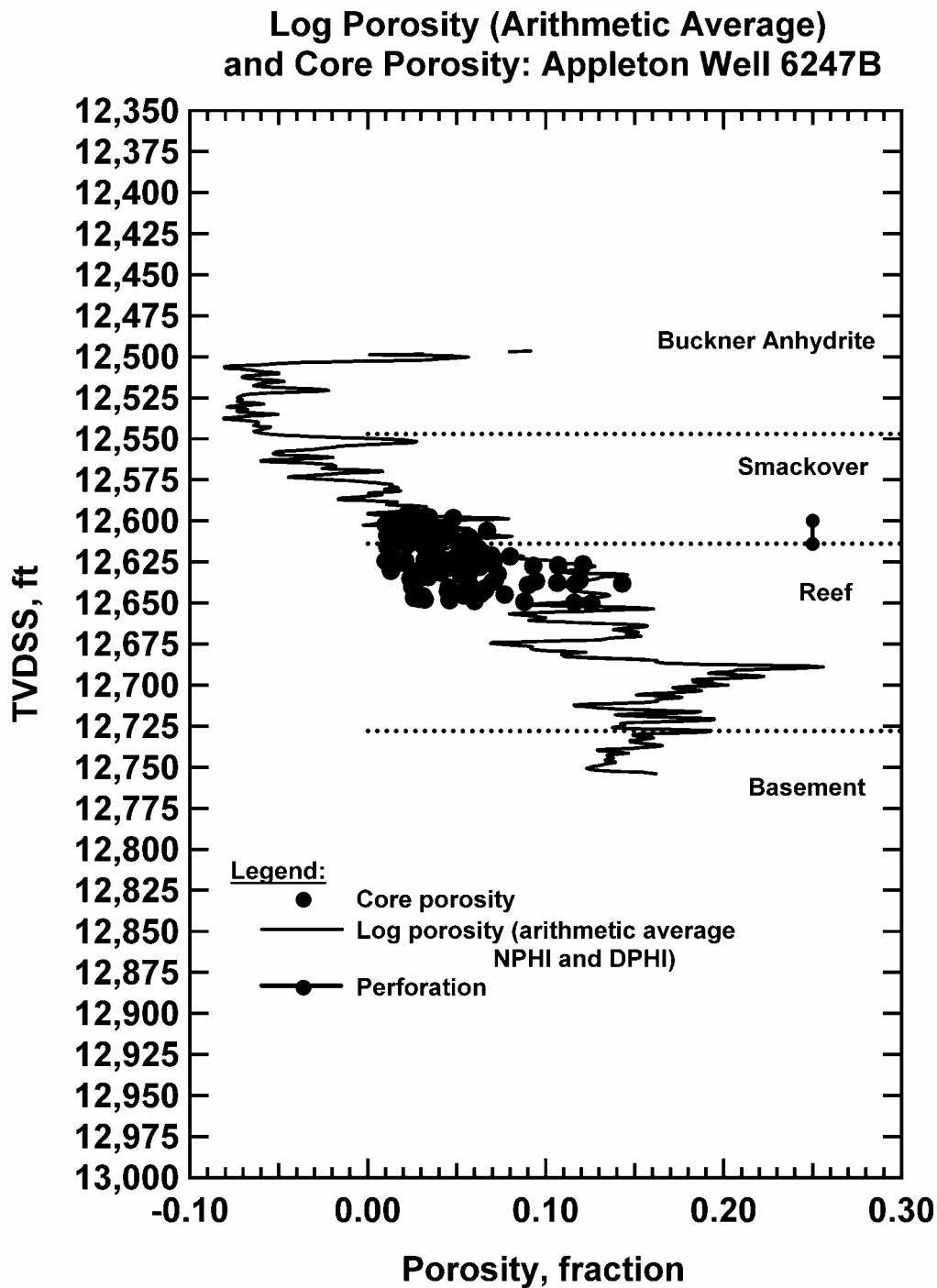
Fig. 142 — Porosity Variation with Depth, Appleton Well 6247B
