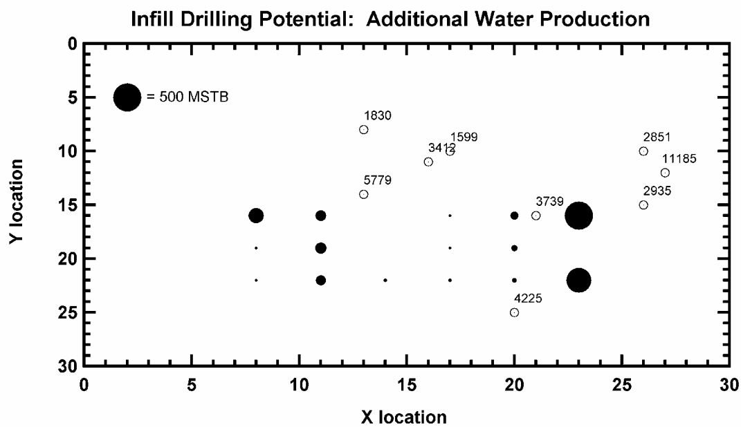
Figure 319 — Incremental water production via an infill well at various locations, Vocation Field.
