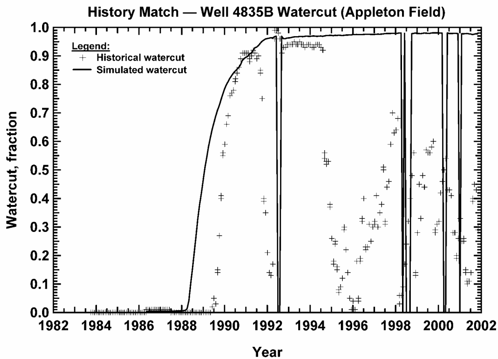
Figure 280 — Watercut history match, Well 4835B (Appleton Field).
