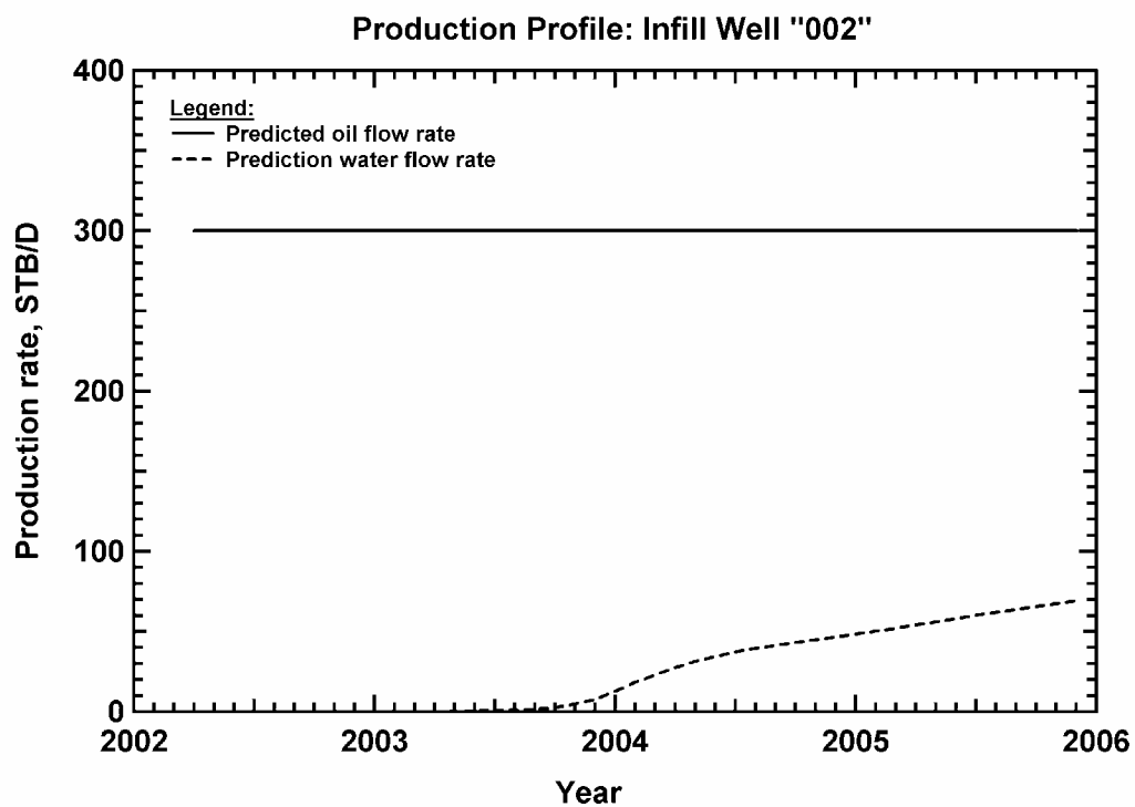
Figure 317 — Oil and water production rates, proposed infill well 002, Vocation Field.
