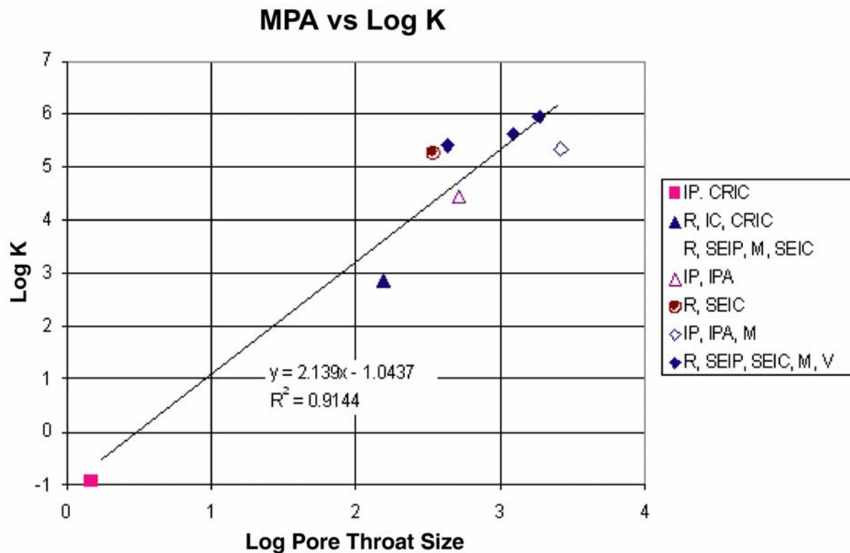
Figure 75. Comparison of median pore aperture size (MPA) and permeability (K).
