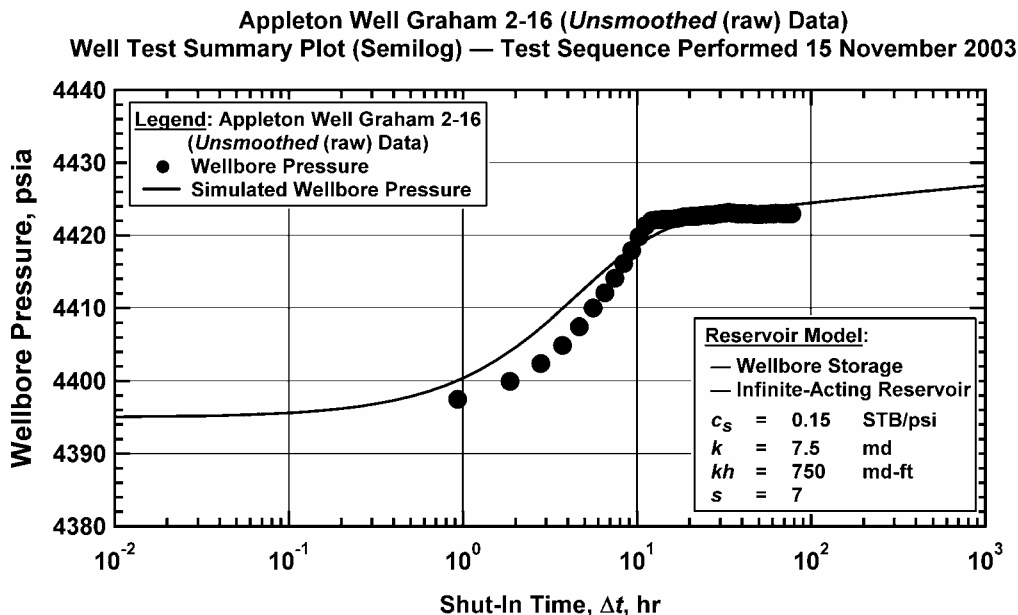
Figure 171c — Semilog Summary Plot (with Analysis) for Graham Well 2-16 (testing sequence of November 2003) — raw pressure buildup data case. Appleton Field (Alabama, USA)
