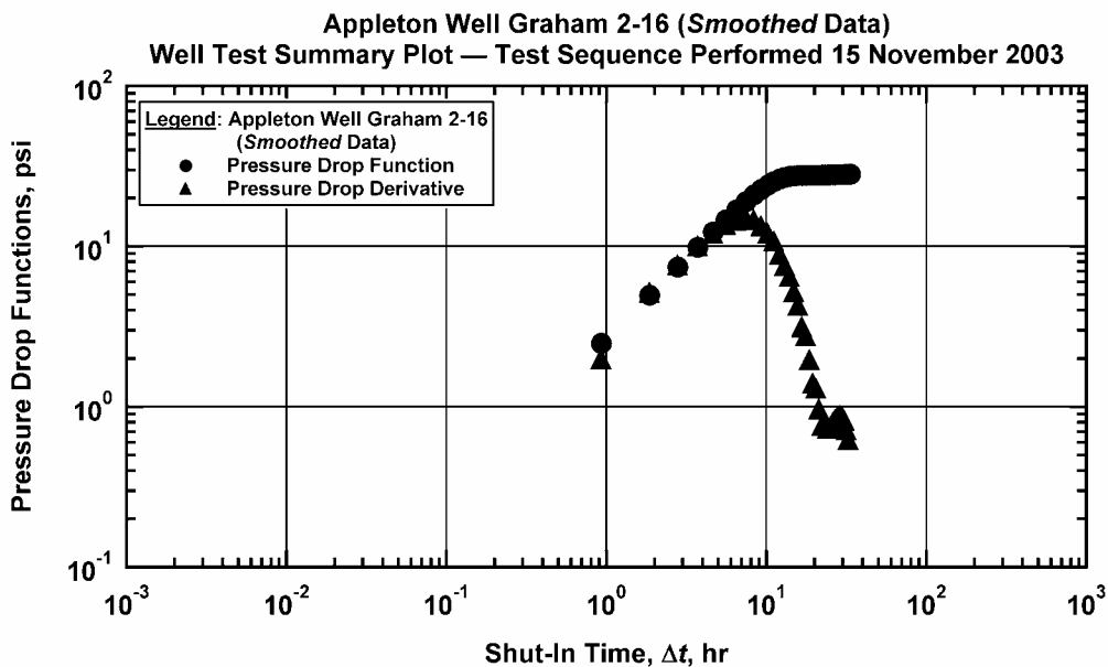
Figure 171e — Log-log Summary Plot (No Analysis) for Graham Well 2-16 (testing sequence of November 2003) — smoothed pressure buildup data case. Appleton Field (Alabama, USA)
