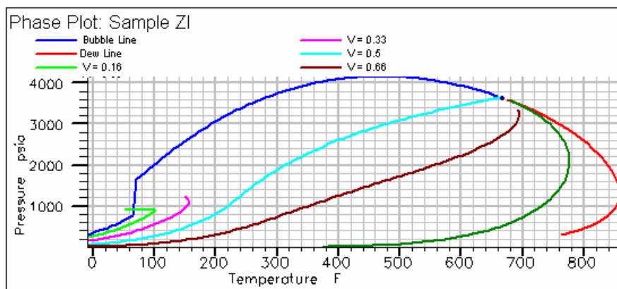
Figure 264 – Phase Envelope, Appleton Oil Field.
