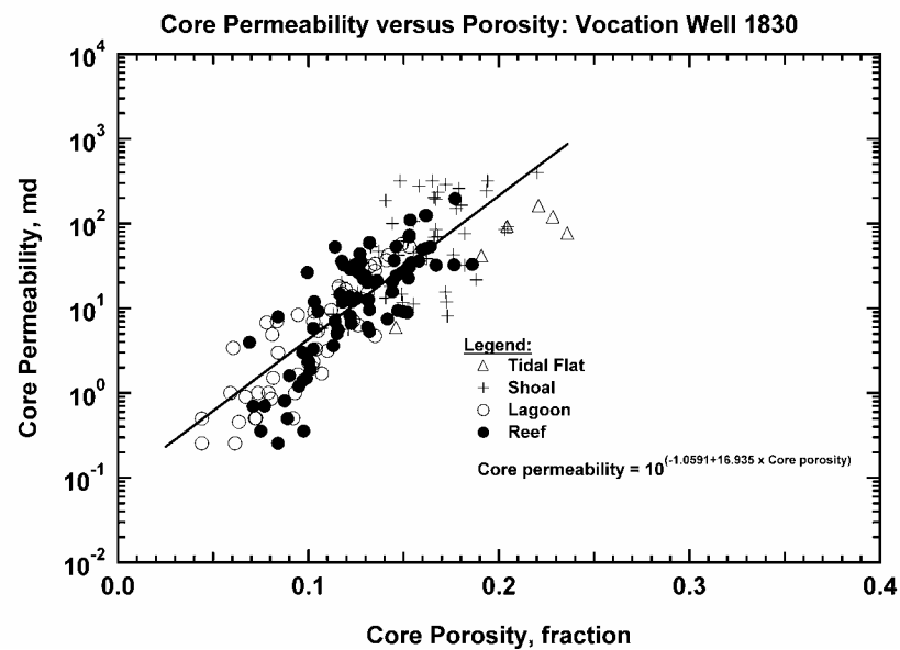
Figure 210 — Core Permeability versus Core Porosity, Vocation Well 1830.
