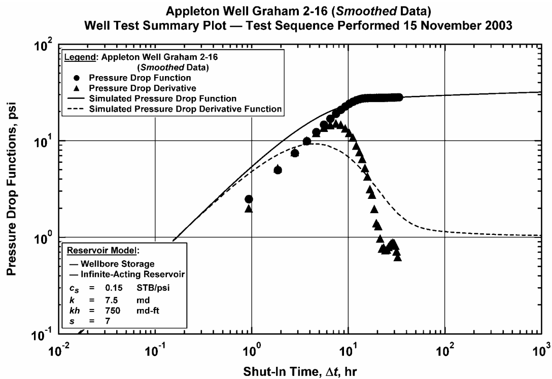
Figure 171g — Log-log Summary Plot (with Analysis) for Graham Well 2-16 (testing sequence of November 2003) — smoothed pressure buildup data case. Appleton Field (Alabama, USA)
