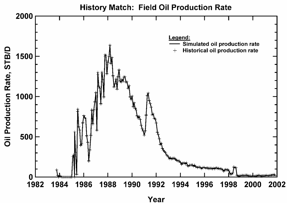
Figure 274 — Oil Production Rate History Match, Appleton Field.
