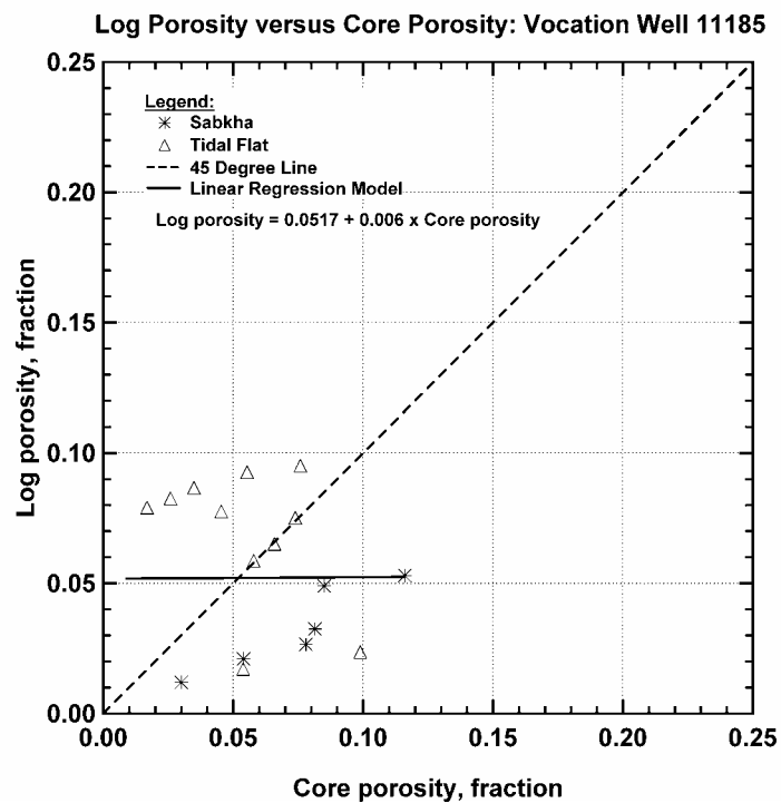
Figure 208 — Log Porosity versus Core Porosity, Vocation Well 11185.
