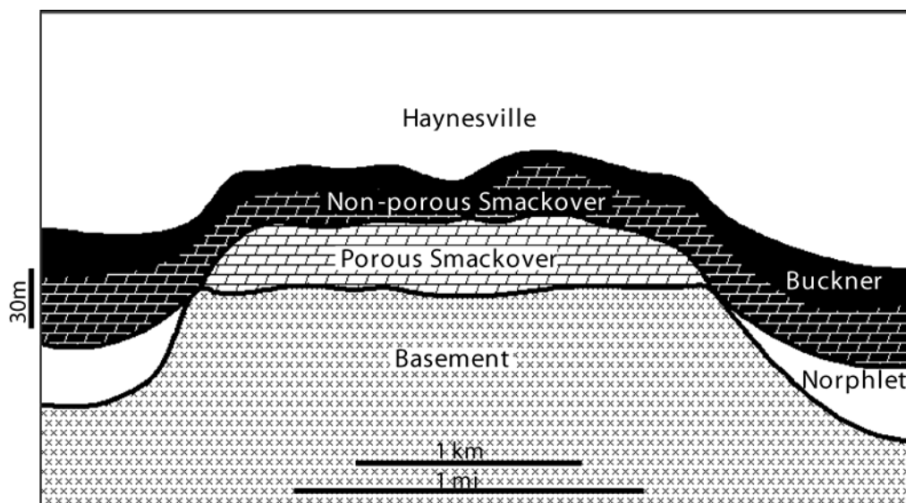
Figure 46: Geologic model depicting the relationship of the main stratigraphic units at Appleton Field (from Hart and Balch, 2000).
