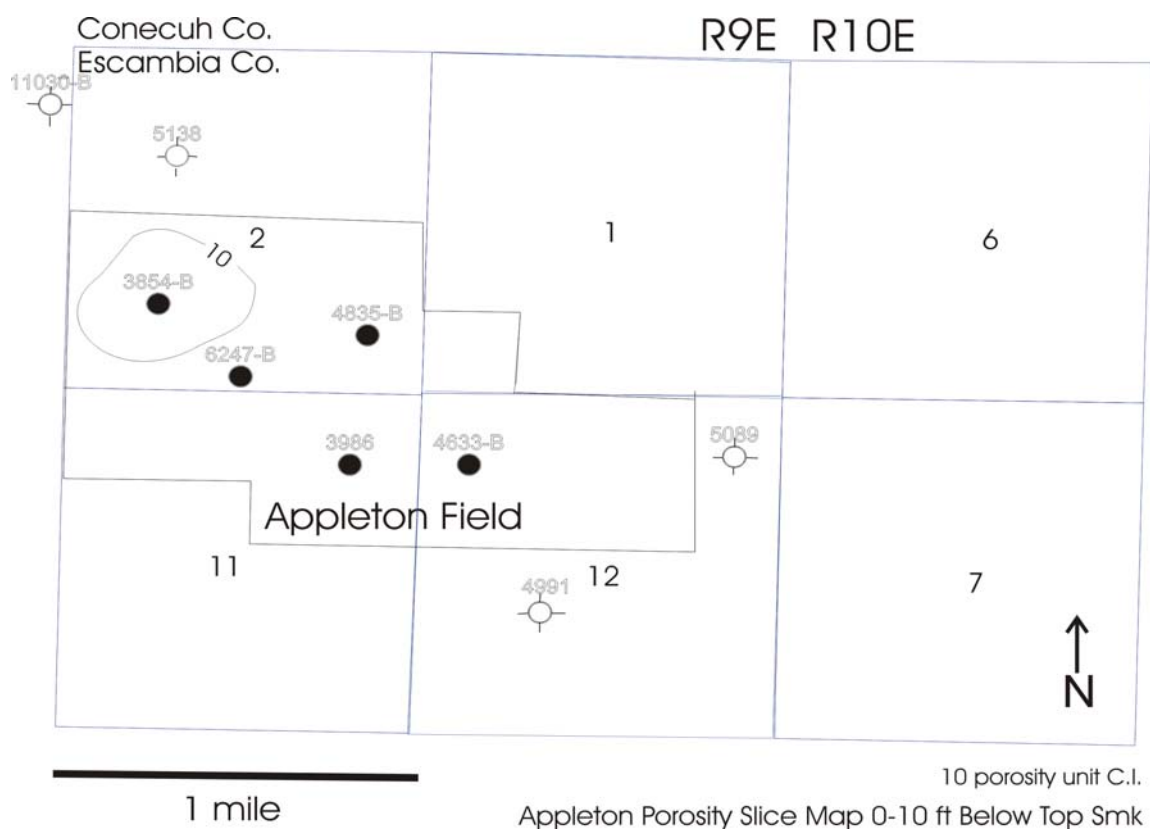
Figure 80. Appleton Porosity Slice Map 0 to 10 ft below Top of Smackover.
