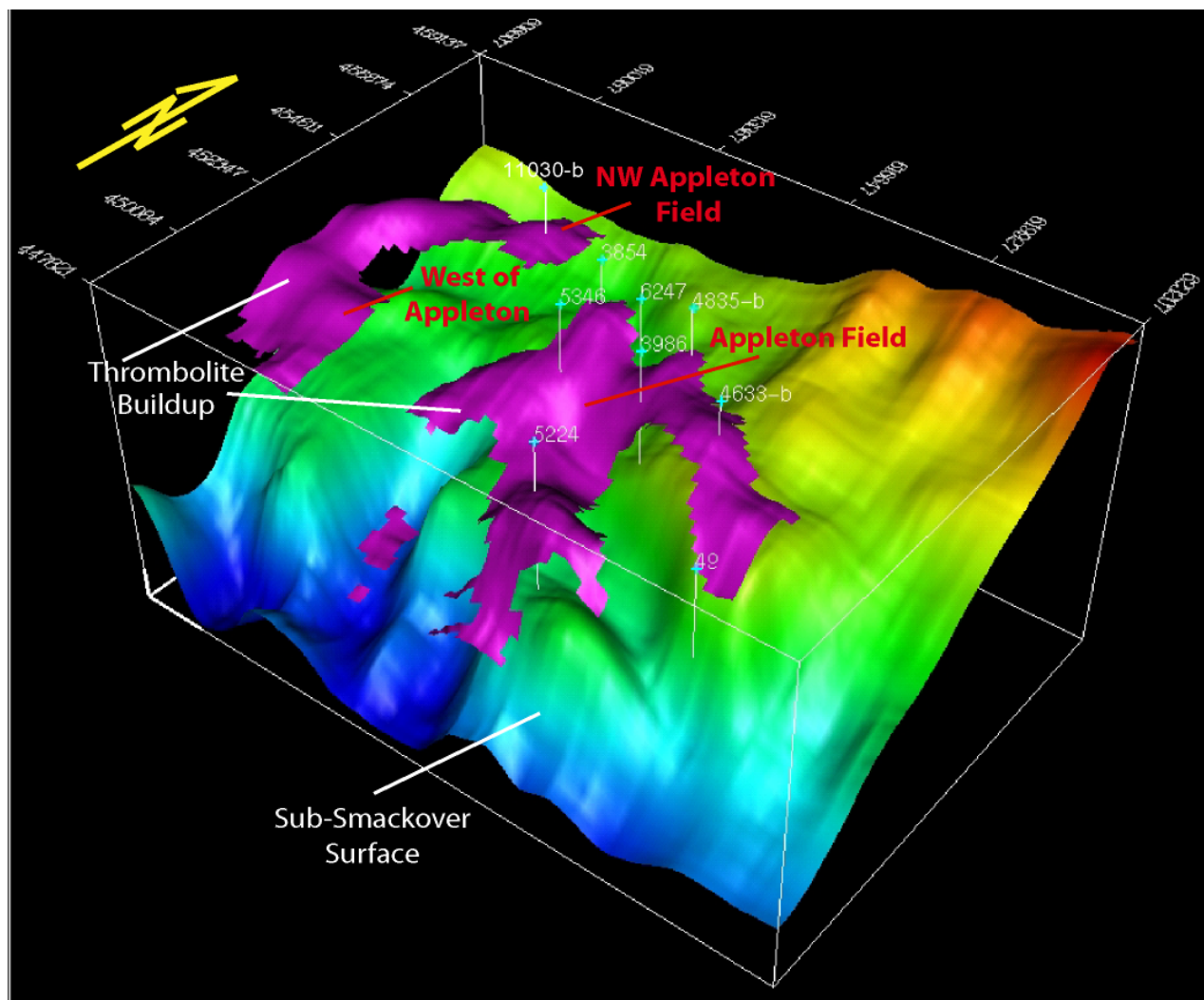
Figure 255. Three dimensional view of the Appleton composite paleohigh, including Appleton Field, Northwest Appleton Field, and an area west of Appleton Field, showing the spatial distribution of the thrombolite buildups on the crest and flanks of the crystalline basement high.
