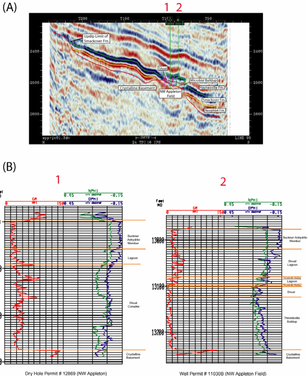
Figure 322. (A) Seismic profile oriented in an approximate dip direction showing the Northwest Appleton paleohigh where thrombolite facies developed on the southern part of this basement high. To the north of Northwest Appleton Field on this paleohigh, the strong reflector that identifies the thrombolite buildup is replaced by a fuzzy low amplitude reflector. (B) representative logs from wells for these areas. Notice that the dry hole (Permit #12869), located in the area north of Northwest Appleton, shows an irregular pattern of relatively high gamma ray (GR) values and lower density (DPHI) and neutron (NPHI) porosities which may indicate the presence of shoal/lagoon facies.
