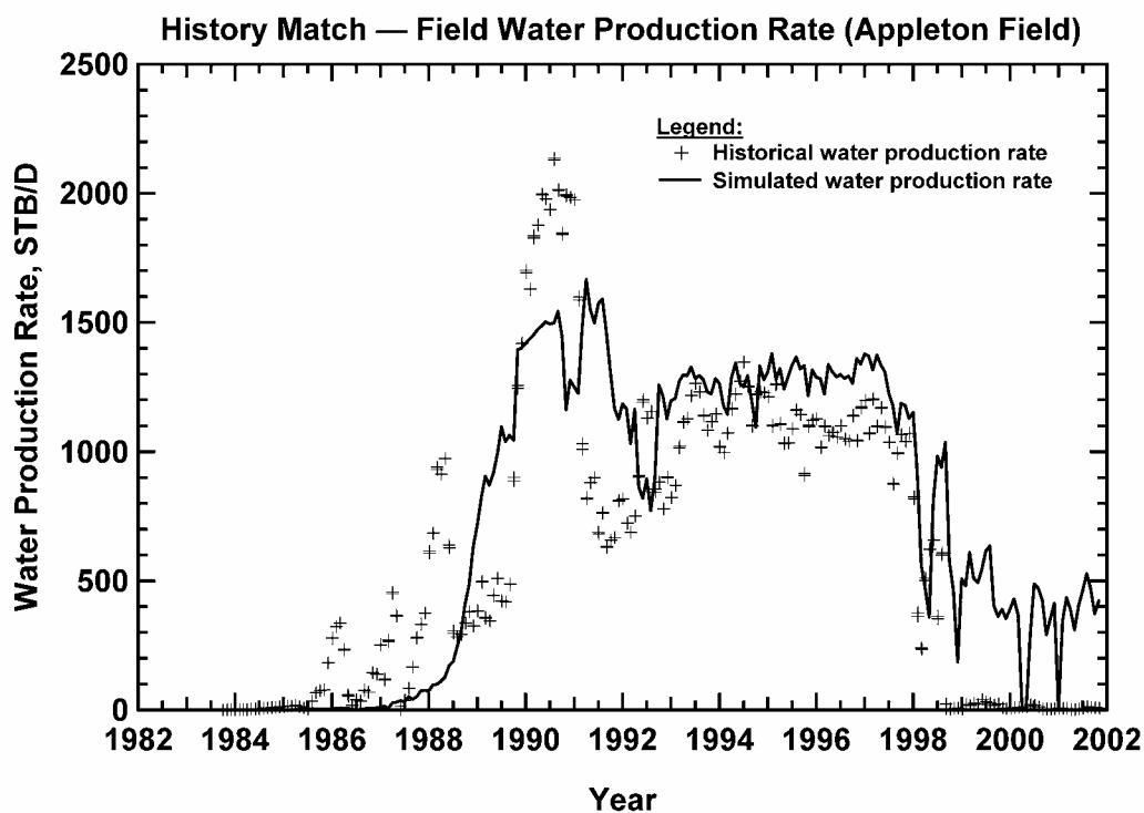
Figure 275 — Fieldwide water production rate history match, Appleton Field.
