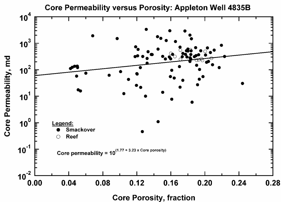
Fig. 151 — Core Permeability versus Core Porosity, Appleton Well 4835B.
