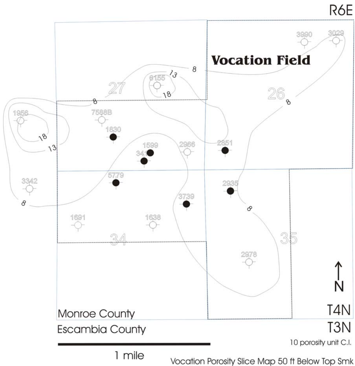
Figure 87. Vocation Porosity Slice Map 50 ft below Top of Smackover.
