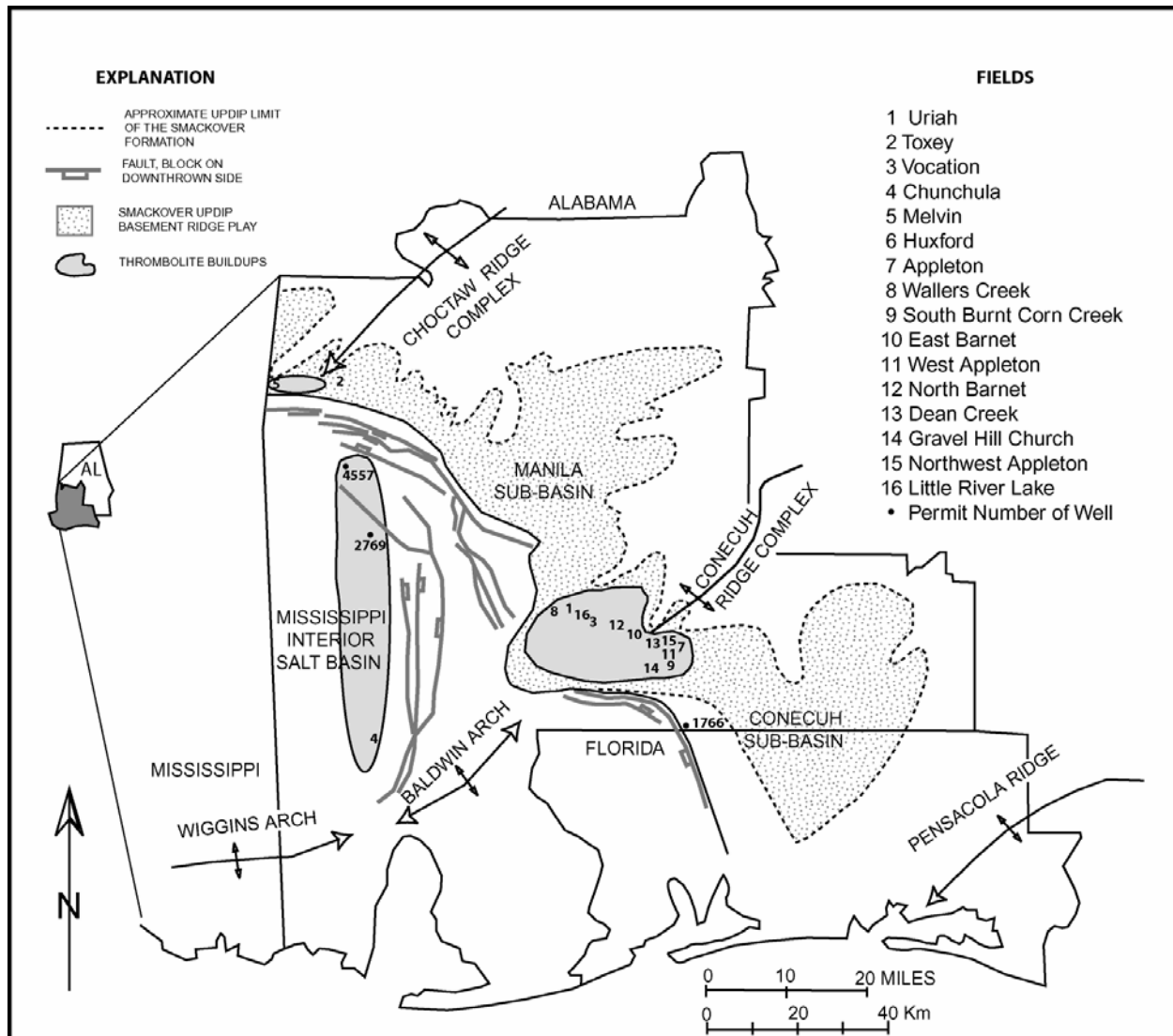
Figure 323. Location map showing major structural features, trend of the Smackover updip basement ridge play, distribution of major thrombolite buildups, and key oil fields with thrombolite facies in southwest Alabama.
