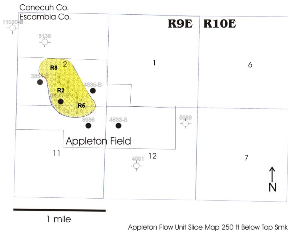
Figure 110. Appleton Flow Unit Slice Map 250 ft below Top of Smackover.
