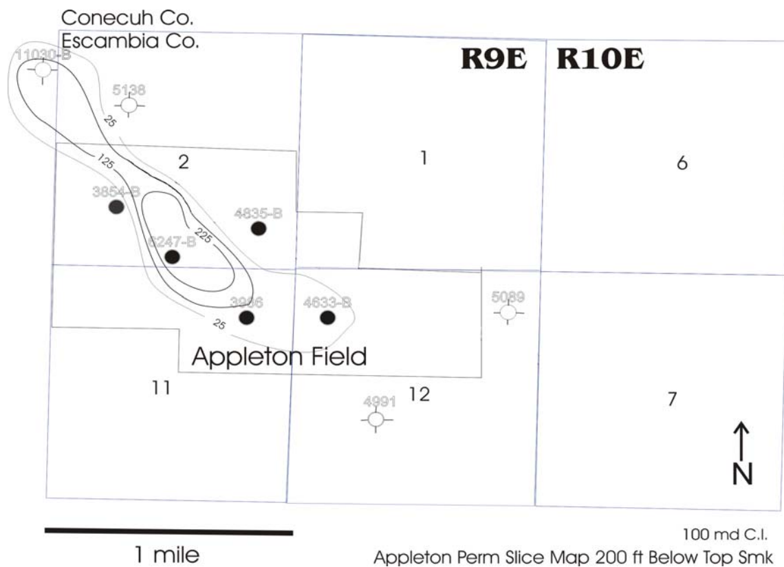
Figure 96. Appleton Permeability Slice Map 200 ft below Top of Smackover.
