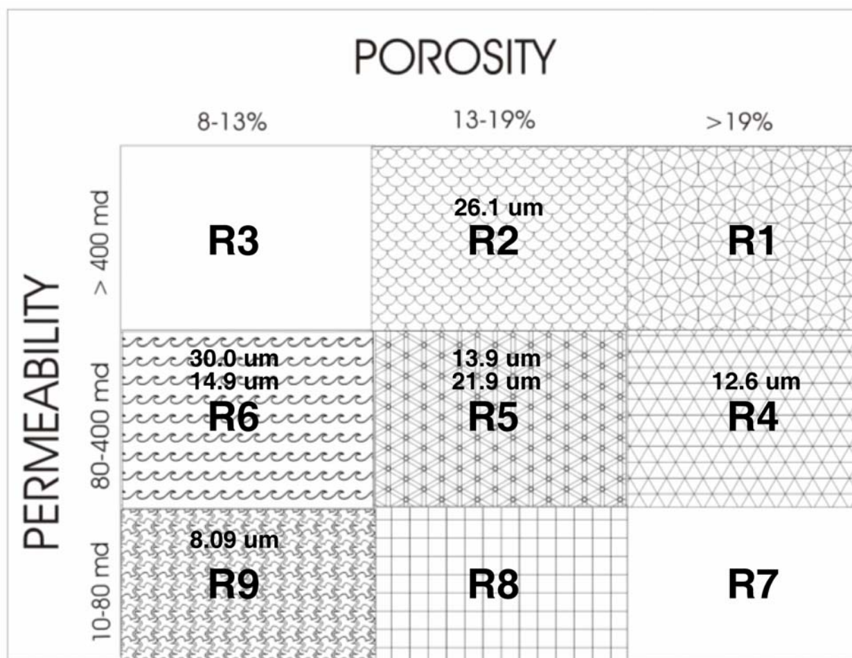
Figure 119. Reservoir quality pairs showing averaged porosity and permeability values along with corresponding MPA values over stratigraphic intervals for flow unit delineation.
