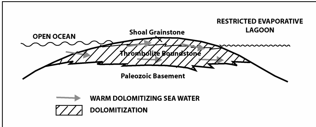
Figure 340. Generalized diagram of evaporative pumping mechanism of Saller and Moore (1986) as a means of explaining dolomitization of boundstone facies associated with basement paleohighs in the northeastern Gulf of Mexico.
