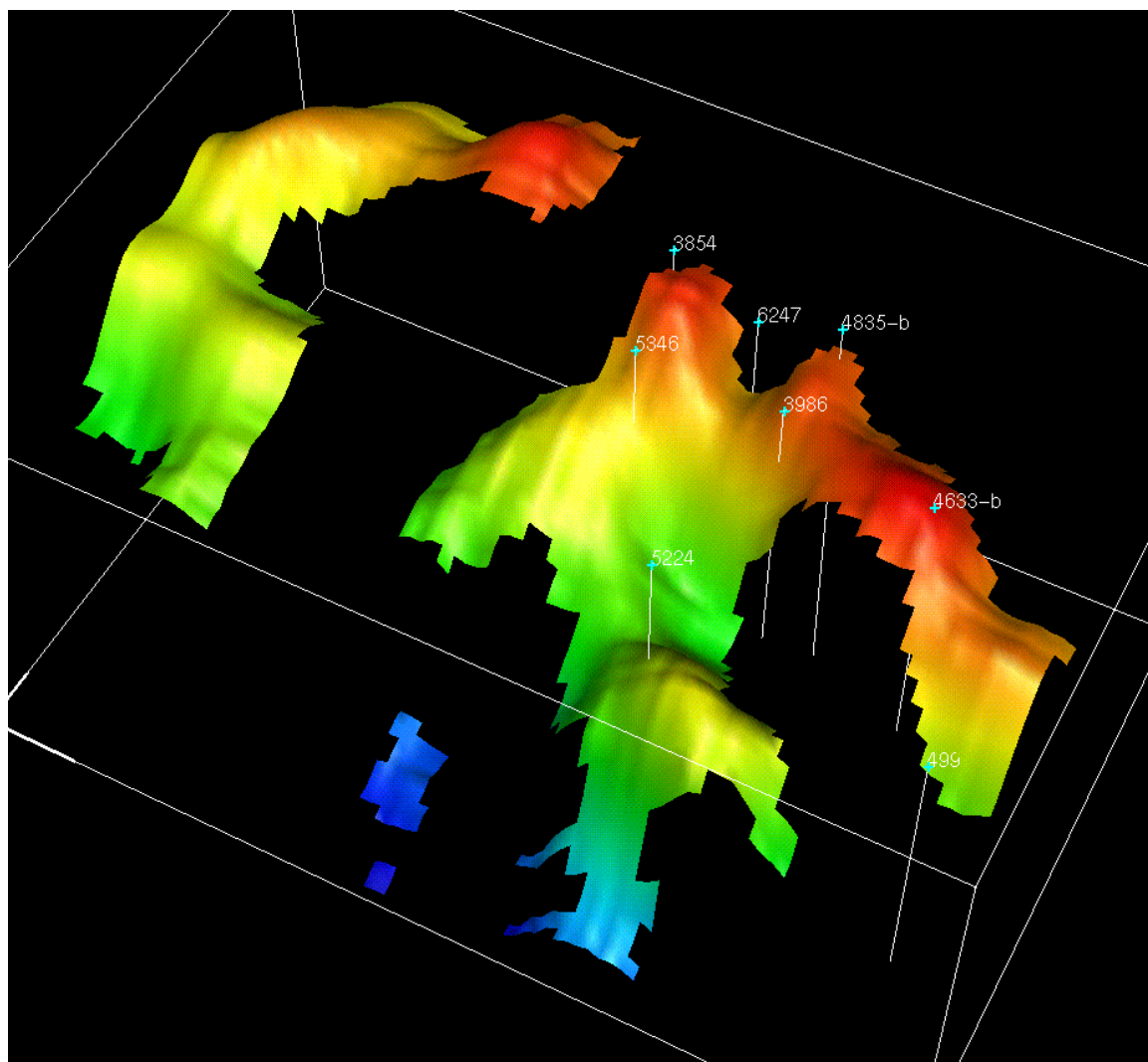
Figure 254. 3-D model of Appleton Field structure on top of the reef interval.
