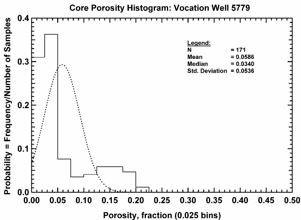
Figure 180 — Core Porosity Histogram, Vocation Well 5779.
