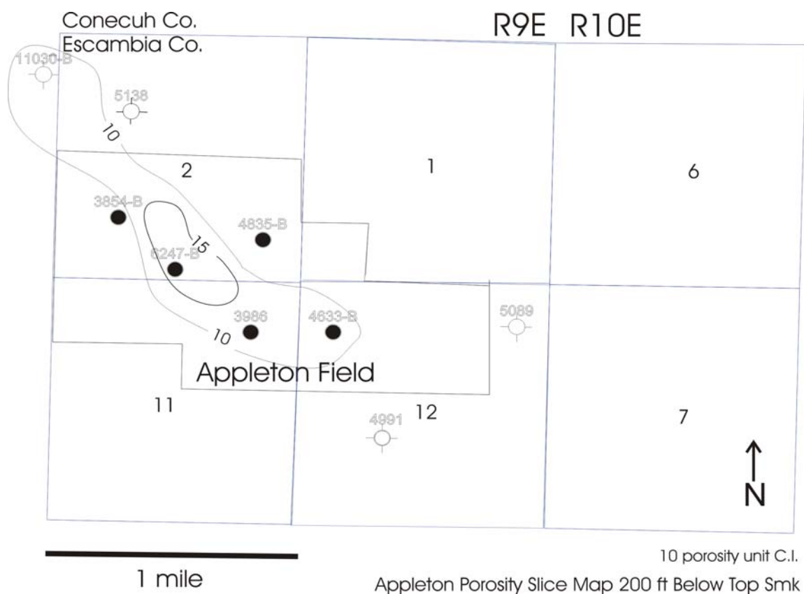
Figure 84. Appleton Porosity Slice Map 200 ft below Top of Smackover.
