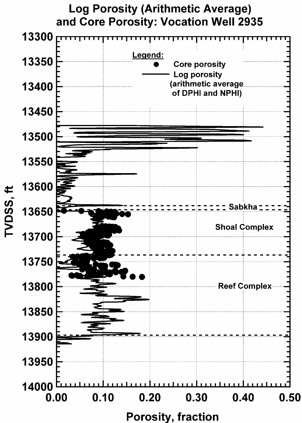
Figure 194 — Porosity Variation with Depth, Vocation Well 2935.
