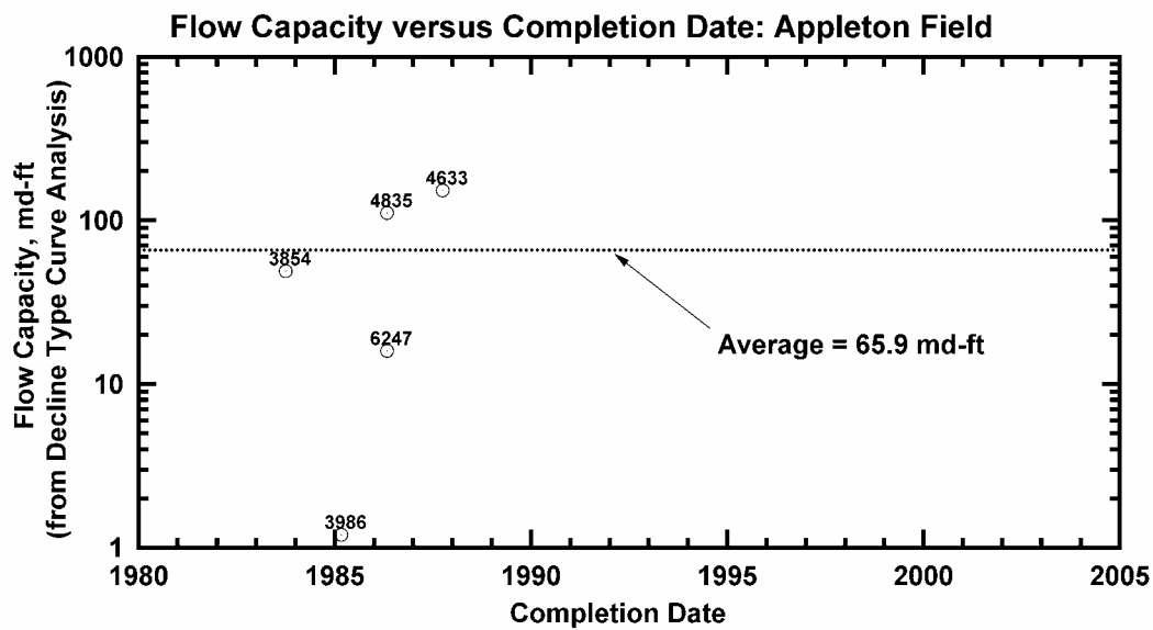
Fig. 166 — Flow Capacity versus Completion Date, Appleton Oil Field.
