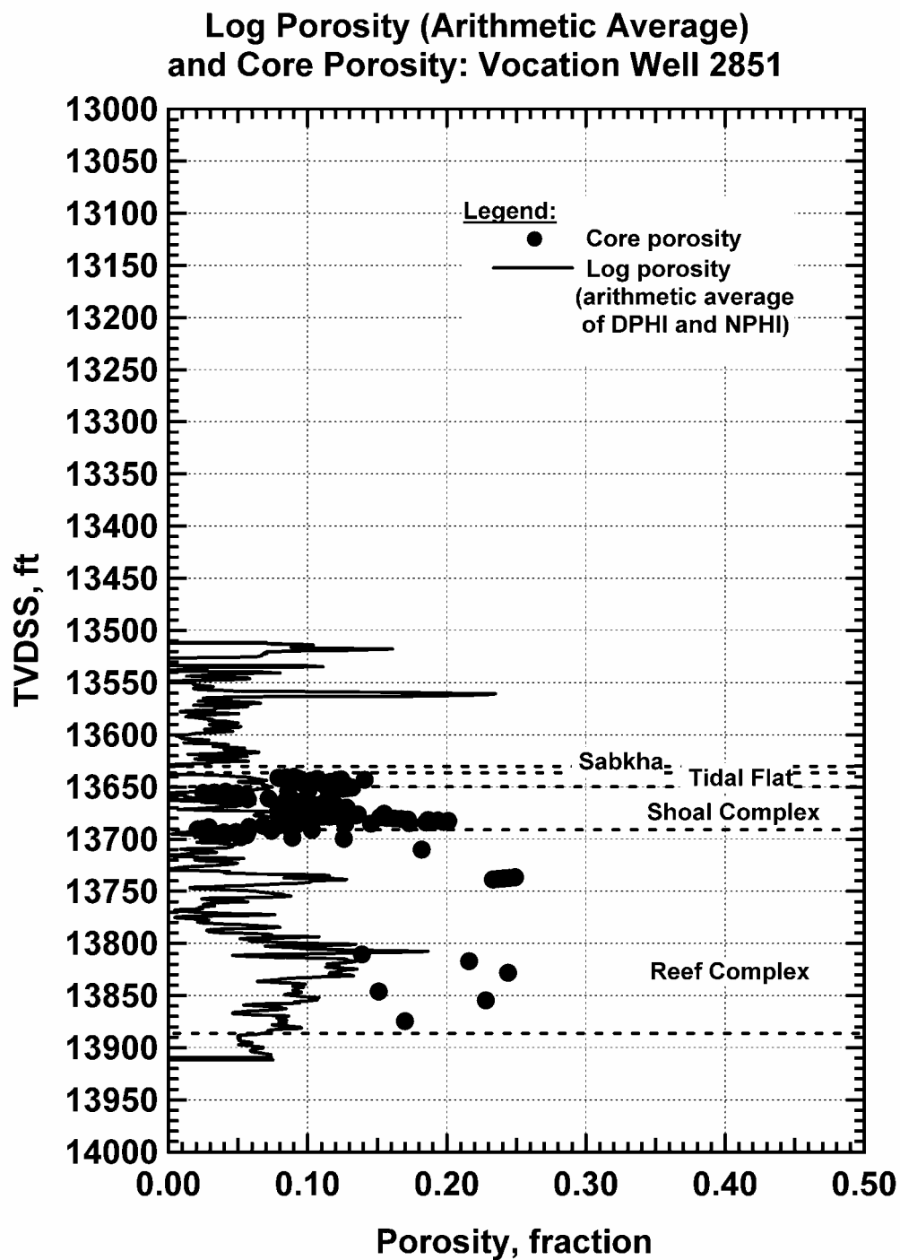
Figure 193 — Porosity Variation with Depth, Vocation Well 2851.
