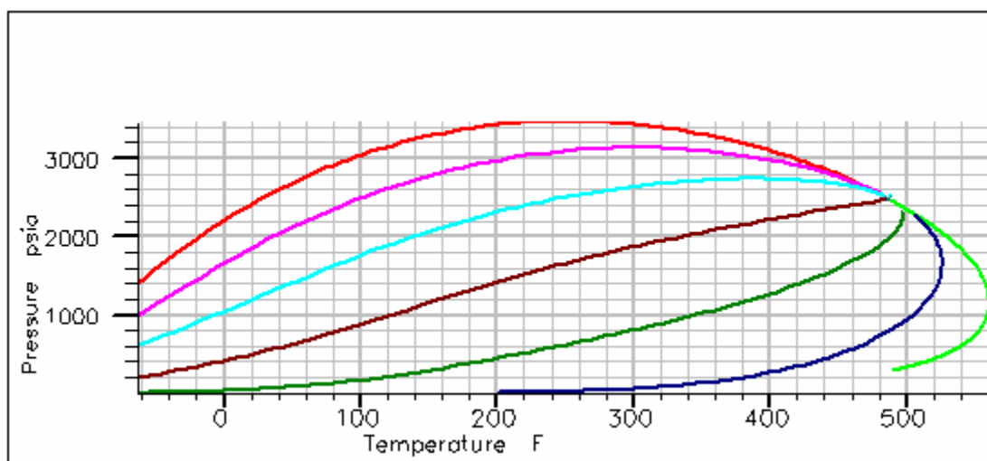
Figure 286 – Phase Envelope, Vocation Field.
