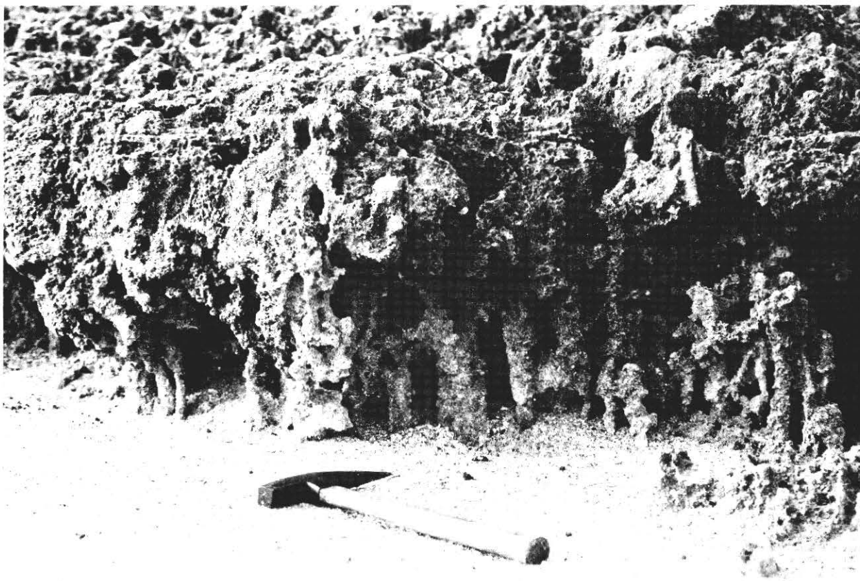
Figure 6. Type # 1 burrows on side of outcrop, Blowing Rocks.
