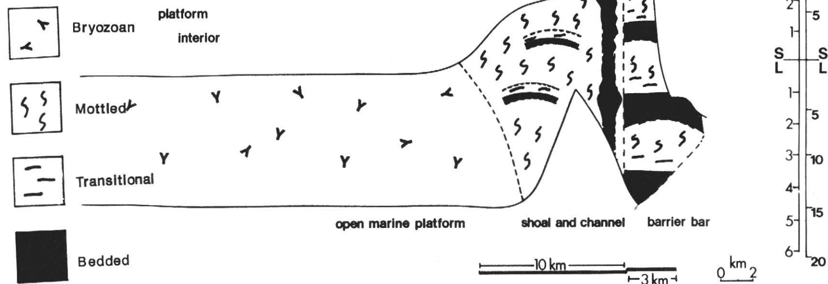
Figure 12. A schematic cross-section of the Miami Limestone. The topography and depth to the base of the section are measured from maps and cores. The internal anatomy is schematic. The seaward barrier bar is 3 km wide, has the thickest section of limestone (11 m) predominantly cross-bedded, and the cross-bedding is intercalated with burrowed horizons. The shoal and channel system is 10 km wide, but no more than 9 meters thick. The section here is predominantly mottled, with isolated outlying lenses of bedded facies, and, where the section intersects a channel, a vertically continuous section of cross-bedding. The open marine platform has the thinnest section of Miami Limestone, 6 meters or less, is laterally extensive, covering an area of about 500 sq.km., and characterized by peloidal sand and bryozoans. The names above the section refer to comparable environments from Joulter's Cays, Bahamas.
