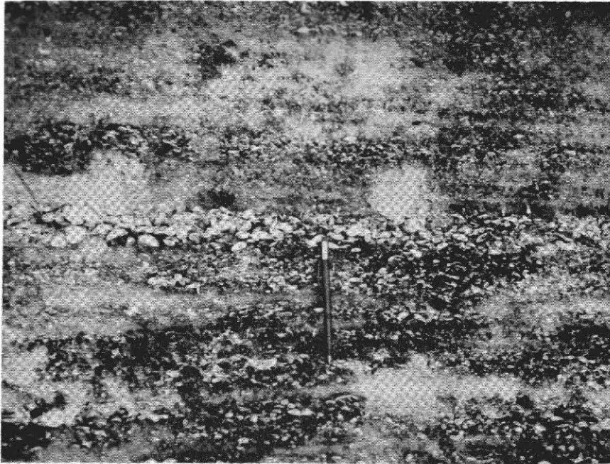
Figure 4. Close-up view of swash-zone bedding in the Wulfert ridge (locality 3 of Figures 16,17, and 18) at an elevation of about 9 feet MSL.
