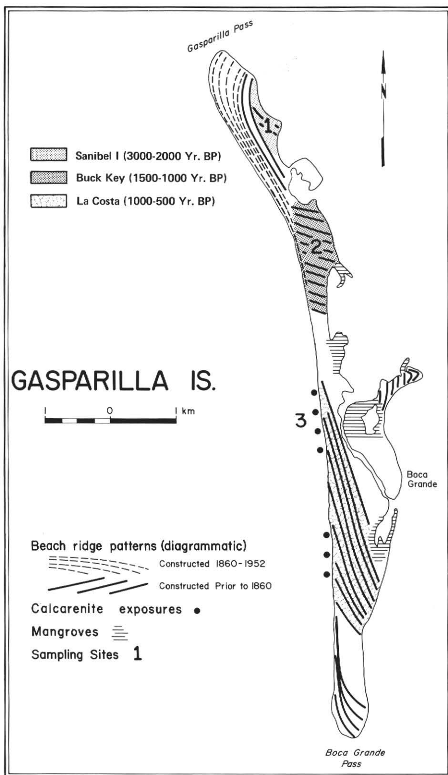
Figure 6. The radiocarbon chronology of beach-ridge sets preserved on Gasparilla Island, Lee County, Lee County, Florida. Beach-ridge patterns are diagrammatic within the various sets and were mapped from 1944 U.S. Department of Agriculture aerial photography. The designations Sanibel I, Buck Key, and La Costa are informal time-stratigraphic units. Thirty-three radiocarbon dates of individual shells collected from localities 1, 2, and 3 are the basis for the chronology of this island.
