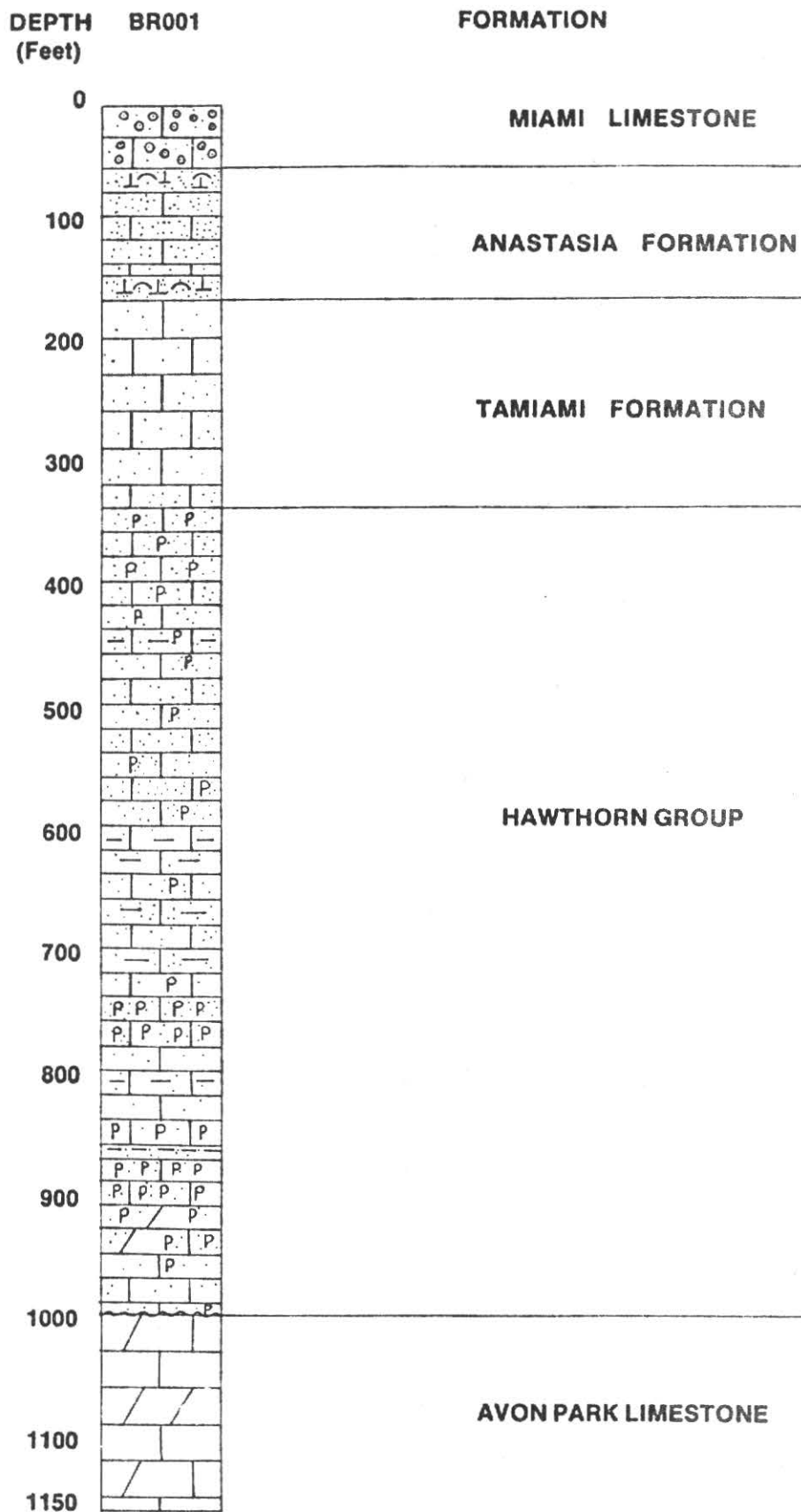
Figure No. 17 Lithologic column in Broward County, Florida
