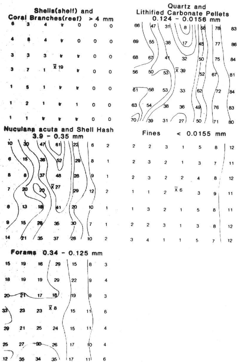
Figure 5 Geographic distribution of the five constituent grain types (wt. %, identified in Fig. 4) from reef and shelf areas. Contour interval 10%. Jeffs' Reef is at center with \bar{X} = mean for all reef samples; other numbers represent individual samples.
