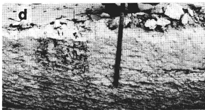
Figure 6. C. Rod type traces viewed in a bedding plane exposure. The rods are horizontally oriented, overlap one another (upper right) and intersect each other (lower left). The picture includes a pen for scale. D. The cross-bedded facies of the Miami Limestone. The large scale beds dip at about 24^{\circ} . Individual beds are 2-3 cm thick and consist of a well cemented layer and a poorly cemented layer, causing the individual beds to weather out in relief. The scale is marked in alternating light and dark bands of 10 cm each.
