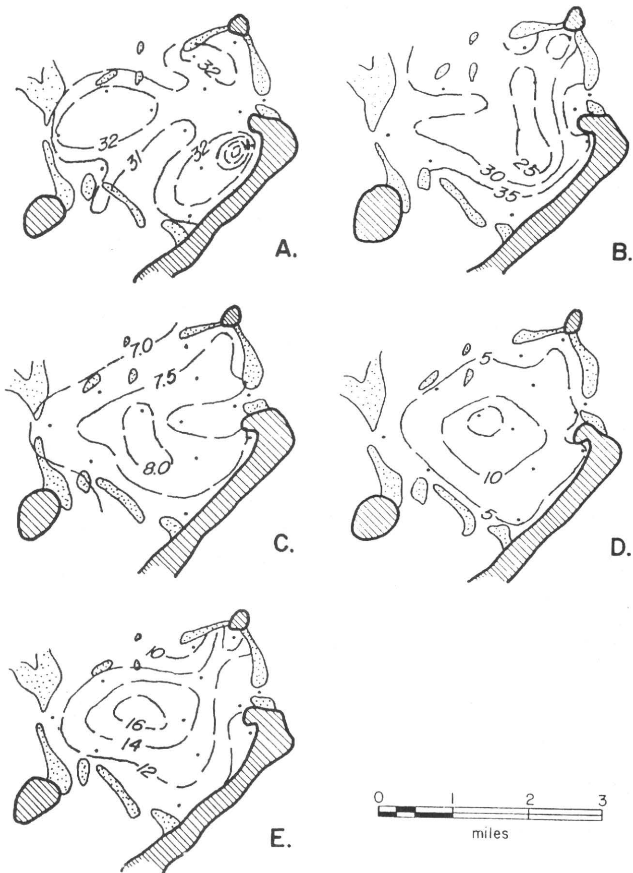
Figure 4. All samples taken just above bottom. A,B,C, and D taken in July 1982; E taken in April 1983. A, salinity, CI = 1 ppt; B, CO 2 mg/l, CI = 5 mg/l, CI = 5 mg/l; C, pH, CI = 0.5 units; D, turbidity, CI = 5 ftu; and E, O 2 , CI = 2 mg/l.
