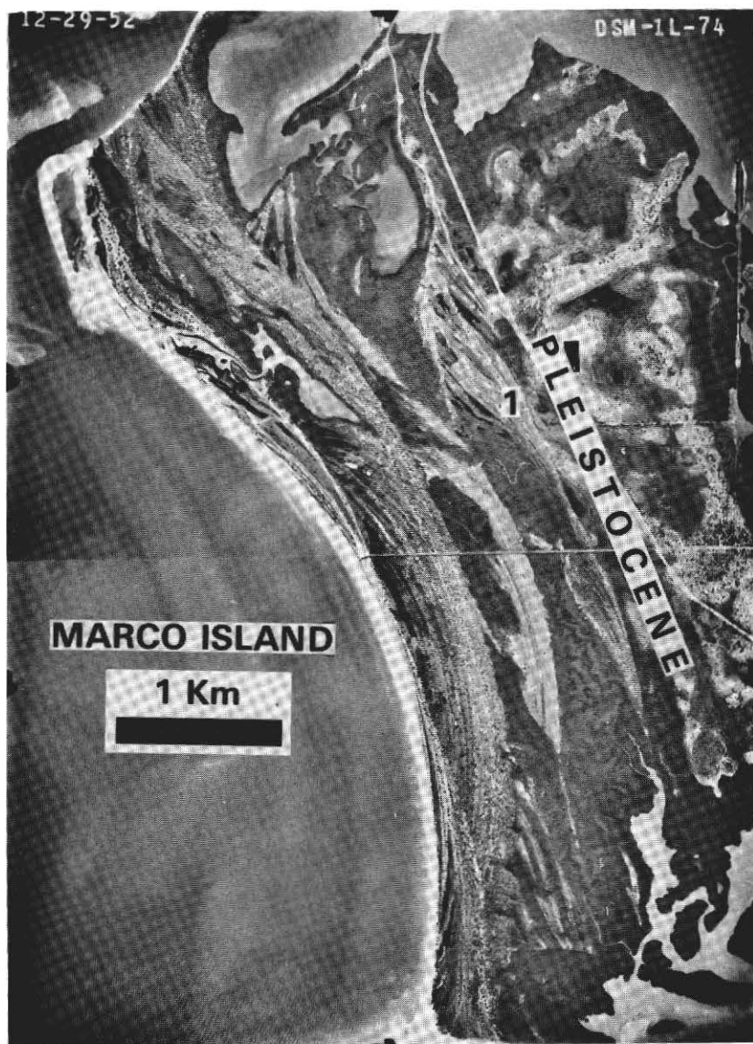
Figure 21. Uncontrolled aerial photo mosaic of Marco Island, Collier County, Florida. The photographs were taken by the U.S. Department of Agriculture in 1952. Shells were collected for radiocarbon dating from the numbered locality.
