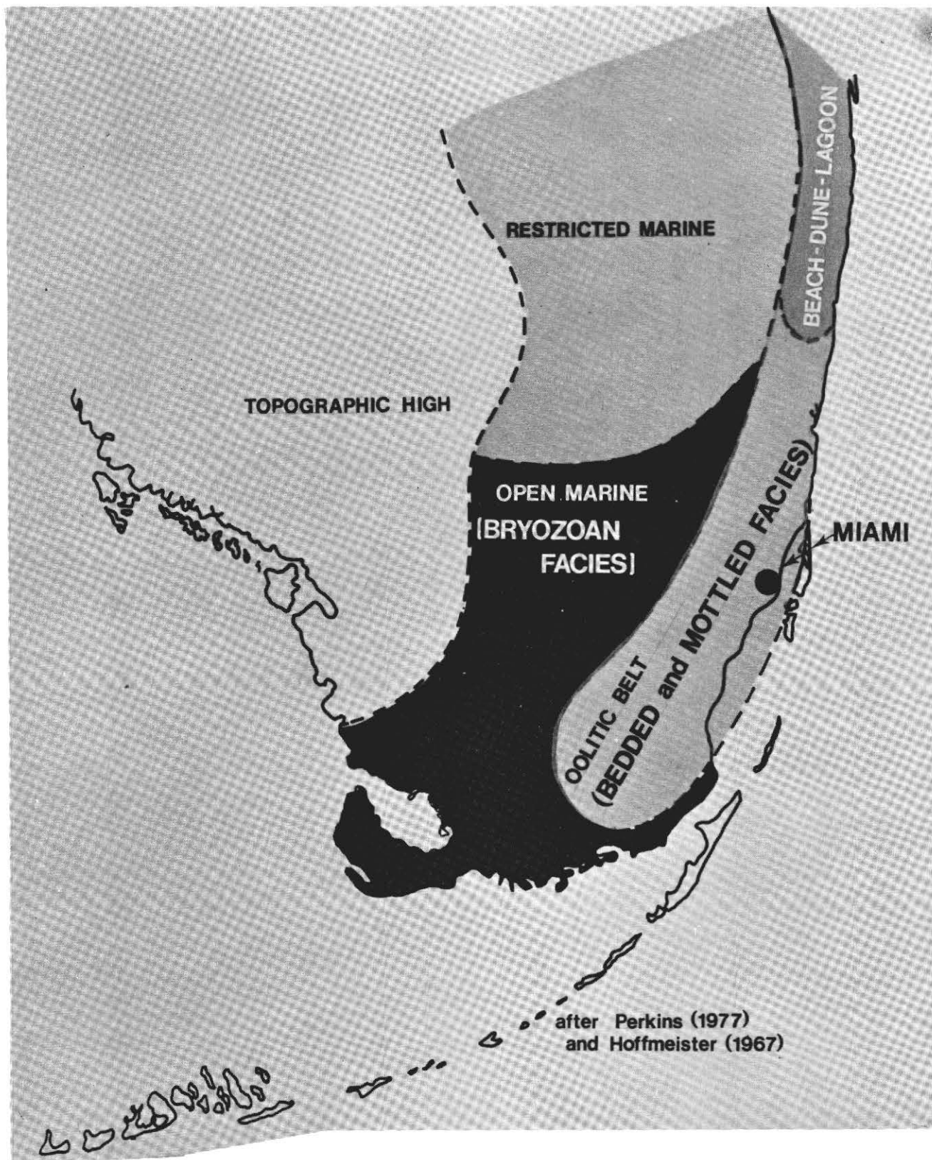
Figure 2. The depositional environments during Miami Limestone time (after Perkins, 1977) and generalized facies distribution of the Miami Limestone (Hoffmeister et al., 1967 and this study). The mobile oolitic belt on the eastern side of the Miami Limestone is a topographic high which forms the southern extension of the Atlantic Coastal Ridge. The bryozoan facies of the low-lying area west of the Ridge was deposited under open marine platform conditions.
