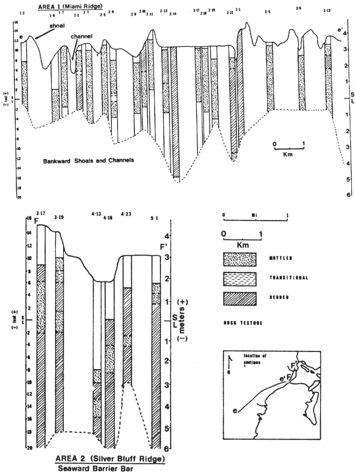
Figure 7. The distribution of the bedded (striped pattern) and mottled (squiggly pattern) facies in sections e-e' (top) and F-F' (bottom) of the Miami Limestone. Section e-e' is in the shoal and channel system, section F-F' is in the seaward barrier bar. The shoal and channel system is predominantly mottled with bedding restricted to the flanks of the individual shoals. The broad flat area between cores 2-13 and 2-21 is an artifact of the section; it parallels a contour line on the flank of a shoal. The seaward barrier bar is predominantly bedded, intercalated with thin mottled zones.
