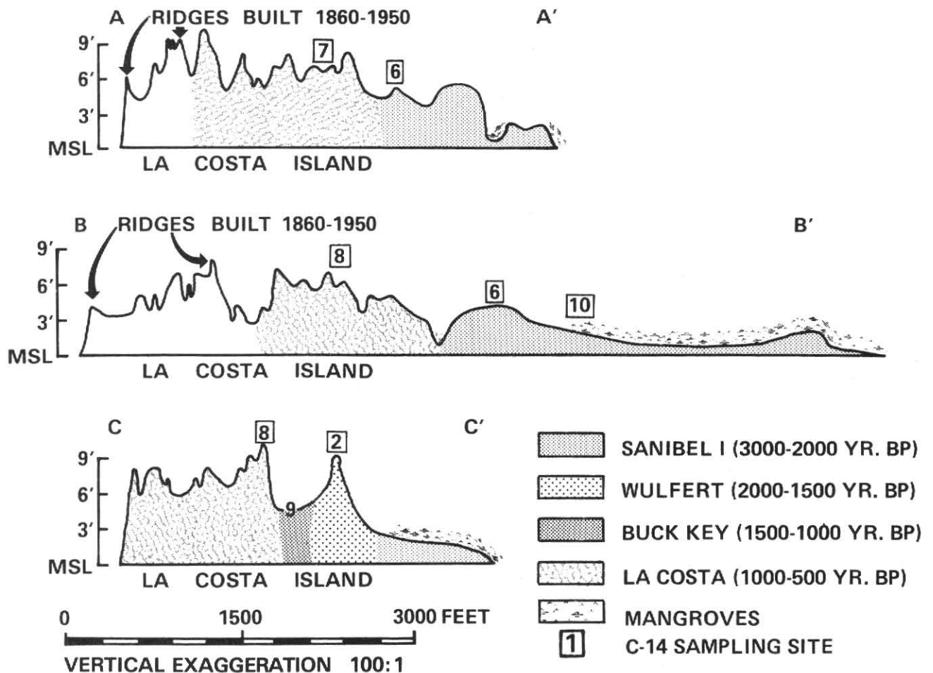
Figure 9. Topographic cross-sections of La Costa Island prepared from Hamrick Aerial Surveys (1981) photo-topographic maps with a 1-foot contour interval. The Gulf of Mexico is to the left and Pine Island Sound is to the right. The locations of these sections are shown in Figures 7 and 8.
