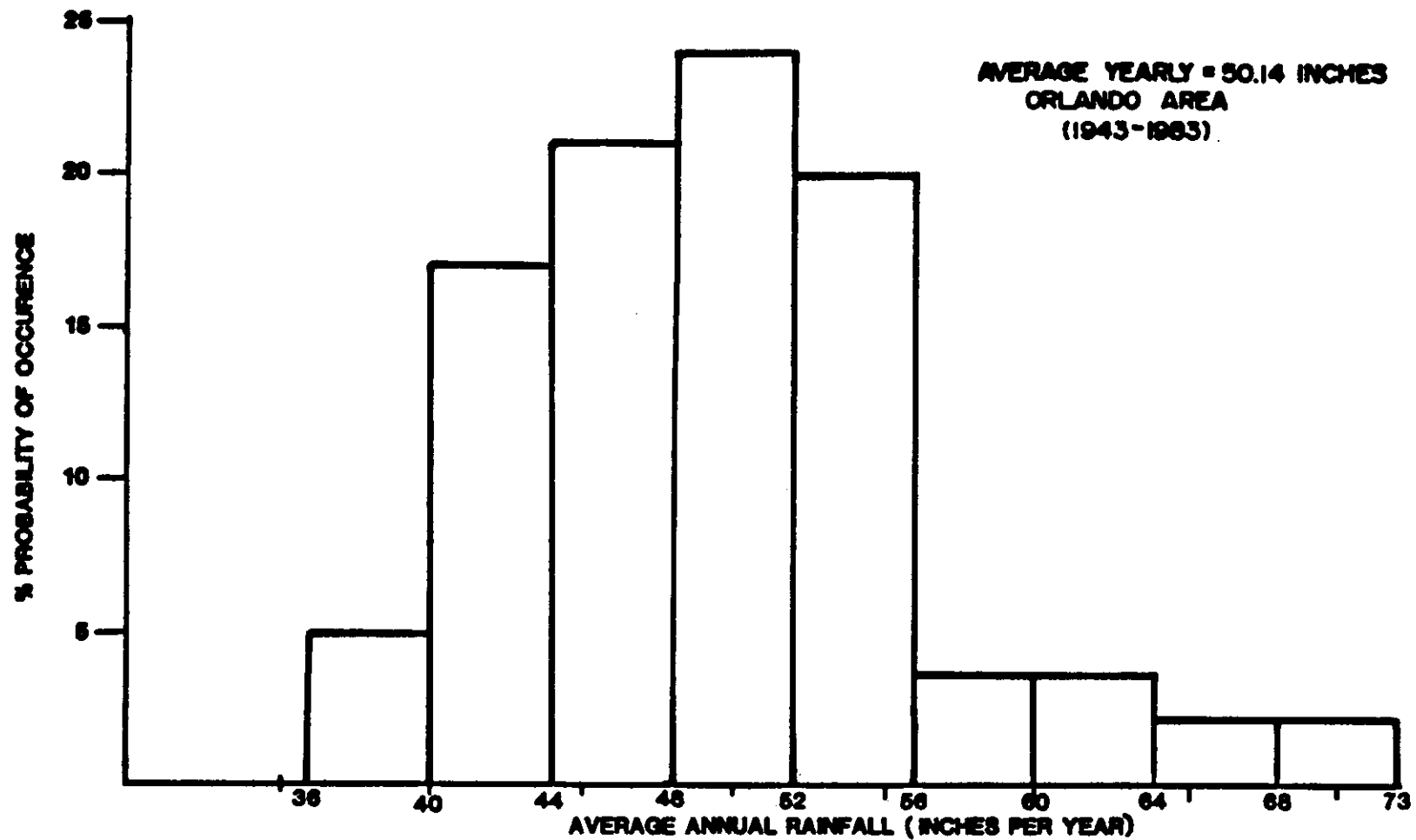
FIGURE 11 PROBABILITY OF OCCURRENCE OF A CERTAIN ANNUAL RAINFALL
