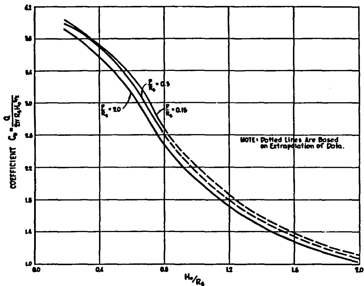
FIGURE 16 RELATIONSHIP OF CIRCULAR CREST COEFFICIENT C_c TO H_o/R_c FOR DIFFERENT APPROACH DEPTHS (AERATED NAPPE)
