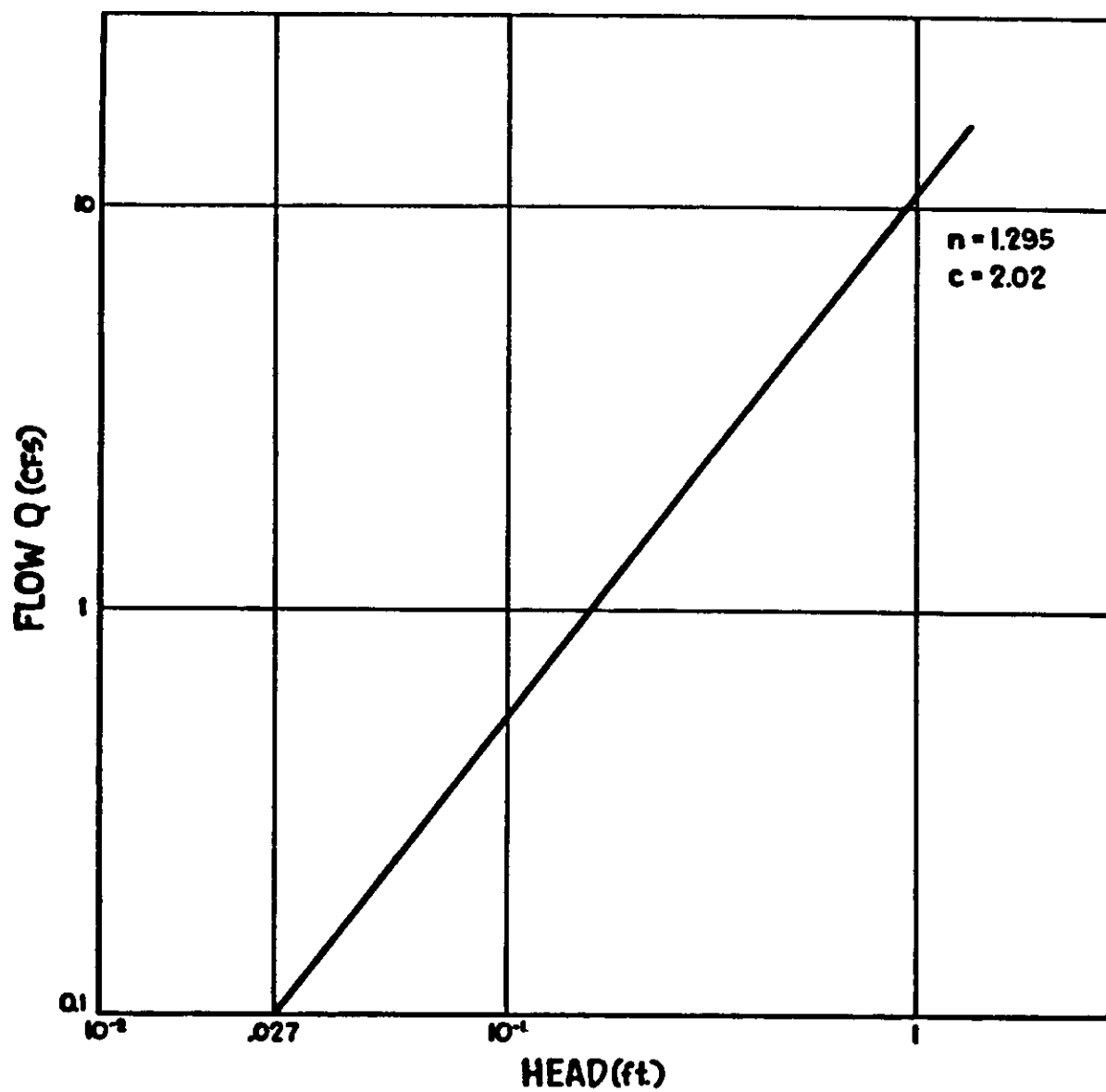
FIGURE 9 LAKE ANGEL WELL CALIBRATION: Q vs H
