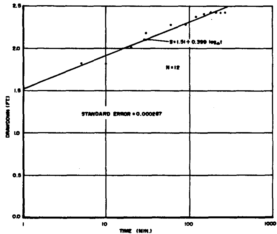
FIGURE 19 COOPER-JACOB SOLUTION FOR LAKE SHERWOOD WELL
