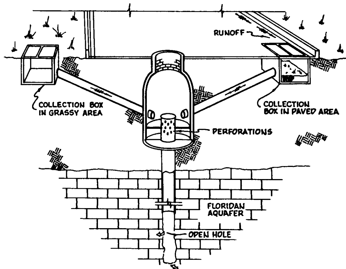
FIGURE 1 STORM SEWER DRAINWELL WITH CONNECTING INLETS
