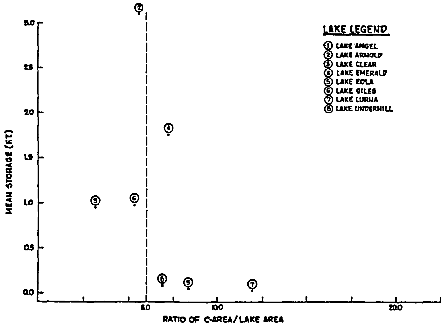
FIGURE 15 STORAGE VS C-AREA/LAKE RATIO FOR SEVEN ORLANDO LAKES
