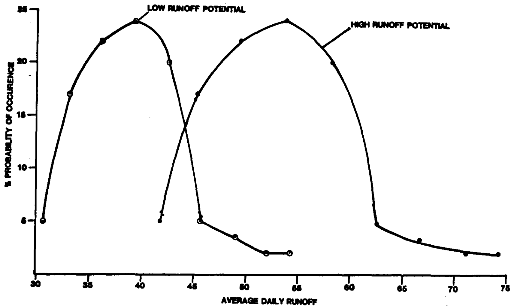
FIGURE 12 PROBABILITY OF AVERAGE DAILY RUNOFF FOR A GIVEN YEARLY RAINFALL
