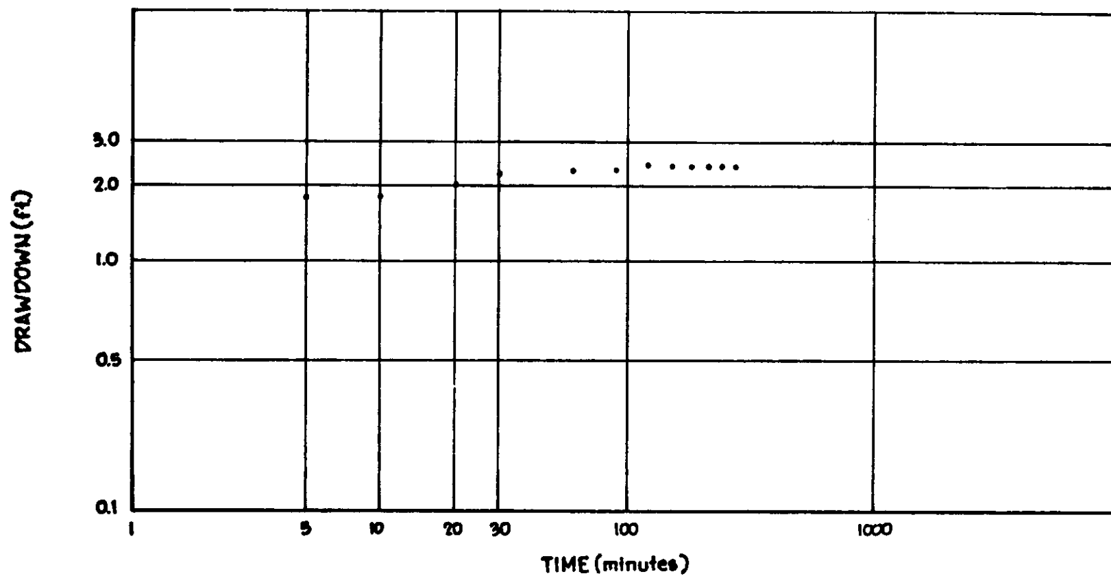
FIGURE 18 LAKE SHERWOOD DRAINAGE WELL PUMPING TEST JAN. 19, 1977 (DATA FROM ECFRPC 208 STUDY ; P. 3-3)
