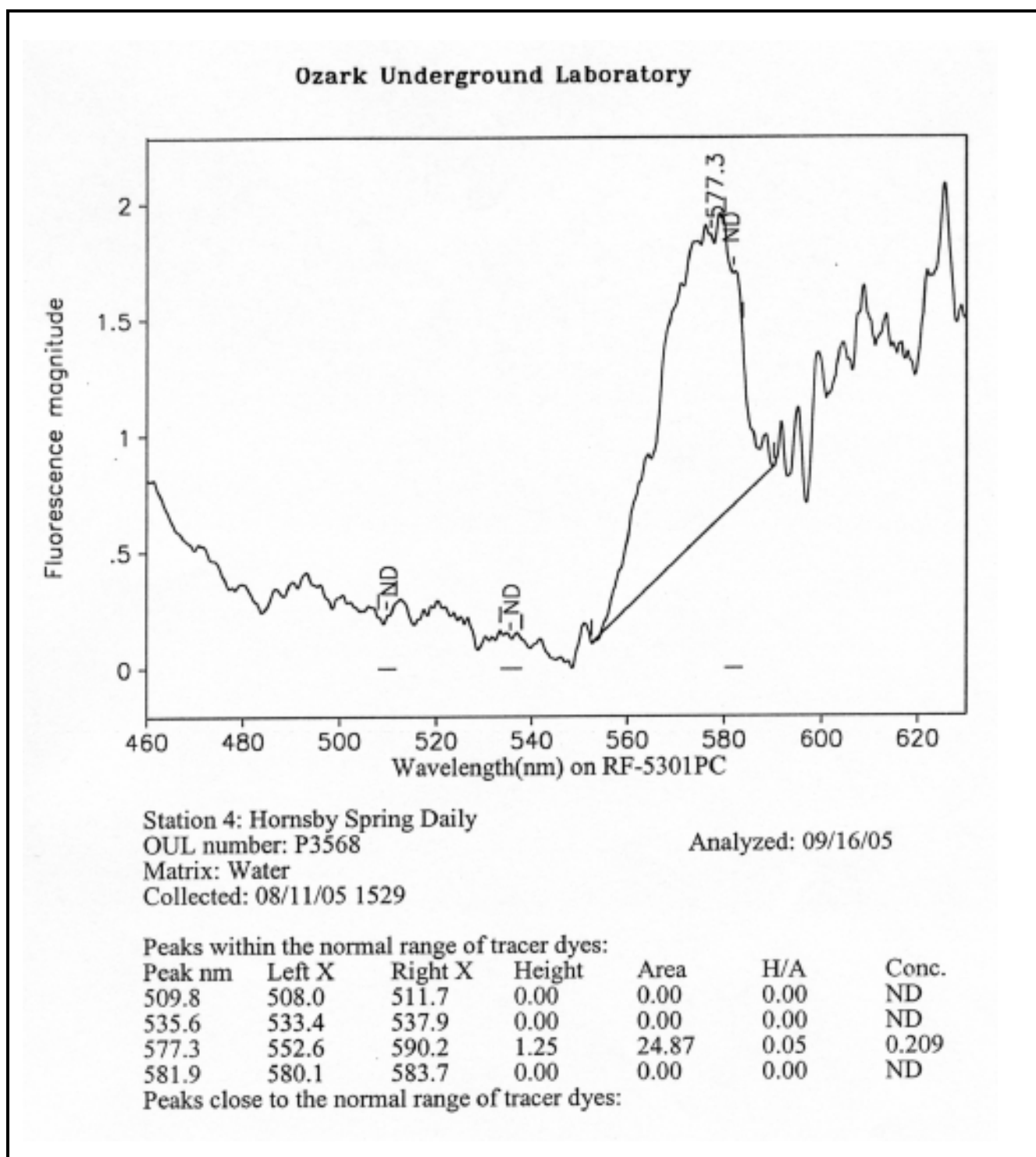
Figure 15. Example of Spectrofluorophotometer Analytical Graph. This graph indicates a positive detection for rhodamine WT dye from a water sample taken at Hornsby Spring. The wavelength peak indicates the specific dye present, and the fluorescence magnitude is used to calculate concentration in the sample.
