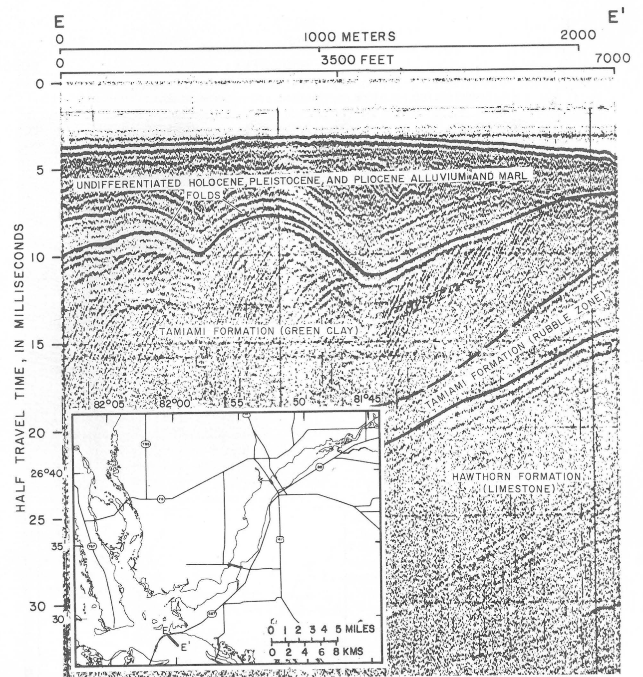
Figure 13.--Approximate 1.5-mile (2.4-kilometer) section of the boomer seismic record showing folds in the Tamiami Formation and the Holocene, Pleistocene, and the Pliocene strata.
