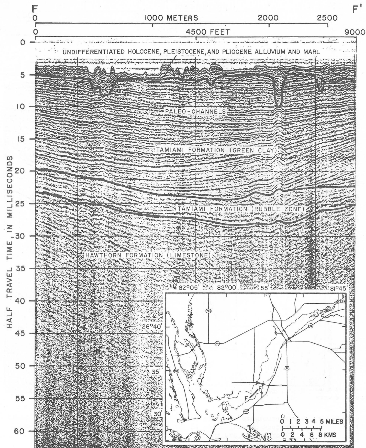
Figure 14.--Approximate 2-mile (3.2-kilometer) section of the boomer seismic record showing paleochannels.
