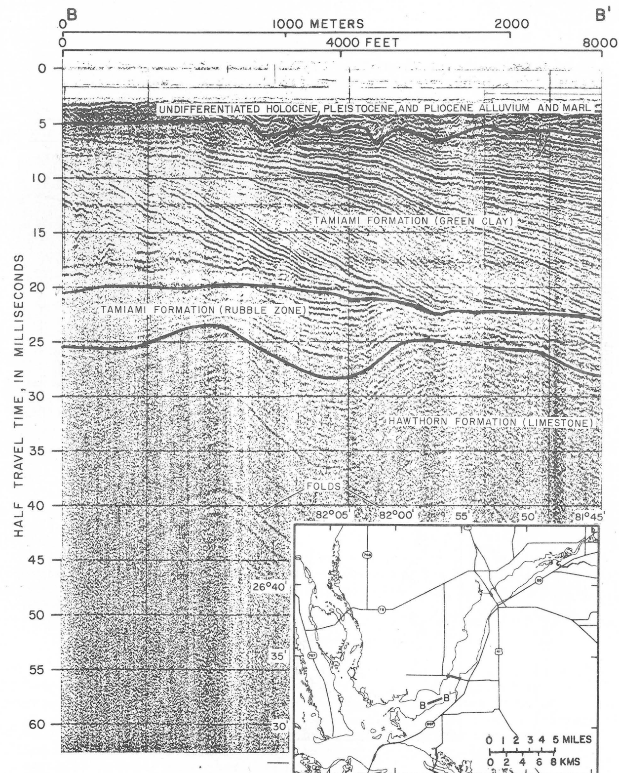
Figure 10.--Approximate 1.5-mile (2.4-kilometer) section of the boomer seismic record showing folds in the Hawthorn Formation.
