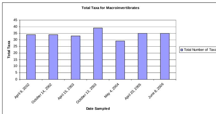
Figure 4: Total macroinvertebrate taxa plotted over time for Juniper Springs.
