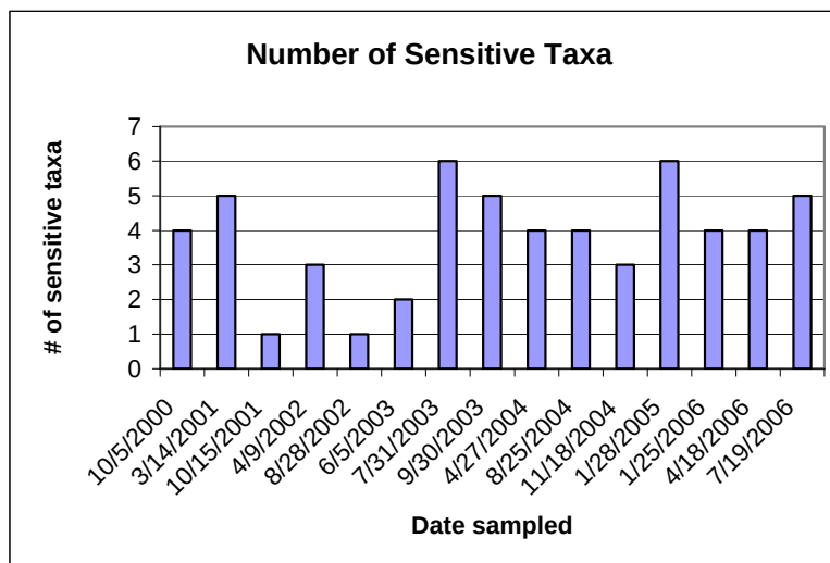
Figure 5: Chart and table showing number of sensitive taxa over the sampling period.
