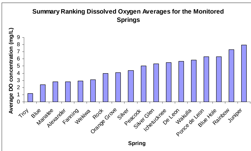
Figure 4. Summary of the average dissolved oxygen concentrations for each of the monitored springs, ranked in order from lowest to highest concentration.
