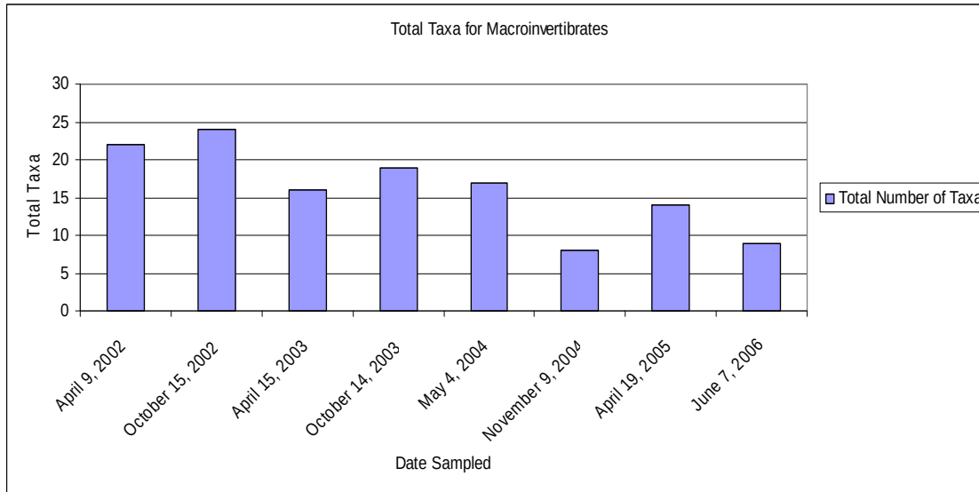
Figure 4: Total macroinvertebrate taxa plotted over time.
