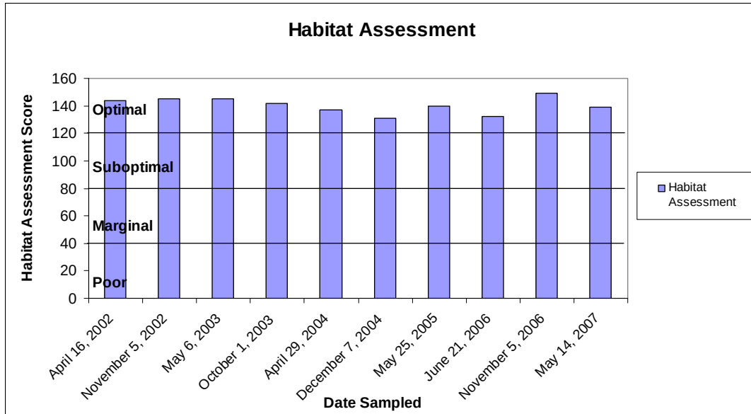
Figure 6: Habitat assessment scores plotted for sampling events.
