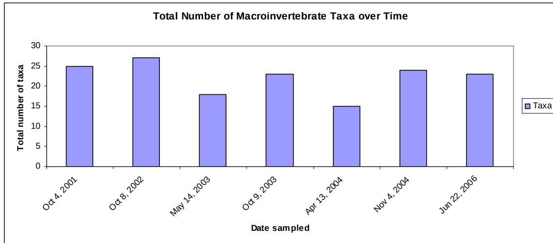
Figure 4: Total macroinvertebrate taxa plotted at each sampling event.
