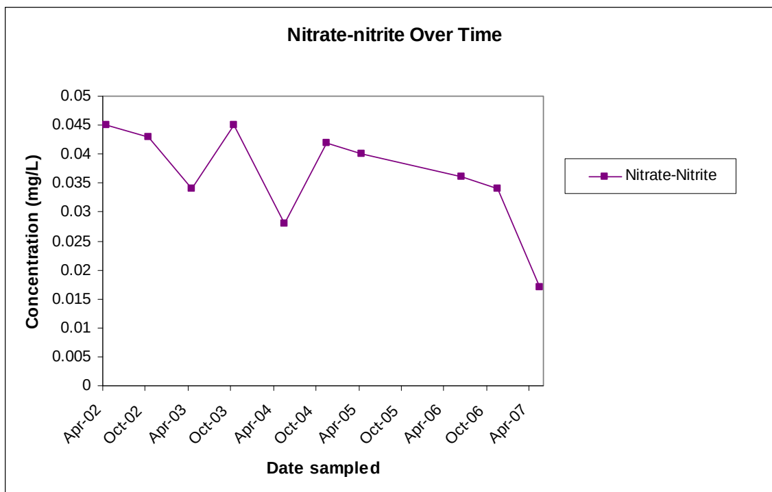
Figure 2: Nitrate-nitrite concentrations plotted over time.
