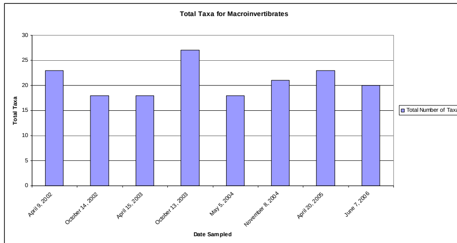
Figure 4: Total macroinvertebrate taxa for each sampling event.
