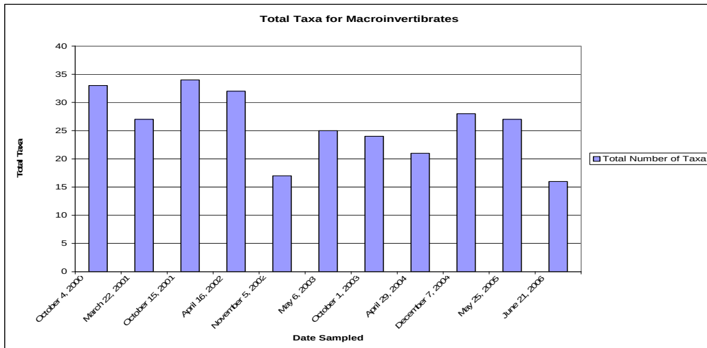
Figure 4: Total macroinvertebrate taxa for each sampling event.
