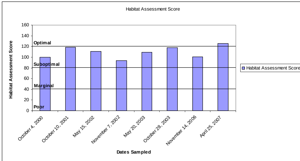
Figure 6: Habitat assessment score for each sampling event.
