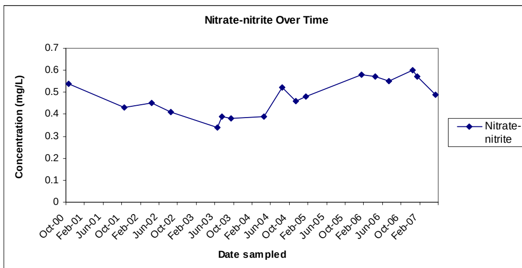
Figure 2: Nitrate-nitrite data plotted over time for Ichetucknee Springs.
