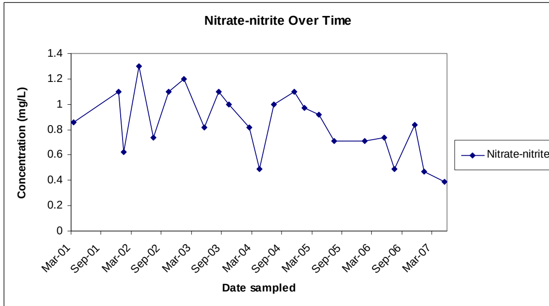
Figure 2: Nitrate-nitrite values plotted over time.
