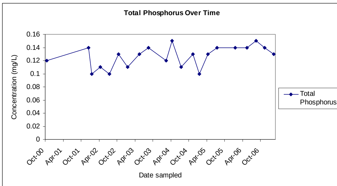
Figure 1: Total Phosphorus concentrations plotted over time.
