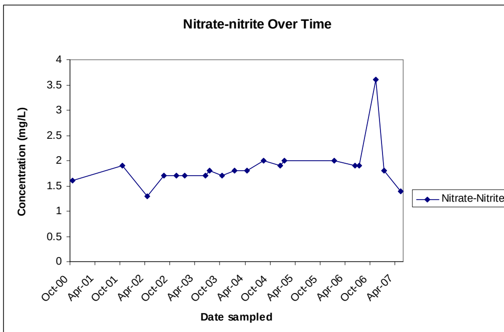
Figure 2: Nitrate-Nitrite values plotted over time.
