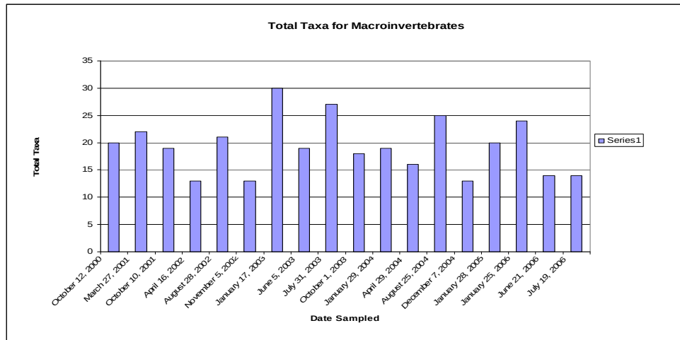
Figure 4: Total macroinvertebrate taxa for each sampling event.
