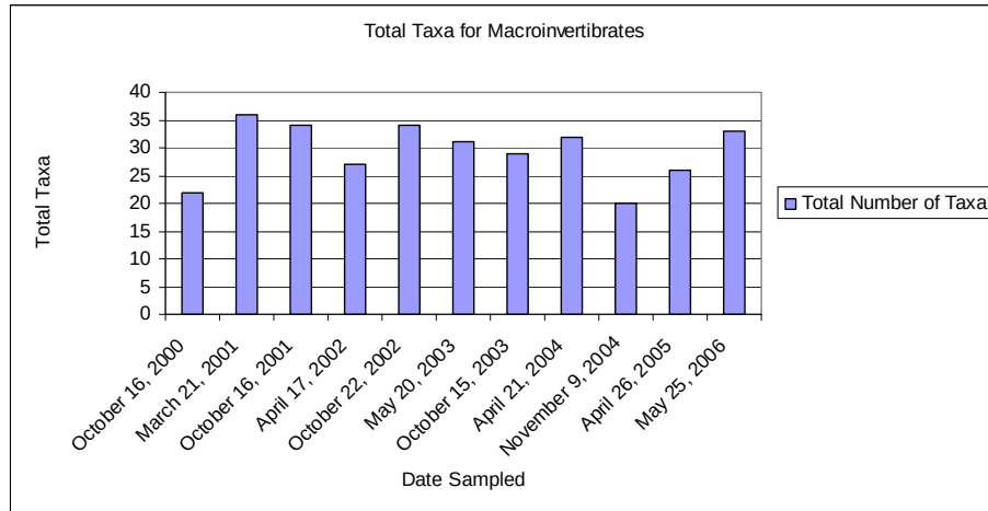
Figure 4: Total macroinvertebrate taxa plotted over time.
