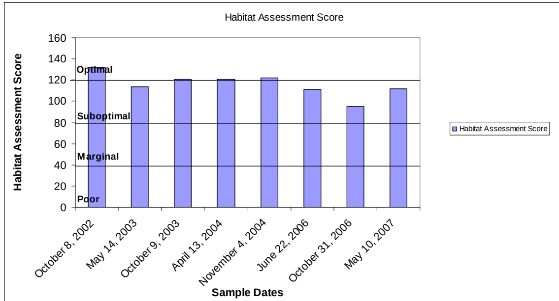
Figure 6: Habitat assessment scores plotted at each sampling event.
