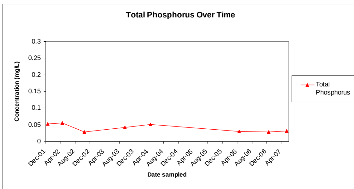
Figure 1: Total Phosphorus values plotted over time.
