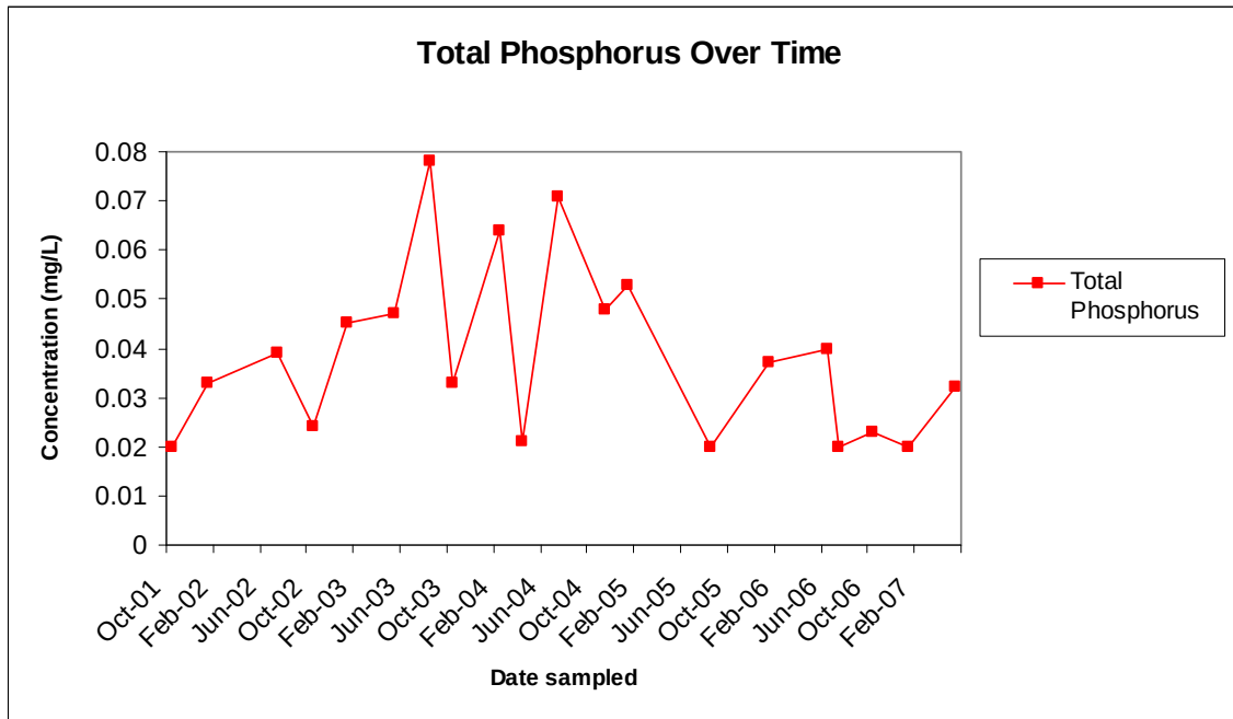
Figure 1: Total phosphorus concentrations plotted over time.
