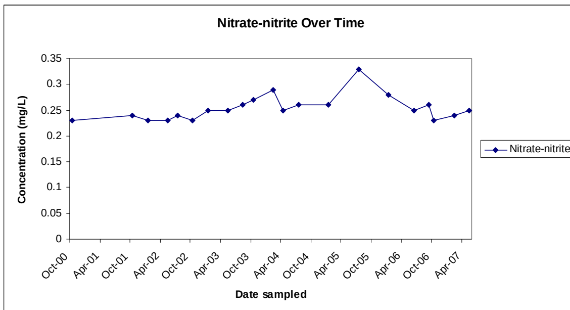
Figure 2: Nitrate-nitrite data plotted over time for Ponce de Leon Springs.
