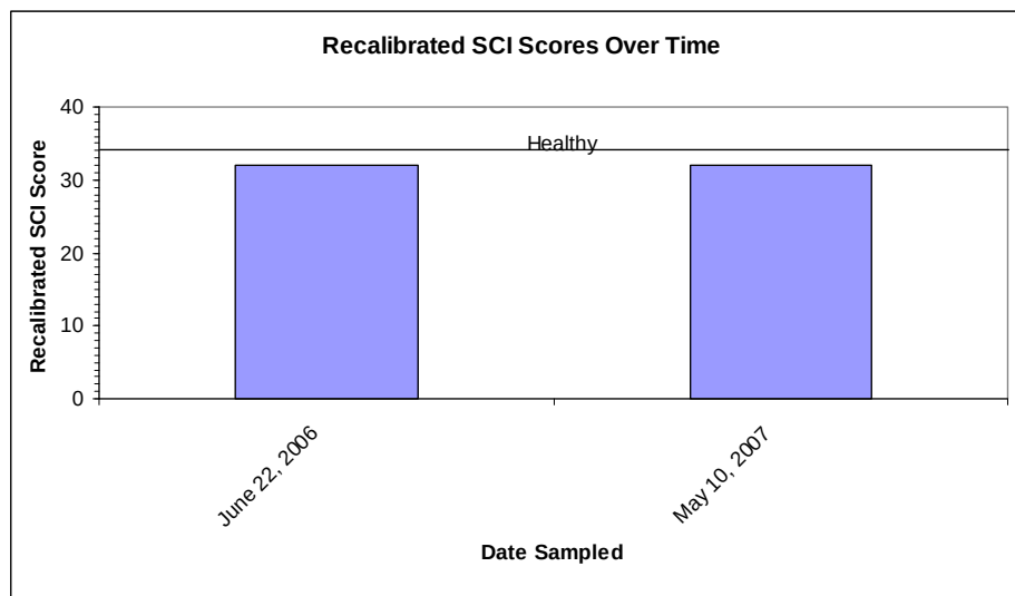
Figure 3: Recalibrated SCI scores with the impairment line drawn at 34.
