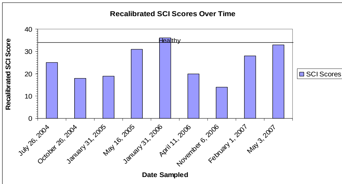
Figure 3: Recalibrated SCI scores for each sampling event, showing the impairment line at 34.
