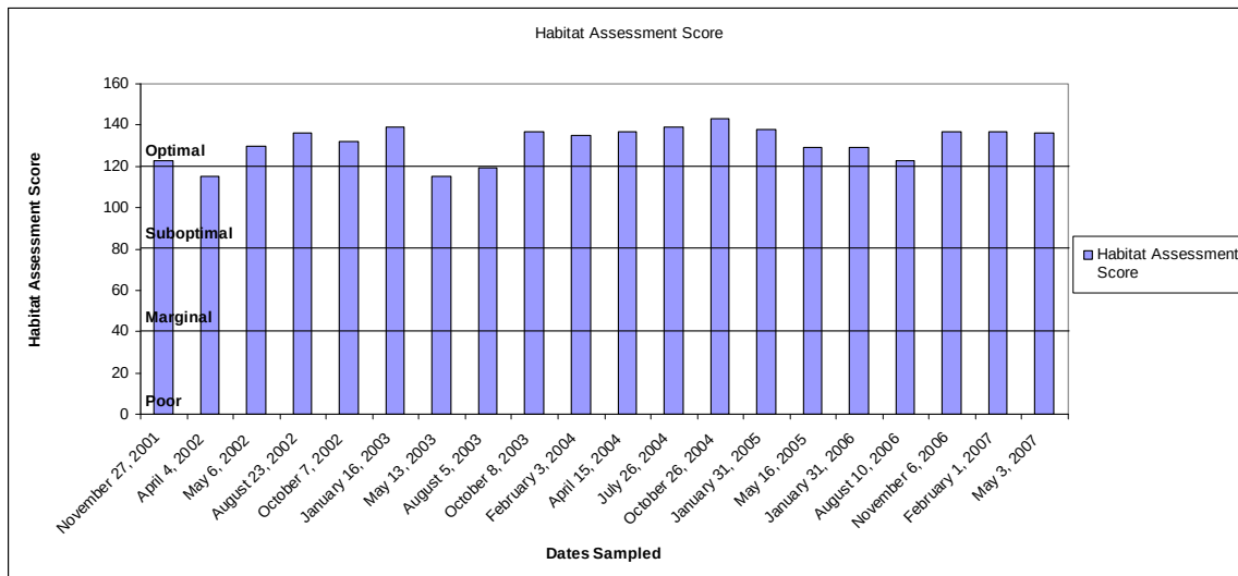
Figure 6: Habitat Assessment scores for each sampling event.
