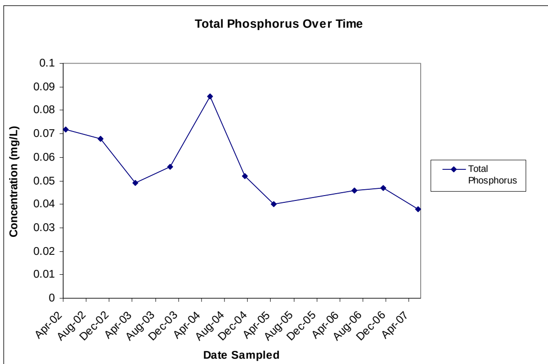
Figure 1: Total phosphorous concentrations plotted over time.
