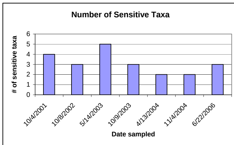
Figure 5: Number of sensitive taxa over the sampling period.
