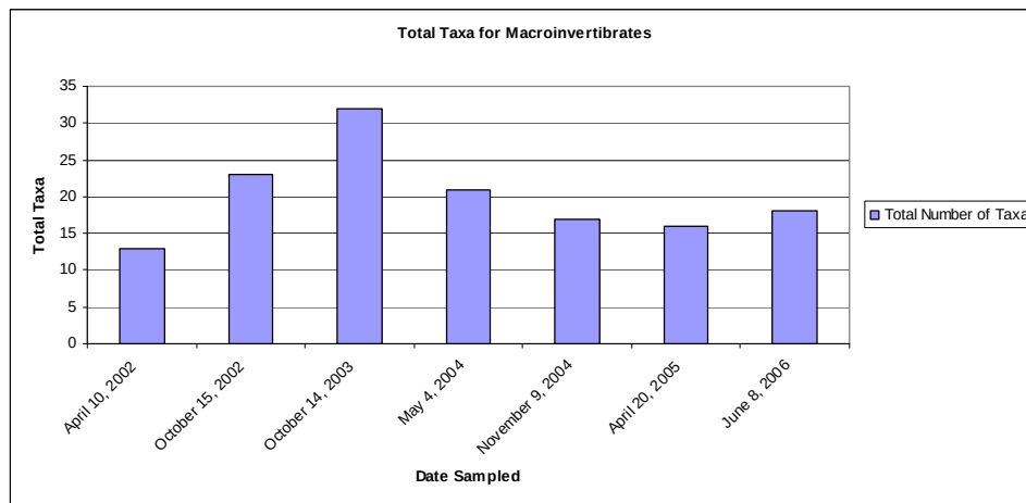
Figure 4: Total macroinvertebrate taxa plotted over time.
