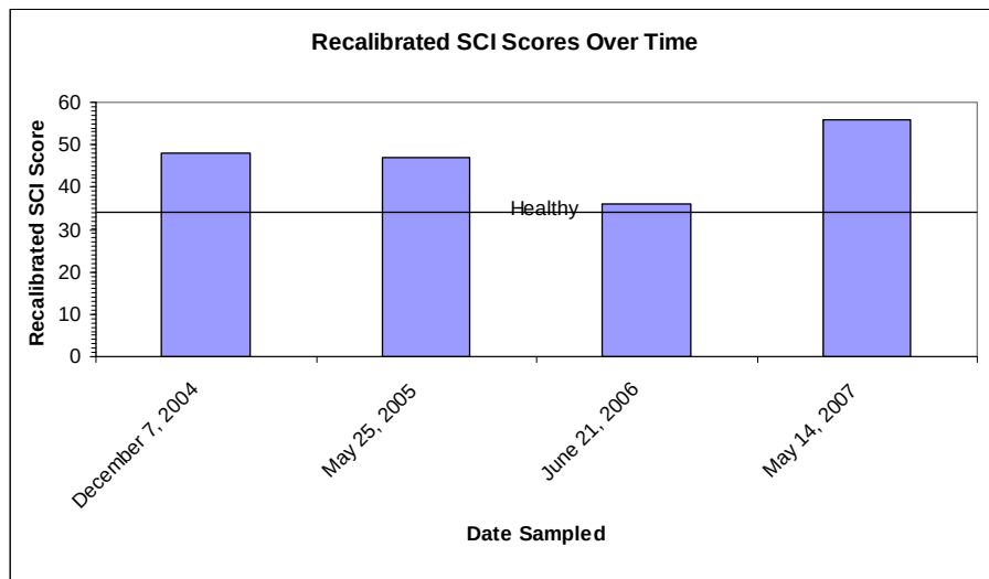
Figure 3: Recalibrated SCI scores with the impairment threshold at 34.
