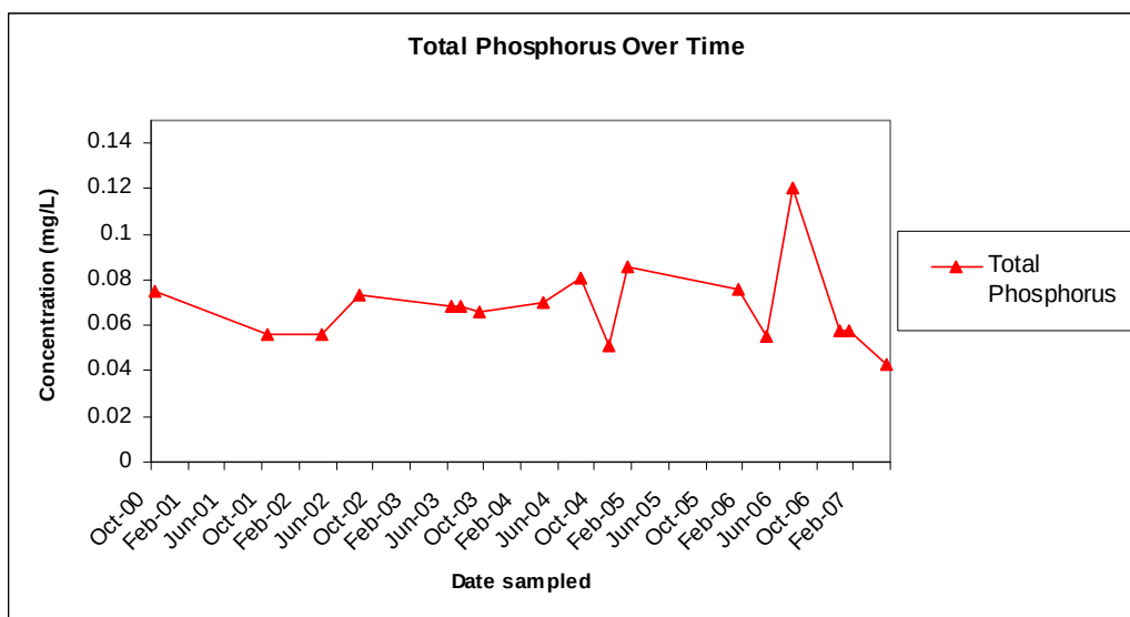
Figure 1: Total Phosphorus data plotted over time for Ichetucknee Springs.
