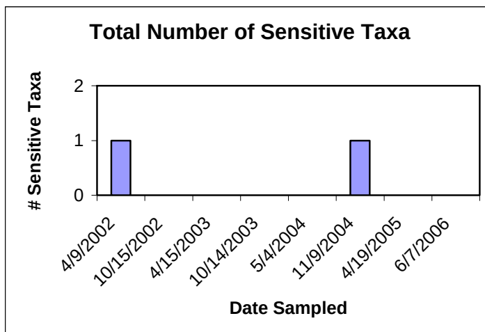
Figure 5: Total number of sensitive taxa over the sampling period.
