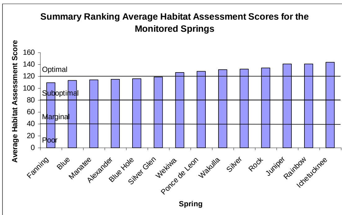
Figure 6. Summary of the average Habitat Assessment scores for each of the monitored springs, ranked in order from lowest to highest score. Lines are drawn showing the optimal, suboptimal, marginal and poor categories.
