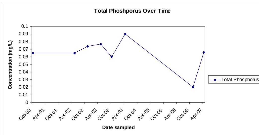
Figure 1: Total Phosphorus values plotted over time.
