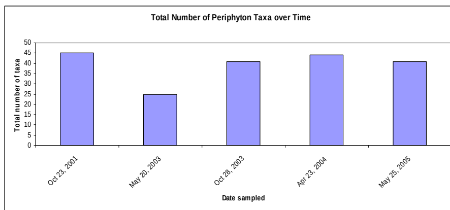
Figure 3: Total number of taxa for periphyton for each sampling event for Peacock Spring.
