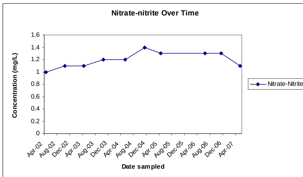
Figure 2: Nitrate-nitrite data plotted over time.
