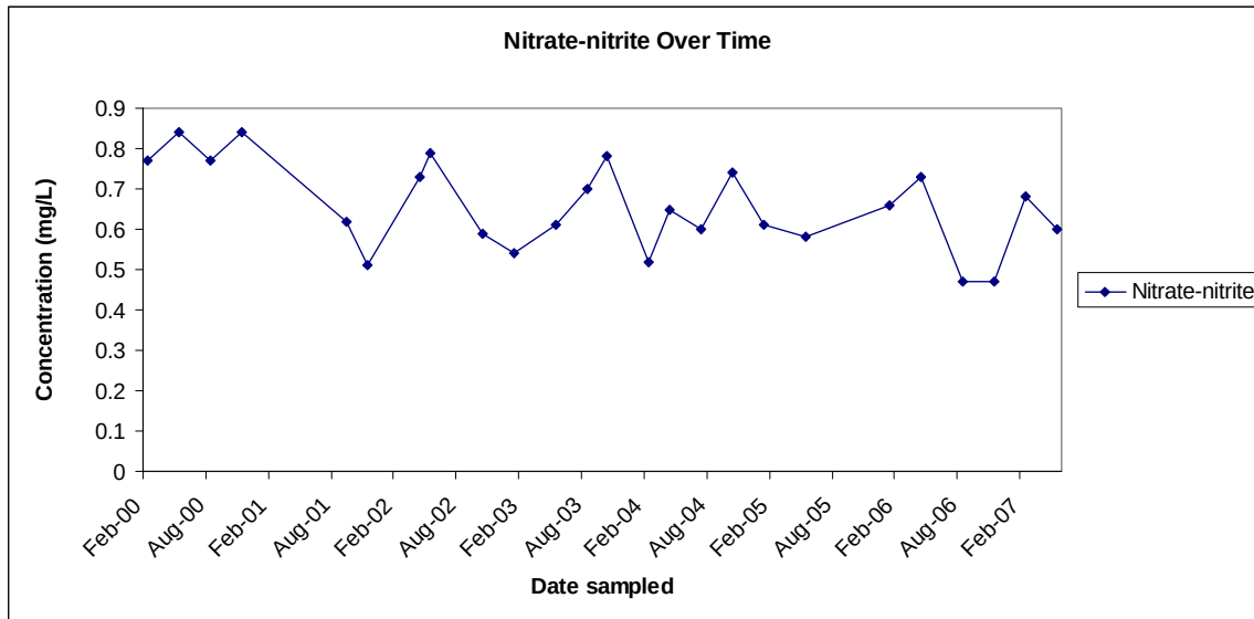
Figure 2: Nitrate-nitrite values plotted over time.
