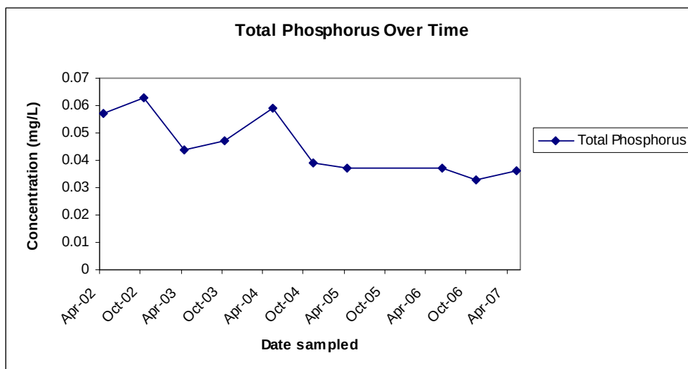
Figure 1: Total Phosphorus data plotted over time.
