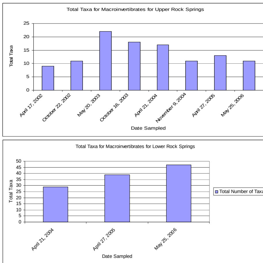
Figure 4: Total macroinvertebrate taxa plotted over time for Upper and Lower Rock Springs.
