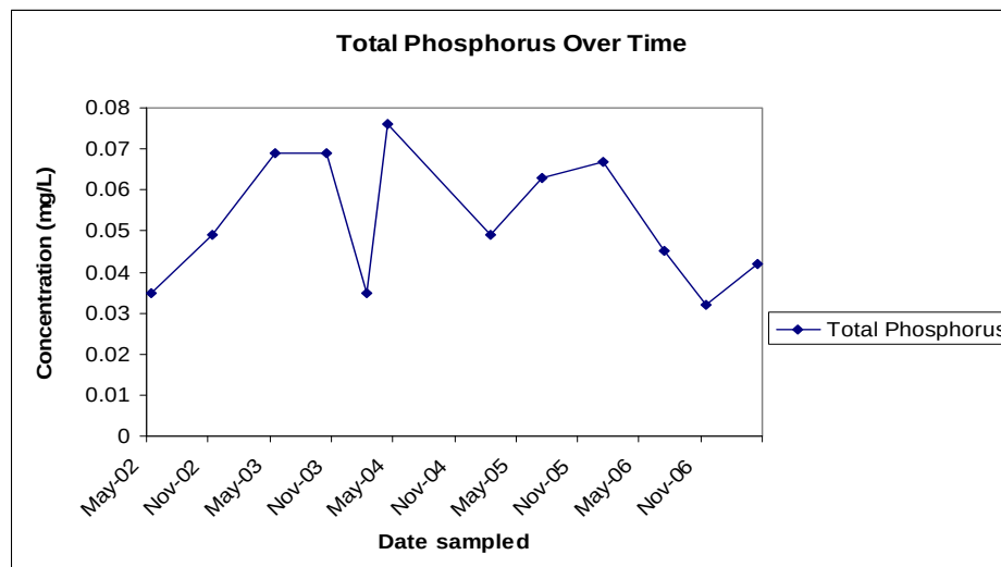
Figure 4: Total Phosphorus values plotted over time for Orange Grove Sink.
