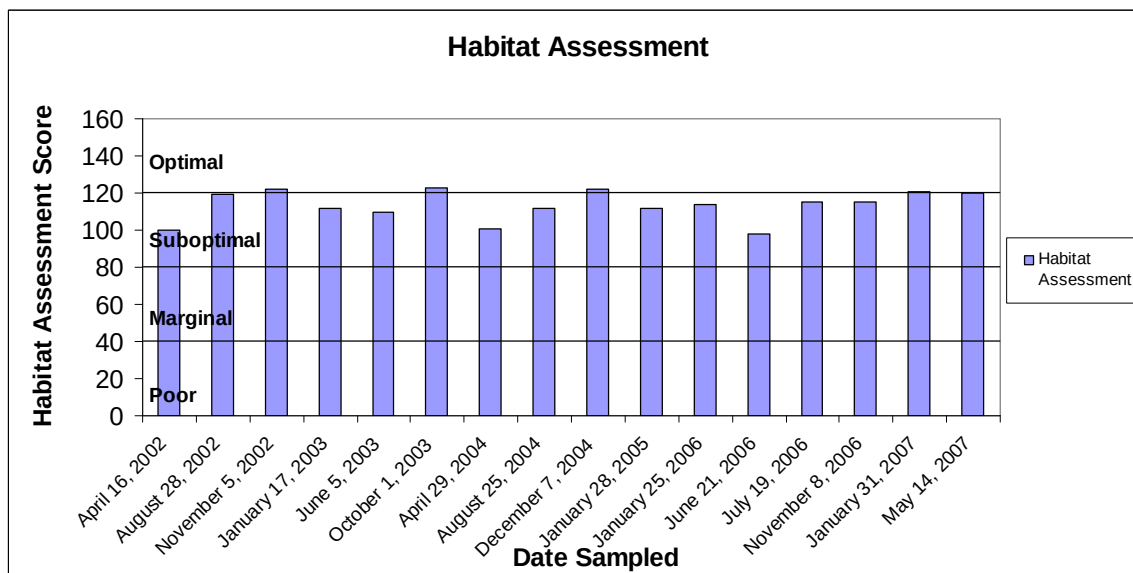
Figure 6: Habitat assessment scores plotted for each sampling event.
