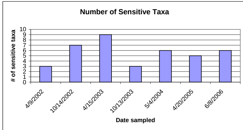
Figure 5: Table and chart showing the number of sensitive taxa over the sampling period.
