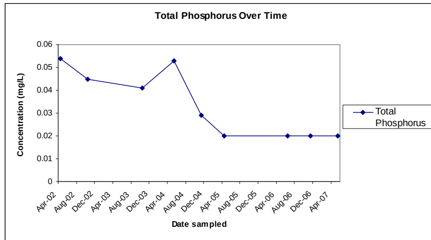
Figure 1: Total Phosphorus concentrations plotted over time.
