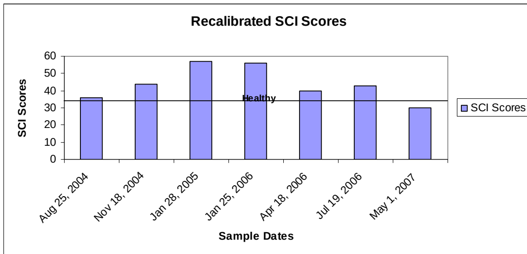
Figure 3: Recalibrated SCI scores over the period from August 25, 2004 to July 19, 2006 showing the impairment line at 34.
