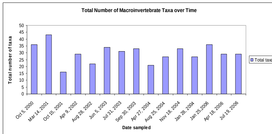
Figure 4: Total macroinvertebrate taxa plotted over time for Ichetucknee Springs.
