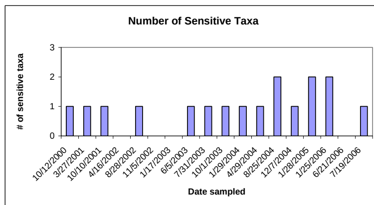
Figure 5: Table and chart showing number of sensitive taxa over time.
