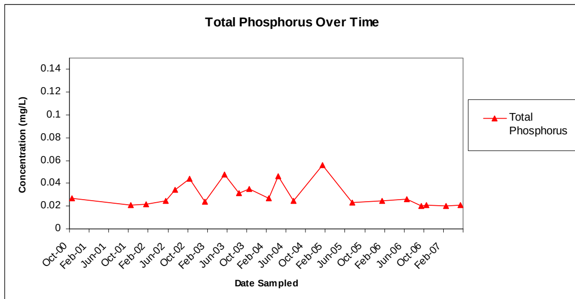
Figure 1: Total Phosphorus concentrations plotted over time for Ponce de Leon Springs.
