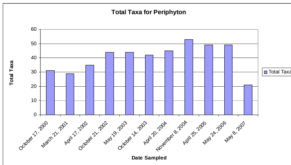
Figure 3: Total number of taxa for periphyton for each sampling event.
