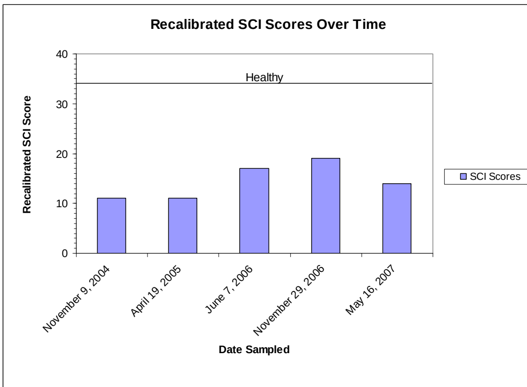
Figure 3: Recalibrated SCI scores over the period showing the impairment line at 34.
