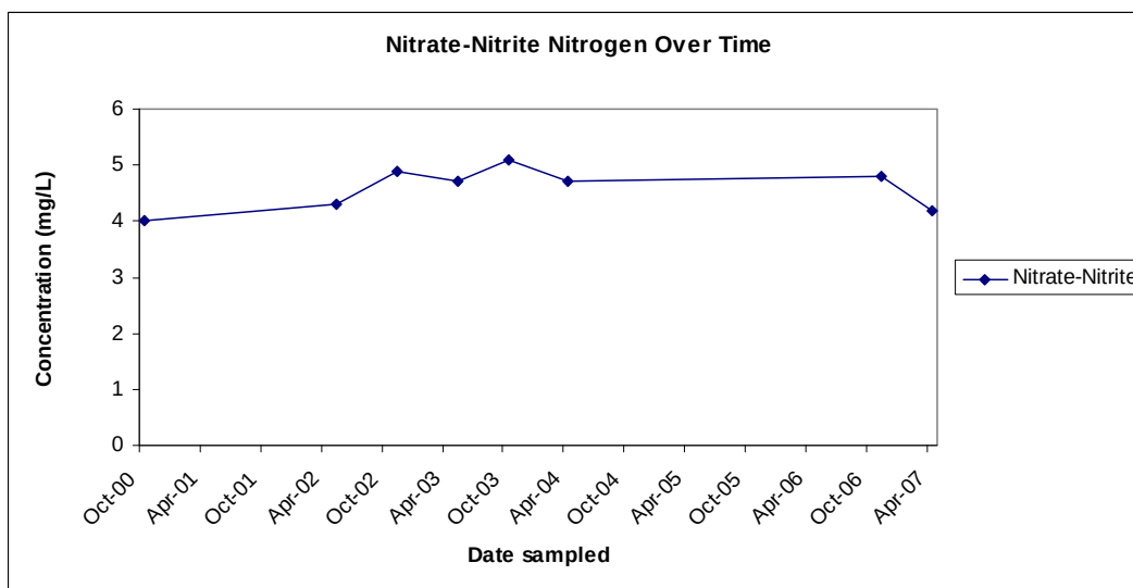
Figure 2: Nitrate-nitrite values plotted over time.
