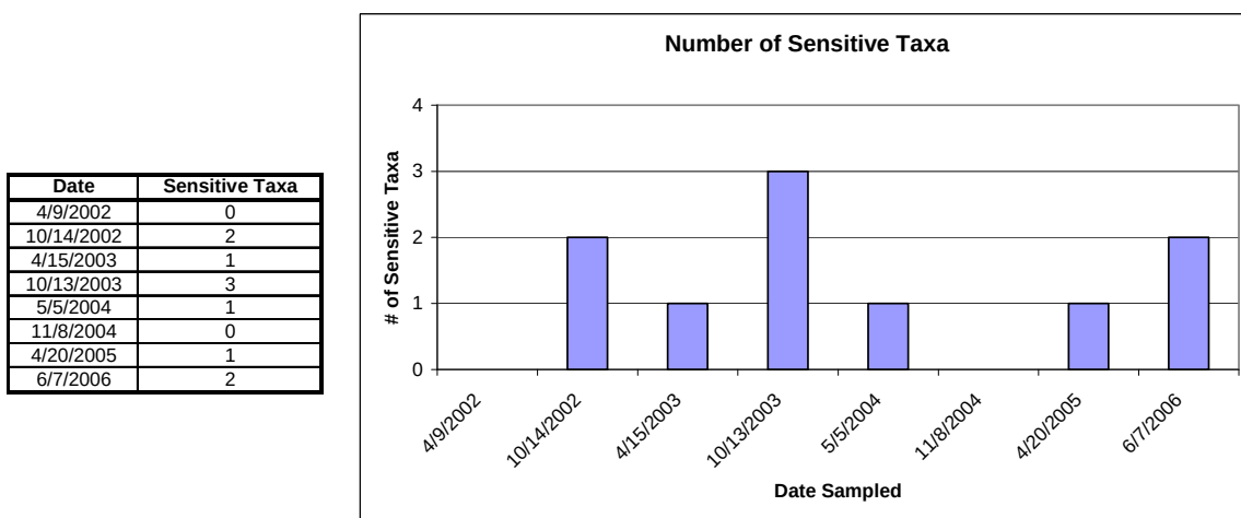
Figure 5: Table and chart showing the number of sensitive taxa over the sampling period.
