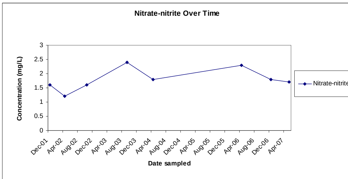
Figure 2: Nitrate-nitrite values plotted over time.
