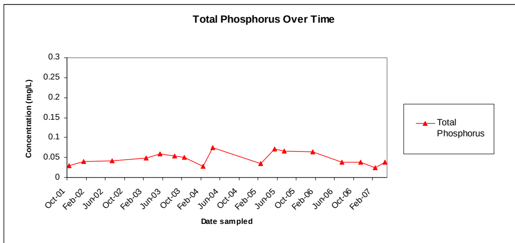
Figure 1: Total Phosphorus values plotted over time for Peacock Spring.
