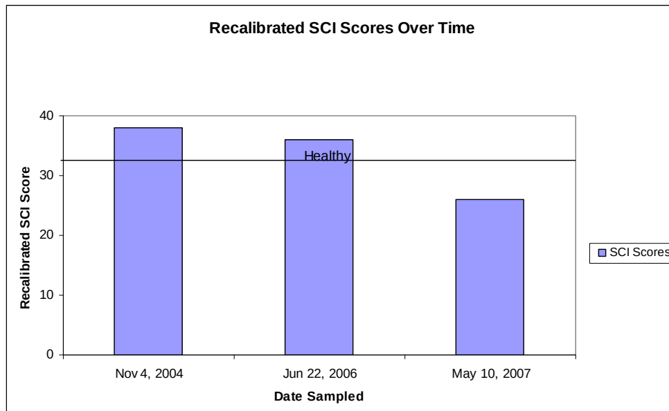
Figure 3: Recalibrated SCI scores over the period showing the impairment line at 34.
