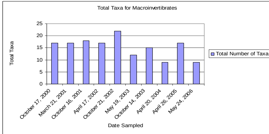
Figure 4: Total macroinvertebrate taxa plotted over time.
