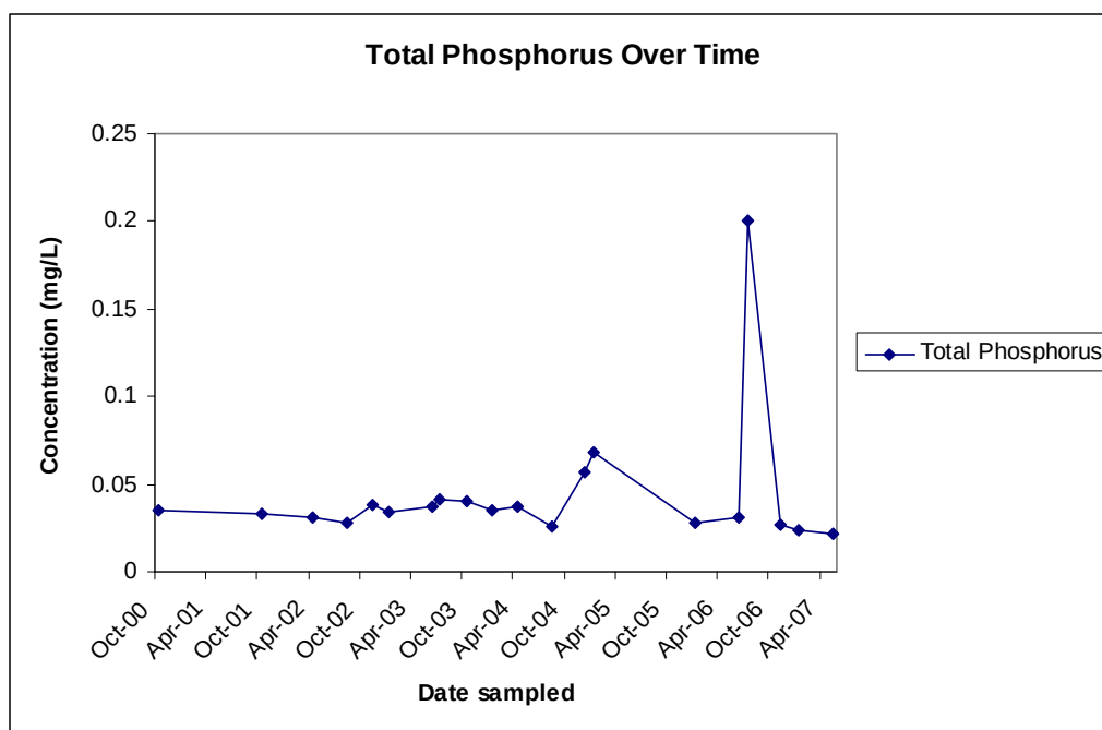
Figure 1: Total Phosphorus values plotted over time.
