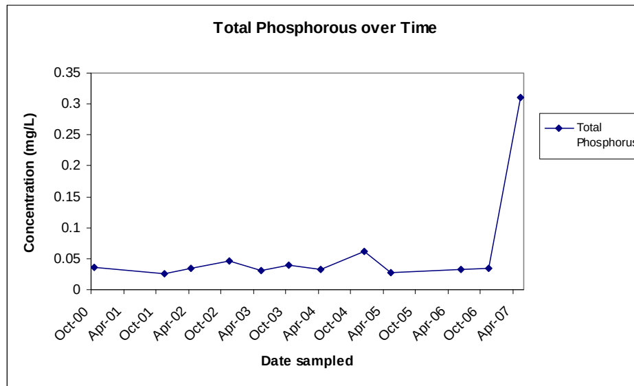
Figure 1: Total phosphorus concentrations plotted over time.
