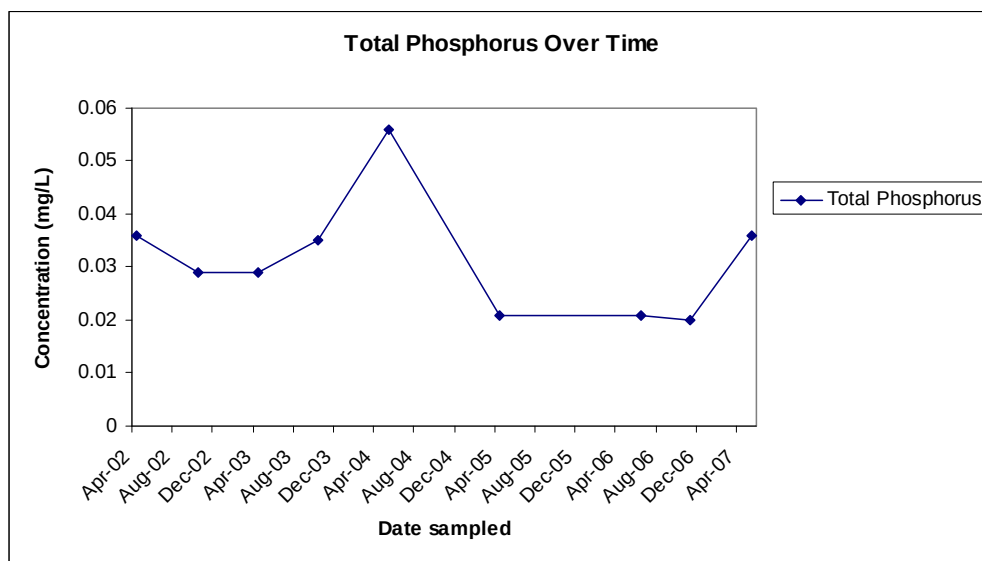
Figure 1: Total Phosphorus concentrations plotted over time.
