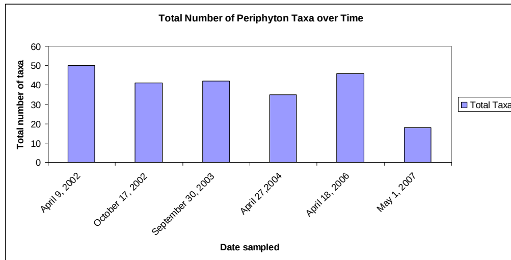
Figure 3: Total number of periphyton taxa plotted for each sampling event.
