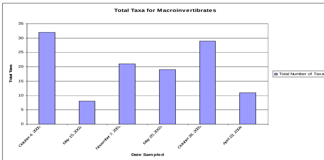
Figure 4: Total number of macroinvertebrate taxa for each sampling event.
