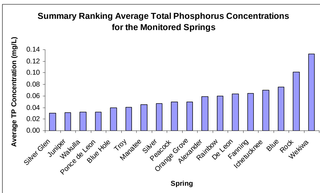
Figure 2. Summary of the average total phosphorus concentrations for each of the monitored springs, ranked in order from lowest to highest concentration.
