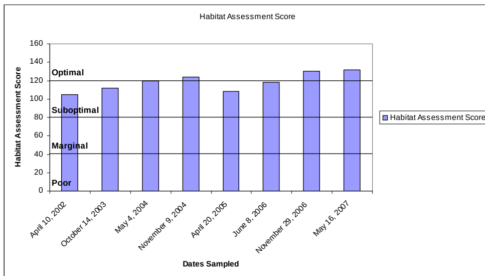
Figure 6: Habitat assessment scores over time.
