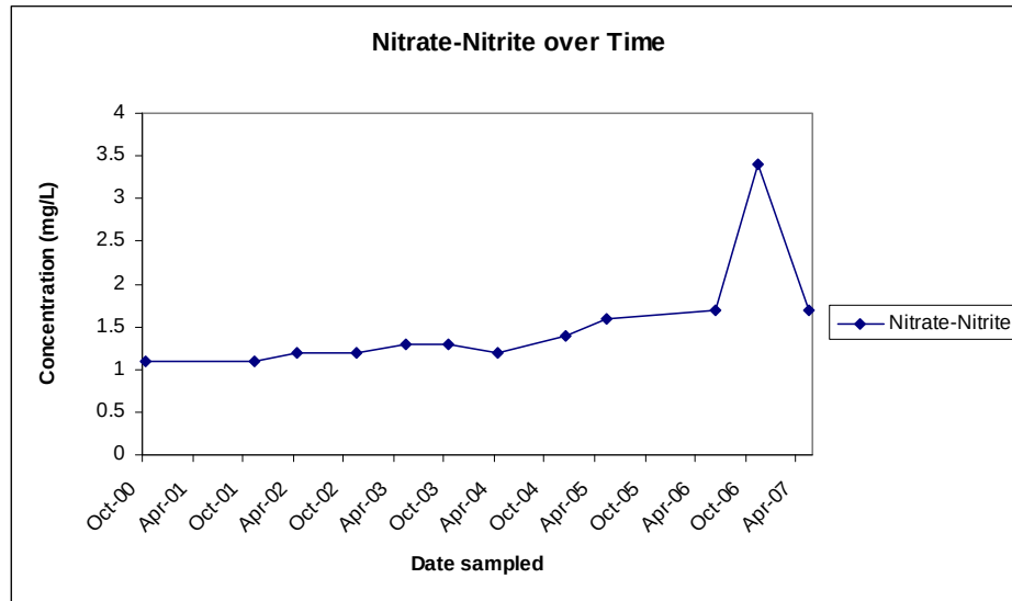
Figure 2: Nitrate-nitrite data plotted over time.
