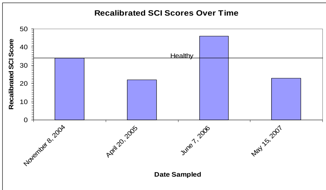
Figure 3: Recalibrated SCI Scores with a line drawn at the impairment threshold of 34.
