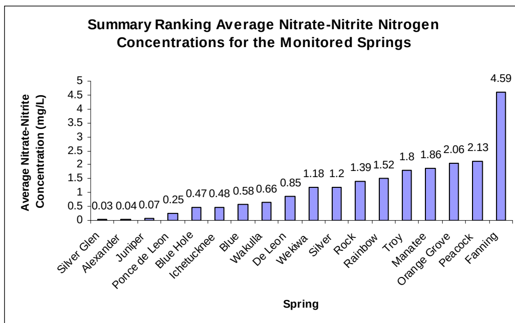
Figure 1: Summary of the average nitrate-nitrite nitrogen concentrations for each of the monitored springs, ranked in order from lowest to highest concentration.
