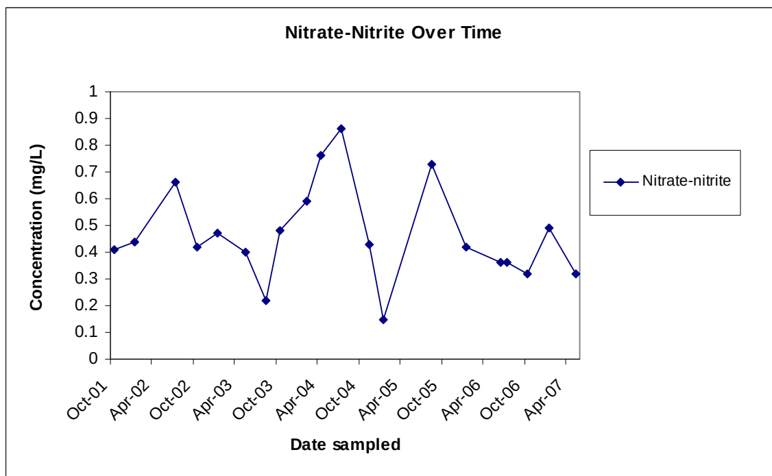
Figure 2: Nitrate-nitrite concentrations plotted over time.
