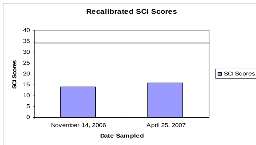
Figure 3: Recalibrated SCI scores.
