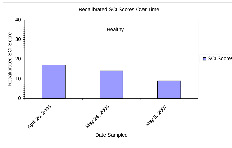
Figure 3: Recalibrated SCI scores over time.
