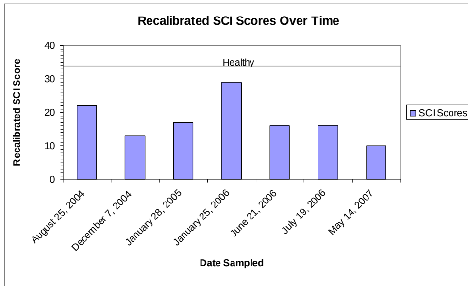
Figure 3: Recalibrated SCI scores plotted for each sampling event.
