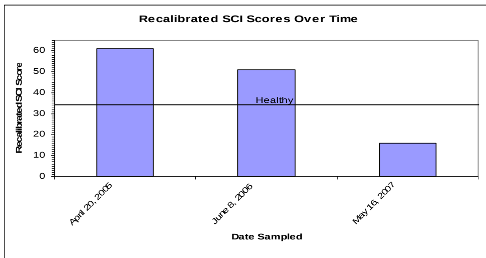
Figure 3: Recalibrated SCI scores with the impairment line at 34.
