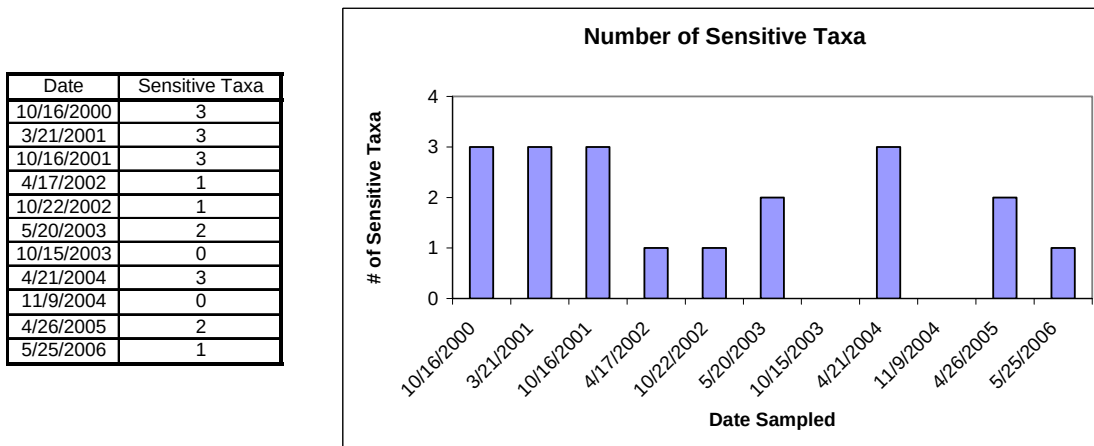
Figure 5: Table and chart showing the number of sensitive taxa over the sampling period.
