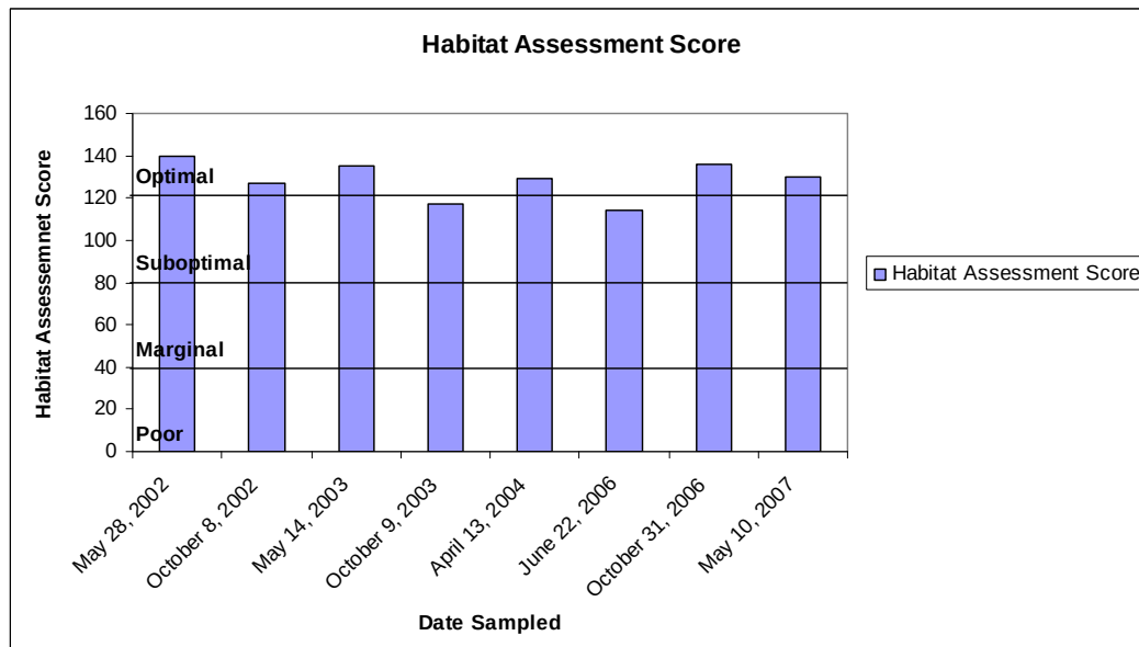
Figure 6: Habitat assessment scores plotted for sampling events.
