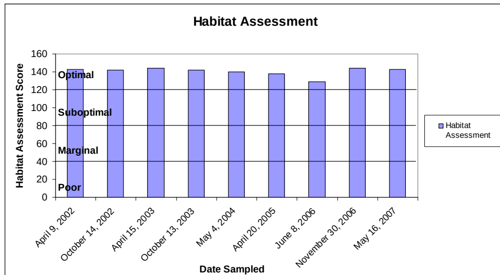
Figure 6: Habitat assessment scores over time.
