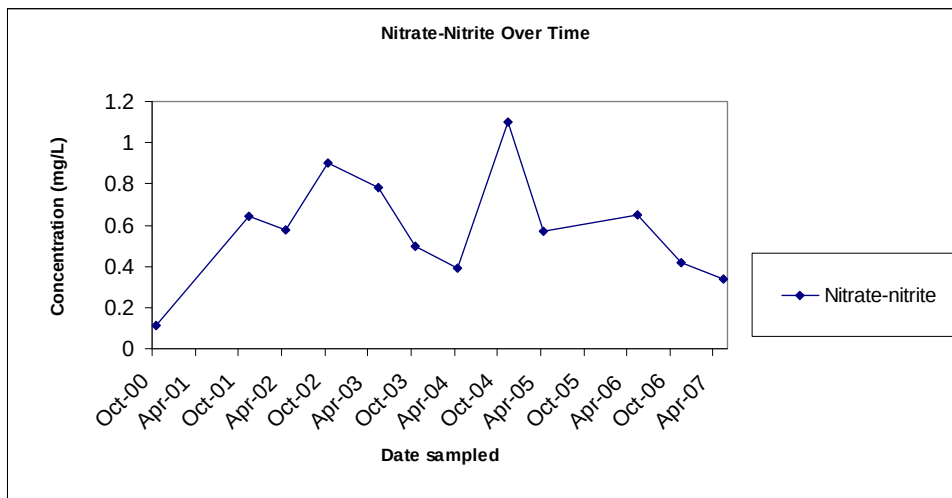
Figure 2: Nitrate-nitrite concentrations plotted over time.
