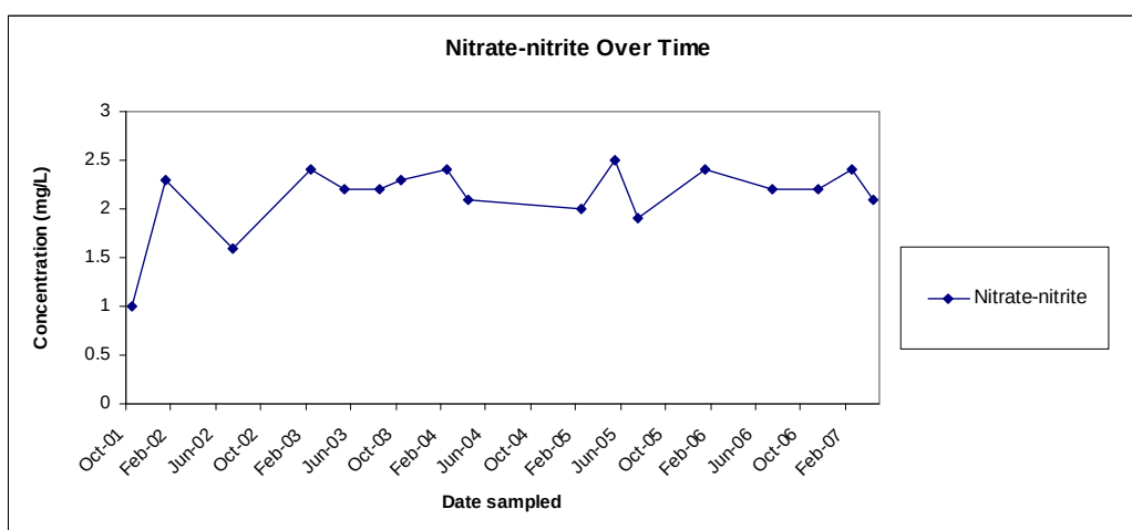
Figure 2: Nitrate-nitrite values plotted over time for Peacock Spring.
