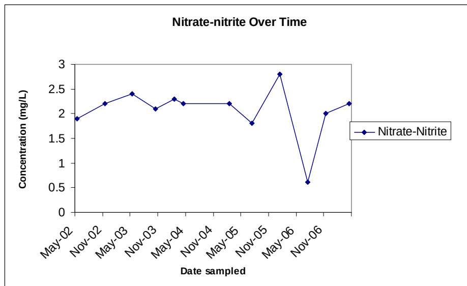
Figure 5: Nitrate-nitrite values plotted over time for Orange Grove Sink.
