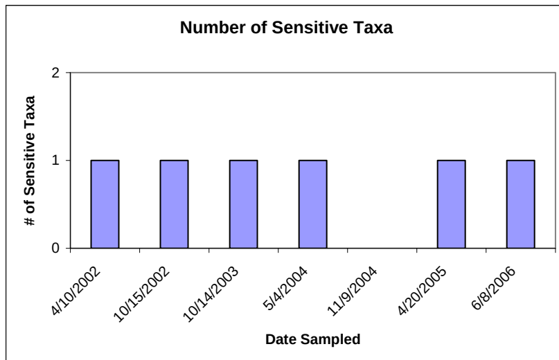
Figure 5: Table and chart showing the number of sensitive taxa over the sampling period.
