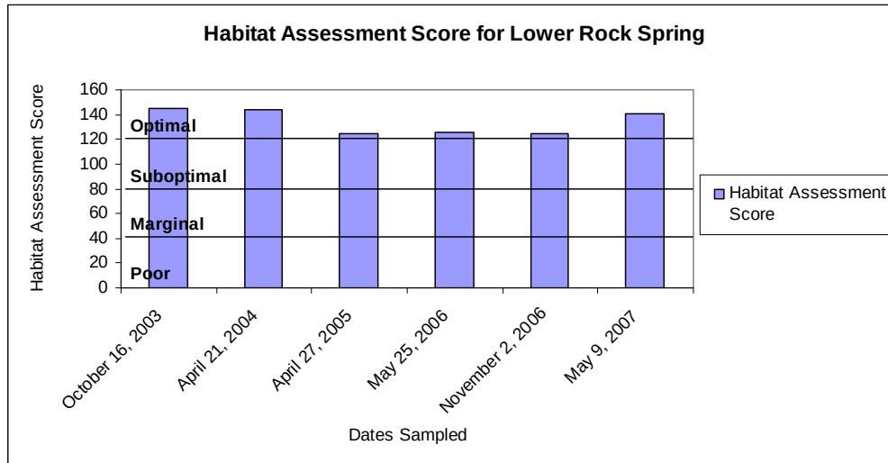
Figure 6: Habitat assessment scores over time for Upper and Lower Rock Springs.
