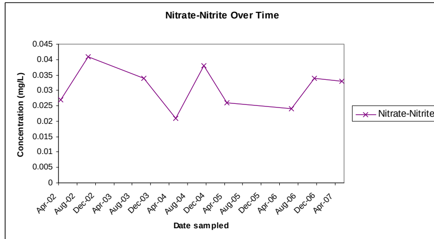
Figure 2: Nitrate-nitrite concentrations plotted over time.
