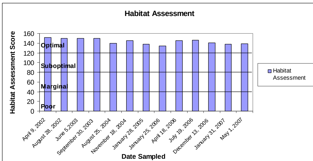
Figure 6: Habitat assessment scores over time.
