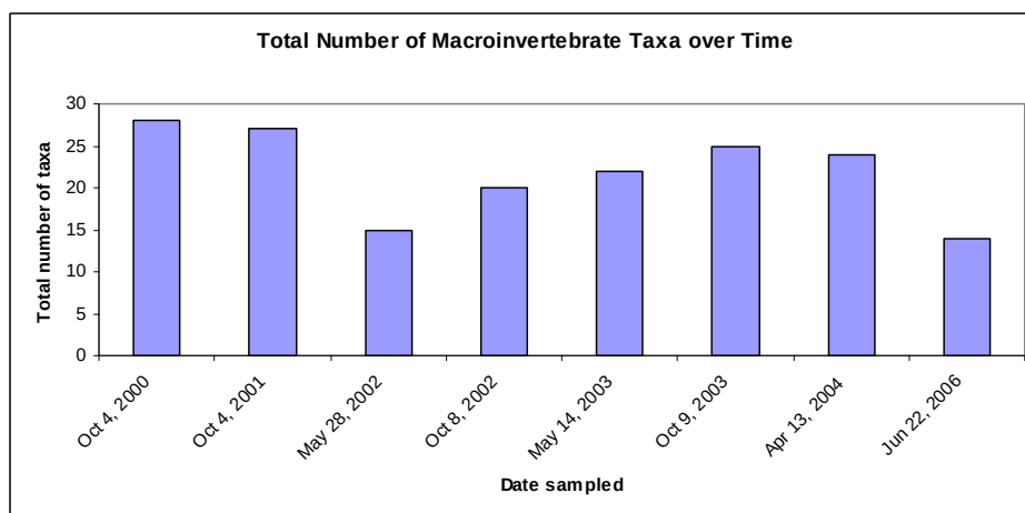
Figure 4: Total macroinvertebrate taxa for each sampling event.
