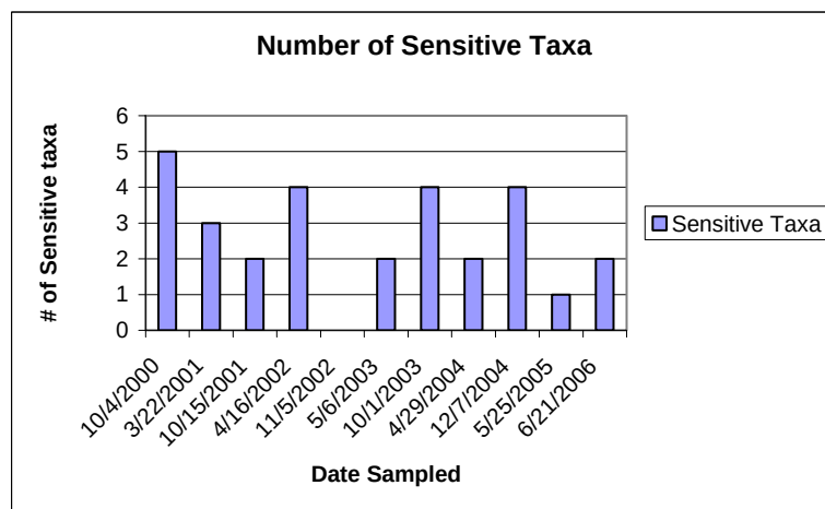
Figure 5: Table and chart showing number of sensitive taxa over the sampling period.
