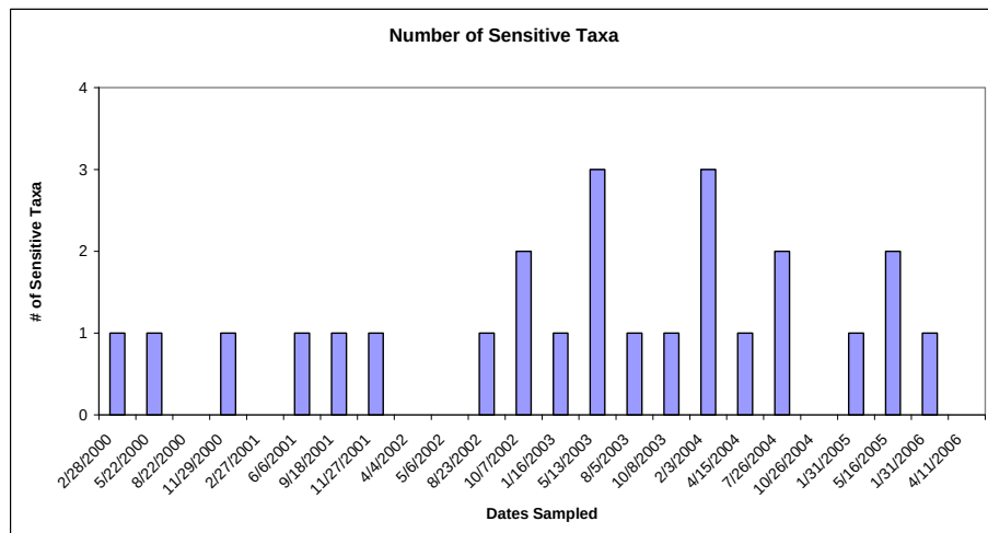
Figure 5: Table and Chart showing the number of sensitive taxa over the sampling period.
