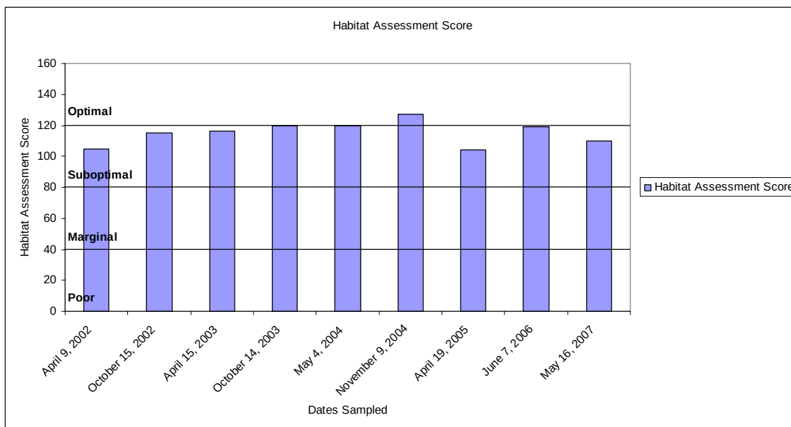
Figure 6: Habitat assessment scores over time.
