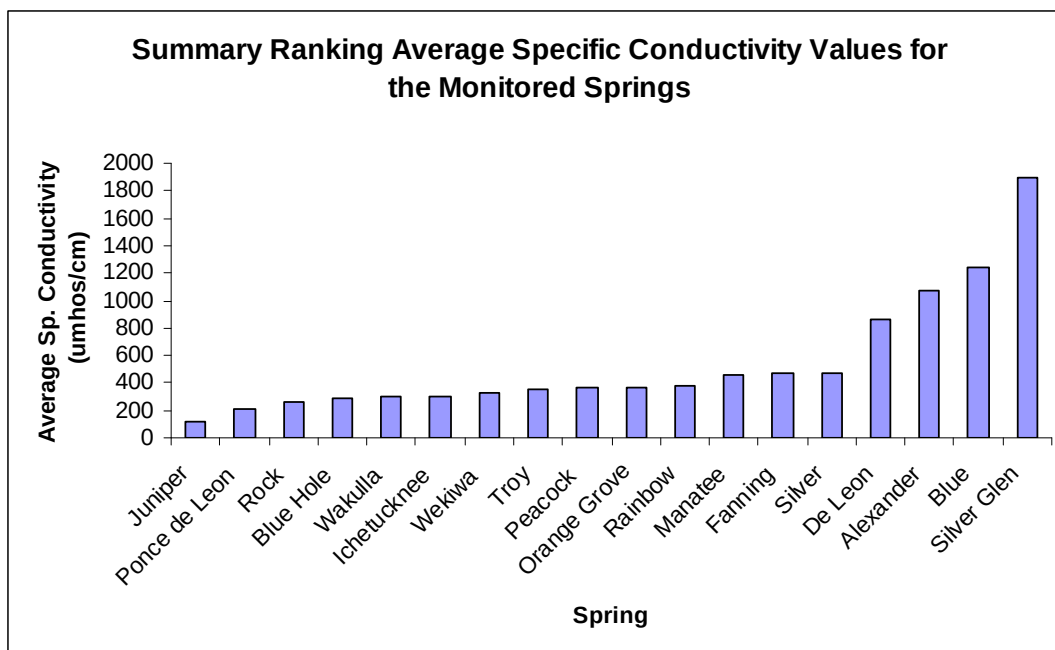
Figure 3. Summary of the average specific conductivity for each of the monitored springs, ranked in order from lowest to highest value.
