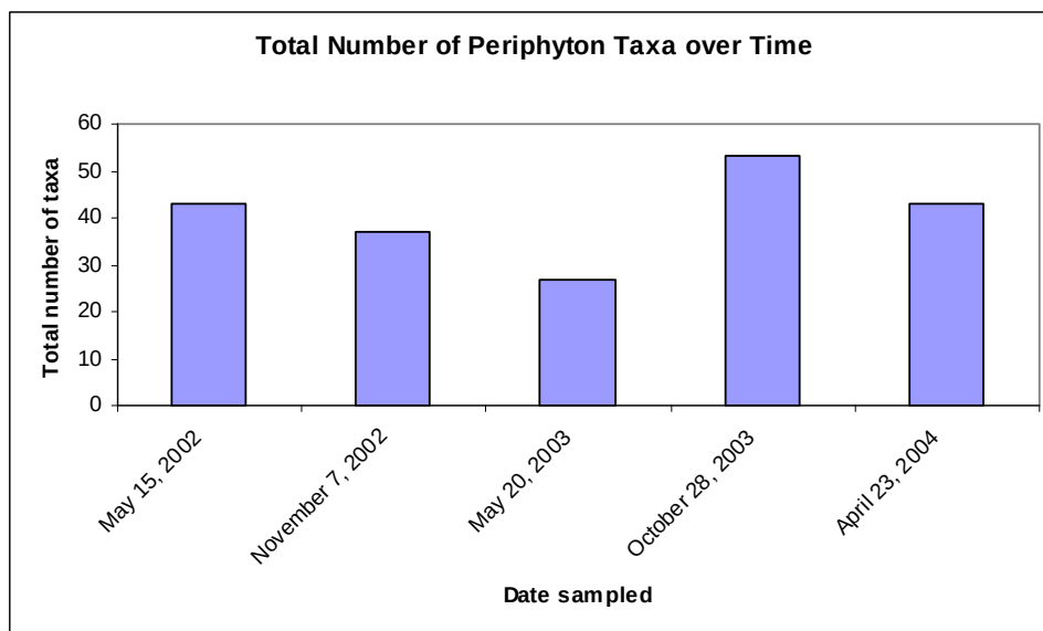
Figure 6: Total number of taxa for periphyton for each sampling event for Orange Grove Sink.
