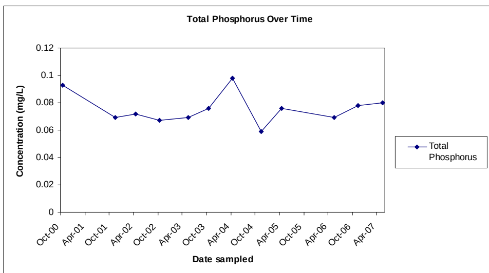
Figure 1: Total Phosphorus concentrations plotted over time.
