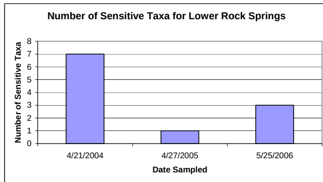
Figure 5: Table and chart showing sensitive taxa over the dates available for the sampling period at Upper and Lower Rock Spring.
