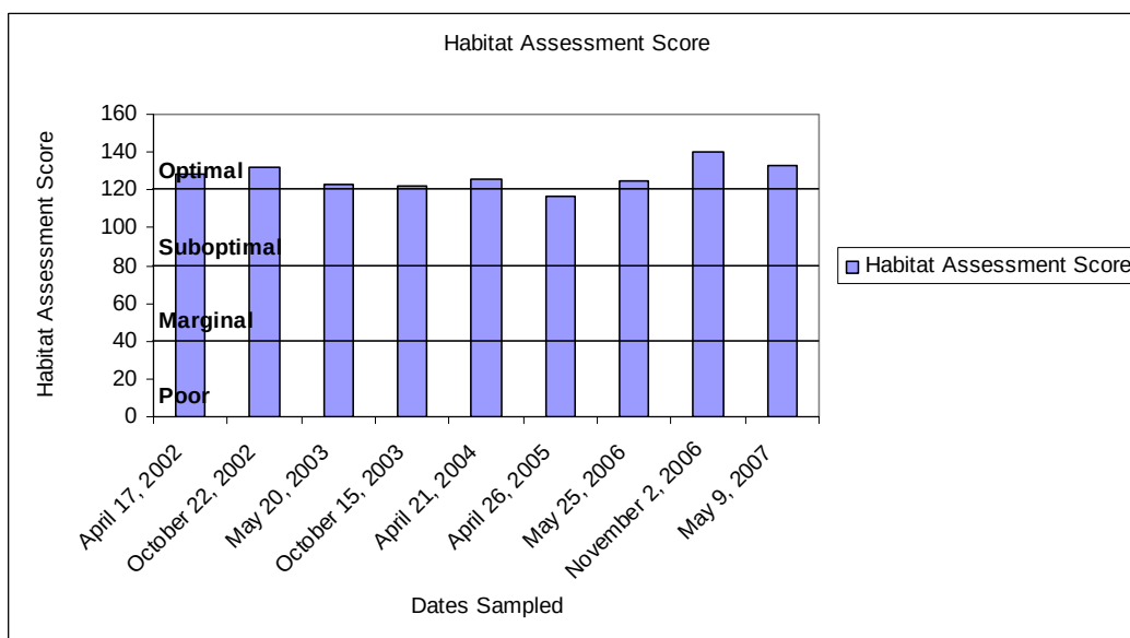
Figure 6: Habitat assessment scores over time.
