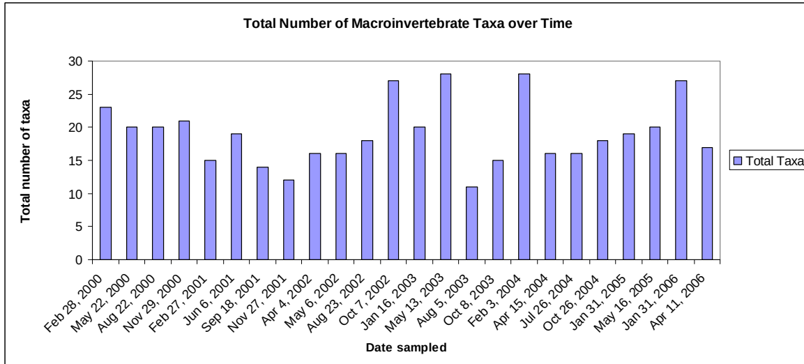
Figure 4: Total macroinvertebrate taxa for each sampling event.
