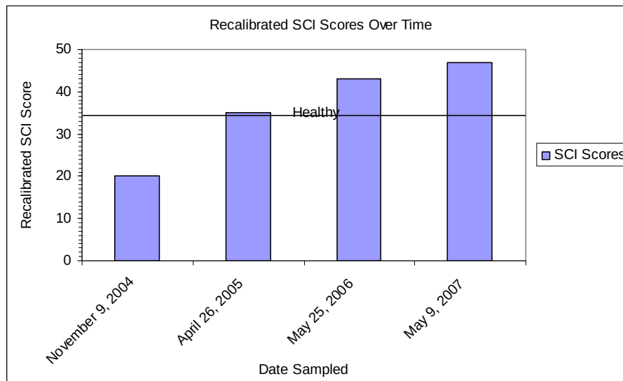
Figure 3: Recalibrated SCI scores with the impairment line drawn at 34.
