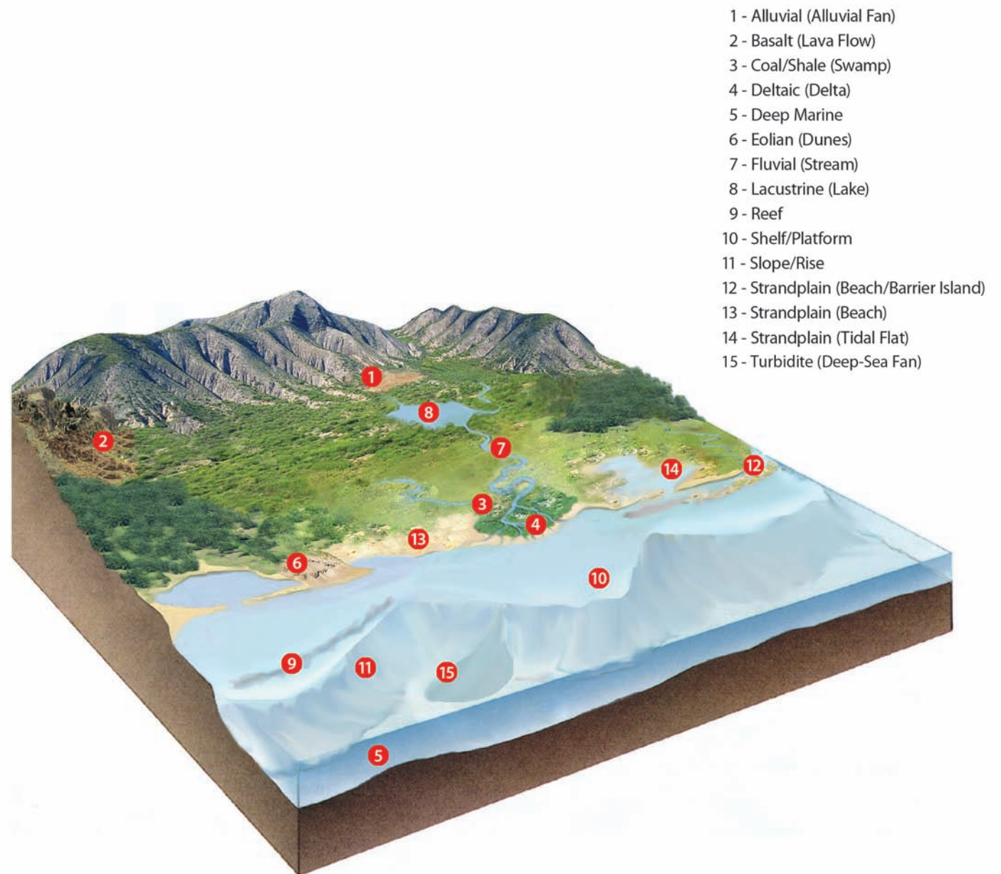
Types of depositional environments.
