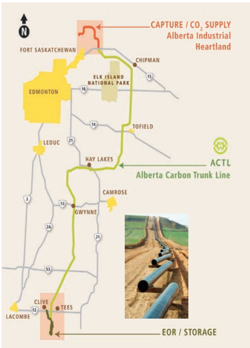
The Alberta Carbon Trunk Line, which will carry CO 2 captured at Alberta's industrial heartland to CO 2 -EOR and storage sites in central Alberta. (Courtesy: Enhance Energy)
