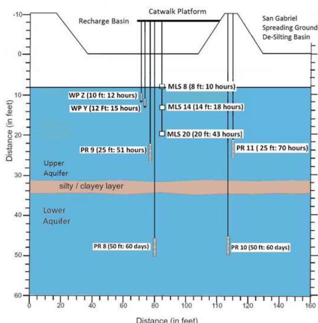
Instrumentation of groundwater recharge test basin associated with monitoring data provided in table below.
