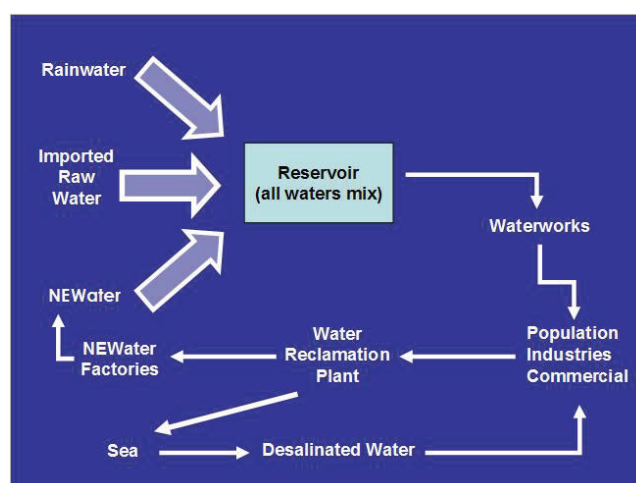
Schematic of the Singapore NEWater system. SOURCE: Ong and Seah, 2003.
