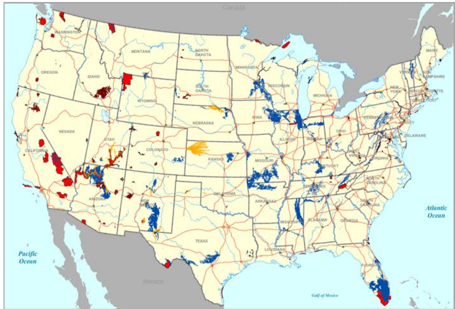
Preliminary data for ArcMap figure provided by Dr. Dan Doctor, US Geological Survey GIS map showing areas with potential karst and pseudokarst that underlie National Park Service properties (red). Blue areas: carbonate bedrock; yellow: evaporite bedrock; brown: volcanic bedrock.
