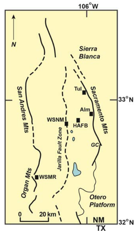
NCKRI map Simplified geologic map of the Tularosa Basin, flanking mountains, and approximate position of the Jarilla Fault. Basin-bounding surface faults = thick solid lines; subsurface faults = dashed lines; blue = Paleozoic bedrock outcrop; WSNM = White Sands National Monument headquarters; HAFB = Holloman Air Force Base; WSMR = White Sands Missile Range headquarters; Tul = Tularosa; Alm = Alamogordo (modified from McLean, 1975).
