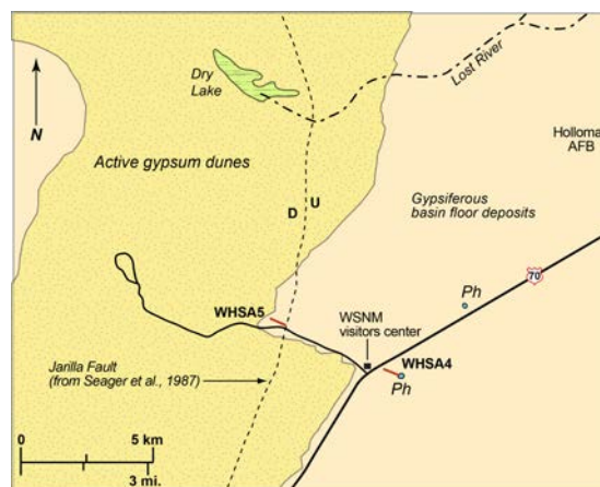
Detailed map of White Sands National Monument study area. Position of the Jarilla Fault is based on the geologic map by Seager et al. (1987) and gravity data from Healy et al. (1978). Ph = Permian Hueco Limestone outcrop. Short red lines show locations of ER surveys.
