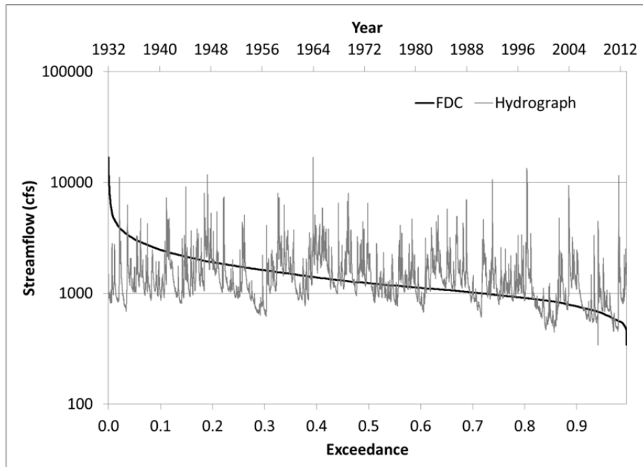
Figure 1. Comparison of the period-of-record hydrograph of the Lower Santa Fe River near Fort White with its period-of-record flow duration curve.
