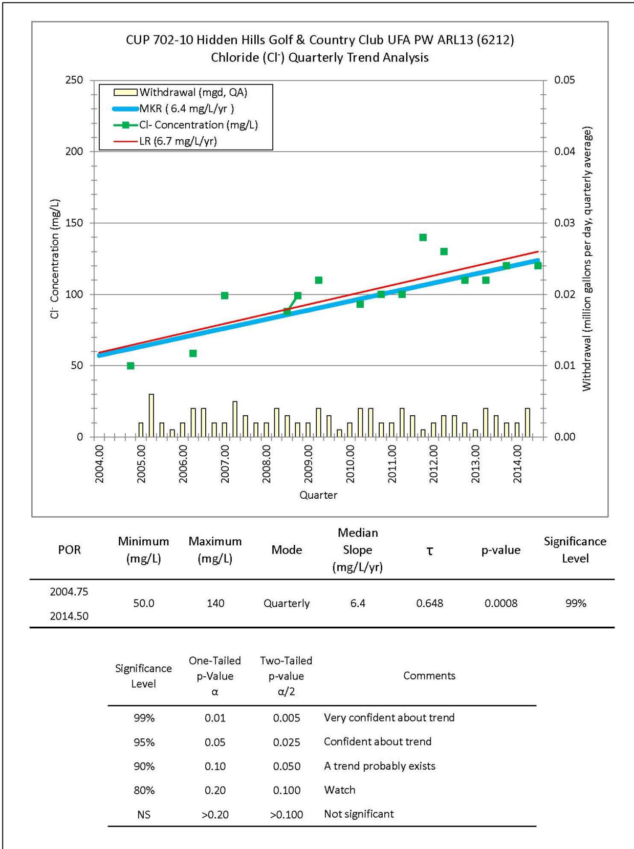
Figure D6a: Time-Series Chloride Trend in a Hidden Hills Golf and Country Club Well
