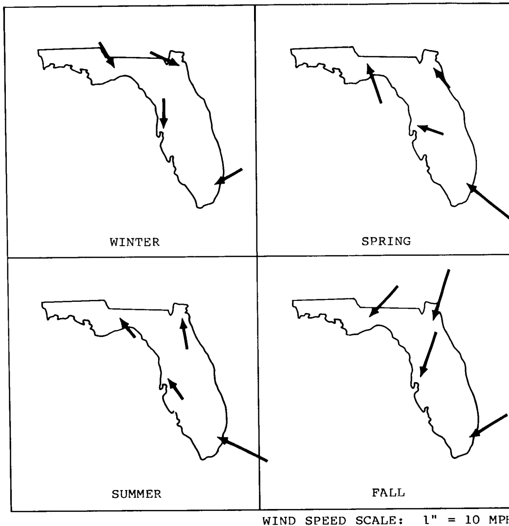
Figure 22. Resultant mid-season surface winds at four locations: Jacksonville, Miami, Tallahassee, Tampa (Gutfreund 1978). Period of record based on hourly observations, 1951-60.
