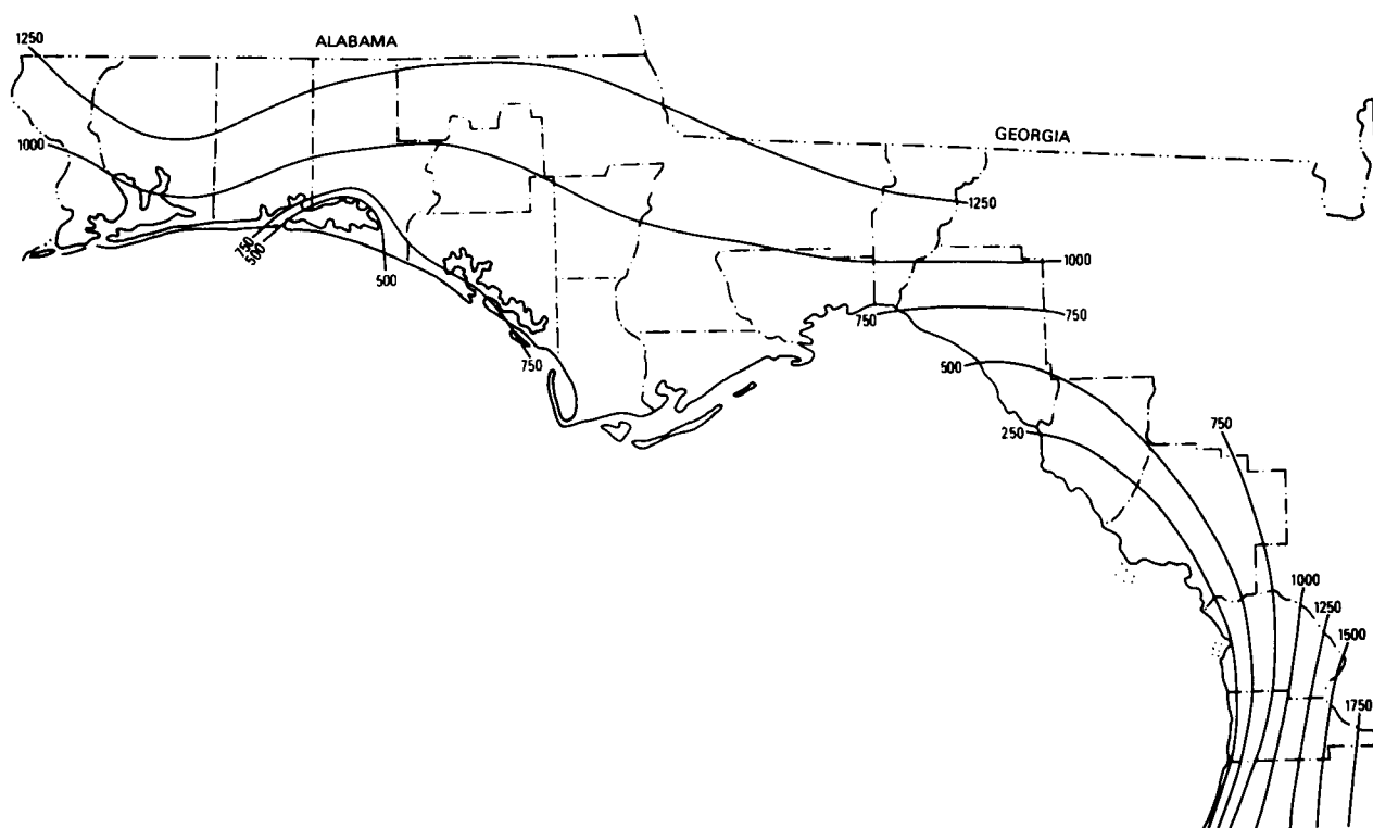
Figure 6. Depth to base of potable water in the Floridan aquifer; contours are in feet below mean sea level (adapted from Franks 1982).
