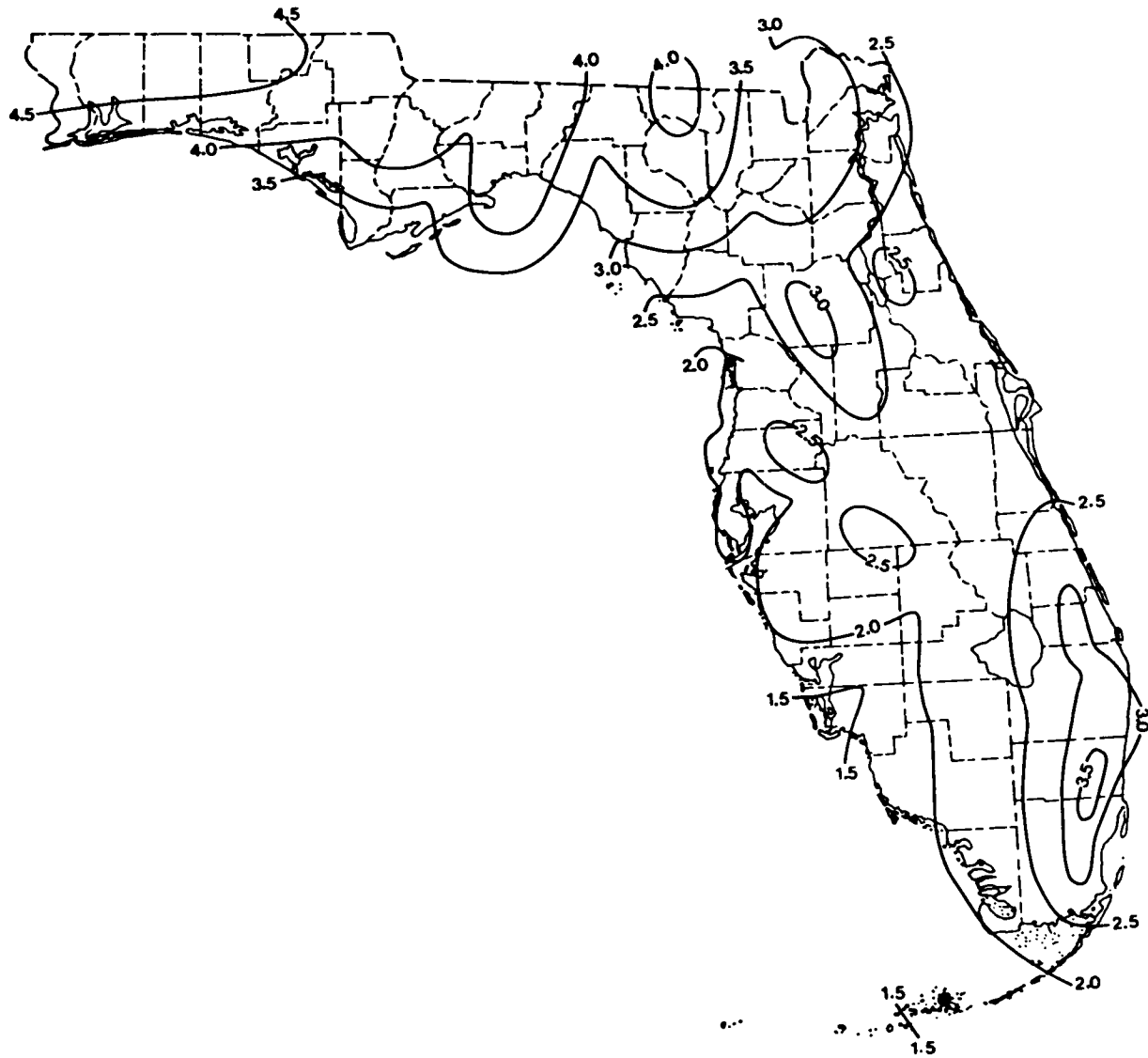
Figure 20. Florida map with isohyets (contour lines showing equal amounts of precipitation) for normal mean rainfall, April 1951-80 (National Climatic Center 1982).
