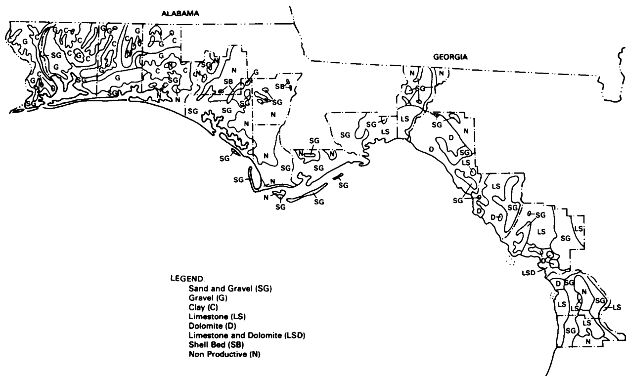
Figure 3. Surface mineral resources of northwest Florida (after Knapp 1978a, 1978b, 1980; Schmidt 1978a, 1978b, 1979; Deuerling 1981).
