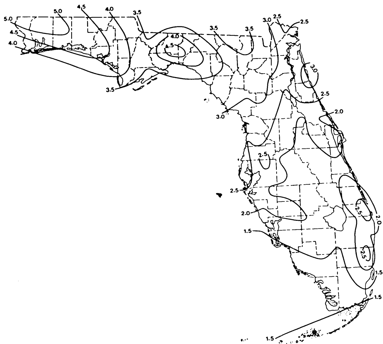
Figure 16. Florida map with isohyets (contour lines showing equal amounts of precipitation) for normal mean rainfall, December 1951-80 (National Climatic Center 1982).
