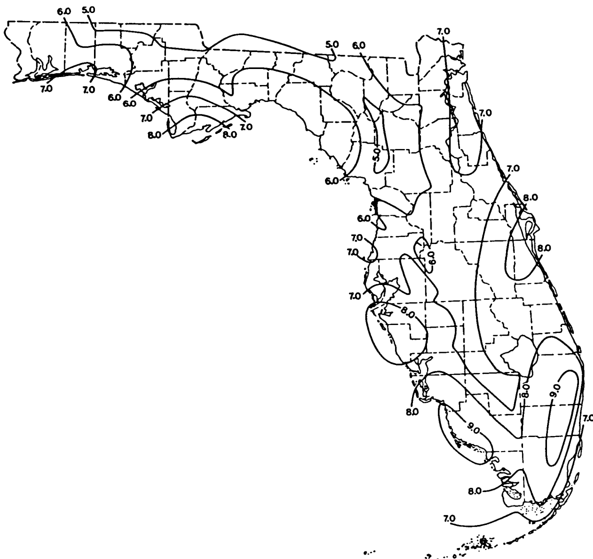
Figure 13. Florida map with isohyets (contour lines showing equal amounts of precipitation) for normal mean rainfall, September 1951-80 (National Climatic Center 1982).
