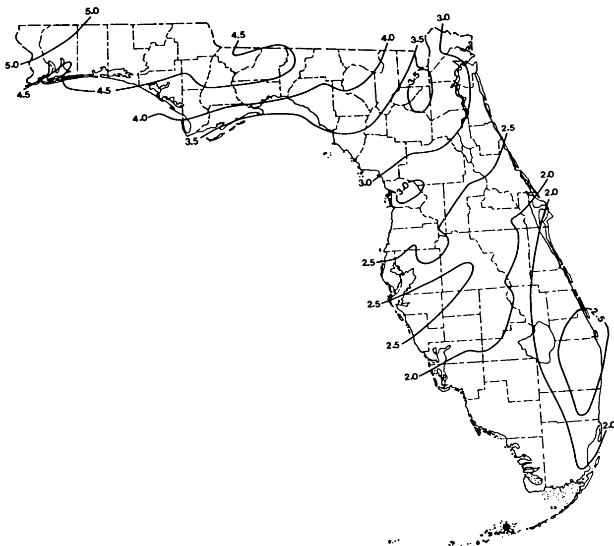
Figure 17. Florida map with isohyets (contour lines showing equal amounts of precipitation) for normal mean rainfall, January 1951-80 (National Climatic Center 1982).
