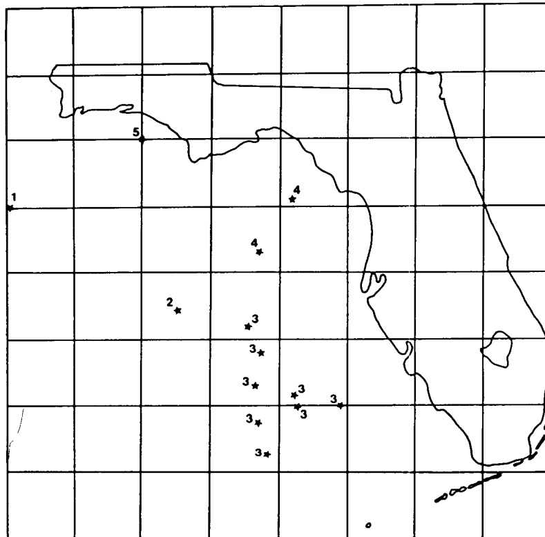
Figure 24. Location map of sites in the eastern Gulf of Mexico where data on currents have been collected. (New England Coastal Engineers 1981). Numbers refer to the following references:
