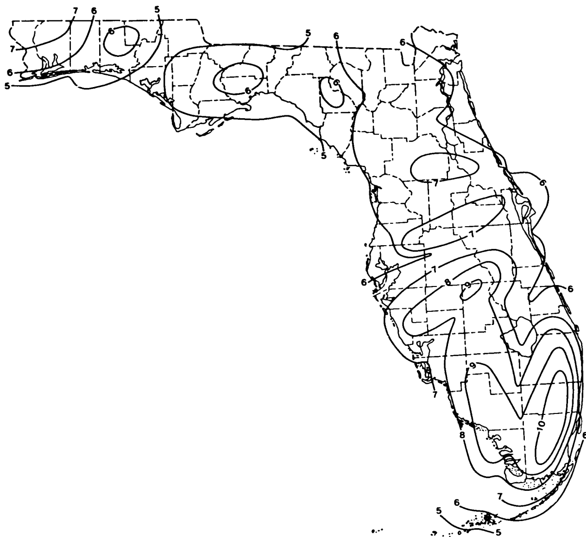
Figure 10. Florida map with isohyets (contour lines showing equal amounts of precipitation) for normal mean rainfall, June 1951-80). (National Climatic Center 1982).
