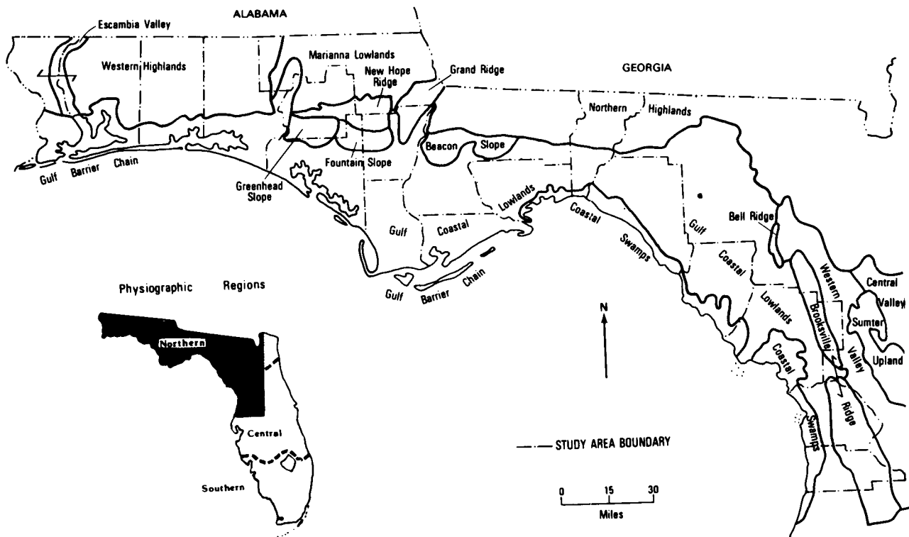
Figure 1. Physiographic provinces of northwest Florida (after Scott et al. 1980).
