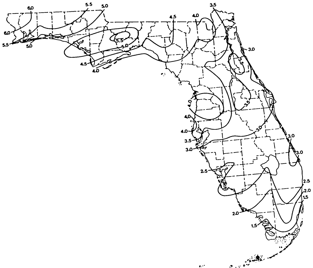
Figure 19. Florida map with isohyets (contour lines showing equal amounts of precipitation) for normal mean rainfall, March 1951-80 (National Climatic Center 1982).
