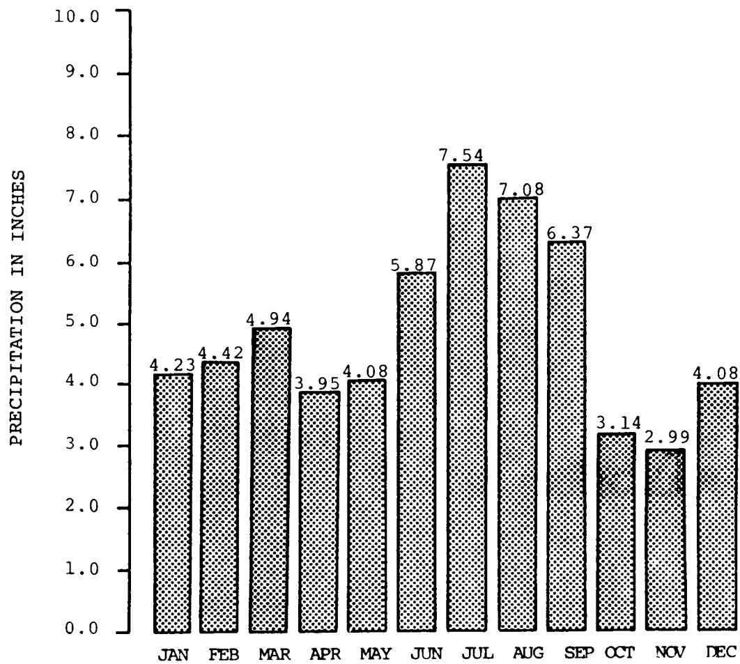
Figure 8. Normal mean monthly precipitation for northwest Florida, 1951-80; represents areal mean of monthly precipitation for study area (National Climatic Center 1982).
