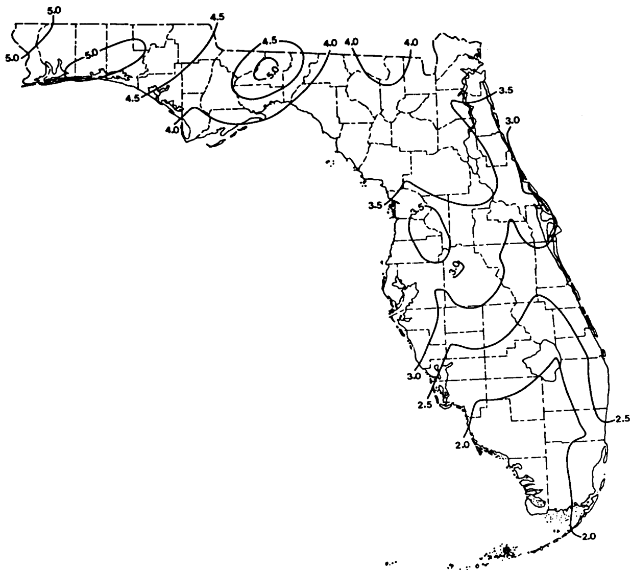
Figure 18. Florida map with isohyets (contour lines showing equal amounts of precipitation) for normal mean rainfall, February 1951-80 (National Climatic Center 1982).
