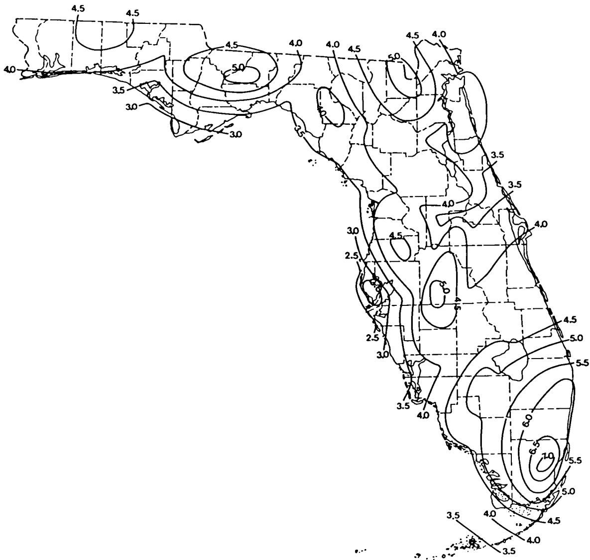
Figure 9. Florida map with isohyets (contour lines showing equal amounts of precipitation) for normal mean rainfall, May 1951-80 (National Climatic Center 1982).
