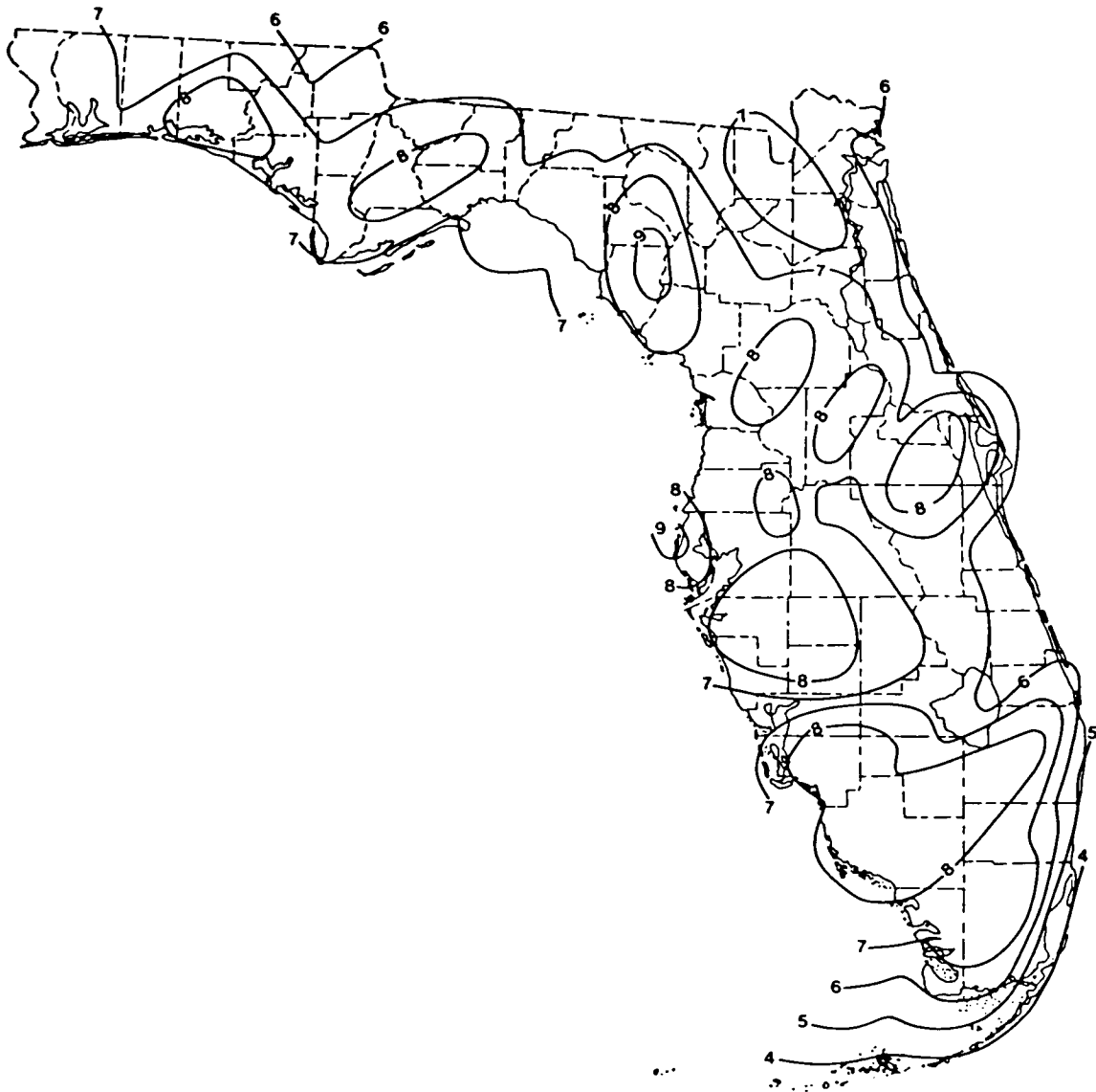
Figure 11. Florida map with isohyets (contour lines showing equal amounts of precipitation) for normal mean rainfall, July 1951-80 (National Climatic Center 1982).
