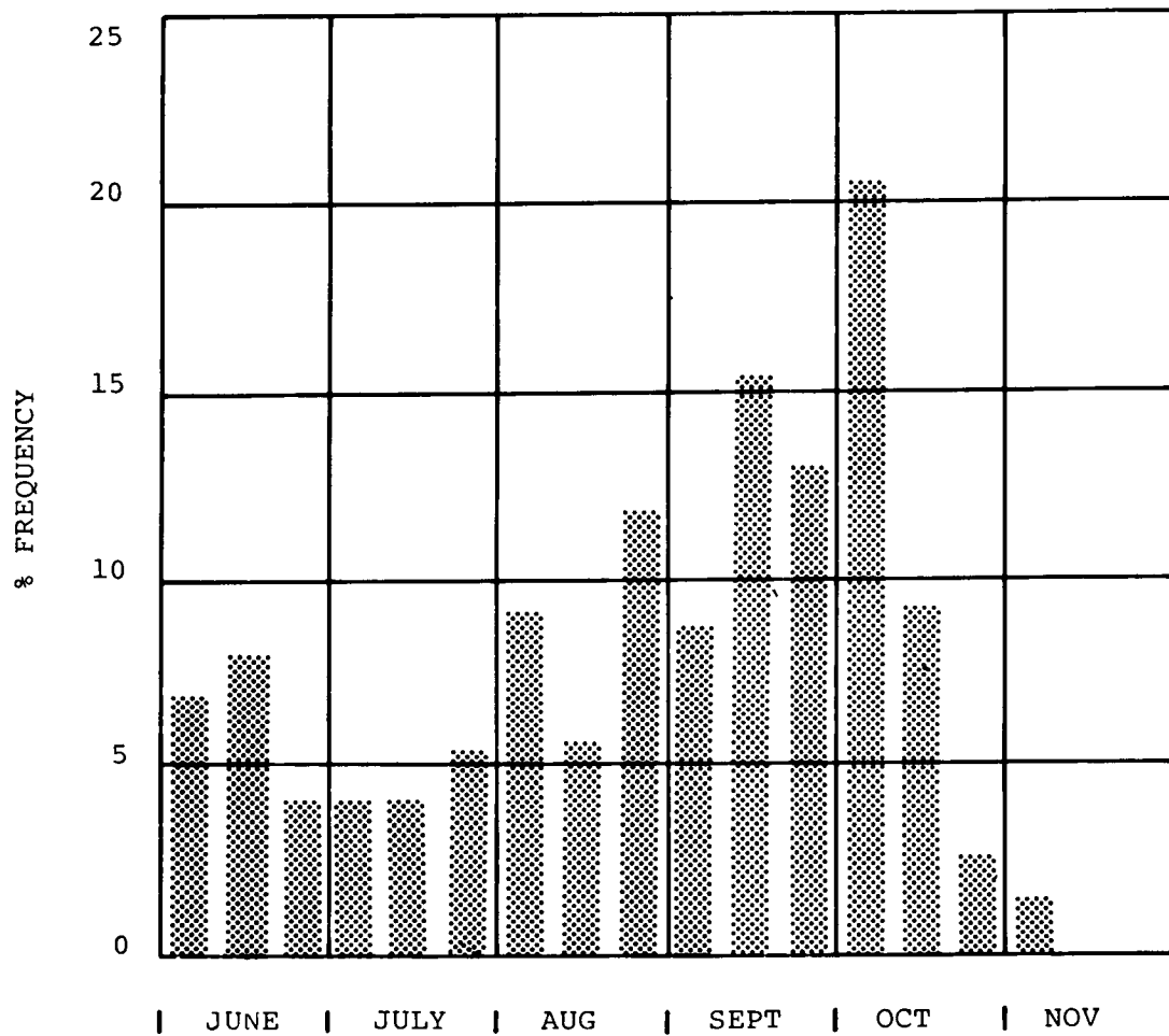
Figure 28. Frequency distribution of hurricanes by time of year in northwest Florida from 1871 to 1980 (Neumann et al. 1981).
