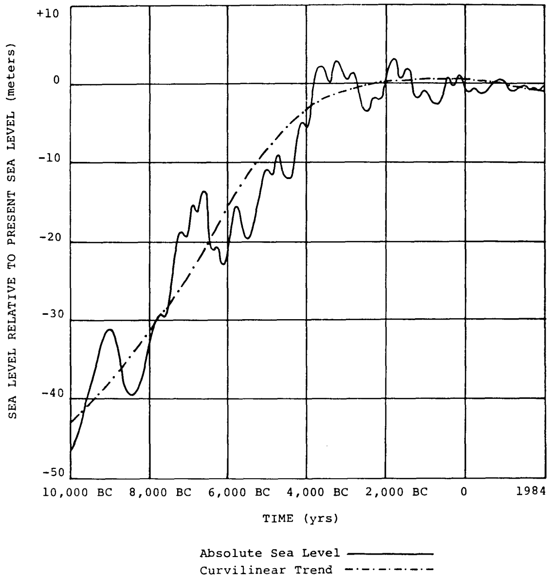
Figure 2. Sea level relative to present sea level for the past 12,000 years (Bruun 1962).
