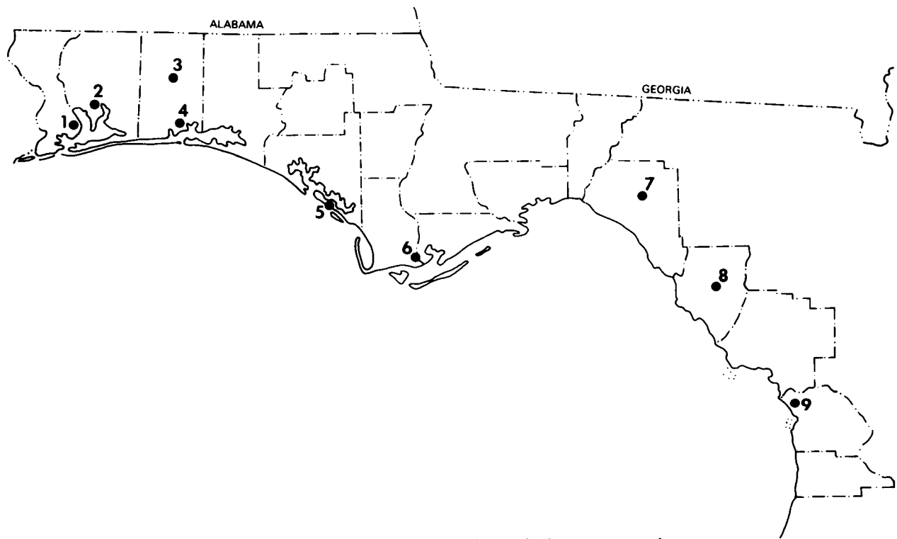
Figure 23. Northwest Florida wind rose stations.
