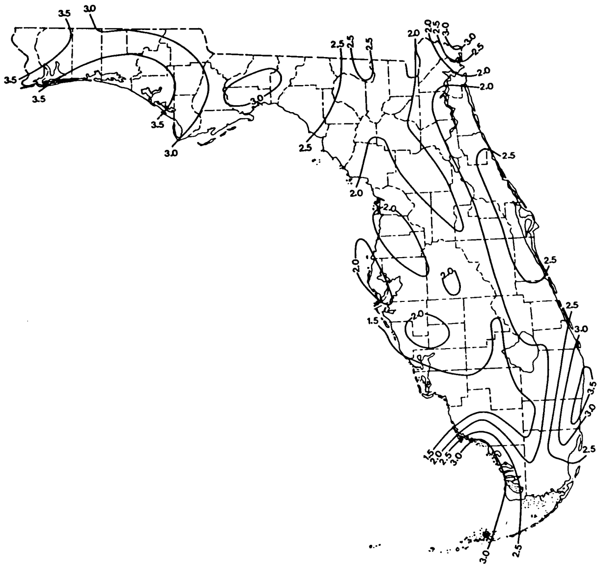
Figure 15. Florida map with isohyets (contour lines showing equal amounts of precipitation) for normal mean rainfall, November 1951-80 (National Climatic Center 1982).
