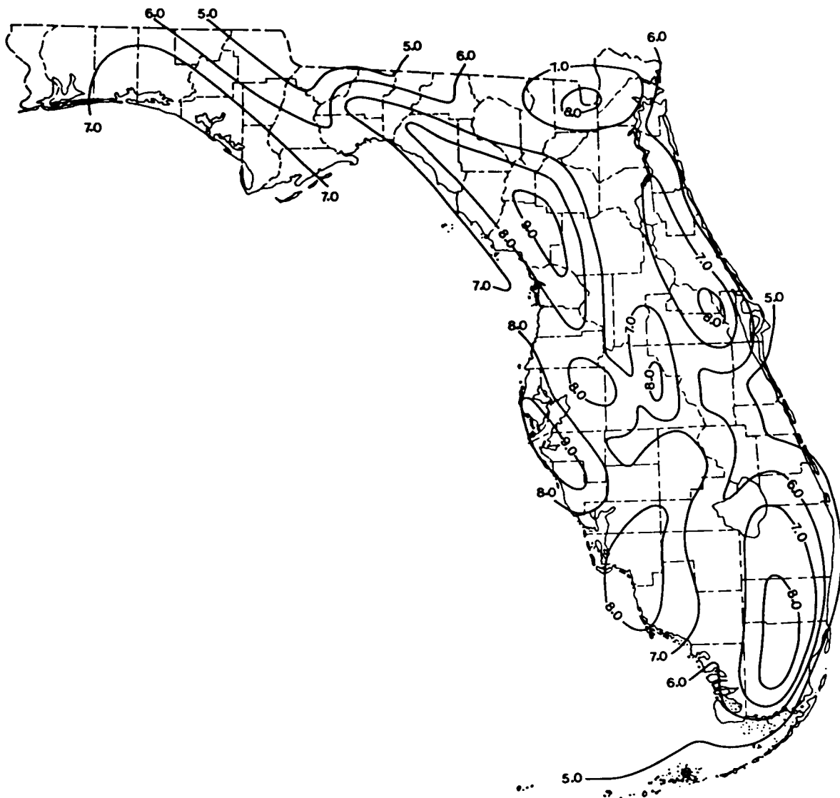
Figure 12. Florida map with isohyets (contour lines showing equal amounts of precipitation) for normal mean rainfall, August 1951-80 (National Climatic Center 1982).
