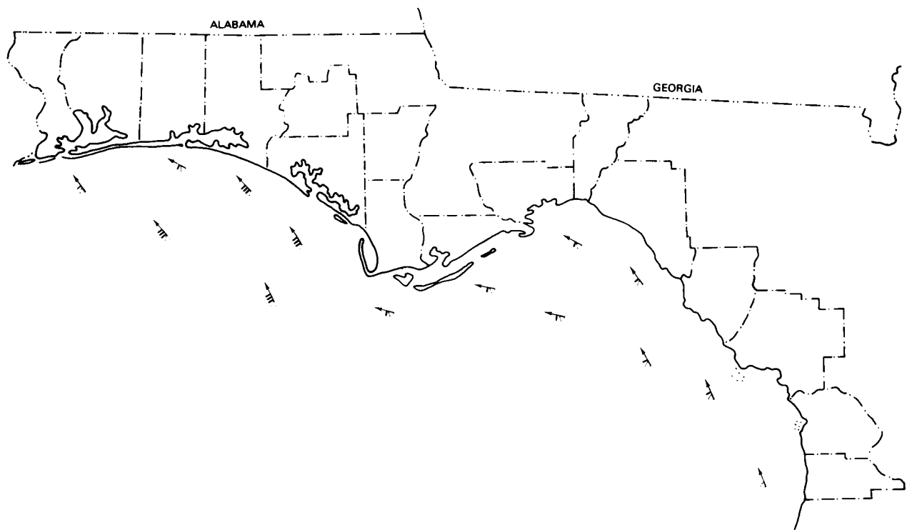
Figure 25. Mean spring surface currents off northwest Florida; number of feathers on current arrow equals velocity in cm/s; open triangle equals 50 cm/s (adapted from New England Coastal Engineers 1982).
