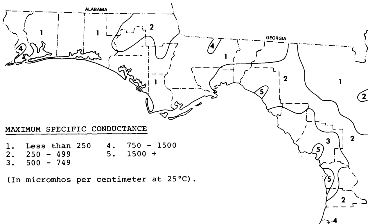
Figure 30. Specific conductance of water in northwest Florida streams and canals (Slack and Kaufman 1973).
