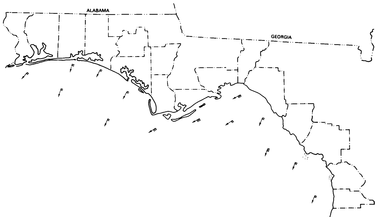
Figure 27. Mean fall and winter surface currents off northwest Florida; number of feathers on current arrow equals velocity in cm/s; open triangle equals 50 cm/s (adapted from New England Coastal Engineers 1982).
