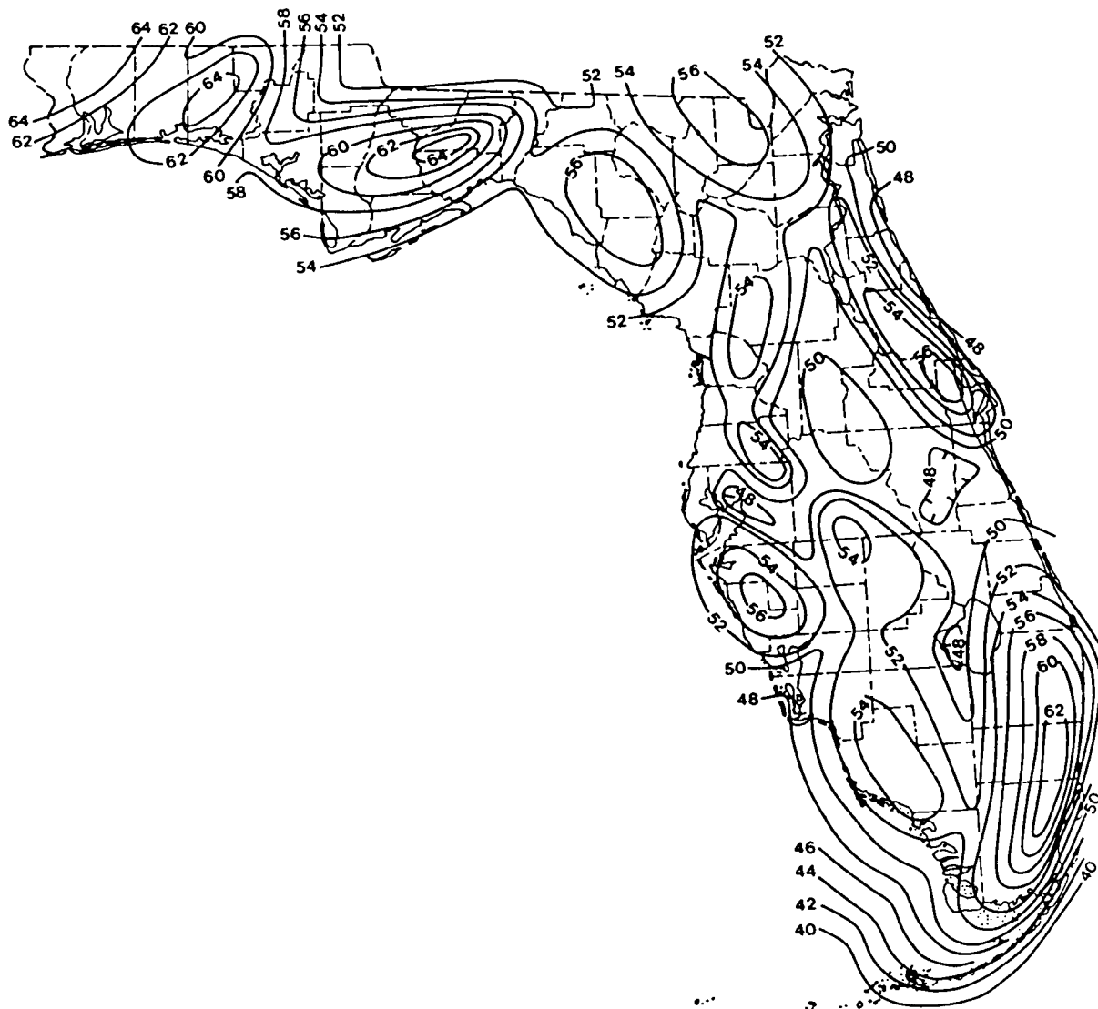
Figure 21. Florida map with isohyets (contour lines showing equal amounts of precipitation) for annual normal mean rainfall, 1951-80 (National Climatic Center 1982).
