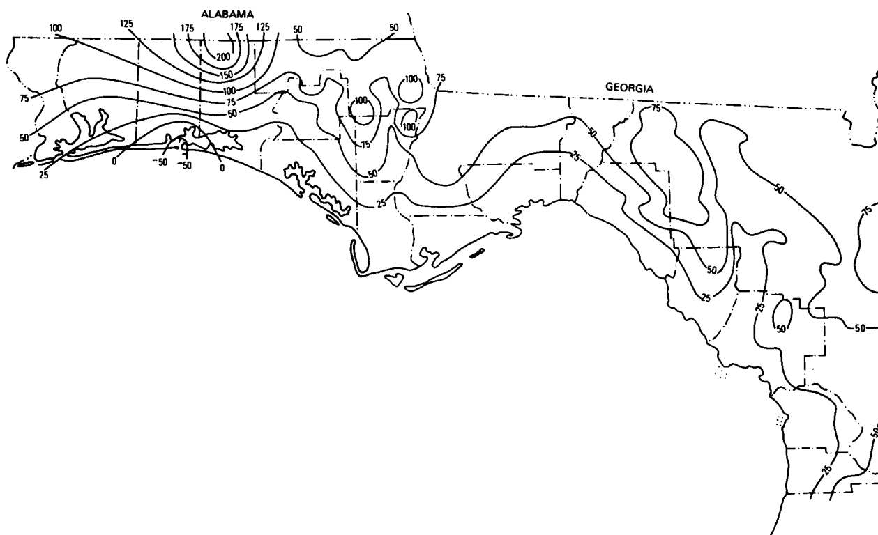
Figure 7. Generalized potentiometric surface of Floridan aquifer across northwest Florida during May 1980 and May 1981; contours are in feet above mean sea level (adapted from Franks 1982).
