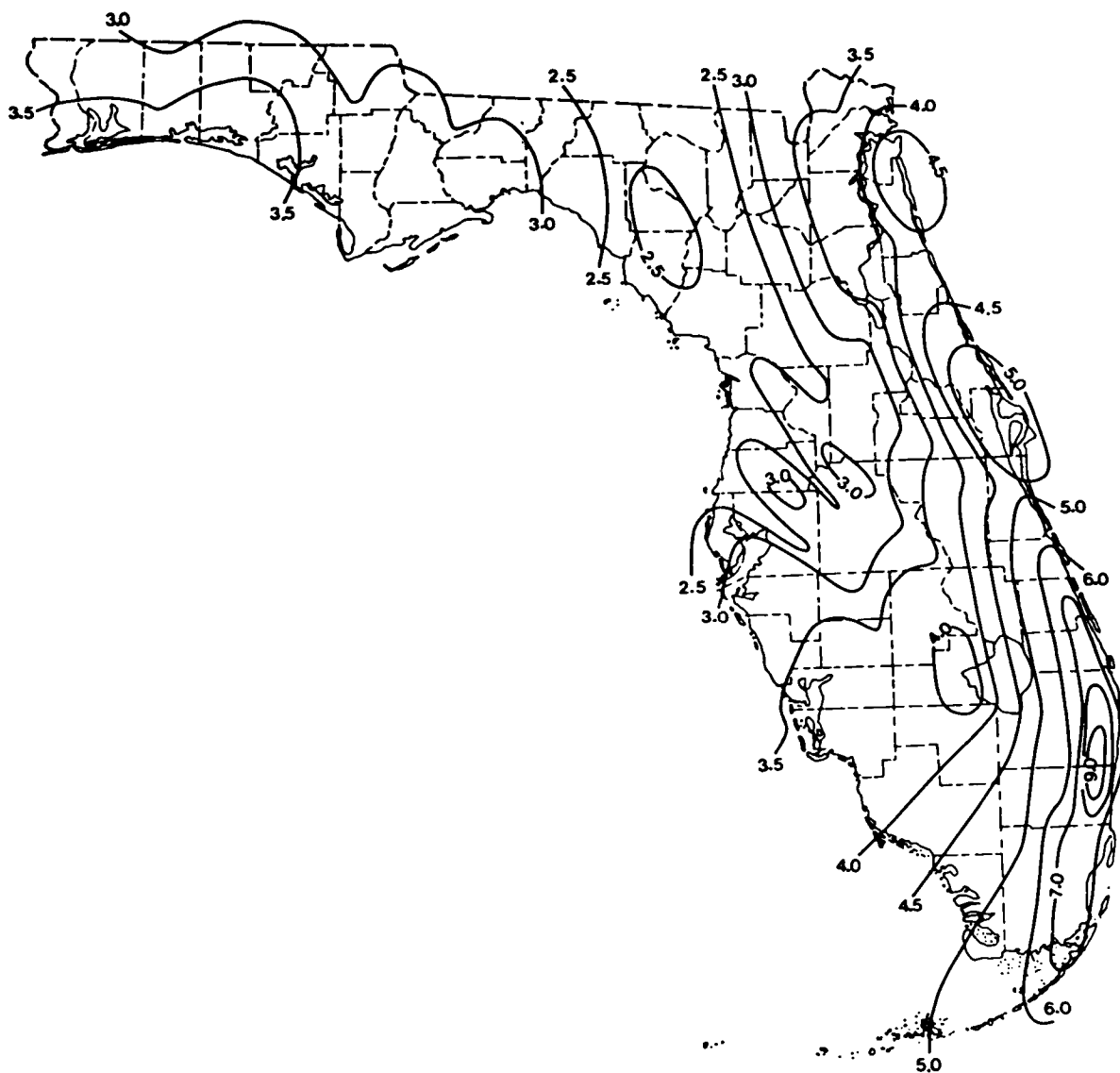
Figure 14. Florida map with isohyets (contour lines showing equal amounts of precipitation) for normal mean rainfall, October 1951-80 (National Climatic Center 1982).
