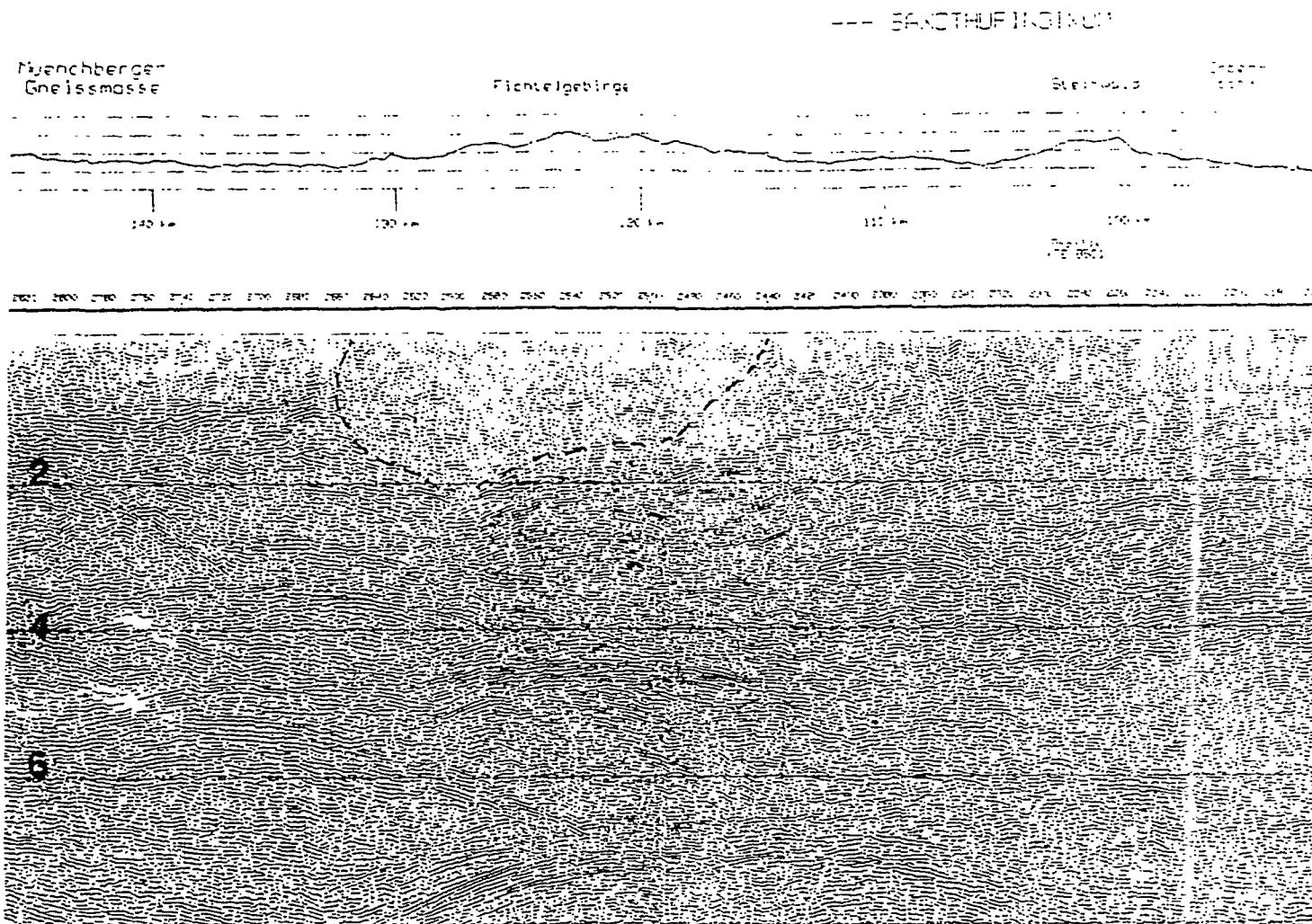
FIGURE 1. Seismic section taken from the Dekorp Atlas, Dekorp 85, line 4N (Meissner and Bortfeld, 1990) that shows the Fichtelgebirge granitic body as a transparent seismic zone. Vertical scale is shown each two seconds, two way travel time, non migrated profile, that is roughly 6 km.
