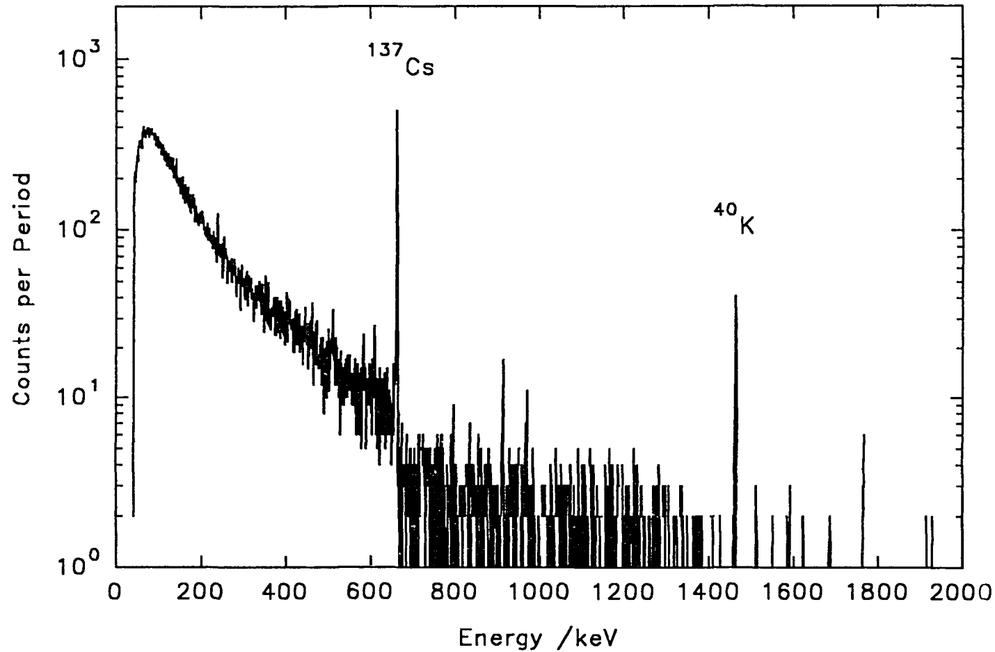
FIG. 5.b Aerial gamma ray spectra at Kirkconnel Merse, showing natural sources and Sellafield derived ^{137}\text{Cs} 50% relative efficiency GMX. Note the enhanced forward scattering and higher ^{137}\text{Cs}/^{134}\text{Cs} compared with Fig. 4.
