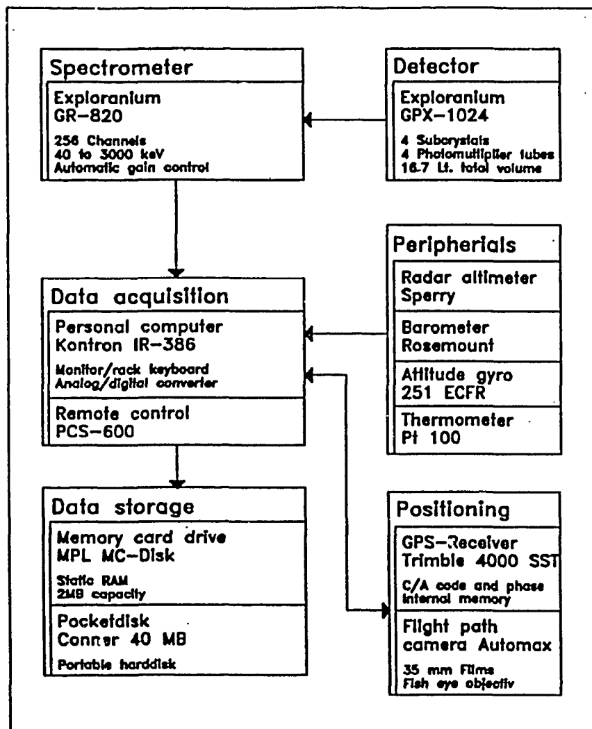
FIG. 1. Block diagram of the measuring system.
