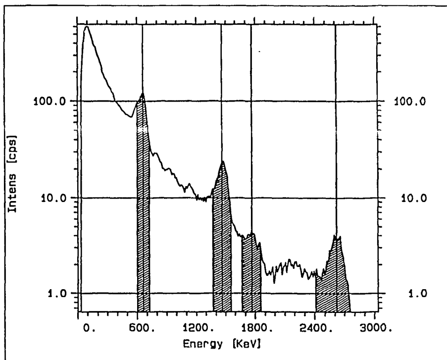
FIG. 1. Spectrum of the \gamma -radiation in the Magadino plain (TI) as measured in July 1991.
