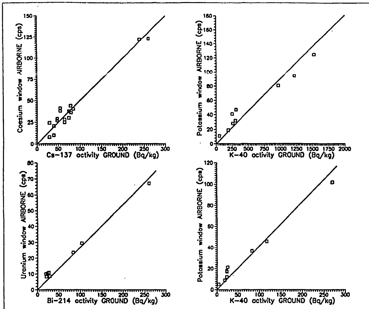
FIG. 4. Experimentally determined detector sensitivities.
