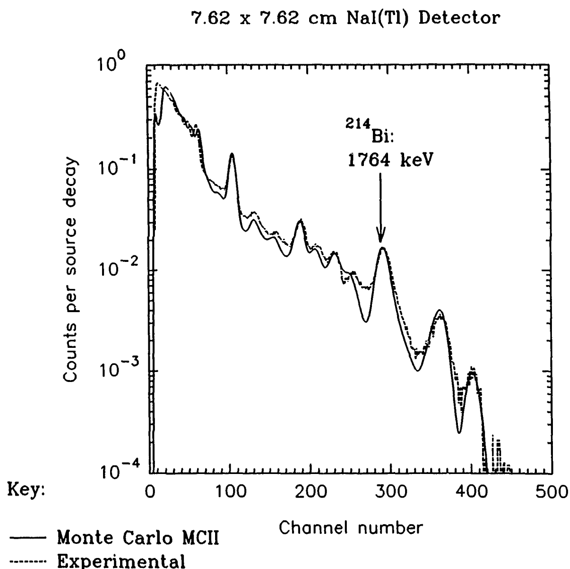
Figure 6. Comparison of Monte-Carlo and experimental spectra above a Uranium calibration Pad for a field based detector.
