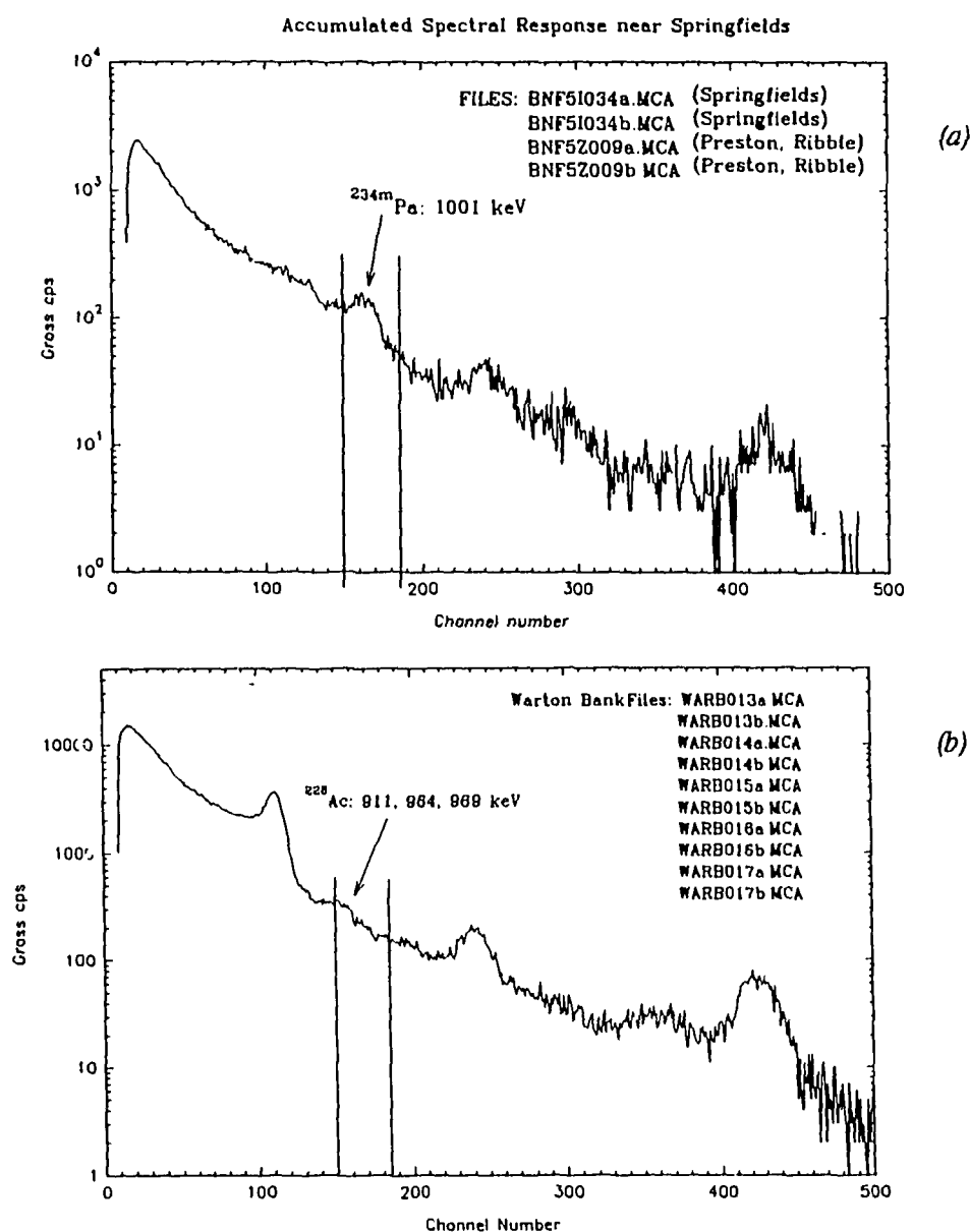
FIG. 8. NaI spectra recorded (a) close to Springfields, showing ^{234\text{m}}\text{Pa} , and (b) at Warton Bank showing ^{137}\text{Cs} and ^{228}\text{Ac} .
