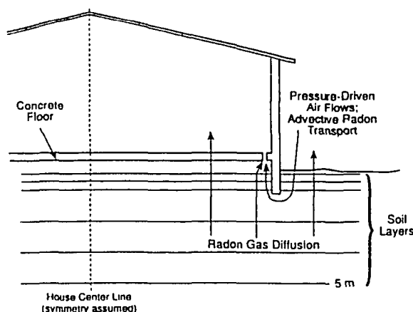
Fig. 1. Diffusive and advective radon entry into a reference house from the underlying soil profile.
