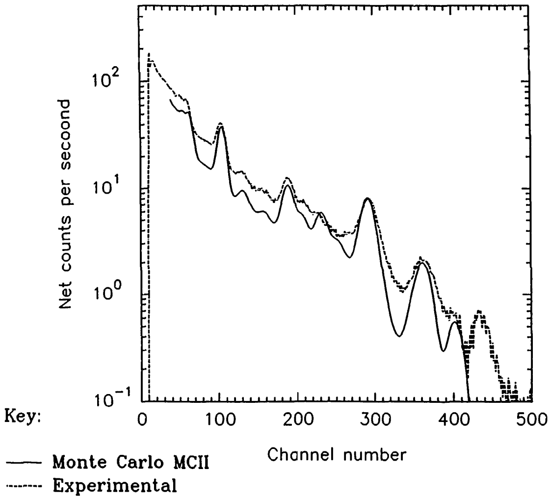
Figure 7. Comparison of Monte-Carlo and experimental spectra above a Uranium calibration Pad for an aerial survey detector.
