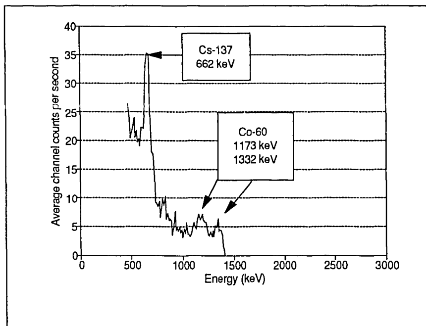
FIG. 5. The same spectrum showing the ^{60}\text{Co} peaks at 1173 and 1332 keV, after removal of the natural gamma ray components.
