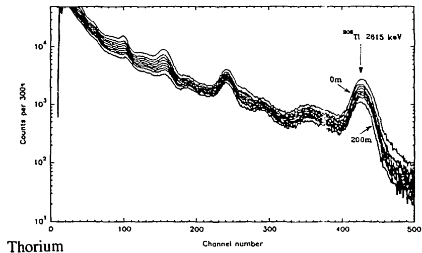
Figure 4. Diagram illustrating the use of perspex absorbers to simulate the variation of spectral response of an aerial survey detector.
