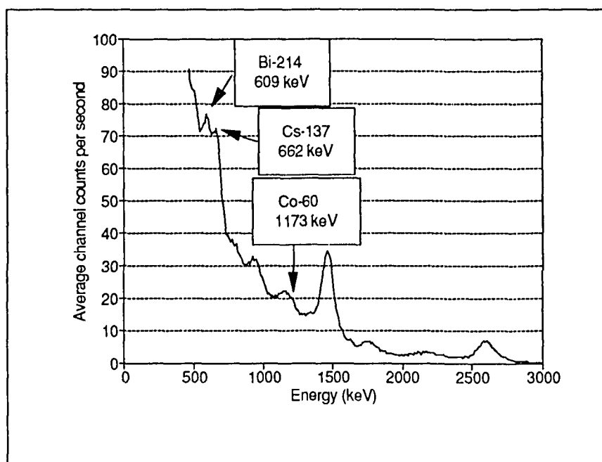
FIG. 4. An average spectrum measured over an area contaminated by ^{60}\text{Co} .
