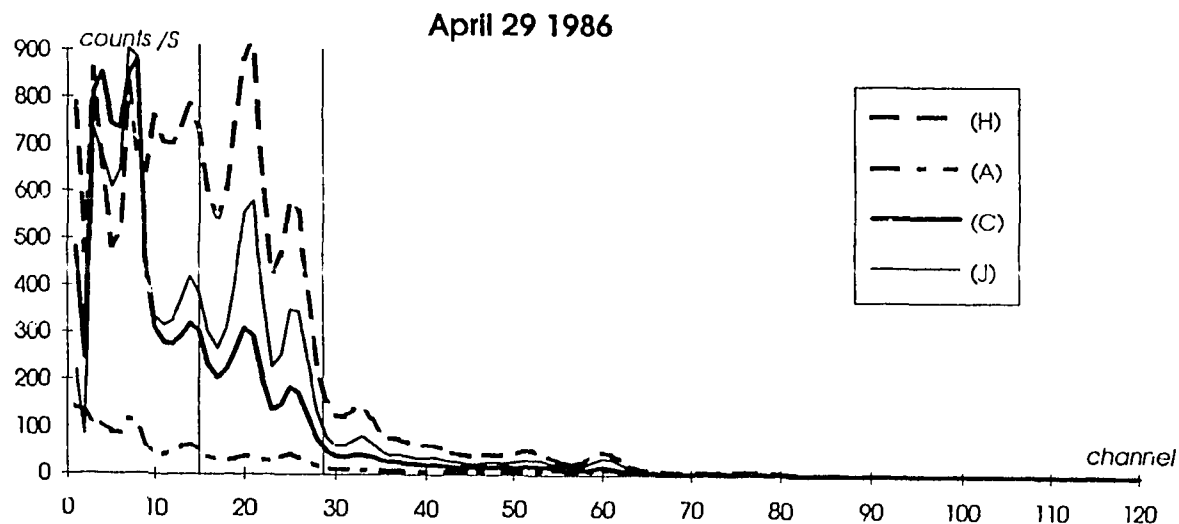
FIG. 3. Four measured spectra from the flight thorough the radiating cloud from Chernobyl accident. The locations (A, C, H and J) respect to the Cesium window count rate profile are show in Fig. 2.
