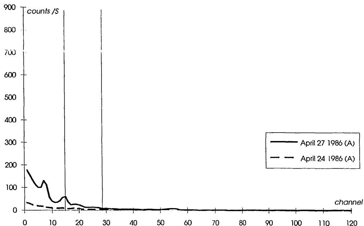
FIG. 1. Two background spectra measured above sea at the altitude of 60 meters. The Cesium window used in Fig. 2 is also plotted.
