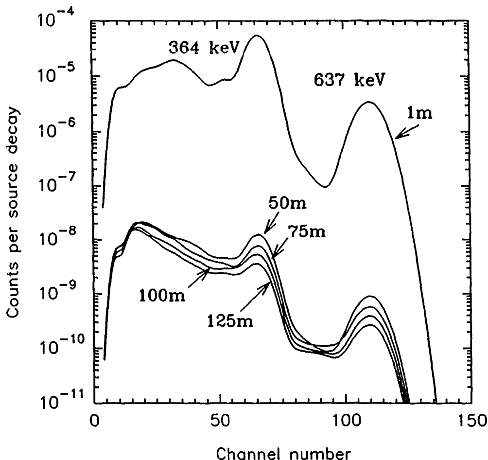
Figure 8. Diagram showing the predicted aerial survey detector response using Monte-Carlo methods of an extended ^{131}\text{I} source.
