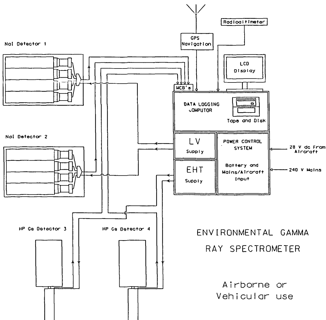
FIG. 1. Schematic diagram of an SURRC airborne gamma ray spectrometer. The system can be configured for one to four detectors, comprising NaI and/or Germanium detectors.
