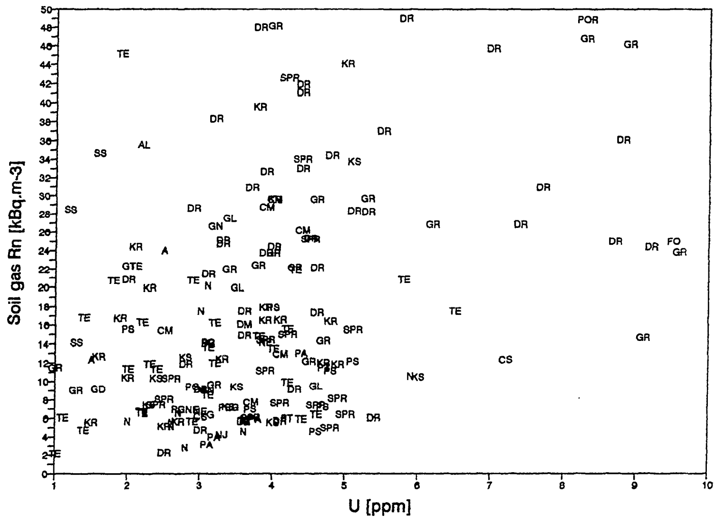
FIG. 3. The Rn-U relationship in the usual ranges of values in the rock types of the Bohemian Massif. Zoomed from Fig. 2 (major codes: DR, GR, GD - granitic rocks, KR - crystalline rocks, TE - river terraces, SPR loess, KS - Cretaceous sediments, GL - glacifluvial sediments).
