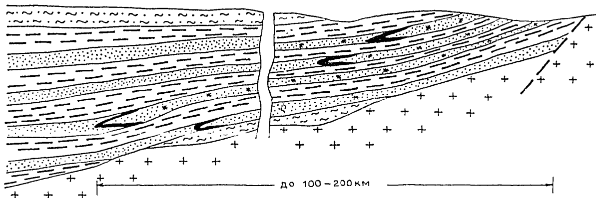
FIG. 3a. Ore-bearing structures of sandstone type deposits (schematic): Large semi-open synclises, sub-type a.
