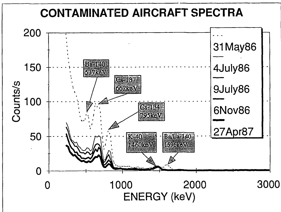
FIG. 4. Background spectra after the Chernobyl accident. Showing the aircraft contamination.
