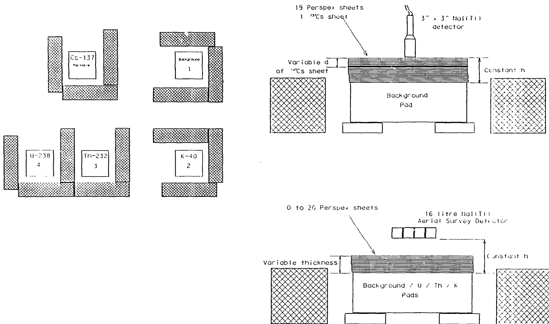
Figure 3. Diagram illustrating the SURRC gamma ray calibration facility.
