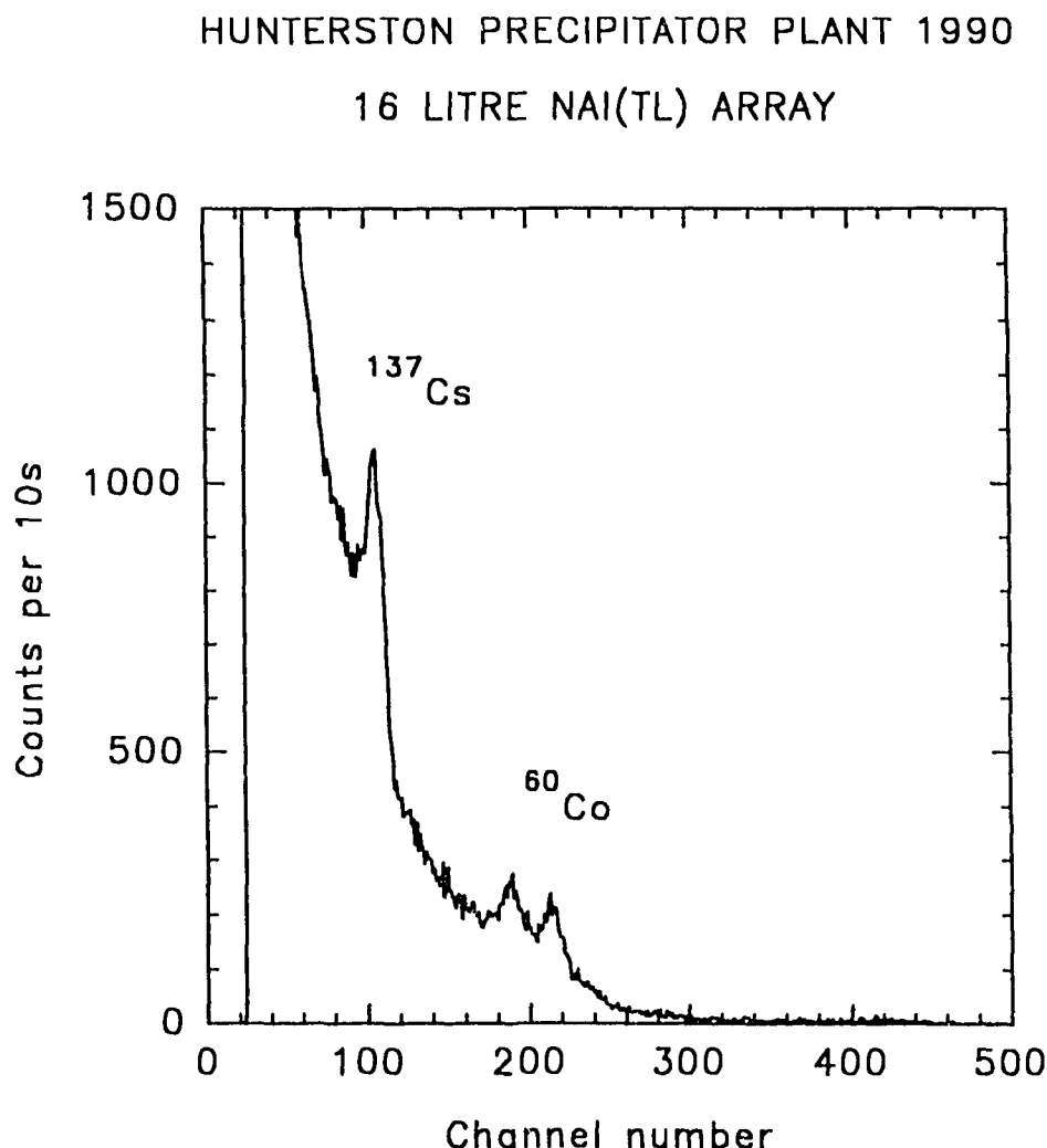
FIG. 7. ^{137}\text{Cs} and ^{60}\text{Co} signals recorded close to the Hunterston "A" station in 1990.
