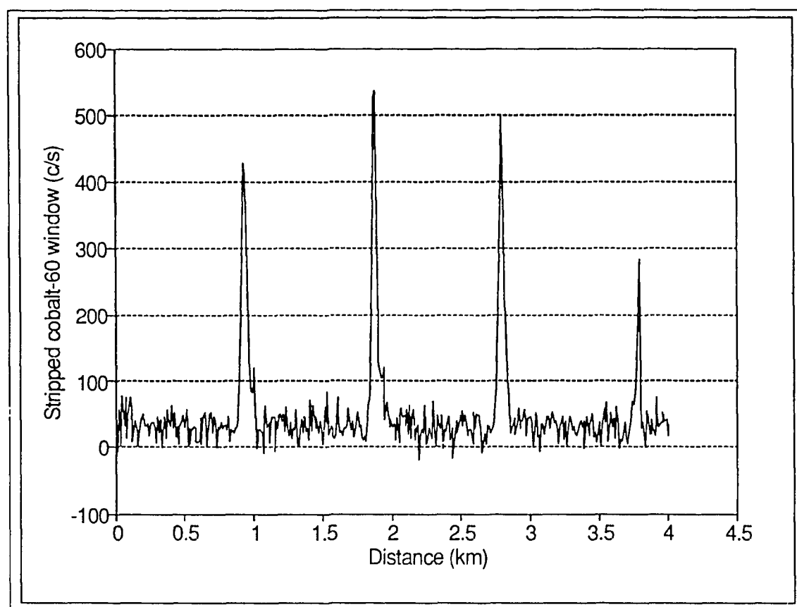
FIG. 3. A profile of a single window, centered around the ^{60}\text{Co} peak at 1173 keV with the natural gamma ray components removed. The profile corresponds to four flights over a contaminated area.
