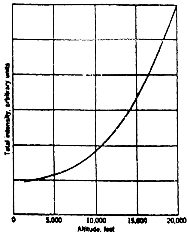
FIG. 3. Total cosmic-ray intensity, plotted as a function of barometric altitude above sea level.
