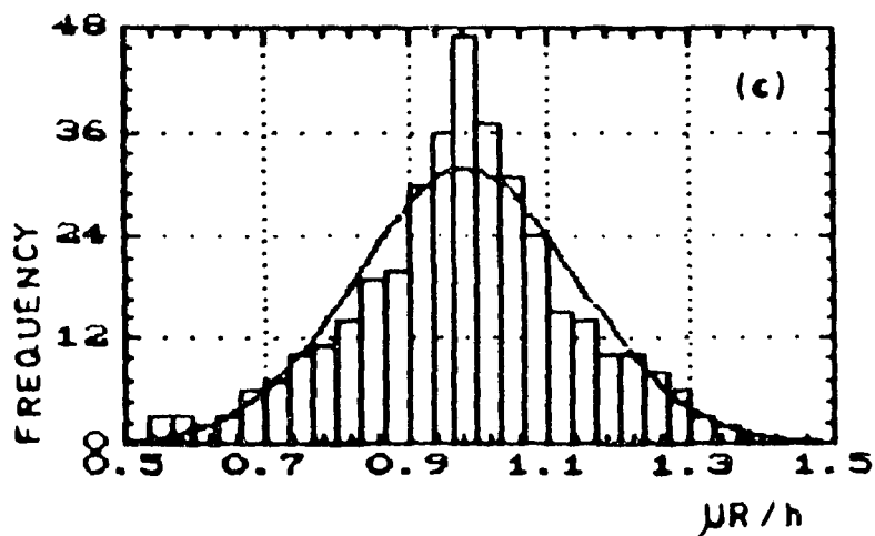
FIG. 7. Frequency histograms of aeroradioactivity data with fitted theoretical curves of the interpreted radiometric units (a) Q 1,2 (b) Q 3,4, and (c) Q 9, 10, 11.
