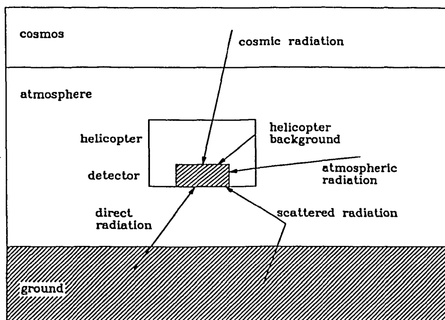
FIG. 2. Situation encountered during airborne radiometric measurements.
