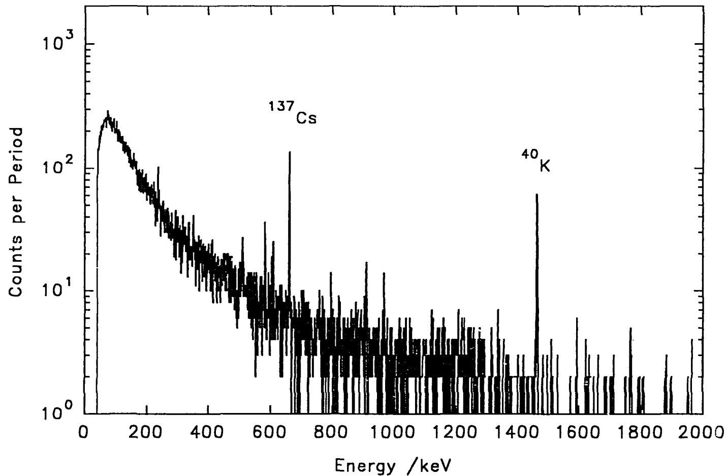
FIG. 4.b Aerial gamma ray spectra at Cairnsmore of Fleet, showing natural sources and Chernobyl derived ^{137}\text{Cs} 50% relative efficiency GMX.
