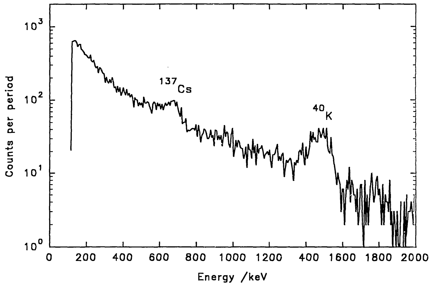
FIG. 4.a Aerial gamma ray spectra at Cairnsmore of Fleet, showing natural sources and Chernobyl derived ^{137}\text{Cs} NaI detector.
