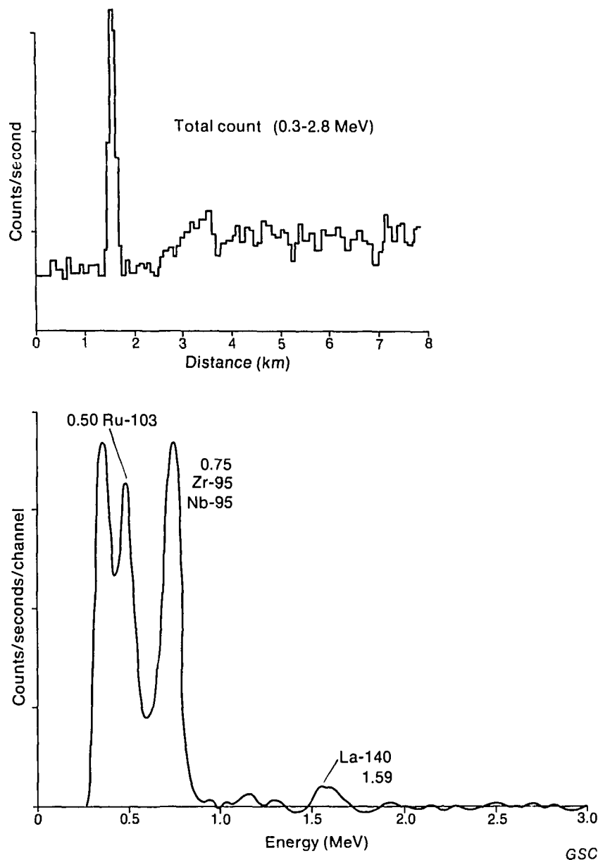
FIG. 2. Total count profile and gamma ray spectrum showing the peaks of ^{103}\text{Ru} , ^{95}\text{Zr} - ^{95}\text{Nb} and ^{140}\text{La} .
