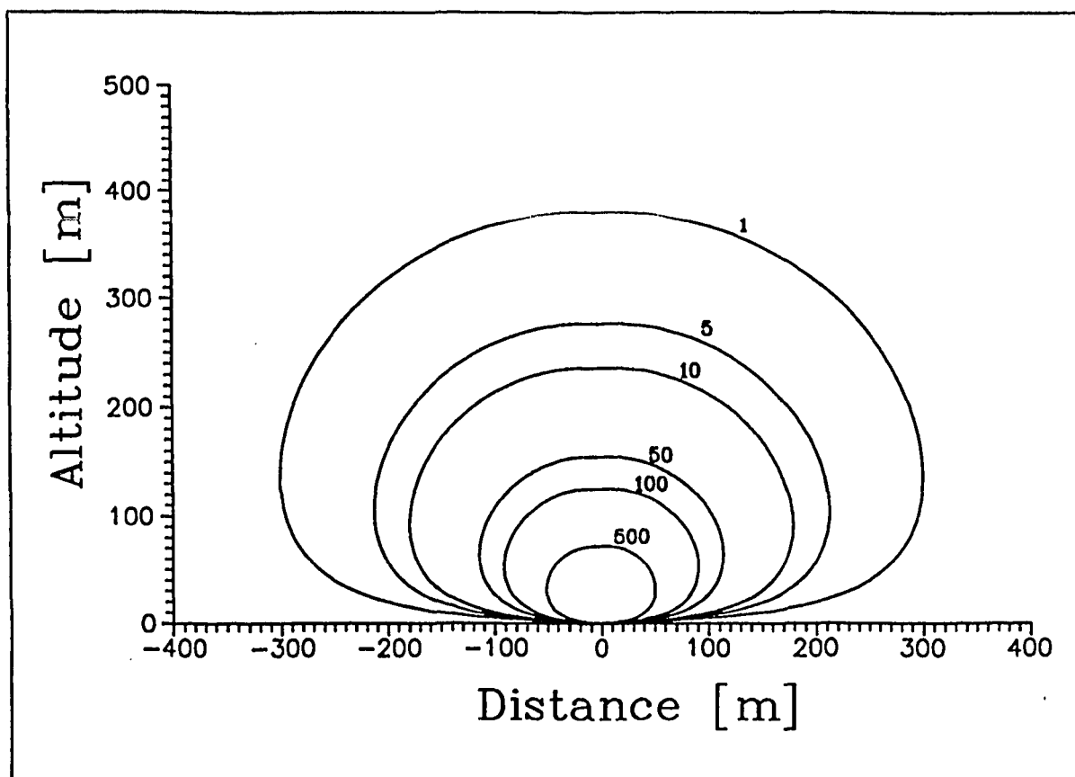
FIG. 6. Modelled count rate (1, 5, 10, 50, 100, 500 cps isolines) of a 1.9 GBq (50 mCi) \text{Cs}^{137} source buried at a depth of 1 cm using the experimentally determined detector efficiency.
