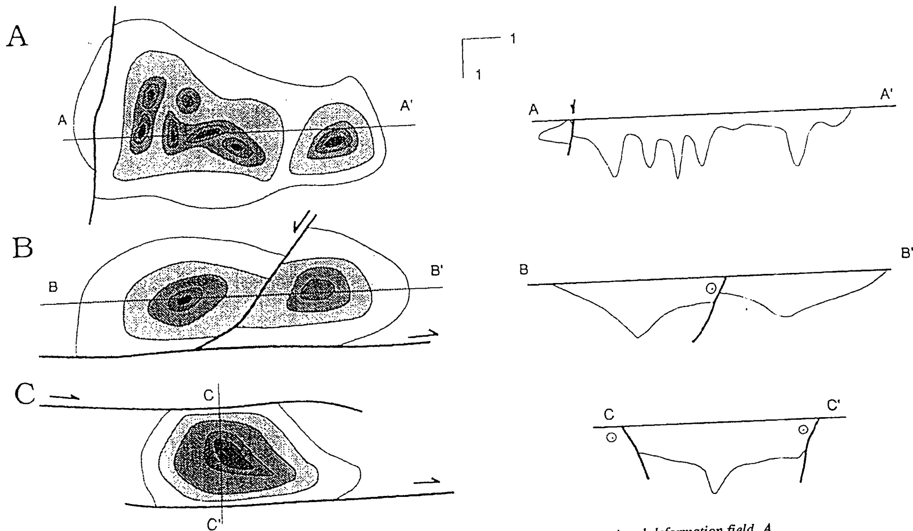
FIGURE 9. Schematic morphology of granitic plutons according to the regional deformation field. A map (on the left) and a cross section (on the right) with no vertical exaggeration are represented that show the style of pluton which can be expected according to the regional deformation regime: A) extension, B) wrench deformation, C) jog within overlapping shear zones.
