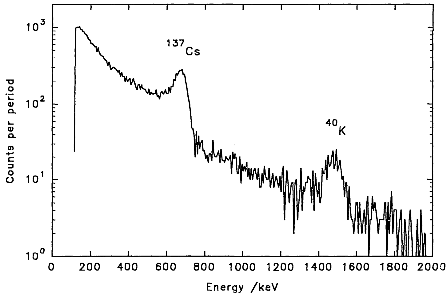
FIG. 5.a Aerial gamma ray spectra at Kirkconnel Merse, showing natural sources and Sellafield derived ^{137}\text{Cs} NaI detector. Note the enhanced forward scattering and higher ^{137}\text{Cs}/^{134}\text{Cs} compared with Fig. 4.
