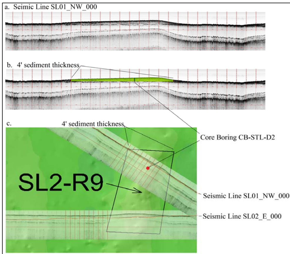
Figure 5. a. Seismic line SL01_NW_000 showing a surficial shoal offshore of St. Lucie County elucidating the triangular nature of the source. b. Boring CB-STL-D2 is projected on the seismic line along with the extents of the source horizontally to a 4-ft thickness. c. The planar extent of the source is outlined as identified using the seismic and bathymetric data.
