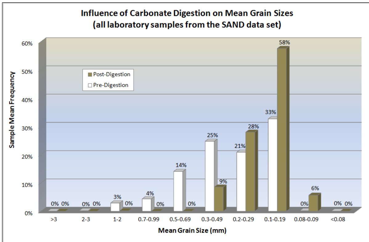
Figure 3. Sample Means (mm) frequency pre- and post-carbonate digestion. The shift in the skewness and kurtosis of the frequency of mean distributions indicates that the carbonate content in the data set occurred in the coarser fractions of the samples.
