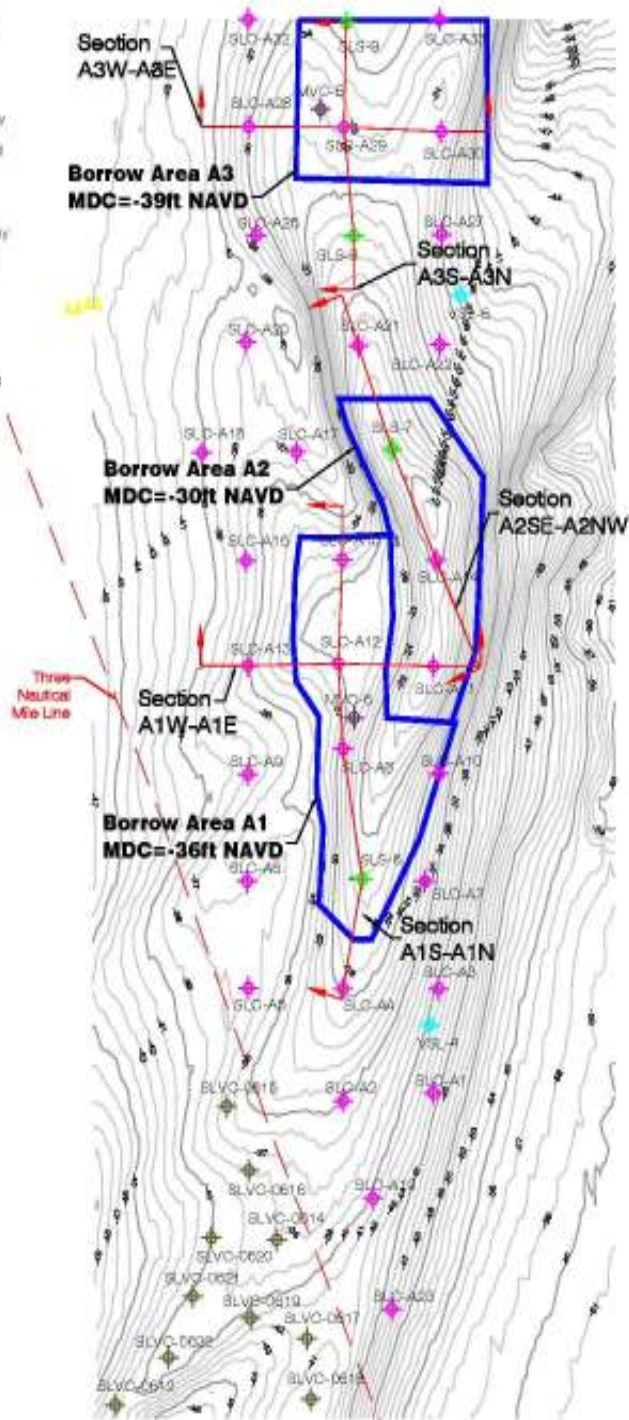
Figure 4a: South County Beach Project – Potential “50-year” Borrow Area
