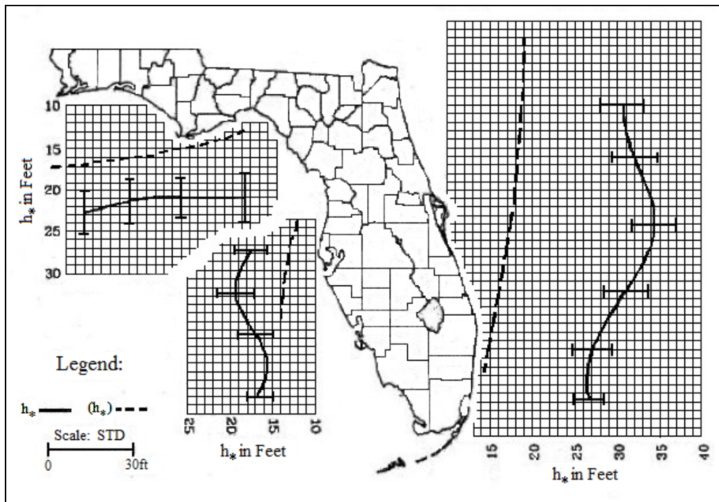
Figure 4. Depth of closure was selected for the study areas from Dean and Malakar (2002). Depth of closure calculated from Dean and Malakar (2002) is represented by h_* with a solid line compared with depth of closure determined by Dean and Grant (1989). The vertical bars represent \pm one standard deviation about the averages of the depth of closure values.
