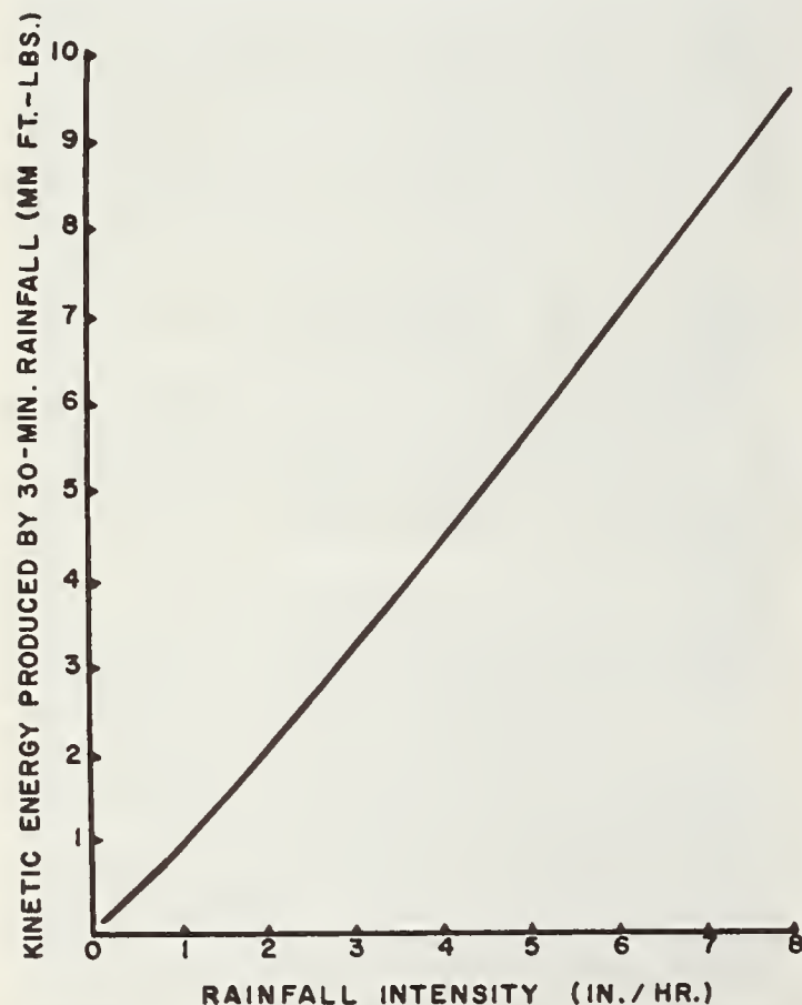
FIGURE 1. — Kinetic energy produced by 30-minute rainfalls of different intensities.
