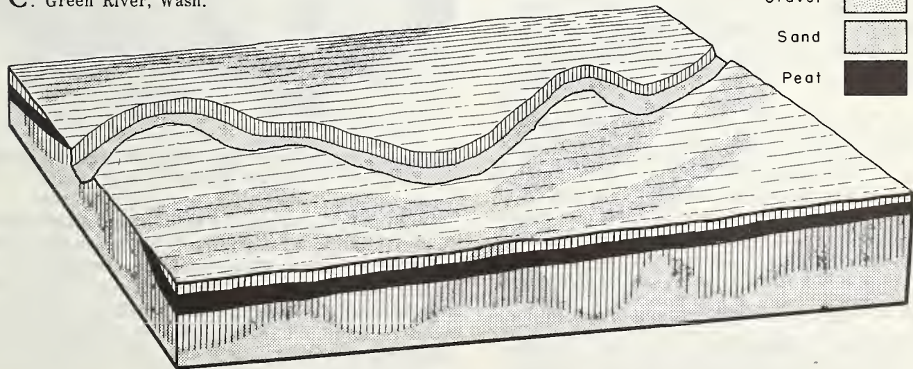
FIGURE 4. — Stratigraphy of alluvial deposits in three western streams.
