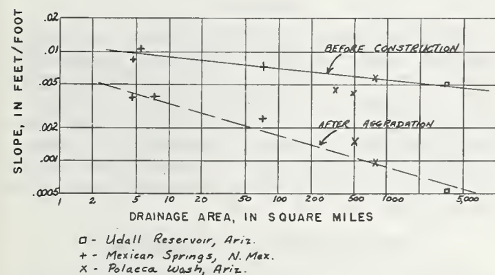
FIGURE 2.—Relation of drainage area to channel slope for several areas in Arizona and New Mexico.
