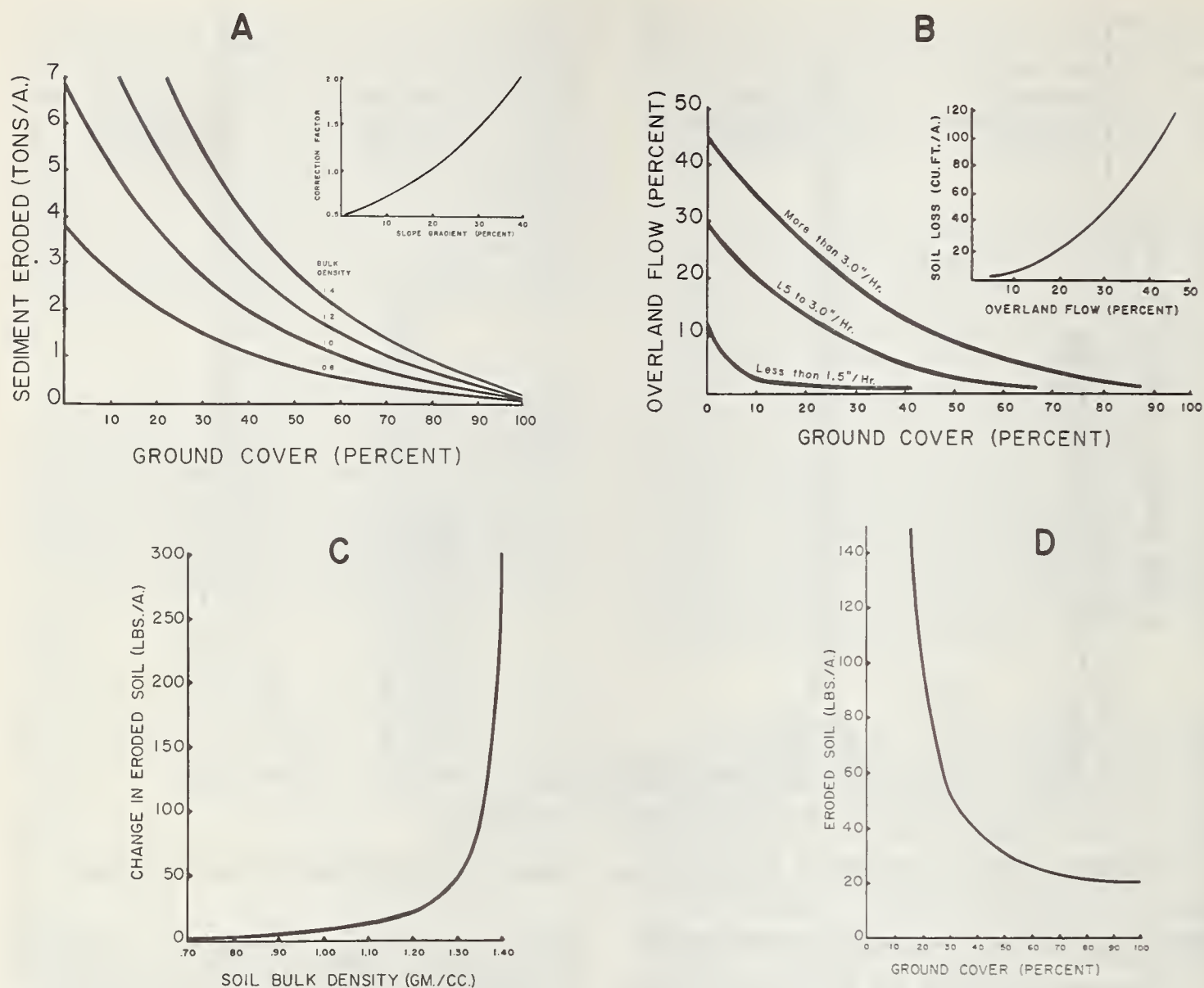
FIGURE 3.—A, Sediment eroded from central Utah rangelands in relation to ground cover and soil bulk density. The inset curve is a correction factor for sediment yield as affected by slope gradient. B, Overland flow by different storm intensity classes as a function of ground cover. The inset curve relates sediment to overland flow (Davis County Experimental Watershed, Utah). C, Changes in the amount of sediment produced in relation to soil bulk density on elk winter range in Montana. D, Sediment production as a function of ground cover at a mean bulk density of 1.14 on elk winter range in Montana.
