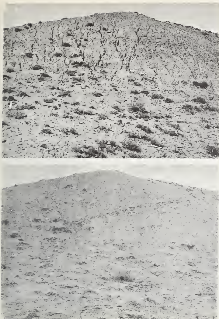
FIGURE 3. — Hillslope at Badger Wash, showing rilled surface in August 1959 (top) and same slope showing unrippled surface with some tracking in March 1961 (bottom).
