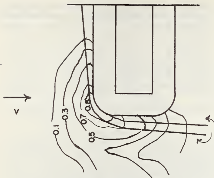
FIGURE 7. — Observed scour at a bridge abutment.
