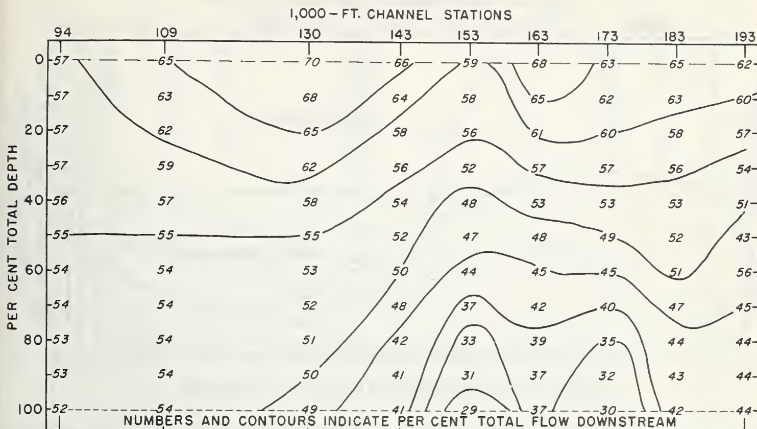
FIGURE 2. — Distribution of flow in Savannah Harbor.
