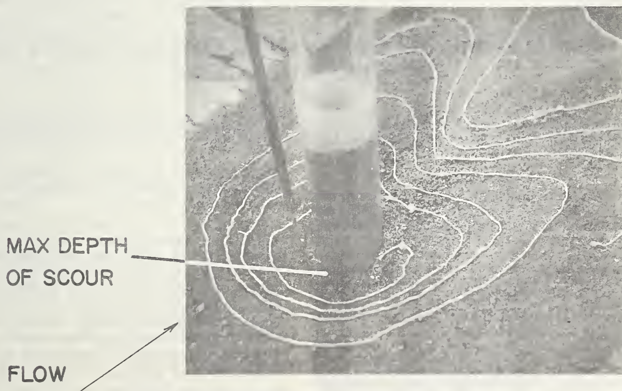
FIGURE 6. — Observed scour pattern at a round-nosed pier.
