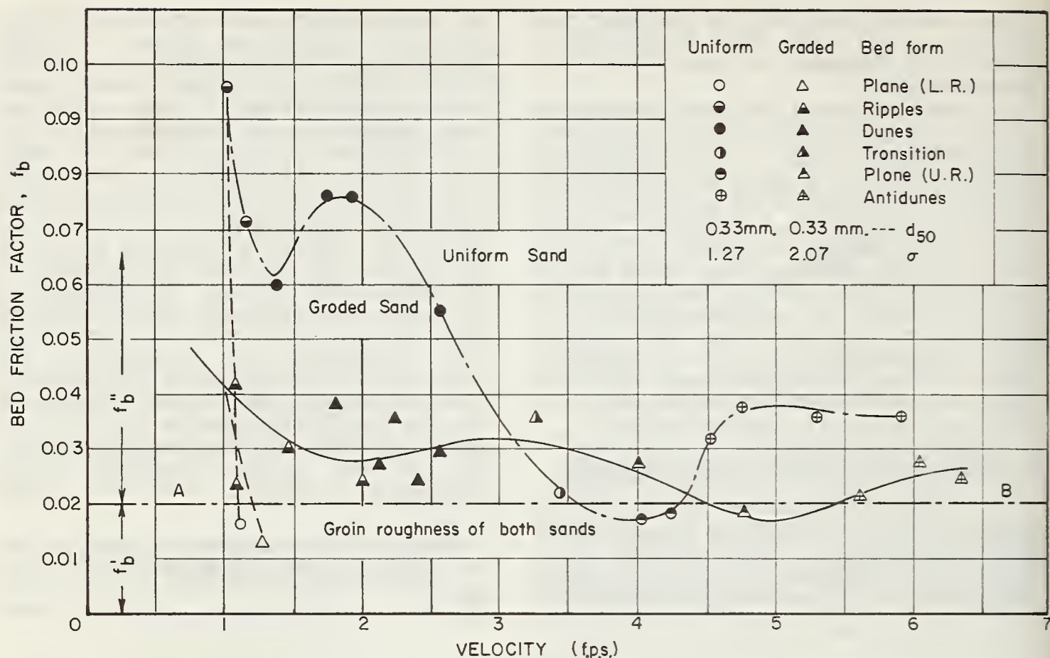
FIGURE 6.— Comparison of total bed friction factor, friction factor pertaining to grains, and friction factor pertaining to form roughness for uniform and graded bed material sands.
