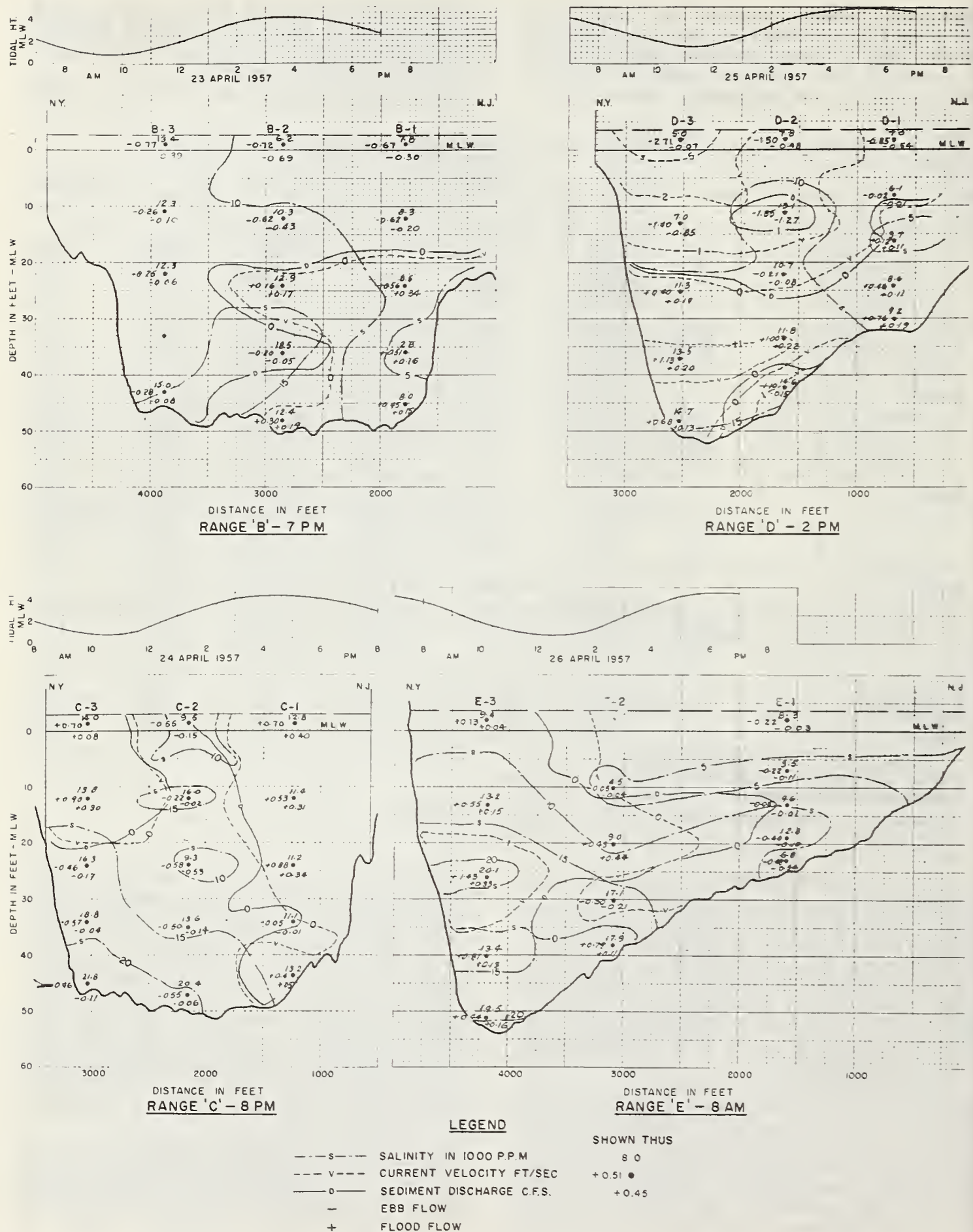
FIGURE 13. — Current velocity, sediment discharge, and salinity at minimum velocity.
