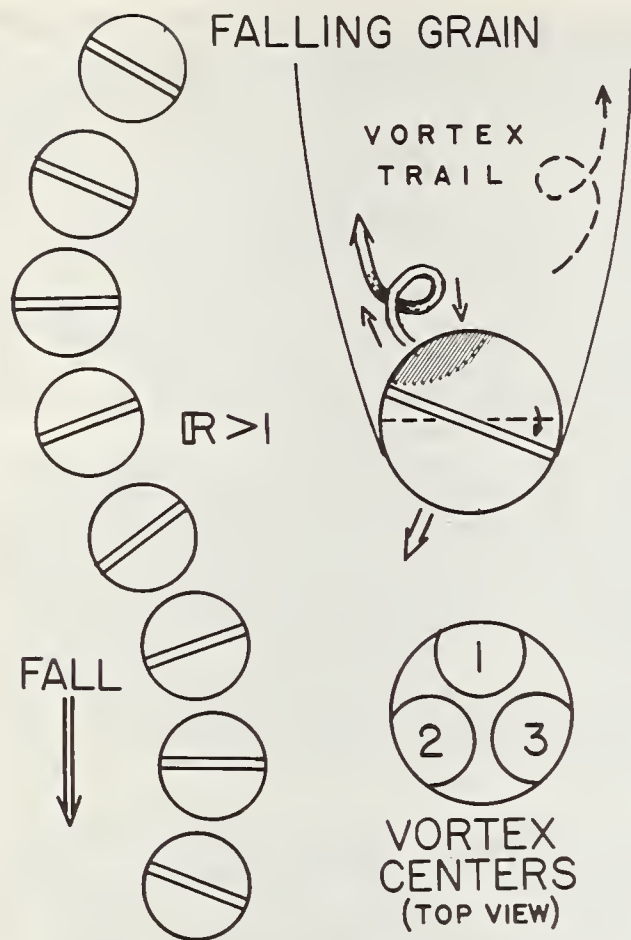
FIGURE 1. — Settling velocities and regimes.
