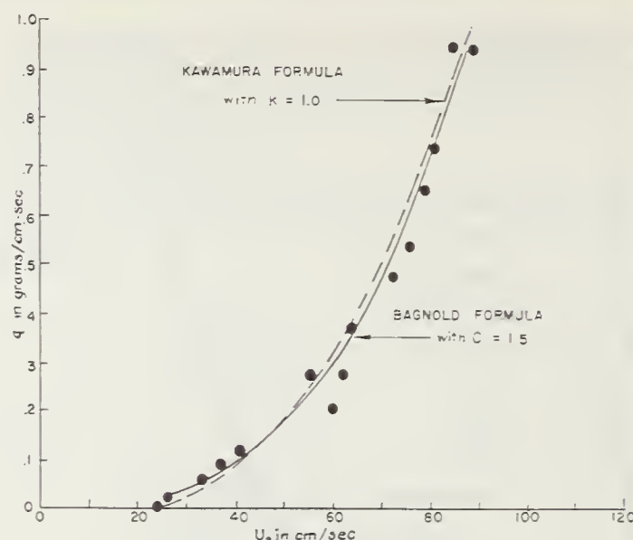
FIGURE 10.— Comparison of experimental data with Bagnold and Kawamura formulas for sand C ( d = 0.145 mm.).
