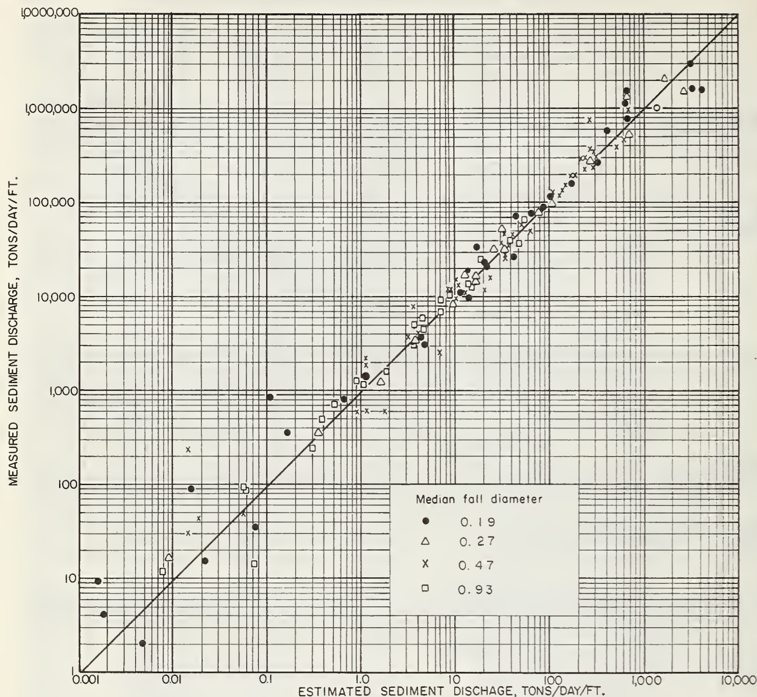
FIGURE 14.— Measured sediment discharge compared to sediment discharge computed using modified \phi\tau\psi' relation.
