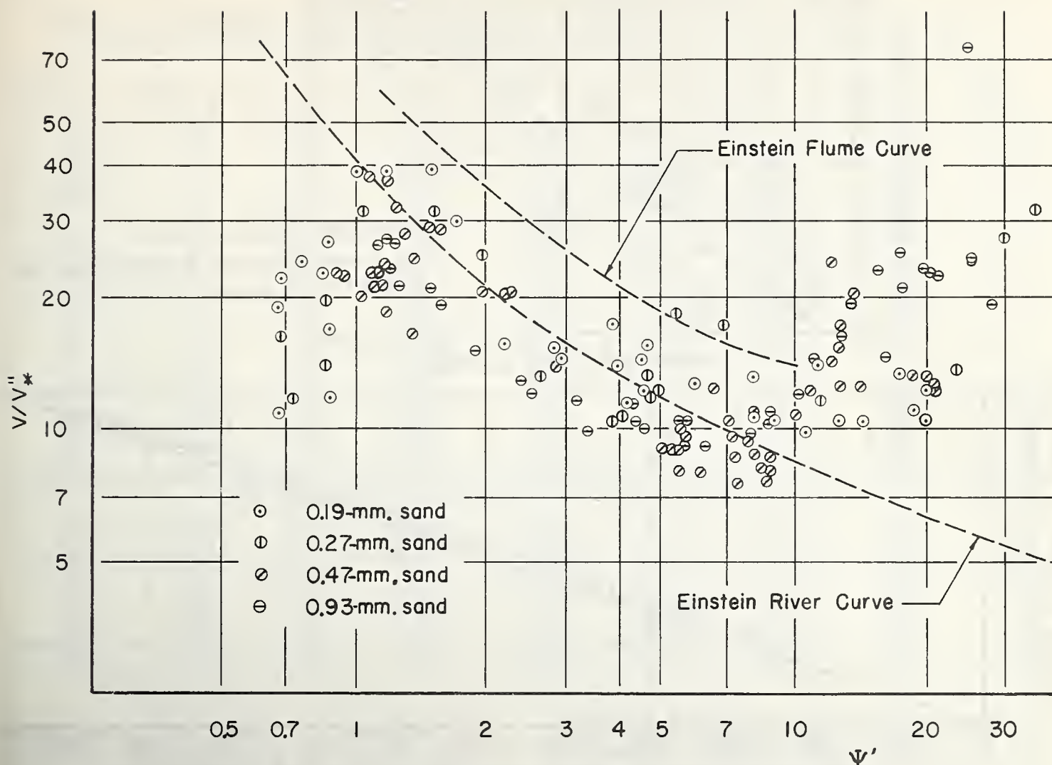
FIGURE 9.—Flume resistance data for various sands in relation to Einstein's bar resistance diagram.
