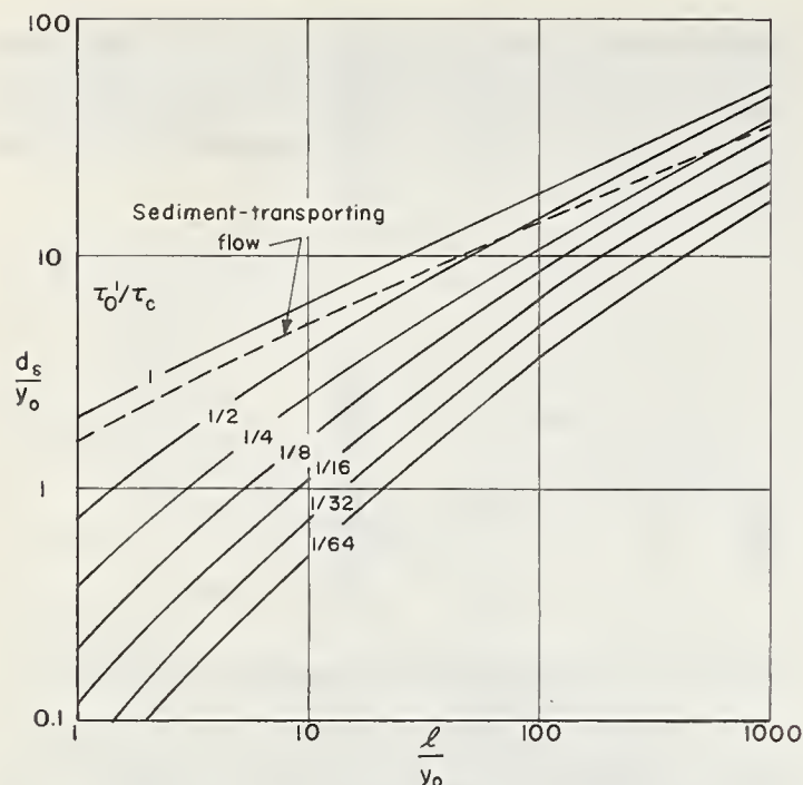
FIGURE 9. — Clear-water scour at an abutment.
