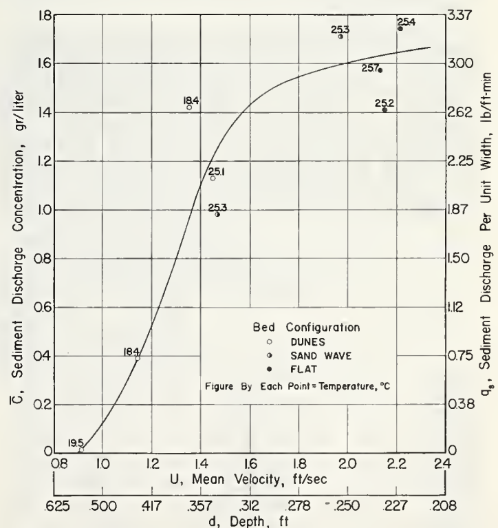
FIGURE 5.—Variation of sediment discharge concentration and sediment transport rate with mean velocity and depth for constant discharge experiments ( q = 0.50 c.f.s. per foot).
