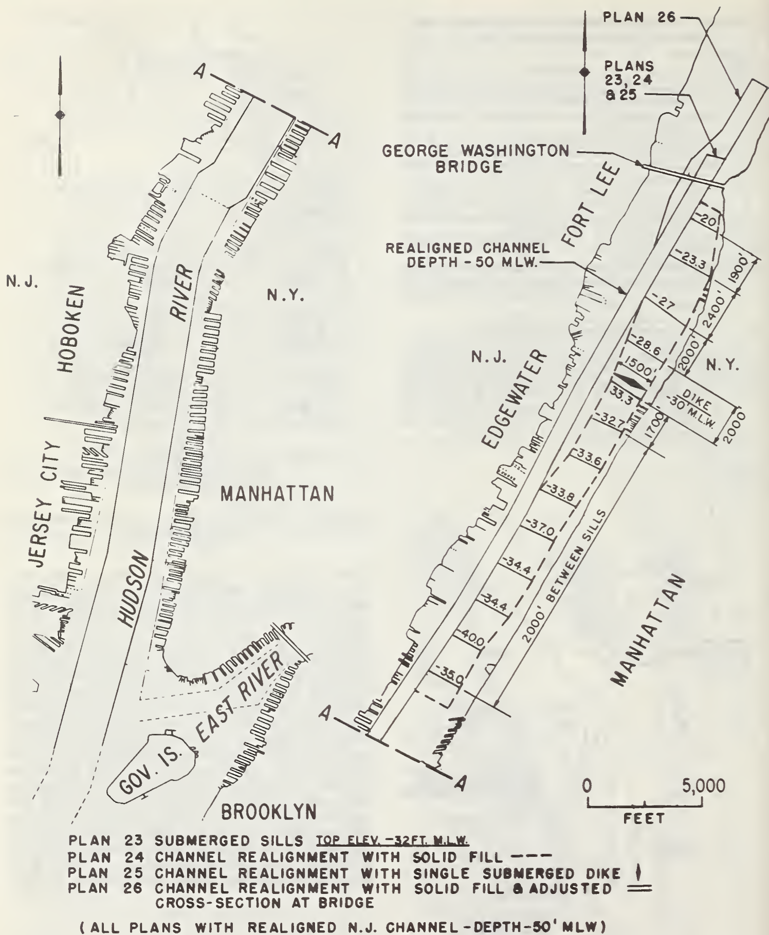
FIGURE 30. — Plan for realigned channel.
