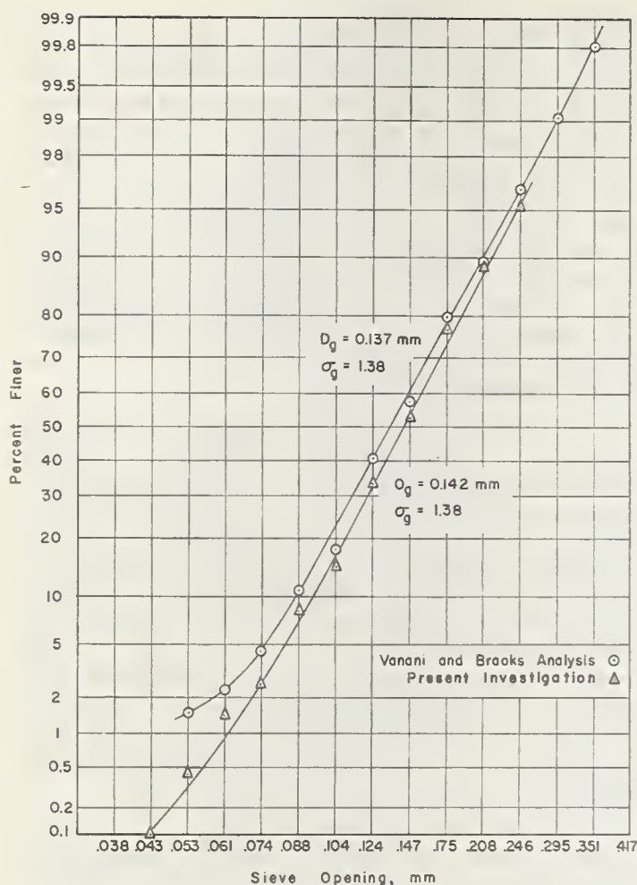
FIGURE 1. — Sieve analyses of the bed material.
