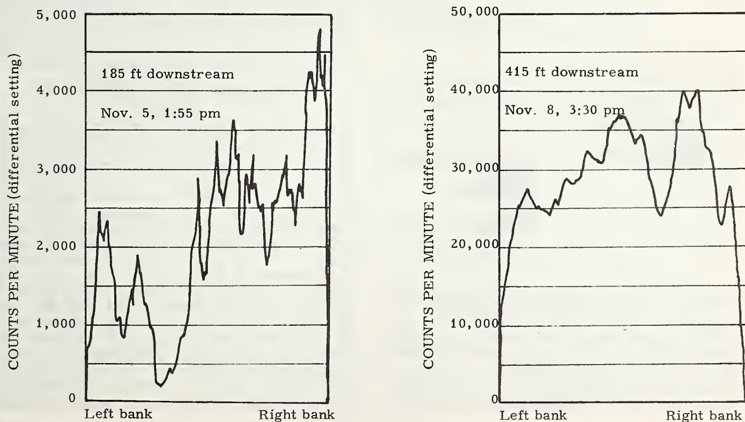
FIGURE 7.—Lateral distribution of labeled particles downstream from the source on Nov. 5 and 8, 1960.
