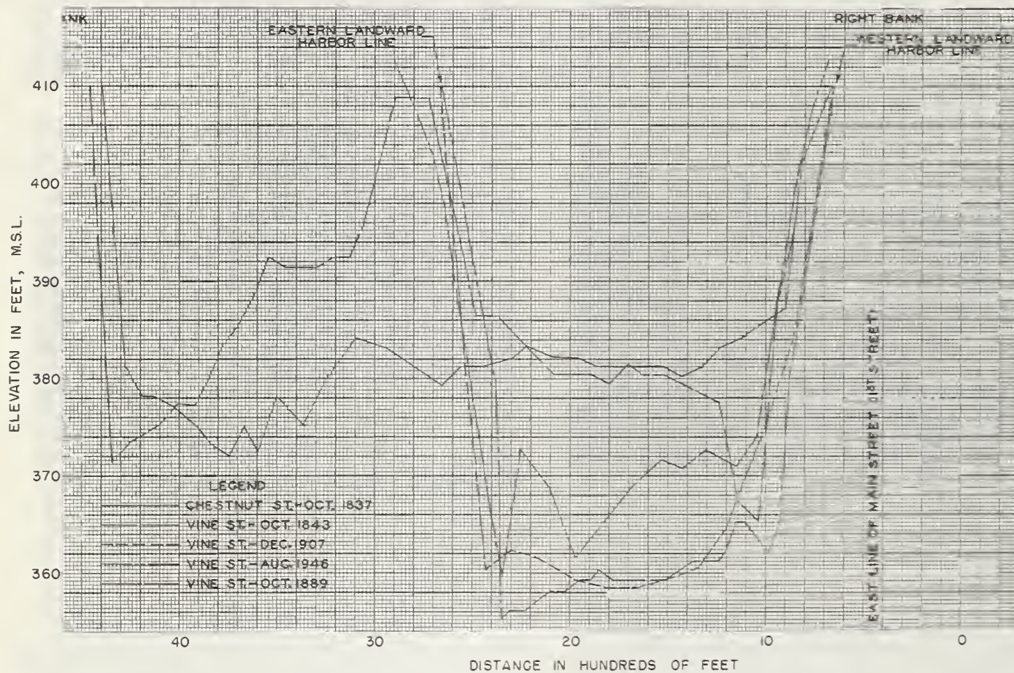
FIGURE 2. — Cross sections of Mississippi, downstream of Eads Bridge, 1837, 1843, 1889, 1907, and 1946.
