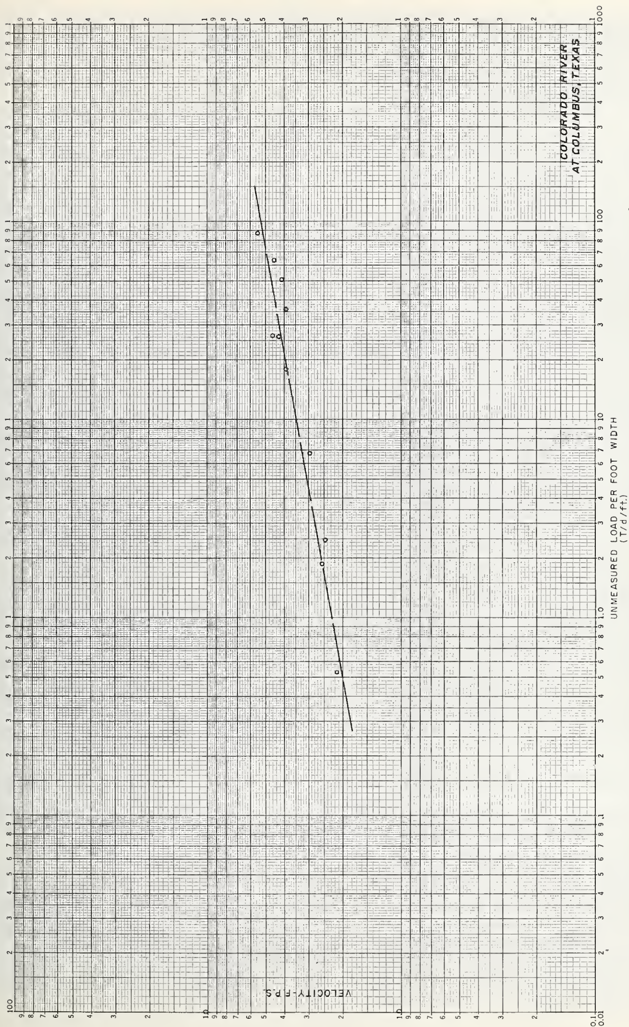
FIGURE 8. — Relation between unmeasured sediment load and mean velocity, Colorado River, at Columbus, Tex.
