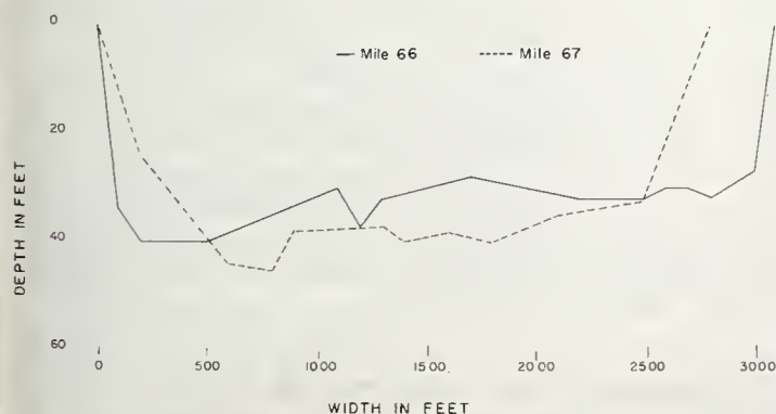
FIGURE 4.—Comparison of river cross sections at middle and head of Slaughters Bar, Columbia River.
