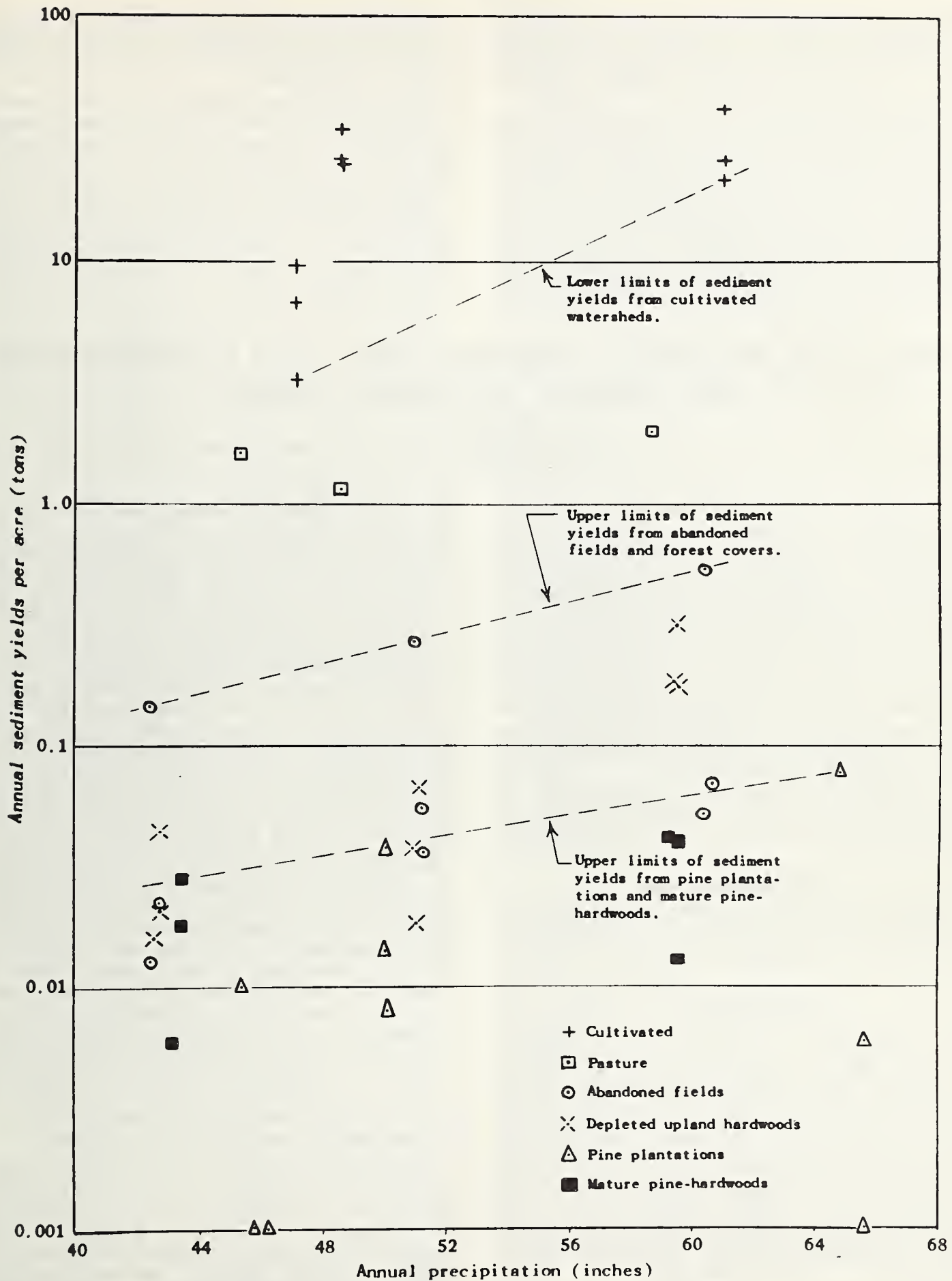
FIGURE 2.—Annual precipitation and sediment yield from individual watersheds in northern Mississippi, 1959-61.
