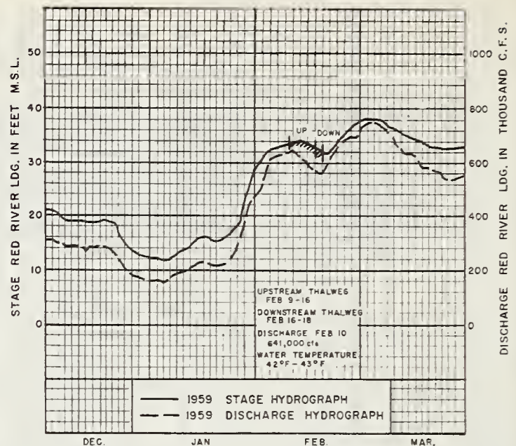
FIGURE 4.—1959 flood: Stage and discharge hydrographs, Mississippi River, Red River Landing, La.
