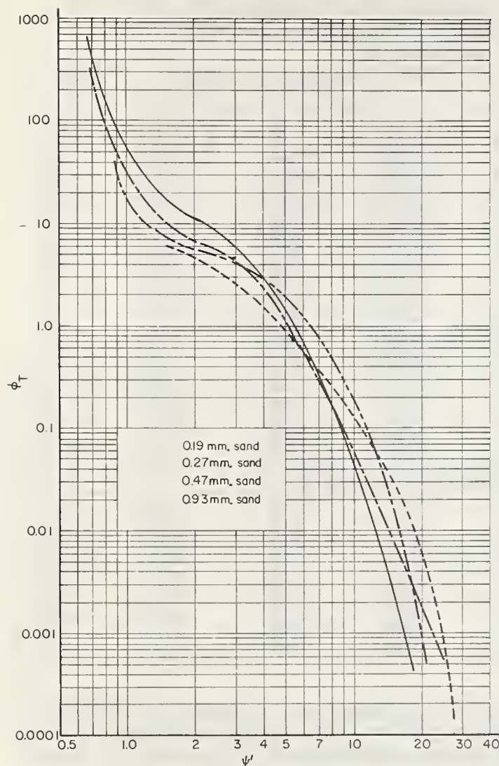
FIGURE 12. — Composite \phi\tau - \psi' curves for various sands from flume data.
