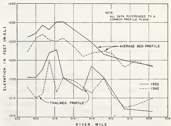
FIGURE 6.—Changes in average bed and channel thalweg elevations as observed at degradation ranges between 1952 and 1962.
