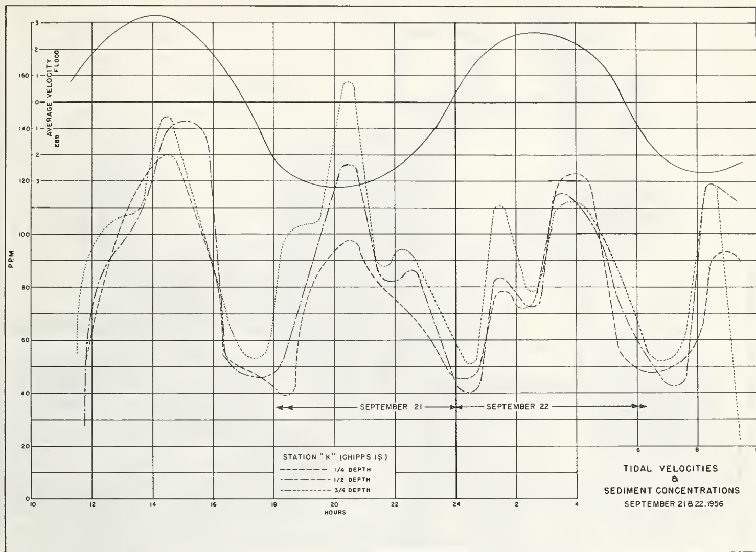
FIGURE 15.—Tidal velocities, phases, and sediment concentrations near Chipp Island, September 21 and 22, 1956.
