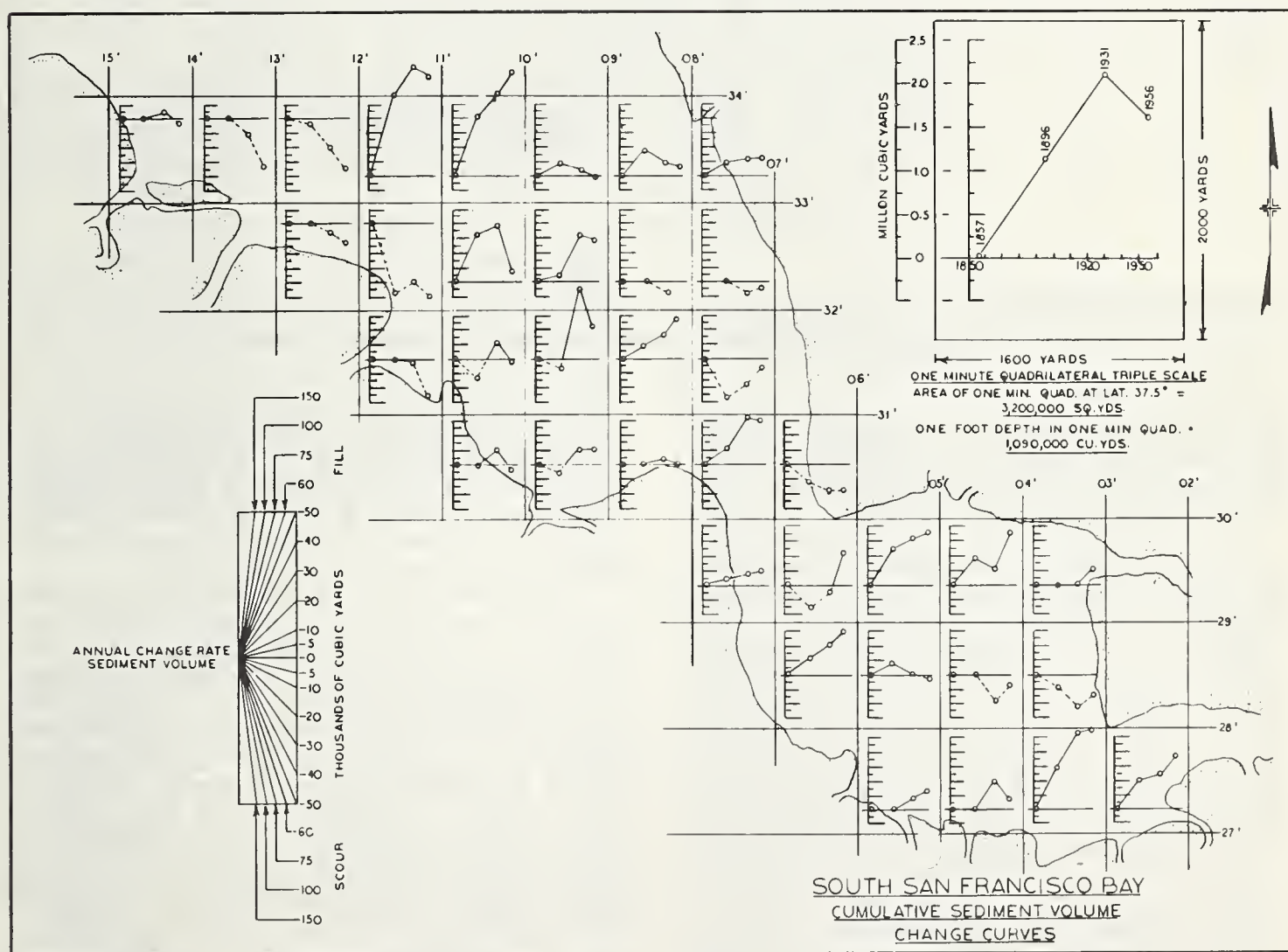
FIGURE 13.—Cumulative sediment volume change curves of South San Francisco Bay, 37° 35' to 37° 27' N.
