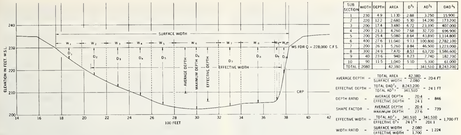
FIGURE 7.—Subdivision of a main channel cross section and determination of the "effective mean depth" and "effective width."
