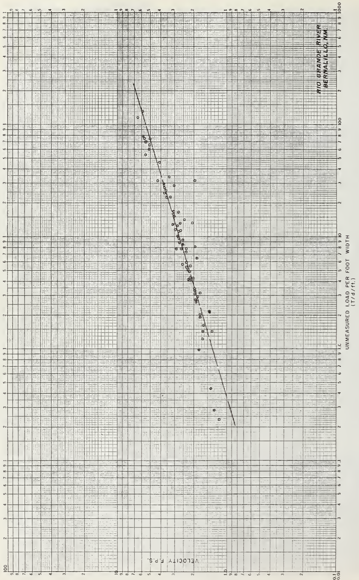
FIGURE 5. — Relation between unmeasured sediment load and mean velocity, Rio Grande, Bernalillo, N. Mex.
