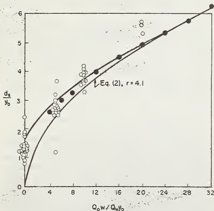
FIGURE 4. — Scour at an overbank constriction.
