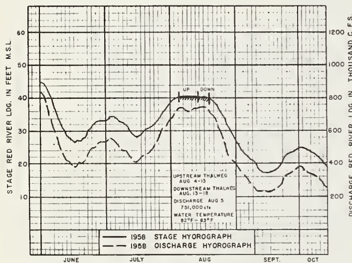
FIGURE 3.—1958 stage and discharge hydrographs, Mississippi River, Red River Landing, La.
