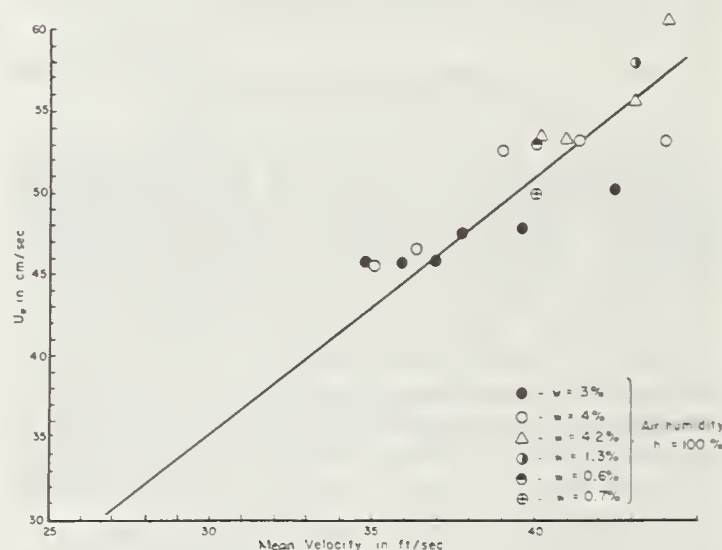
FIGURE 16.—Relation between shear velocity and mean velocity for high water contents.
