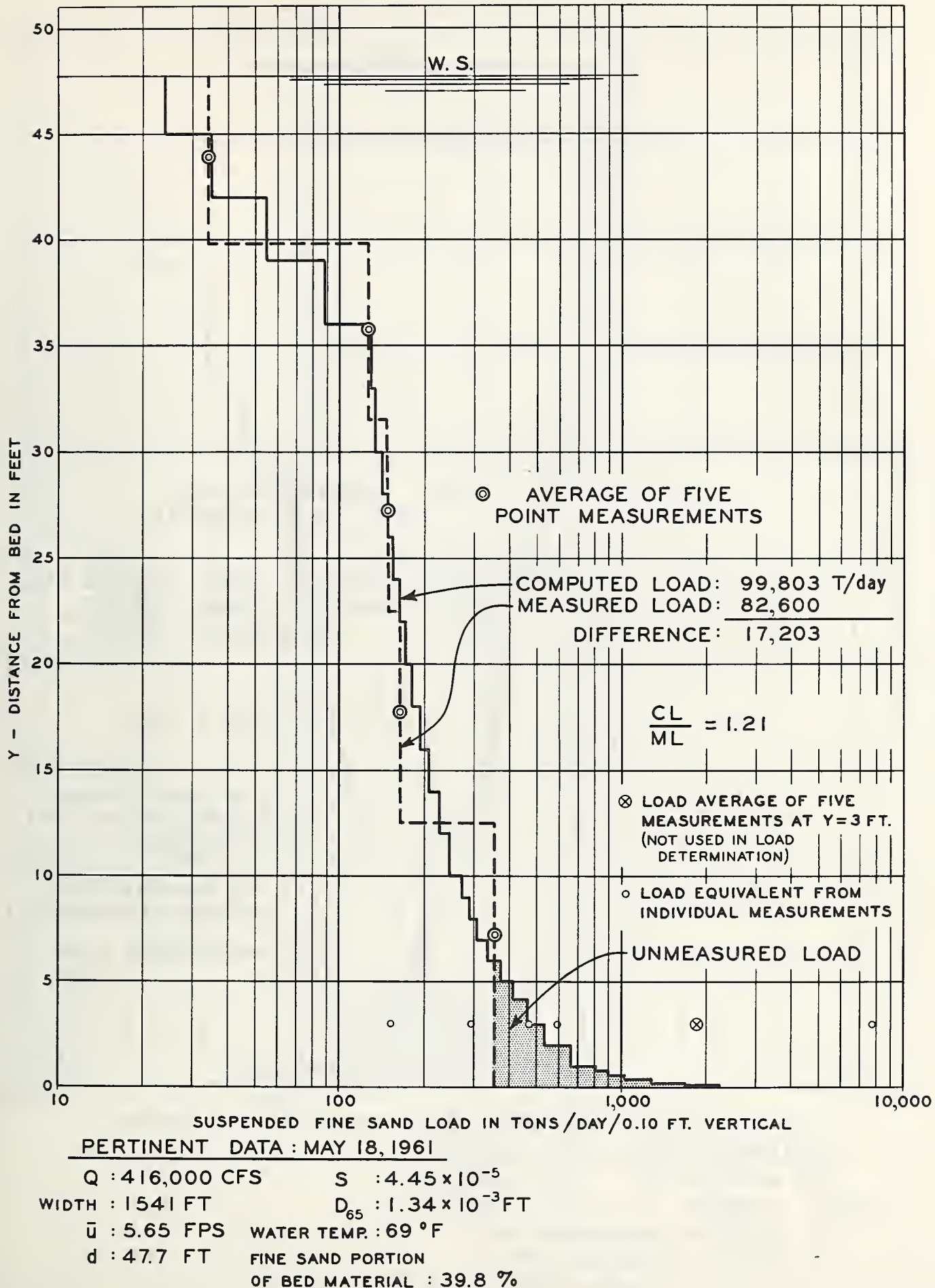
FIGURE 7.— Computed, measured, and unmeasured suspended fine sand load at Simmesport, Atchafalaya River, May 18, 1961.
