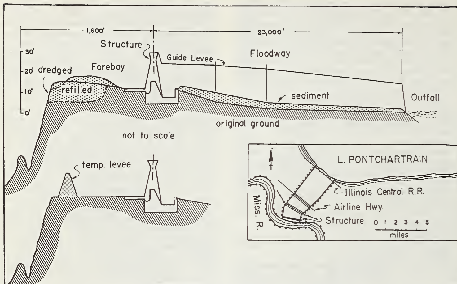
FIGURE 5. — Bonnet Carre spillway.
