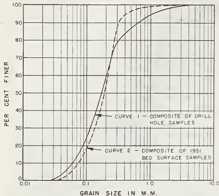
FIGURE 2.—Grain-size distribution of available bed materials as determined from drill hole and bed surface sampling.
