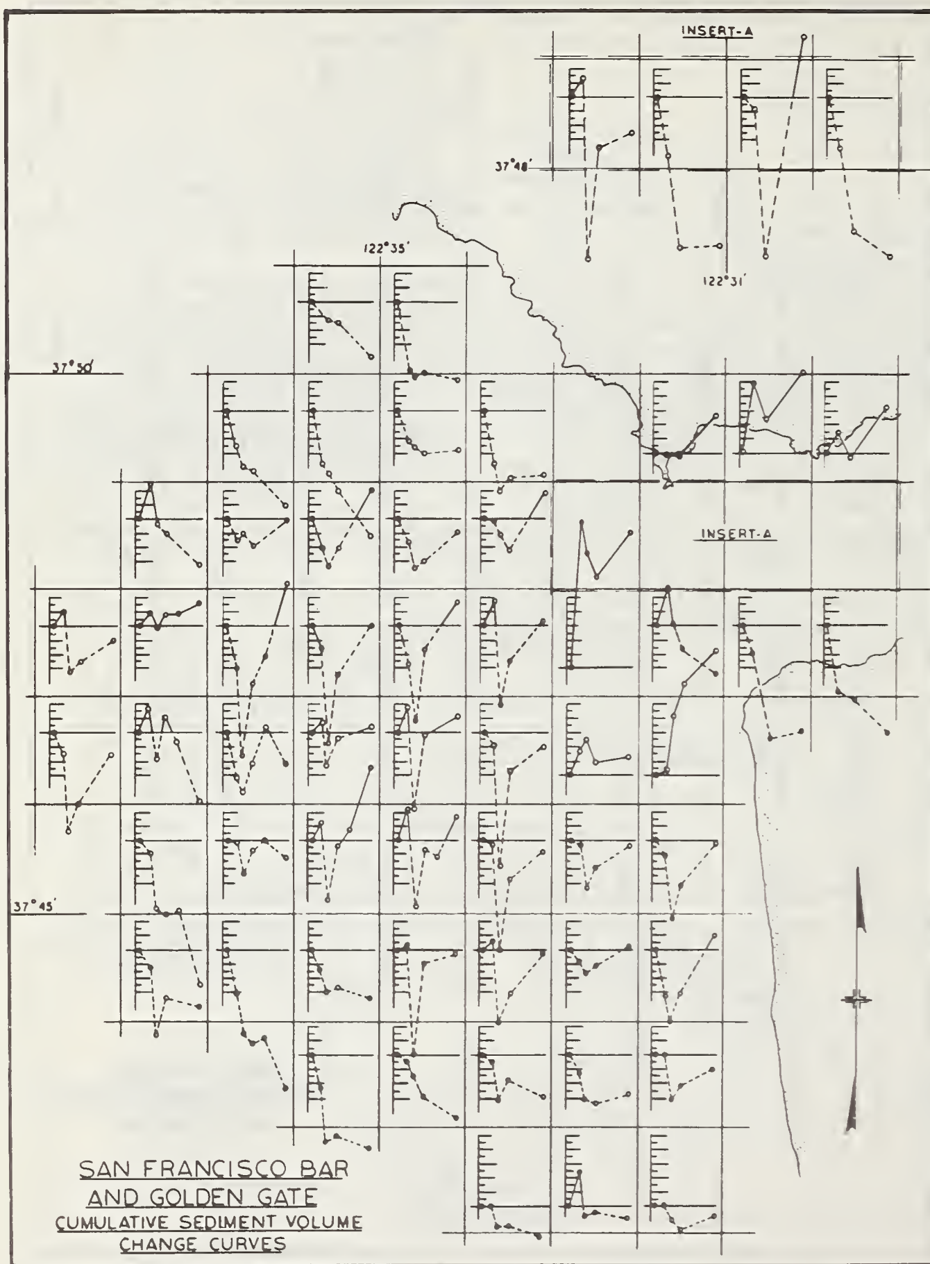
FIGURE 10. — Cumulative sediment volume change curves of San Francisco Bar and Golden Gate.
