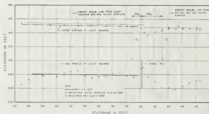
FIGURE 13.—Typical bed and water surface profiles from the University of Iowa tests.
