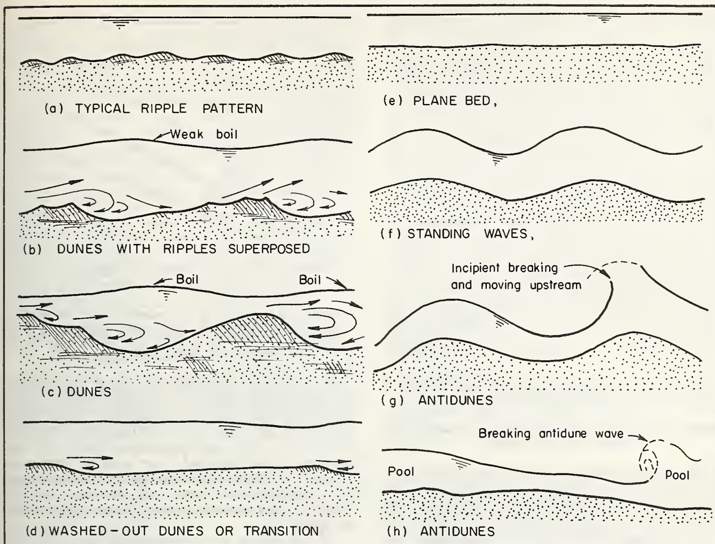
FIGURE 1. — Forms of bed roughness in alluvial channels.
