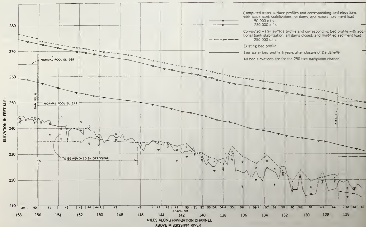
FIGURE 10.—Streambed and water surface profiles in Arkansas River Pool No. 7 for basic conditions and computed modified regime conditions.
