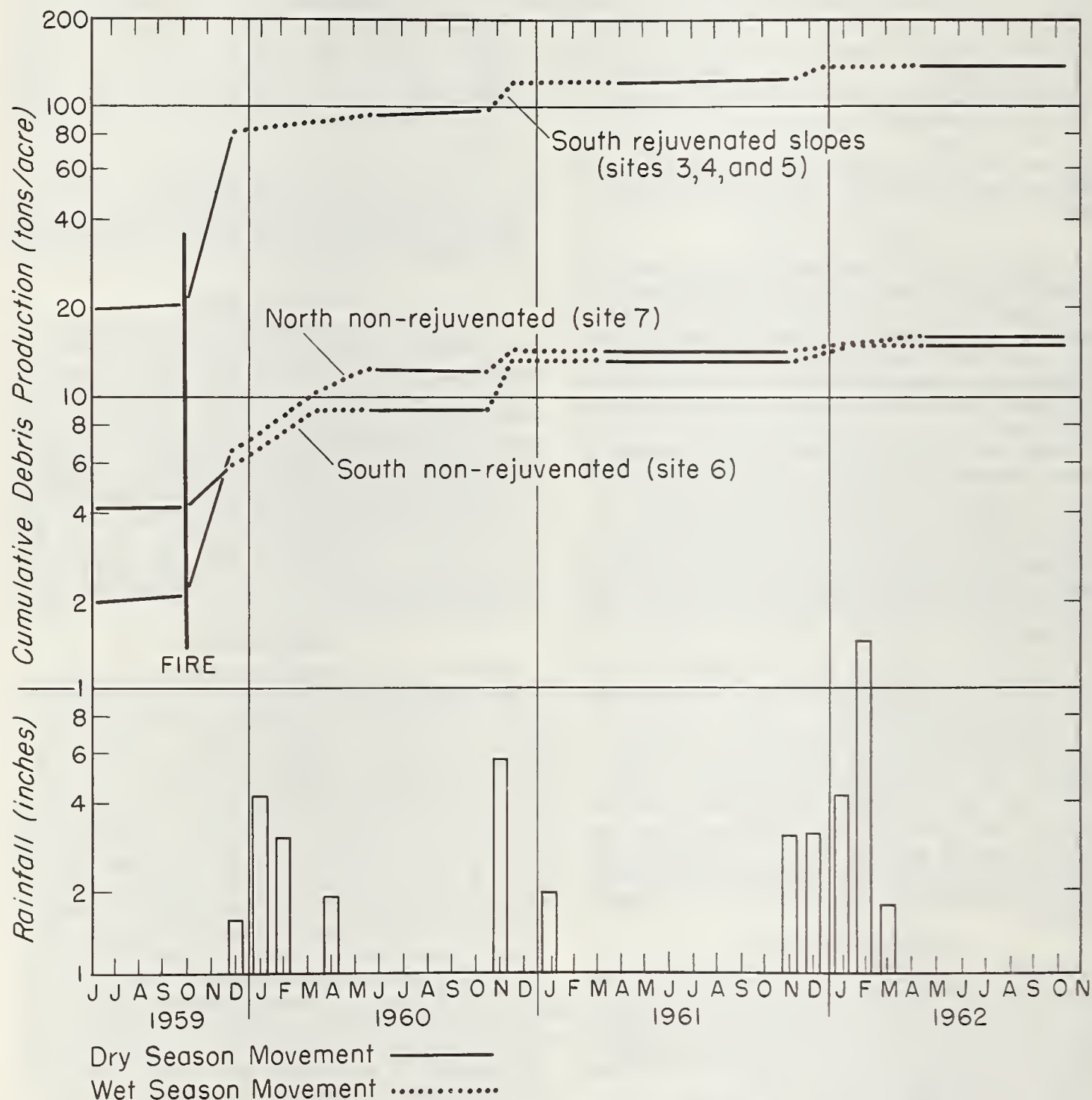
FIGURE 1. — Seasonal debris movement before and after fire in the Los Angeles watershed.
