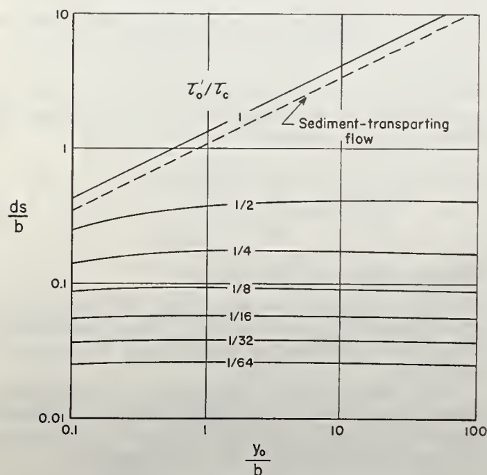
FIGURE 10. — Clear-water scour at a pier.
