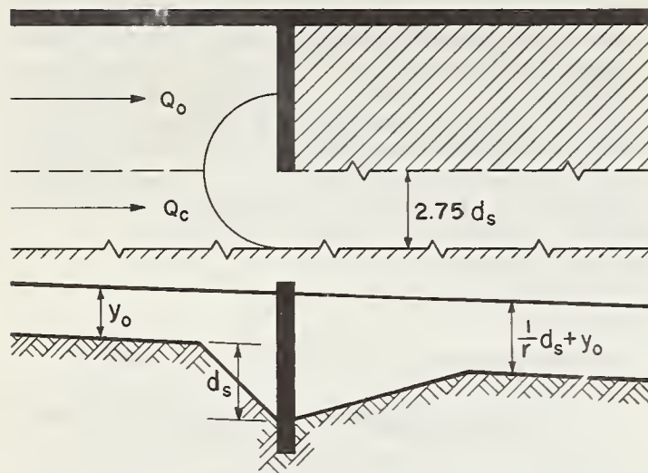
FIGURE 3. — Definition sketch of overbank constriction.
