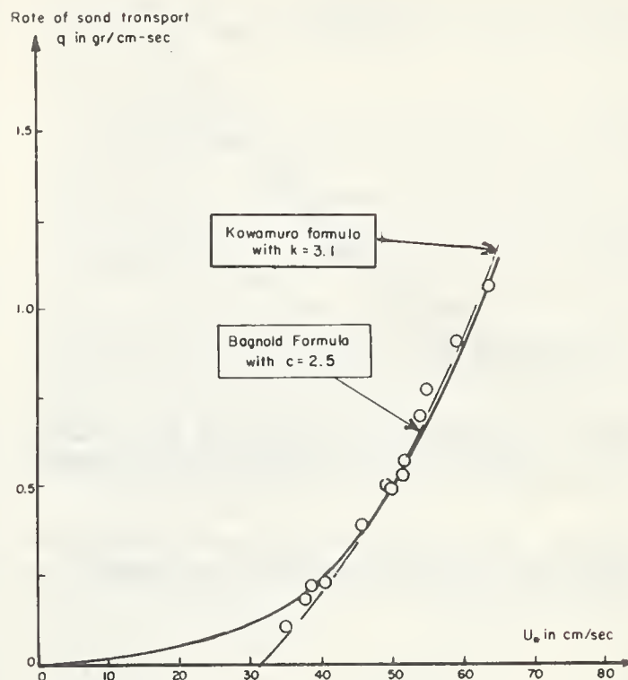
FIGURE 7.— Comparison of experimental data with the Bagnold and Kawamura formulas for sand A ( d = 0.44 mm.).
