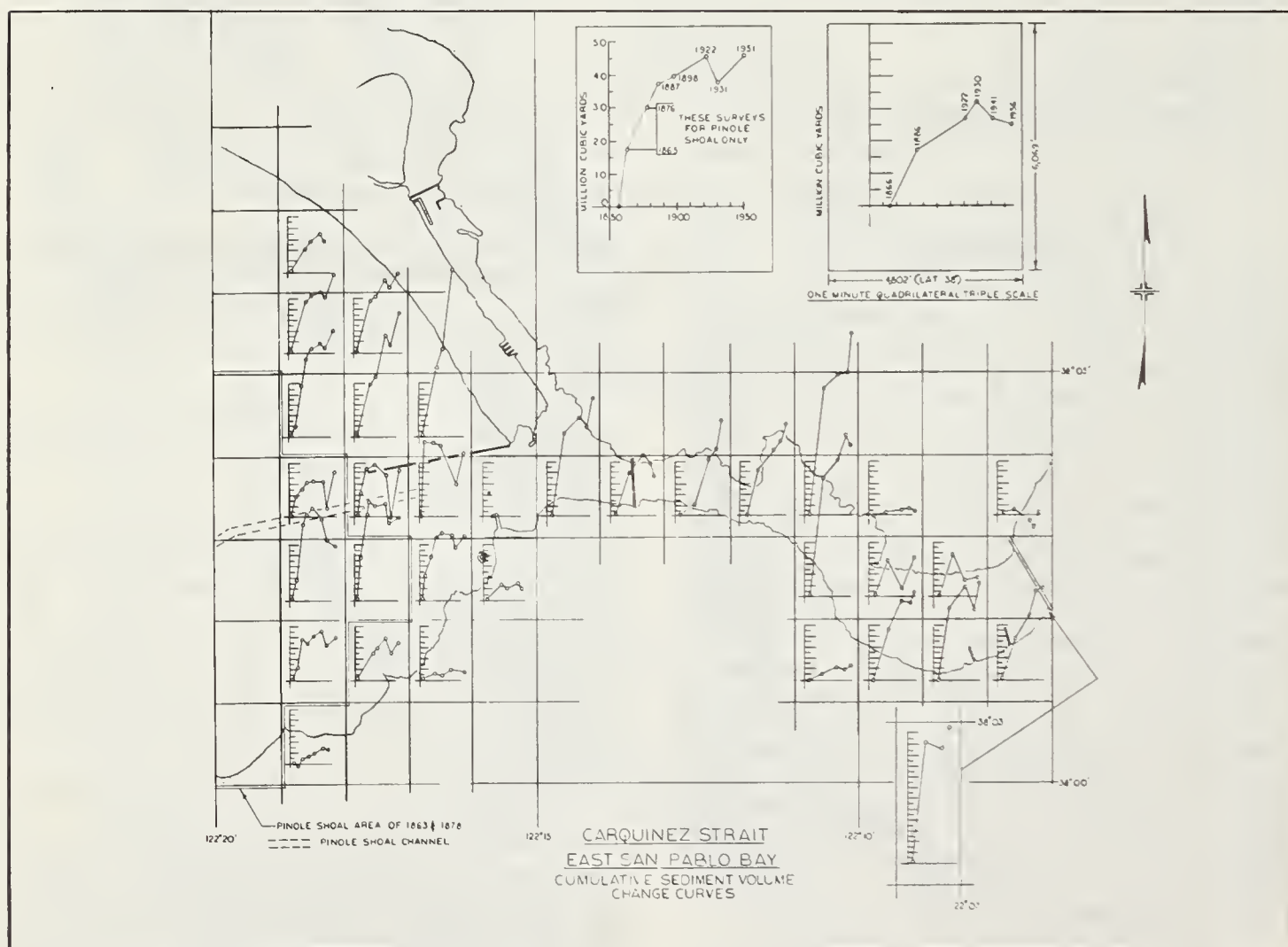
FIGURE 8.—Cumulative sediment volume change curves of Carquinez Strait, East San Pablo Bay.
