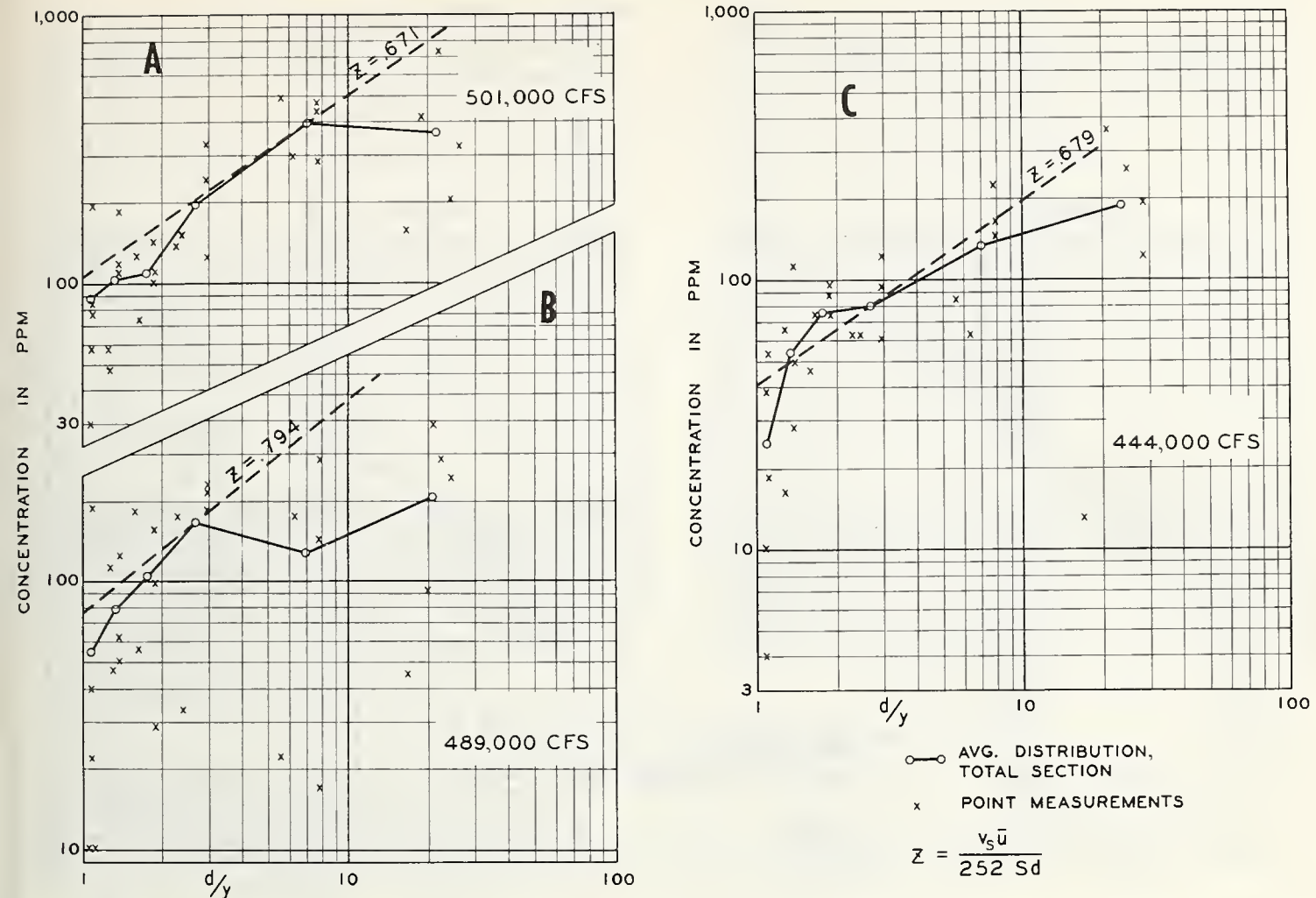
FIGURE 3.—Measured suspended fine sand at 6 levels at each of 5 verticals in cross section of Atchafalaya River at Simmesport, La.: A, for 501,000 c.f.s.; B, for 489,000 c.f.s.; C, for 444,000 c.f.s.
