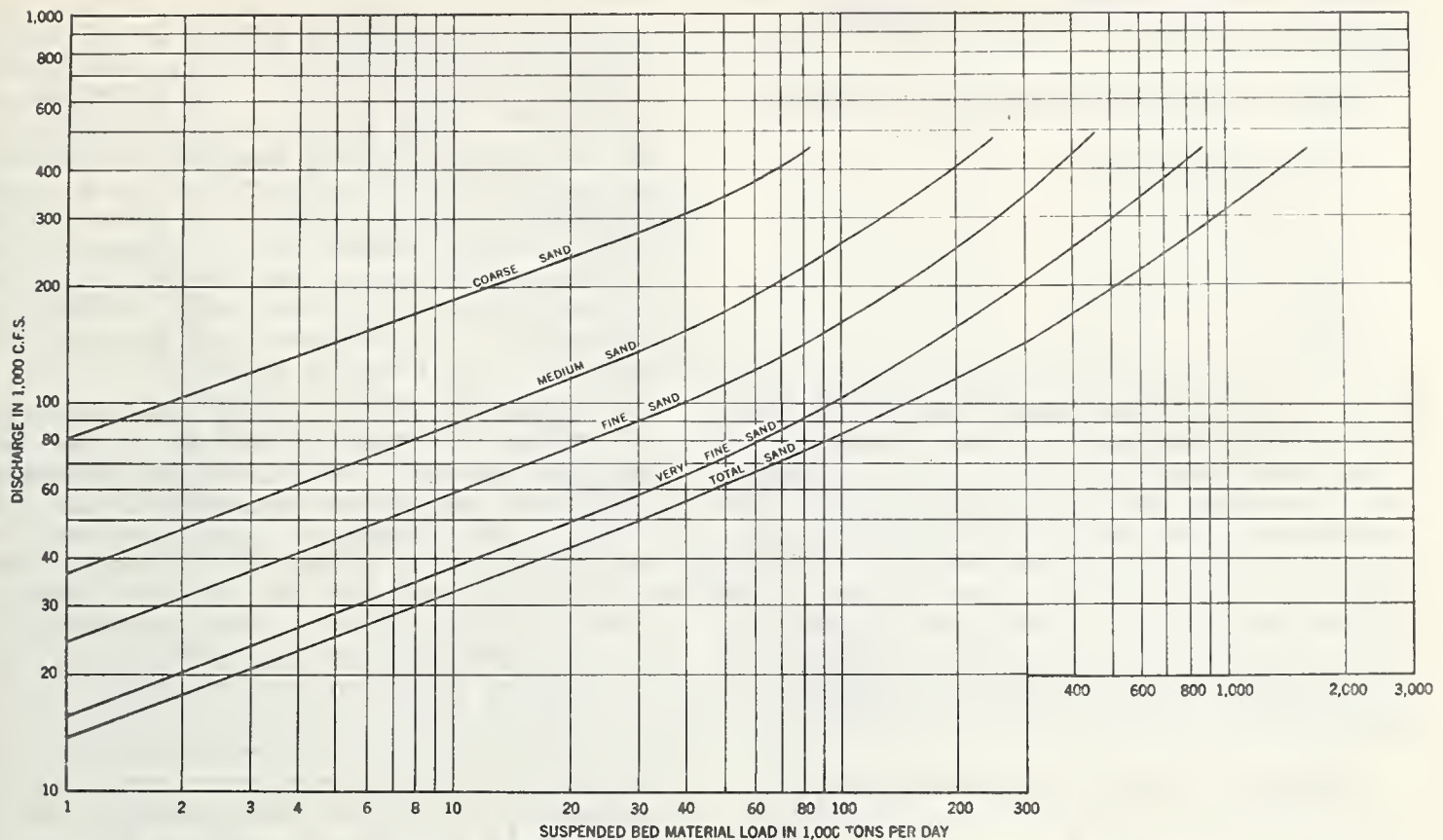
FIGURE 2.—Rating curve of suspended bed-material sediment load versus discharge for the Arkansas River at Little Rock, Ark.
