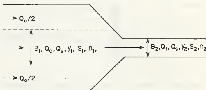
FIGURE 1. — Definition sketch of long contraction.
