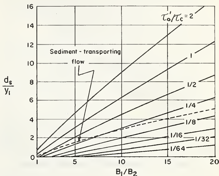
FIGURE 8. — Effect of shear ratio and width ratio on scour in a long contraction.
