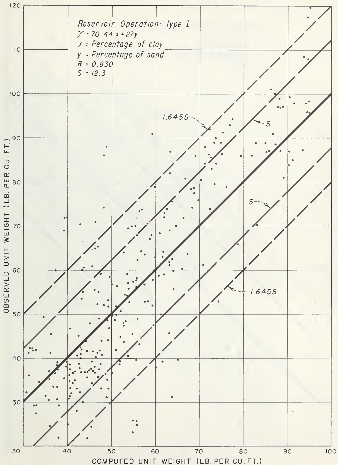
FIGURE 1. — Correlation of observed vs. computed unit weights. Reservoir operations: Type I.
