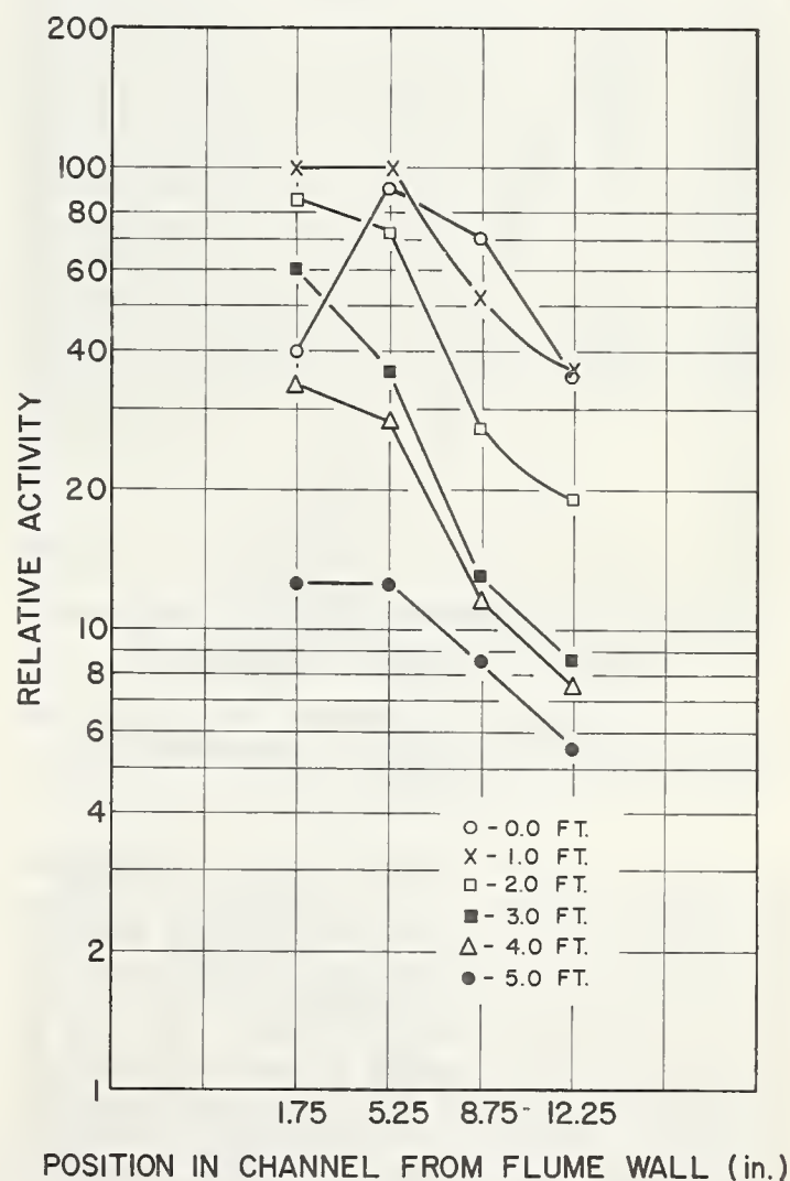
FIGURE 4. — Distribution of scandium-46 labeled sand within defined sections of the channel bed.
