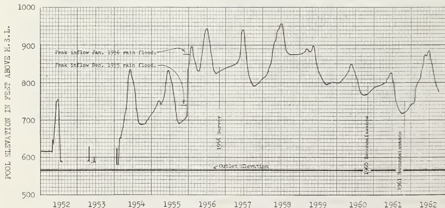
FIGURE 3. — Pine Flat Reservoir pool elevations.
