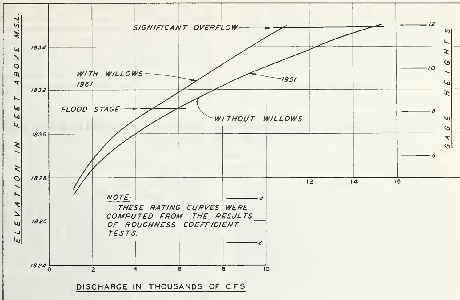
FIGURE 10. — Republican River stage-discharge relations near Bloomington, 1951 and 1961.
