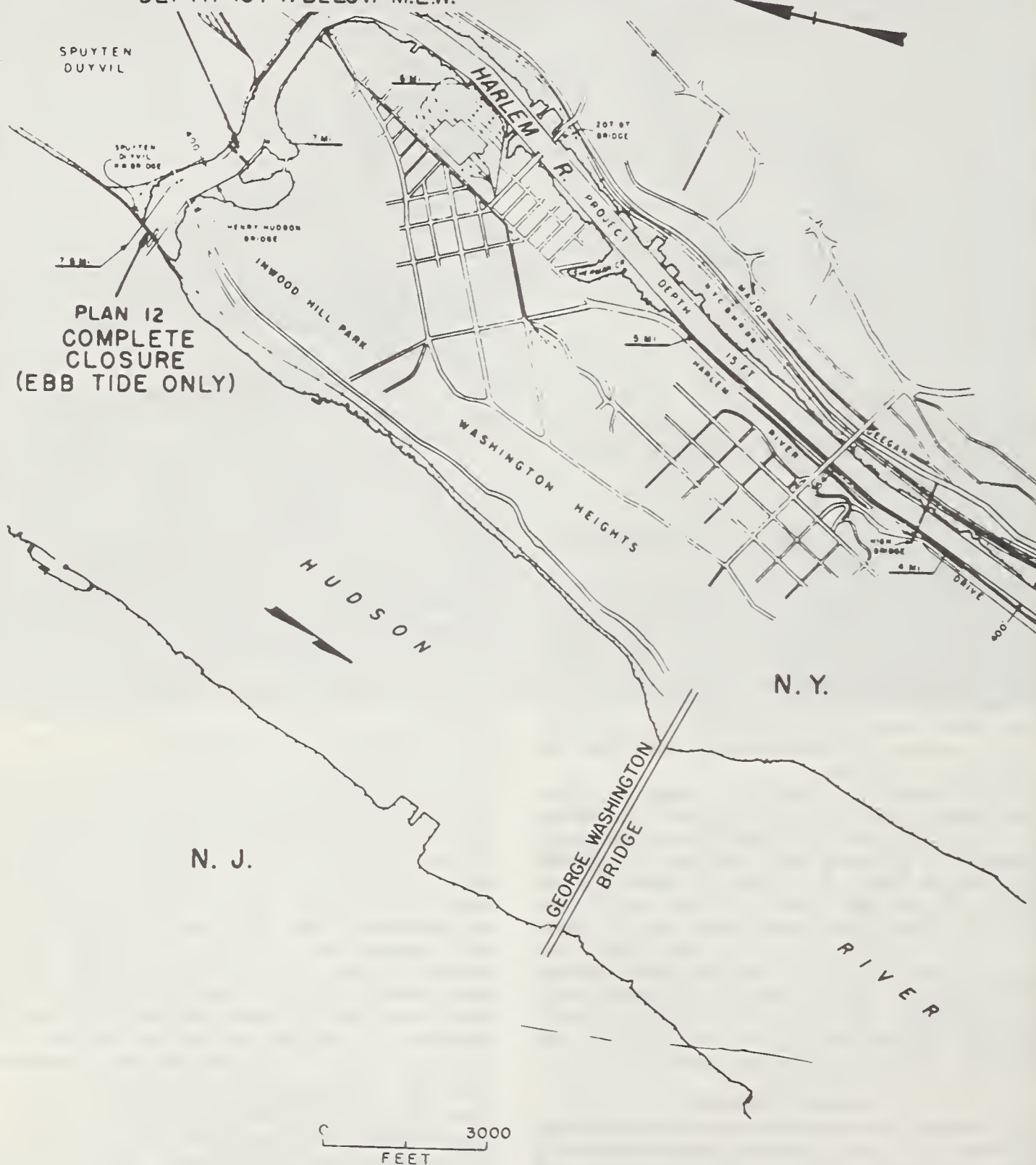
FIGURE 25. — Comprehensive model of Harlem River series.
