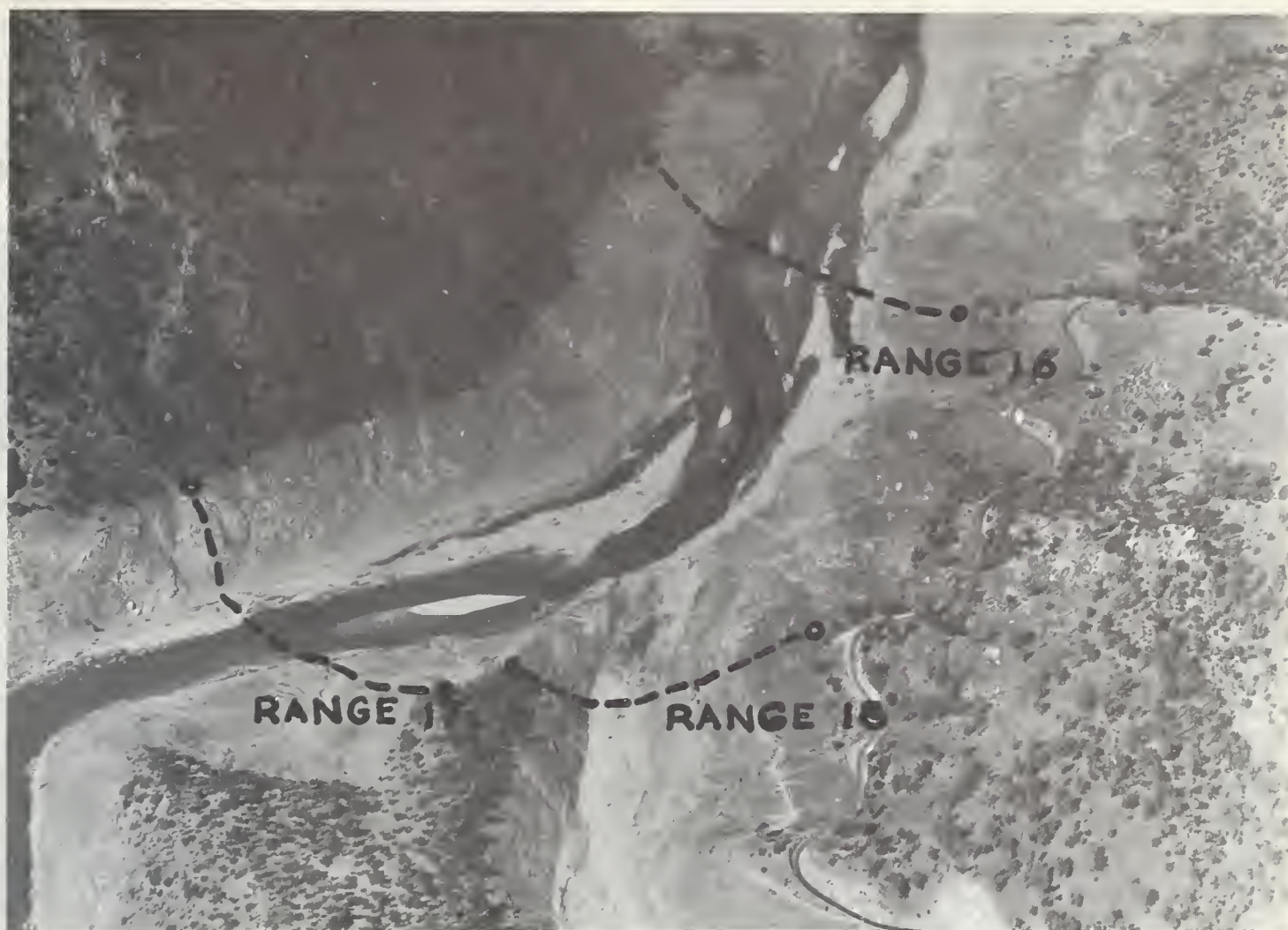
FIGURE 5. — Sediment deposits, ranges 16, 17, 18, Pine Flat Reservoir.
