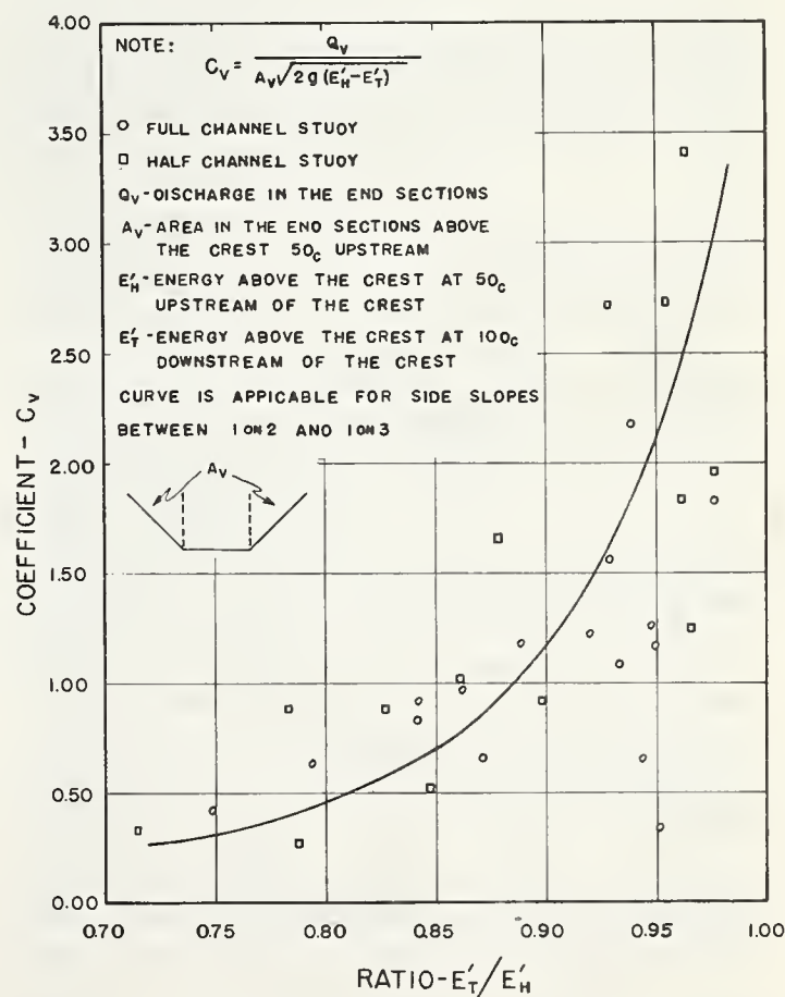
FIGURE 15.—Discharge coefficient for the end sections of a sill in a trapezoidal channel.
