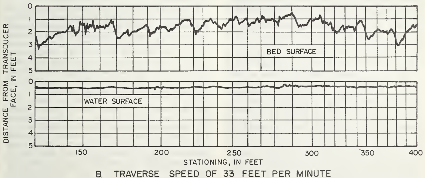
FIGURE 9.—Water- and bed-surface profiles defined by the dual-channel stream monitor. (From Hubbell and Haushild, 1962.)
