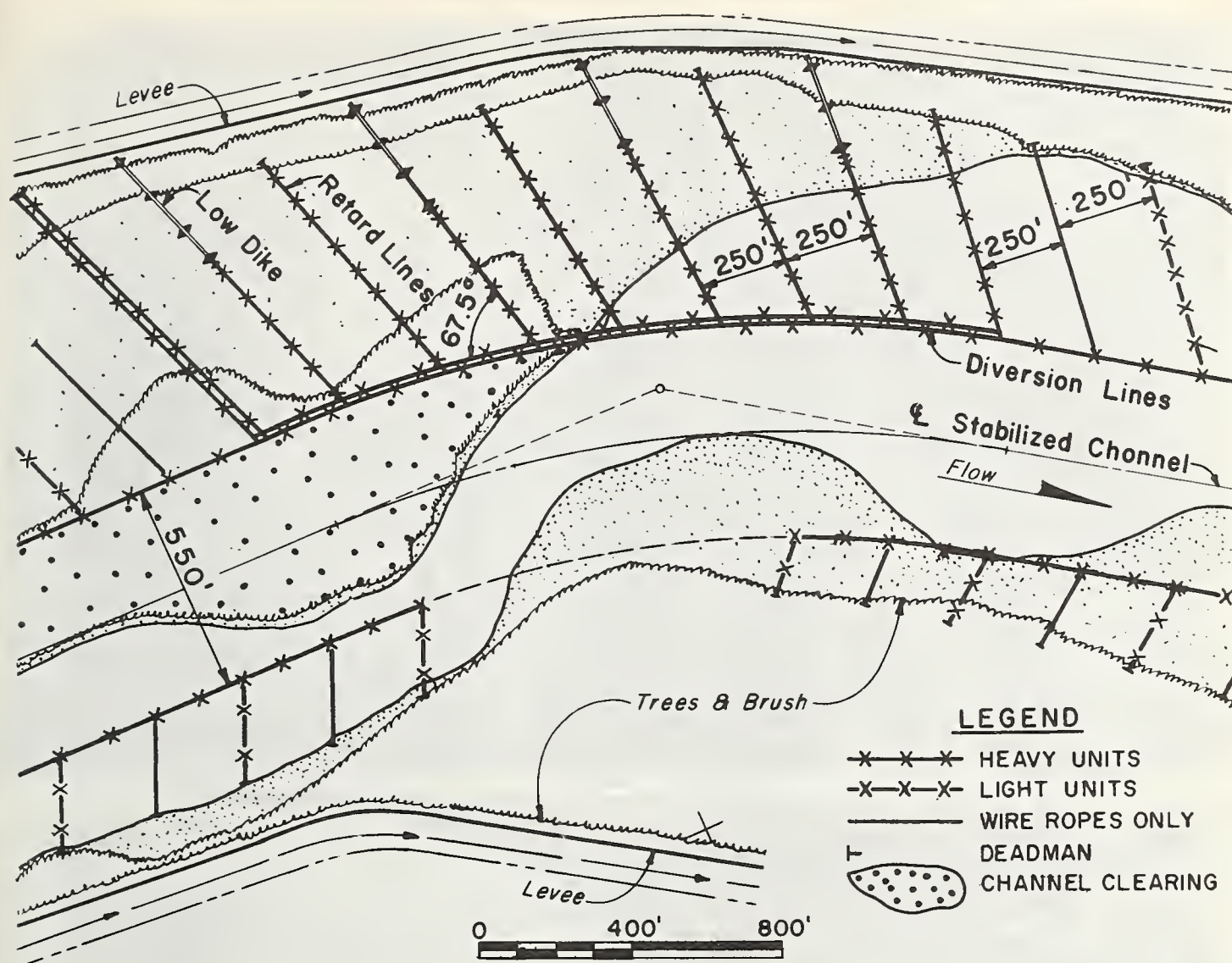
FIGURE 4. — Typical Kellner jetty field—Rio Grande, N. Mex.
