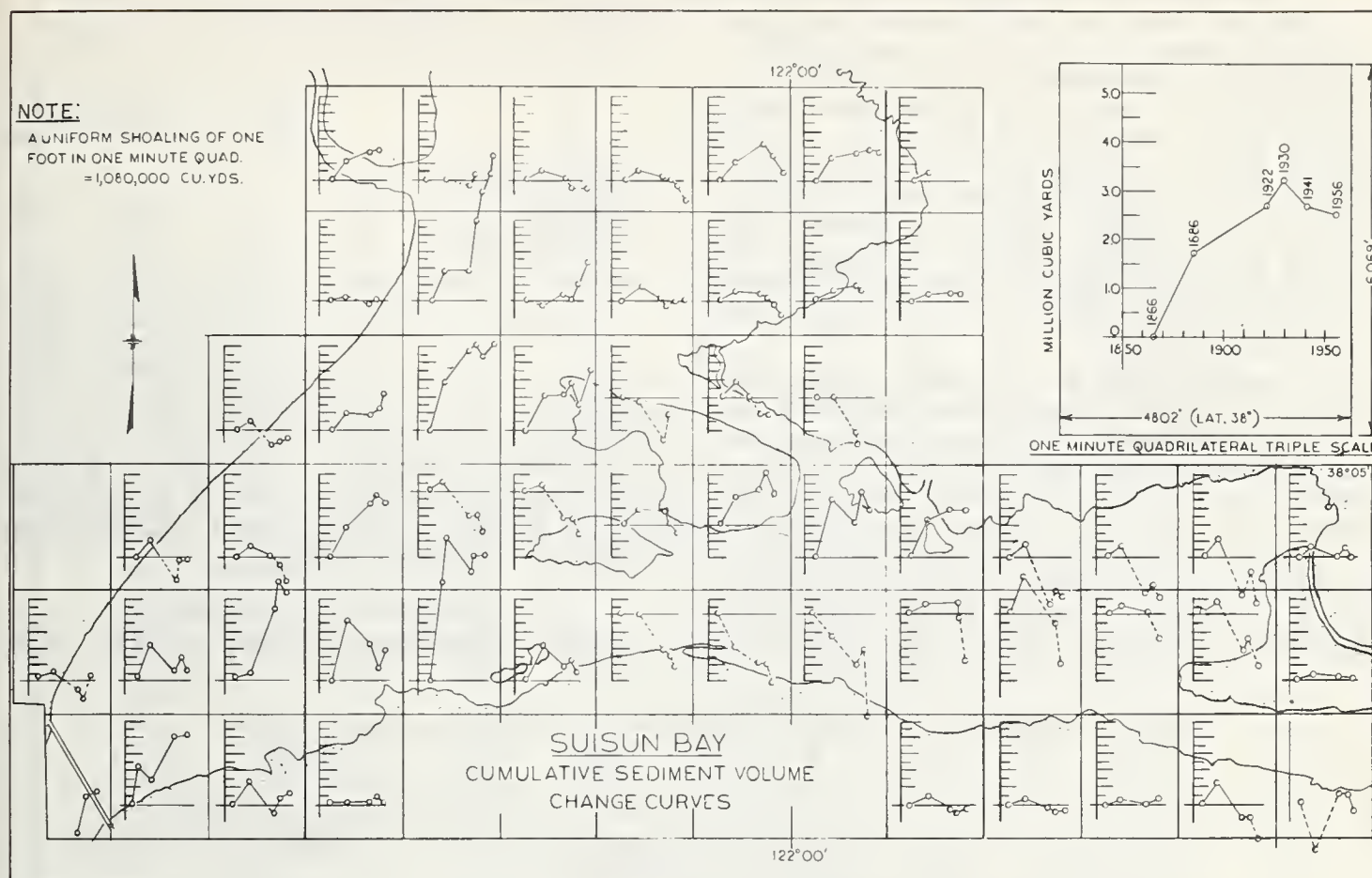
FIGURE 7. — Cumulative sediment volume change curves of Suisun Bay.
