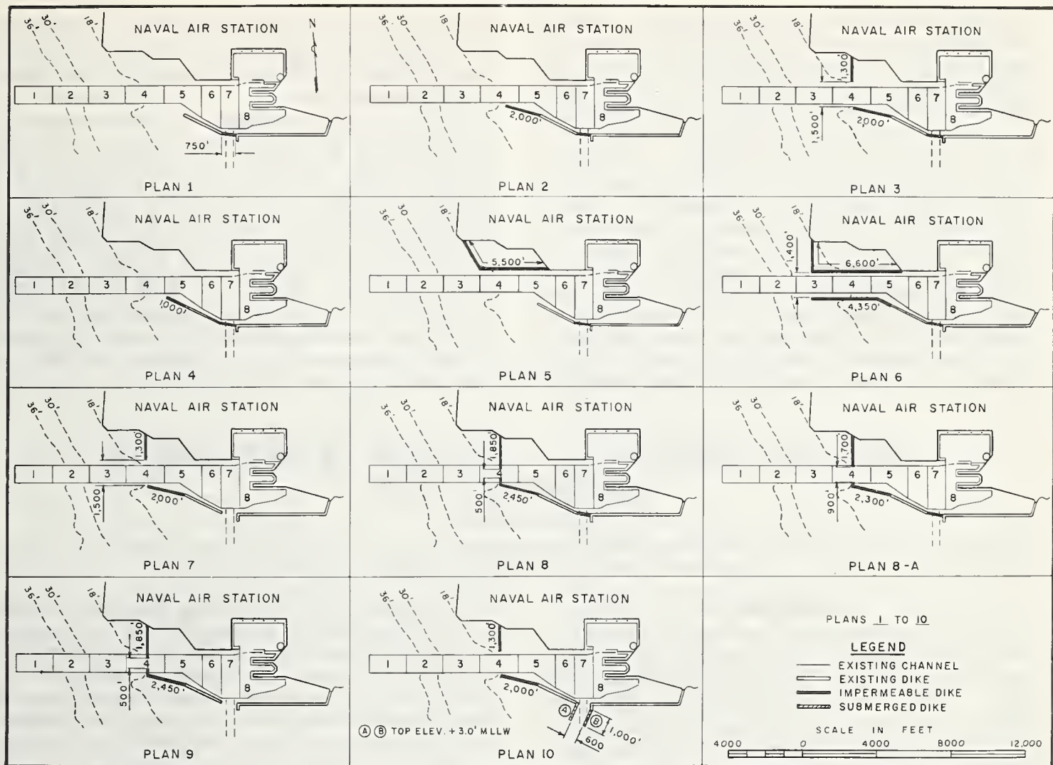
FIGURE 6. — Models of plans 1 to 10, to study shoaling in navigation projects.
