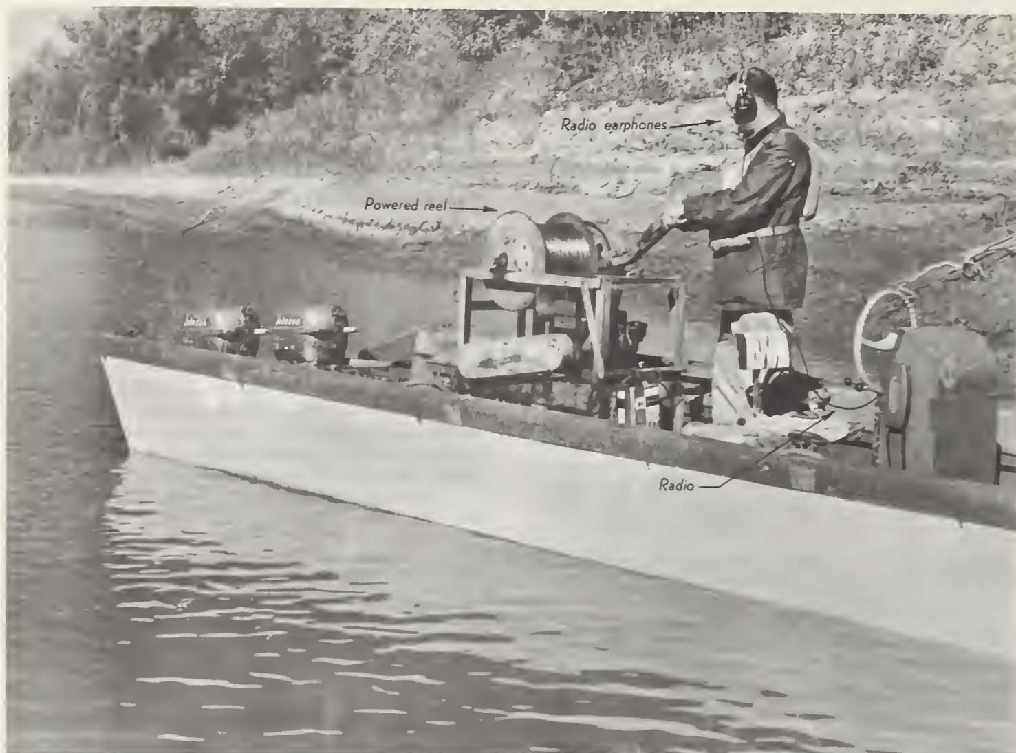
FIGURE 3. — Powered reel for piano wire.
