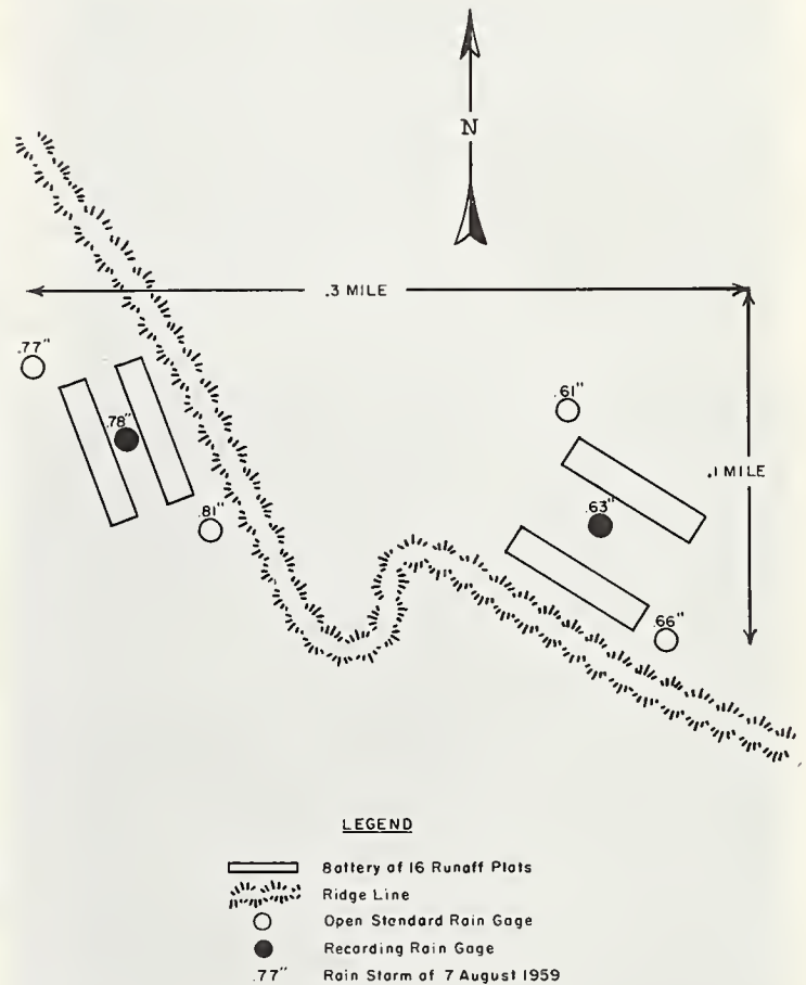
FIGURE 11. — Study layout and location of rain gages. Note the variation in rainfall measured after a single summer rainstorm.
