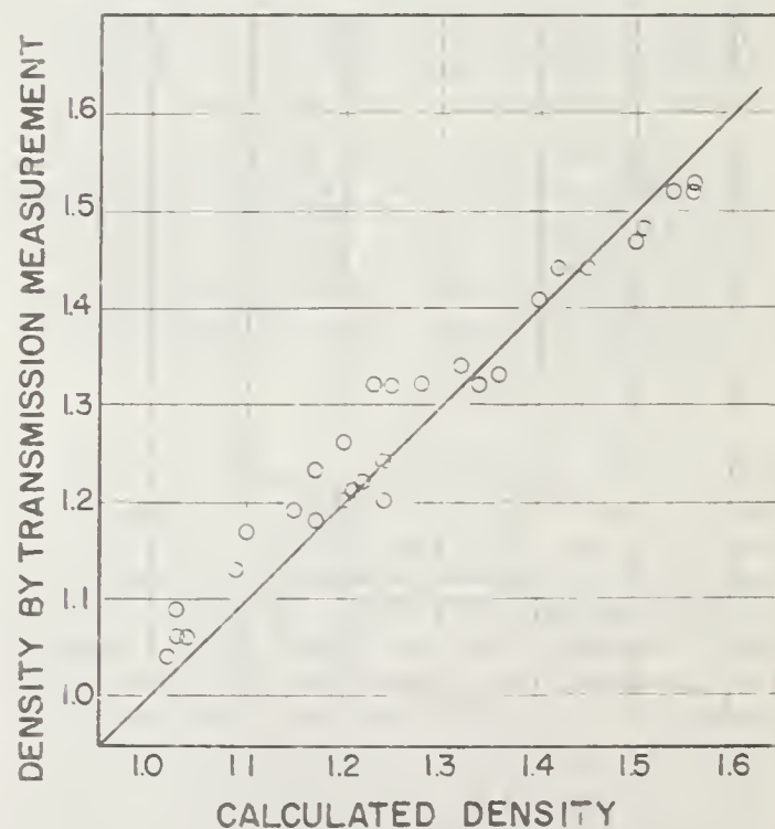
FIGURE 4.—The density of a prepared sediment measured by the dual-probe system plotted as a function of the calculated density. (Specified gravity assumed as 2.65.)
