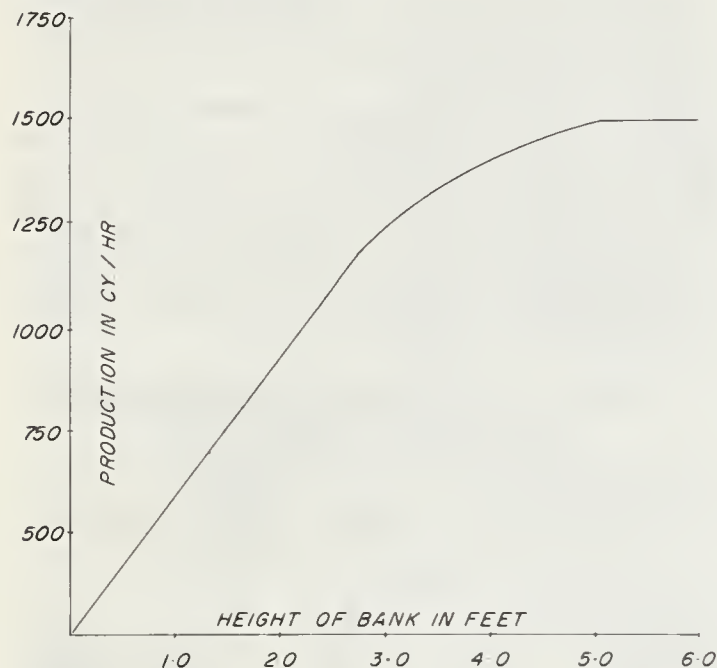
FIGURE 6.—Production curve for 30-inch-pipeline dredge Clackamas pumping through 2,000-3,000 feet of discharge line, Columbia River.
