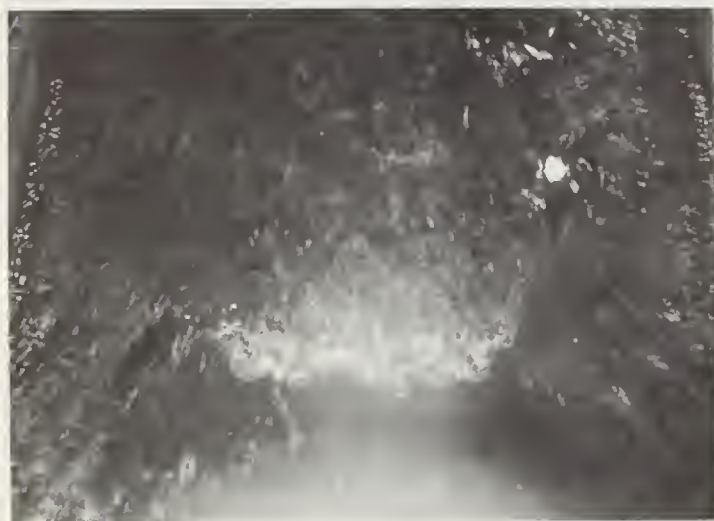
FIGURE 12.—Downstream surface turbulence resulting from the design discharge over the three-dimensional model.
