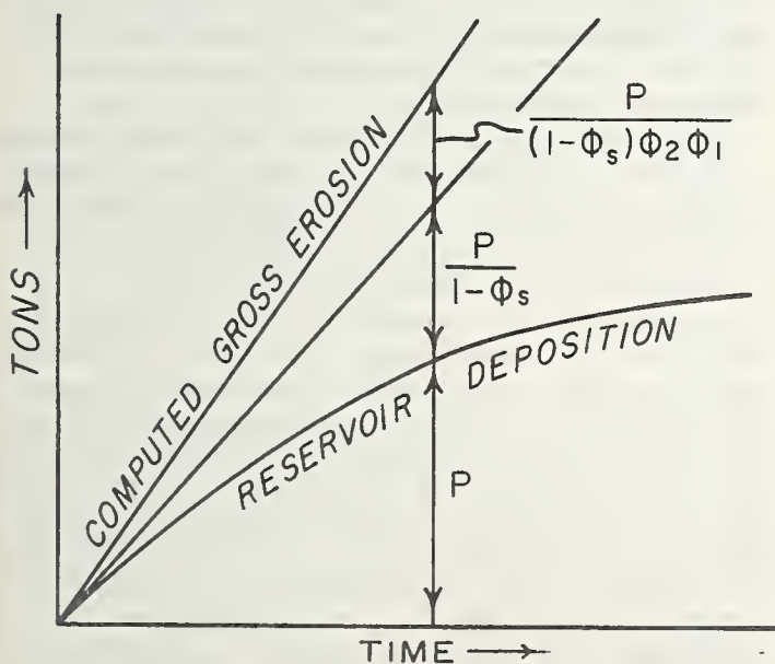
FIGURE 4. — Mass curves of erosion and deposition.
