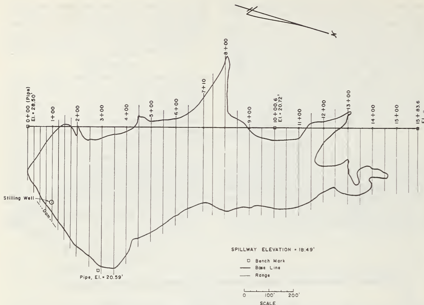
FIGURE 3. — Al Olsen Reservoir, Newell, S. Dak., sedimentation survey, July 1958.
