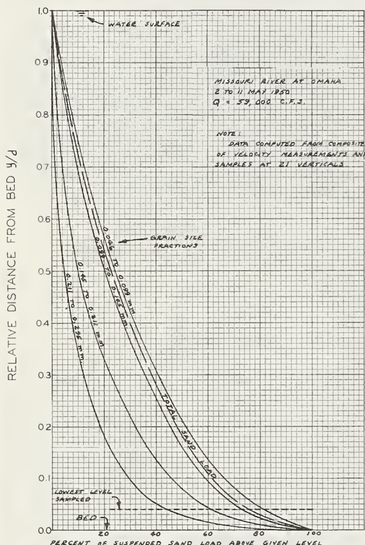
FIGURE 2.— Vertical distribution of suspended sand load in Missouri River.
