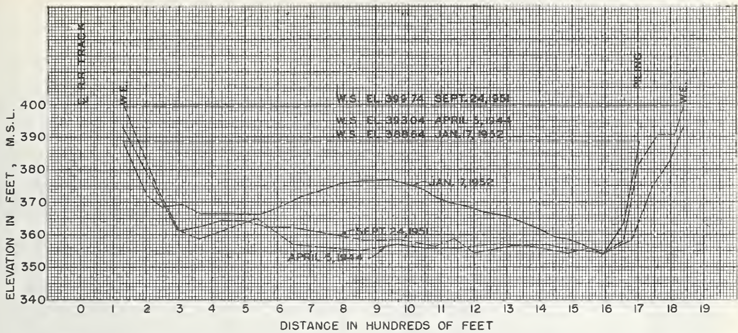
FIGURE 5.— Cross sections of Mississippi River at mile 180.2, prior to and after 1951 flood.
