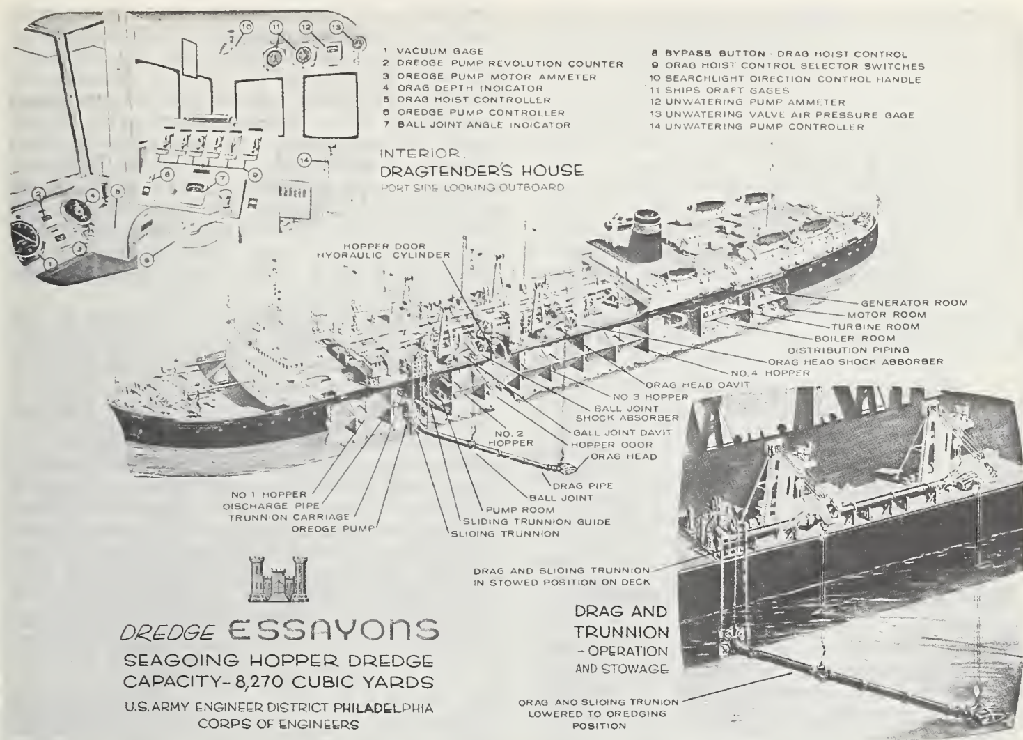
FIGURE 3.—Cutaway view of hopper dredge Essayons .
