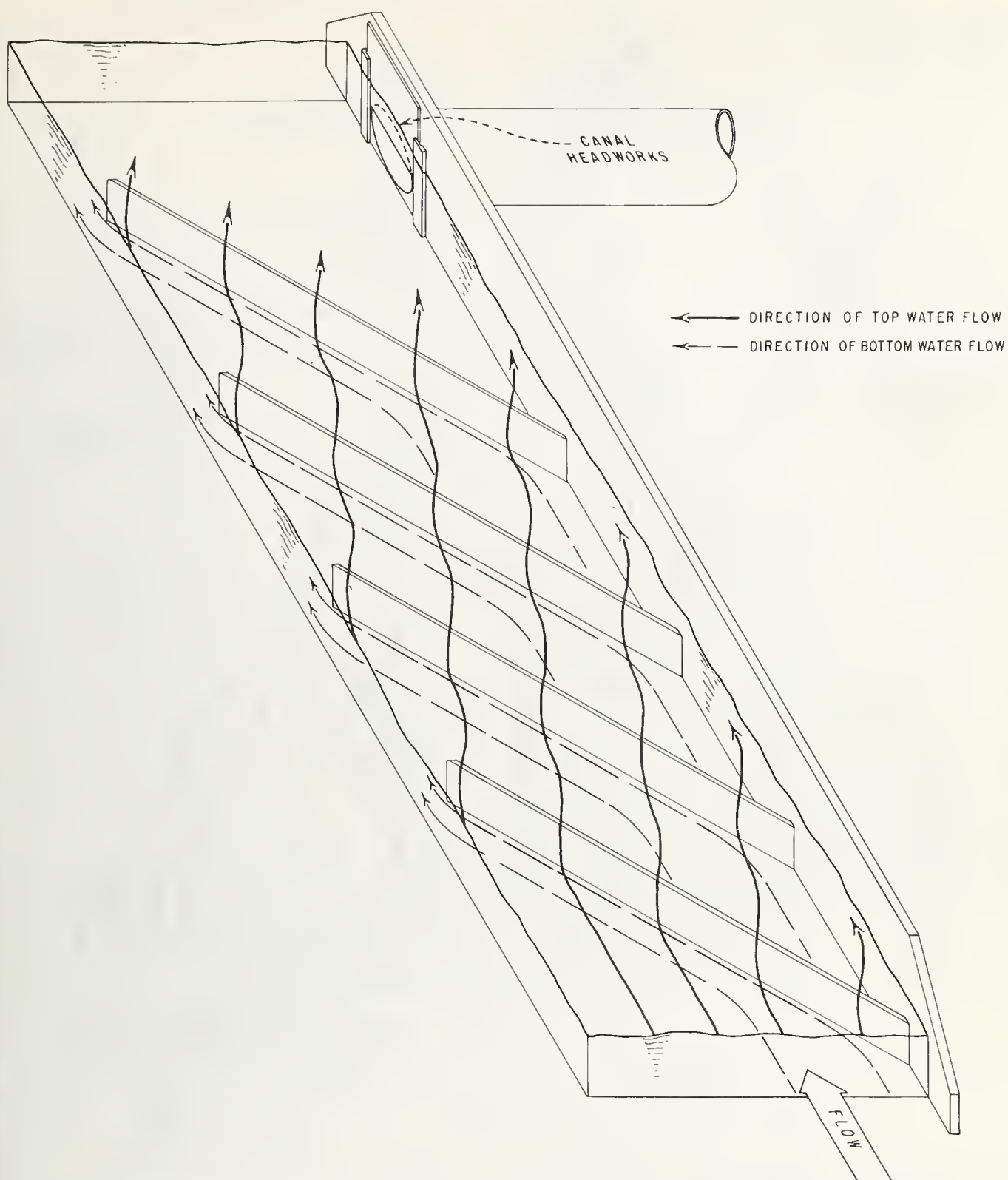
FIGURE 1. — Bottom guide vane method of producing secondary currents for sediment control.
