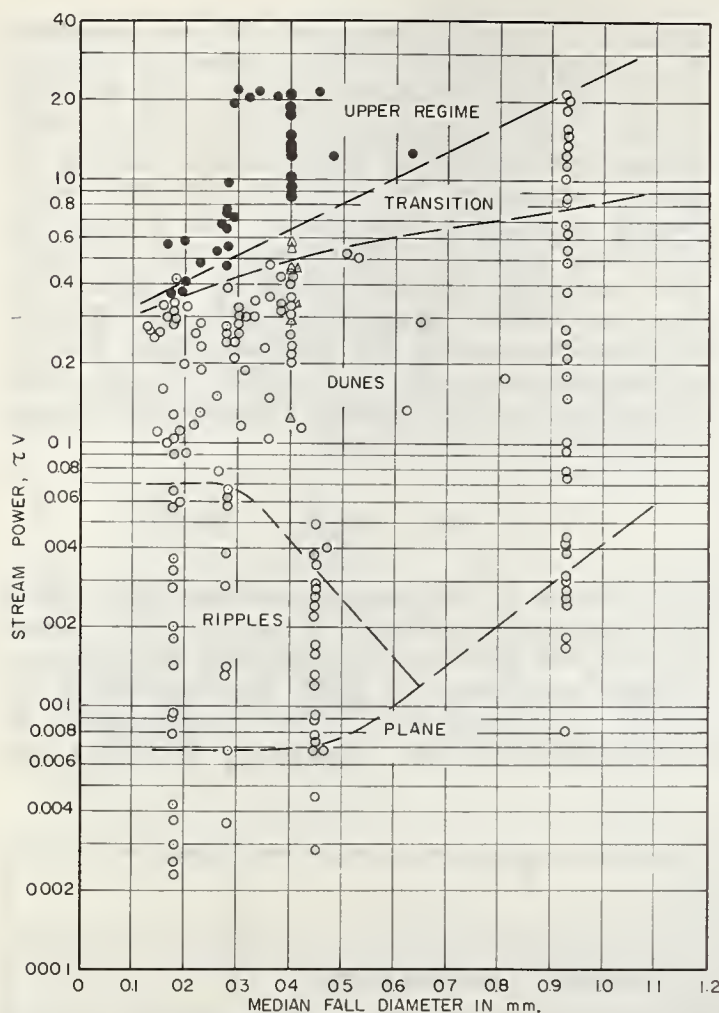
FIGURE 8. — Relation of stream power and median fall diameter of bed material to form of bed roughness.
