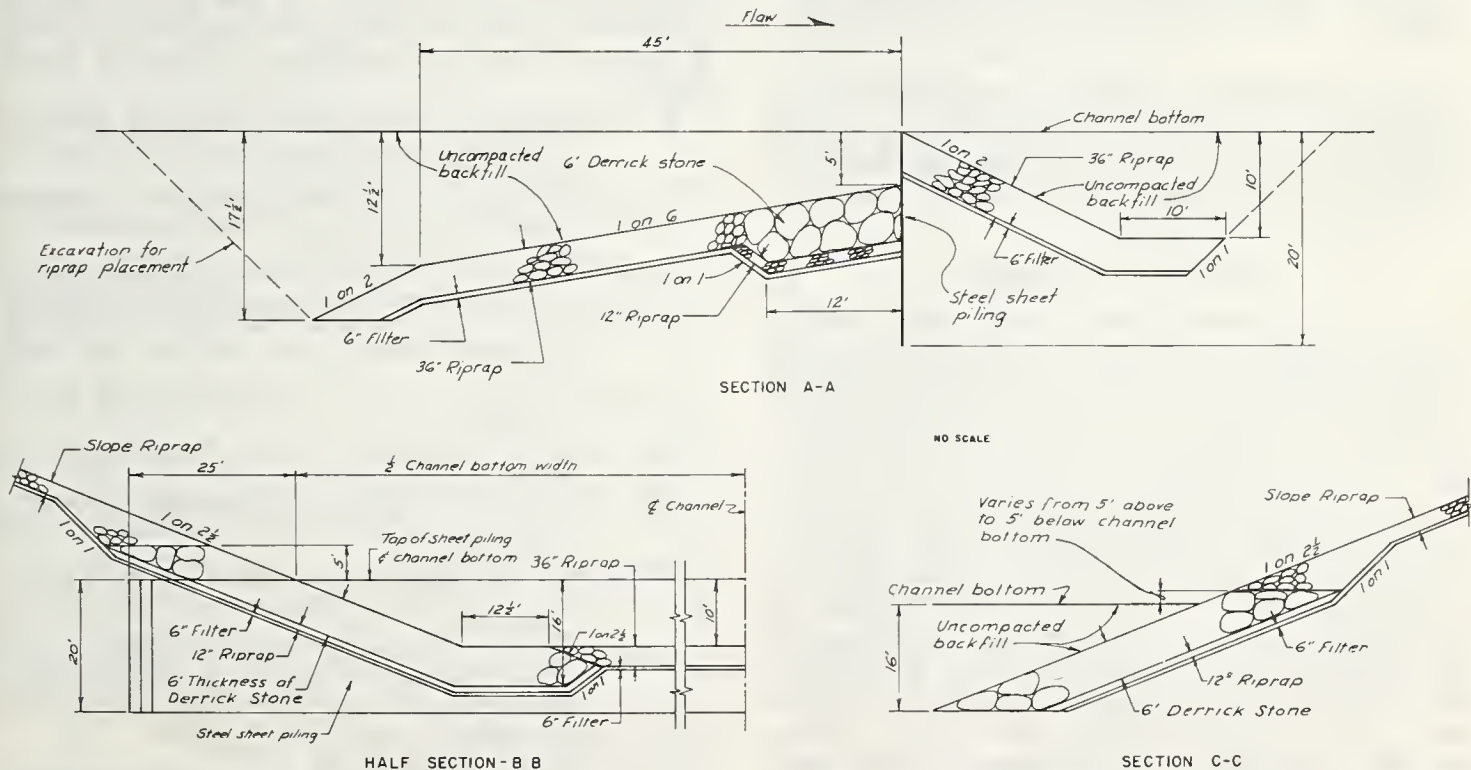
FIGURE 11. — Sectional views of the final sill design.
