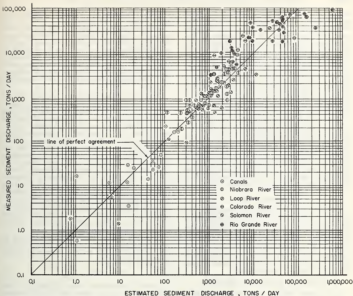
FIGURE 15.— Comparison of bed material load estimated from laboratory curves with measured bed material load.
