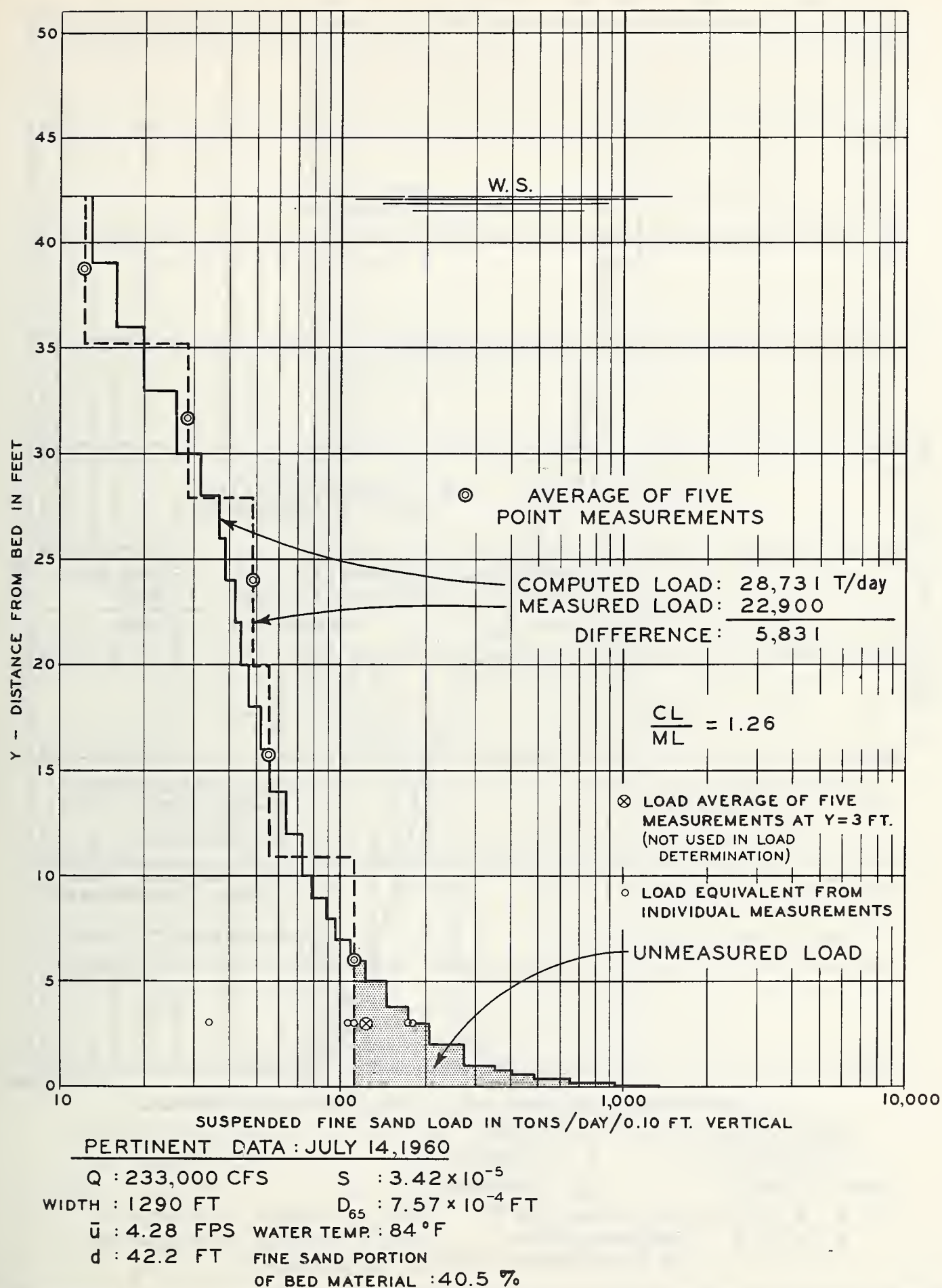
FIGURE 11.— Computed, measured, and unmeasured suspended fine sand load at Simmesport, Atchafalaya River, July 14, 1960.
