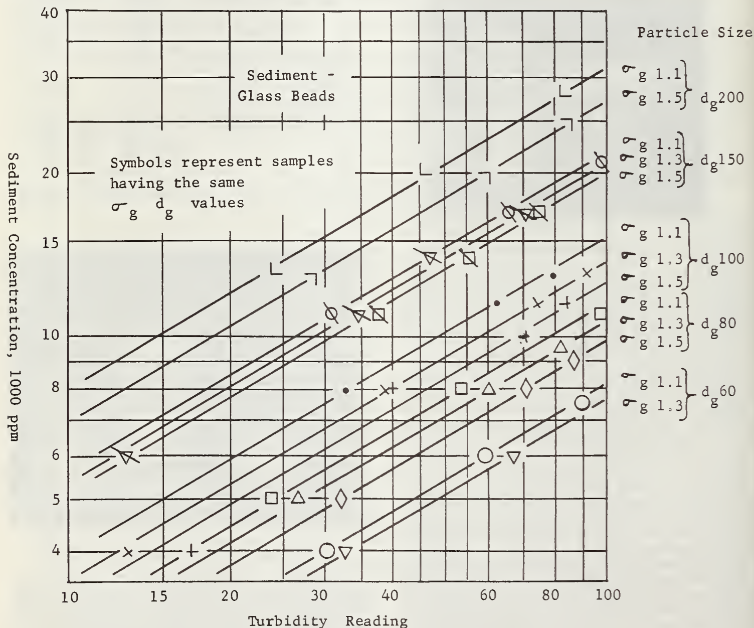
FIGURE 7. — Concentration-turbidity calibration graph.
