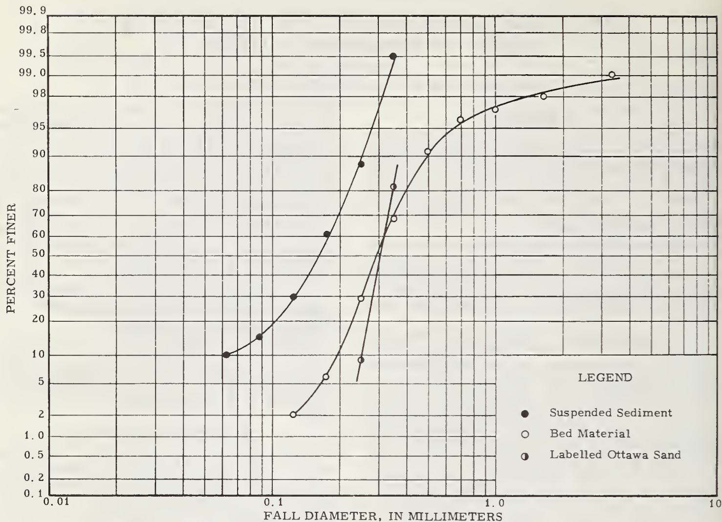
FIGURE 1. — Size distributions of measured suspended sediment, labeled Ottawa sand, and bed material.
