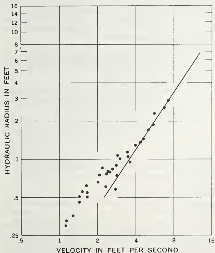
FIGURE 3.—Velocity-hydraulic radius ( V - R ) relation for South Fork Powder River near Kaycee, Wyo.
