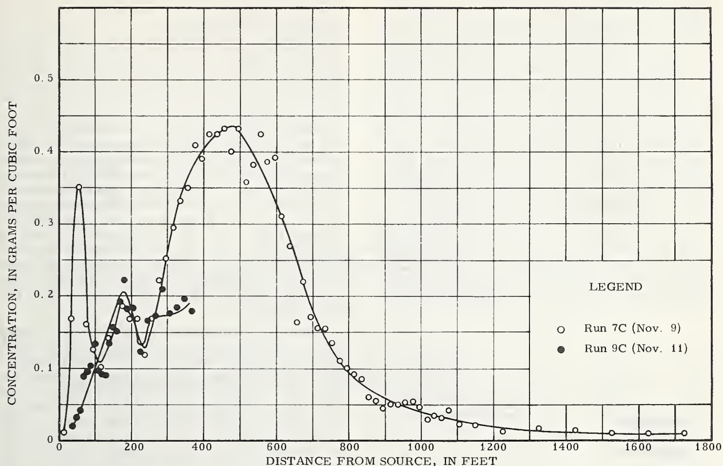
FIGURE 6.—Longitudinal distribution of labeled particles along the center of the channel, Nov. 7 and 9, 1960.
