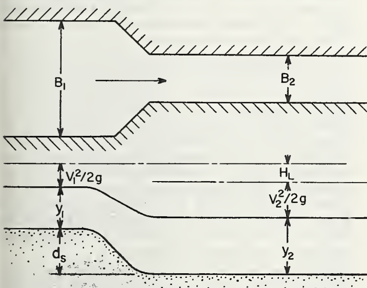
FIGURE 7. — Definition sketch of long contraction.
