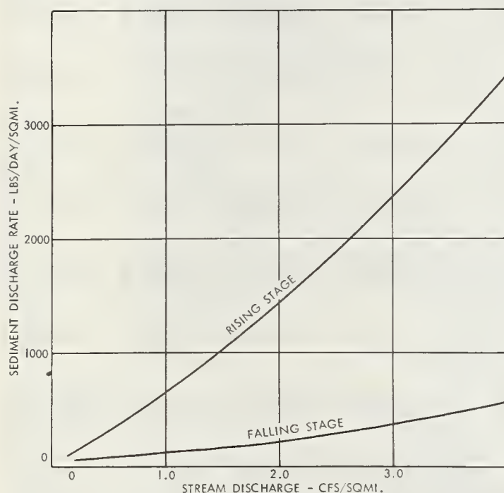
FIGURE 4.—General relation between stream discharge and sediment discharge rate for northern Michigan trout streams.
