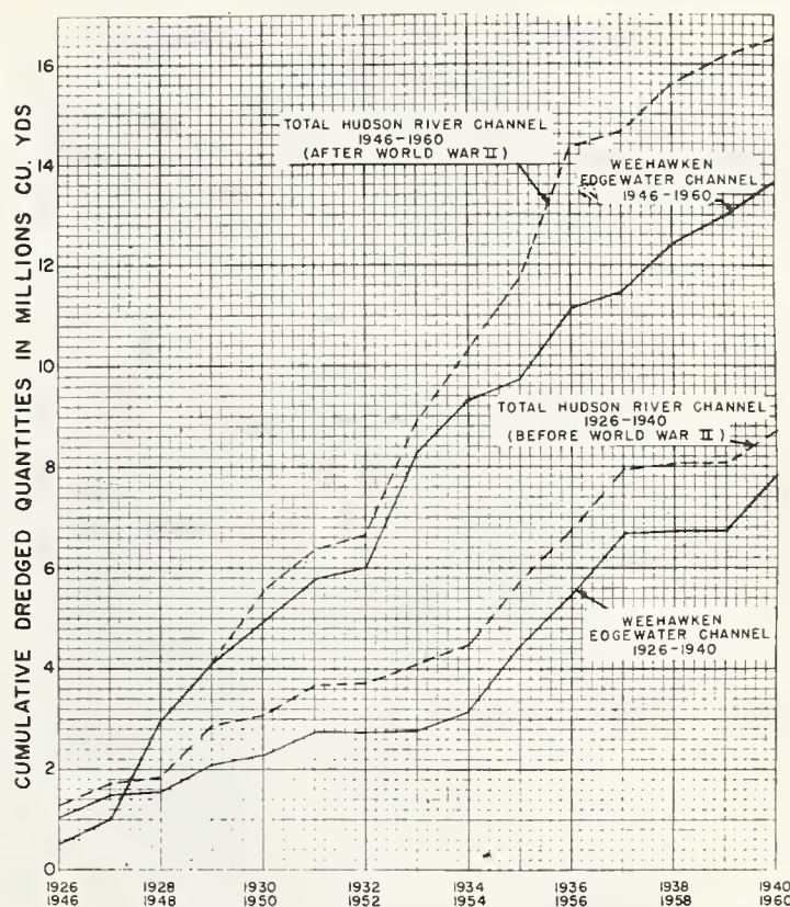
FIGURE 7.—Mass curve of dredged quantities before and after World War II spoil operations, New York Harbor.
