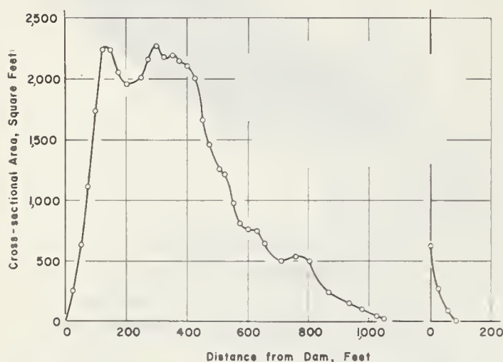
FIGURE 9.—Bertha Armour Reservoir cross-sectional area versus distance from dam.
