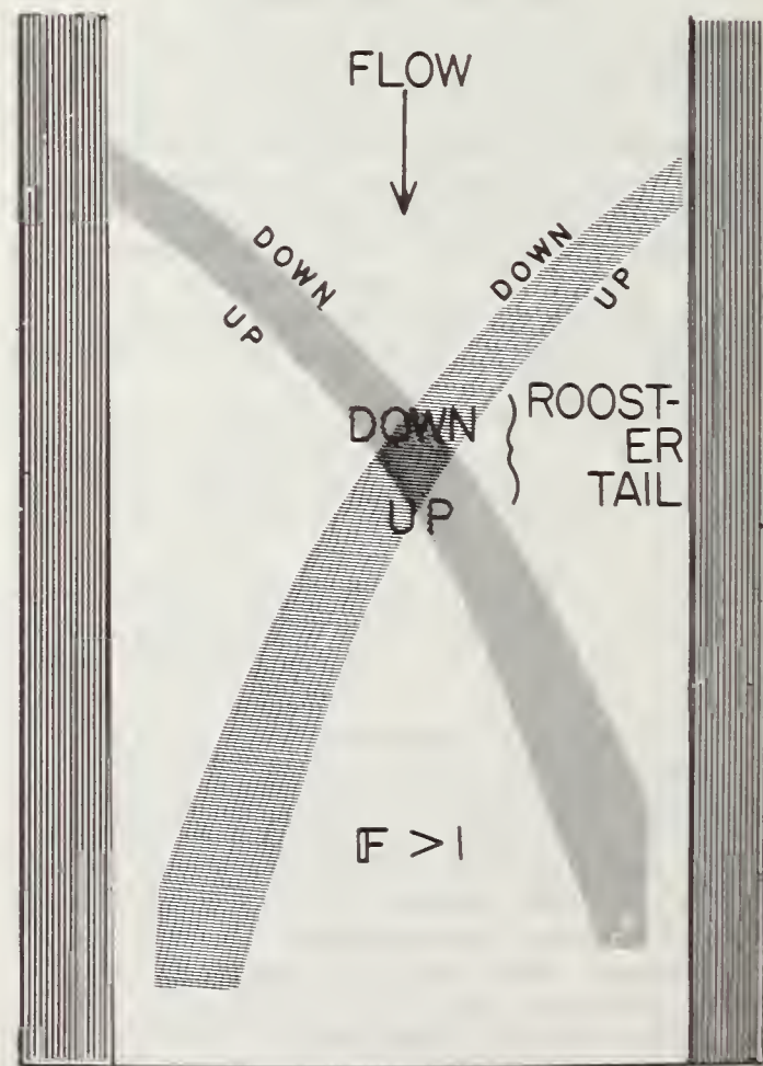
FIGURE 2. — Vortex and wave patterns of streamflow for Froude numbers above 1.
