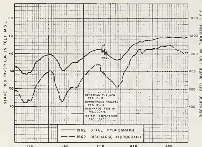
FIGURE 7.—1962 flood: Stage and discharge hydrographs, Mississippi River, Red River Landing, La.
