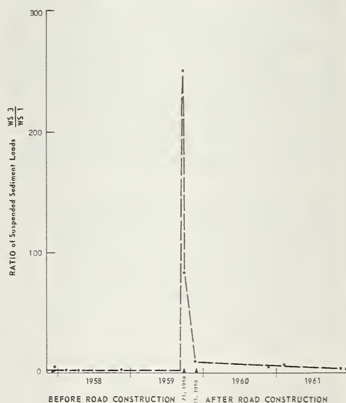
FIGURE 3.—Relative suspended sediment loads near peak flows: Watersheds 1 and 3, before and after road construction.
