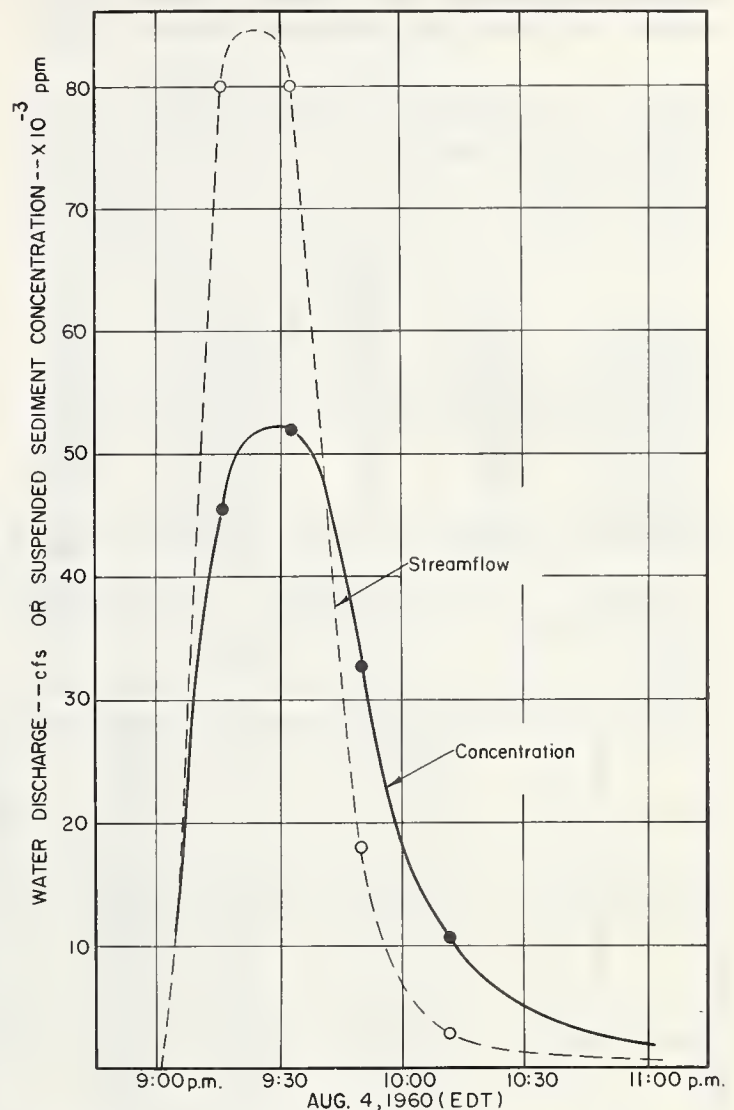
FIGURE 3.—Runoff hydrograph and suspended-sediment concentration graph for storm of August 4, 1960, on a 58-acre area at Kensington, Md.
