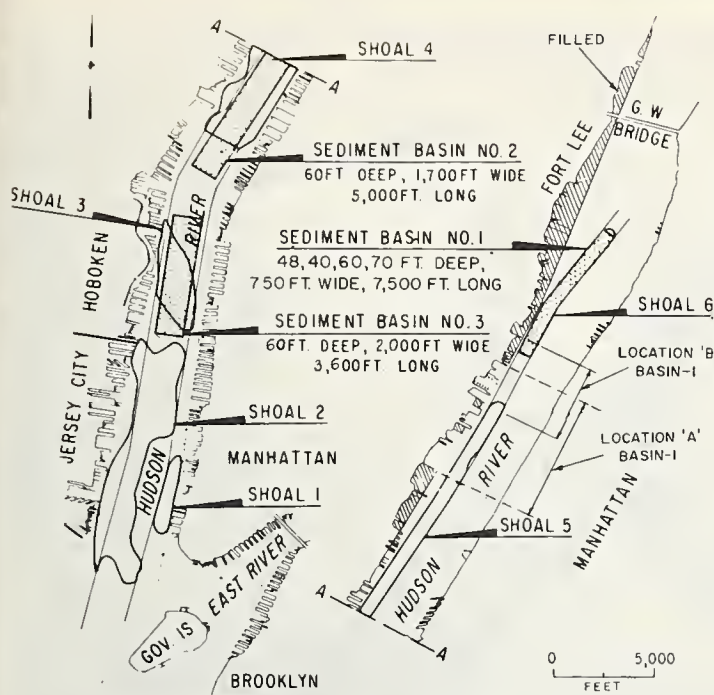
FIGURE 24. — Comprehensive model of basin series.
