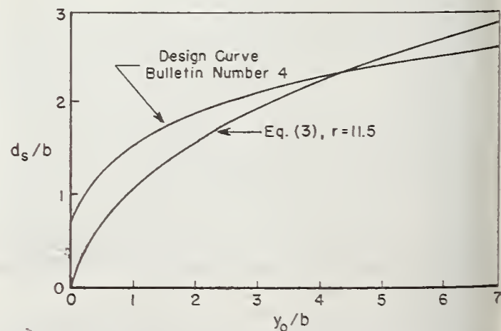
FIGURE 6. — Scour around basic bridge pier.
