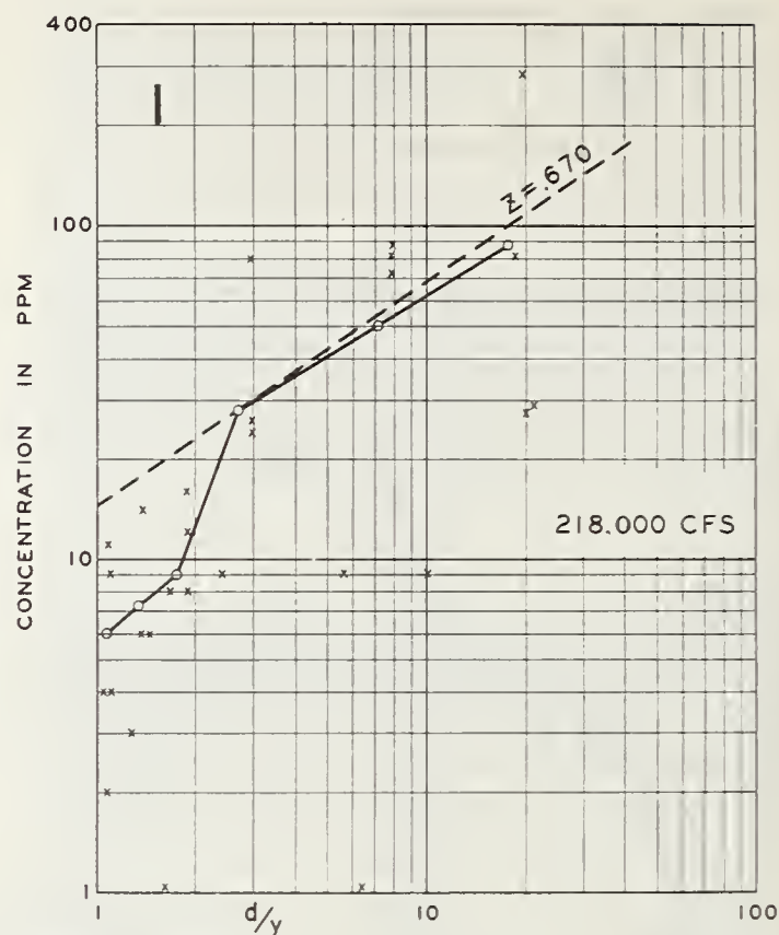
FIGURE 3 (continued).—Measured suspended fine sand at 6 levels at each of 5 verticals in cross section of Atchafalaya River at Simmesport, La.: H, for 233,000 c.f.s.; I, for 218,000 c.f.s.
