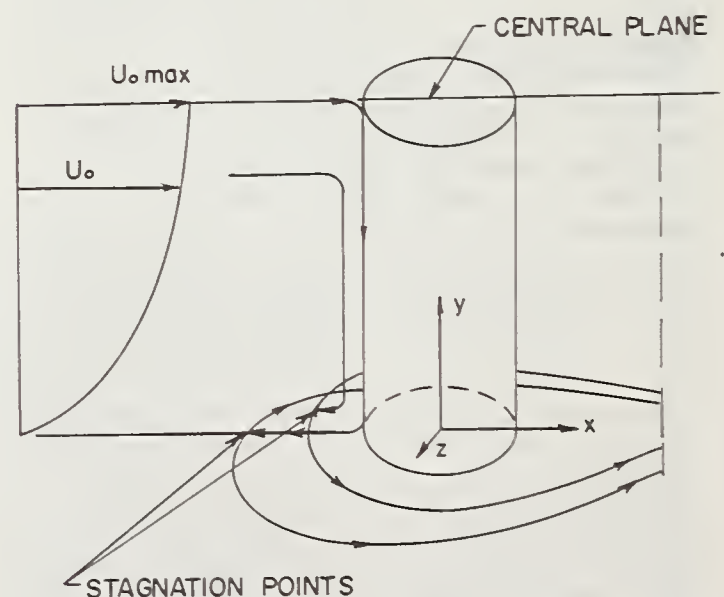
FIGURE 3. — Cylindrical pier with nonuniform approach velocity — rigid bed.
