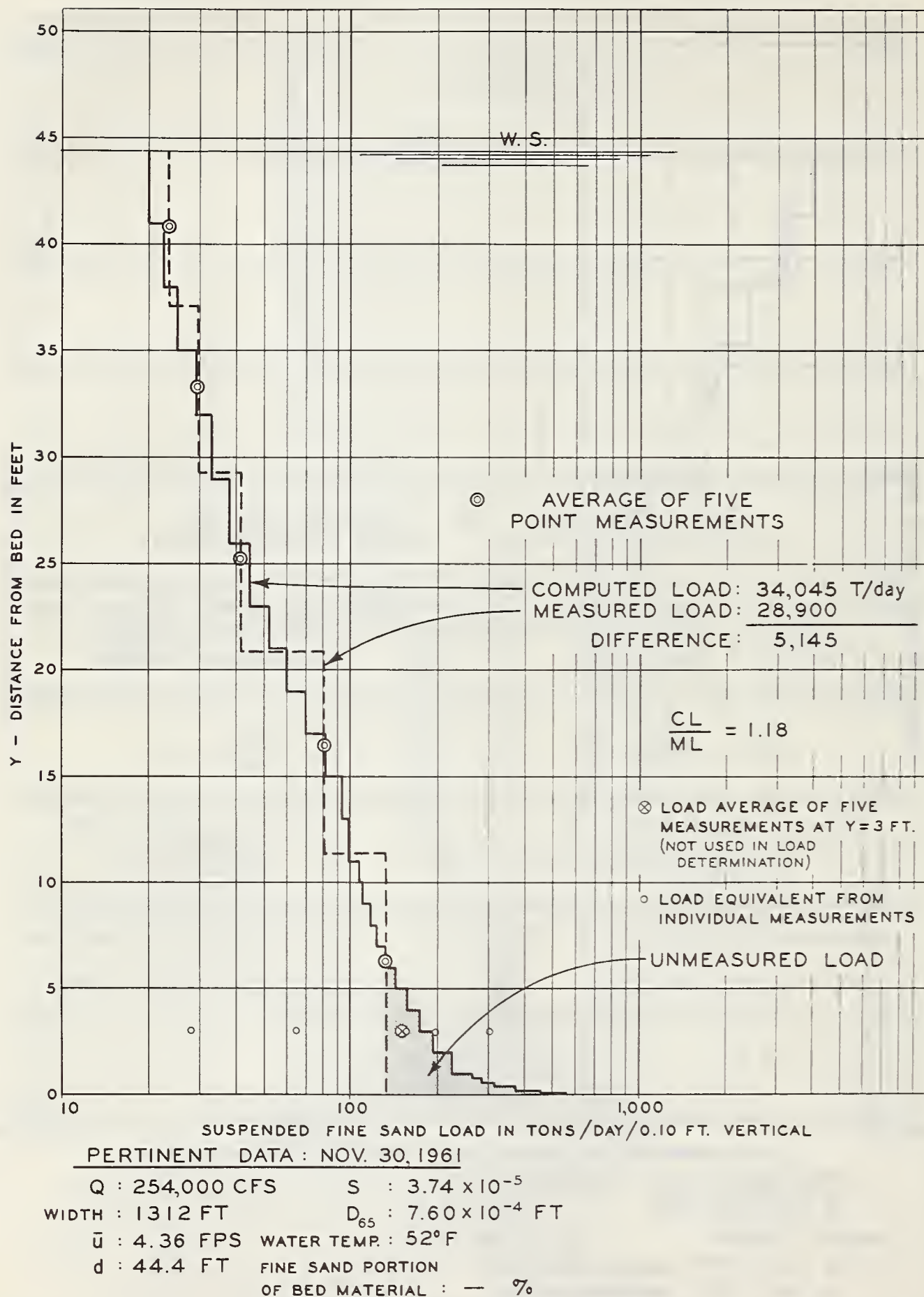
FIGURE 10.— Computed, measured, and unmeasured suspended fine sand load at Simmesport, Atchafalaya River, November 30, 1961.
