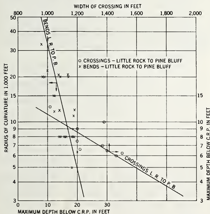
FIGURE 8.—Relations between radius and curvature and maximum depth in bends and between channel width and maximum depth in crossings.
