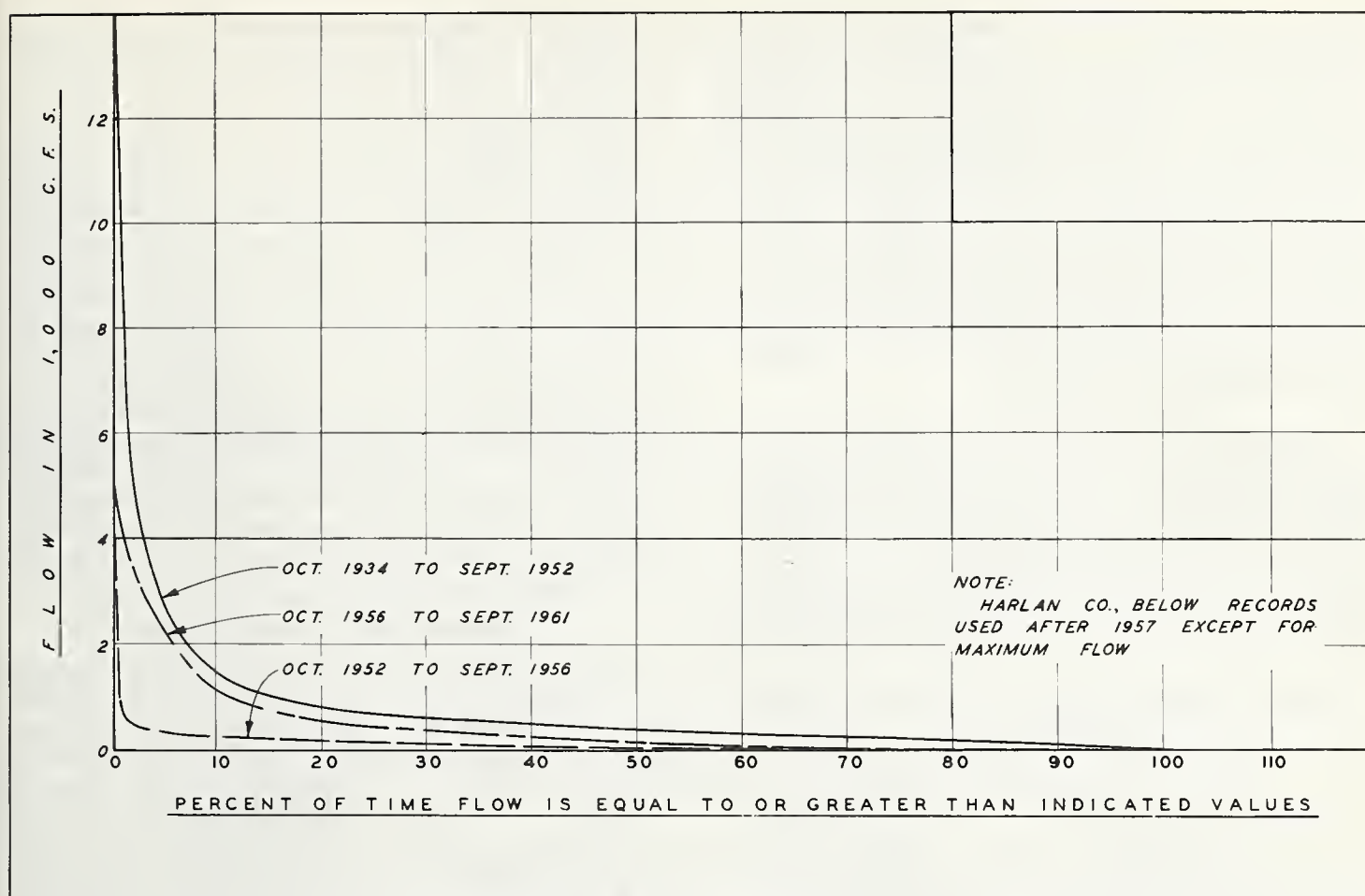
FIGURE 7. — Durations of flow below Harlan County Dam at Bloomington.
