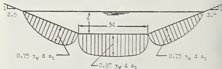
FIGURE 1. — Distribution of actual tractive forces in a trapezoidal channel.
