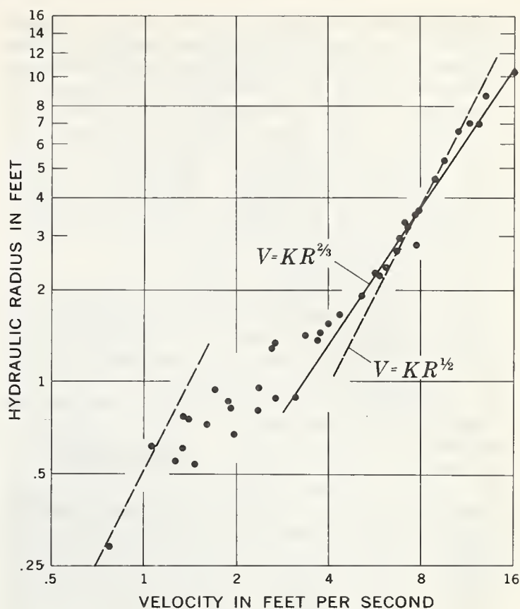
FIGURE 4.—Velocity-hydraulic radius ( V - R ) relation for Canadian River near Logan, N. Mex.
