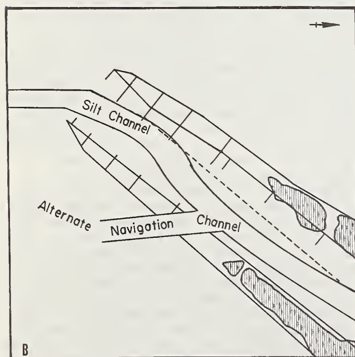
FIGURE 3. — Southwest Pass channel showing (A) improved alignment; and (B) alternate channel.
