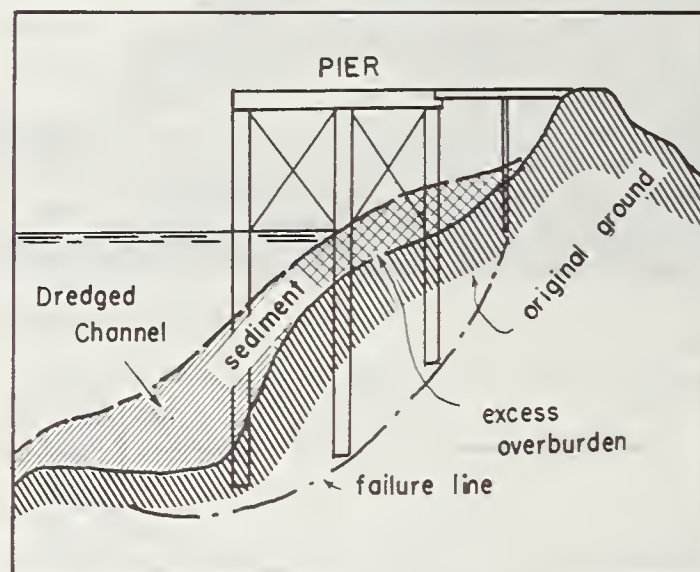
FIGURE 4. — Pier siltation.
