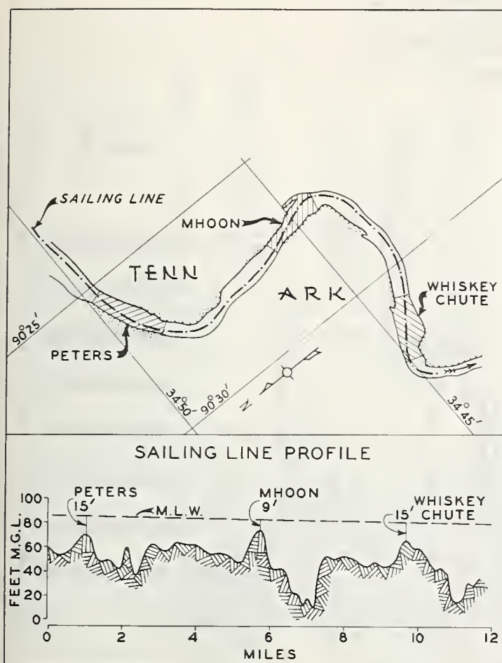
FIGURE 2. — Typical crossing.
