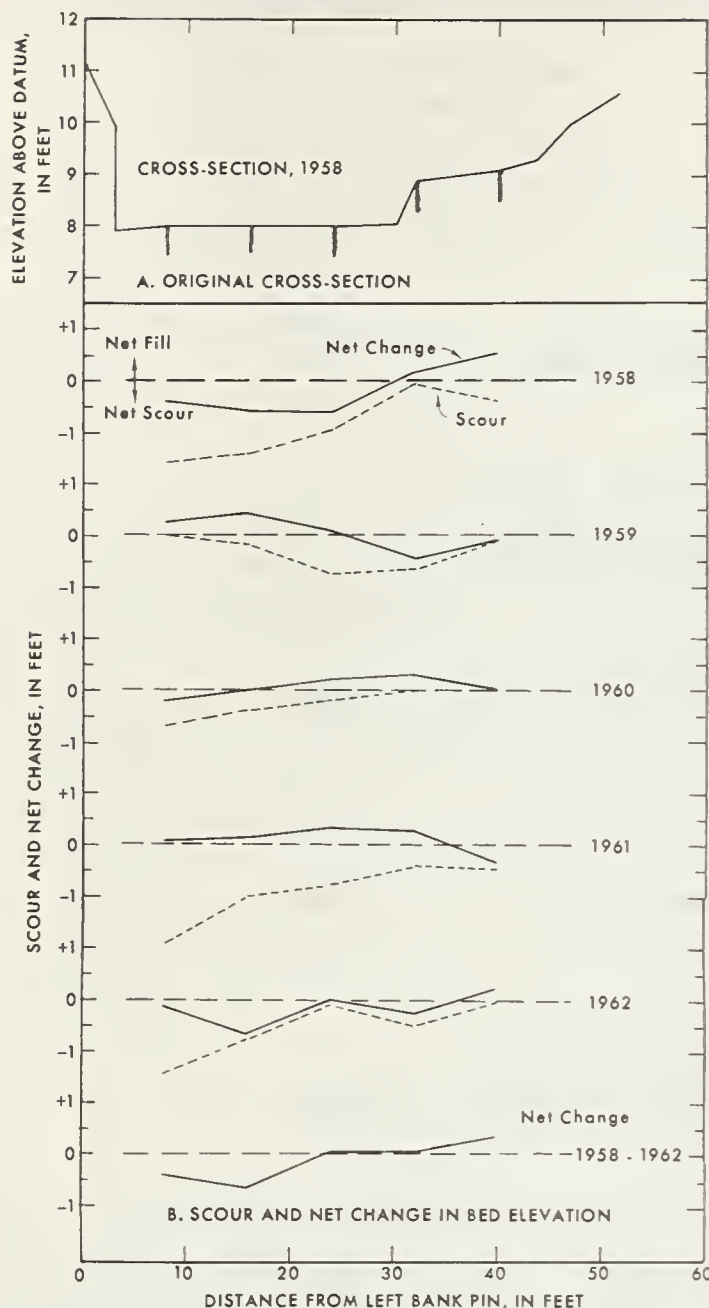
FIGURE 4.—Scour and net change in bed elevation at stationing 9,700 feet for a 5-year period.
