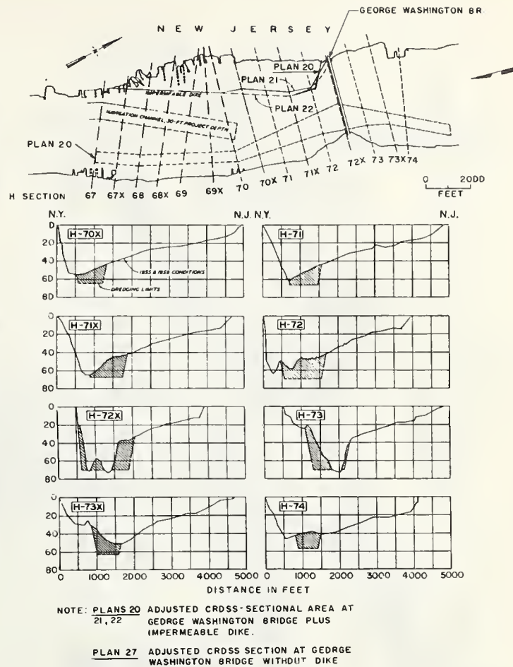
FIGURE 29.—Comprehensive model of George Washington Bridge series.
