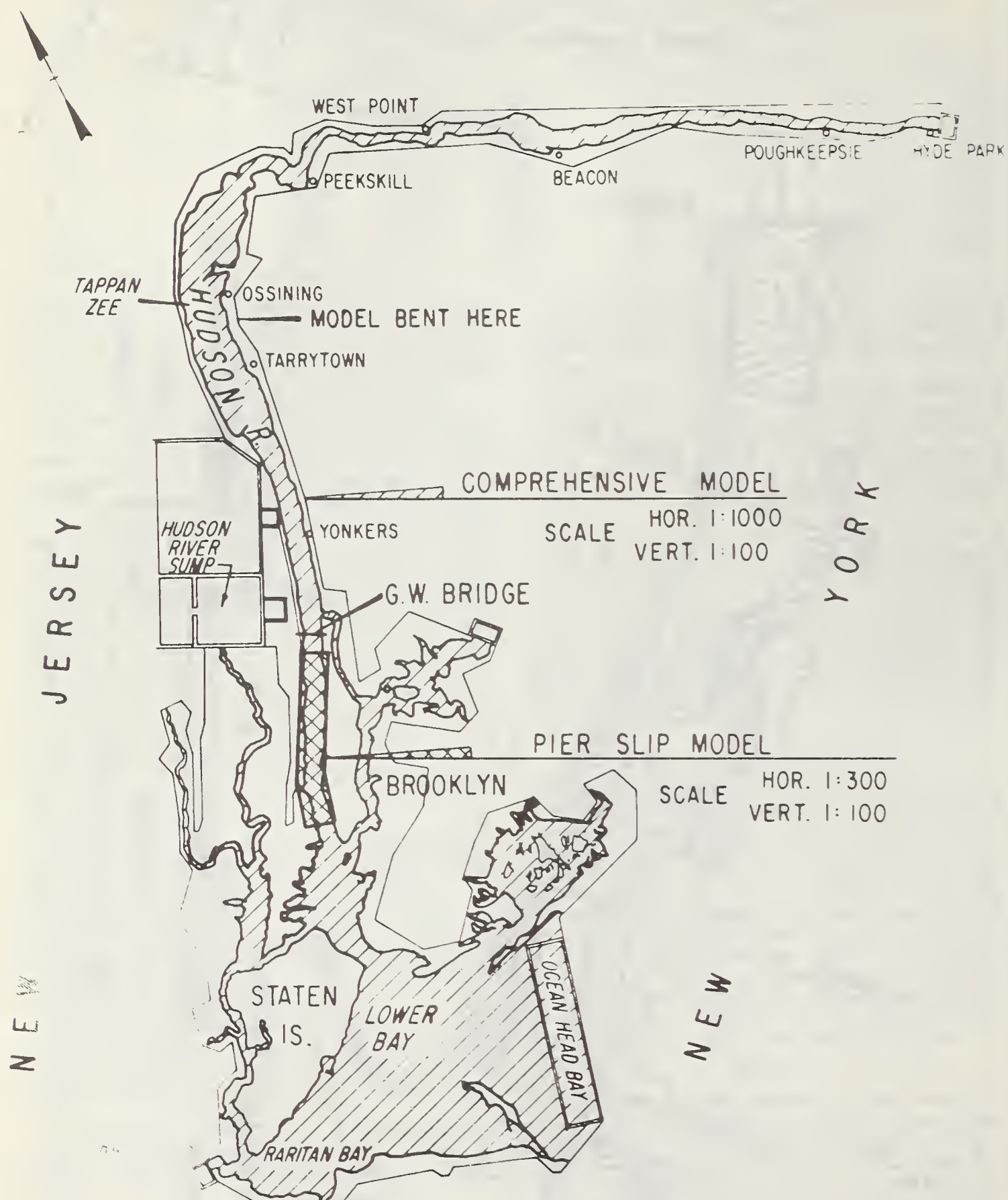
FIGURE 21. — Lower Hudson River model layouts.
