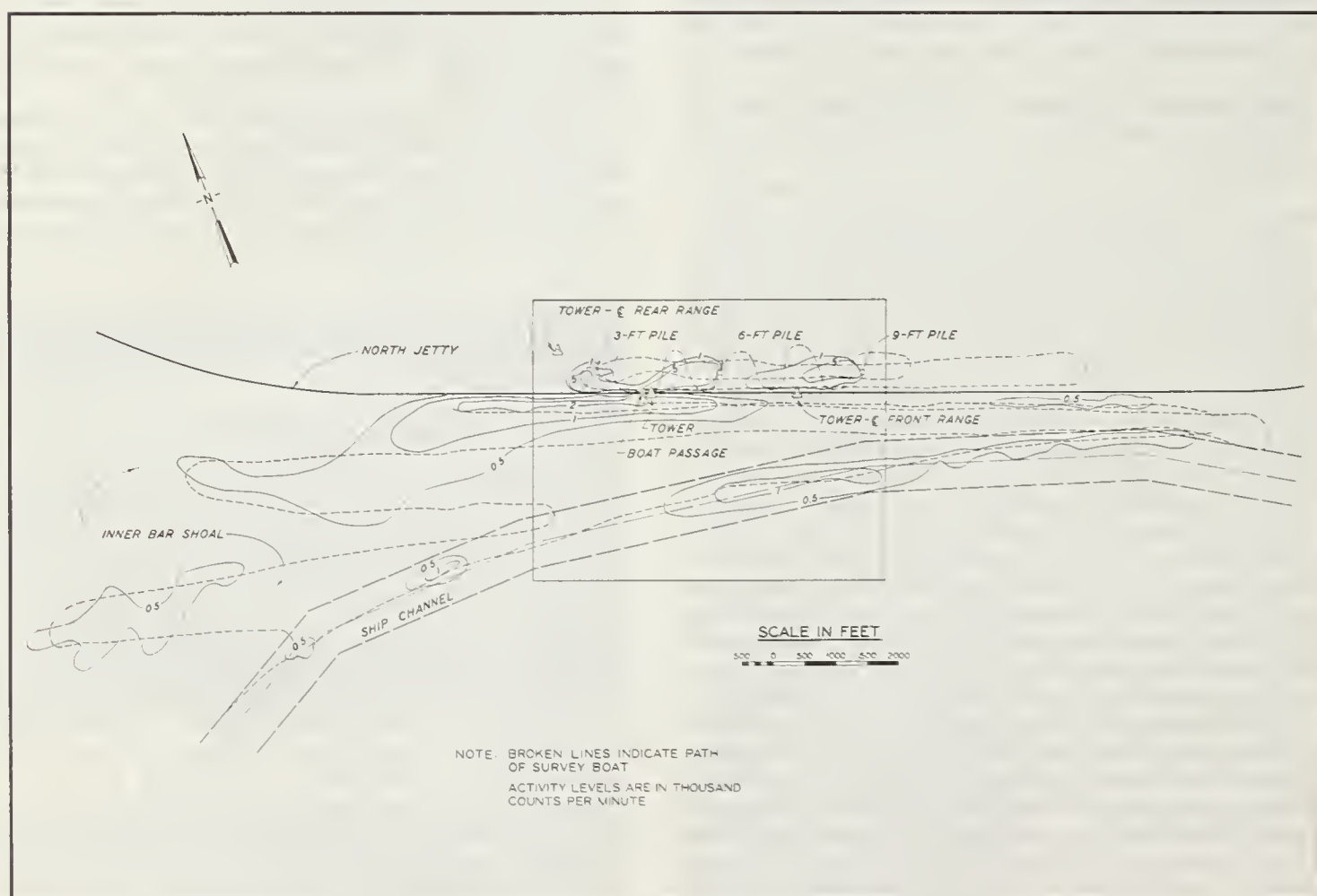
FIGURE 7. — Radioactivity contours on 10 June 1961; Galveston tracer tests.
