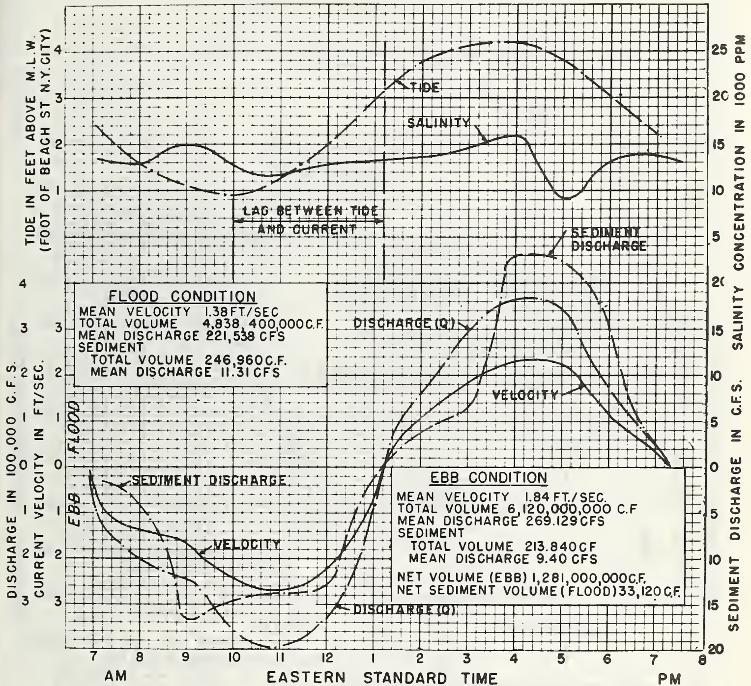
FIGURE 18. —Variation in average velocity, salinity, and sediment, range A, 23 April 1957.
