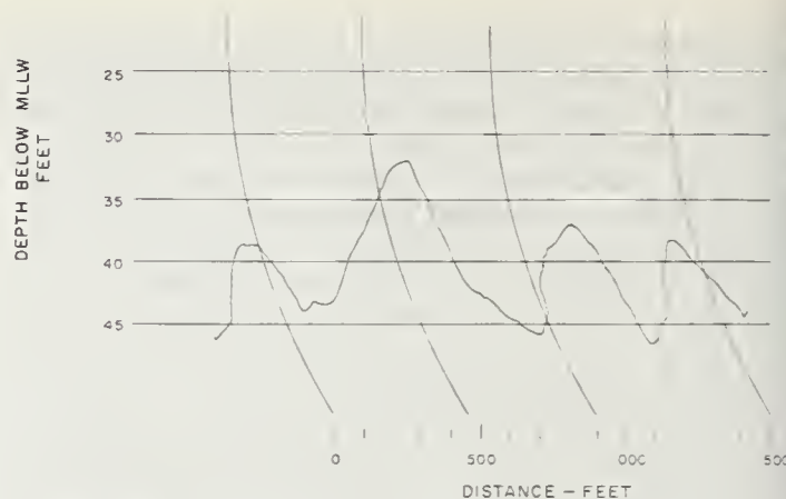
FIGURE 7.—Fathogram along centerline navigation channel, showing sand wave shoaling.
