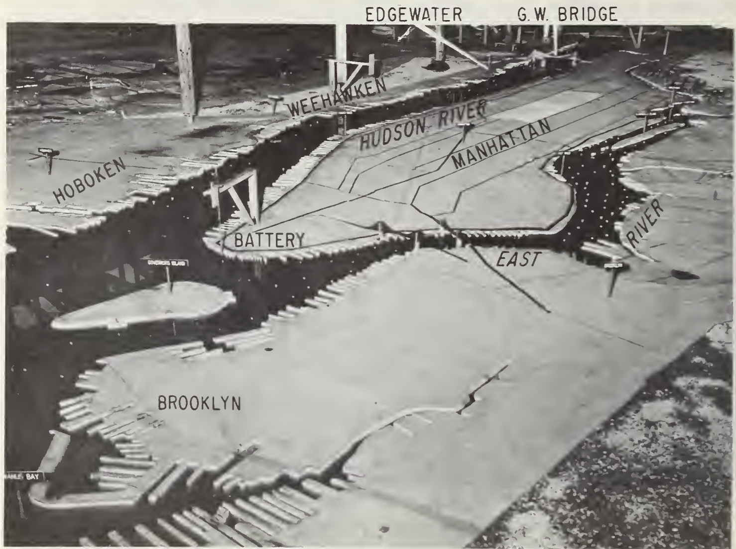
FIGURE 23. —Photograph of comprehensive model, lower New York Harbor.
