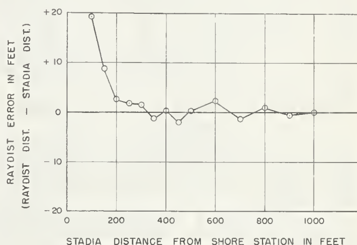
FIGURE 10.—Raydist error when master station is operating near shore station.
