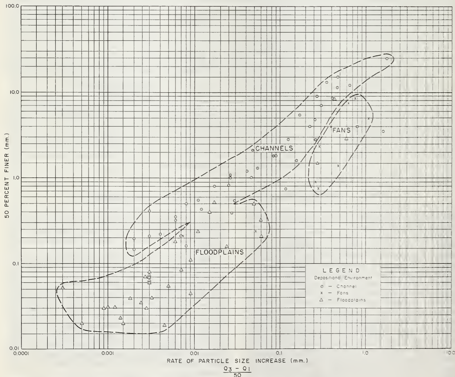
FIGURE 2. — Relationship of particle size increase to size of which 50 percent is finer.
