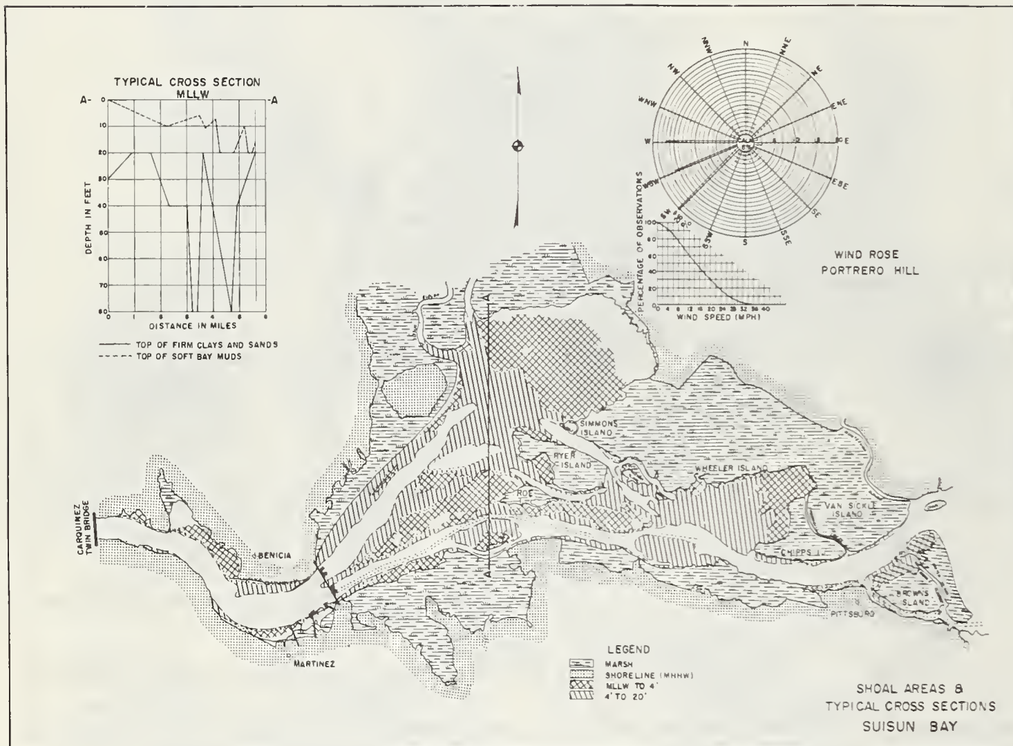
FIGURE 18. — Shoal areas, wind roses, and typical cross section of Suisun Bay.
