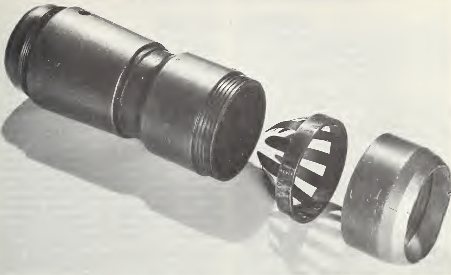
FIGURE 6. — Basket shoe assembly, Swedish Foil Sampler.
