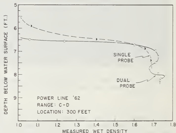
FIGURE 7.—A depth-density profile of a sediment as measured by a gamma and a dual probe: Range C-D, 300 feet, Power Line Reservoir, Lafayette County, Miss.
