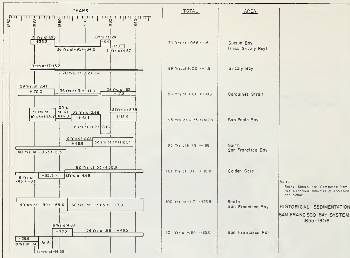
FIGURE 20. — History of sedimentation in San Francisco Bay system, 1855-1956.
