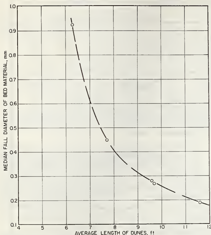
FIGURE 2.—Relation of length of dunes to median fall diameter of bed material.
