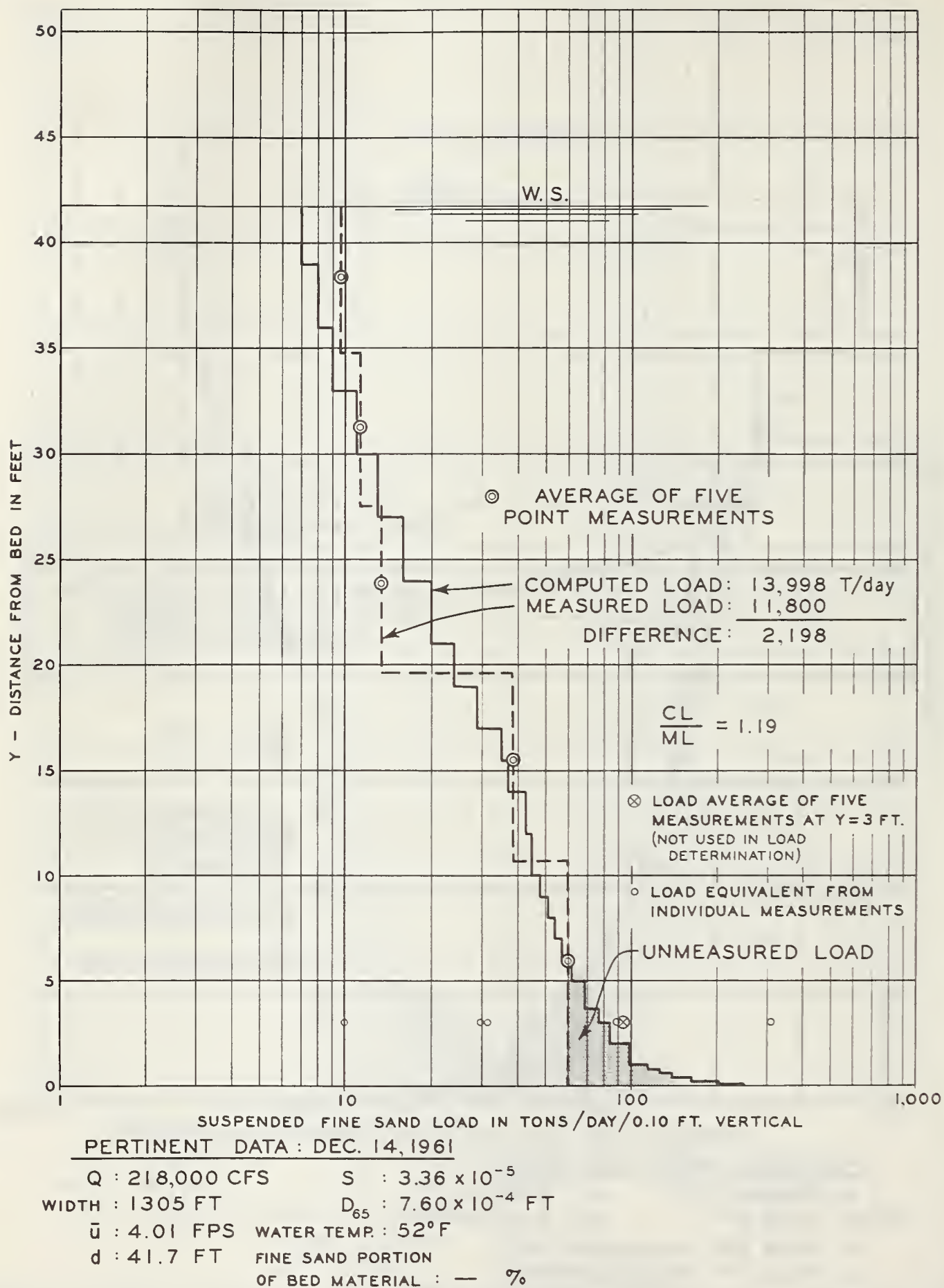
FIGURE 12. — Computed, measured, and unmeasured suspended fine sand load at Simmesport, Atchafalaya River, December 14, 1961.
