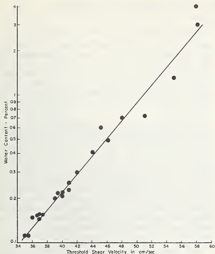
FIGURE 17.—Variation of the threshold shear velocity with moisture content (from figs. 12 and 16).
