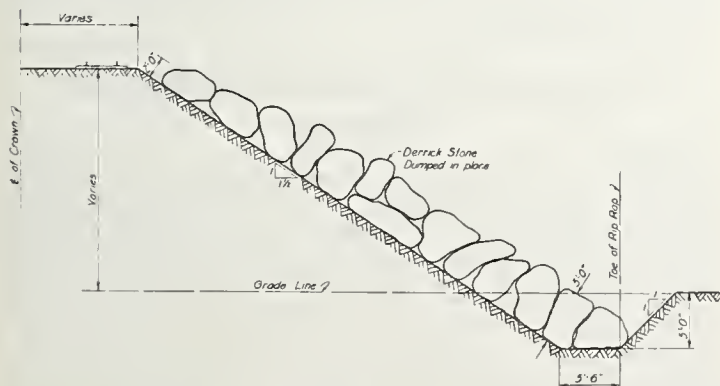
FIGURE 2. — Riprap bank protection; typical section.
