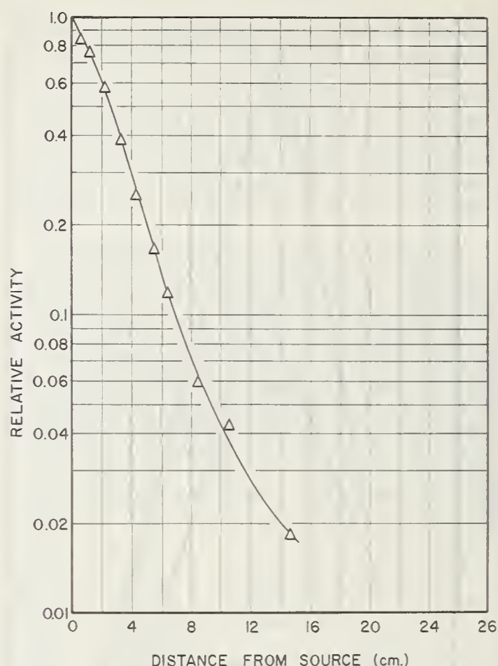
FIGURE 8. — The attenuation of scandium-46 photons by sand (bulk density 1.70 g./cm. 3 ; differential spectrometer; 1.12 Mev peak, 1-volt gate).
