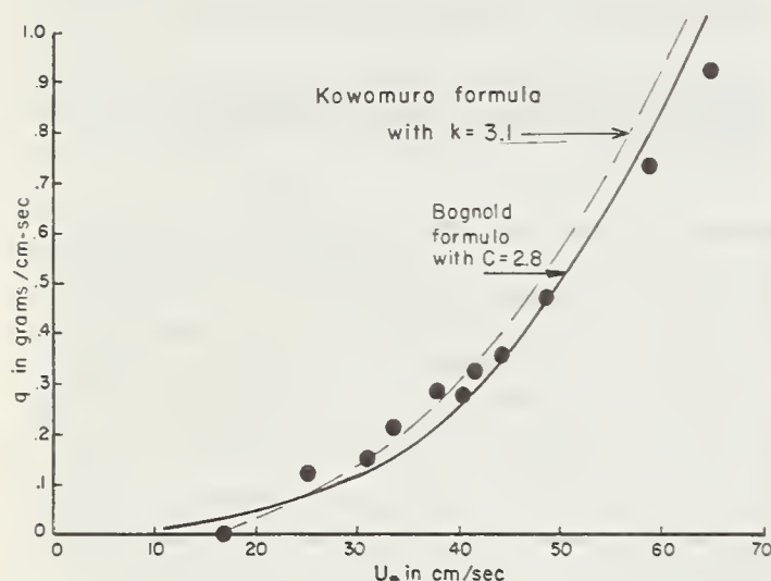
FIGURE 9.— Comparison of experimental data with Bagnold and Kawamura formulas for sand B ( d = 0.30 mm.).
