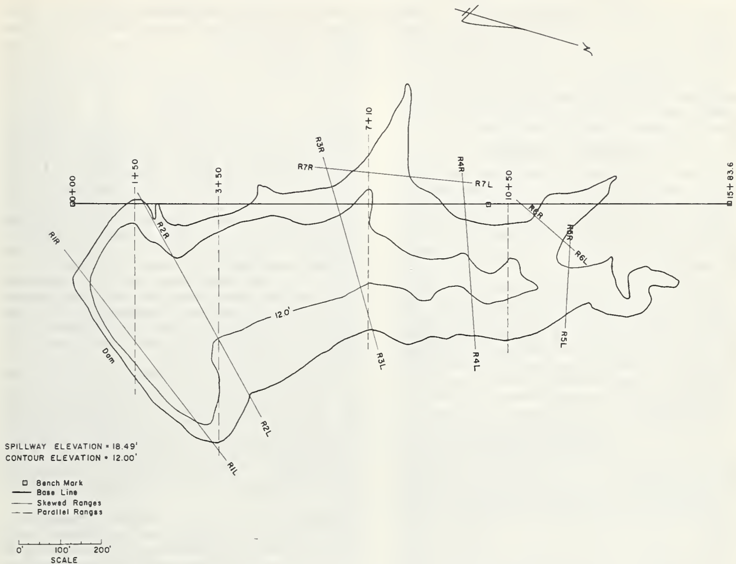
FIGURE 12. — Imposed survey, Al Olsen Reservoir.
