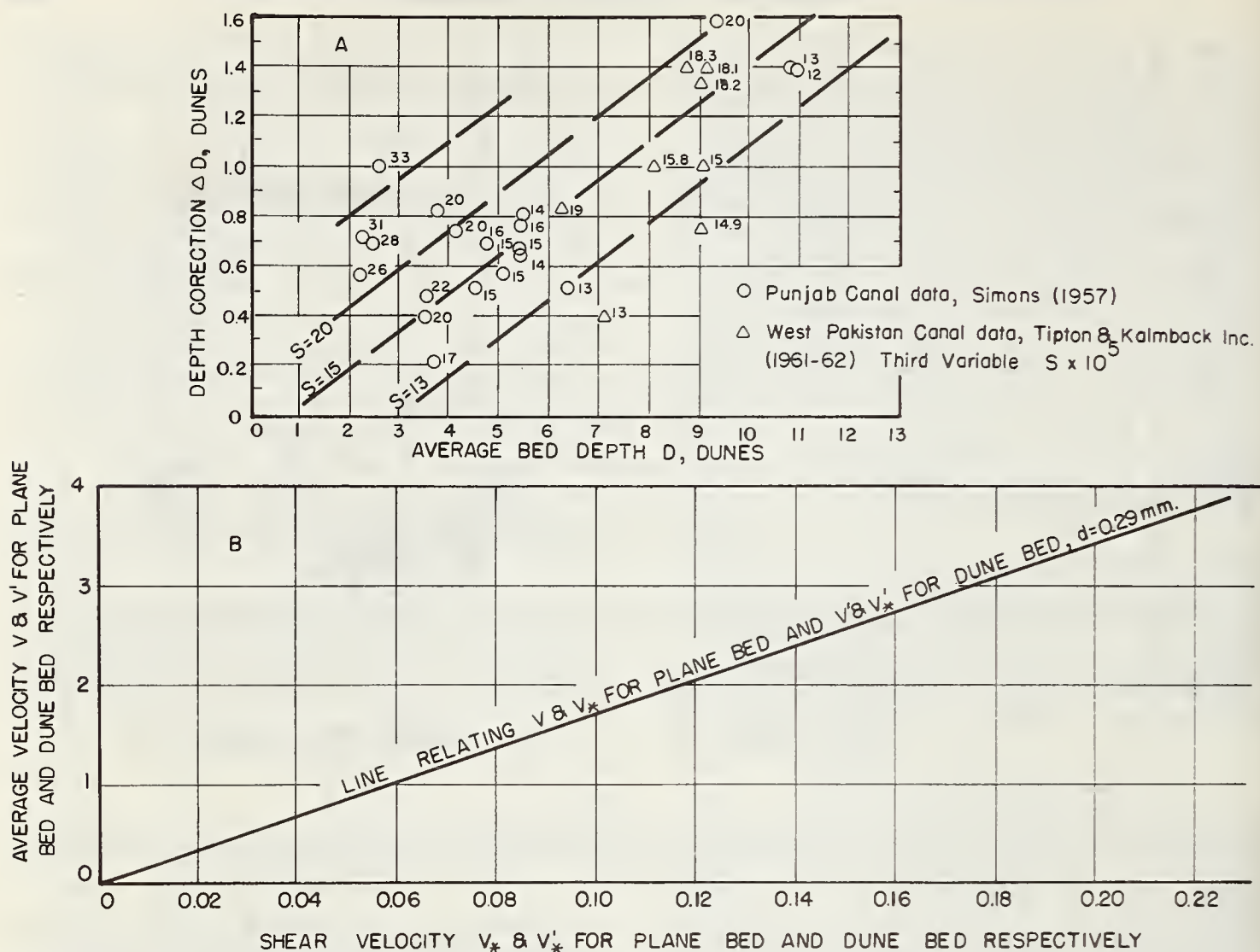
FIGURE 10. — Relation of V and V' to V_* and V'_* , respectively, for bed material with a median fall diameter of about 0.29 mm. for plane bed and dunes.
