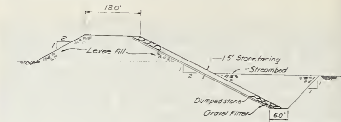
FIGURE 24. — Santa Maria River typical levee section.
