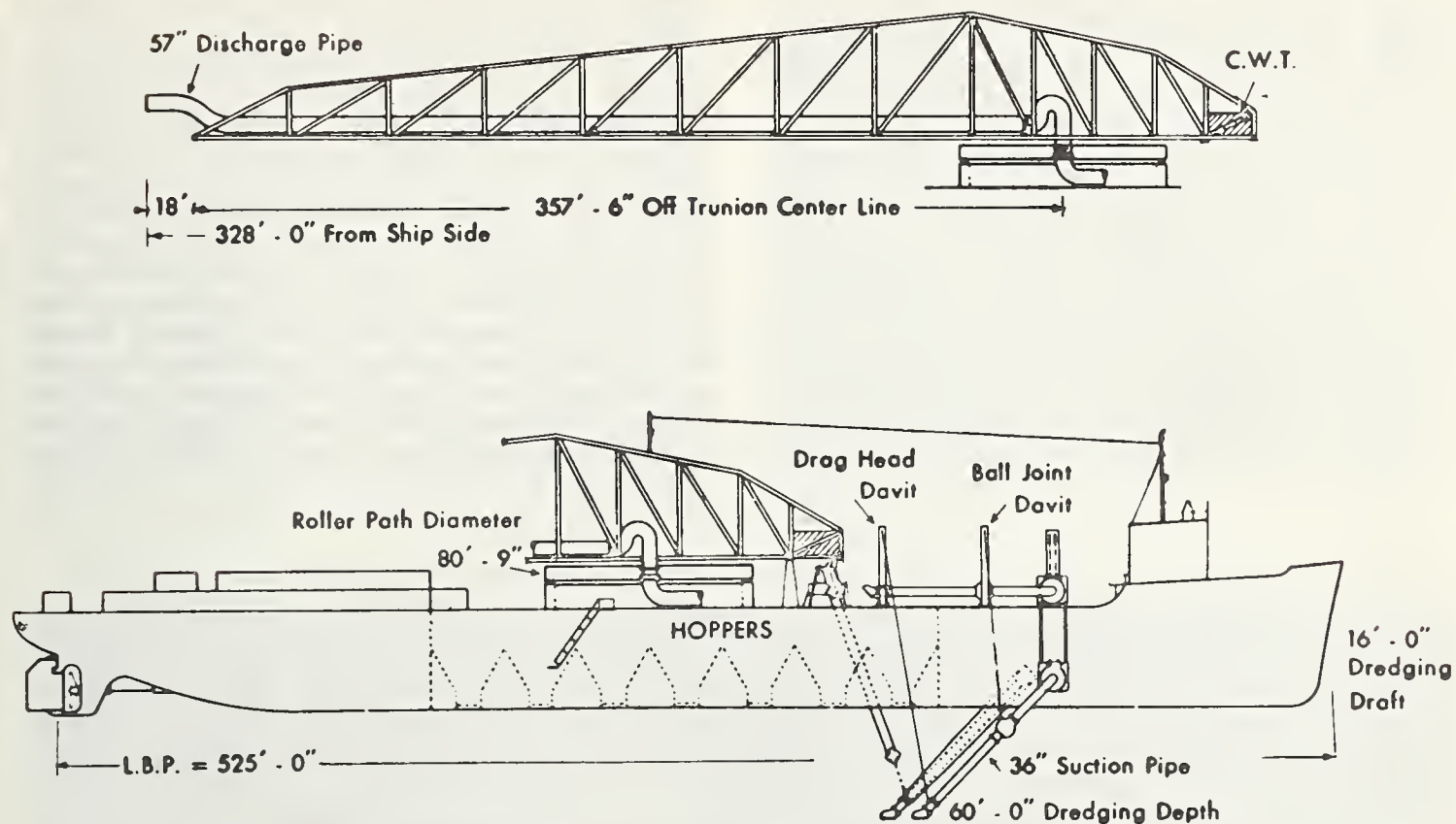
FIGURE 10. — Dredge Zulia : Elevations showing arrangement of boom discharge pipe.
