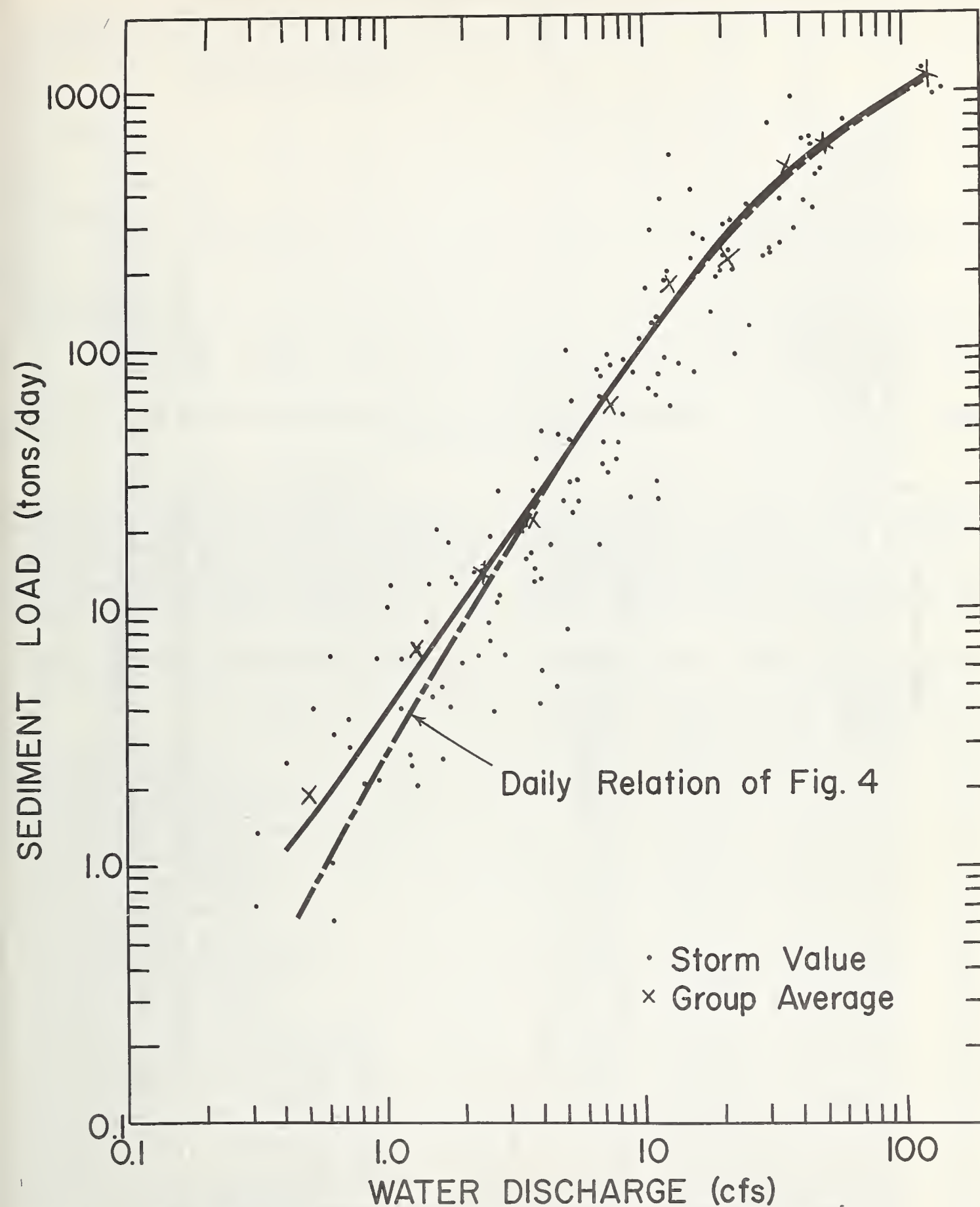
FIGURE 5.— Direct runoff versus sediment discharge, by storm, Pigeon Roost Creek Watershed 5, January 1957–December 1960.
