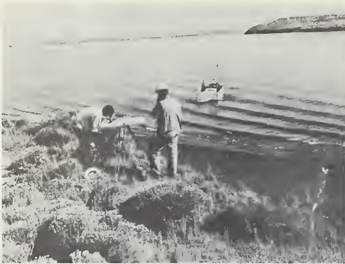
FIGURE 12.—Plane table being oriented over cut-in point and boat proceeding to range location to start sounding operations.
