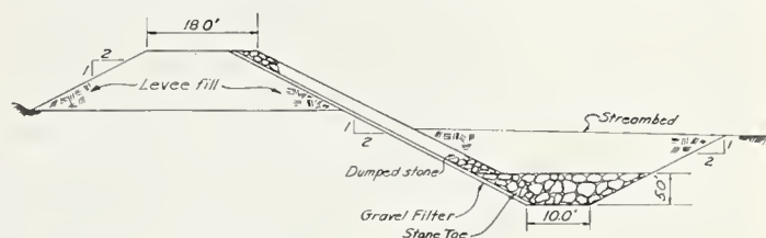
FIGURE 19.—Santa Clara River typical levee section.
