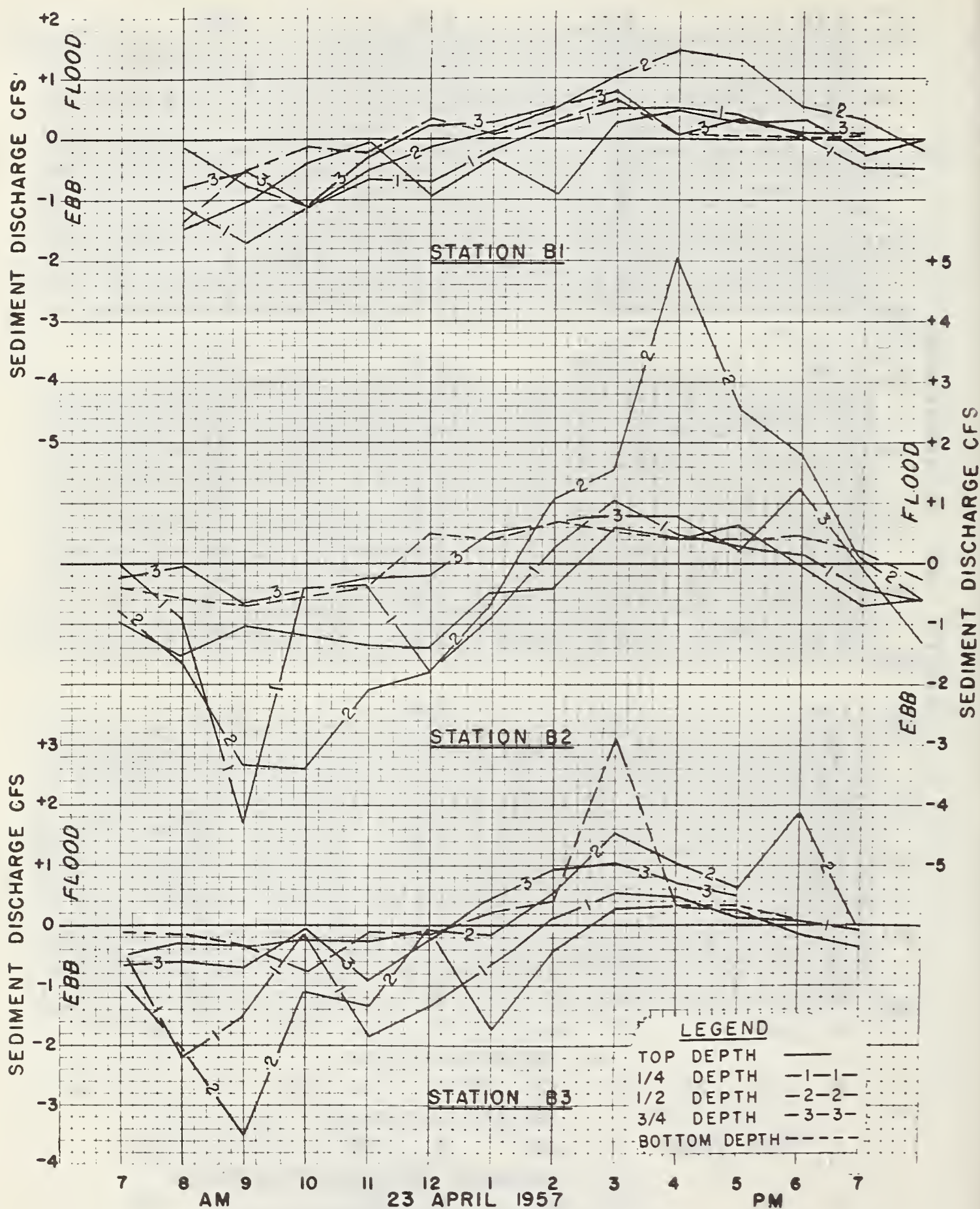
FIGURE 17. —Vertical and horizontal variation in sediment discharge over one tidal cycle.
