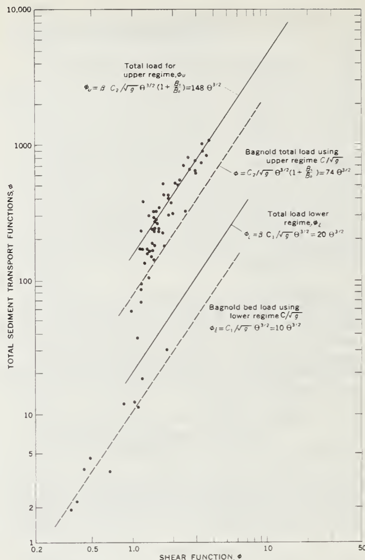
FIGURE 2.—Bagnold shear-transport functions: Rio Grande near Belen, N. Mex., Casa Colorado reach.
