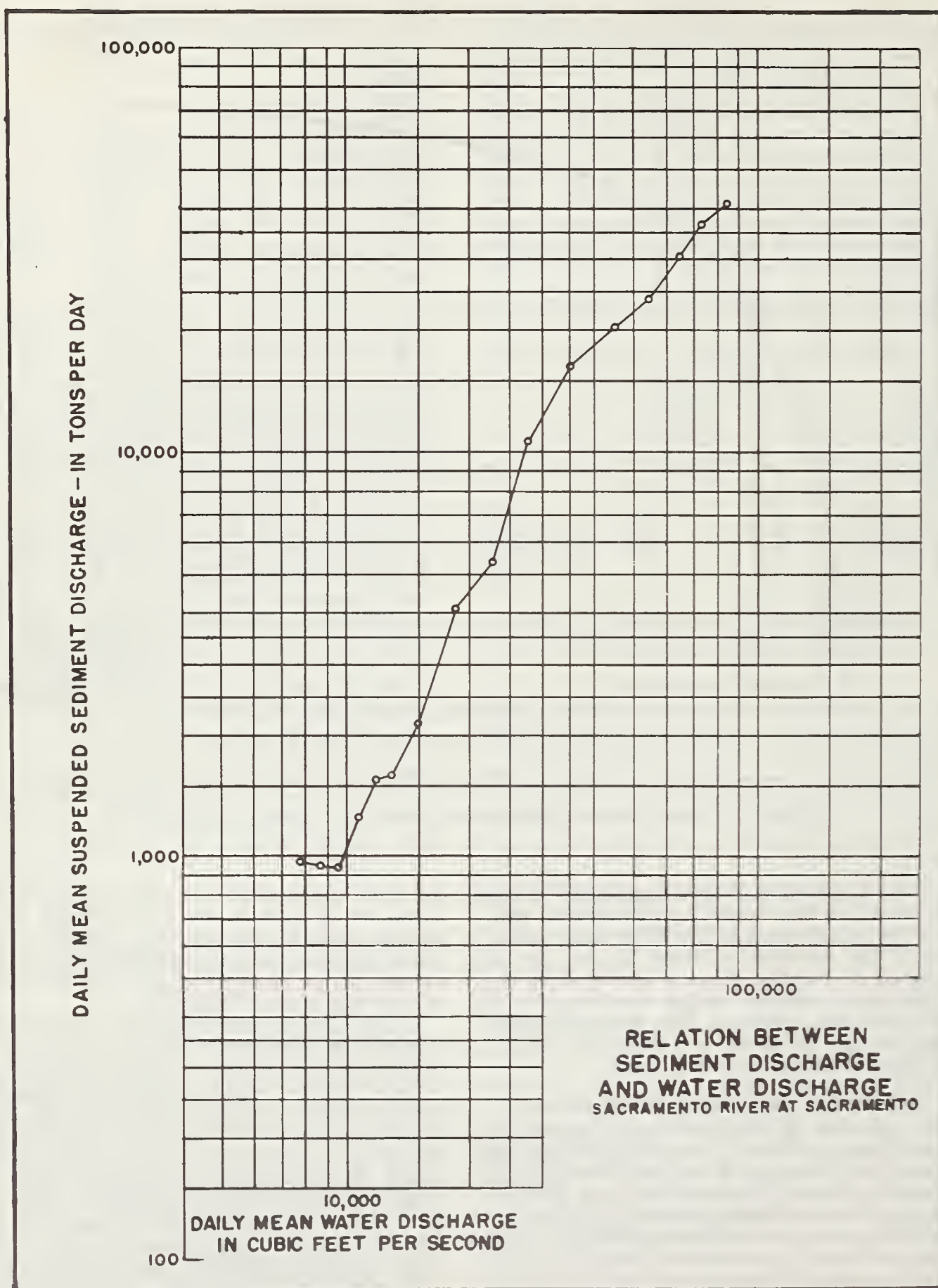
FIGURE 4. — Relation between sediment discharge and water discharge of Sacramento River at Sacramento.
