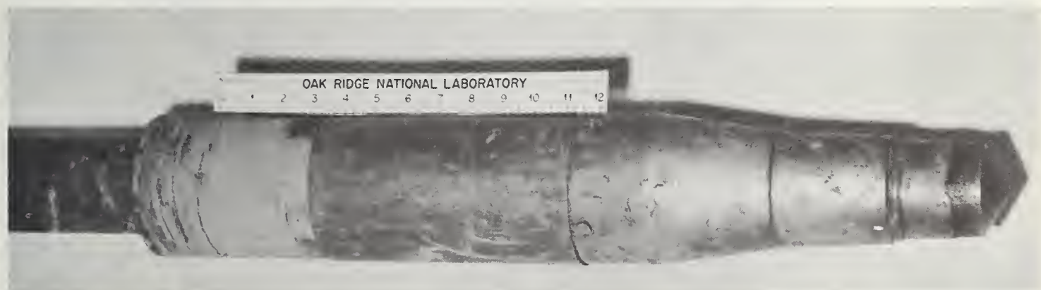
FIGURE 4. — Sampler head ready for sampling run, Swedish Foil Sampler.
