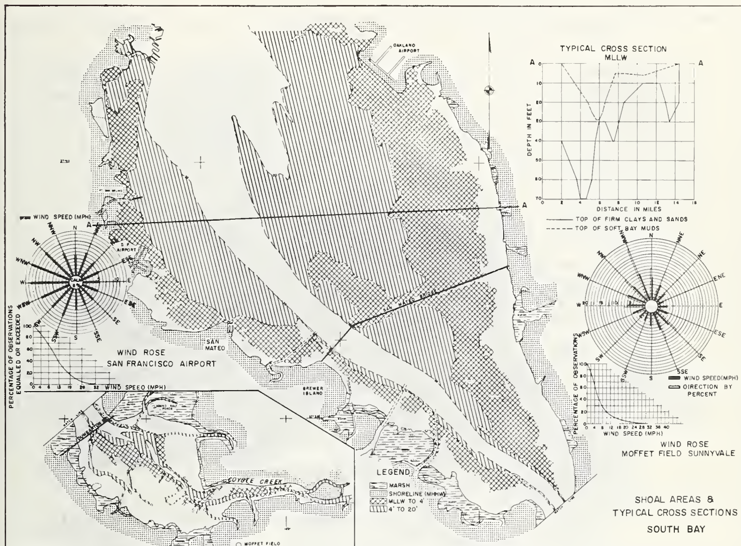
FIGURE 17. — Shoal areas, wind roses, and typical cross section of South San Francisco Bay.
