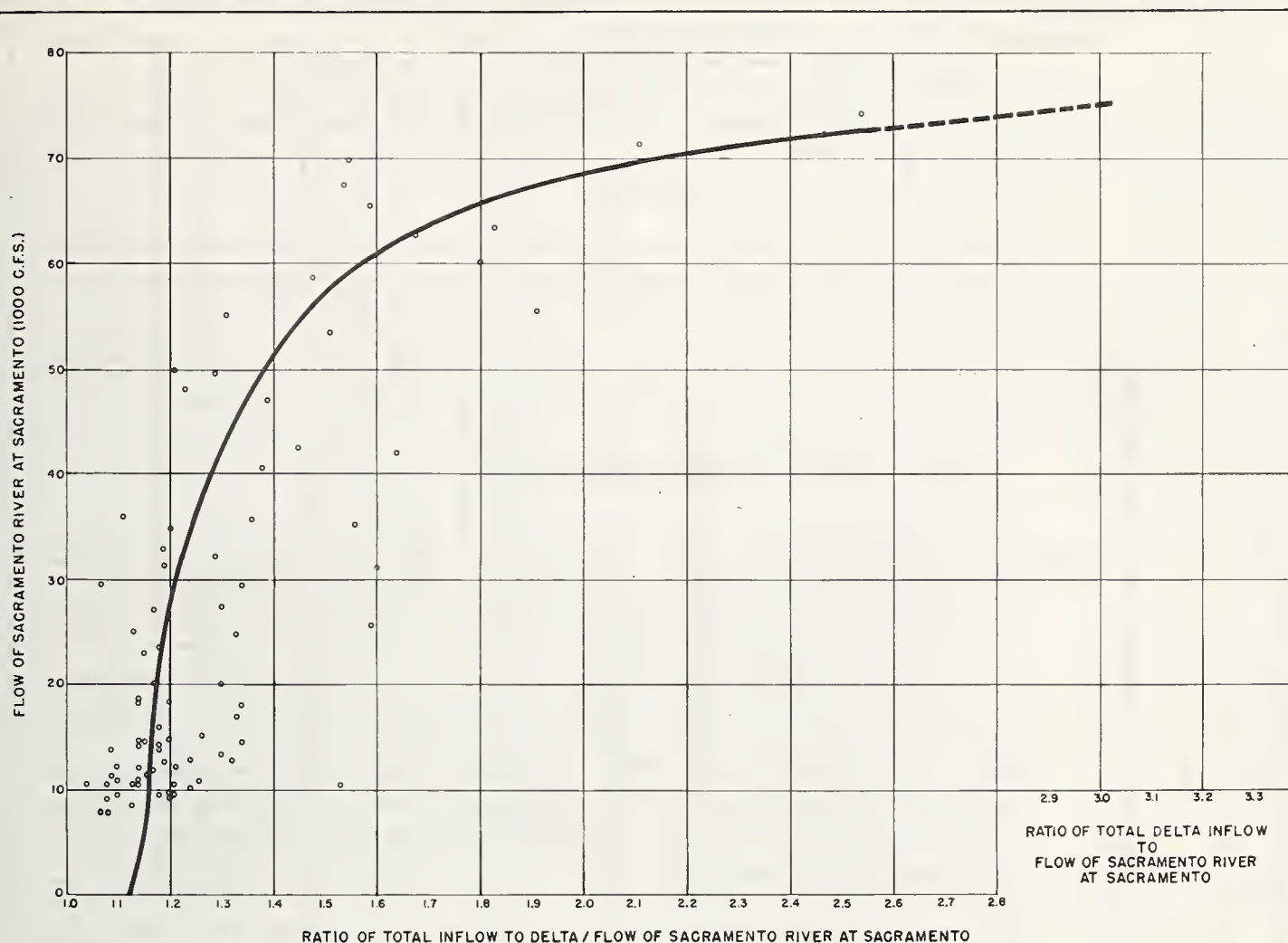
FIGURE 3. — Ratio of total delta inflow to flow of Sacramento River at Sacramento.
