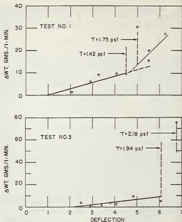
FIGURE 5. — Weight loss per 1 minute vs. deflection.
