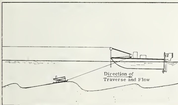
FIGURE 4. — Arrangement of boat and sled for the longitudinal traverses.
