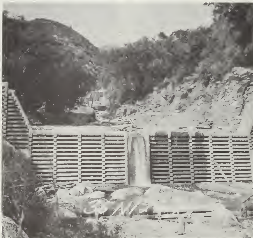
FIGURE 8. — Construction progress on a typical structure.
