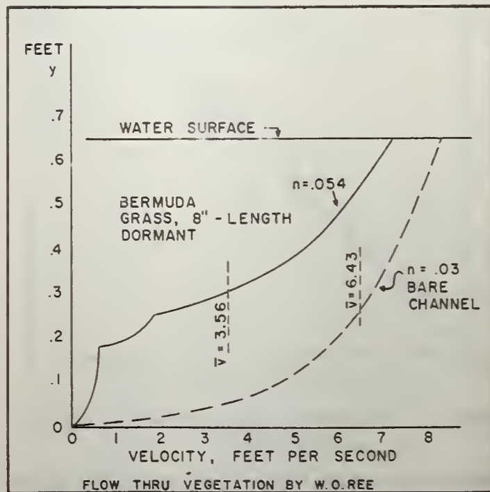
FIGURE 1.—Flow through vegetation (after W. O. Ree).
