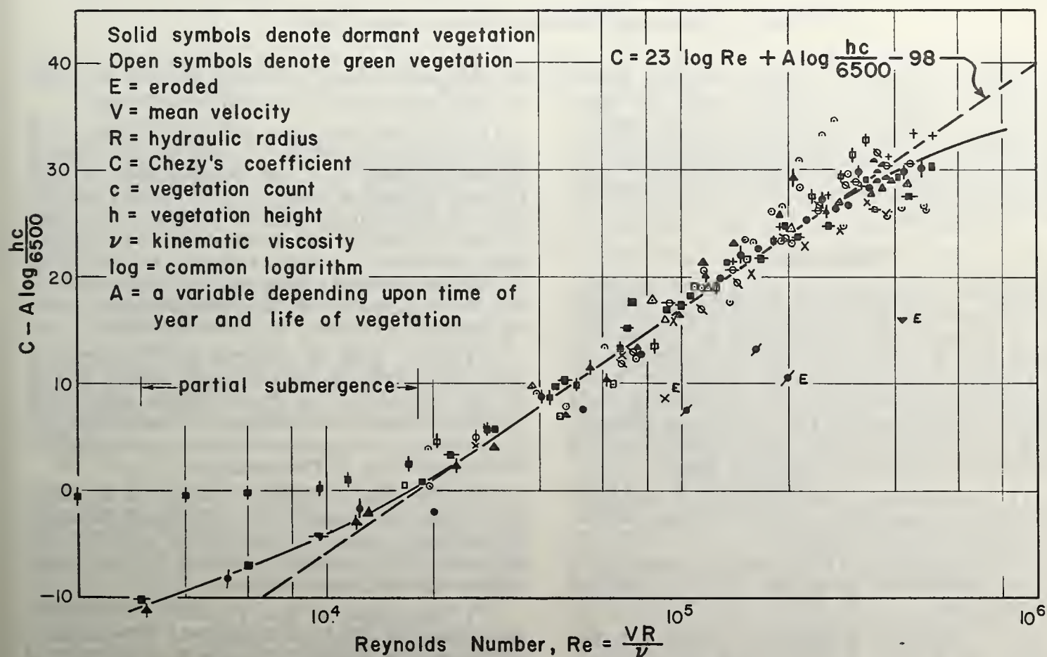
FIGURE 2. — Bermudagrass channels, Spartanburg, S. C.
