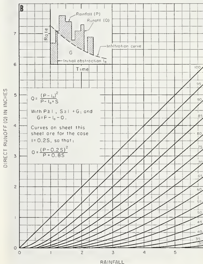
FIGURE 6.—A, Based on soil group, vegetal type, and ground cover density, curve number (fig. 6, B) is selected for solution of the runoff equation. B, With runoff curve number selected from figure 6, A, surface runoff can be computed for various rainfall intensities (13).
