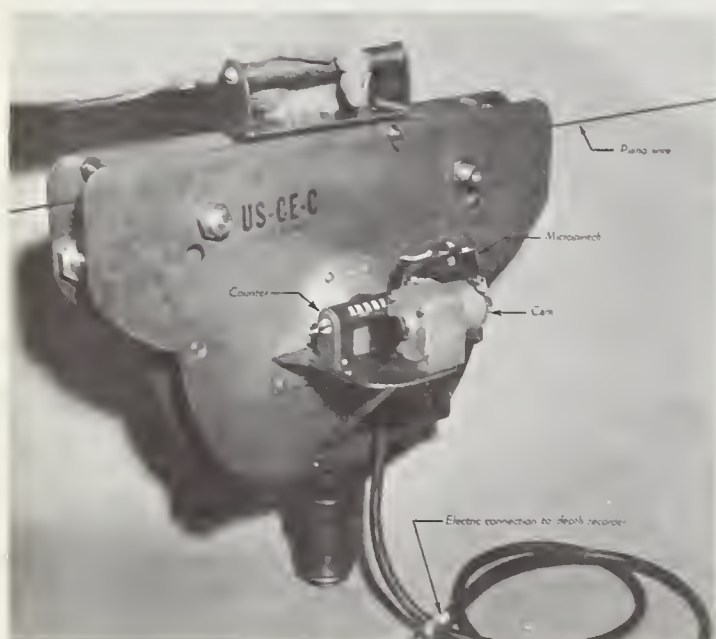
FIGURE 4. — Distance-measuring wheel.
