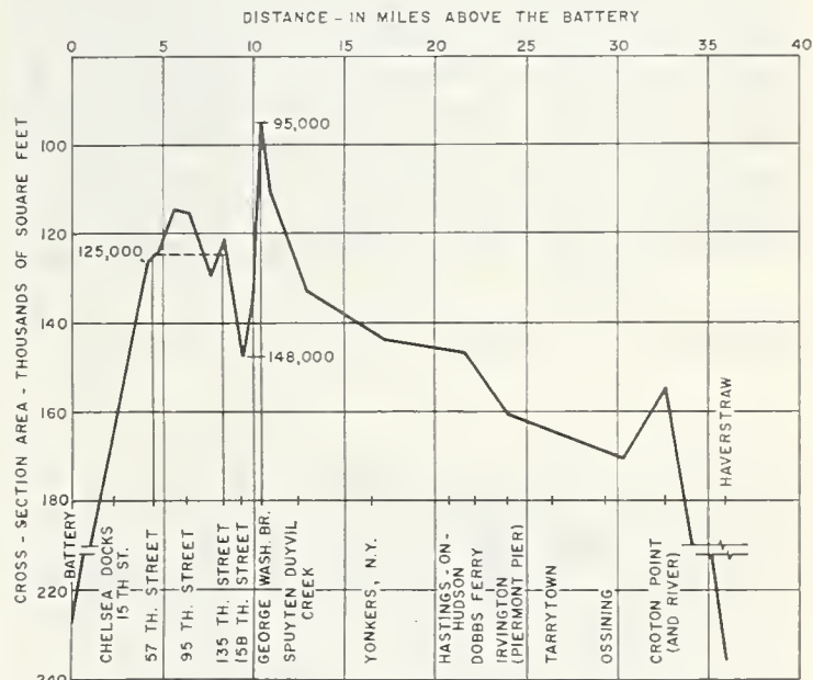
FIGURE 5.—Lower Hudson River: cross sectional areas at mean low water.
