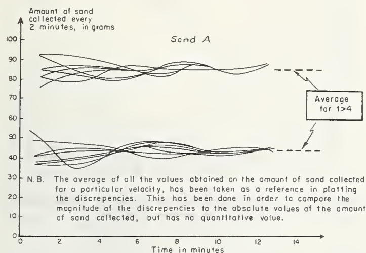
FIGURE 11.—Change in rate of transport with time following a change in wind velocity.
