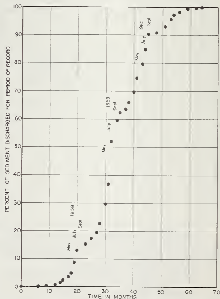
FIGURE 5.—Cumulative sediment discharged from the construction area with time. Note the higher rates of yield during summer months.
