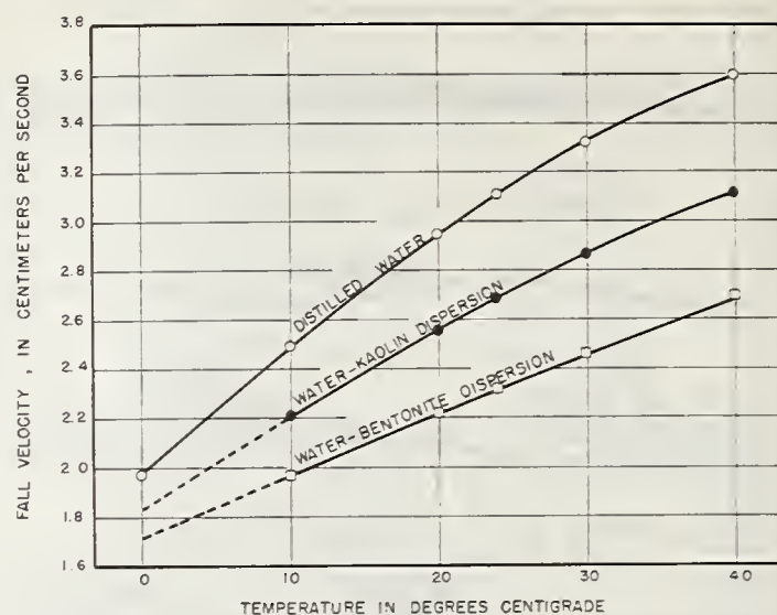
FIGURE 3.—Variation in fall velocity of median particle size of Elkhorn River, Nebr., sand with changes in temperature in distilled water and with 5 percent by weight dispersions of kaolin and of bentonite.
