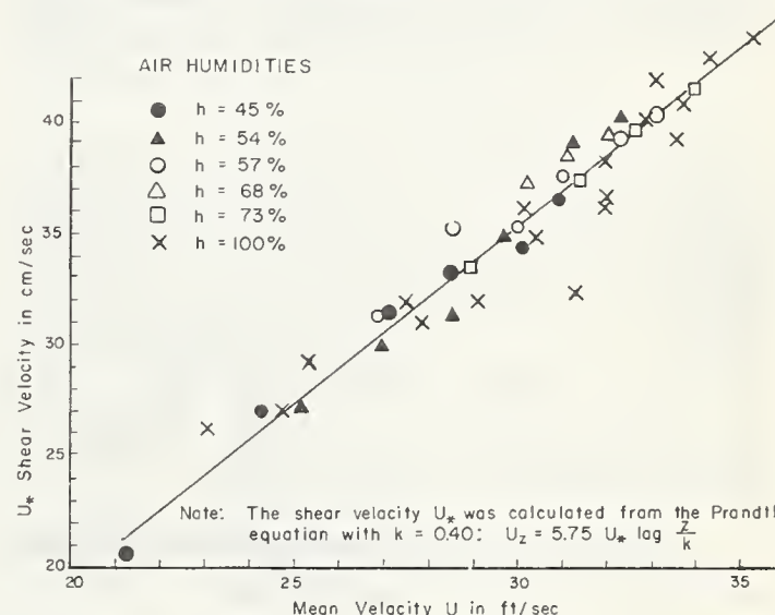
FIGURE 12.—Relation between mean velocity and shear velocity for various air humidities.
