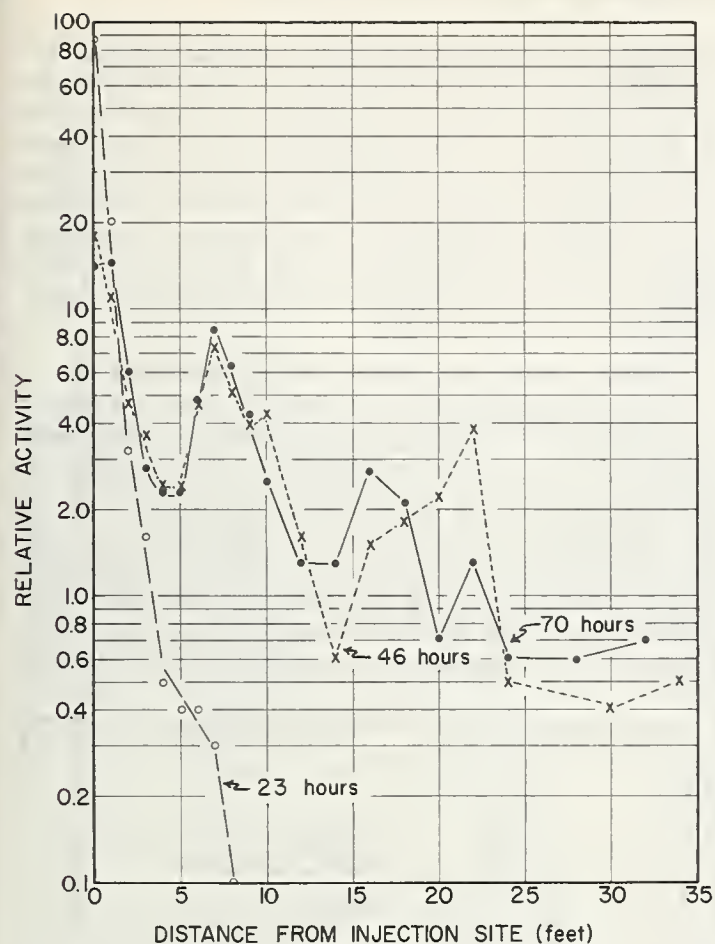
FIGURE 3. — Distribution of scandium-46 labeled sand in the channel bed after 23, 46, and 70 hours of flow.
