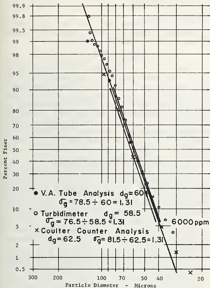
FIGURE 8.—Results of visual-accumulation-tube, turbidimeter, and electronic sensing device.
