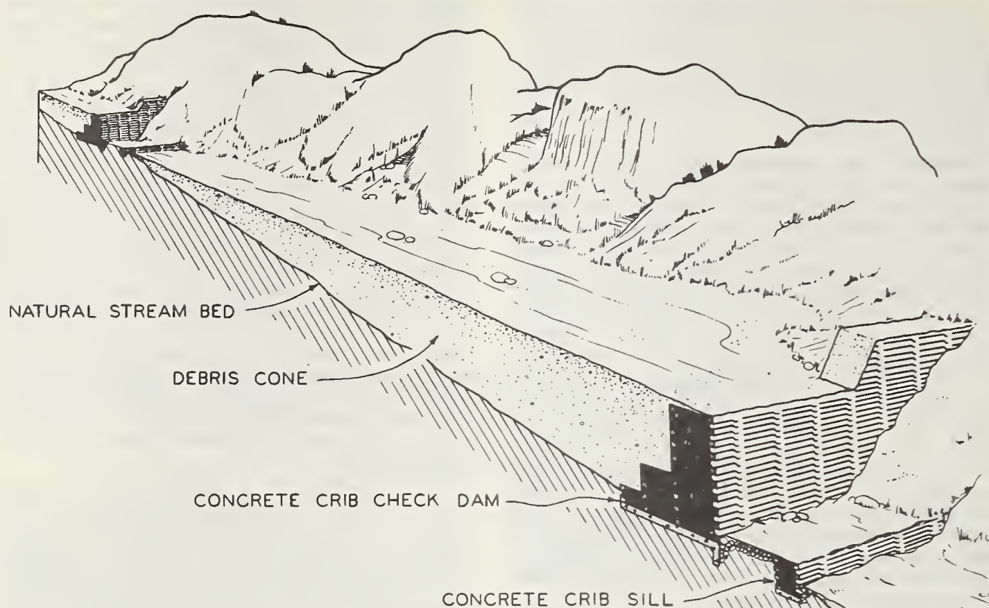
FIGURE 2. — Cutaway view of channel stabilization system.
