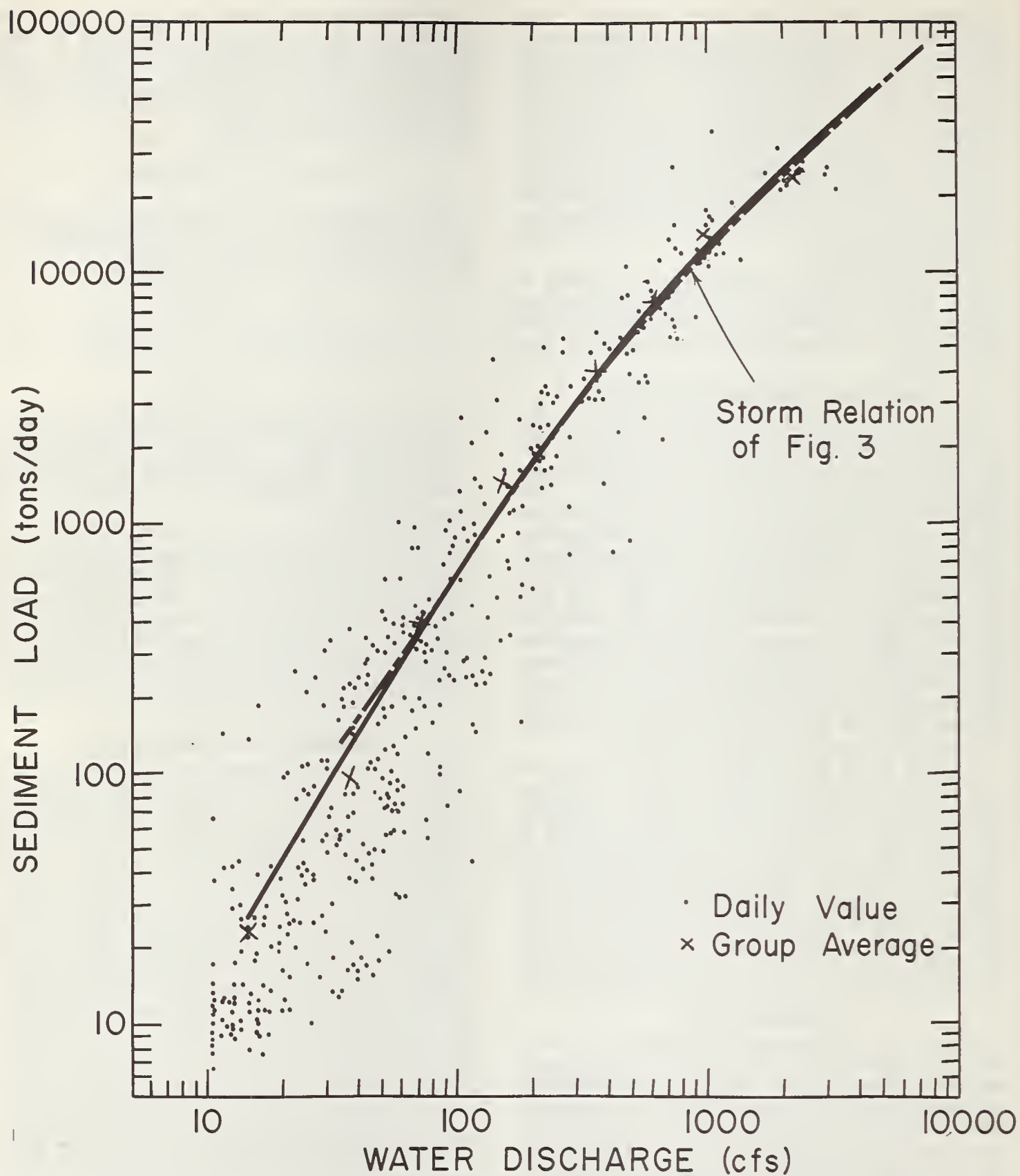
FIGURE 2. — Direct runoff versus sediment discharge, by day, Pigeon Roost Creek Watershed 34, January 1957–December 1960.
