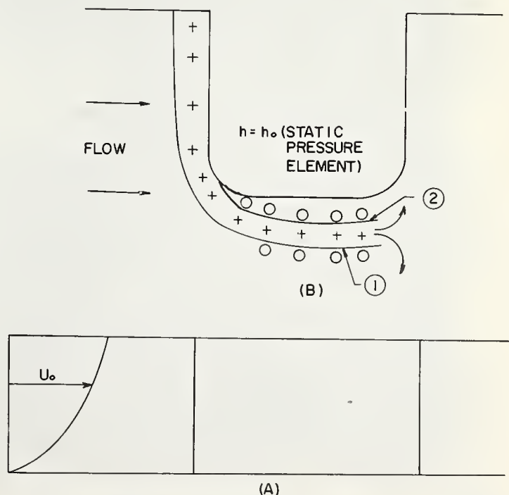
FIGURE 5.—Secondary flow at a bridge abutment.
