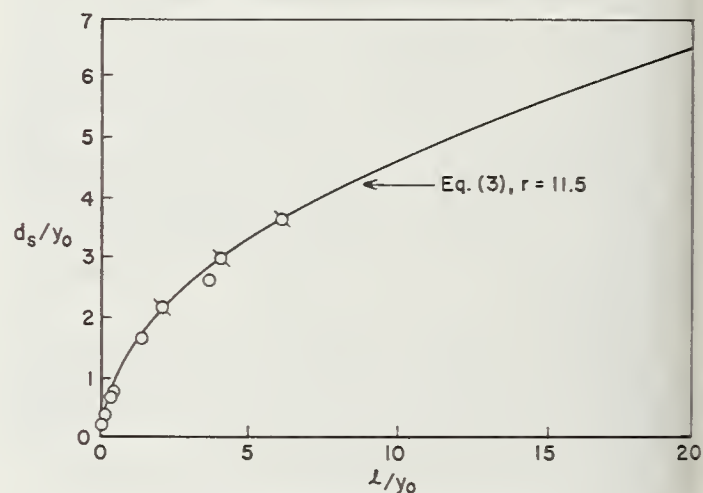
FIGURE 5. — Scour at an encroaching abutment.
