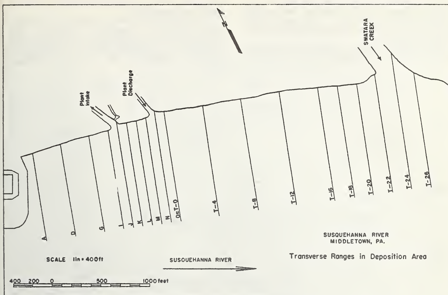
FIGURE 6. — Susquehanna River, Middletown; transverse ranges in deposition area.
