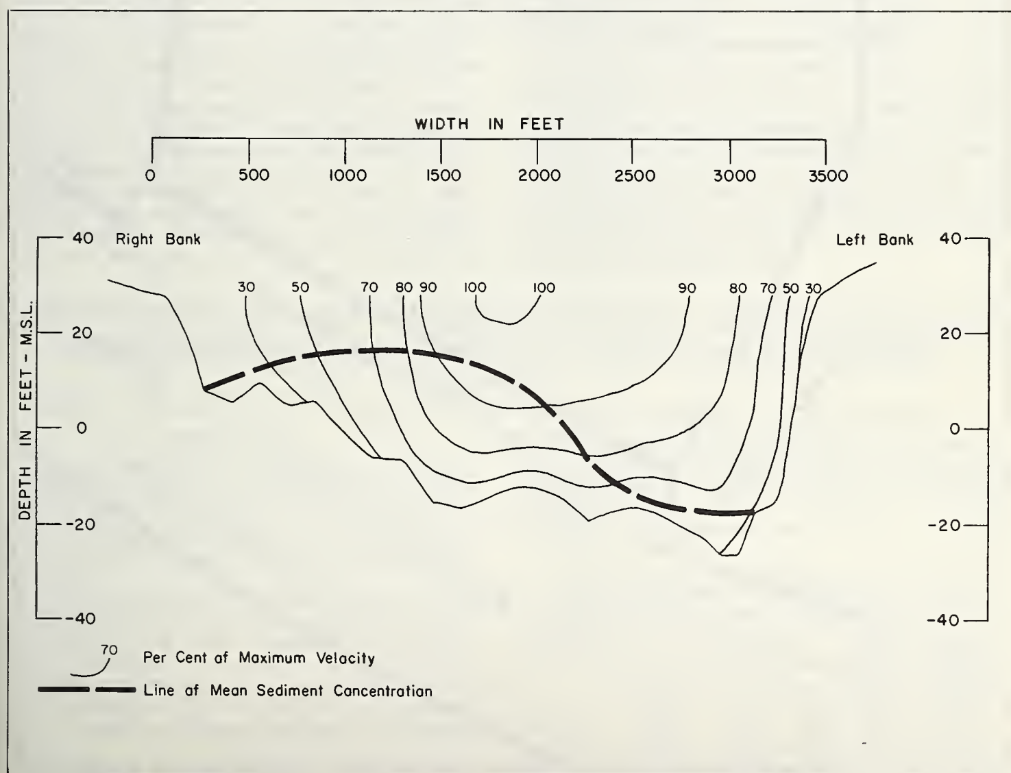
FIGURE 4.— Cross section of Mississippi River above Old River.
