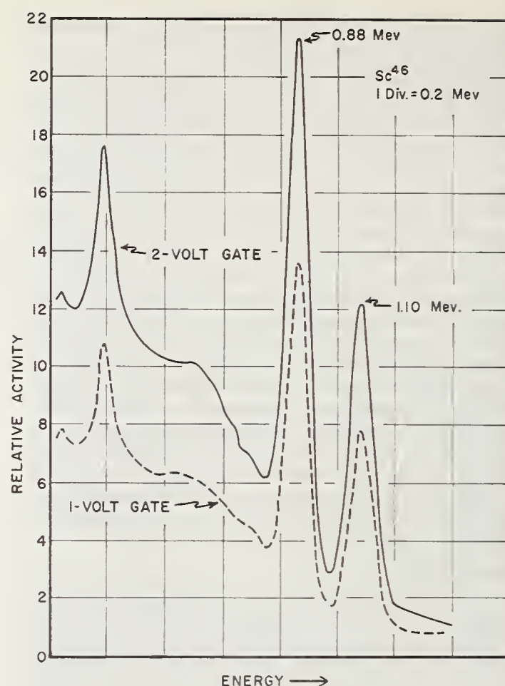
FIGURE 1. — The gamma ray energy spectrum of scandium-46. (Differential scintillation spectrometer: 1- and 2-volt gates.)
