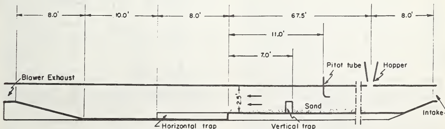
FIGURE 4.—Wind tunnel used in sand transport studies.
