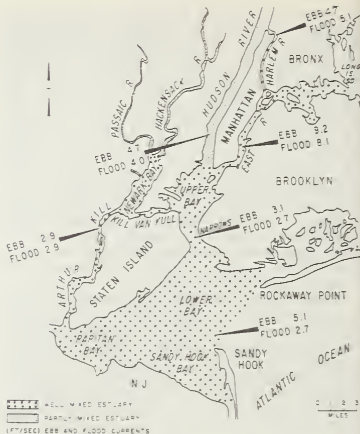
FIGURE 3. — New York Harbor estuarine system.
