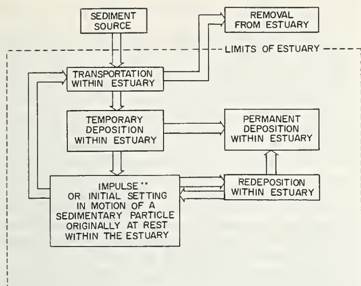
FIGURE 1.—Block model for evaluating sedimentation in an estuary.
