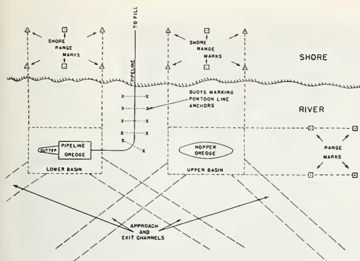
FIGURE 5.—Typical rehandling scheme.
