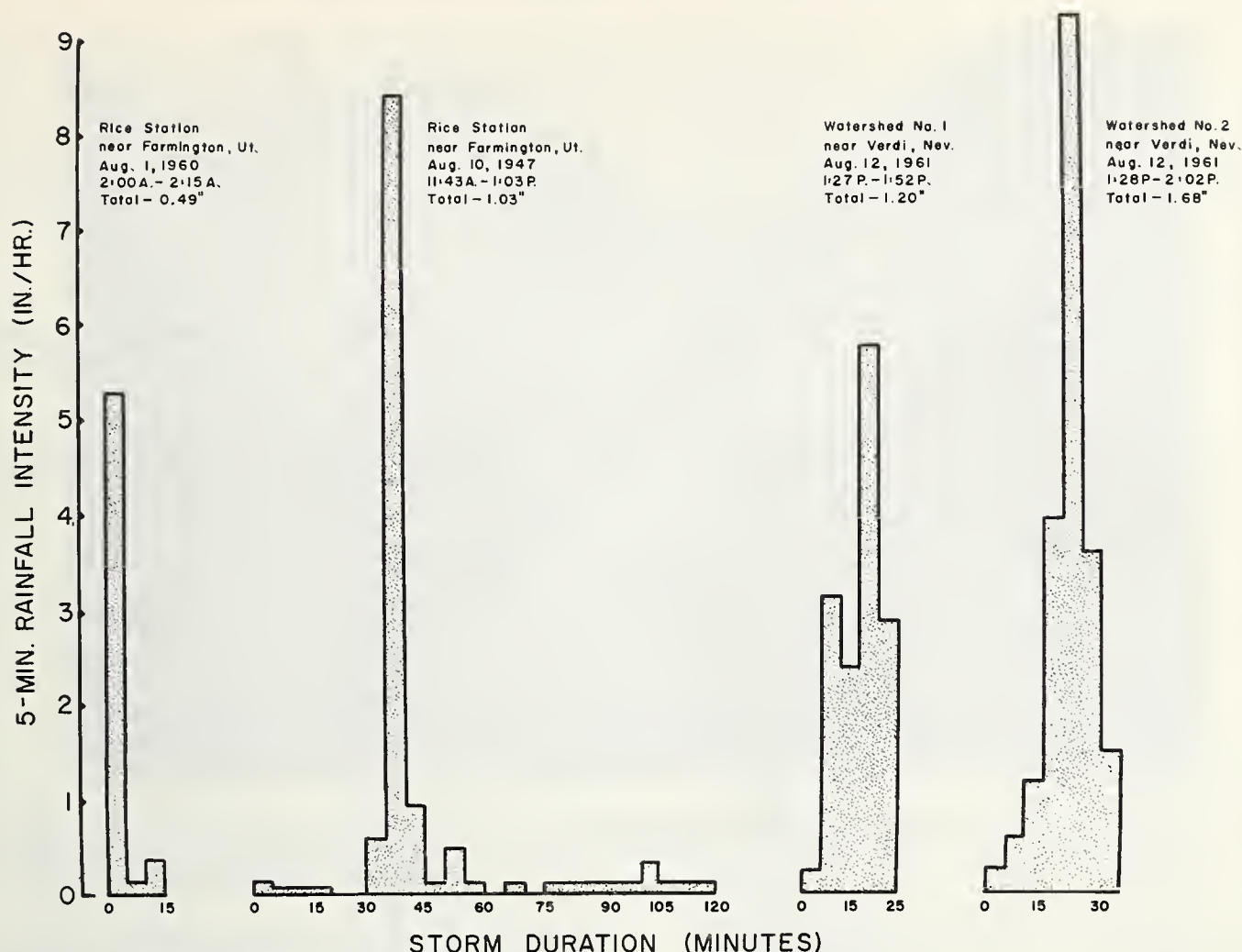
FIGURE 2.—Rainfall intensities of three storms (one measured at two locations) by 5-minute periods.
