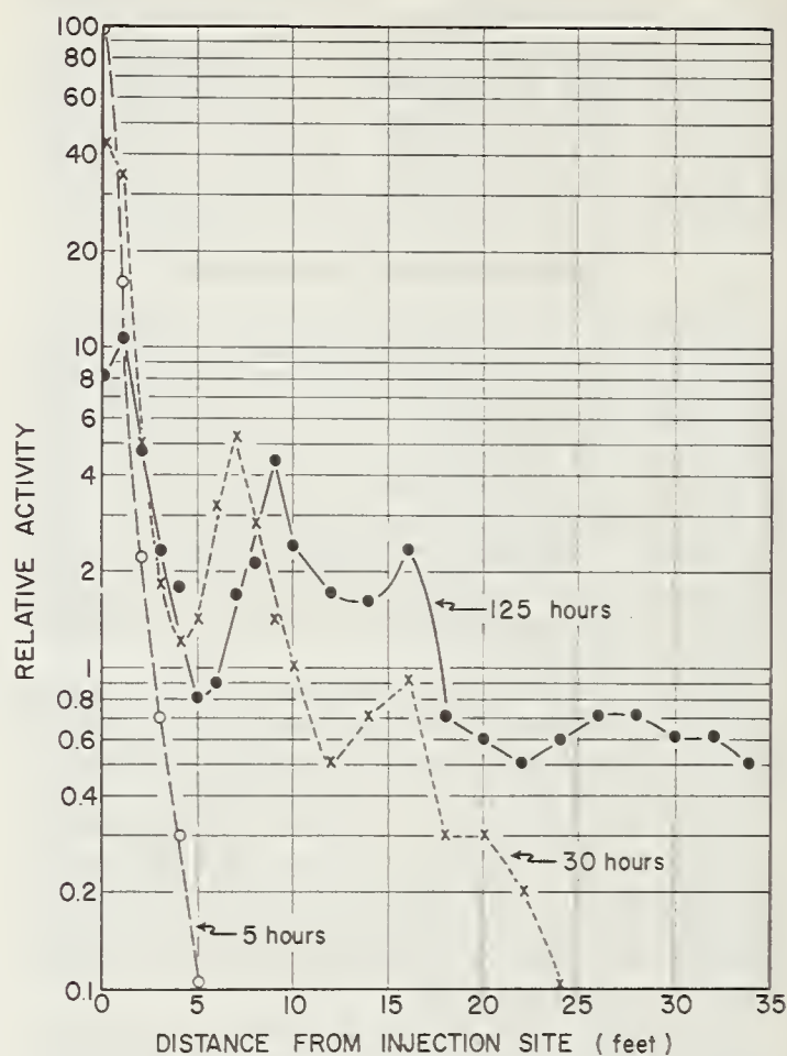
FIGURE 2.—Distribution of scandium-46 labeled sand in the channel bed after 5, 30, and 125 hours of flow.
