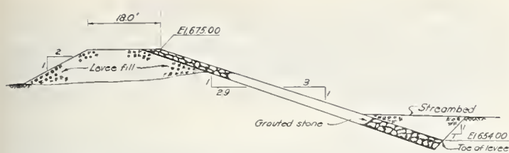
FIGURE 15.—Ventura River typical levee revetment of grouted cobblestone.
