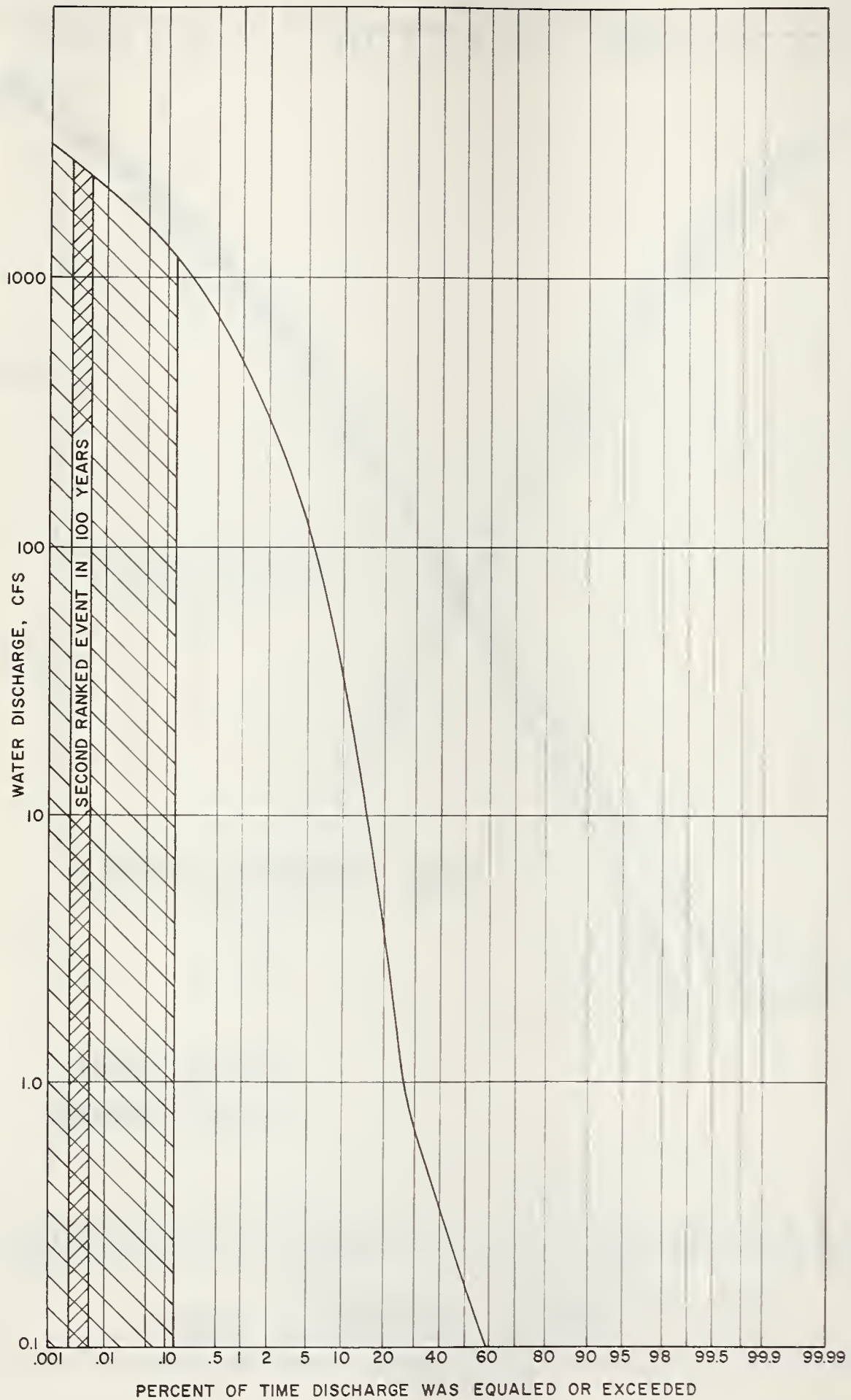
FIGURE 6. — Long term discharge-duration curve representing top-ranked runoff events, Watershed 32, Pigeon Roost Creek Basin, Miss.
