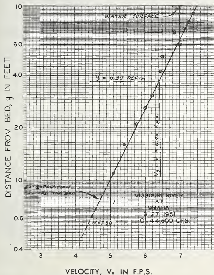
FIGURE 3.—Semilogarithmic plot of velocity distribution.
