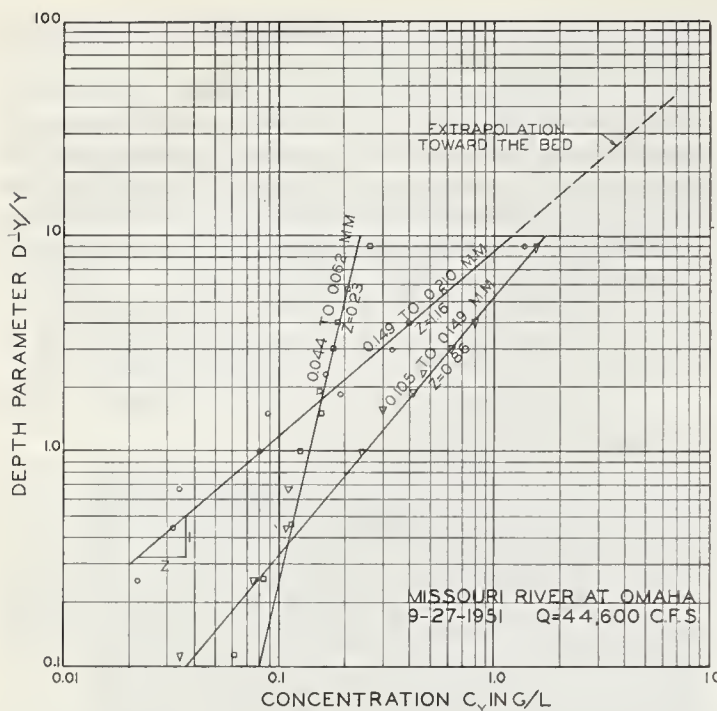
FIGURE 4. —Logarithmic plot of sand concentration distributions.
