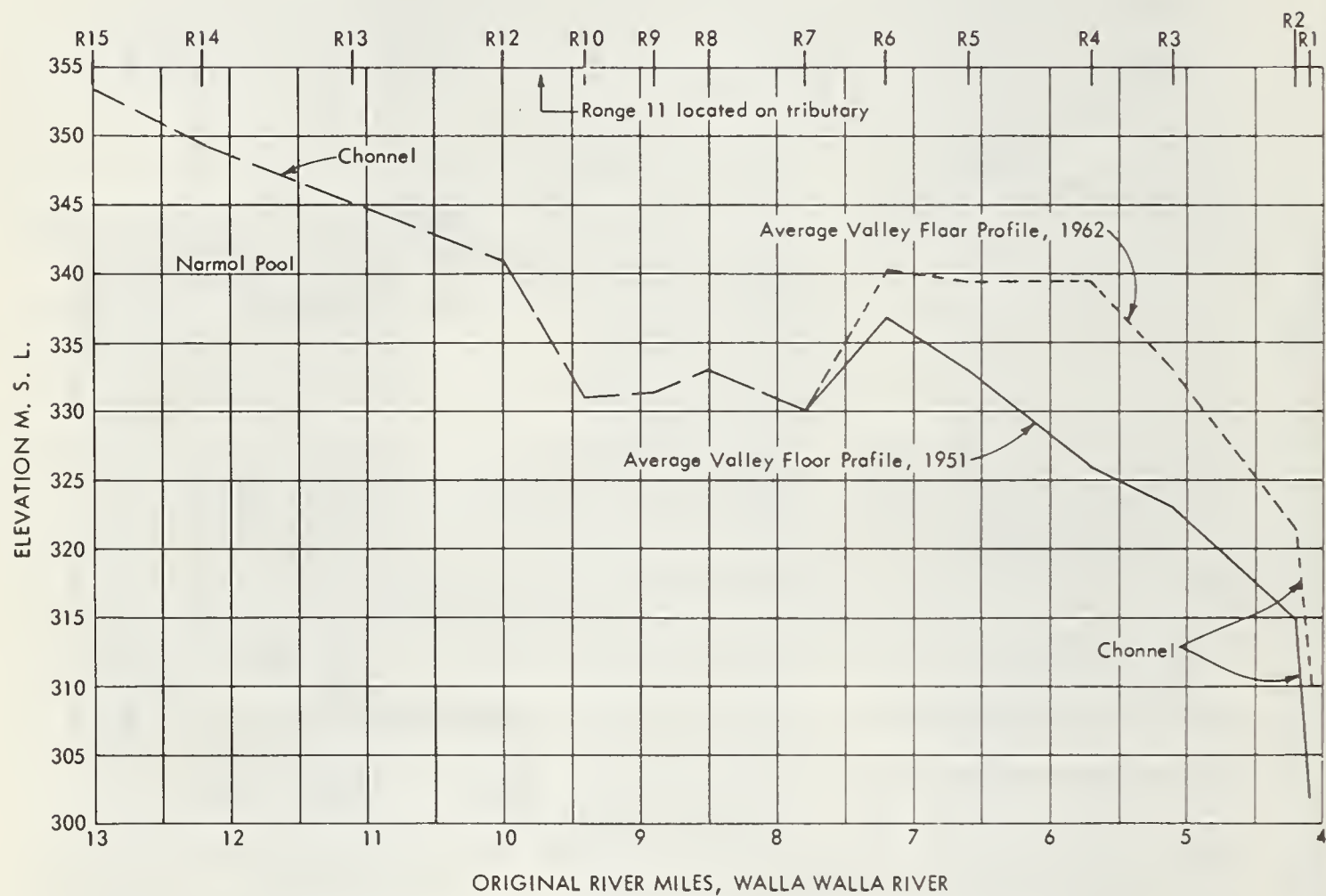
FIGURE 16. — Longitudinal profile sediment ranges, Walla Walla River.
