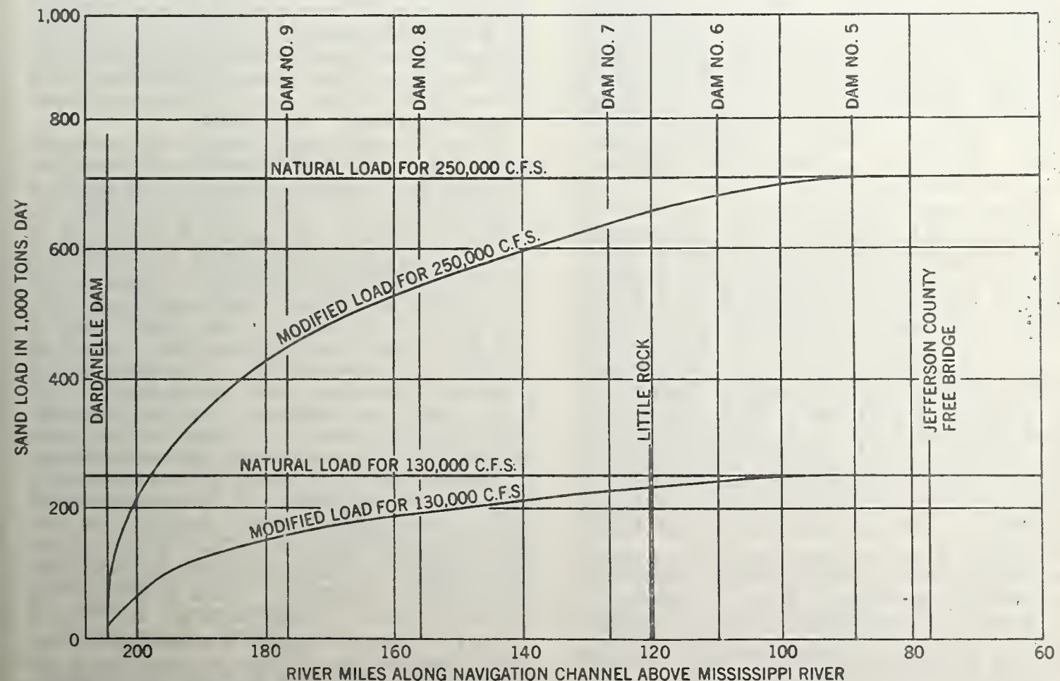
FIGURE 5. — Estimated variation of modified sand load with distance downstream from Dardanelle Dam.
