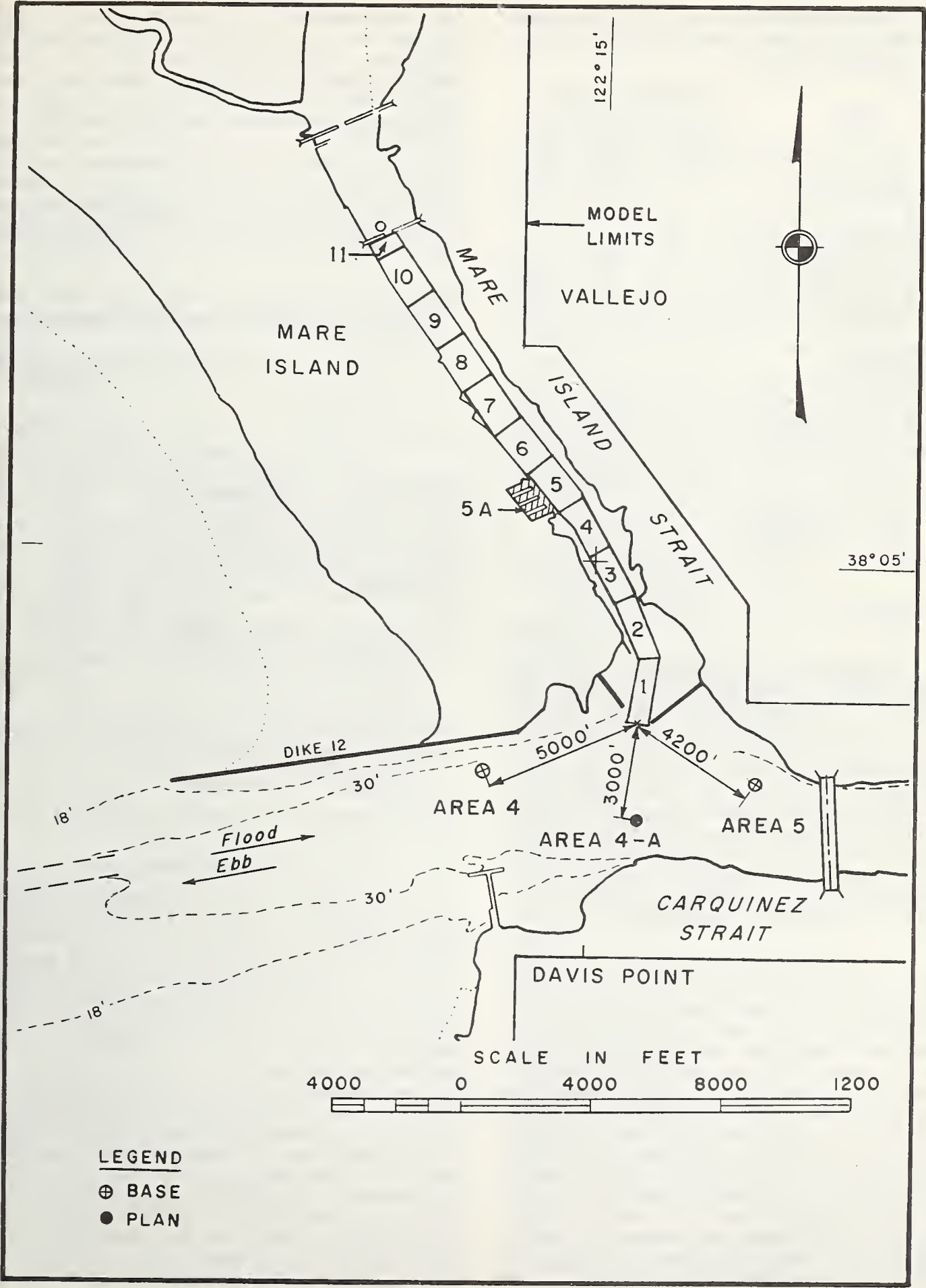
FIGURE 5. — Model of Mare Island Strait.
