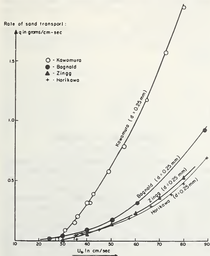
FIGURE 3.—Experimental data on sand transport determined by previous investigators.
