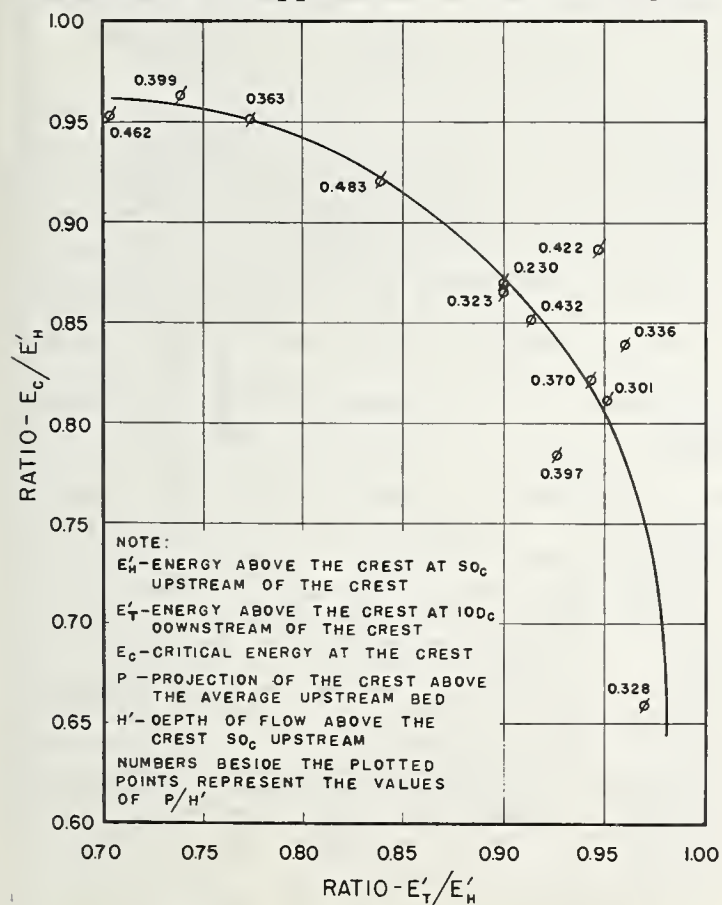
FIGURE 14.—Energy losses for a two-dimensional sill.
