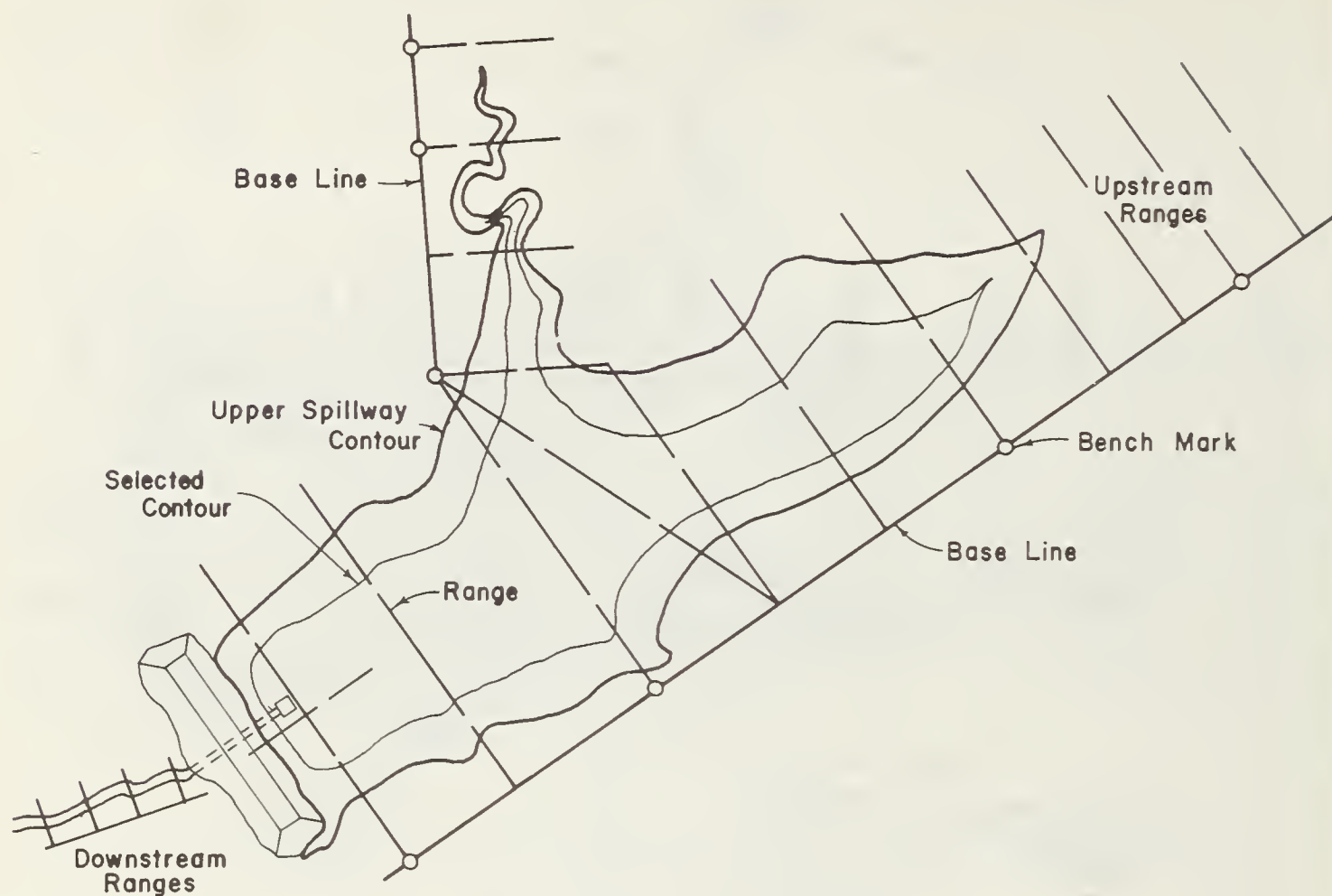
FIGURE 5. — Suggested range layout for a typical reservoir.
