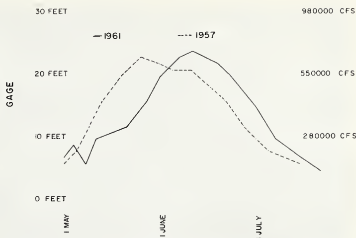
FIGURE 1.—Comparative flood-stage-discharge hydrographs, Columbia River at Vancouver, Wash., for 1957 and 1961.
