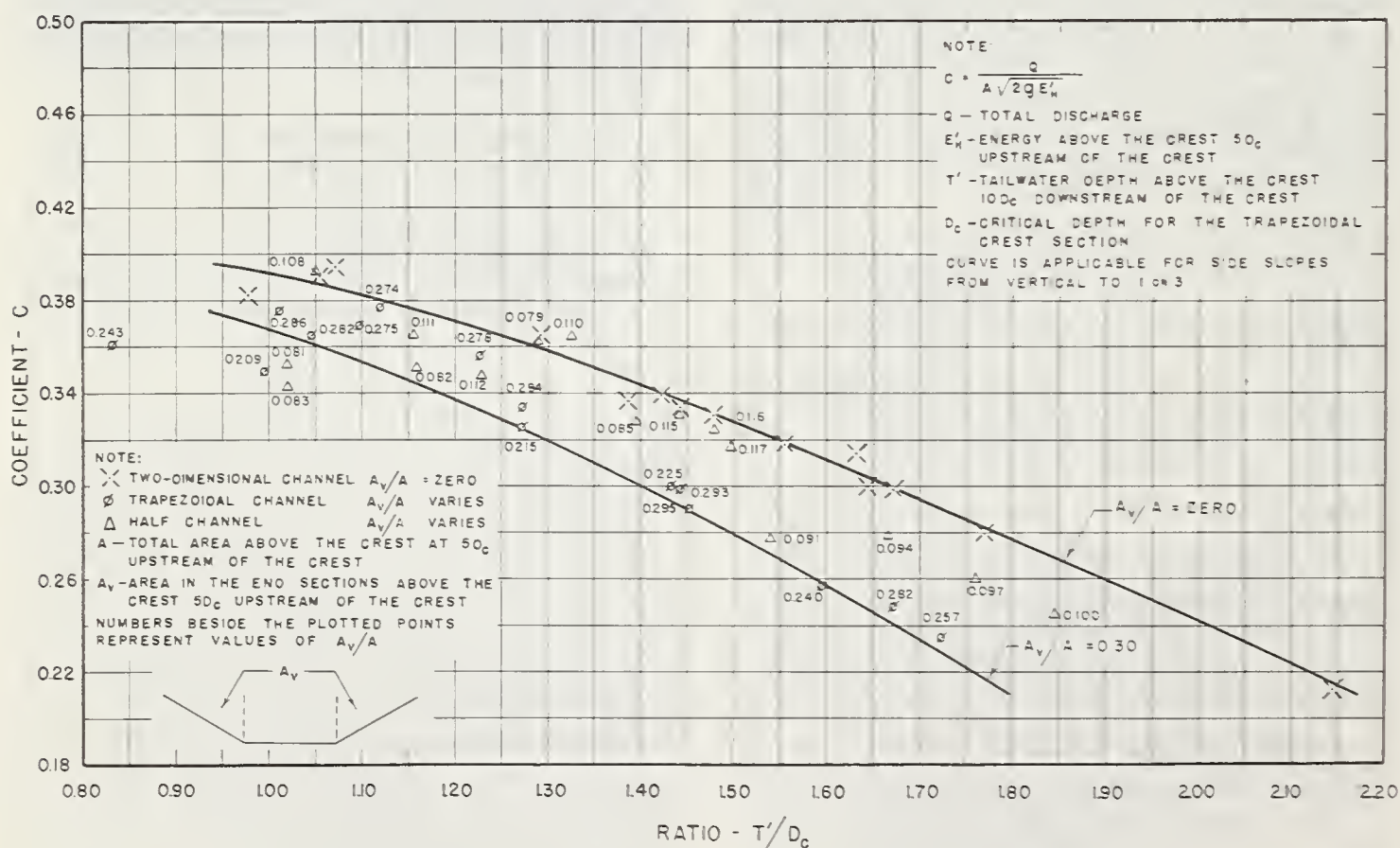
FIGURE 16. — Total discharge coefficient for a sheet piling and rock sill.
