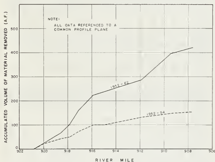
FIGURE 7.—Estimated volume of material removed by natural stream transport from the upper Fort Randall degradation reach between 1952 and 1962.
