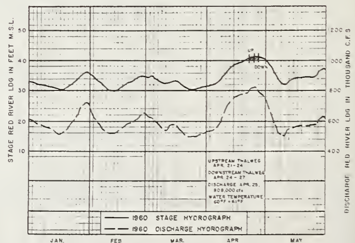
FIGURE 5.—1960 flood: Stage and discharge hydrographs, Mississippi River, Red River Landing, La.
