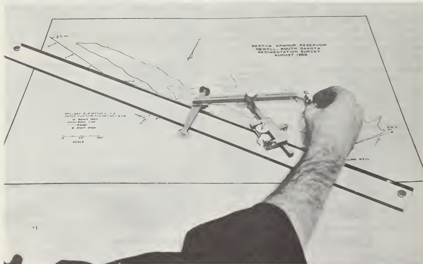
FIGURE 10.—Integrimeter.
