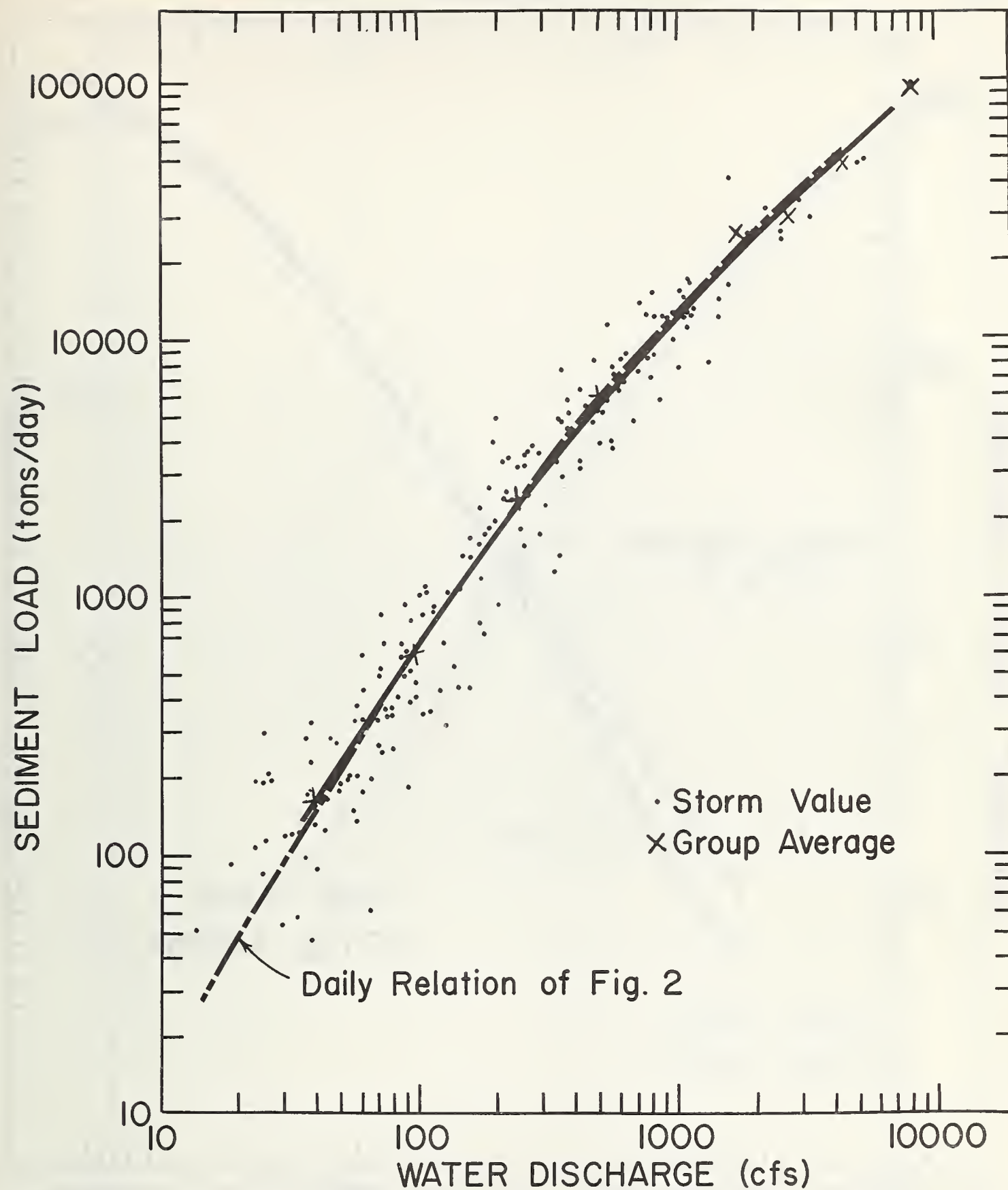
FIGURE 3.— Direct runoff versus sediment discharge, by storm, Pigeon Roost Creek Watershed 34, January 1957–December 1960.
