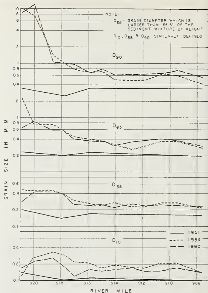
FIGURE 8.—Changes in the grain-size distribution of the streambed surface material between 1951 and 1960.
