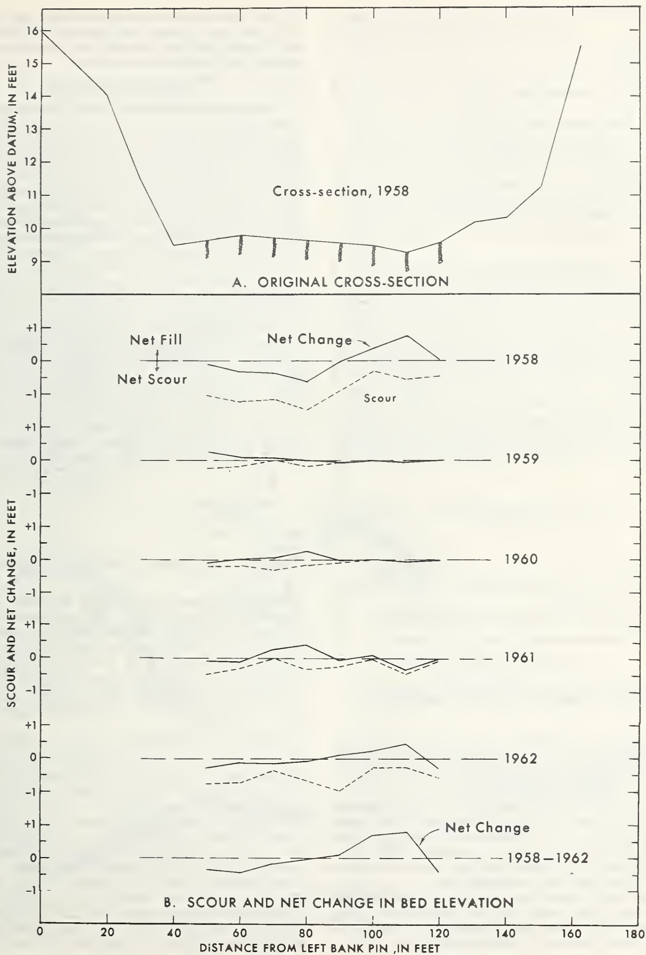
FIGURE 3. — Scour and net change in bed elevation at stationing 25,000 feet for a 5-year period.
