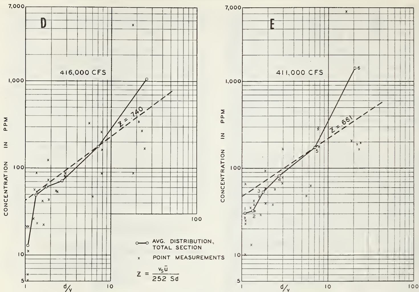
FIGURE 3 (continued). — Measured suspended fine sand at 6 levels at each of 5 verticals in cross section of Atchafalaya River at Simmesport, La.: D, for 416,000 c.f.s.; E, for 411,000 c.f.s.
