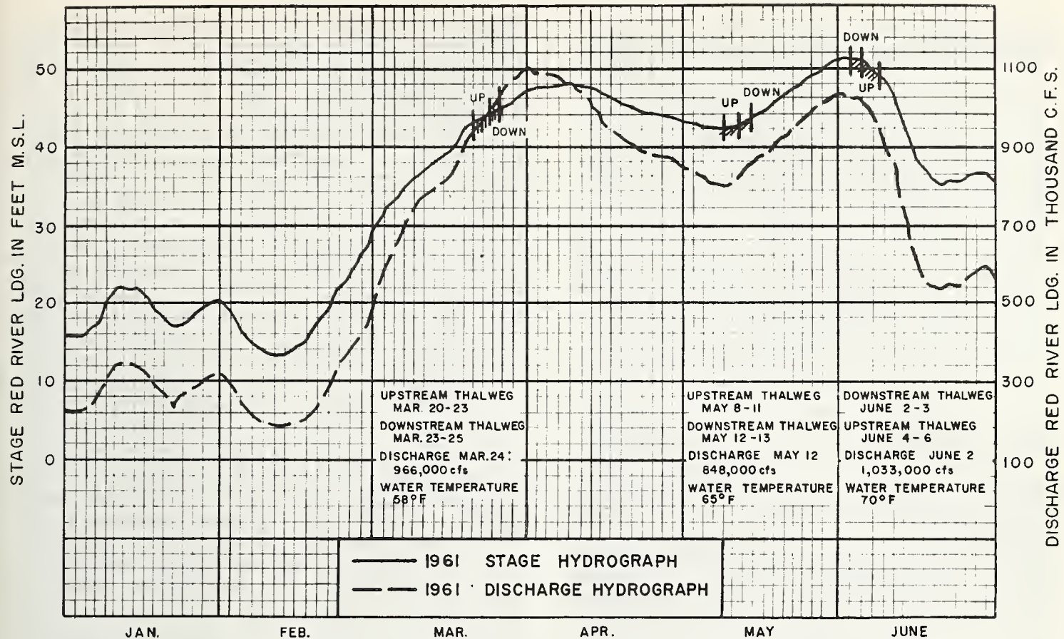
FIGURE 6. — 1961 flood: Stage and discharge hydrographs, Mississippi River, Red River Landing, La.
