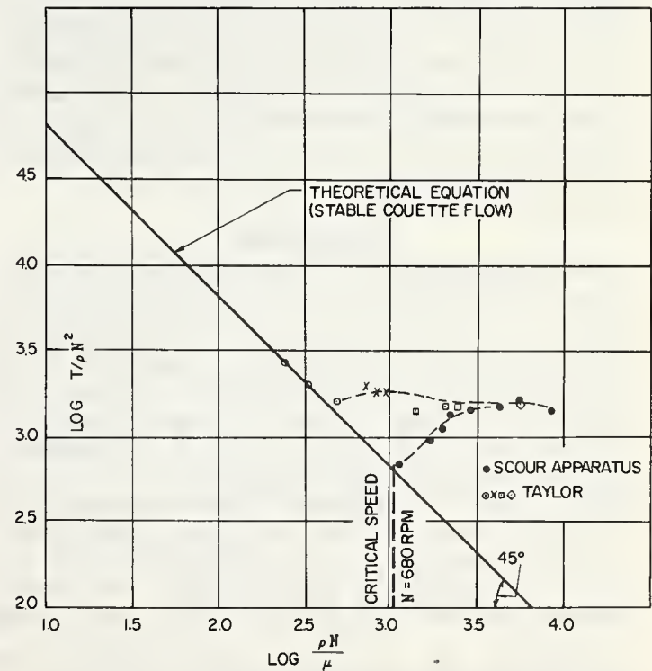
FIGURE 4.— T/\rho N^2 vs. \rho N/\mu . (After Taylor, 1960.)
