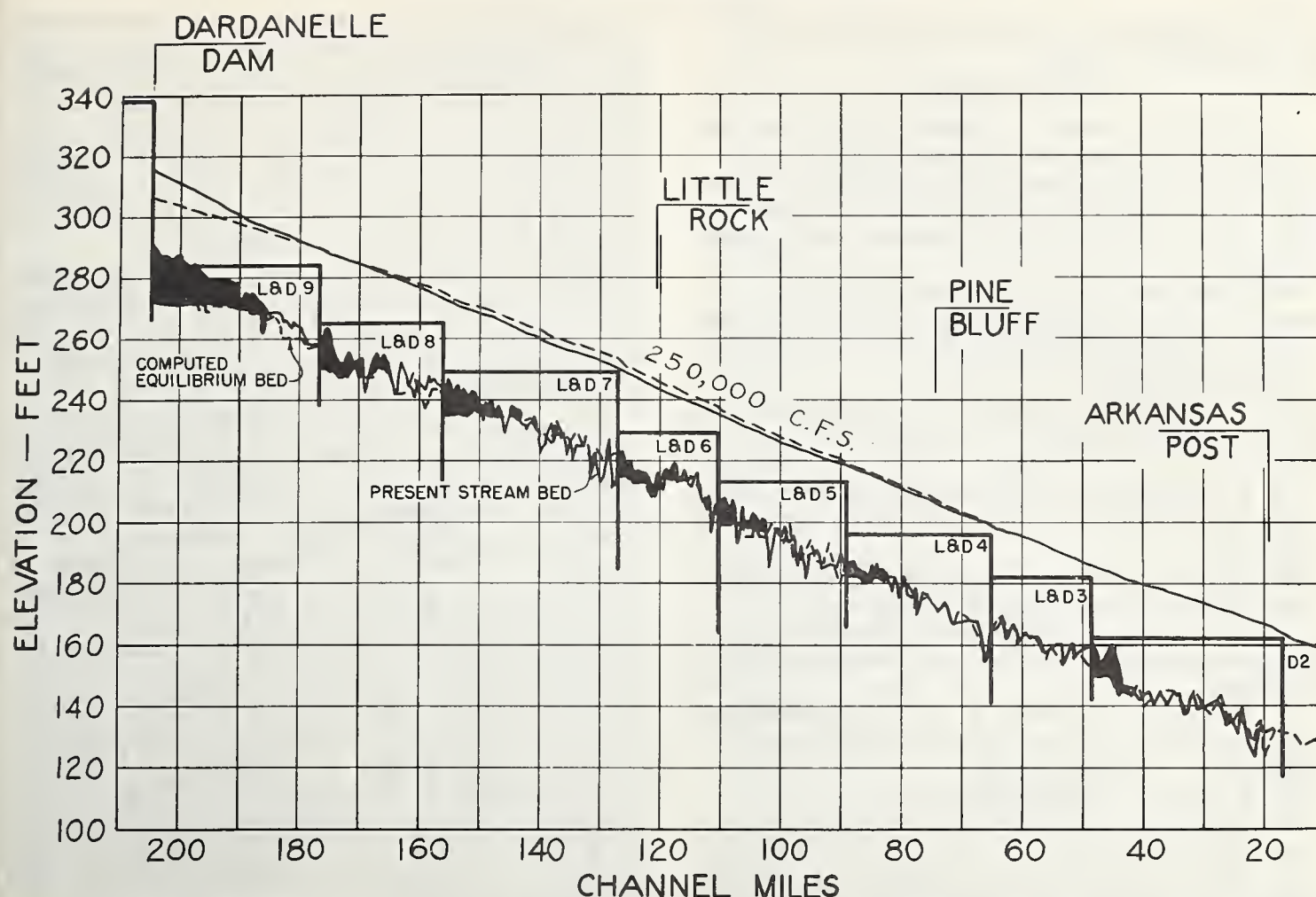
FIGURE 12.— Profiles for existing conditions and computed modified regime conditions between Arkansas Post and Dardanelle Dam.
