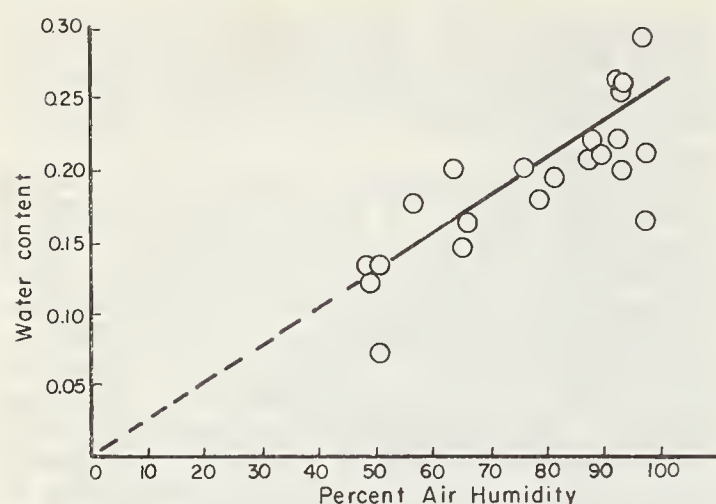
FIGURE 13.—Relation between water content of sand and air humidity.
