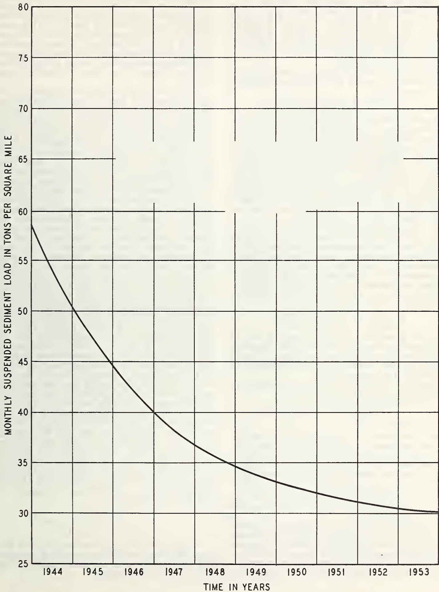
FIGURE 1.— Chestuee Creek Watershed: Average monthly sediment load — regression with time (equation 1).
