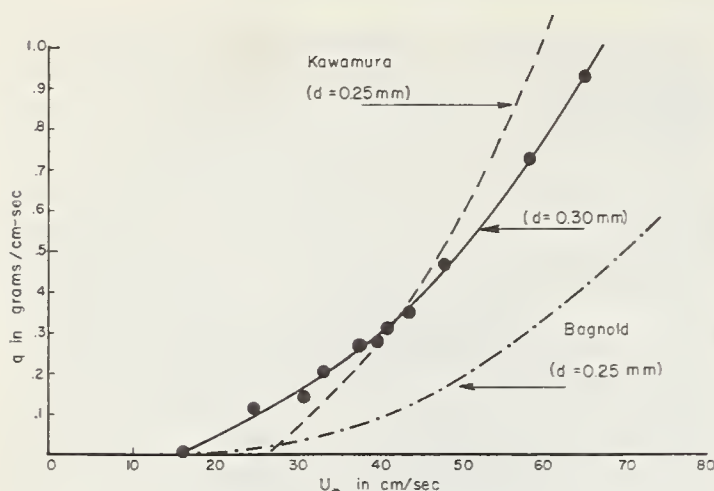
FIGURE 8.— Comparison of experimental data on sand B ( d = 0.30 mm.) with the experiments of Bagnold and Kawamura on a sand 0.25 mm. in diameter.
