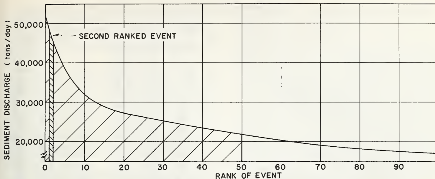
FIGURE 7.—Long term sediment discharge-duration curve representing top-ranked events, watershed 32, Pigeon Roost Creek Basin, Miss.
