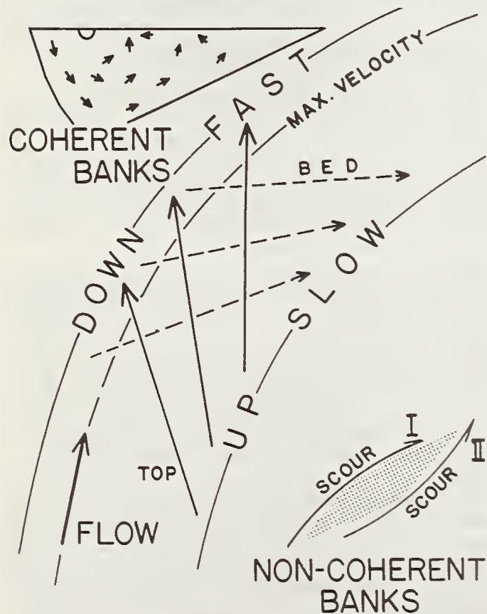
FIGURE 3. — Directions of scour patterns.
