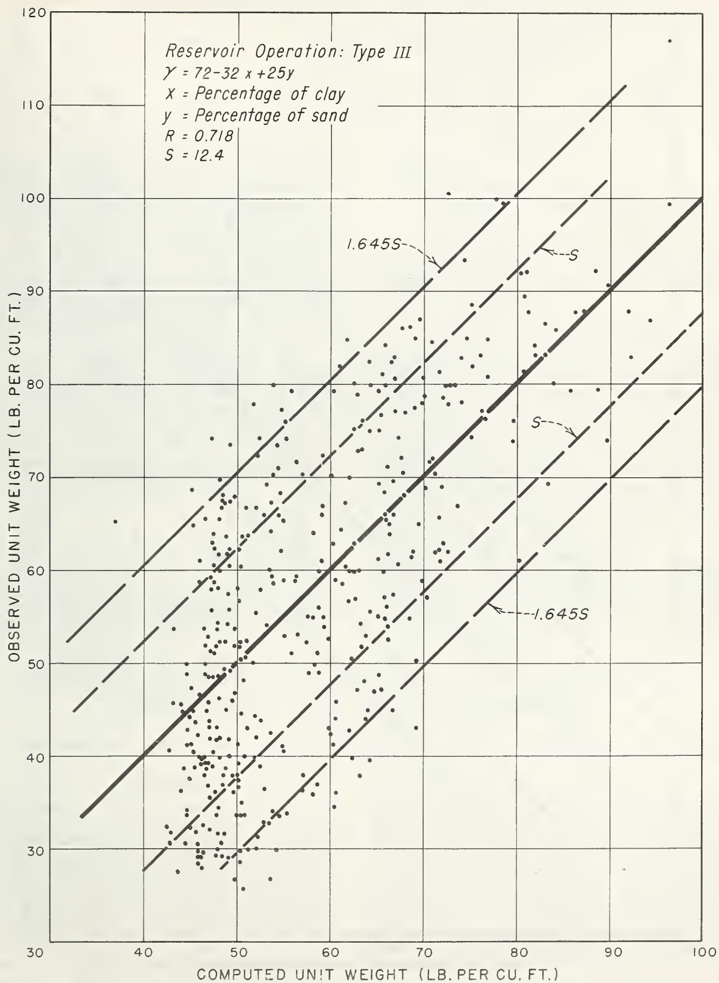
FIGURE 3. — Correlation of observed vs. computed unit weights. Reservoir operation: Type III.
