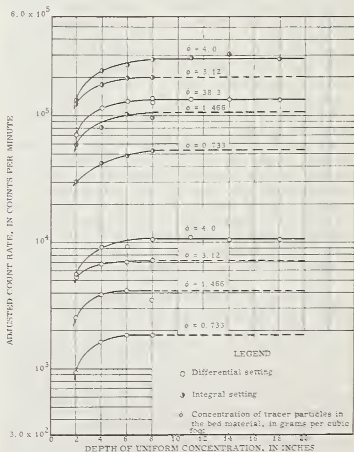
FIGURE 3.—Variation in adjusted count rate with the depth to which different concentrations of tracer particles are uniformly mixed.
