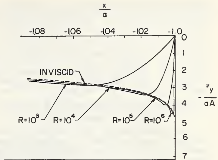
FIGURE 4.—Profiles of viscous secondary flow in the plane of symmetry in front of circular cylinder.
