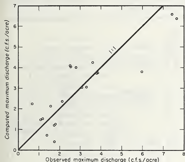
FIGURE 3.—Actual vs. predicted highest annual flood peak.
