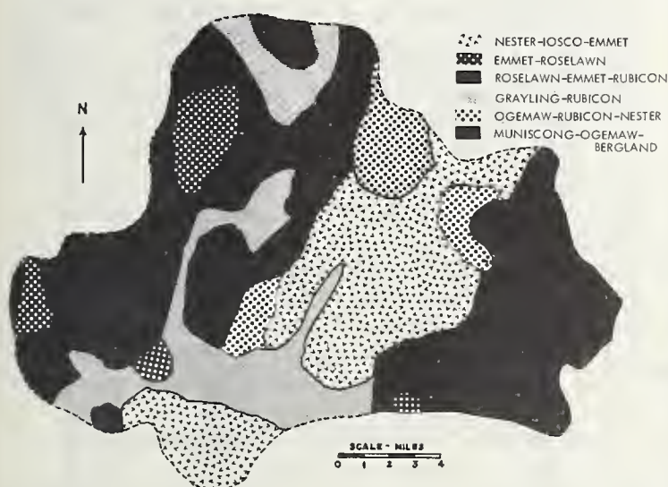
FIGURE 3.—Major soil associations, Tobacco River Watershed. (After Veatch (10)).
