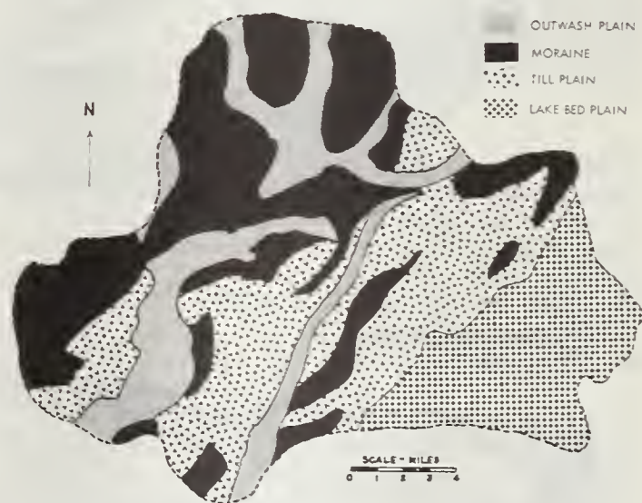
FIGURE 2. — Surface geology, Tobacco River Watershed. (After Martin (9)).
