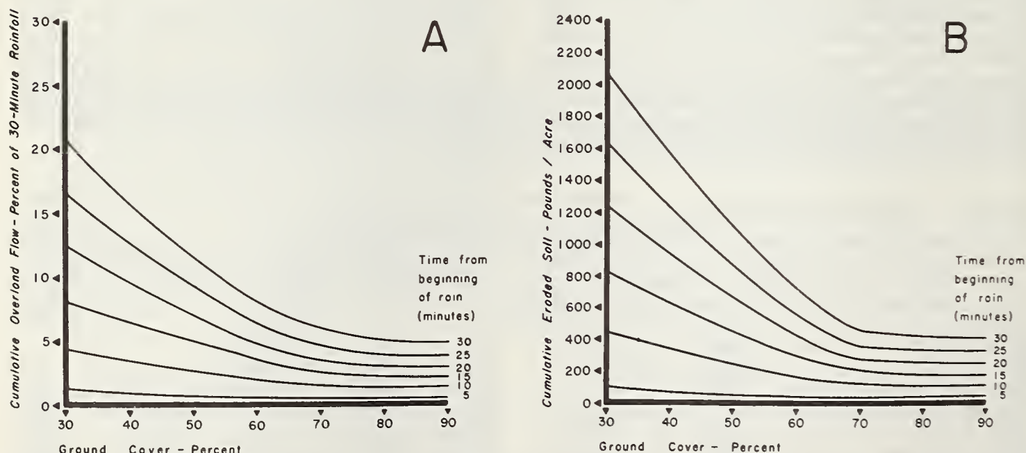
FIGURE 5.—A, Cumulative overland flow; and B, cumulative soil eroded by a simulated rainfall of 1.87 inches for 30 minutes by 5-minute periods in relation to ground-cover density. This study was conducted on wheatgrass range sites on soils derived from granite (17).
