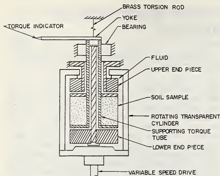
FIGURE 1. — Diagram of modified rotating cylinder test apparatus.
