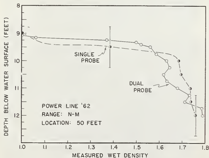
FIGURE 6.—A depth-density profile for a sediment as measured by the gamma and dual probes: Range N-M, 50 feet, Power Line Reservoir, Lafayette County, Miss.
