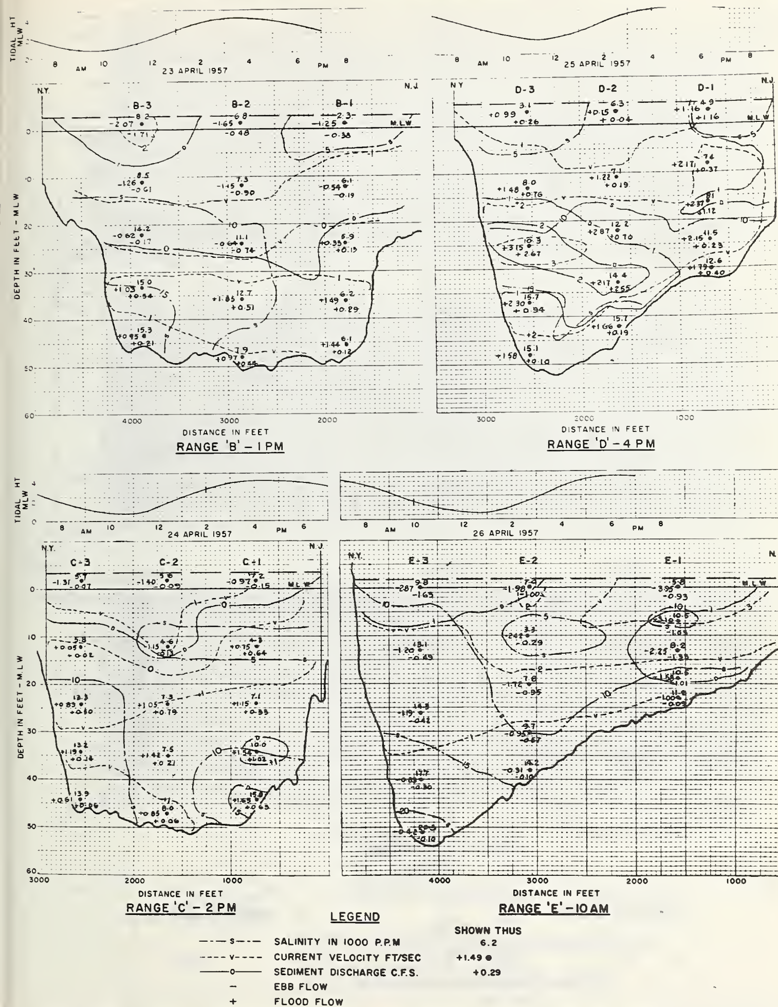
FIGURE 14. — Current velocity, sediment discharge, and salinity at mid-velocity.
