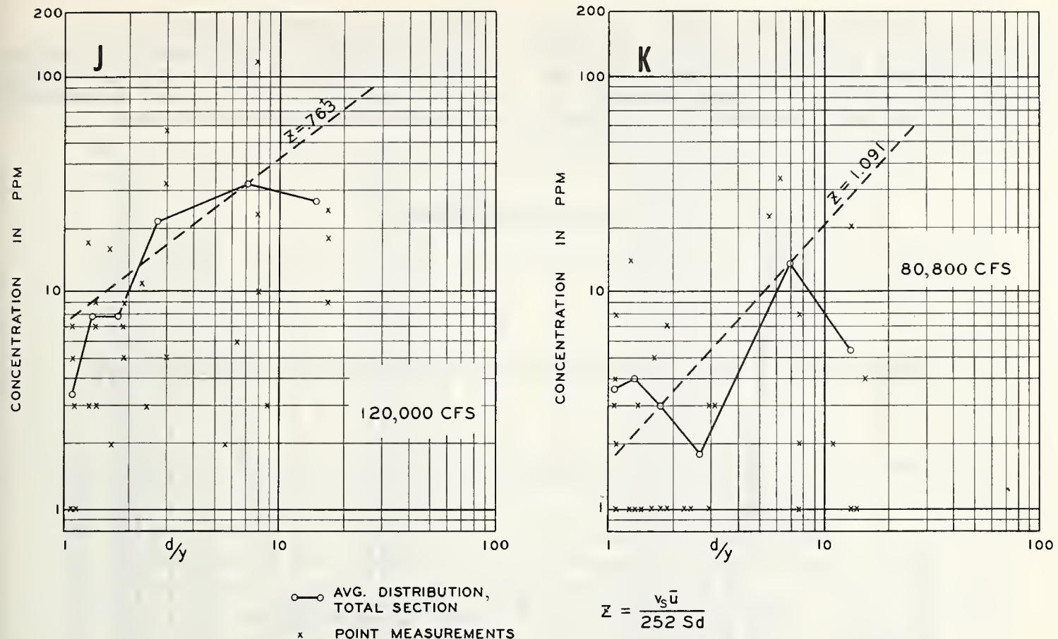
FIGURE 3 (continued).—Measured suspended fine sand at 6 levels at each of 5 verticals in cross section of Atchafalaya River at Simmesport, La.: J, for 120,000 c.f.s.; and K, for 80,800 c.f.s.
