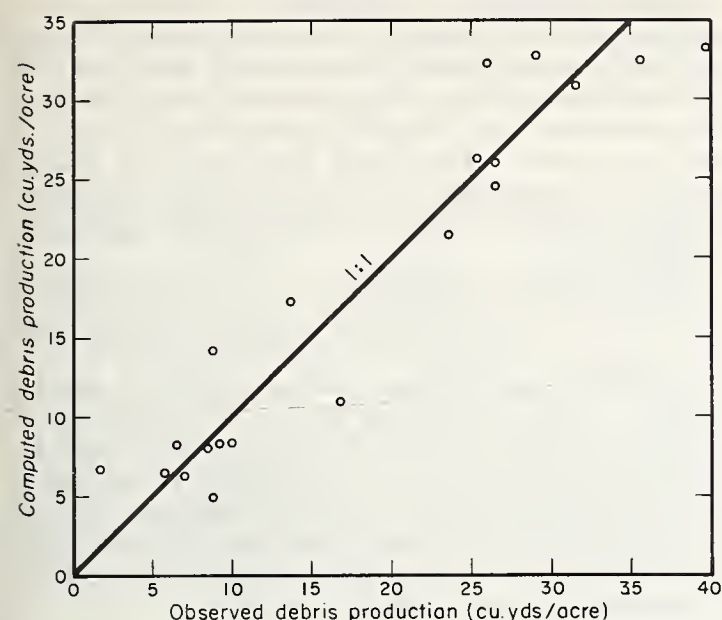
FIGURE 2.—Actual vs. predicted annual debris production (1962).
