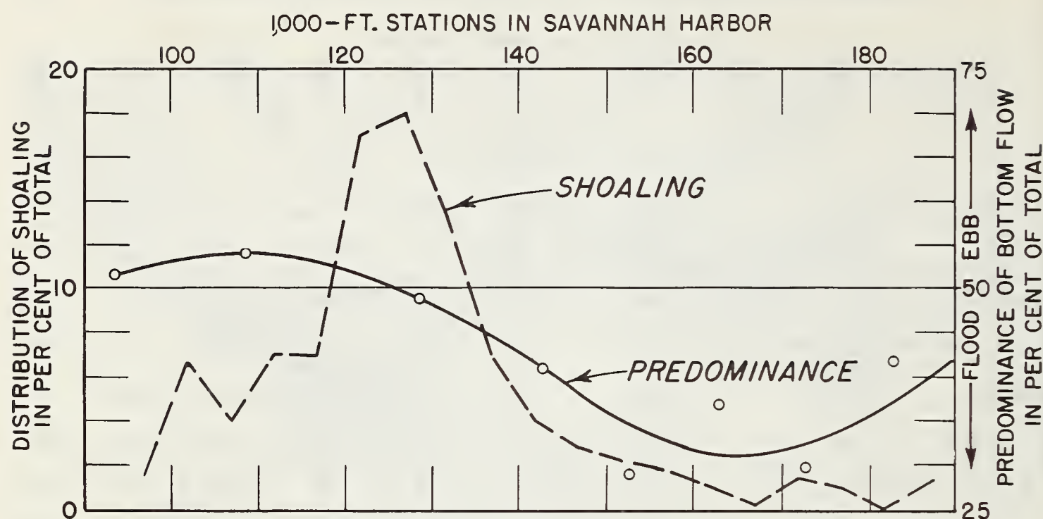
FIGURE 3. — Relation of shoaling and predominance of bottom flow.
