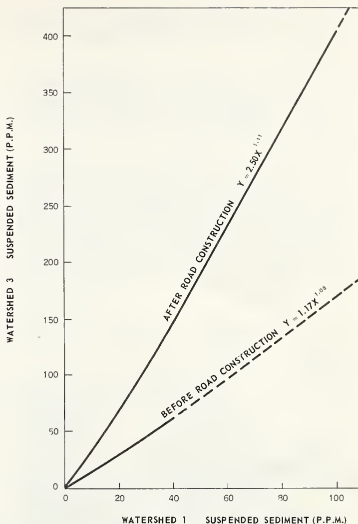
FIGURE 4.—Suspended sediment concentrations: Watersheds 1 and 3, before and after road construction.
