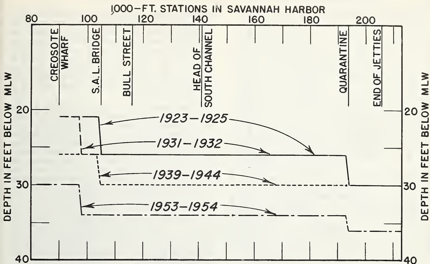
FIGURE 4. — Past and present channel depths.
