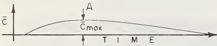
FIGURE 4. — Theoretical relationship of concentration of tracer material versus time.
