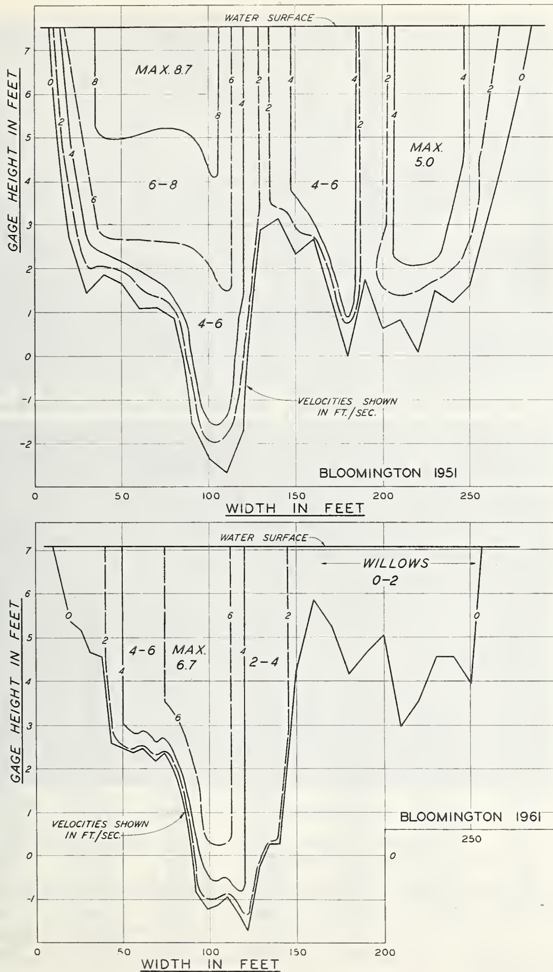
FIGURE 3. — Measured velocities of Republic River near Bloomington, 1951 and 1961.
