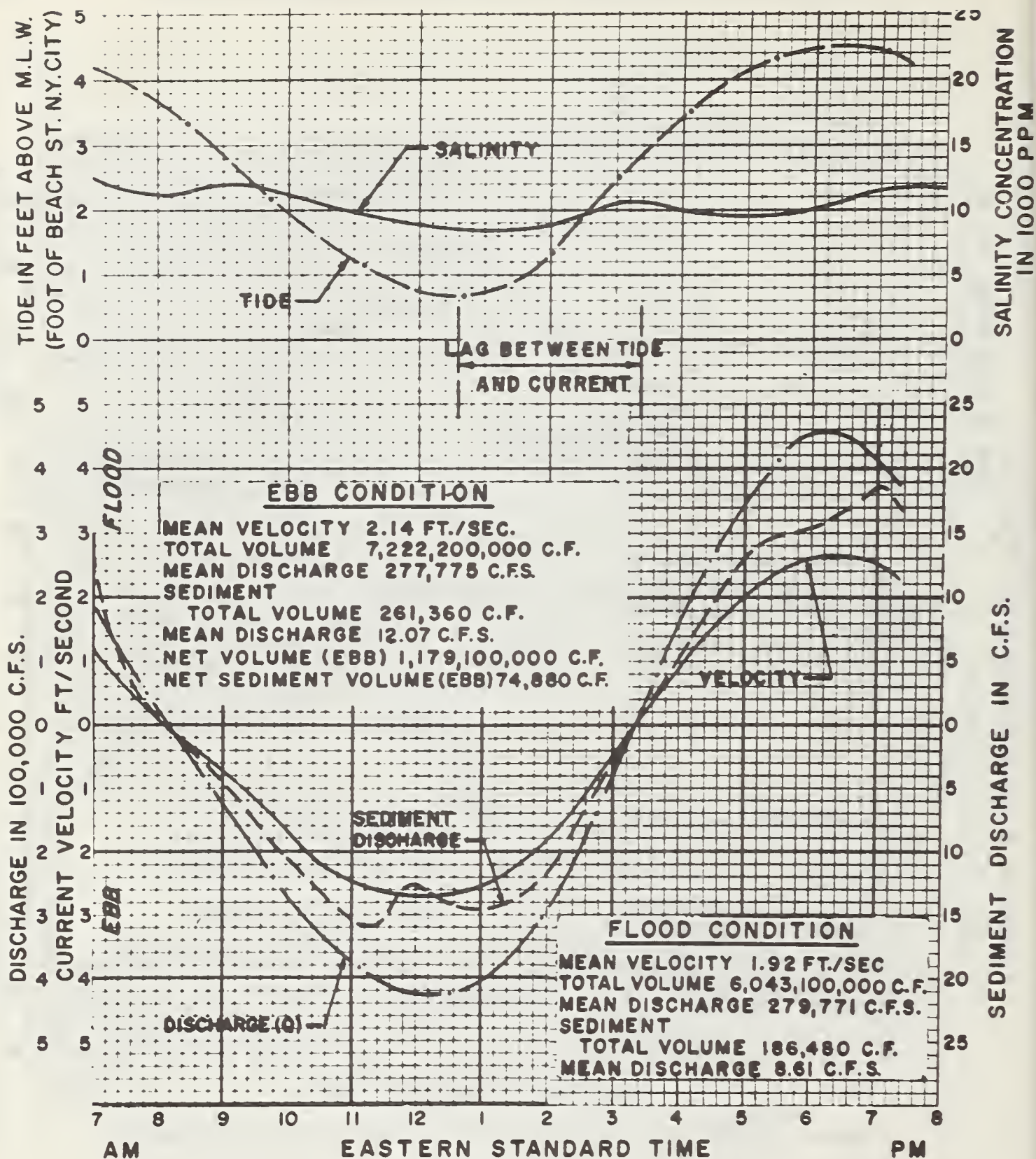
FIGURE 19. — Variation in average velocity, salinity, and sediment, range E, 26 April 1957.
