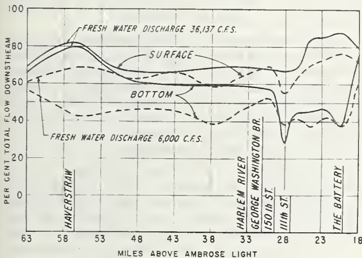
FIGURE 4.—Flow predominance at surface and bottom of Hudson River within the New York Harbor.
