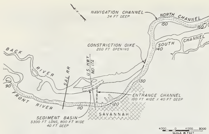
FIGURE 4.—Sediment basin with entrance channel at station 116.
