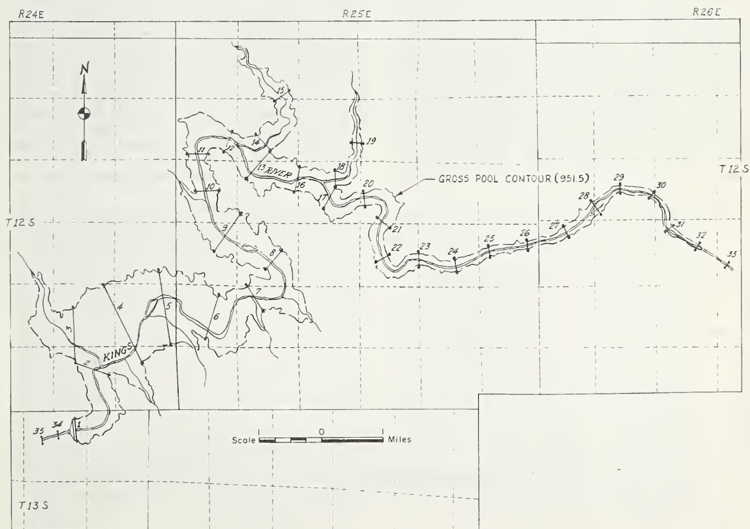
FIGURE 2. — Sediment ranges, Pine Flat Reservoir.
