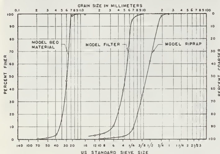
FIGURE 4. — Mechanical analysis of the sand and crushed rock used for model construction.
