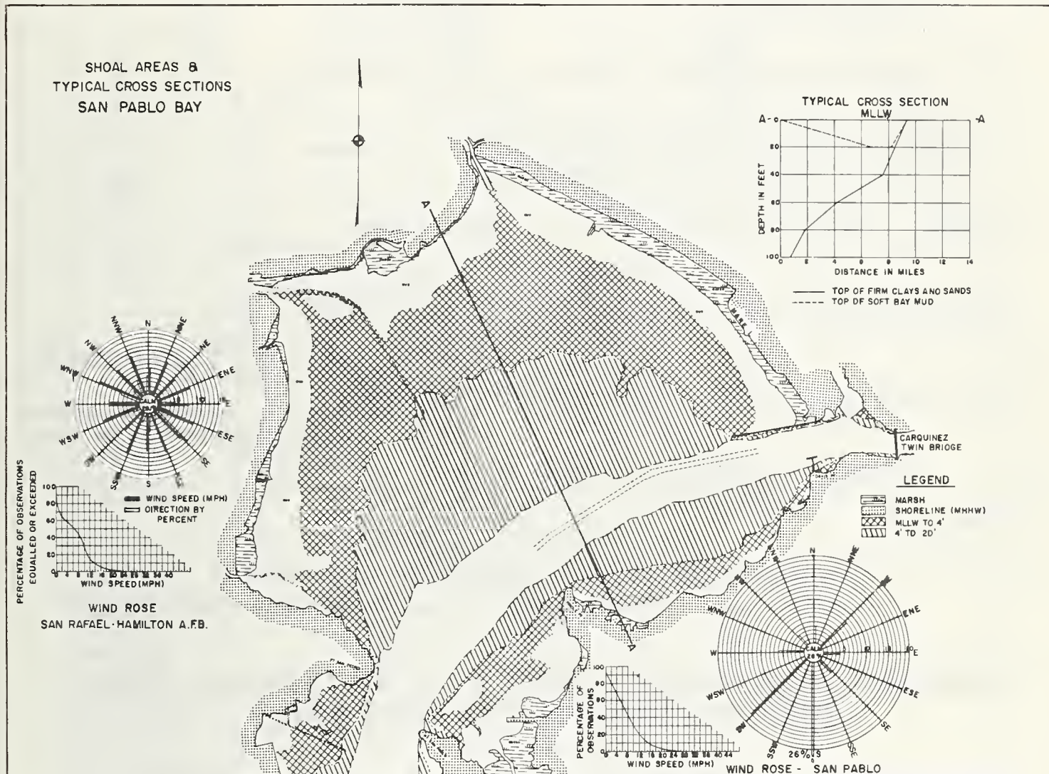
FIGURE 19. — Shoal areas, wind roses, and typical cross section of San Pablo Bay.
