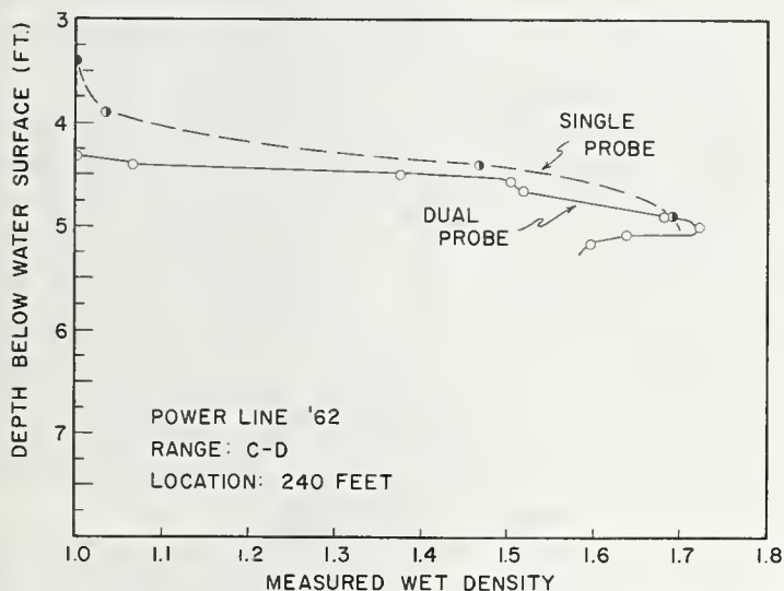
FIGURE 9.—A depth-density profile of a sediment measured with a gamma and a dual probe: Range C-D, 240 feet, Power Line Reservoir, Lafayette County, Miss.
