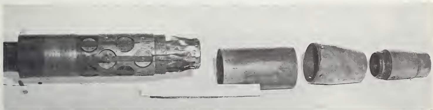
FIGURE 3. — Exploded view of sampler head, Swedish Foil Sampler. Left to right: sampler magazine, magazine cover, cutting shoe housing, cutting shoe.
