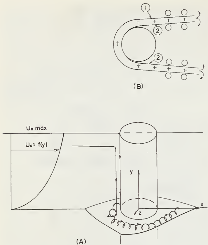
FIGURE 2. — Cylindrical pier with nonuniform approach velocity.
