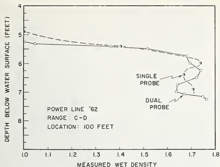
FIGURE 8.—A depth-density profile of a sediment measured with a gamma and a dual probe: Range C-D, 100 feet, Power Line Reservoir, Lafayette County, Miss.
