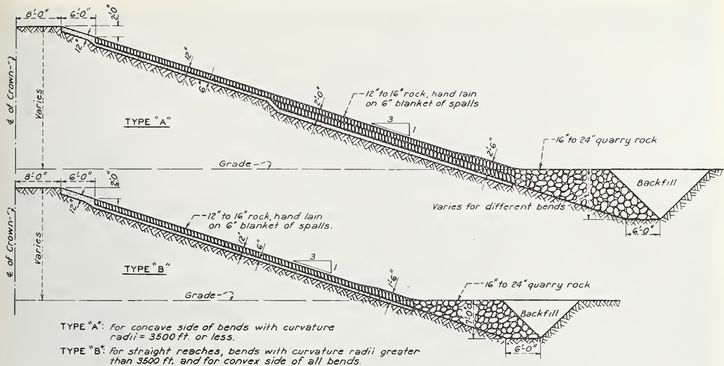
FIGURE 1. — Rock paving bank protection; typical section.
