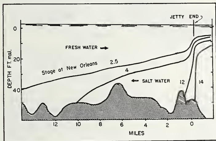
FIGURE 2. — Longitudinal profile of lower Mississippi River.
