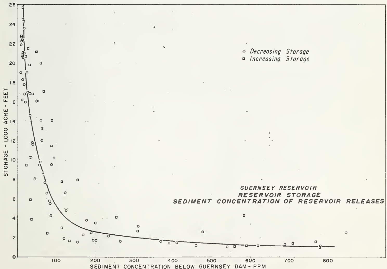
FIGURE 8.—Reservoir storage-sediment concentration of reservoir releases.
