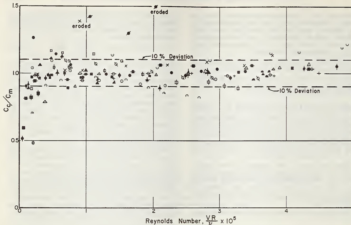
FIGURE 3. — Ratio of calculated to measured values of Chezy's C .
