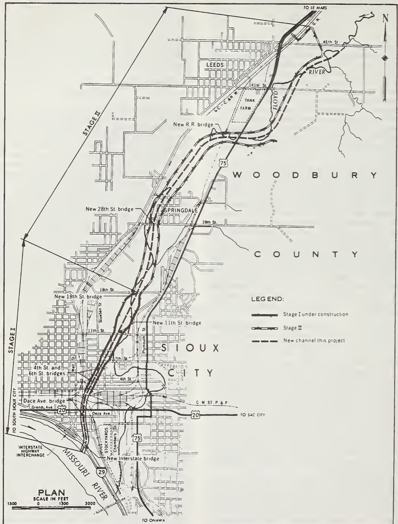
FIGURE 1. — General plan of the Floyd River Flood Control project.
