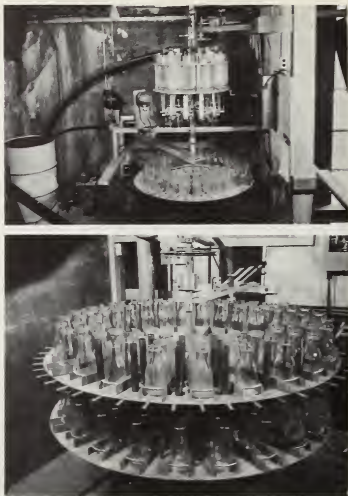
FIGURE 2.—Sample handling systems for pumping sampler: Top, Sediment volume recording system; bottom, individual-sample bottling system.
