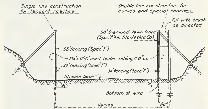
FIGURE 3. — Pipe-and-wire bank protection; typical section.
