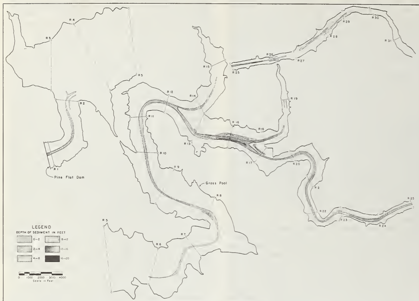
FIGURE 4. — Sediment deposition in Pine Flat Reservoir, May 1952 to November 1956.
