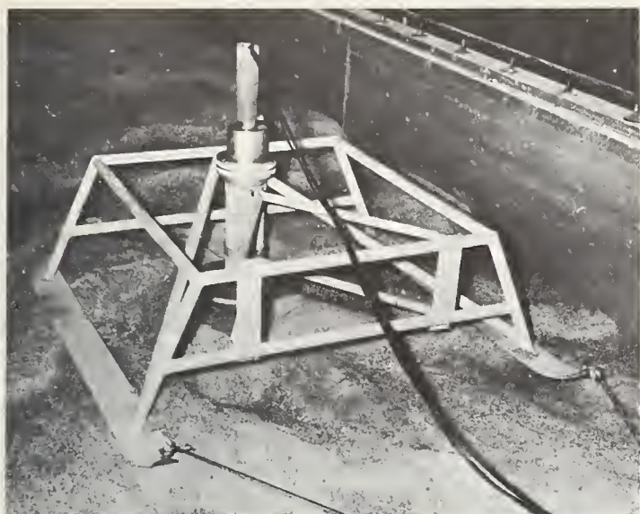
FIGURE 2.—Sled and scintillation detector. Note the parallelogram linkage that allows the detector to move independently of the sled and the wooden dish-shaped piece that supports the detector on the bed.
