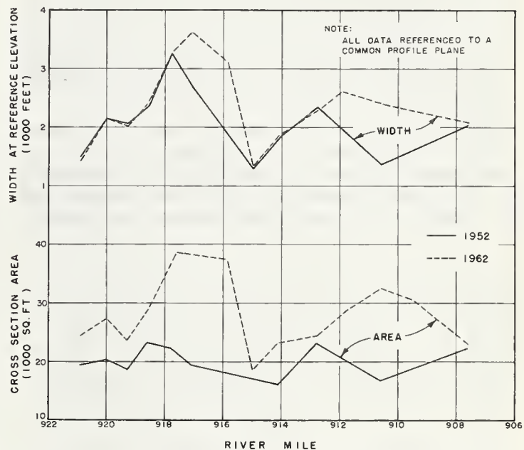
FIGURE 5.—Changes in cross sectional width and area as observed at degradation ranges between 1952 and 1962.
