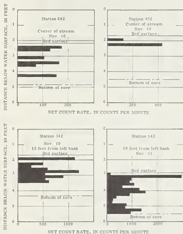
FIGURE 8. — Vertical distribution of labeled particles at selected verticals on Nov. 10 and 11, 1960.
