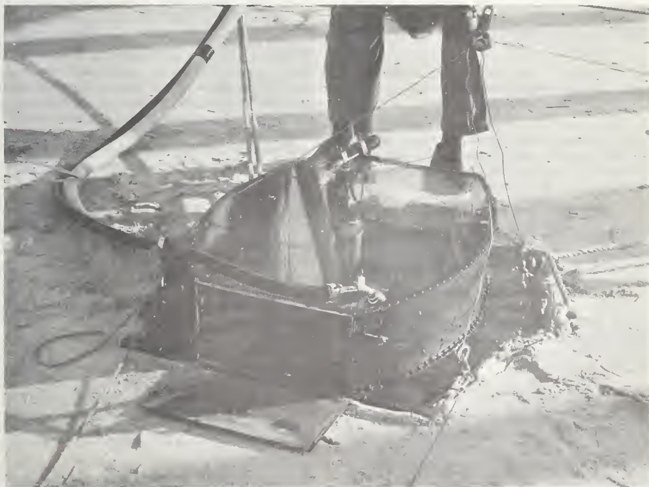
FIGURE 3.—Bedload trap.
