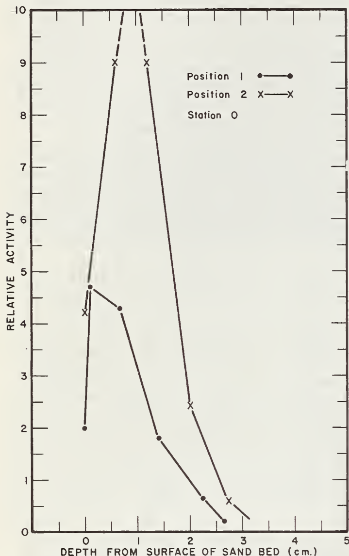
FIGURE 5.—Vertical distribution of scandium-46 labeled sand in the channel bed after 125 hours of flume operation (station 0).
