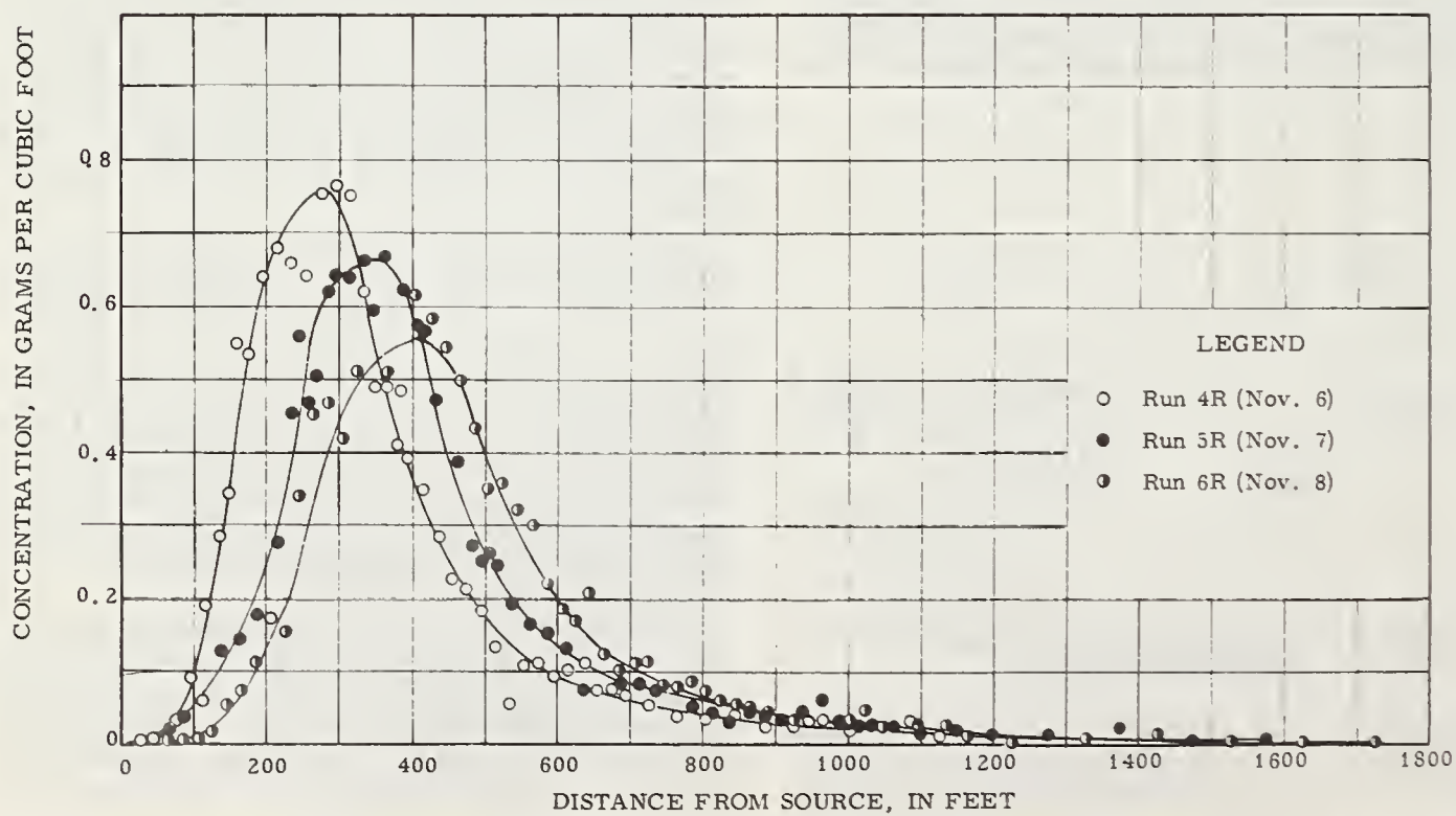
FIGURE 5.— Longitudinal distribution of labeled particles along the right side of the channel, Nov. 3 to 8, 1960.
