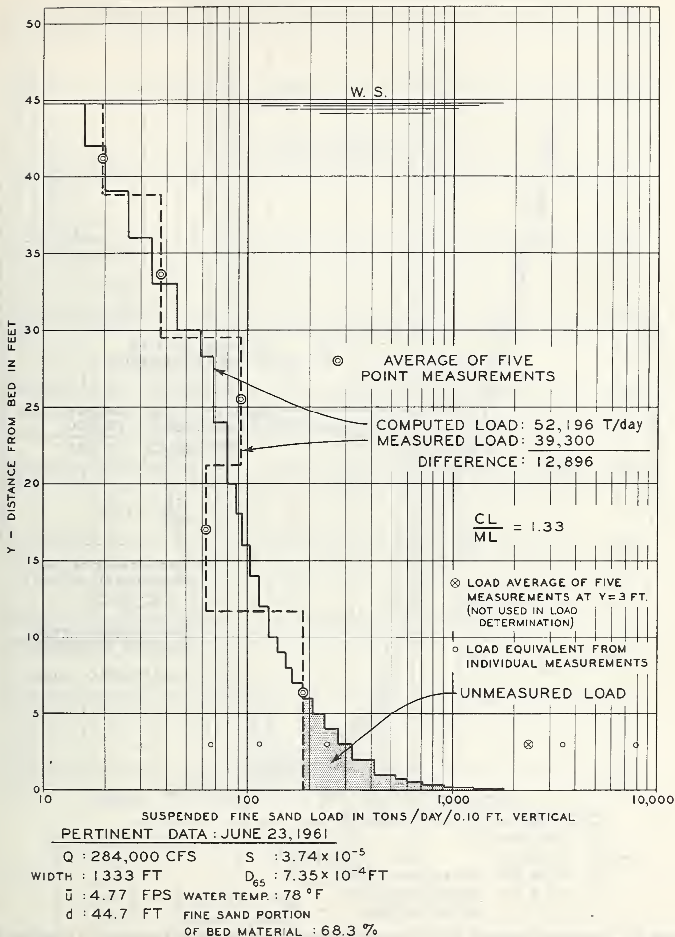
FIGURE 9.—Computed, measured, and unmeasured suspended fine sand load at Simmesport, Atchafalaya River, June 23, 1961.
