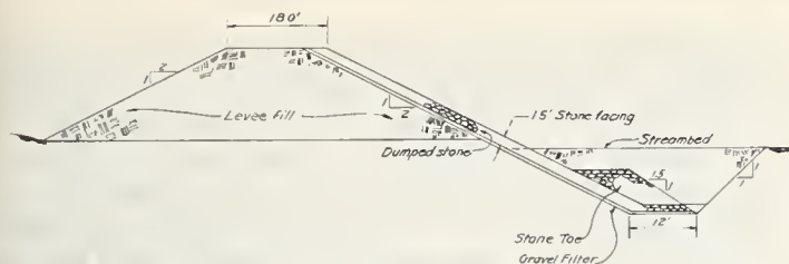
FIGURE 18.—Santa Ana River typical levee section.
