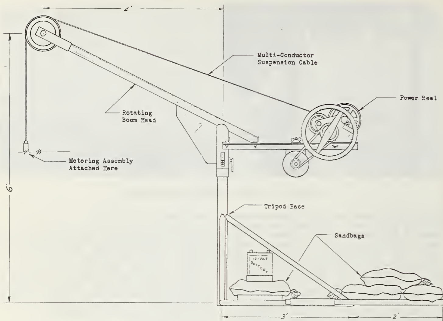
FIGURE 13. — Pillar crane.
