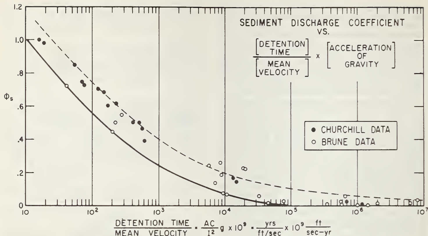
FIGURE 3. — Sediment discharge coefficient.
