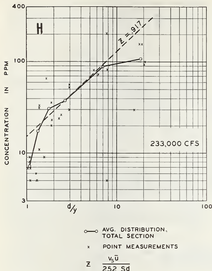
FIGURE 3 (continued).—Measured suspended fine sand at 6 levels at each of 5 verticals in cross section of Atchafalaya River at Simmesport, La.: H, for 233,000 c.f.s.; I, for 218,000 c.f.s.
