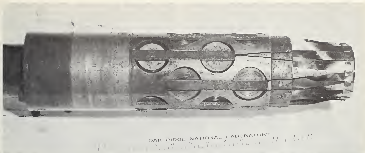
FIGURE 2. — Close-up of sampler magazine, Swedish Foil Sampler.
