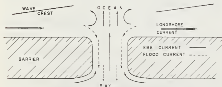
FIGURE 1. — Typical current action of barrier and inlet shore.
