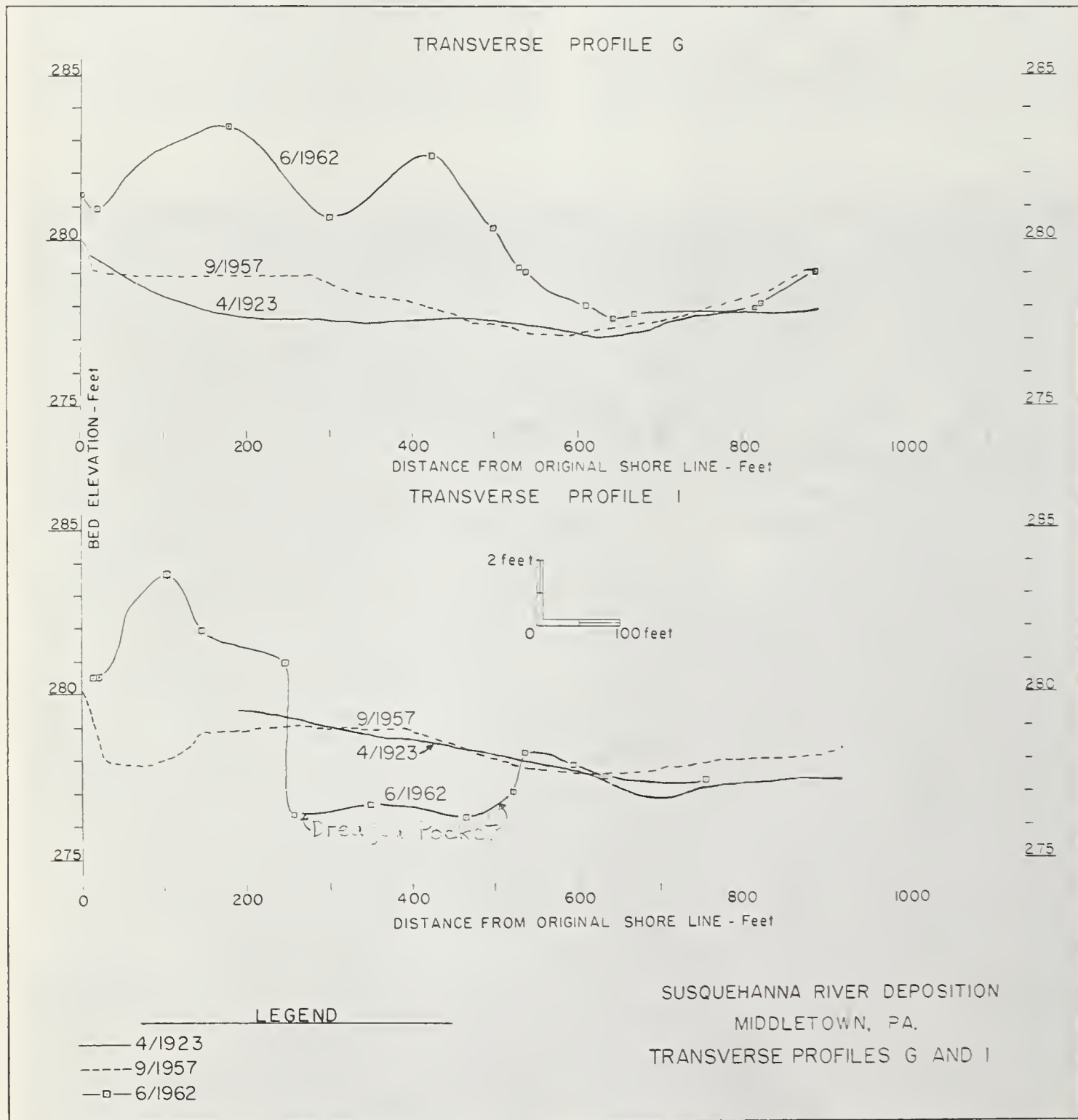
FIGURE 7. — Susquehanna River deposition at Middletown; transverse profiles G and I.
