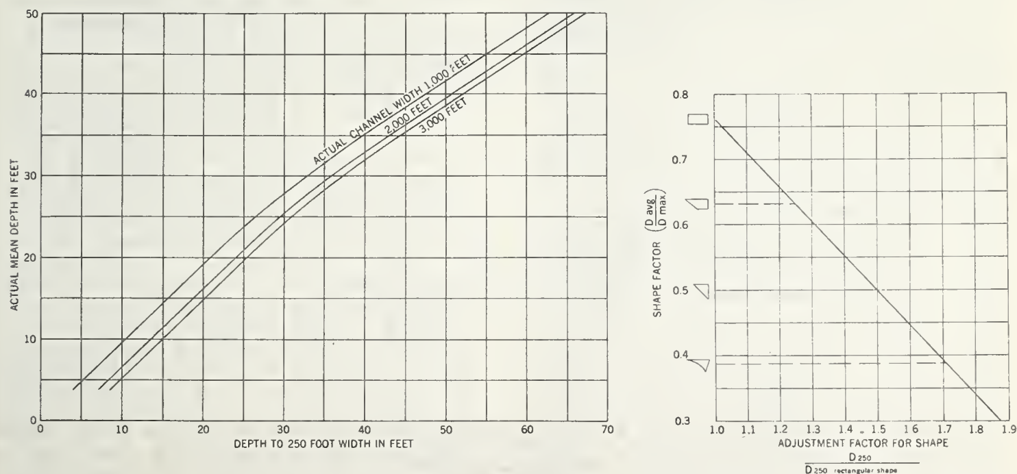
FIGURE 9.—Left, relation between mean channel depth, width, and depth to the highest point in the lowest 250-foot width of near-rectangular cross sections; right, adjustment factors for determining depth to the lowest 250-foot width for cross sections of shapes other than near-rectangular.
