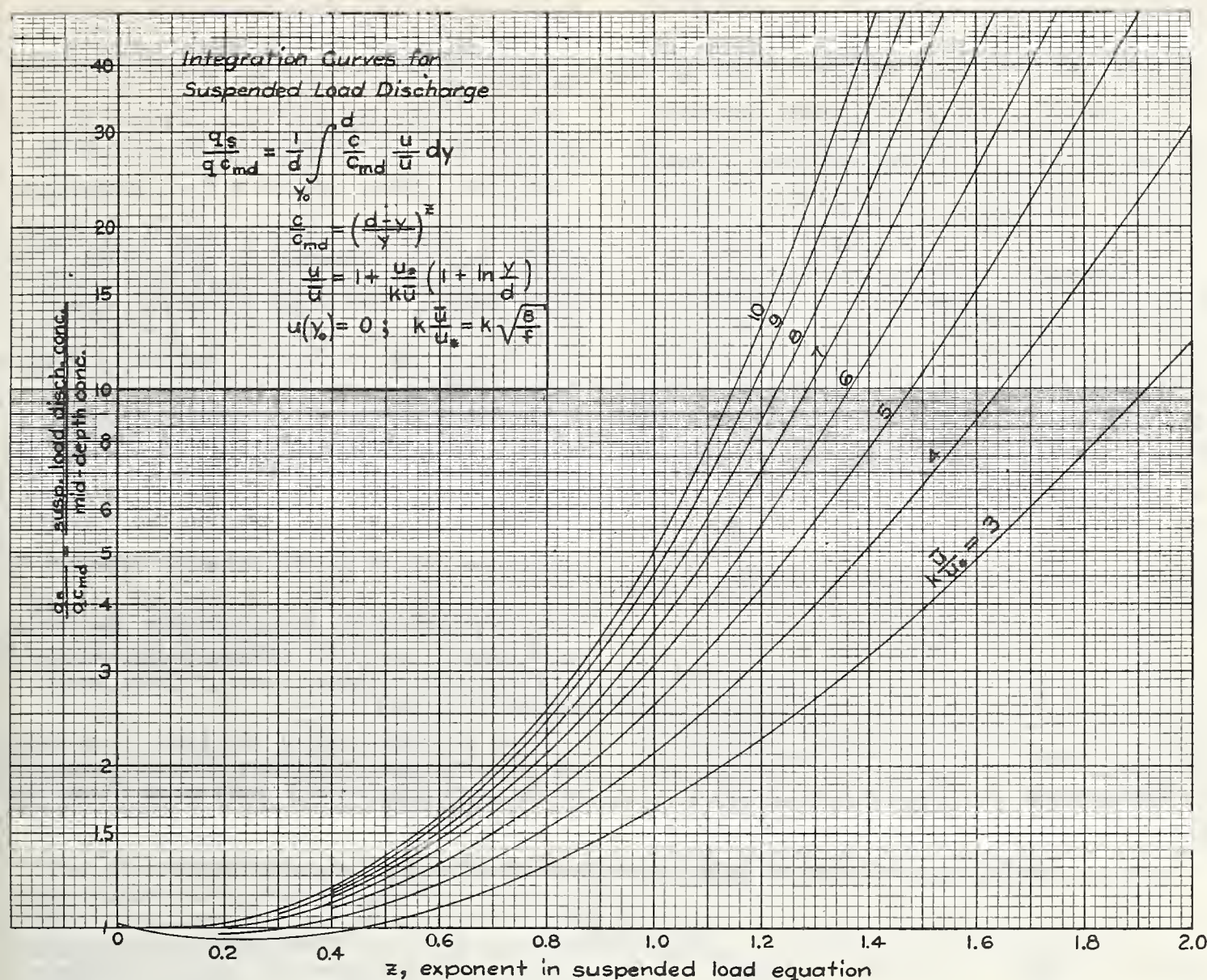
FIGURE 2.— Integration curves for suspended load discharge by equations 15 and 21.
