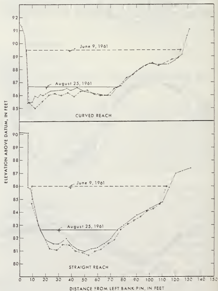
FIGURE 8.—Typical cross-sectional data, Popo Agie River, 1961.
