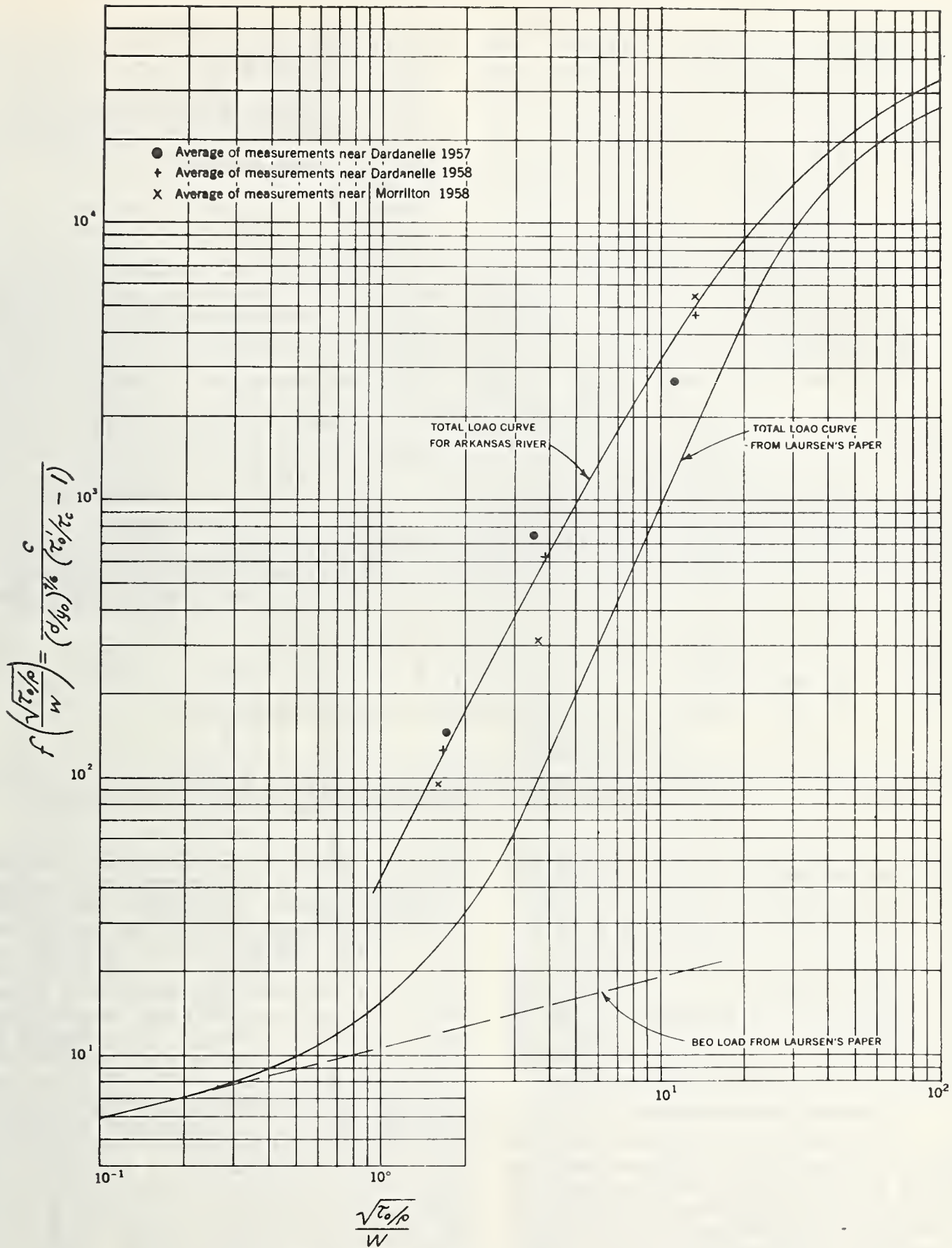
FIGURE 3. — Laursen sediment load function.
