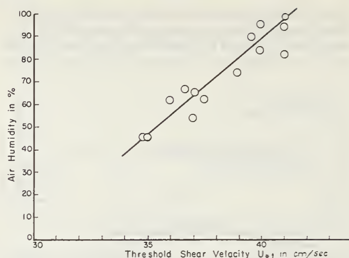
FIGURE 15.—Relation between threshold shear velocity and air humidity (sand A).
