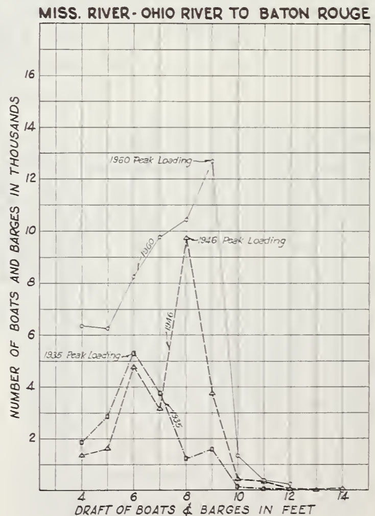
FIGURE 5.—Vessel draft increase.
