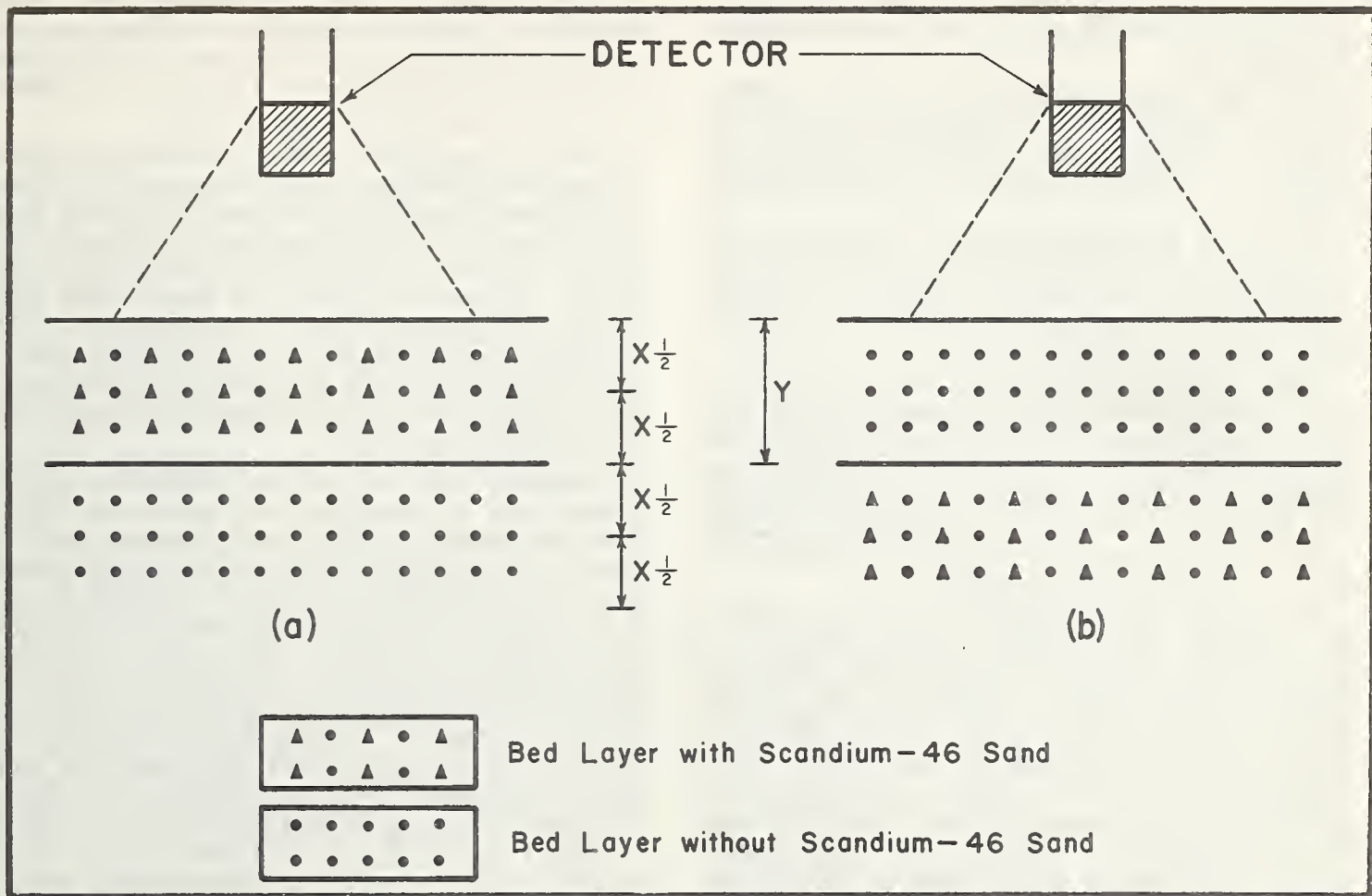
FIGURE 9. — Ideal vertical distribution of labeled sand: a , Uniform burial without overlying sediment; b , uniform burial overlain by nonradioactive sediment.
