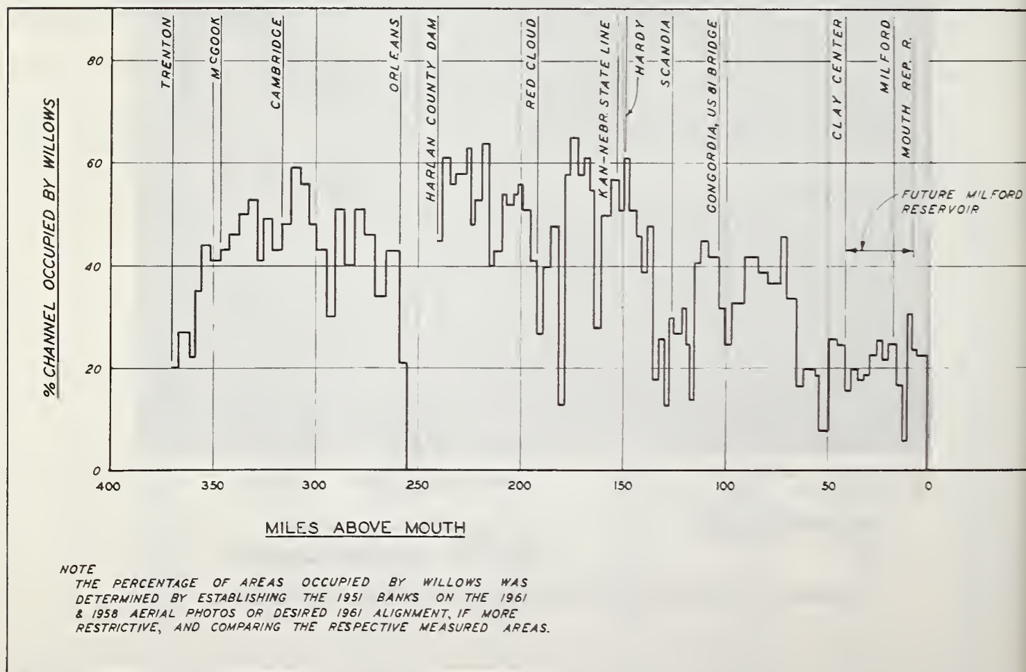
FIGURE 5. — Percentage of channel occupied by willows in Republican River.
