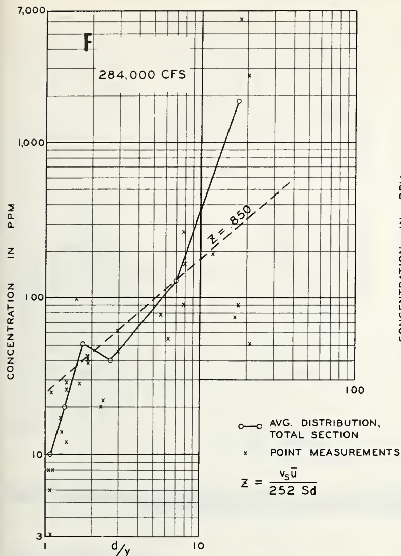
FIGURE 3 (continued).—Measured suspended fine sand at 6 levels at each of 5 verticals in cross section of Atchafalaya River at Simmesport, La.: F, for 284,000 c.f.s.; G, for 254,000 c.f.s.
