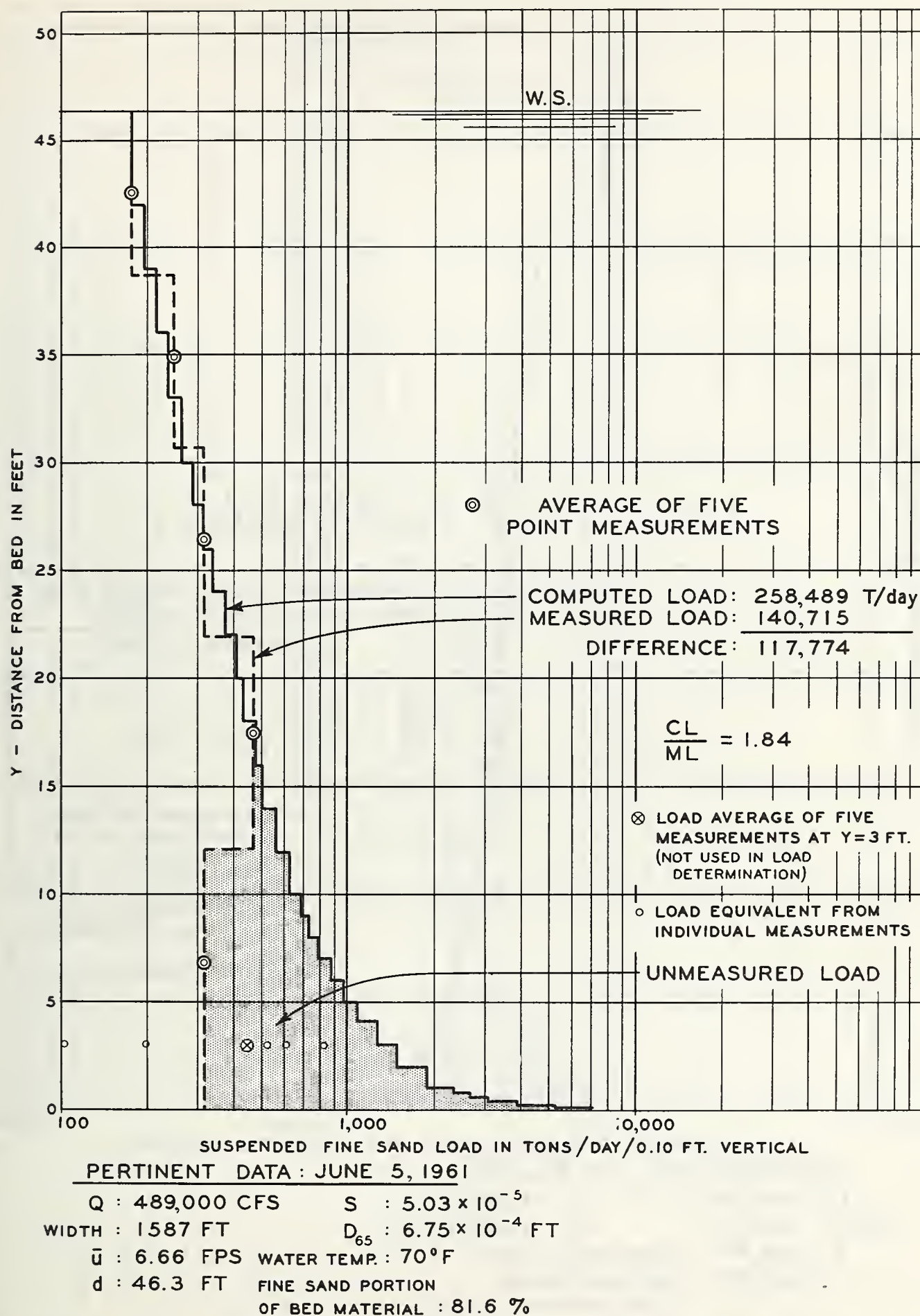
FIGURE 5.— Computed, measured, and unmeasured suspended fine sand load at Simmesport, Atchafalaya River, June 5, 1961.
