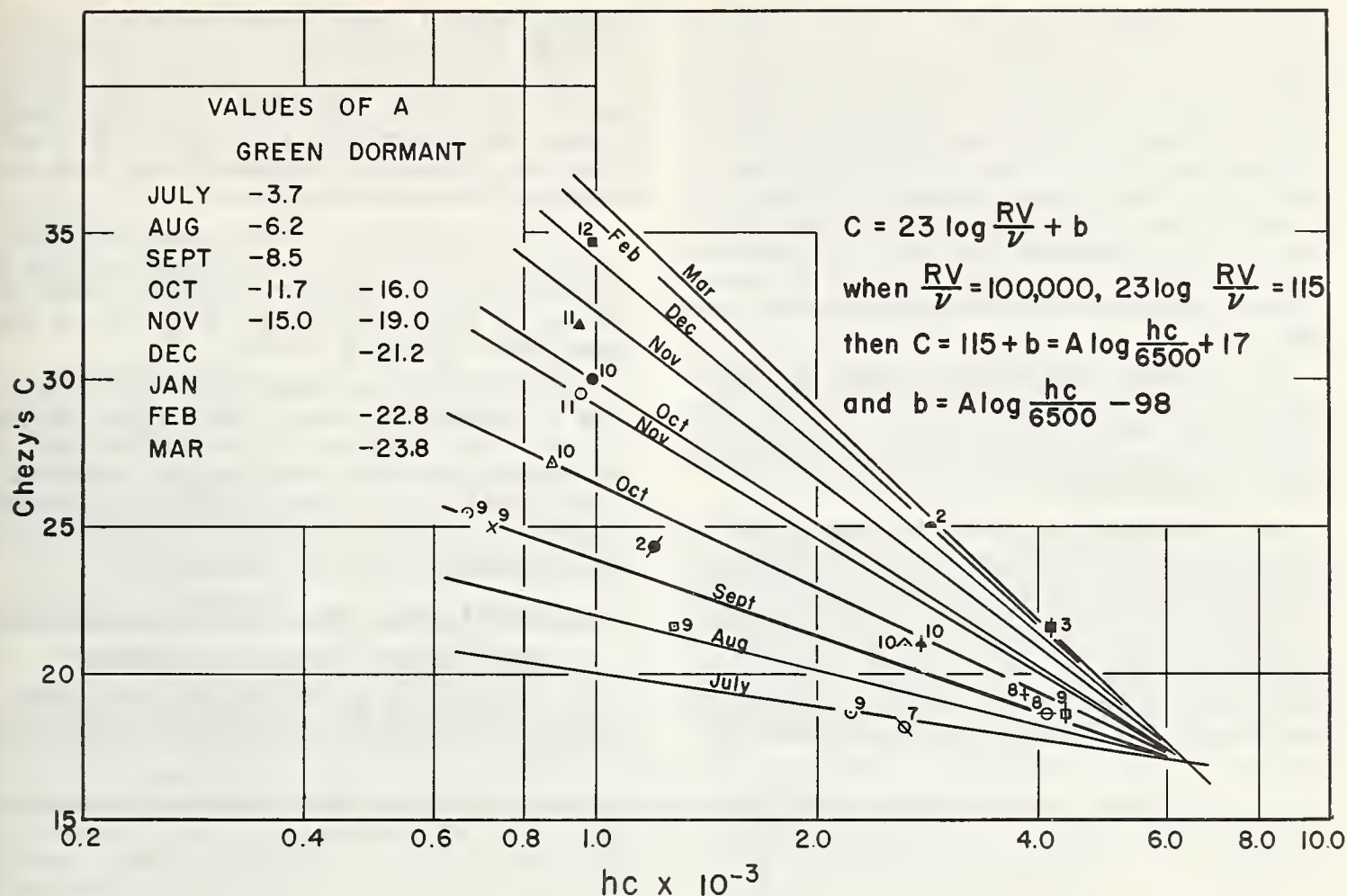
FIGURE 4.—Variation of Chezy's C with vegetation count and height at Re=VR/v=100,000 (Spartanburg bermudagrass channels).
