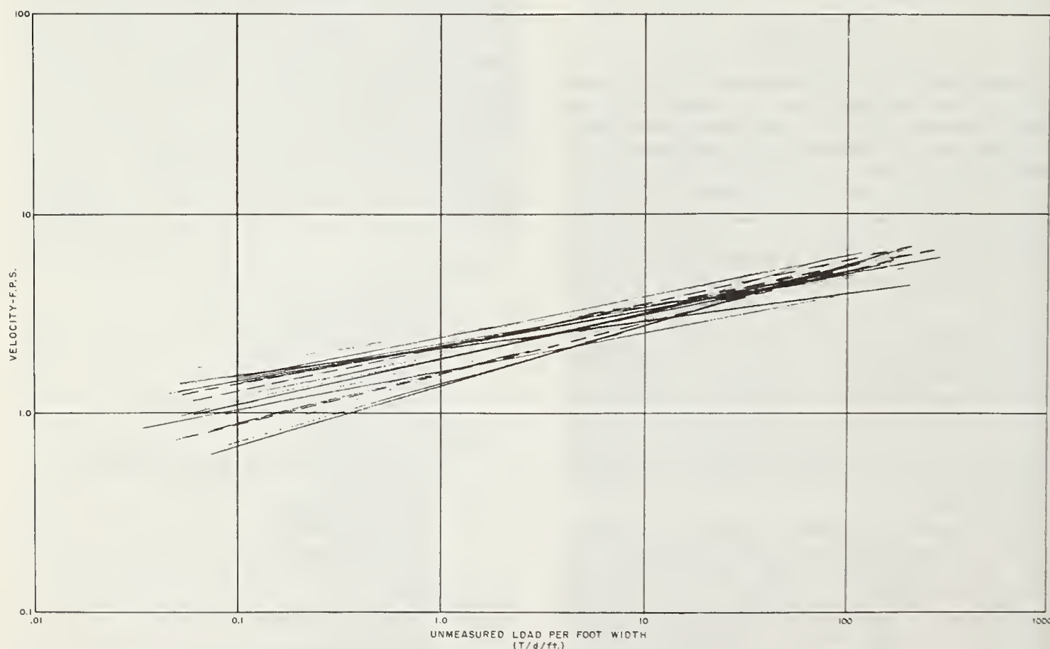
FIGURE 1. — Composite plot of relation between unmeasured sediment load and mean velocity.
