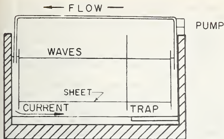
FIGURE 8. — Cross section of wave tank for littoral drift experiments.
