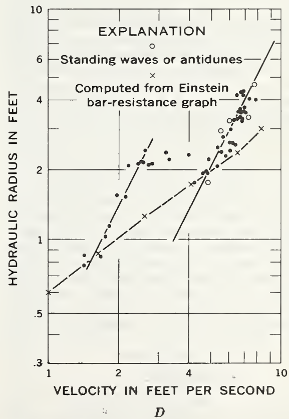
FIGURE 1.—Relation of velocity to hydraulic radius: A, Middle Loup River at St. Paul, Nebr.; B, Huerfano River near Undercliffe, Colo.; C, Pigeon Roost Creek near Byhalia, Miss.; and D, Rio Grande near Bernalillo, N. Mex.
