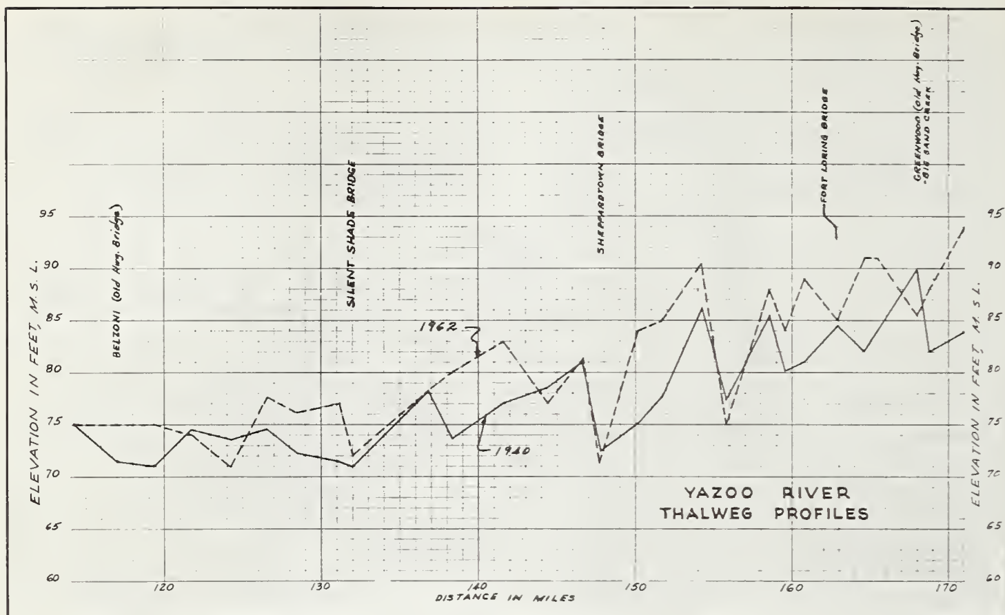
FIGURE 7. — Thalweg profiles of the Yazoo River, 1940 and 1962.
