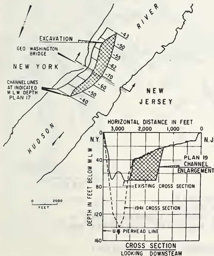
FIGURE 28.—Comprehensive dredging to 1941 cross section.
