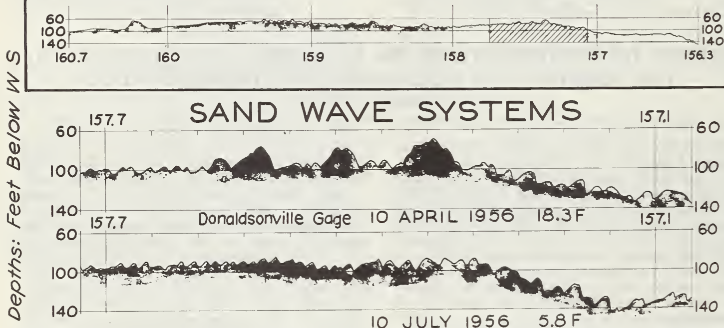
FIGURE 1. — Segments of sailing-line (thalweg) profiles at 18.3 and 5.8 feet, respectively, Donaldsonville gage, showing sand-wave systems.
