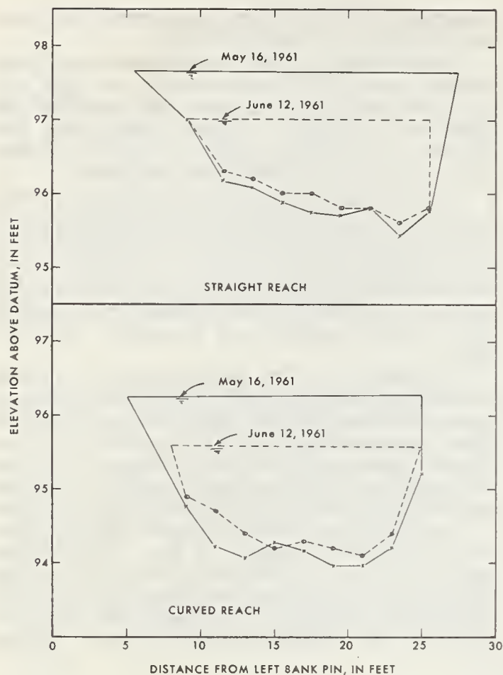
FIGURE 7.—Typical cross sections, Rio Grande del Ranchos, 1961.
