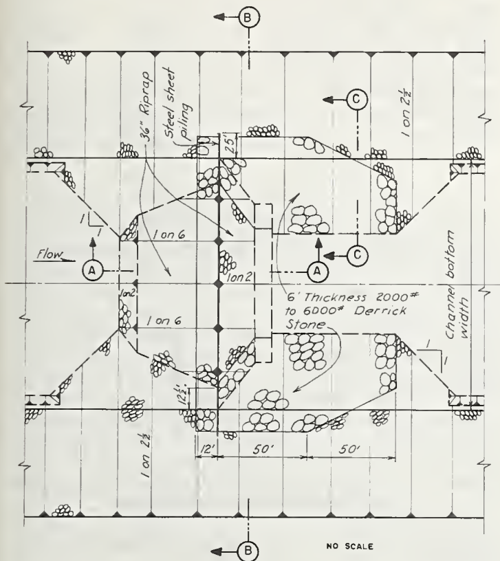
FIGURE 10. — Plan view of the final sill design.
