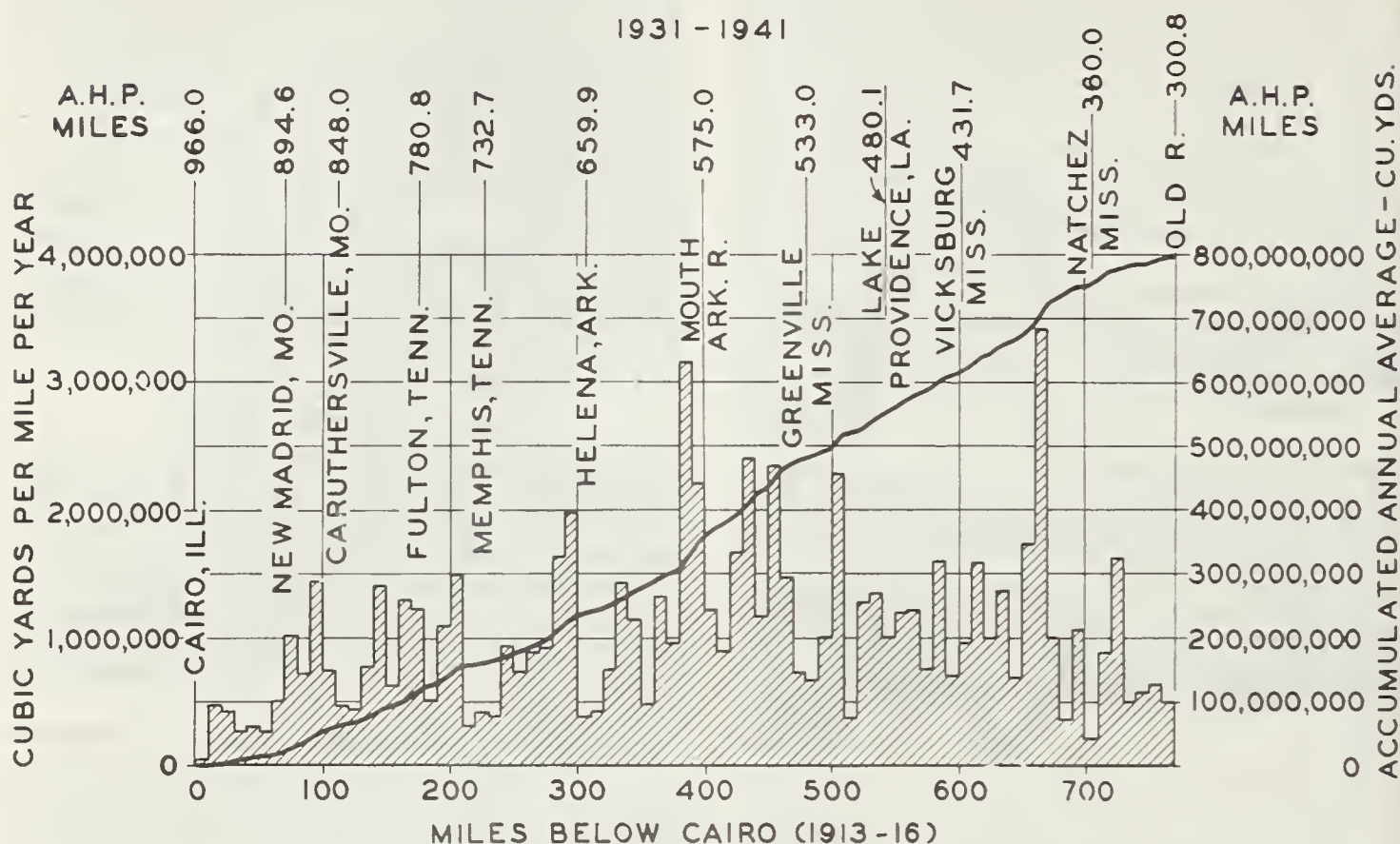
FIGURE 3. — Caving bank history.
