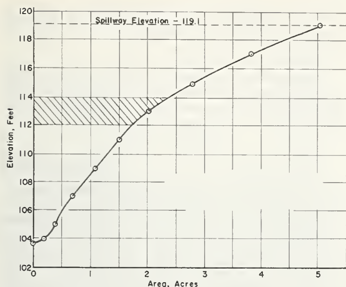
FIGURE 6. — Matt Hafner Reservoir stage-area curve.
