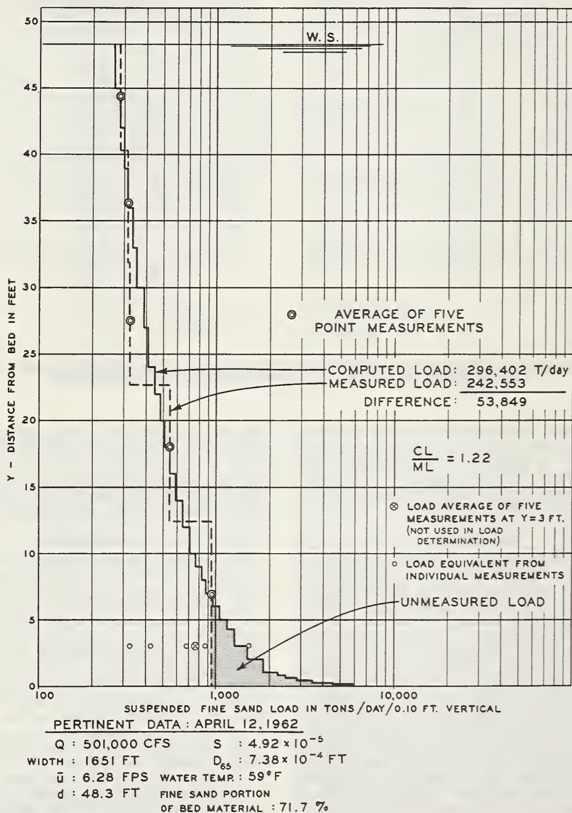
FIGURE 4. — Computed, measured, and unmeasured suspended fine sand load at Simmesport, Atchafalaya River, April 12, 1962.
