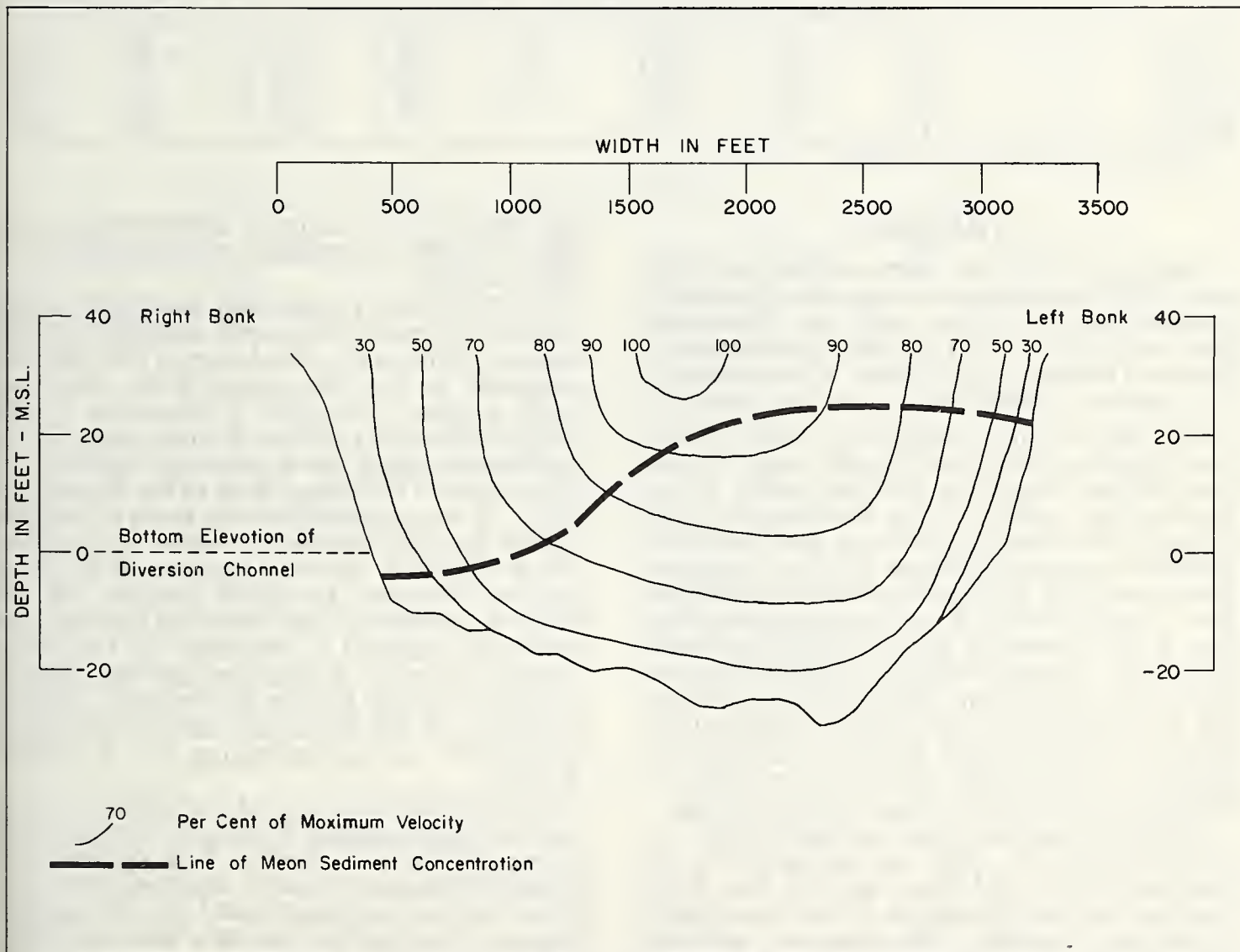
FIGURE 3. — Cross section of Mississippi River above diversion channel.
