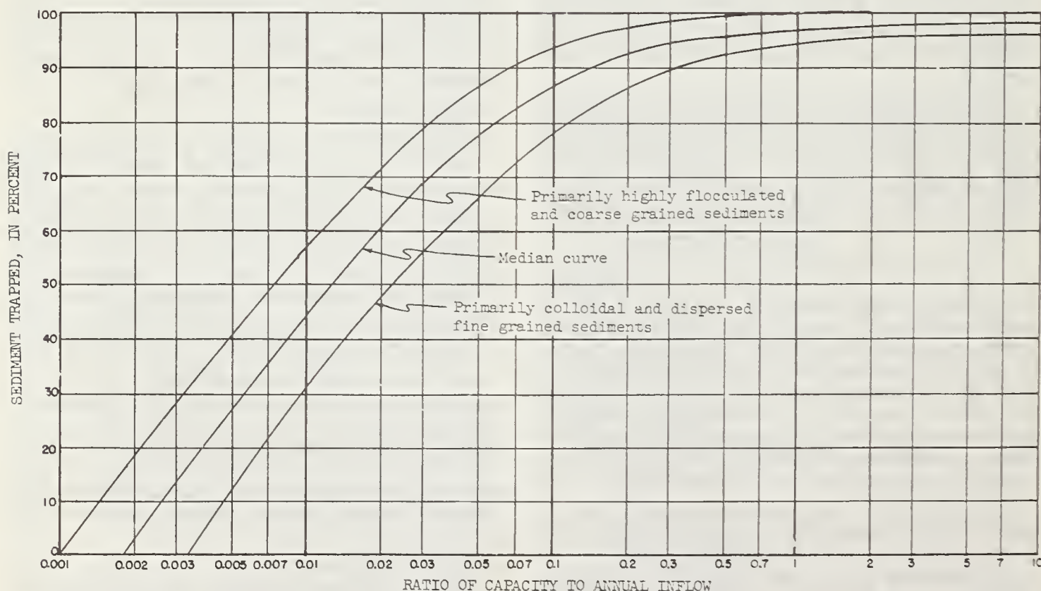
FIGURE 1. — Trap efficiency of reservoirs. (Adapted from Brune.)
