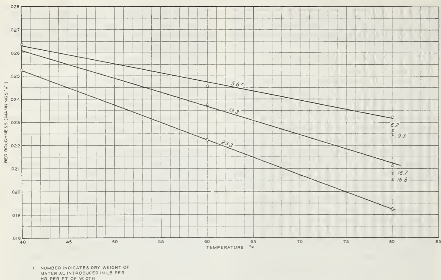
FIGURE 2. — Bed roughness-temperature curves; fine sand bed material.
