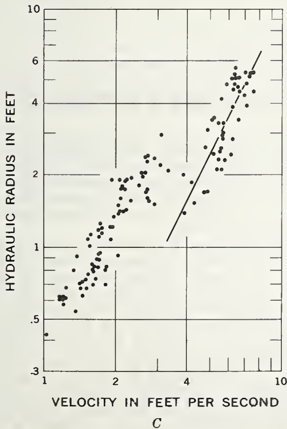
FIGURE 1.—Relation of velocity to hydraulic radius: A, Middle Loup River at St. Paul, Nebr.; B, Huerfano River near Undercliffe, Colo.; C, Pigeon Roost Creek near Byhalia, Miss.; and D, Rio Grande near Bernalillo, N. Mex.
