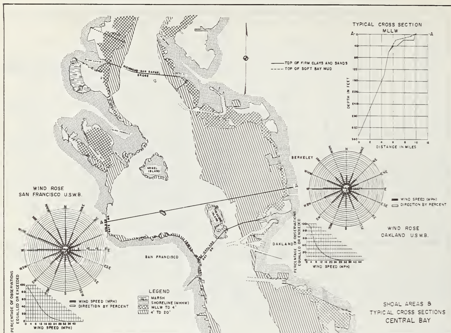
FIGURE 16. — Shoal areas, wind roses, and typical cross section of Central San Francisco Bay.
