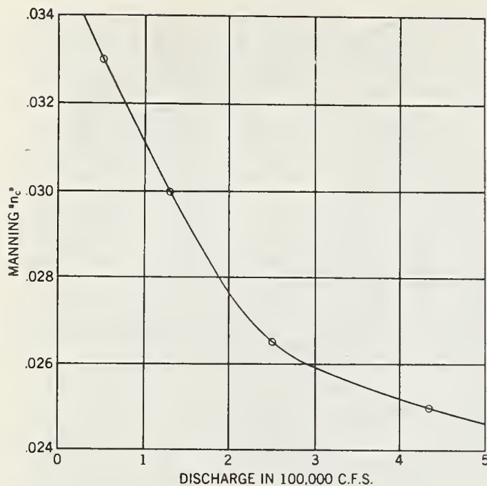
FIGURE 6. — Variation of the main channel Mannings "n" values with total discharge on the Arkansas River in the vicinity of Little Rock.
