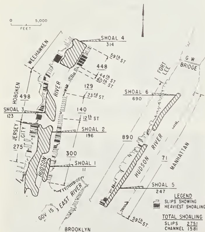
FIGURE 6.—Slip and channel shoaling (thousands of cubic yards), Hudson River.
