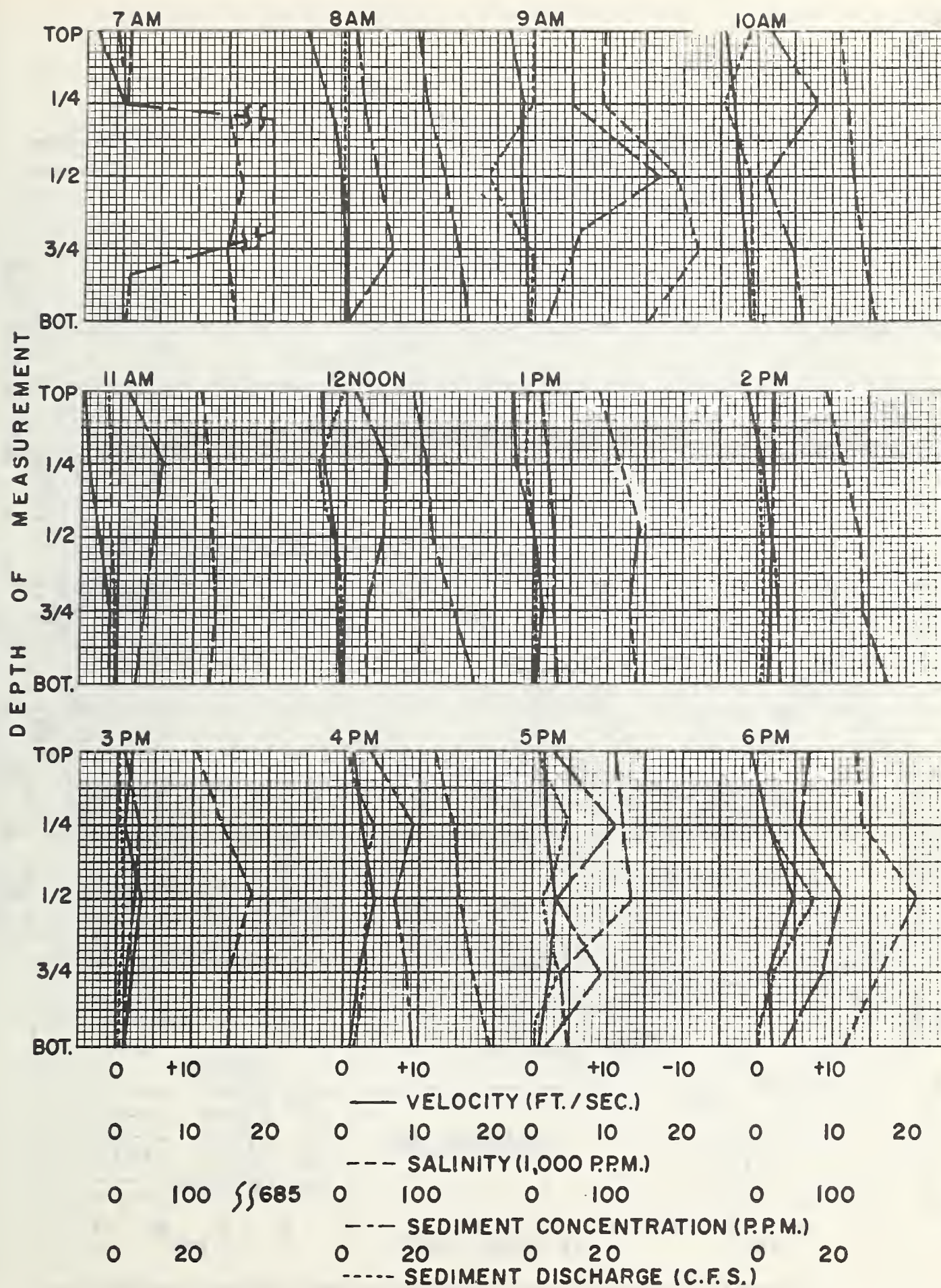
FIGURE 16.—Vertical variation in velocity, salinity, and sediment, lower Hudson River range A, 23 April 1957.
