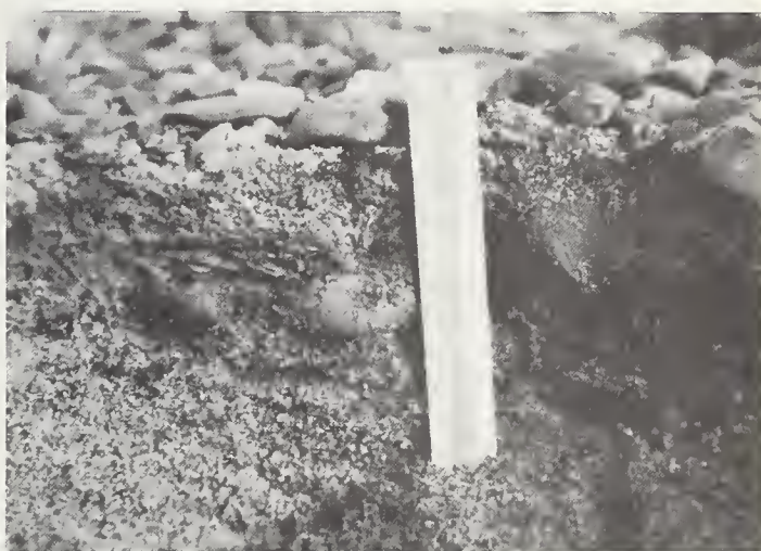
FIGURE 13. — Cross sectional closeup view of streambed armor, showing isolated example of a concentration of coarse gravel in the underlying strata.
