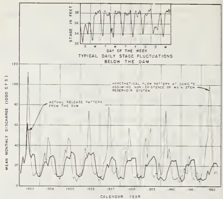
FIGURE 3.—Actual and hypothetical release trends from Fort Randall Dam.
