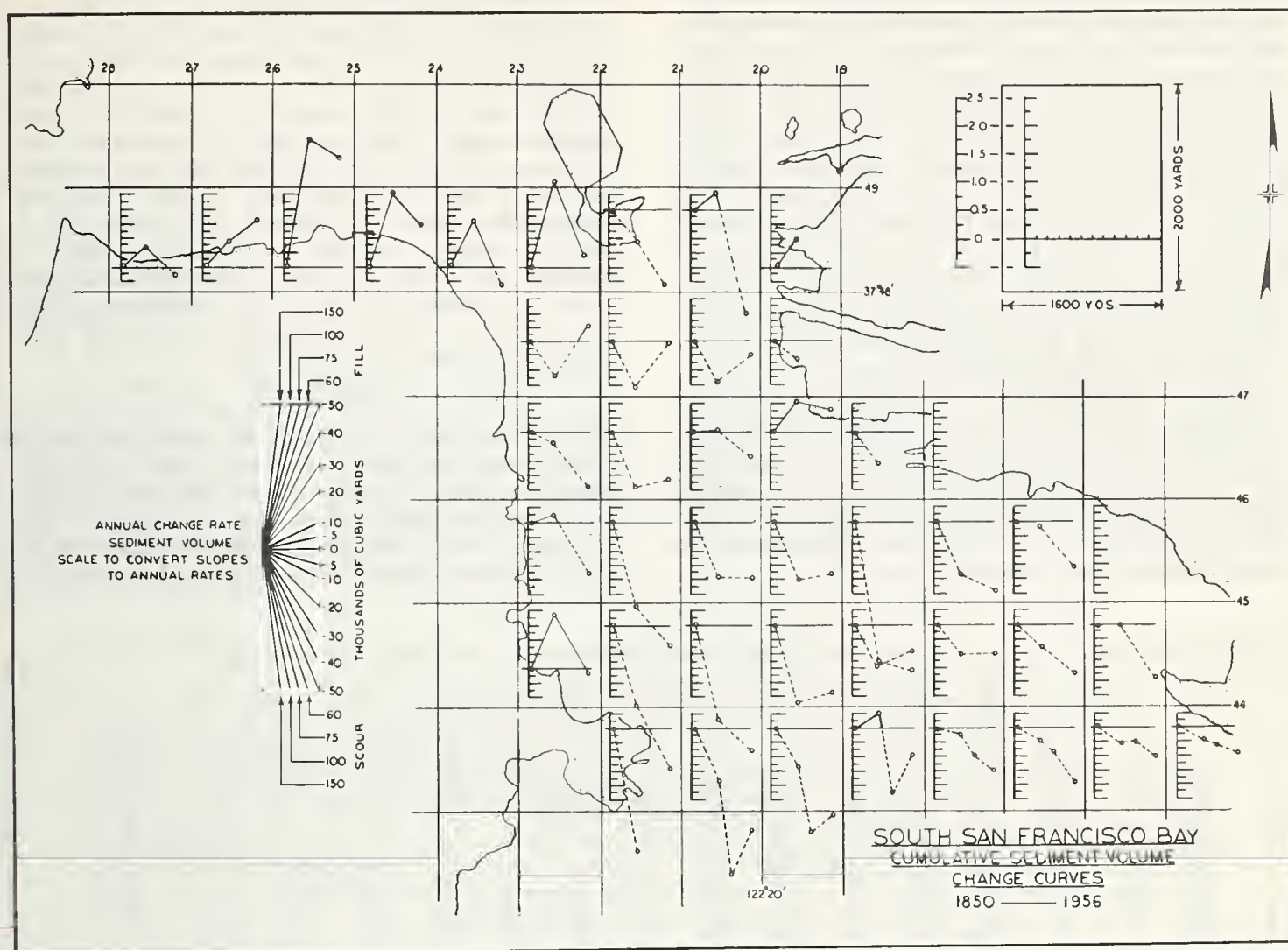
FIGURE 11.— Cumulative sediment volume change curves of South San Francisco Bay, 37^{\circ} 49' to 37^{\circ} 43' N .
