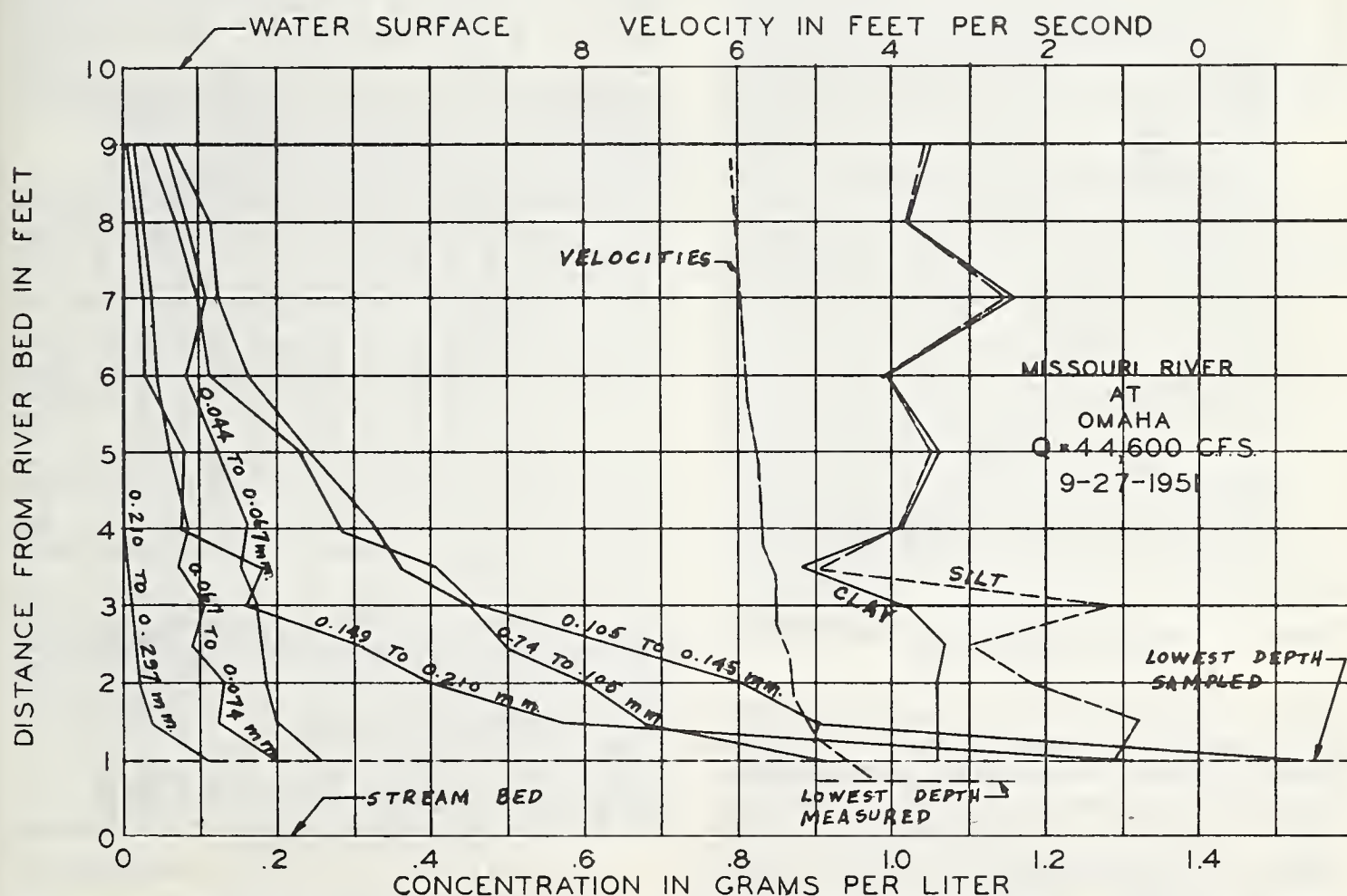
FIGURE 1. — Vertical velocity and concentration distributions in Missouri River.
