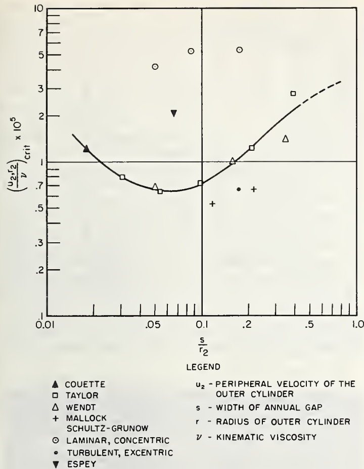
FIGURE 2.—Critical Reynolds number vs. relative annular spacing. (After Schlichting (5).)
