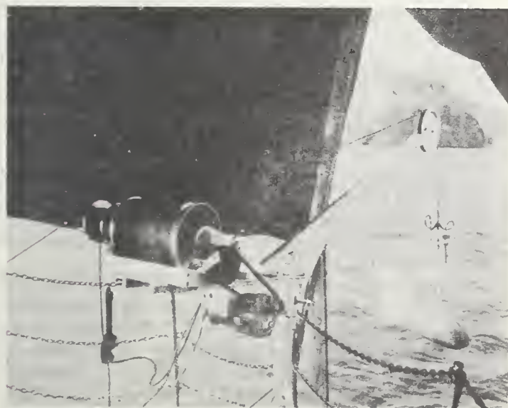
FIGURE 12. — Salinity — temperature assembly.
