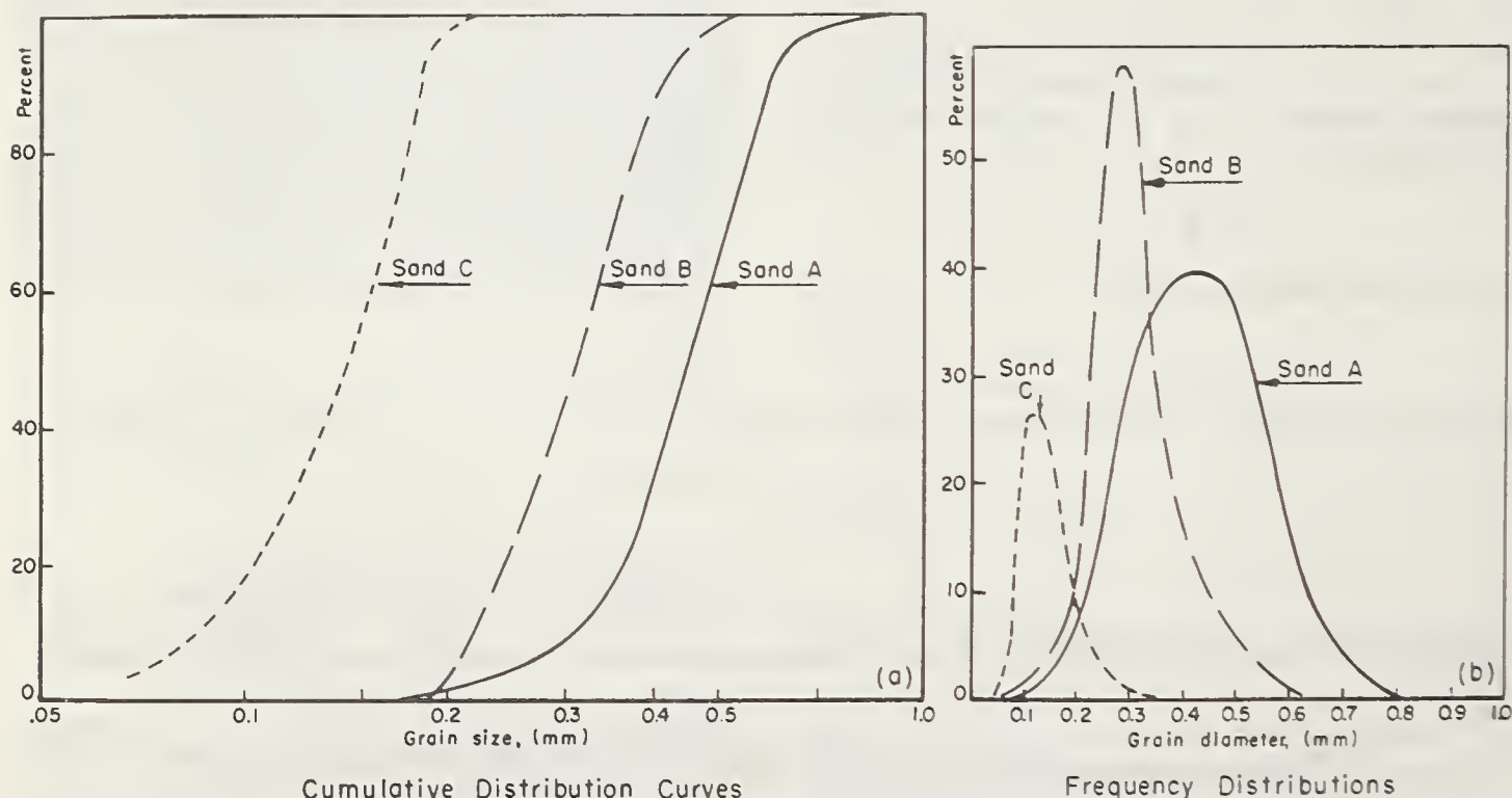
FIGURE 5. — Mechanical composition of sands tested.
