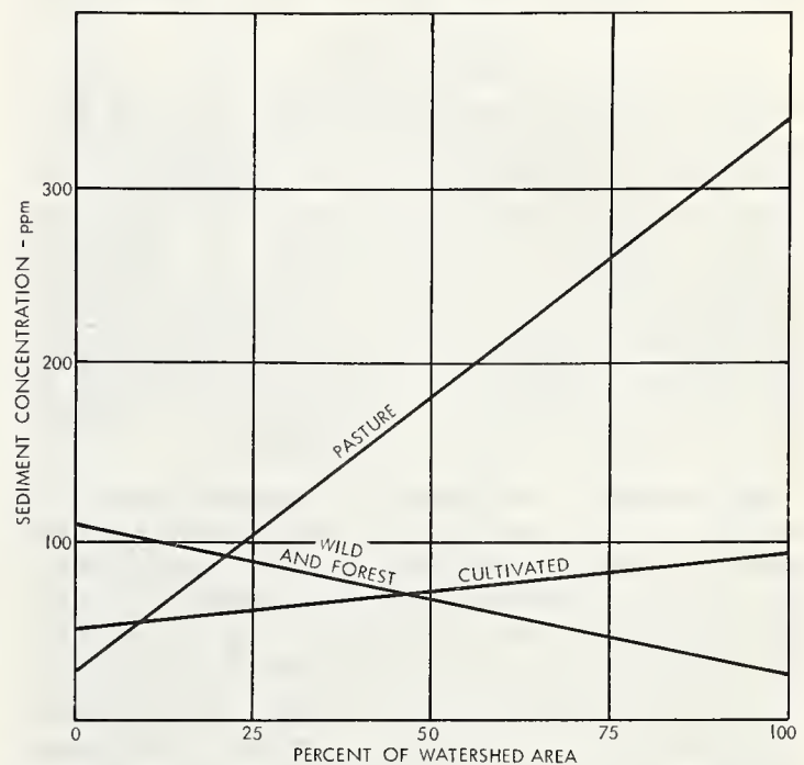
FIGURE 5.— General relation between land use and sediment concentration in the Tobacco River Watershed.
