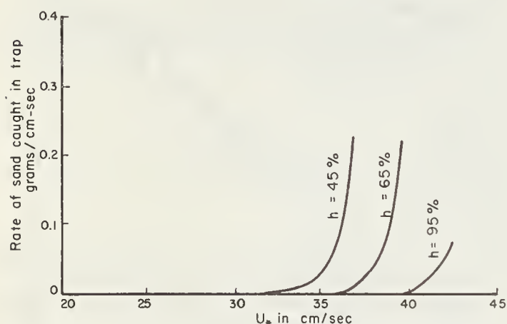
FIGURE 14.—Variation of rate of sand transport with air humidity.
