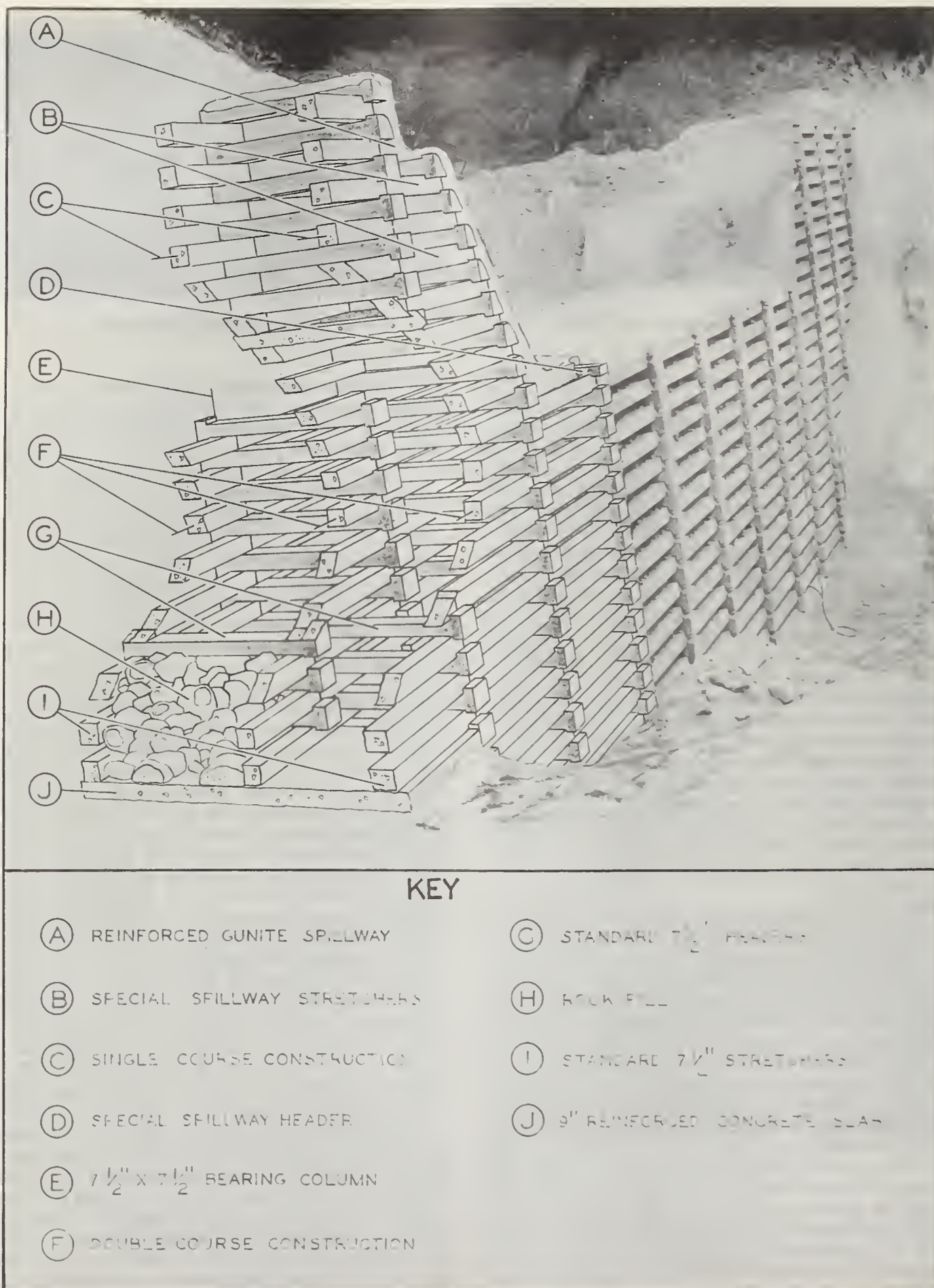
FIGURE 4.— Combination photograph and cutaway drawing of a concrete crib structure designed for the Cooks Canyon project.
