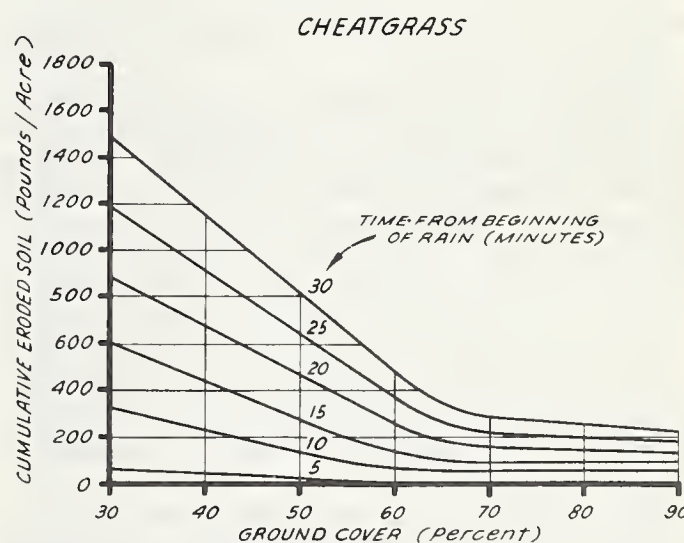
FIGURE 3.—Cumulative overland flow and soil erosion from wheatgrass and cheatgrass sites on soil derived from granite at different ground cover densities by successive 5-minute periods. Based on a simulated rainfall of 1.87 inches for 30 minutes (12).
