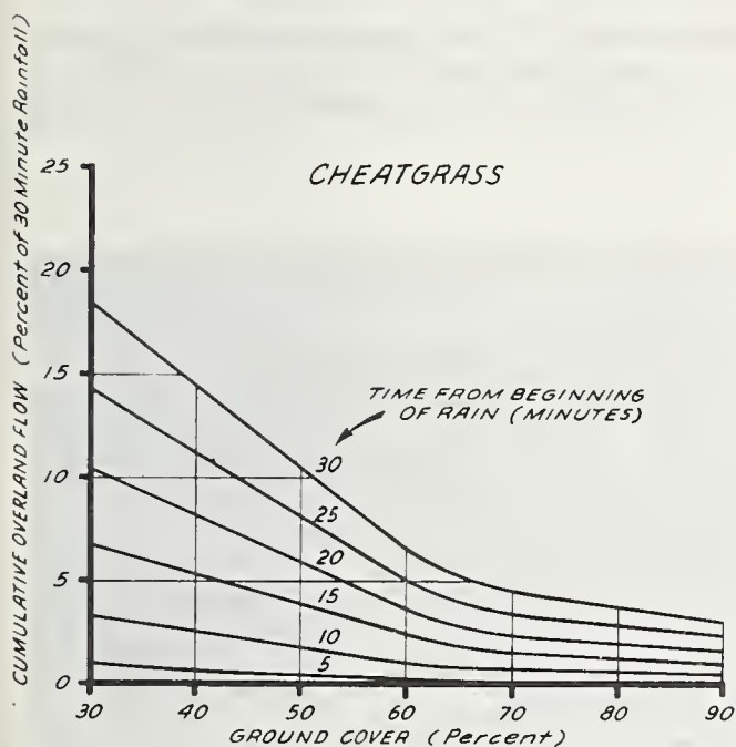
FIGURE 3.—Cumulative overland flow and soil erosion from wheatgrass and cheatgrass sites on soil derived from granite at different ground cover densities by successive 5-minute periods. Based on a simulated rainfall of 1.87 inches for 30 minutes (12).
