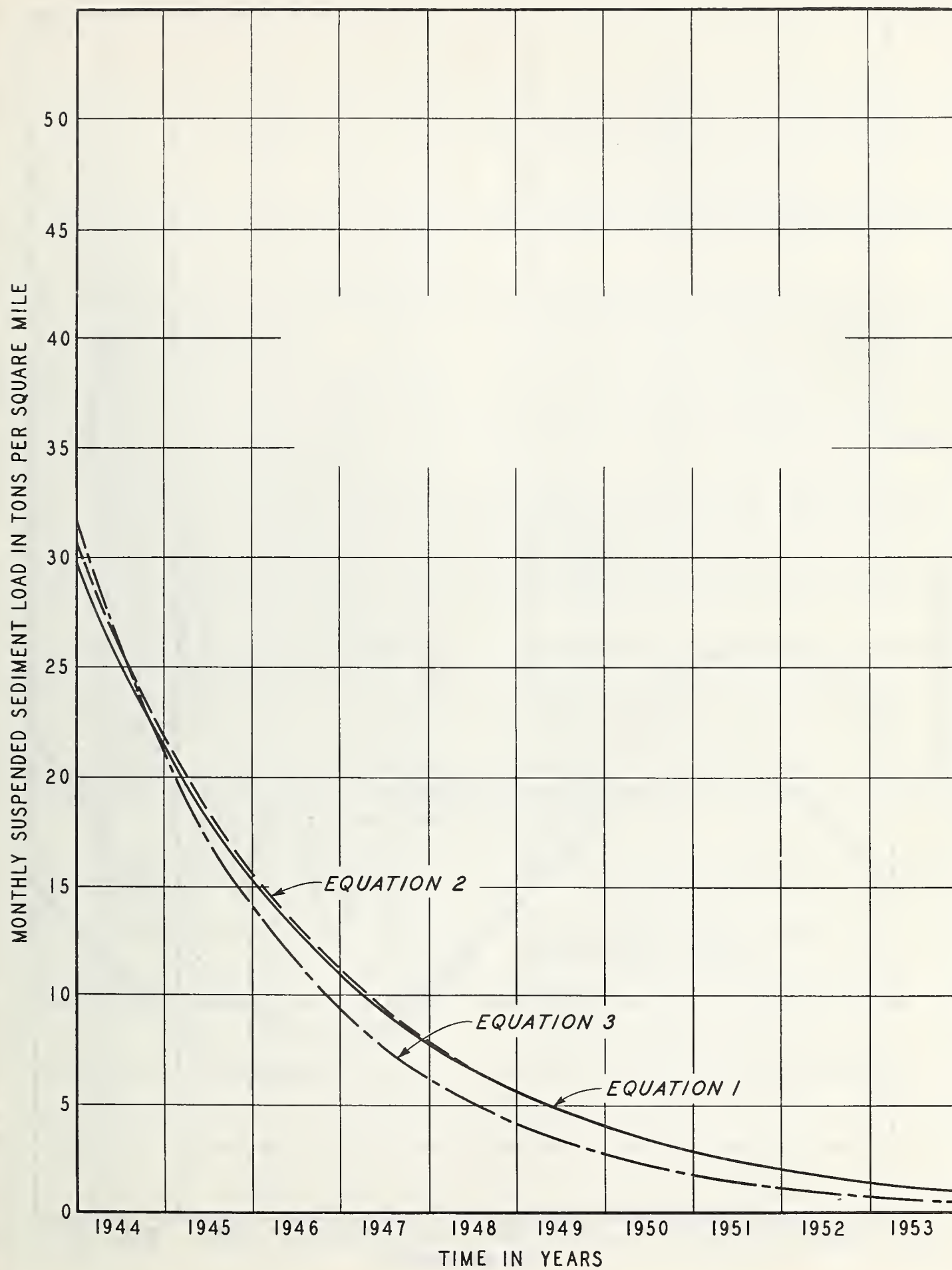
FIGURE 2. — Chestuee Creek Watershed: Suspended sediment prediction by time regression function.
