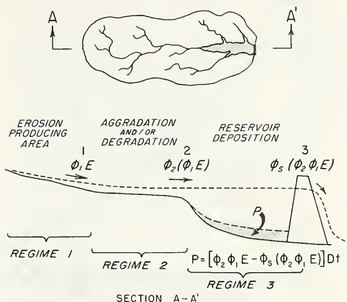
FIGURE 2.—Three regimes associated with soil erosion and deposition.
