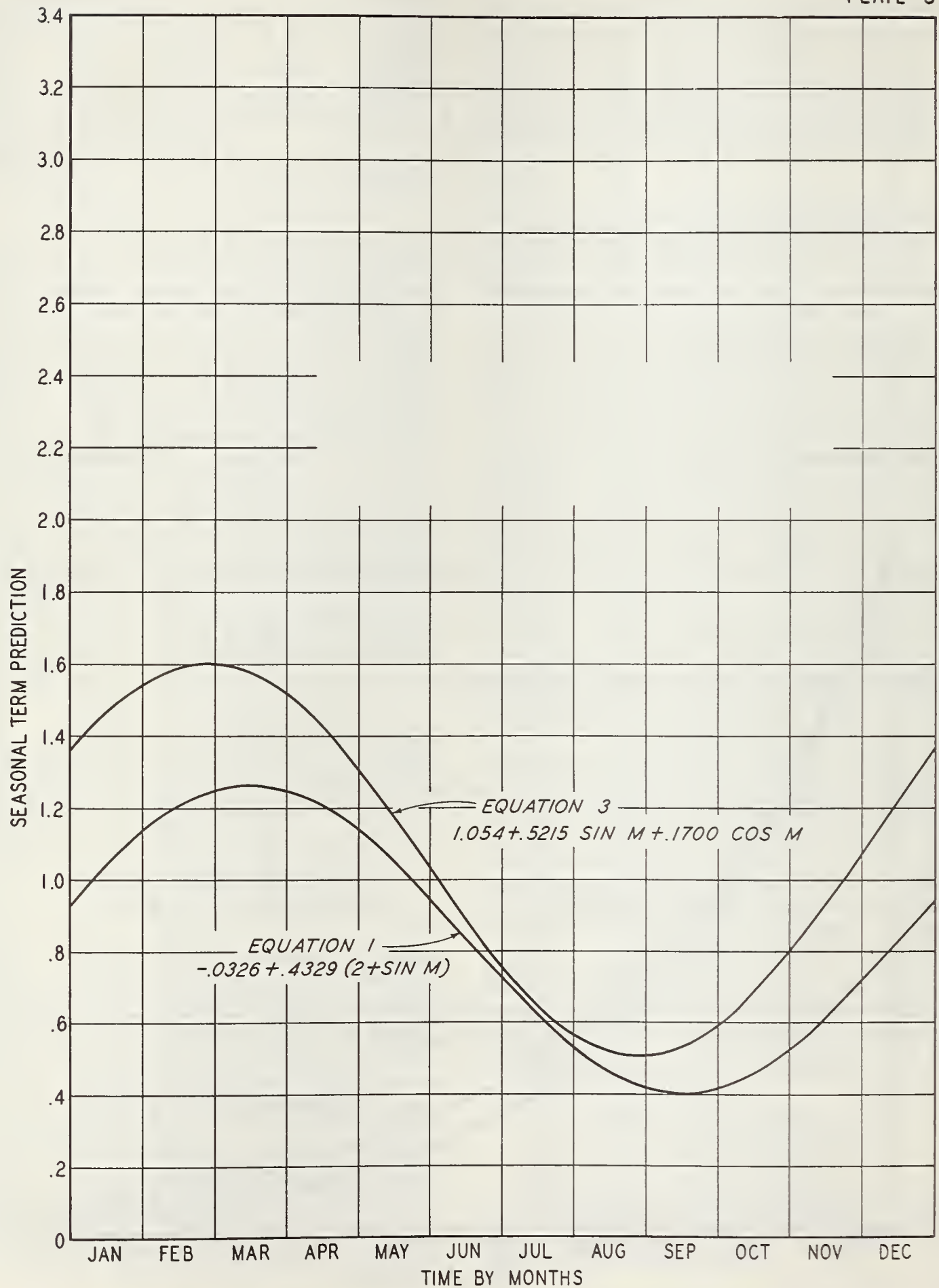
FIGURE 3. — Chestuee Creek Watershed: Comparison of season-regression terms (equation 1 vs. equation 3).
