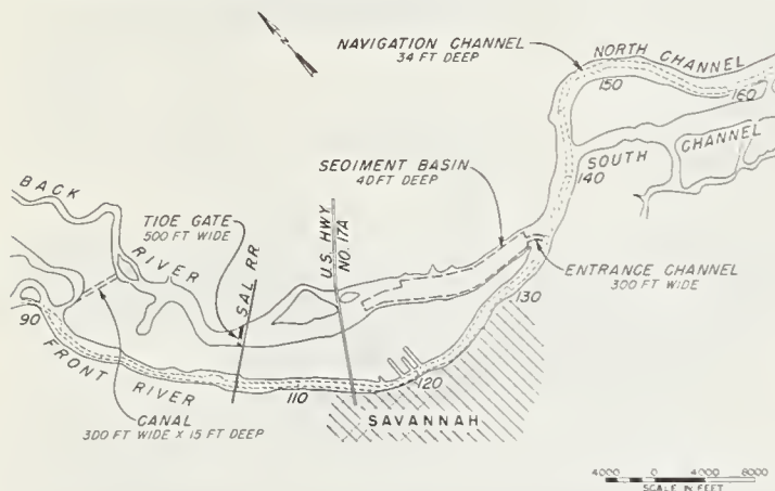
FIGURE 5.—Sediment basin with tide gate in upstream location.
