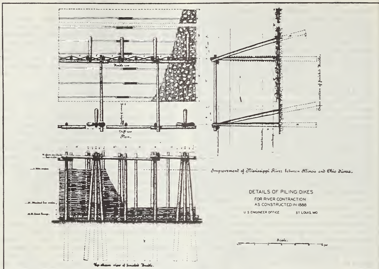
FIGURE 4. — Early type of permeable dike.
