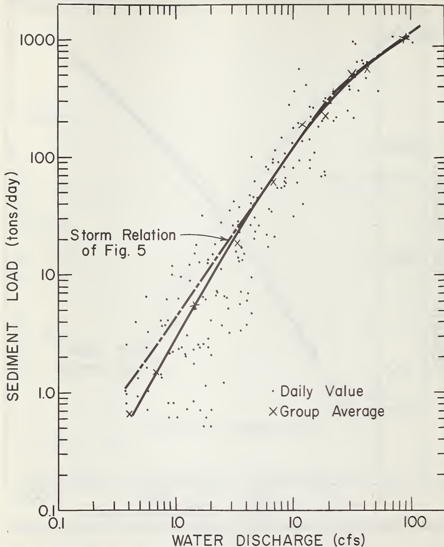
FIGURE 4.— Direct runoff versus sediment discharge, by day, Pigeon Roost Creek Watershed 5, January 1957-December 1960.
