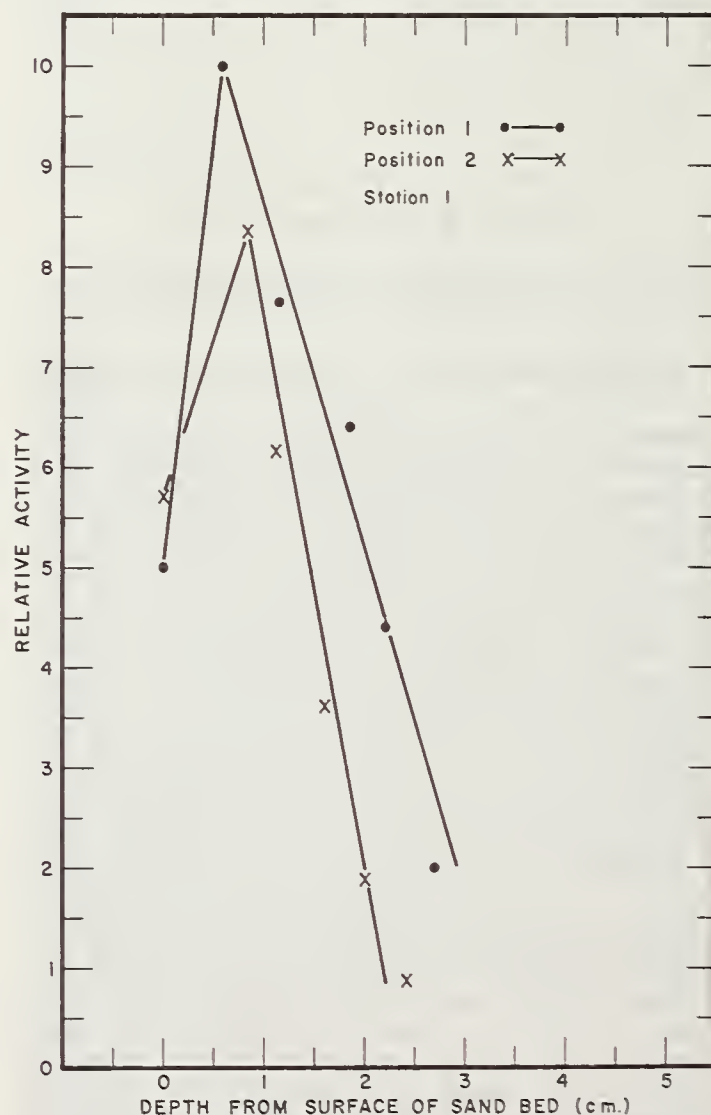
FIGURE 6.—Vertical distribution of scandium-46 labeled sand in the channel bed after 125 hours of flume operation (station 1).
