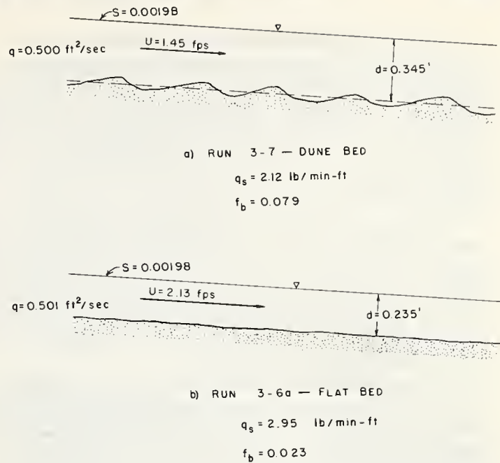
FIGURE 4.—Schematic diagram of two different equilibrium flows with same slope and discharge.
