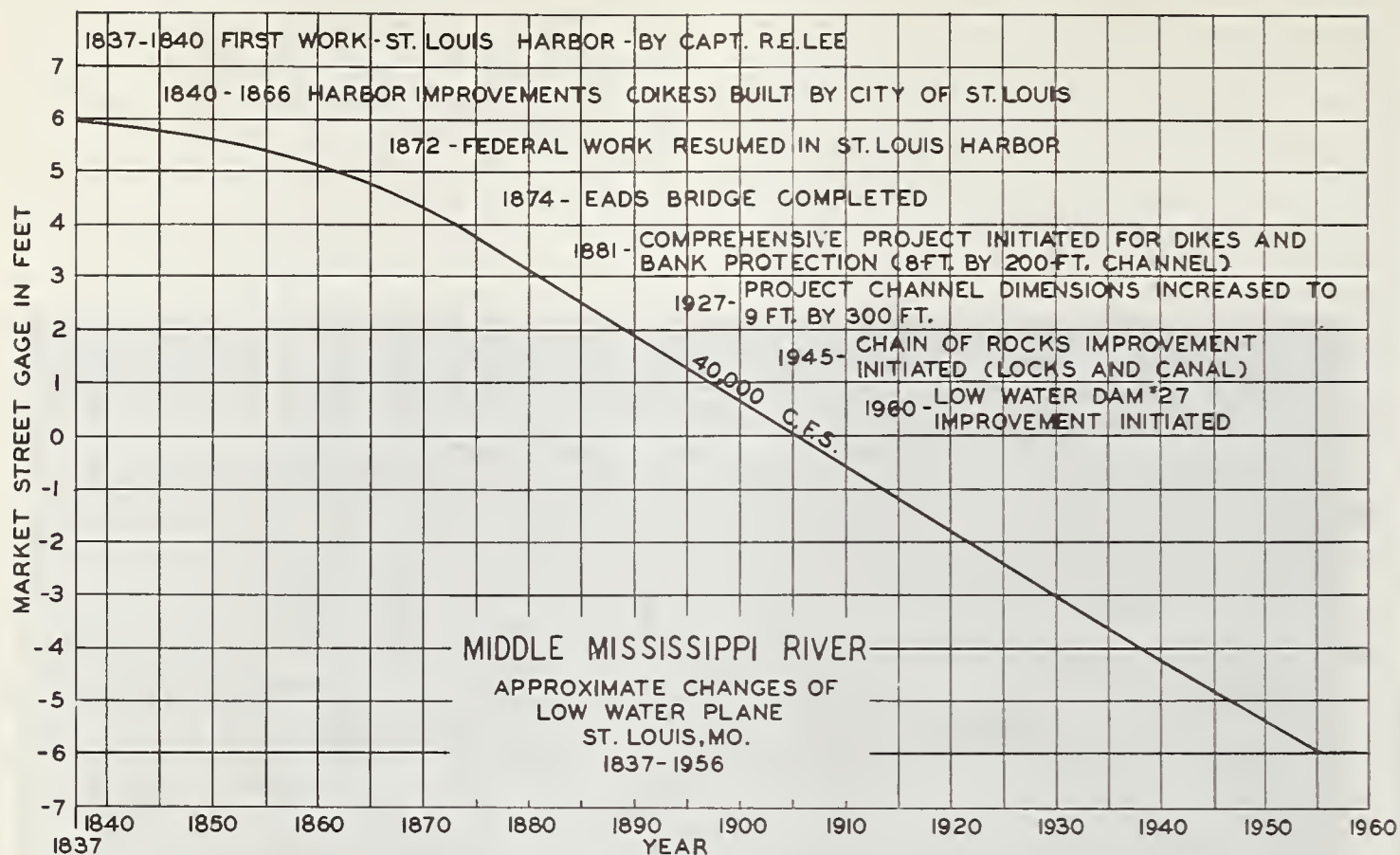
FIGURE 4. — Stage-time graph for 40,000 c.f.s., Mississippi River at St. Louis, 1837-1955.
