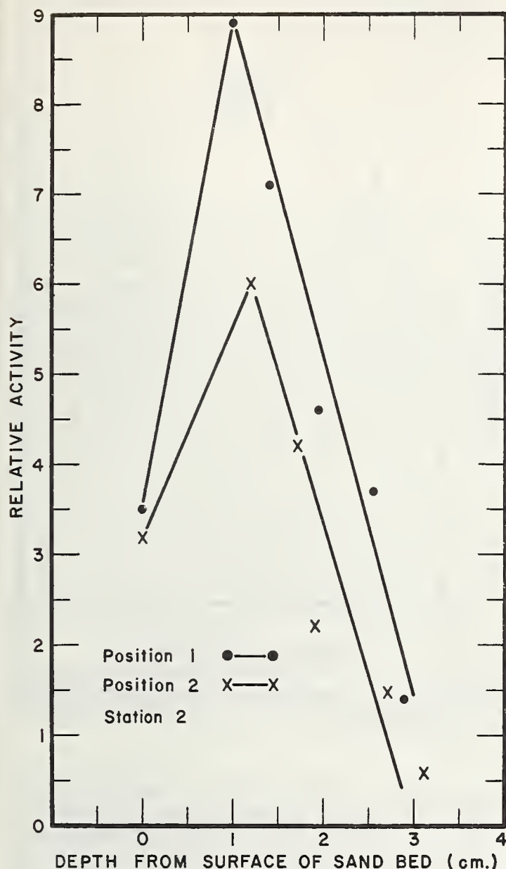
FIGURE 7.—Vertical distribution of scandium-46 labeled sand after 125 hours of flume operation (station 2).
