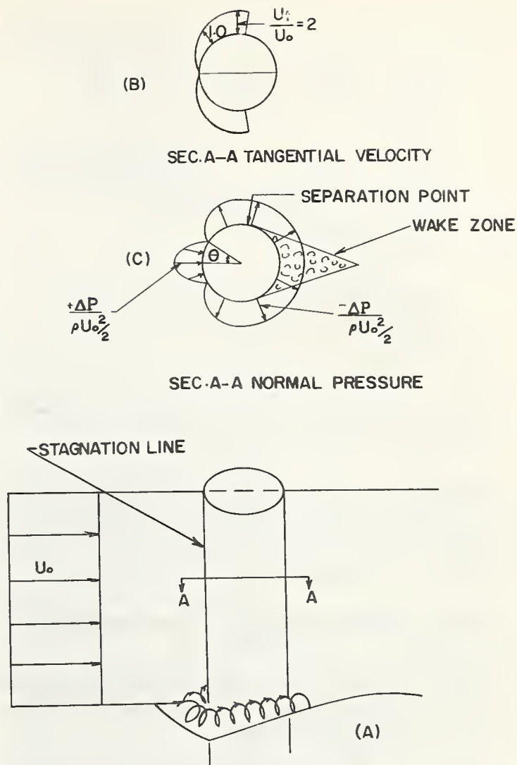
FIGURE 1.—Cylindrical pier with uniform approach velocity.
