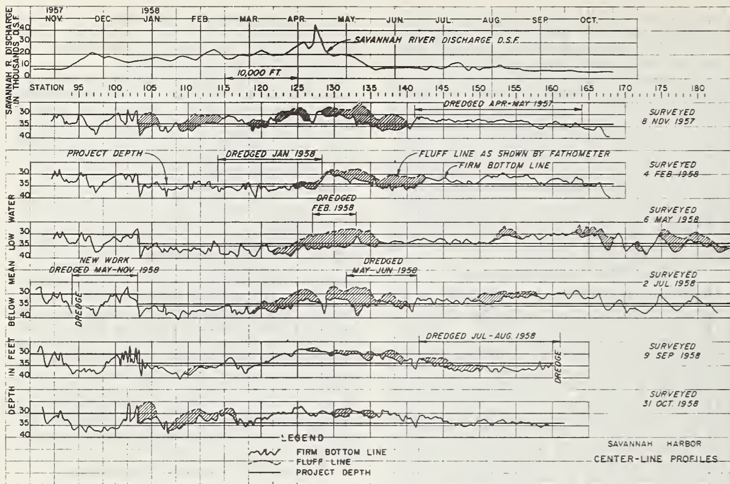
FIGURE 7. — Effect of Savannah River discharges on shoaling.
