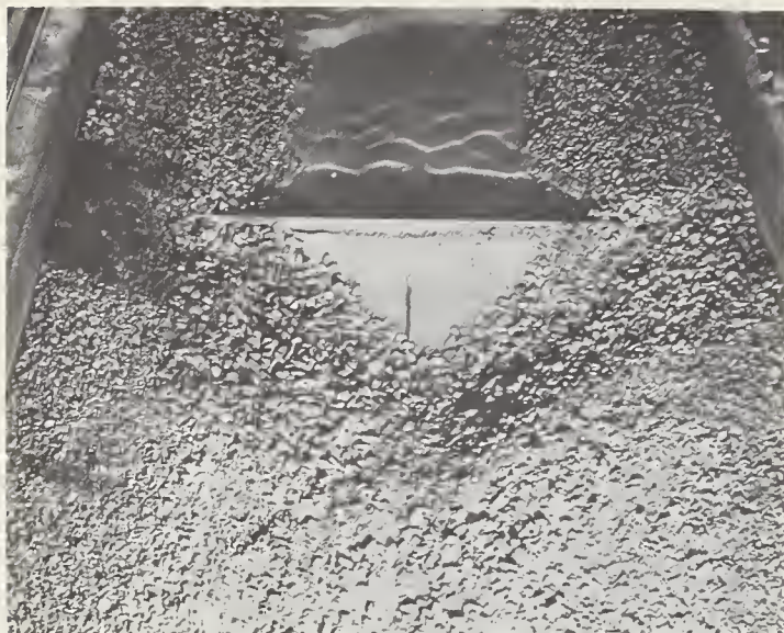
FIGURE 9.— Three-dimensional model sill; flow from top to bottom.
