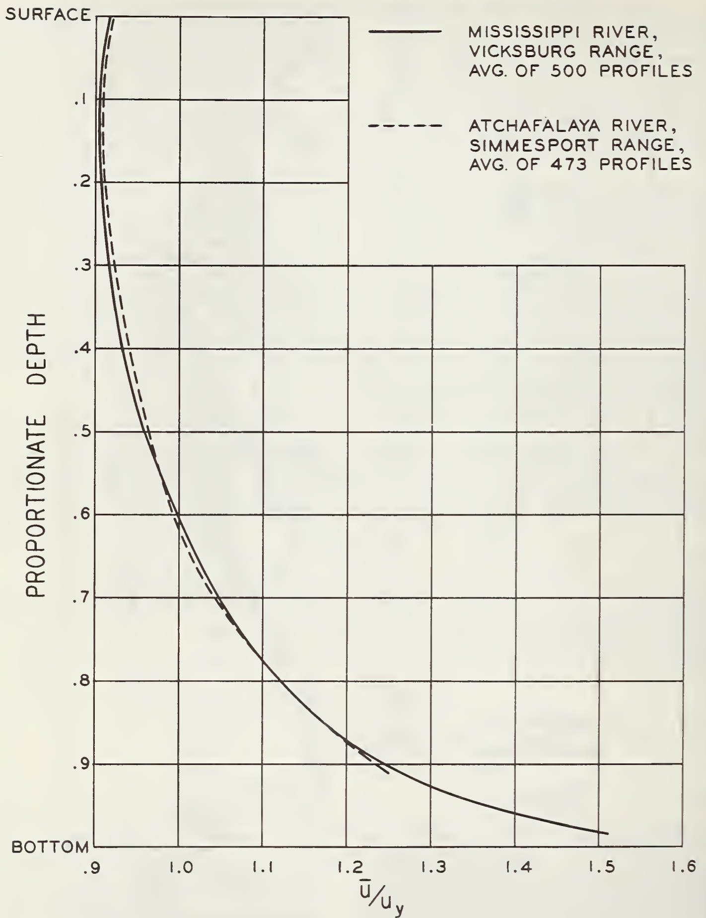
FIGURE 2. — Velocity profiles at Simmesport and Vicksburg ranges.
