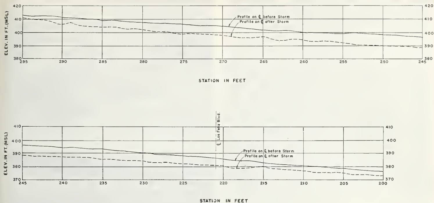
FIGURE 11. — Los Angeles River streambed profile before and after flood of March 1938.
