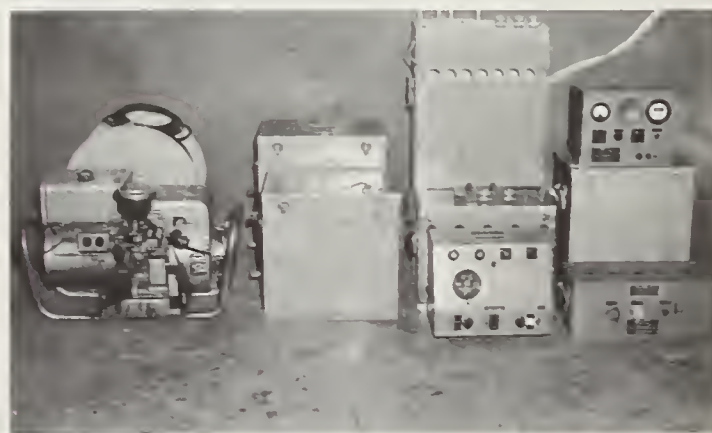
FIGURE 1.— Equipment comprising the three Raydist groups: Left to right are (1) generator and cable, (2) shore station units, (3) master station group, and (4) the test set, mobile transmitter and master power supply.
