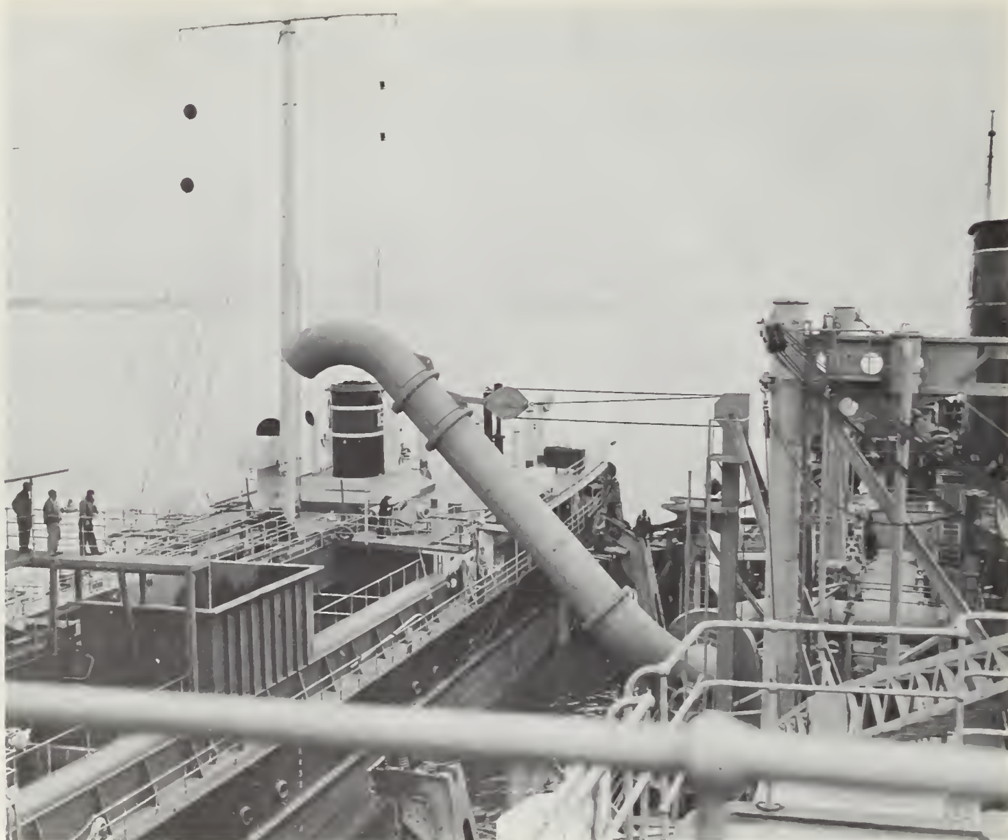
FIGURE 9. — Hopper dredge discharge being set into receiving hopper of sump rehandler New Orleans .
