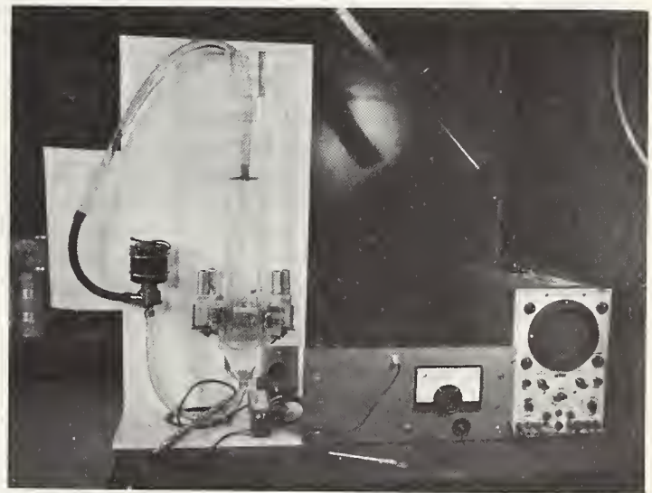
FIGURE 9.—Ultrasonic equipment to measure sediment.
