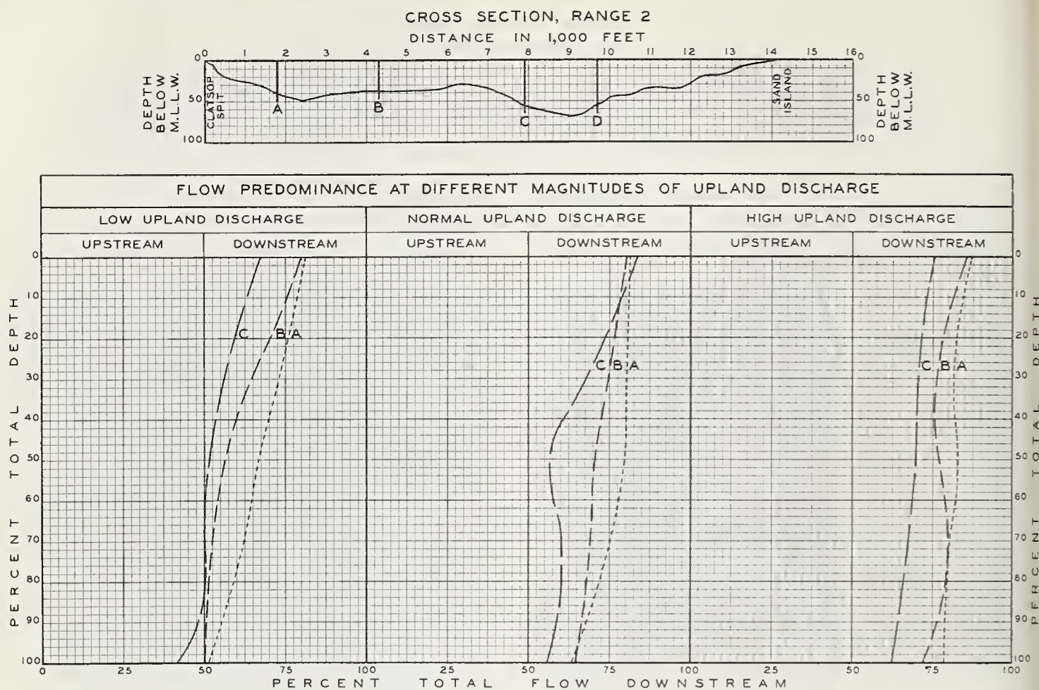
FIGURE 16. — Flow predominance, range 2.
