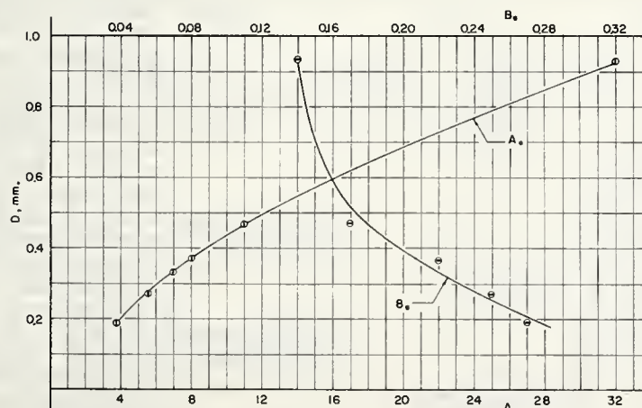
FIGURE 11.—Measured sediment discharge compared to sediment discharge computed by Einstein's function.
