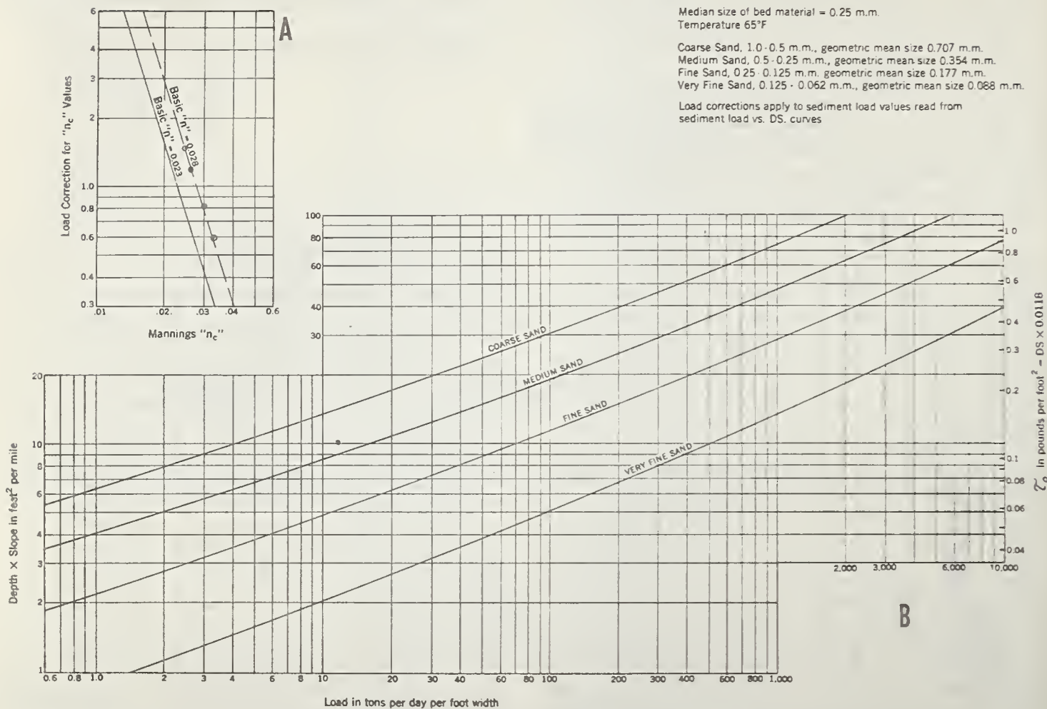
FIGURE 4.— A, Load correction factors for variations in Mannings "n" (main river channel); B, relation between bed tractive force, \tau_o , or product of depth and slope, DS , and bed-material sediment load per foot width.
