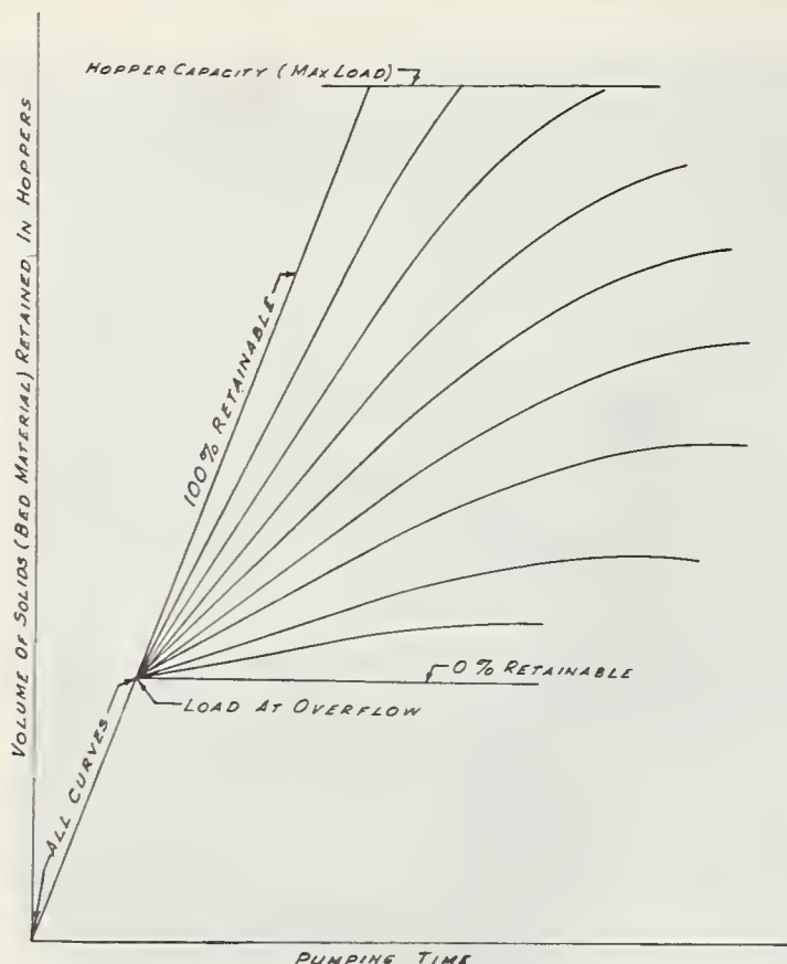
FIGURE 4. — Retention in hoppers of varying grain-sized materials.
