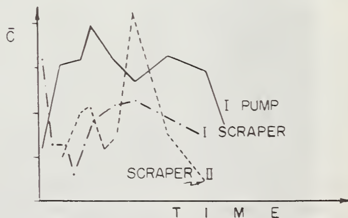
FIGURE 5. — Results of a test of concentration of tracer material versus time.
