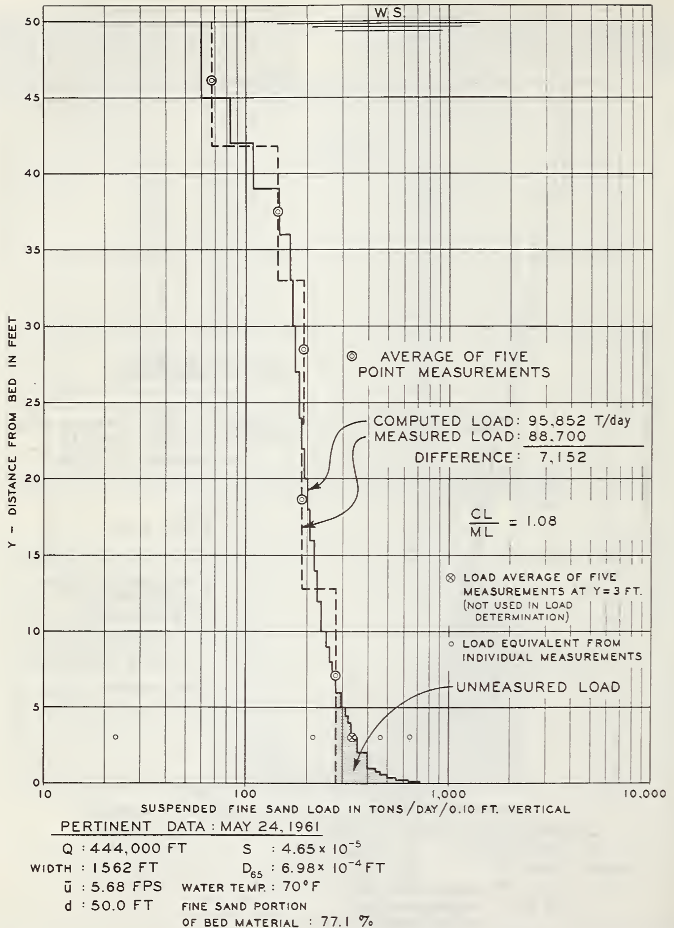
FIGURE 6.—Computed, measured, and unmeasured suspended fine sand load at Simmesport, Atchafalaya River, May 24, 1961.
