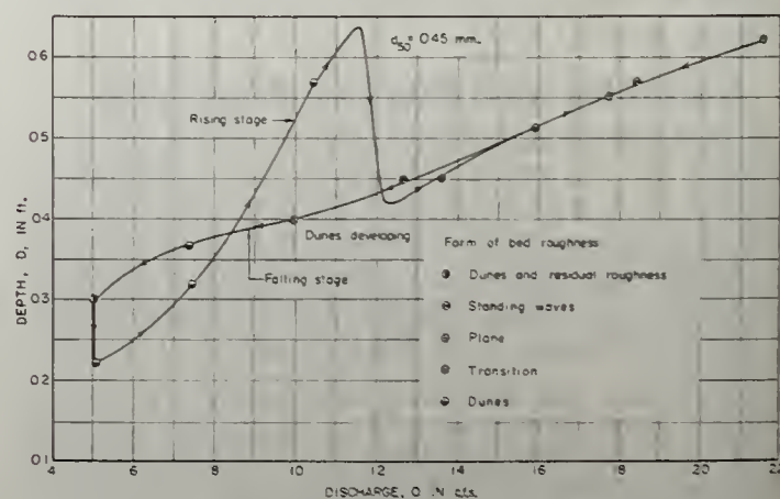
FIGURE 4.—Typical depth-discharge relation involving lower and upper regime flow.
