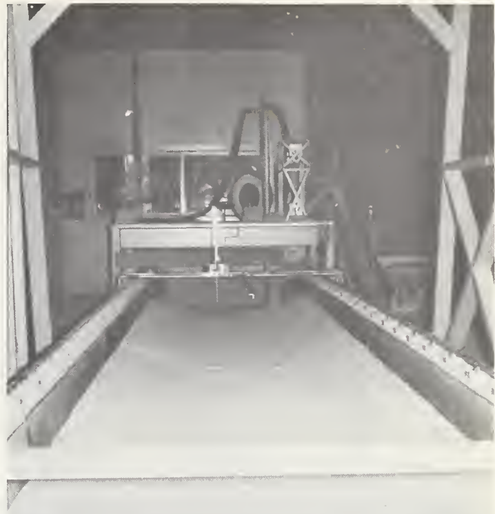
FIGURE 2.—Downstream view of the University of Iowa flume and the sand base for a model channel.
