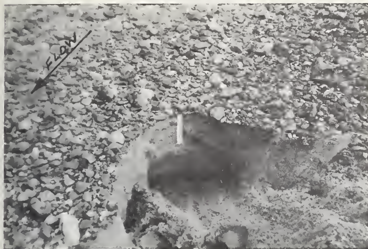
FIGURE 10. — General view of bed surface armor below Fort Randall Dam. Observations were made during extremely low stages in 1962. Reference scale in the examination hole has a 6-inch length.
