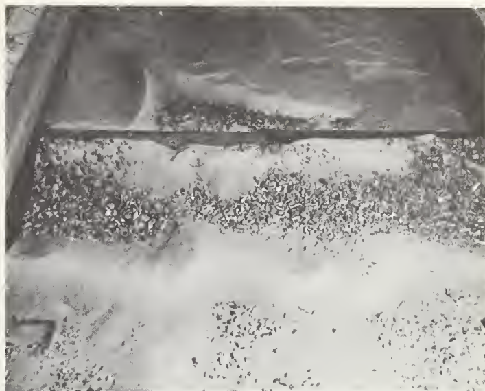
FIGURE 7.— Two-dimensional model sill; flow from top to bottom.
