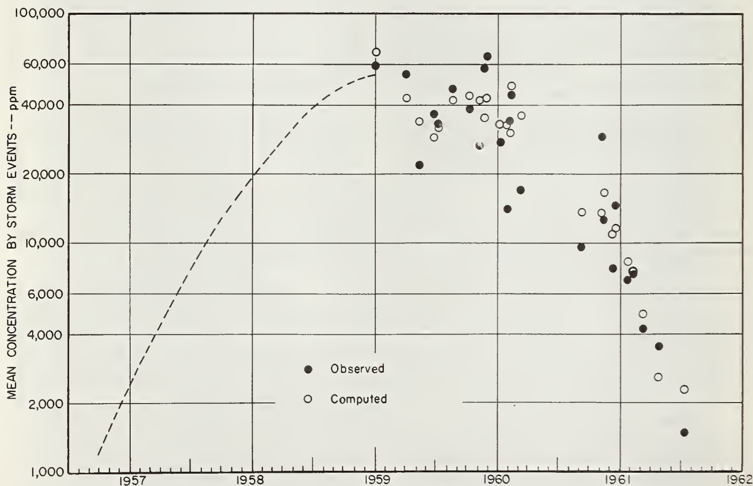
FIGURE 4.—Variation of mean sediment concentration of storm runoff from an area of residential construction at Kensington, Md., 1957-62. The line to July 1959 is estimated on basis of visual observations of construction area and the drainage channels.
