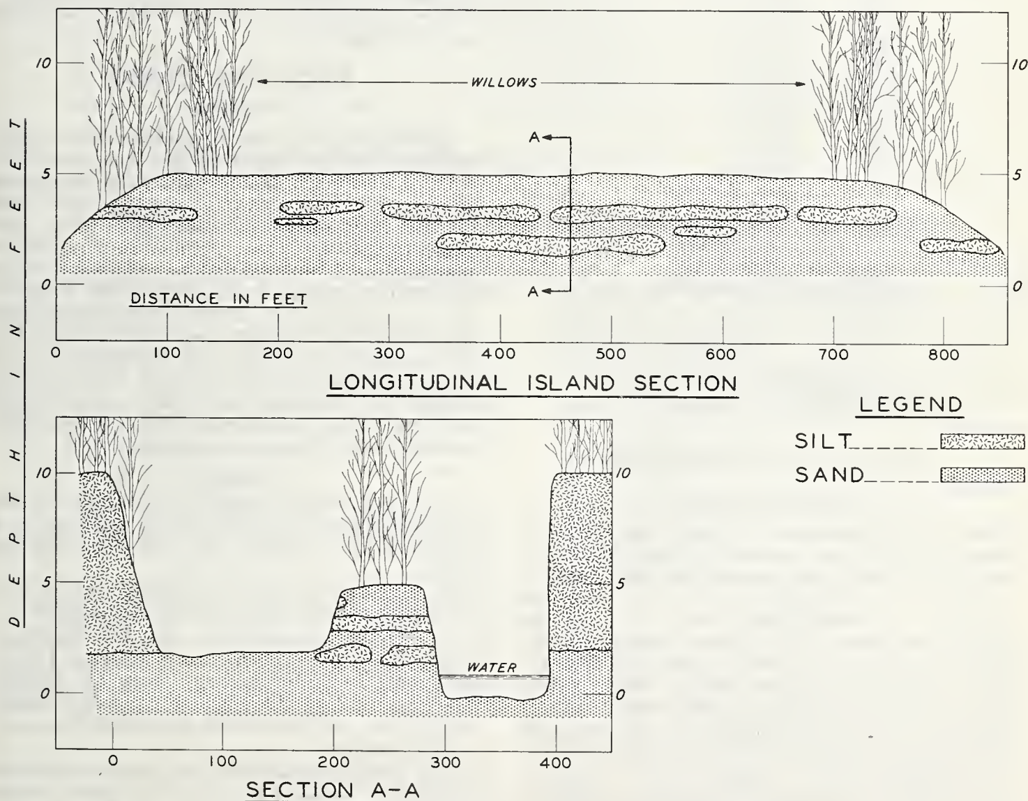
FIGURE 8.—Schematic sections of typical island in Republican River.
