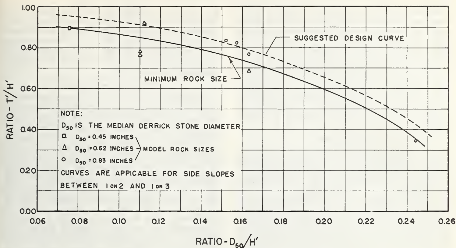
FIGURE 17. Derrick stone sizes required for sill protection.
