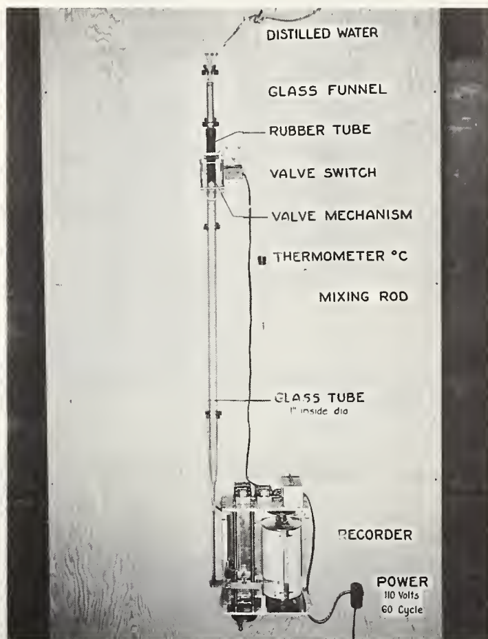
FIGURE 3.—Visual-accumulation-tube sand size analyzer.
