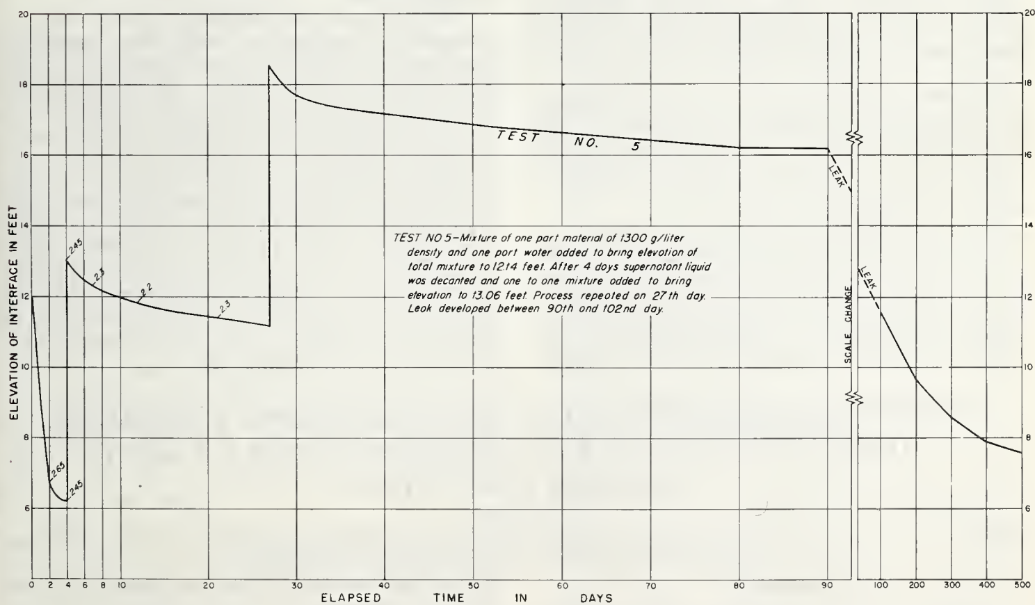
FIGURE 3. — Relationship between elevation of interface with elapsed time: Test 5.
