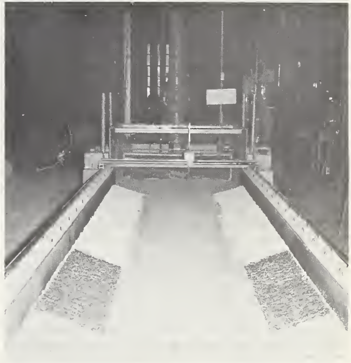
FIGURE 3.—Upstream view of the University of Iowa flume and the rock-lined model channel.
