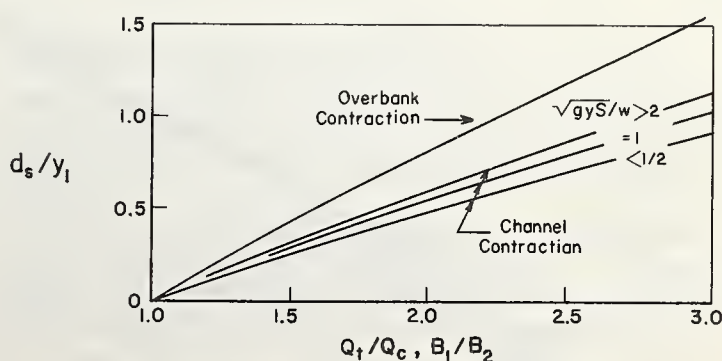
FIGURE 2. — Scour in a long contraction.
