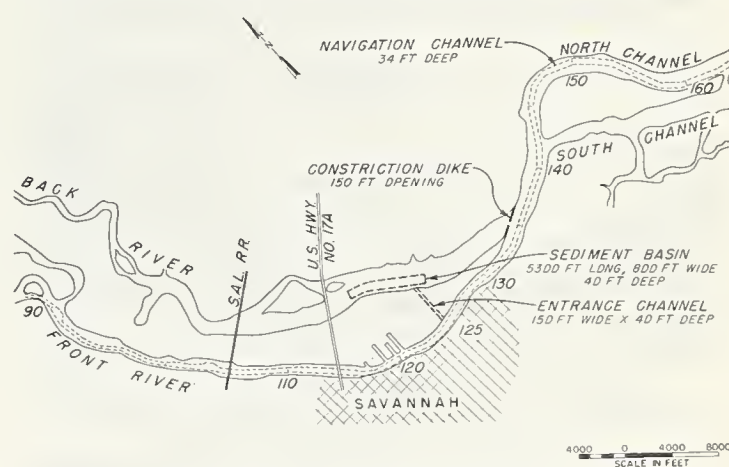
FIGURE 3.—Sediment basin with entrance channel at station 125.
