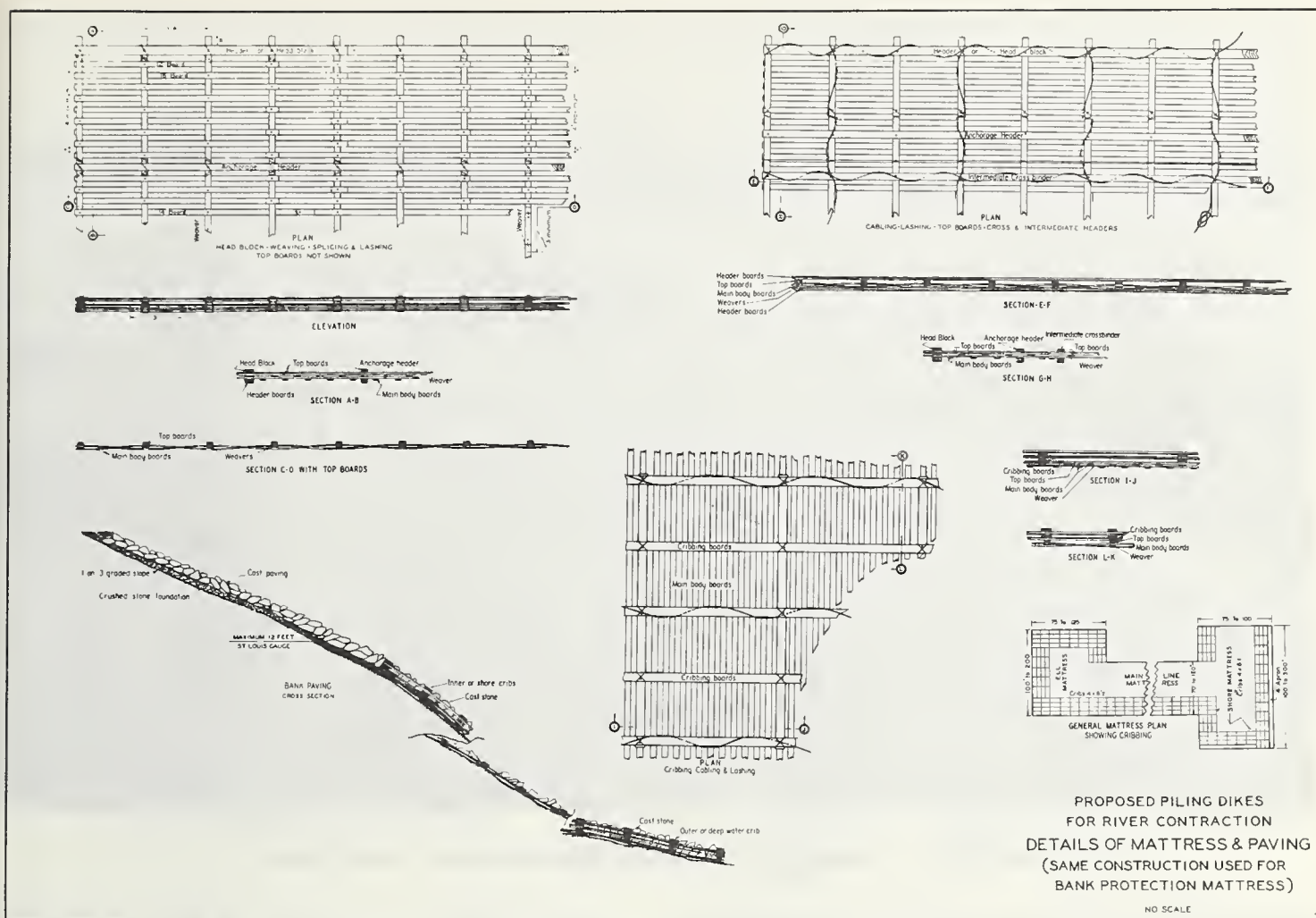
FIGURE 5. — Details of mattress and paving for piling dikes.
