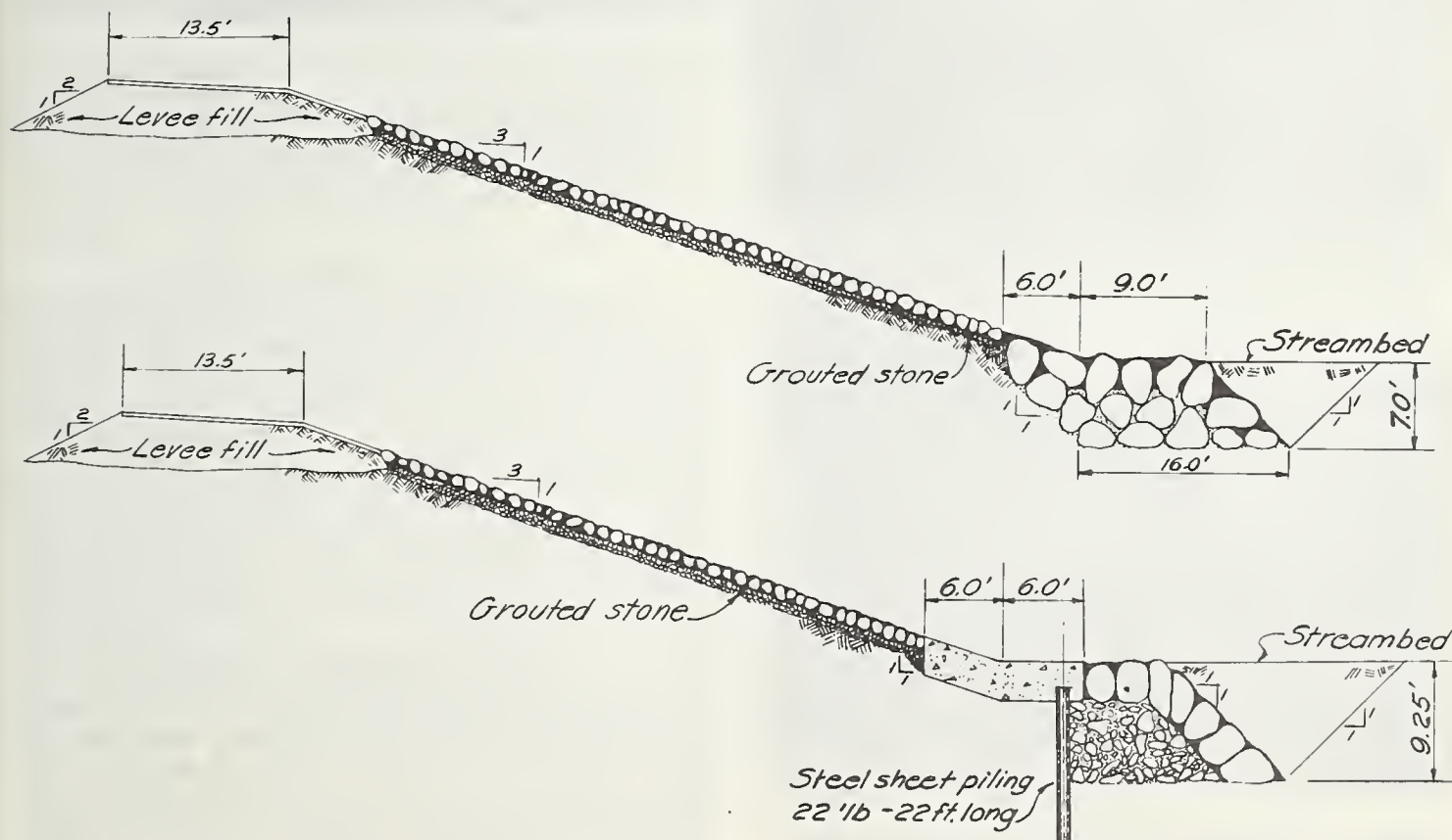
FIGURE 12. — Los Angeles River typical levee revetment; toe design used after 1938 flood.
