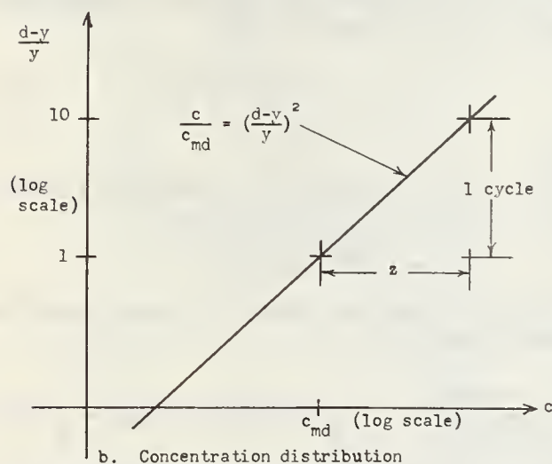
FIGURE 1.—Definition of intercepts and slopes: a , Velocity distribution; b , concentration distribution.
