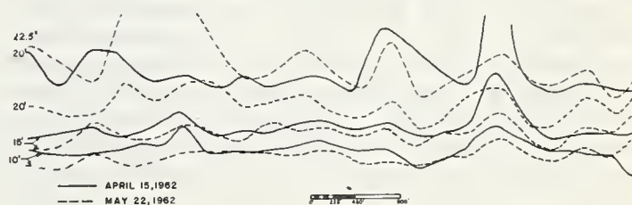
FIGURE 6. — Profiles of migrating sand waves, Fernandina Beach.
