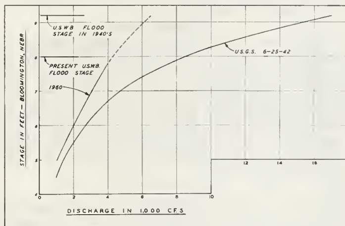
FIGURE 2. — Stage-discharge relations in 1942 and 1960, Republican River near Bloomington.
