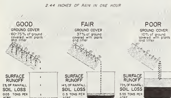
FIGURE 2. — The effect of watershed condition on rain-storm runoff and erosion, Subalpine Range, Ephraim Watershed, Utah.
