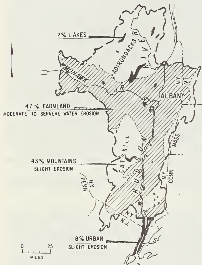
FIGURE 8.—Physiography and erosion of Hudson River watershed.
