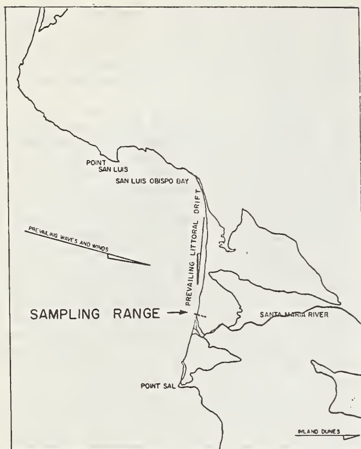
FIGURE 1.—Example of usual shoreline configuration for major dunes on the California coast.
