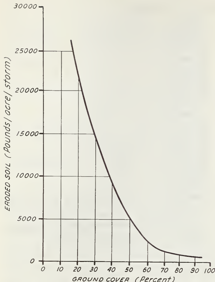
FIGURE 4.—Relation of eroded soil to ground cover density on experimental watershed A, subalpine-herbaceous range, Utah. Based on simulated rainfall of 1.5 inches per hour for 20 minutes (10).
