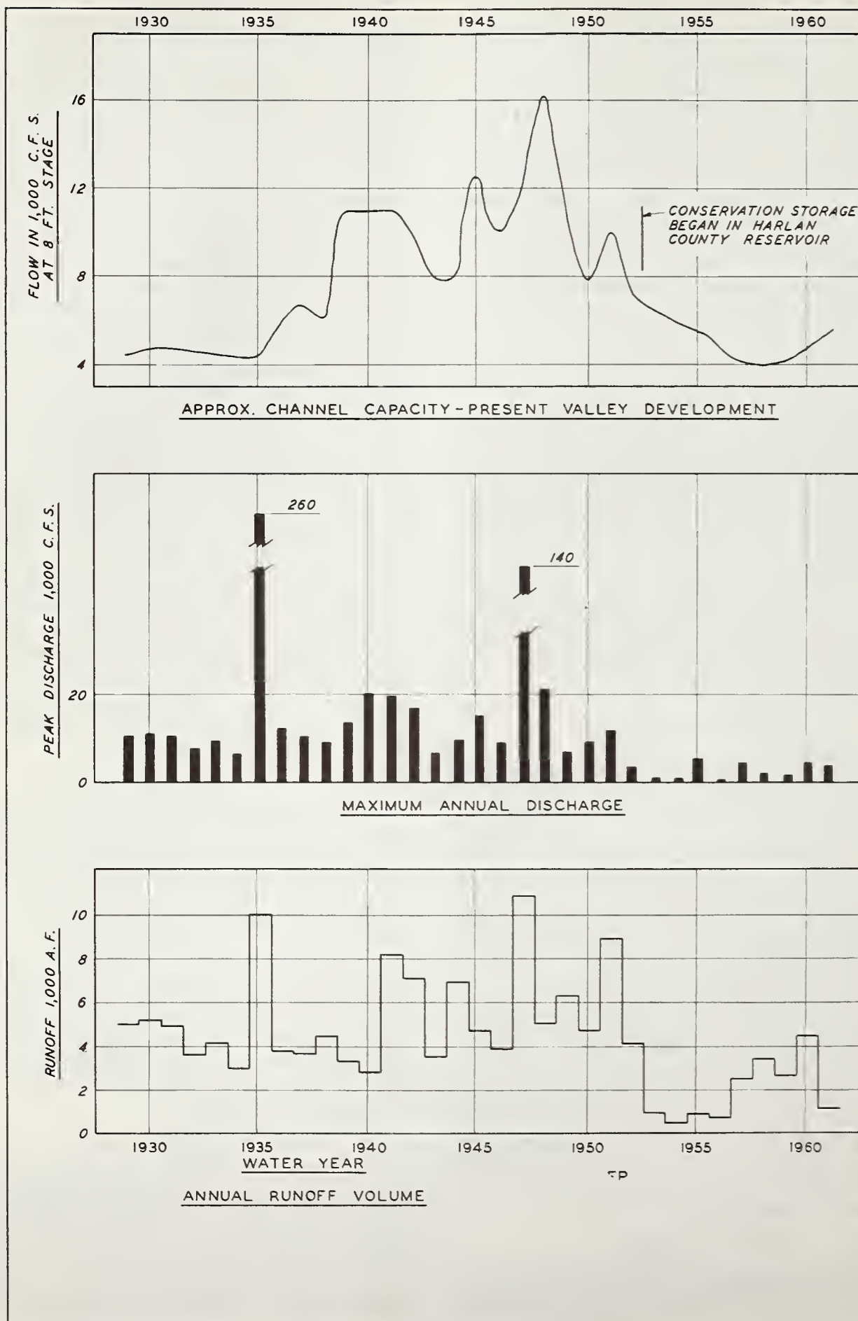
FIGURE 6. — Hydrologic history of Republican River at Bloomington, 1930-60.
