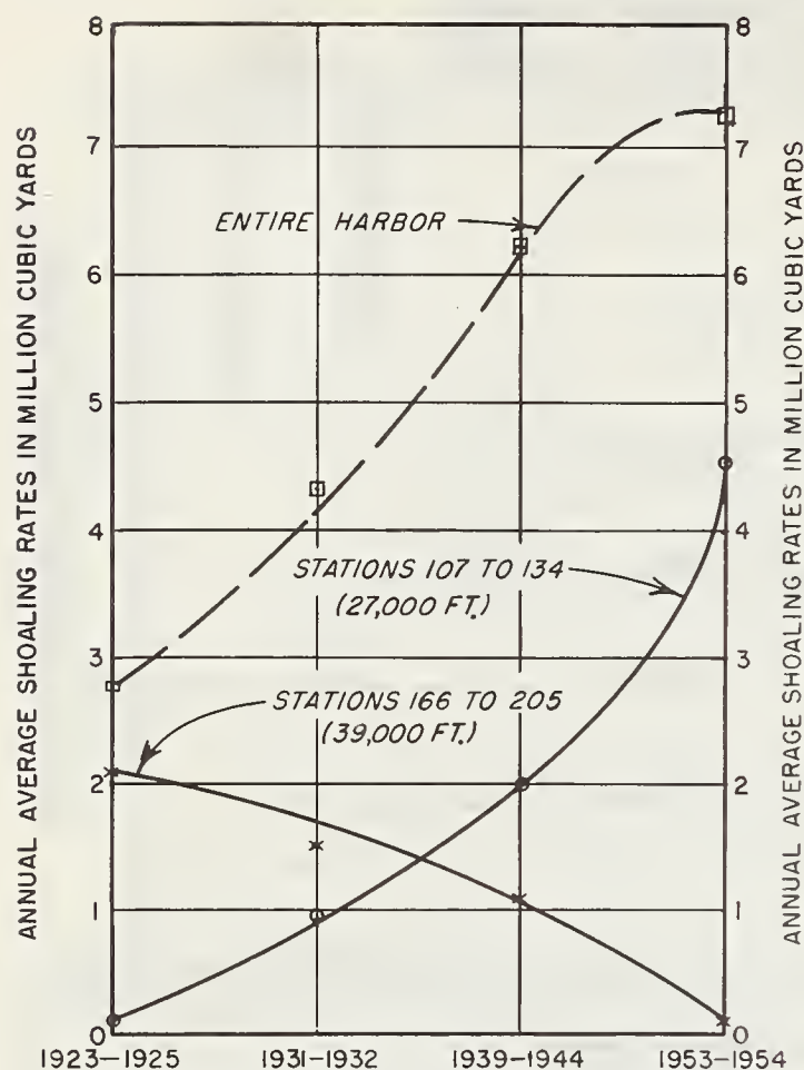
FIGURE 5. — Past and present shoaling characteristics of Savannah Harbor.
