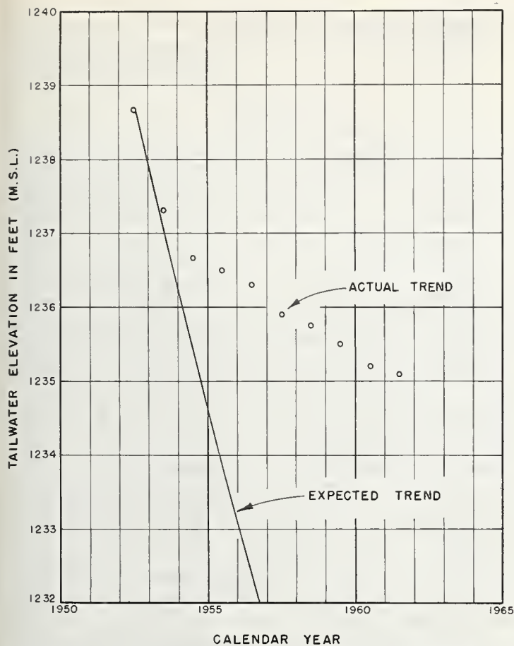
FIGURE 4.—Tailwater elevation trend since closure of Fort Randall Dam in 1952.
