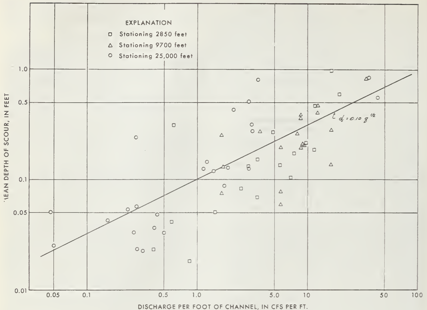
FIGURE 2. — Depth of scour as a function of unit discharge.
