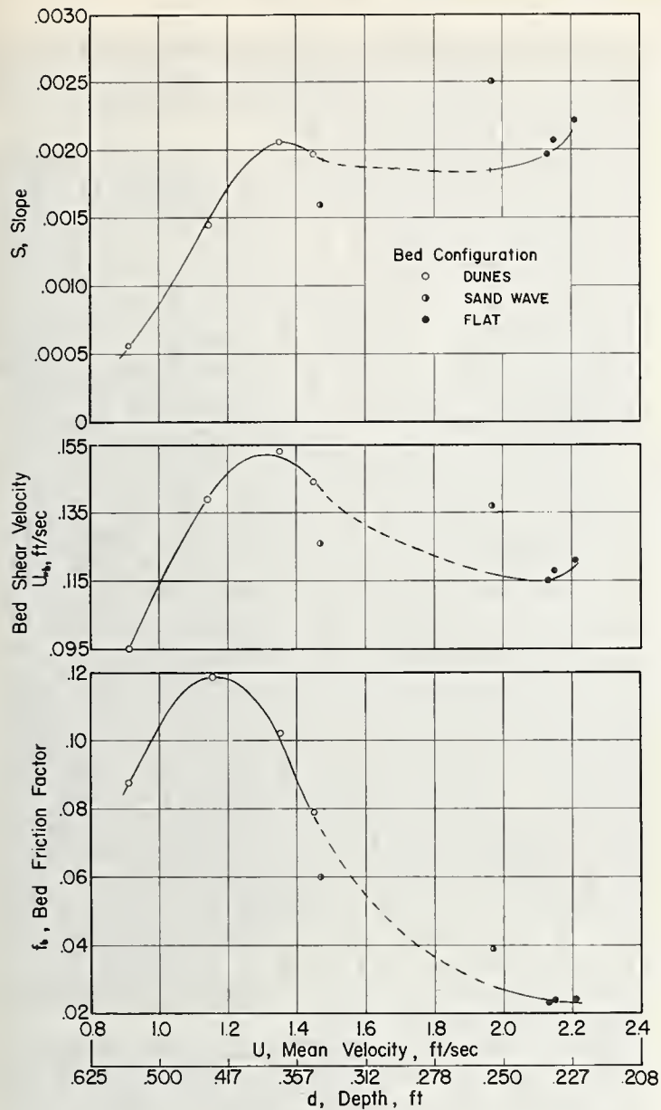
FIGURE 3.—Variation of slope, bed shear velocity, and bed friction factor with mean velocity and depth for constant-discharge experiments ( q = 0.50 c.f.s. per foot).
