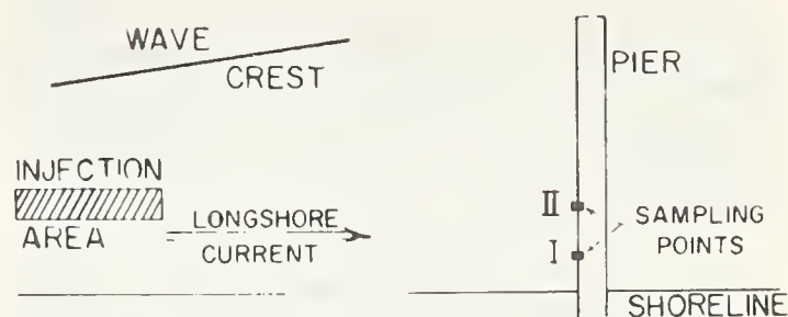
FIGURE 2.—Location of tracer material in relation to Fernandina Beach pier, northwestern Florida.
