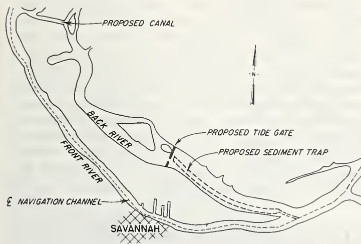
FIGURE 6. — Elements of sediment trap plan for Savannah Harbor.
