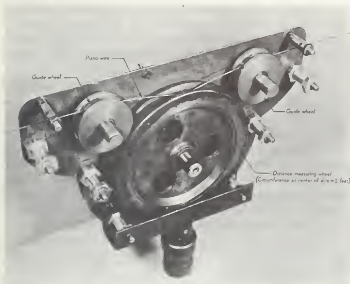
FIGURE 5. — Distance-measuring wheel with cover removed.
