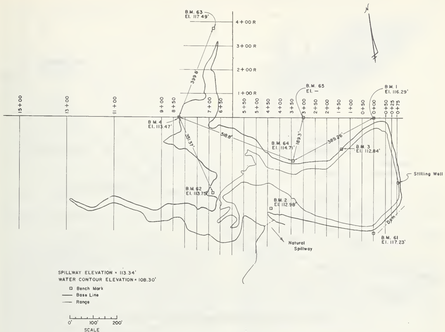
FIGURE 4. — Mitchell Reservoir, Newell, S. Dak., sedimentation survey, May 1960.
