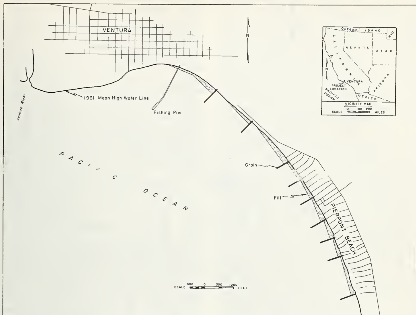
FIGURE 1. — Ventura area, California, general plan of improvement.
