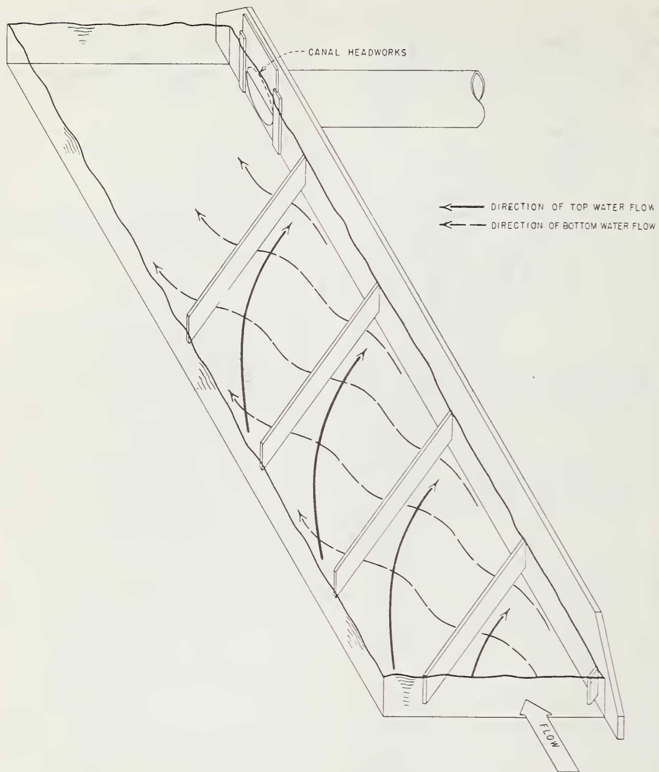
FIGURE 2. — Surface guide vane method of producing secondary currents for sediment control.
