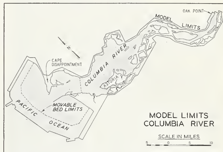
FIGURE 27. — General layout of Columbia hydraulic model.
