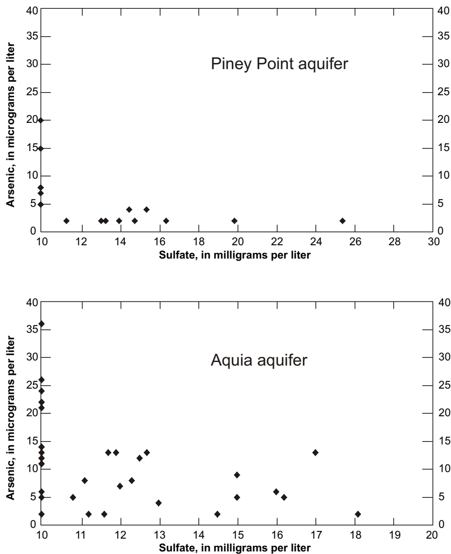
Figure 16. Variation of sulfate content with arsenic in the Aquia and Piney Point aquifers. Samples with more than 20 mg/L chloride were excluded because of possible interference with arsenic analyses.
