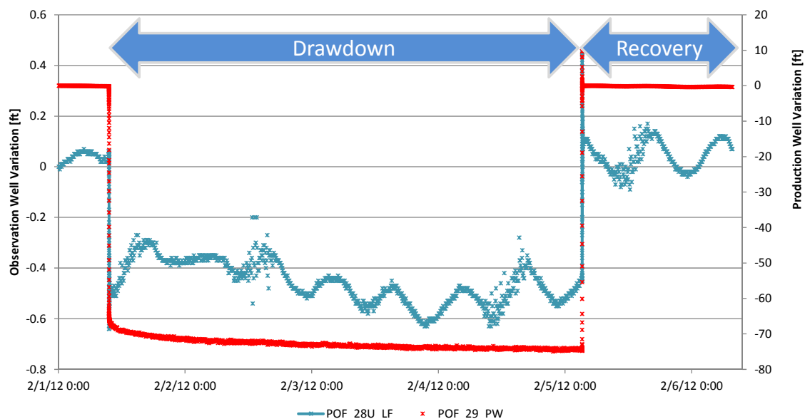
Figure 31. Observed drawdown [ft] in the production zone during the CRDT.
