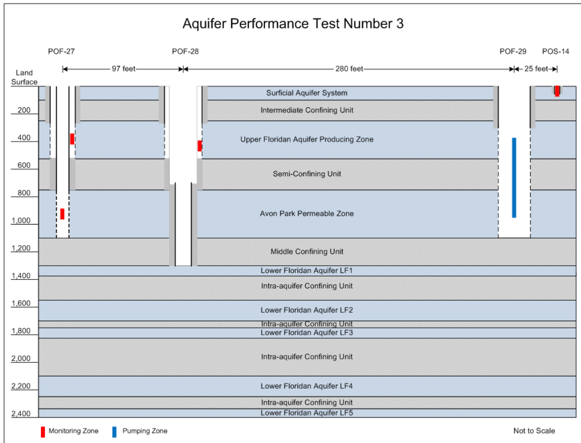
Figure 27. Well configuration for APT 3.
