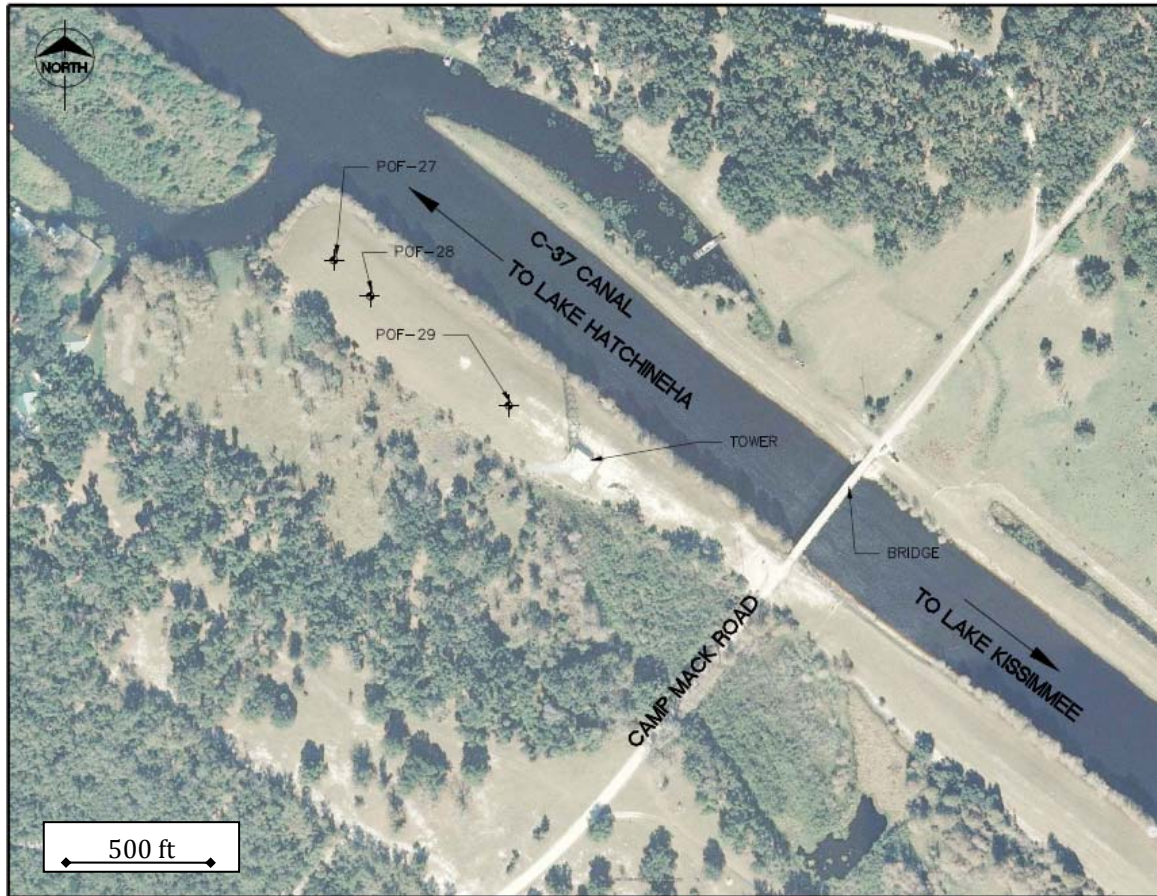
Figure 2. Site B general layout.
