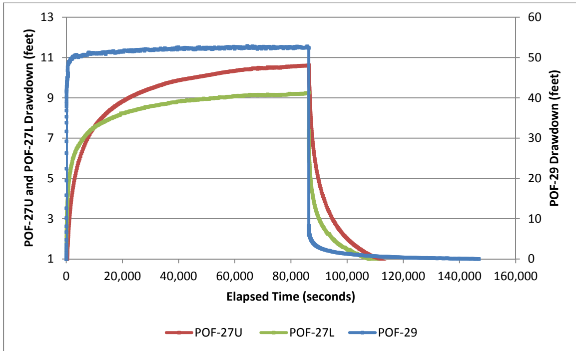
Figure 28. Observed drawdown in the production-zone during APT 3.
