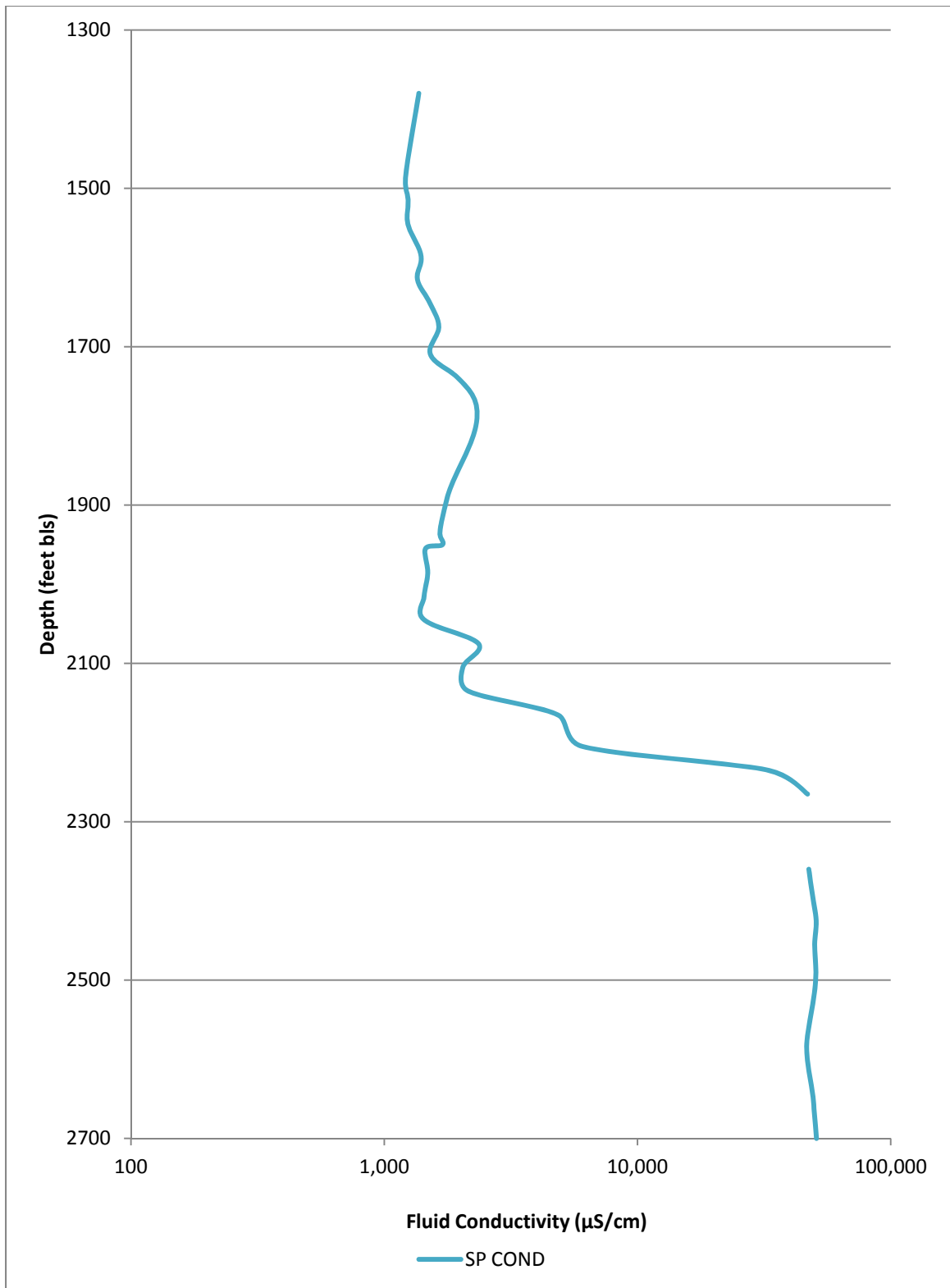
Figure 14. Drill-stem specific conductance from POF-28 (data gap due to an electrical short in the sensor).
