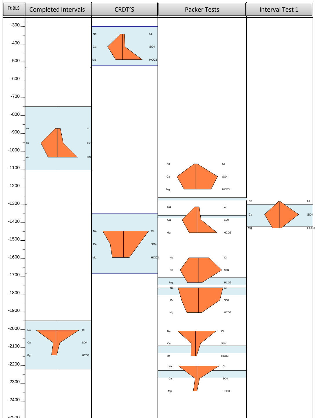
Figure 17. Stiff plots illustrating the relative distribution of major cations ( \text{Na}^+ , \text{Ca}^{2+} , \text{Mg}^{2+} ) and anions ( \text{Cl}^- , \text{SO}_4^{2-} , \text{HCO}_3^- ) with depth (milliequivalents per liter). Each plot represents a discretely sampled depth interval within the Floridan aquifer system at Site B.
