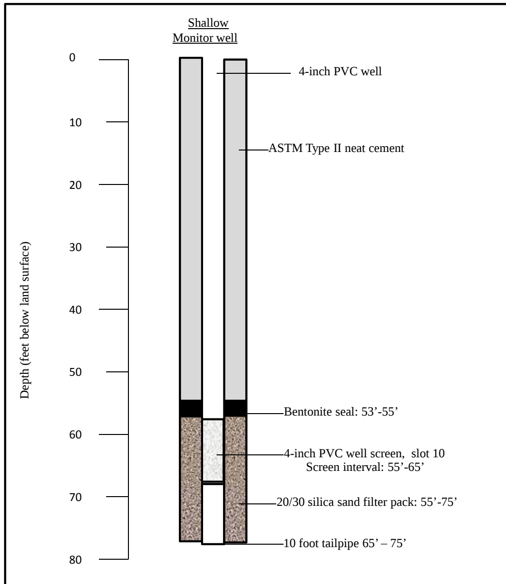
Figure 3. POS-14 completed well construction.
