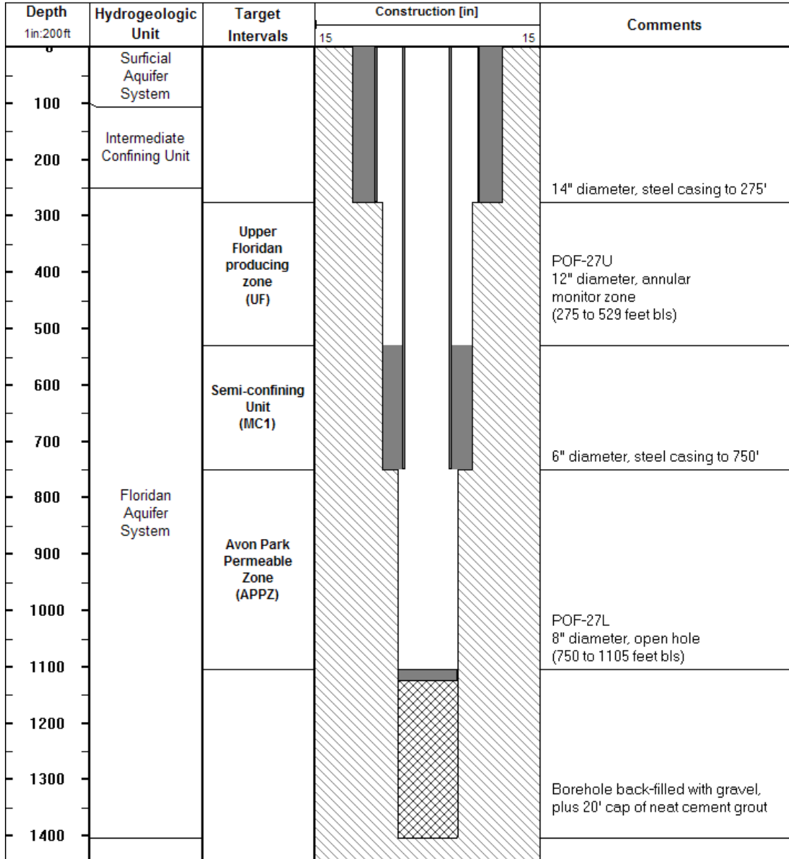
Figure 4. Well completion diagram, POF-27.
