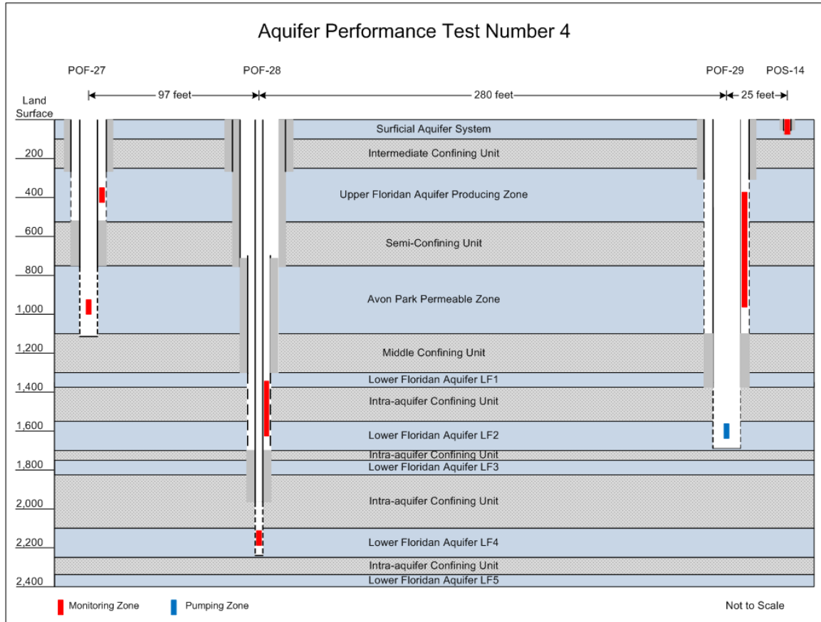
Figure 30. Well configuration for APT 4.
