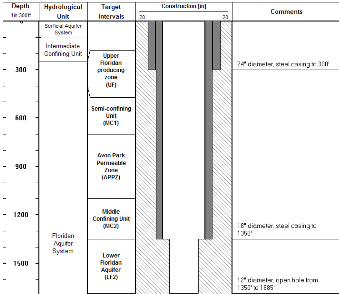
Figure 9. Well completion diagram, POF-29.
