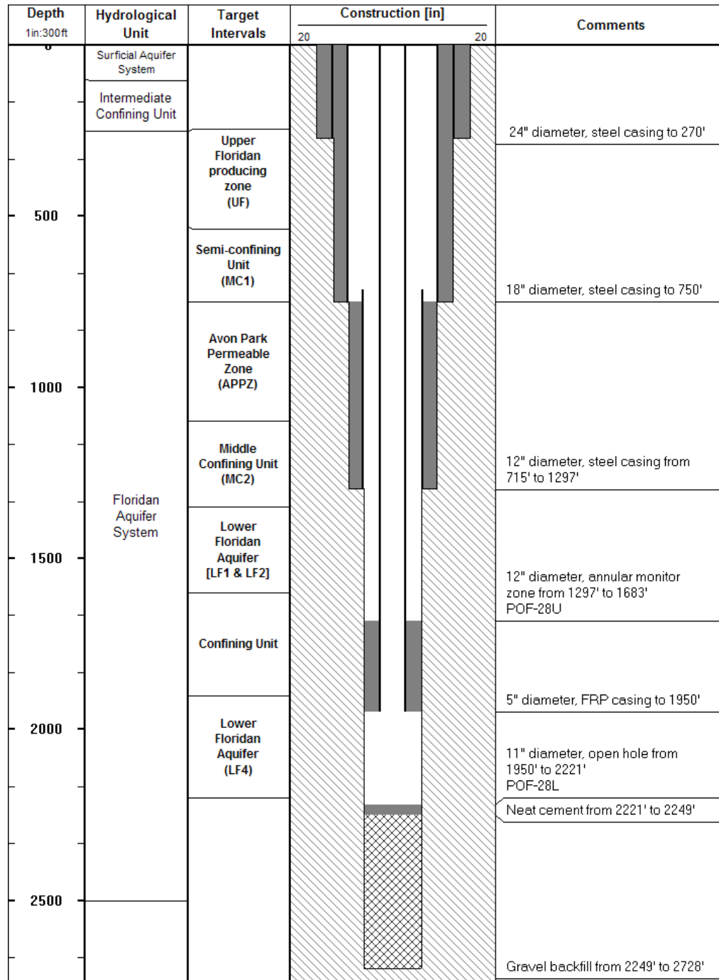
Figure 6. Well completion diagram, POF-28.
