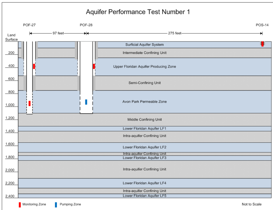
Figure 19. Well configuration for APT 1.
