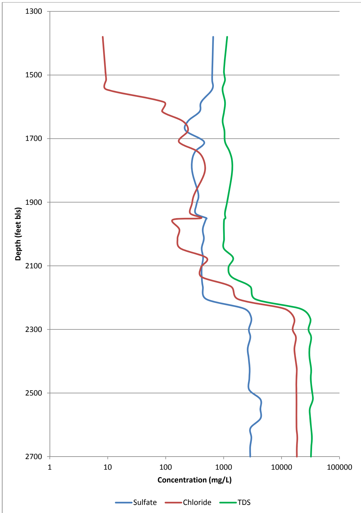
Figure 15. Chloride, sulfate, and TDS data from POF-28 drill stem water quality samples.
