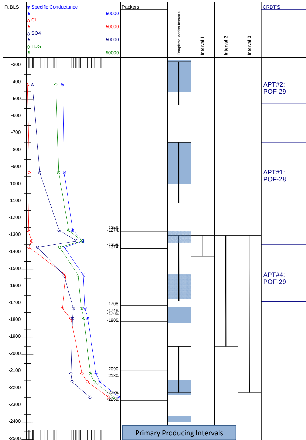
Figure 16. Locations of sample depth intervals, most productive intervals, and distribution of specific conductance ( \mu\text{S}/\text{cm} ), and \text{Cl}^- , \text{SO}_4^{2-} , and TDS concentrations ( \text{mg}/\text{L} ) from those sample results from POF-27, POF-28, and POF-29. For packer tests, the water quality results are centered between the two packer depths. For larger sampled intervals, results are positioned in the graph according to the most likely source depth based on flow logging interpretation of the most productive section of the borehole open to that sample.
