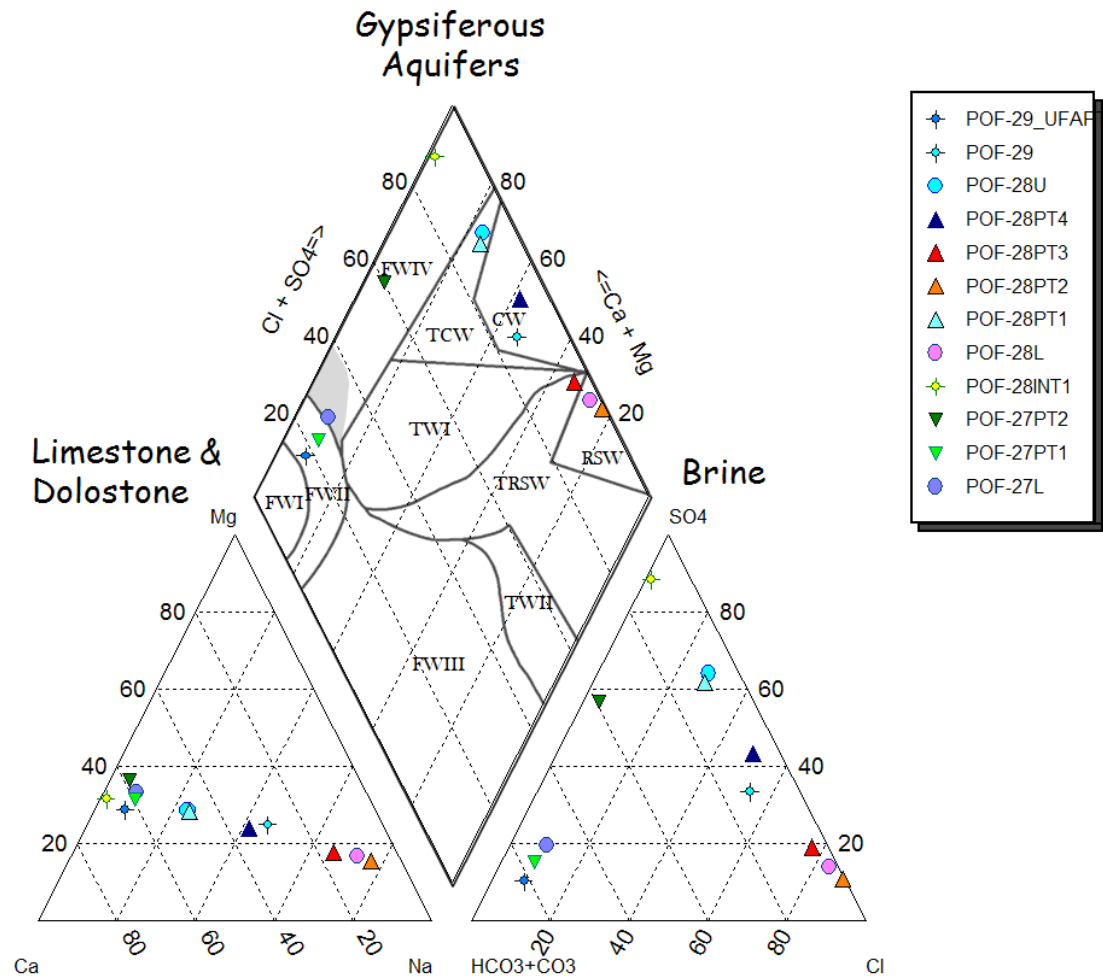
Figure 18. Water type classification of Site B sample data (after Frazee 1982).
