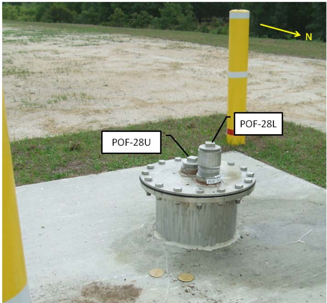
Figure 7. Final wellhead, POF-28.
