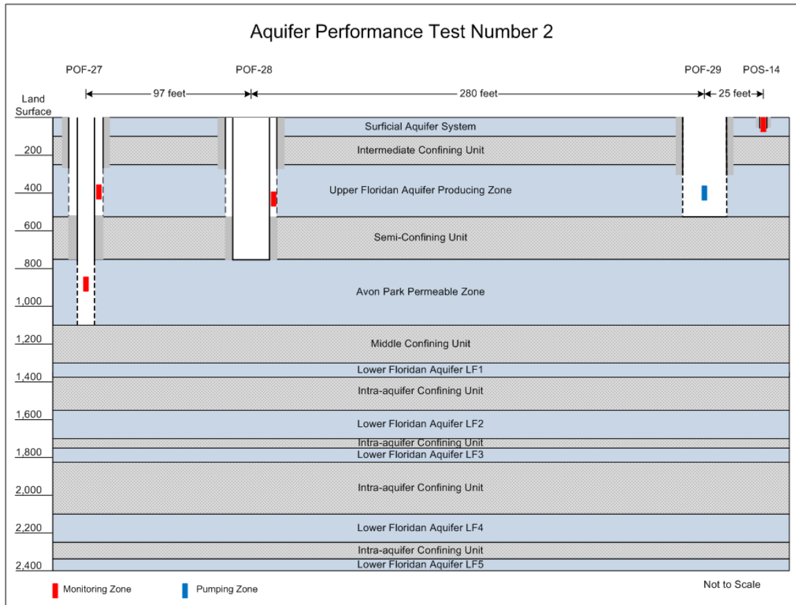
Figure 23. Well configuration for APT 2.
