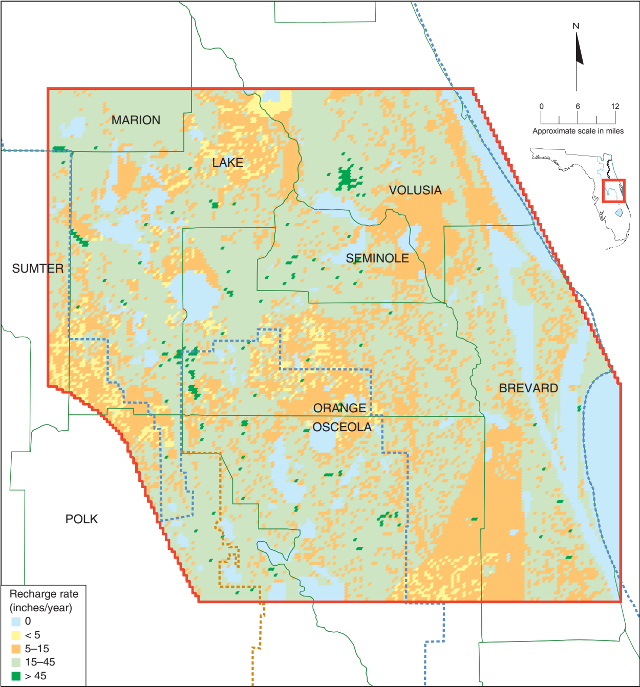
Figure 86. Recharge applied to the surficial aquifer system for average 2020 conditions
