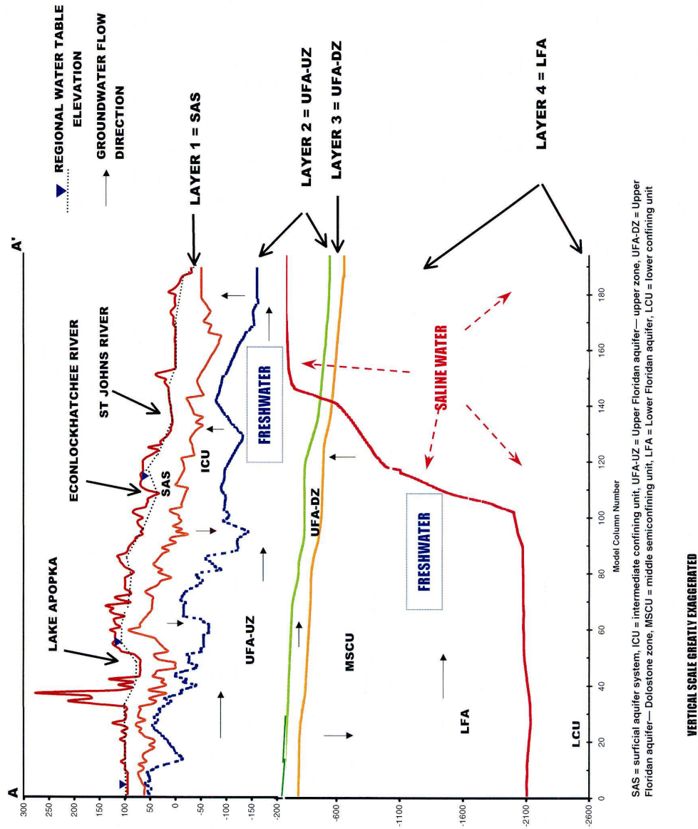
Figure 25. Hydrogeologic cross section along model row 80 showing the conceptual model of regional groundwater flow in east-central Florida
