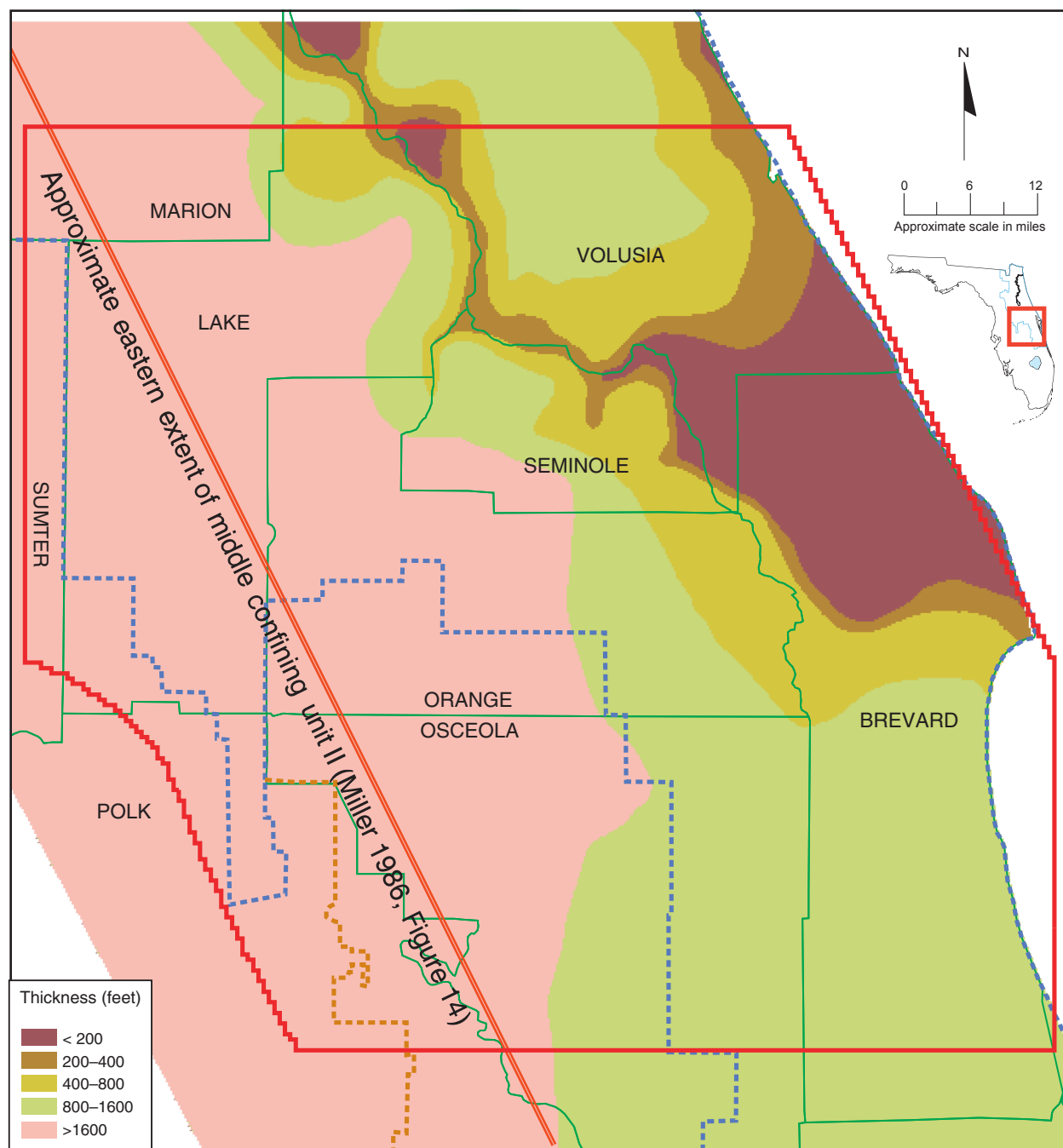
Figure 24. Thickness of the Floridan aquifer system containing chloride concentrations less than 5,000 milligrams per liter (from McGurk et al. 1998)
