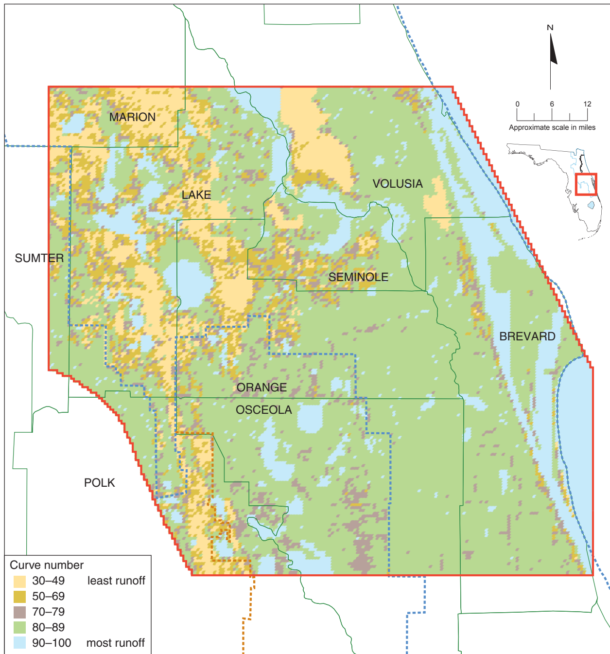
Figure 39. Soil Conservation Service curve numbers, used for estimation of total overland runoff
