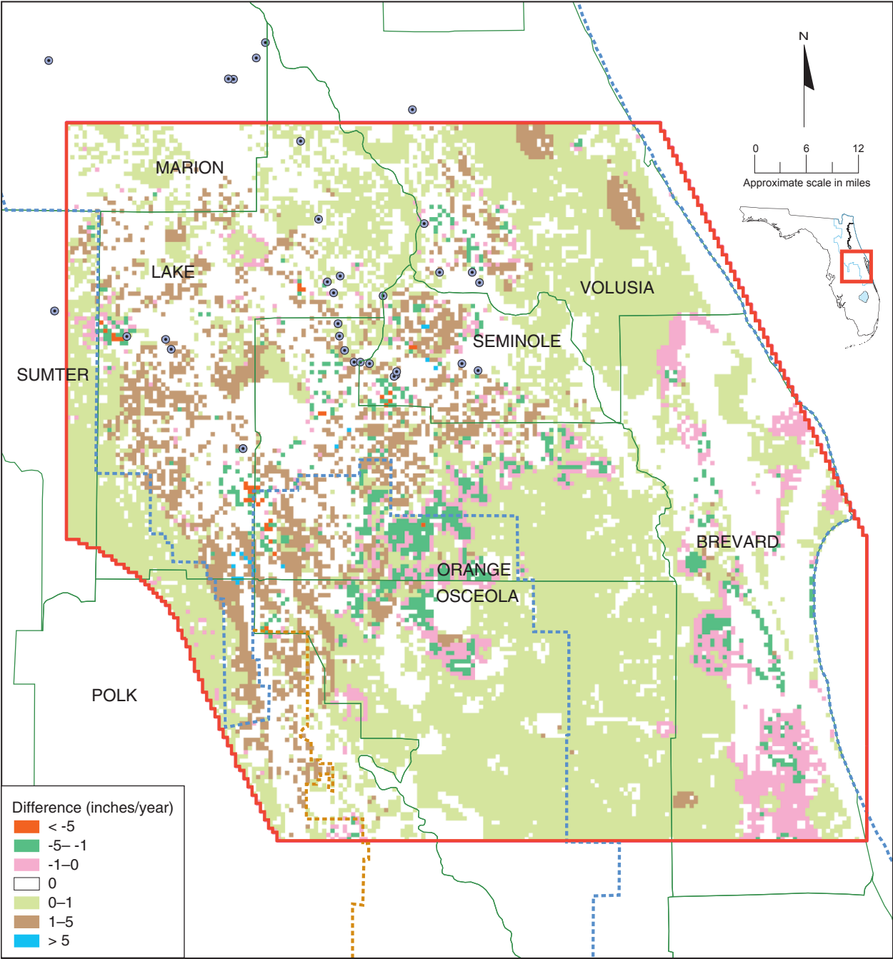
Figure 91. Difference between simulated average evapotranspiration rates, 1995–2020
