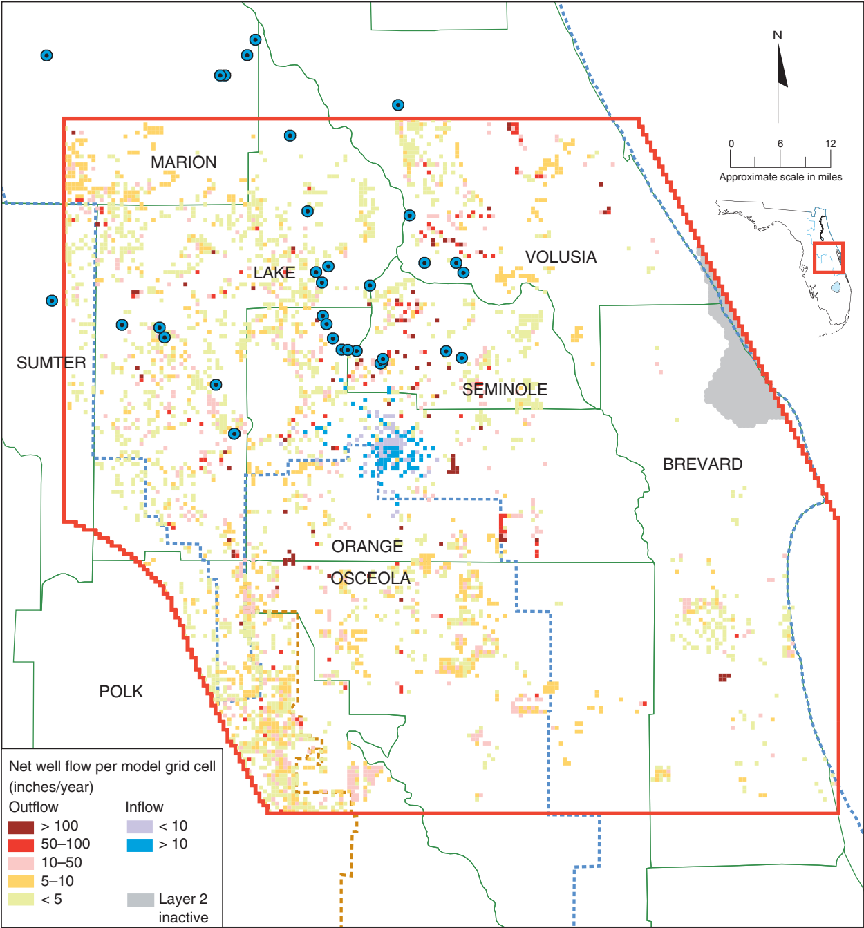
Figure 80. Average 2020 well fluxes, model layer 2 (Upper Floridan aquifer—upper zone)
