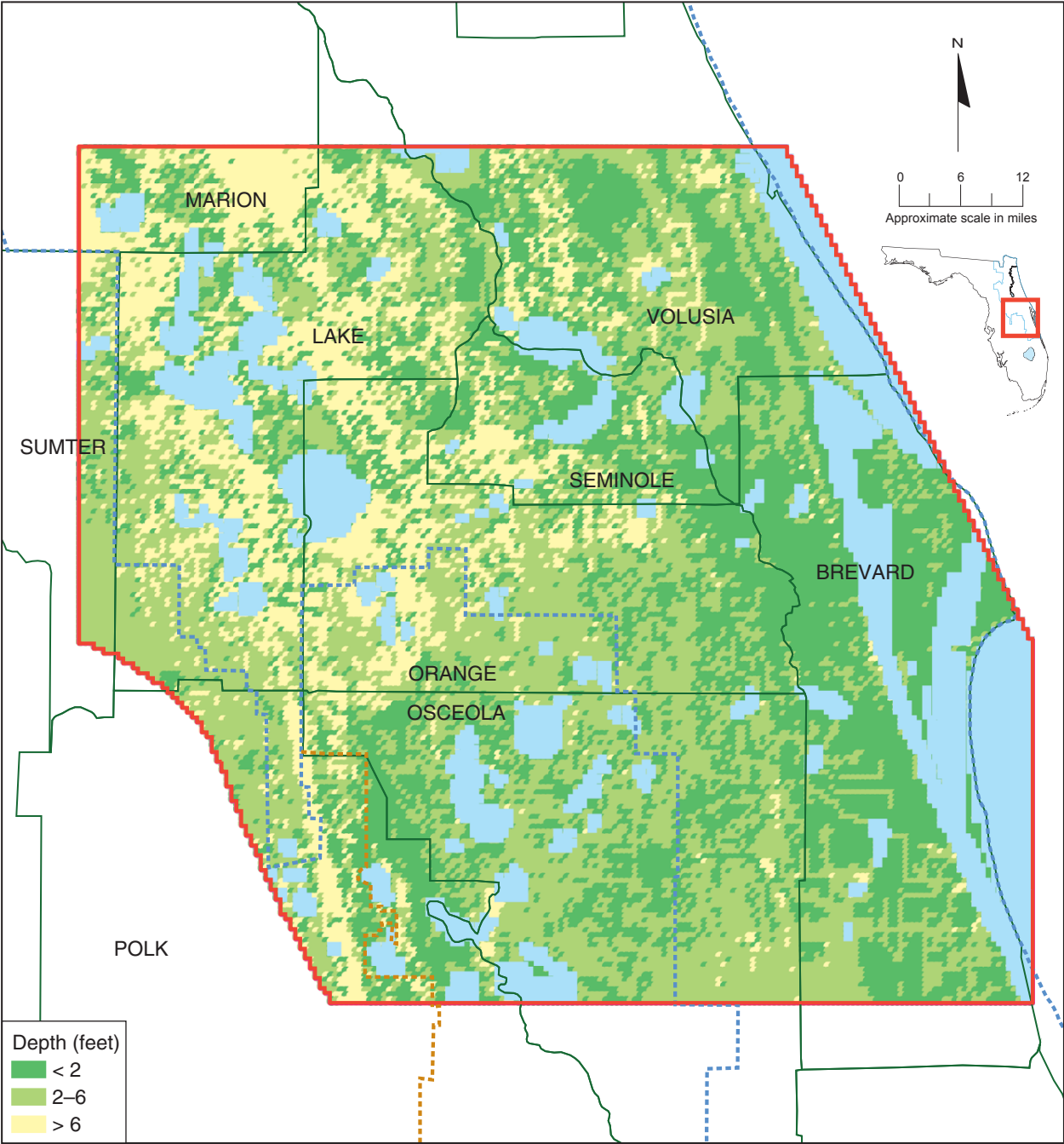
Figure 50. Average topographic elevation minus simulated layer 1 water level for average 1995 conditions
