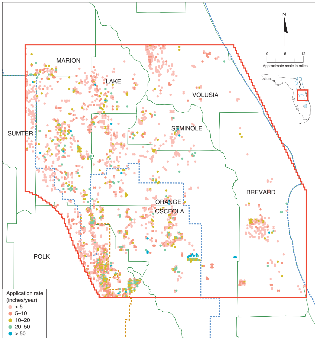
Figure 85. Average 2020 agricultural and golf course irrigation rates (derived from Floridan aquifer system withdrawals)
