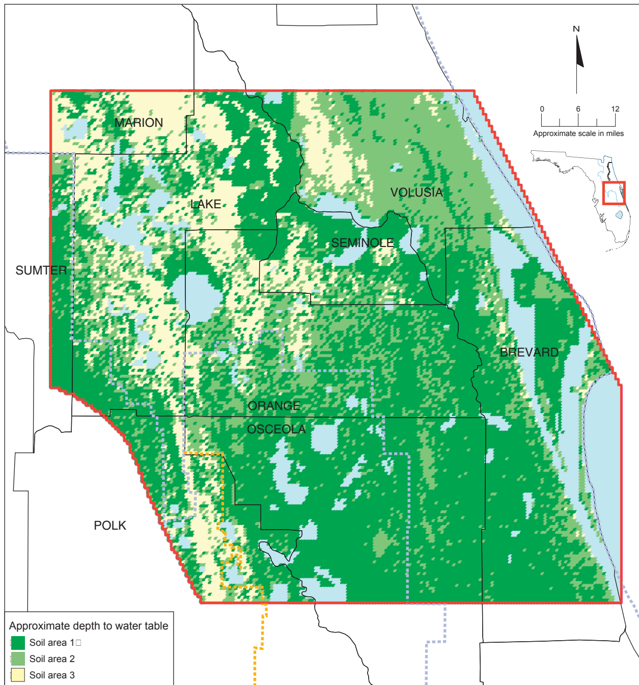
Figure 38. Soil area delineation, based upon estimated depth to the regional water table
