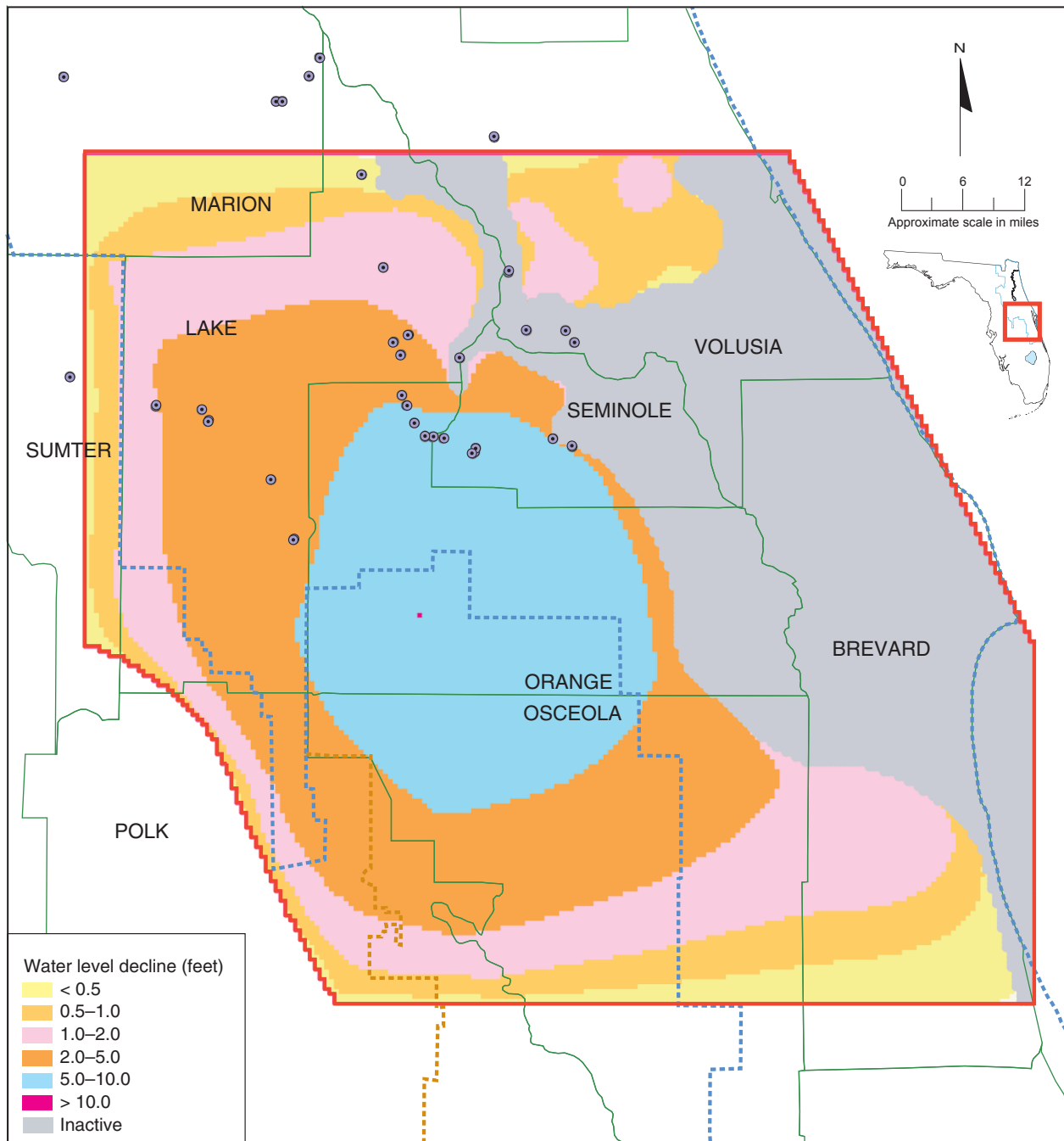
Figure 90. Predicted change in average layer 4 (Lower Floridan aquifer) water levels, 1995–2020
