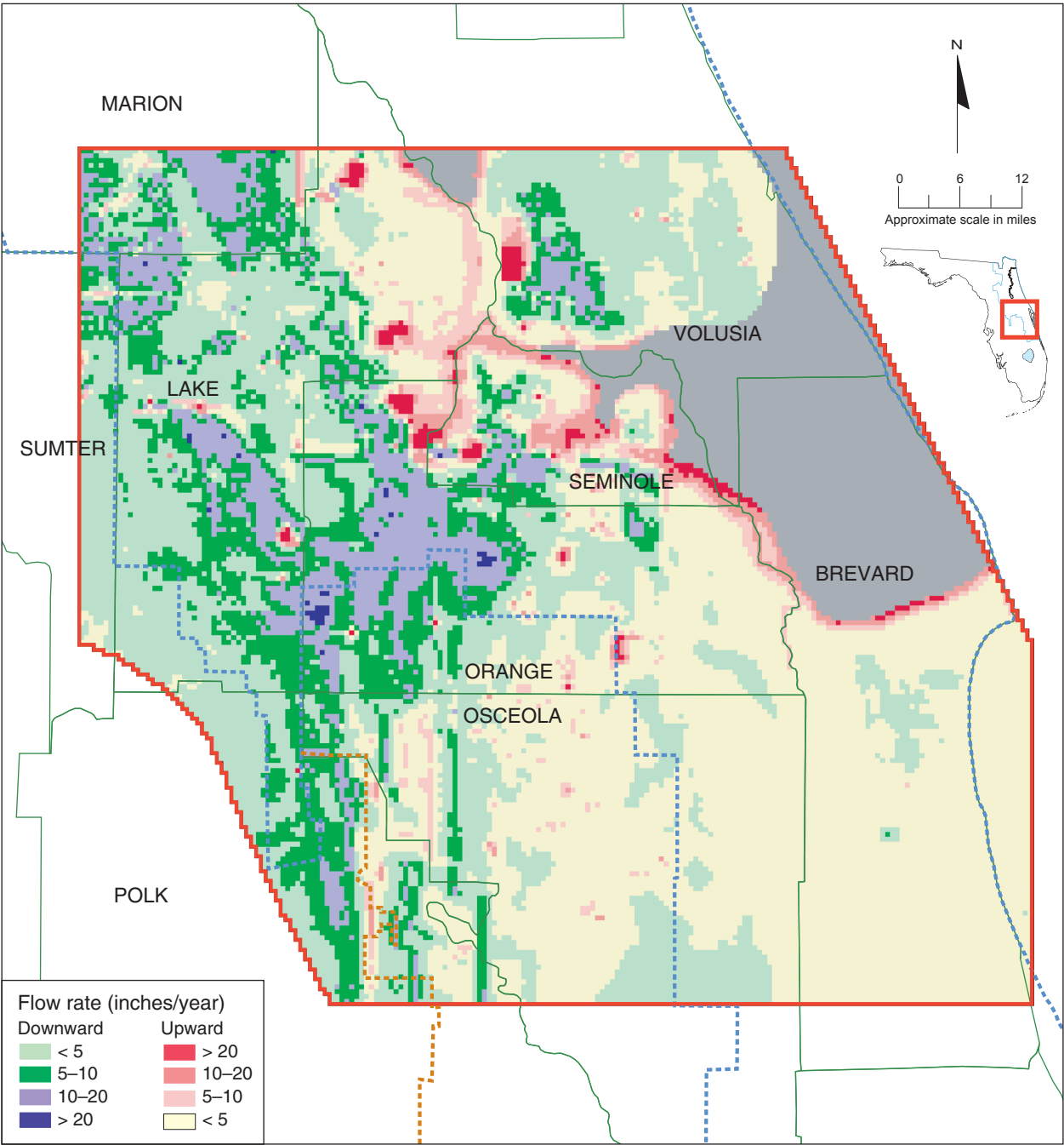
Figure 57. Simulated vertical flow between layer 2 (Upper Floridan aquifer—upper zone) and layer 3 (Upper Floridan aquifer—lower zone) for average 1995 conditions
