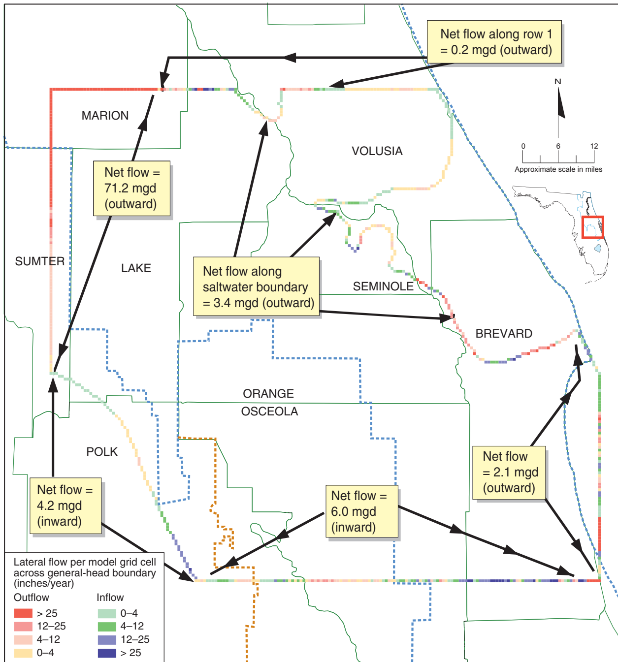
Figure 60. Simulated layer 3 (Upper Floridan aquifer—lower zone) lateral boundary flows, predevelopment conditions
