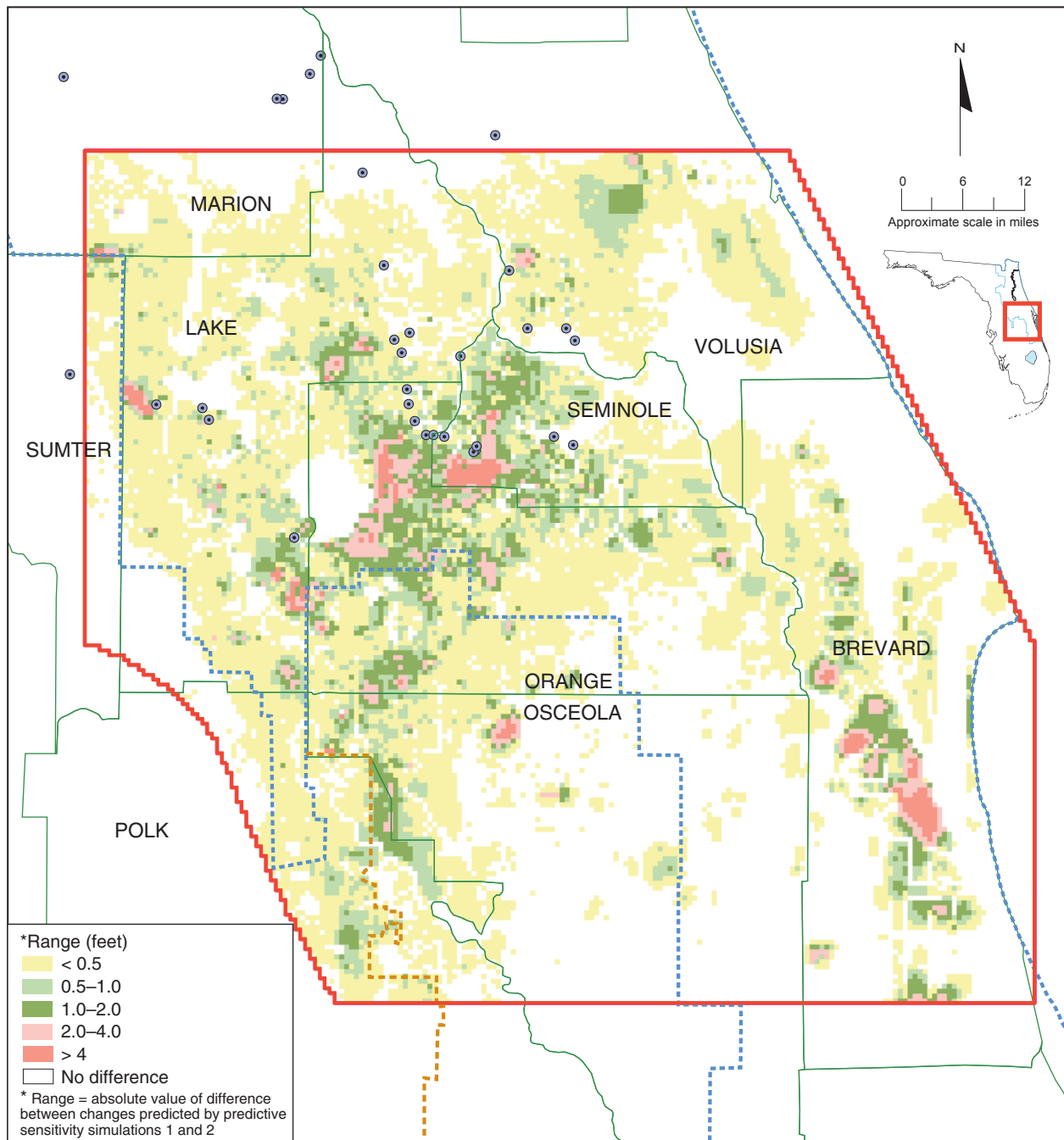
Figure 94. Range of predicted change in average surficial aquifer system water levels
