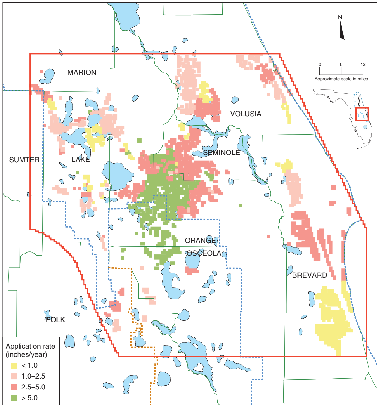
Figure 37. Average 1995 public-water supply landscape irrigation rates
