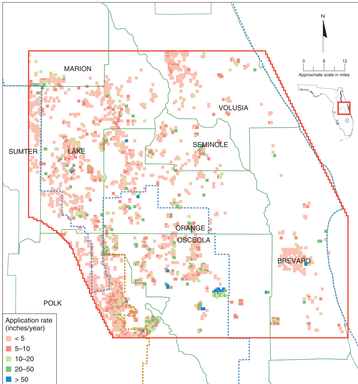
Figure 36. Average 1995 agricultural and golf course irrigation rates (derived from Floridan aquifer system withdrawals)
