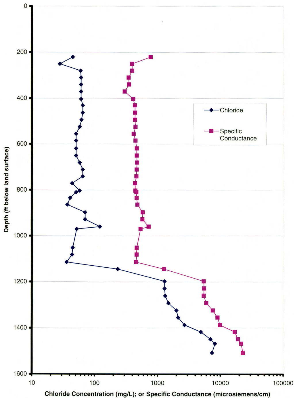
Figure 23. Chloride concentration and specific conductance versus depth at well 288 in eastern Orange County (data collected during drilling of test well)
