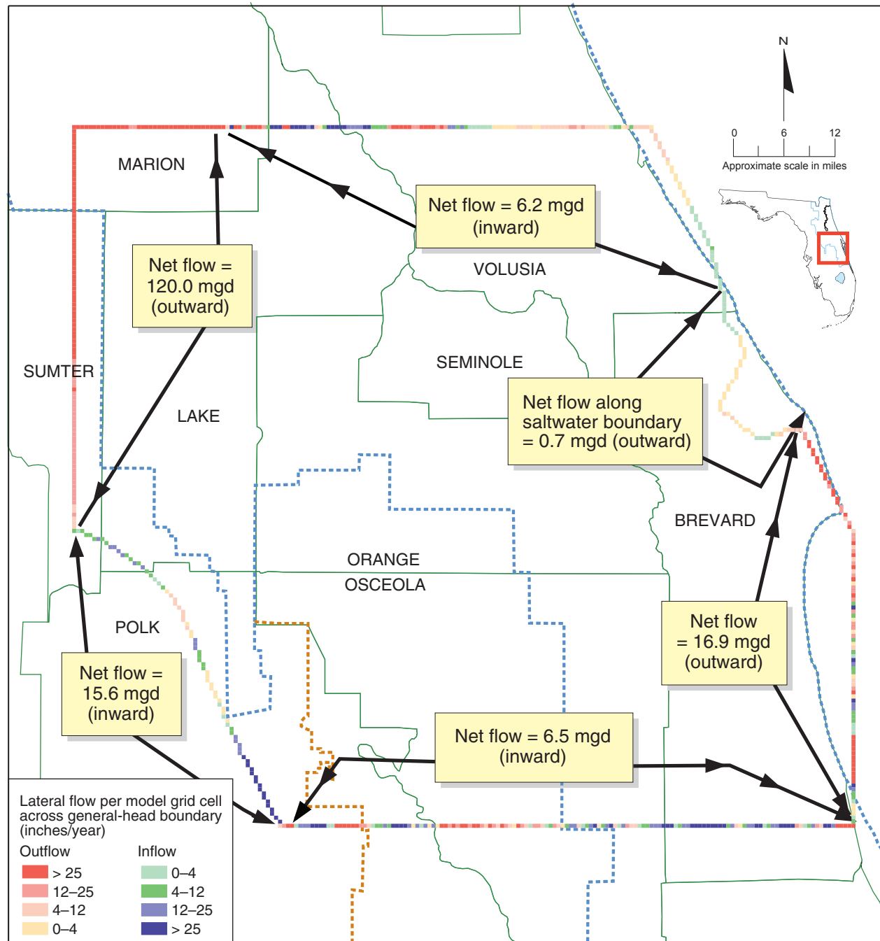
Figure 59. Simulated layer 2 (Upper Floridan aquifer—upper zone) lateral boundary flows, predevelopment conditions
