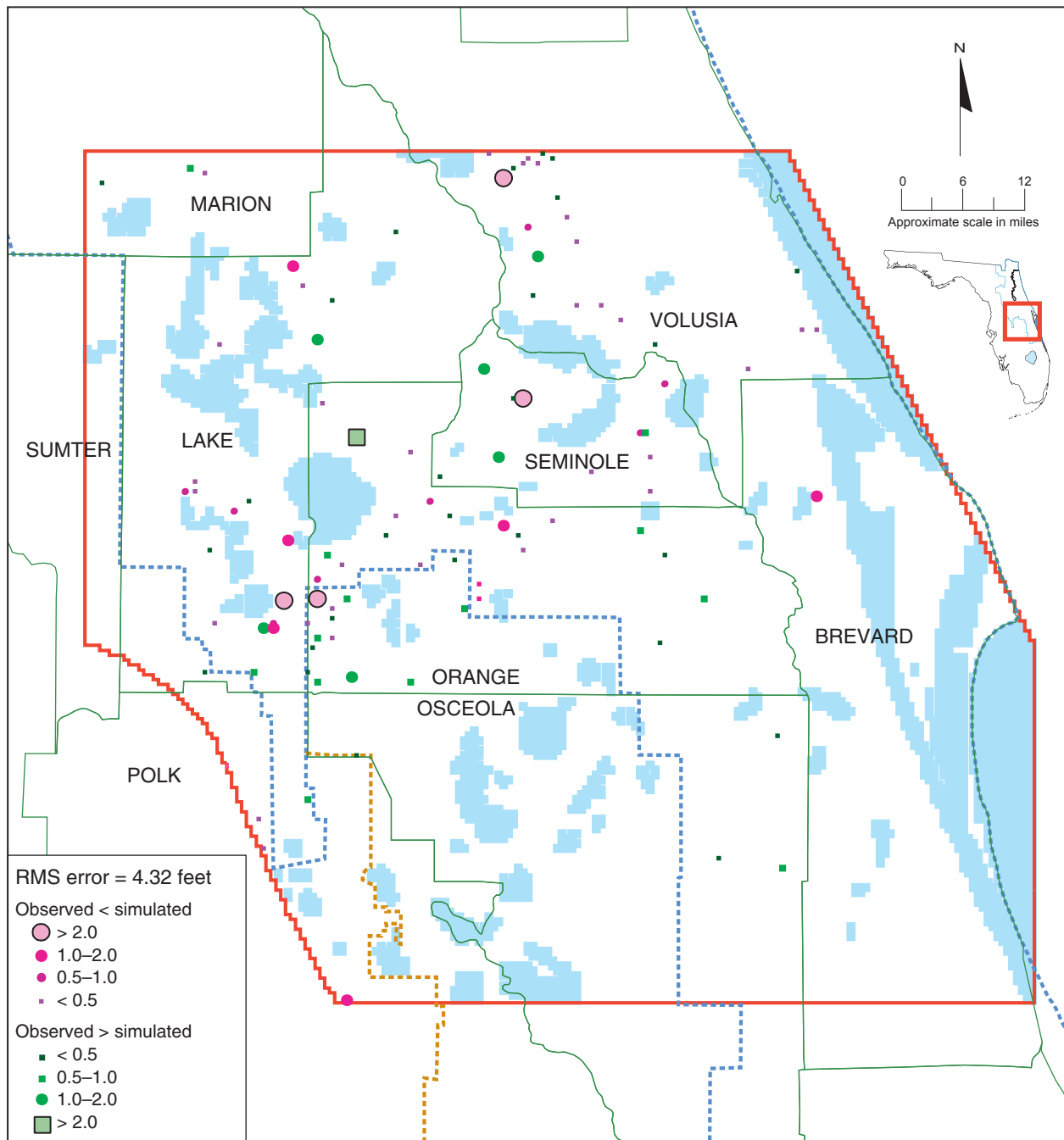
Figure 47. Surficial aquifer system head residuals for 1995 calibration, scaled by standard deviation (root-mean-square [RMS] error)
