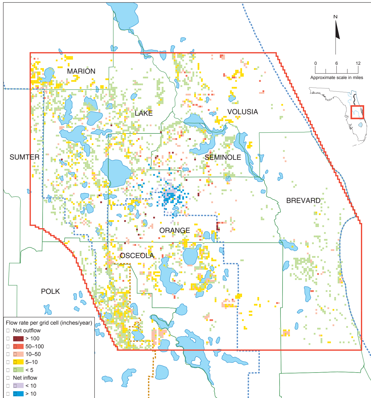
Figure 30. Average 1995 withdrawals applied to model layer 2
