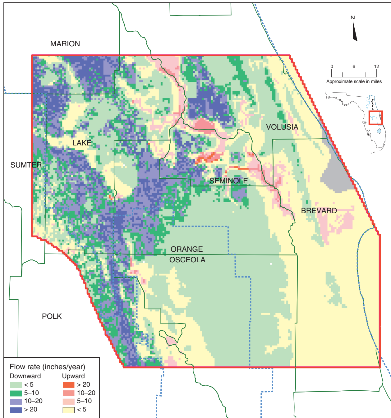
Figure 56. Simulated vertical flow between layer 1 (surficial aquifer system) and layer 2 (Upper Floridan aquifer—upper zone) for average 1995 conditions
