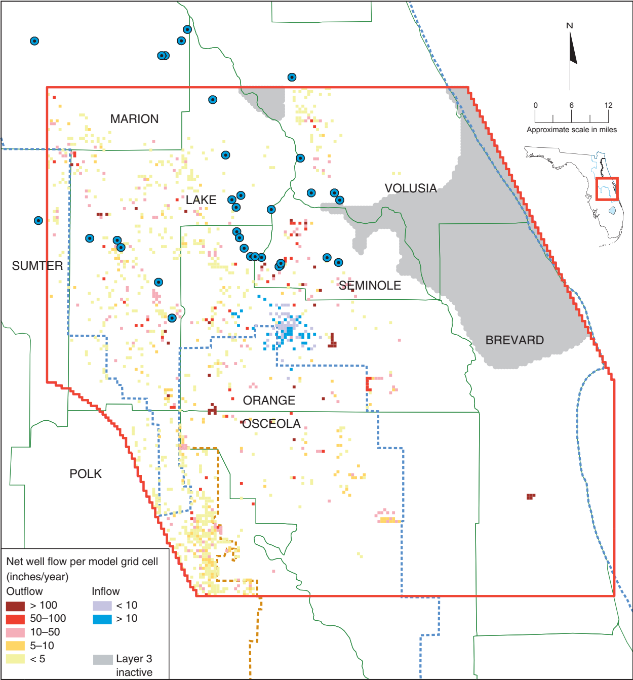
Figure 81. Average 2020 well fluxes, model layer 3 (Upper Floridan aquifer—lower zone)
