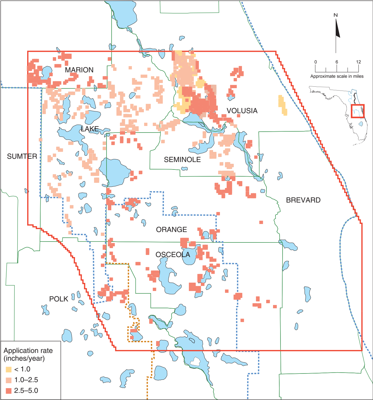
Figure 35. Estimated average 1995 septic tank effluent rates
