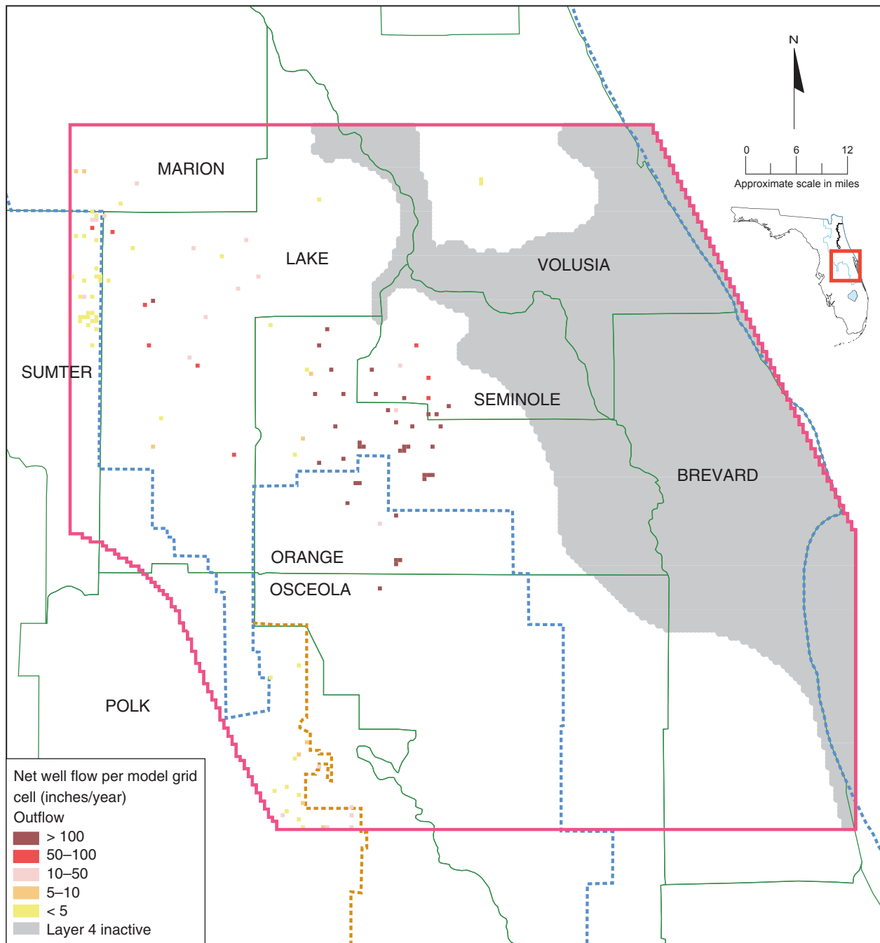
Figure 82. Average 2020 well fluxes, model layer 4 (Lower Floridan aquifer)
