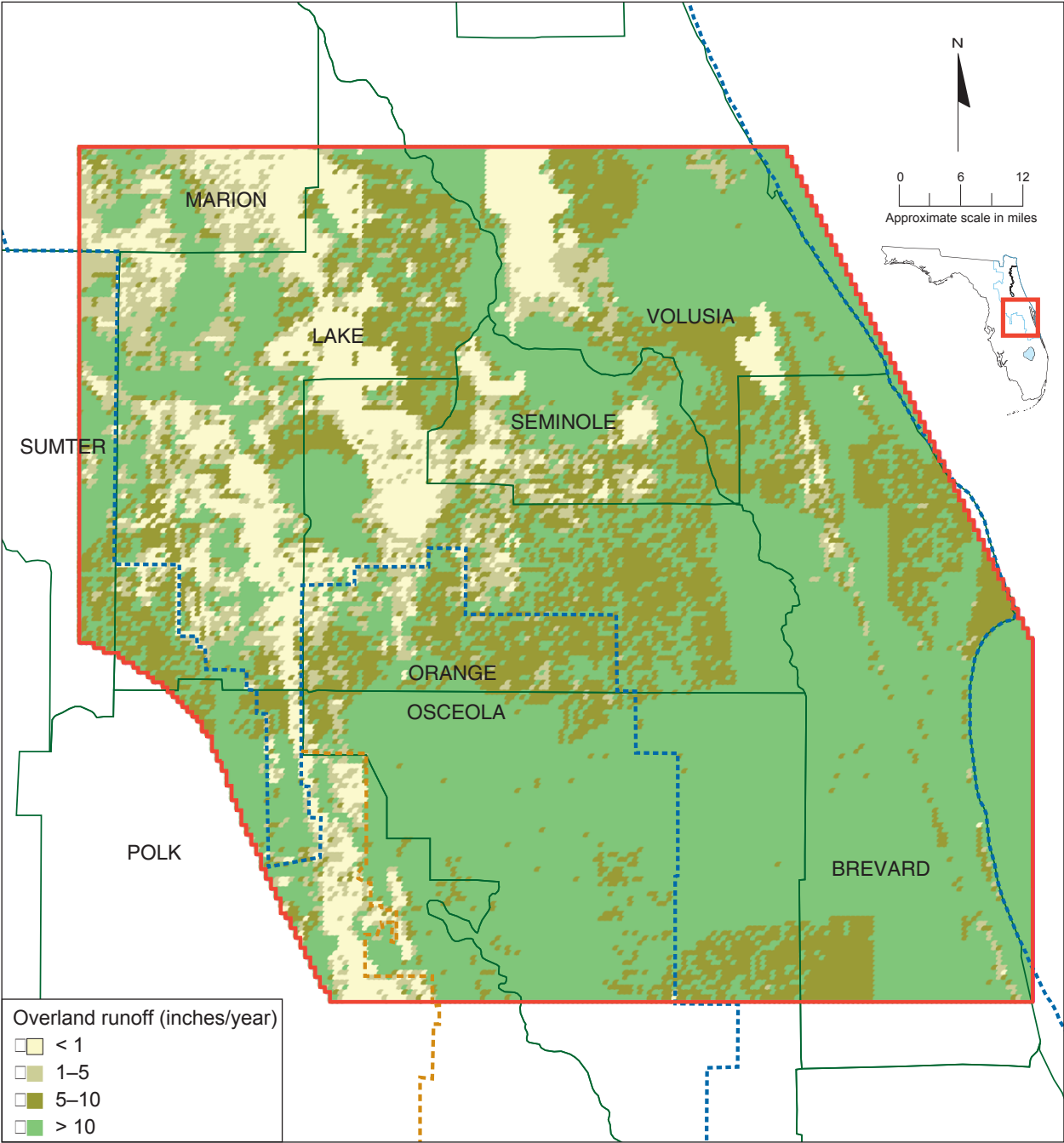
Figure 40. Total 1995 overland runoff
