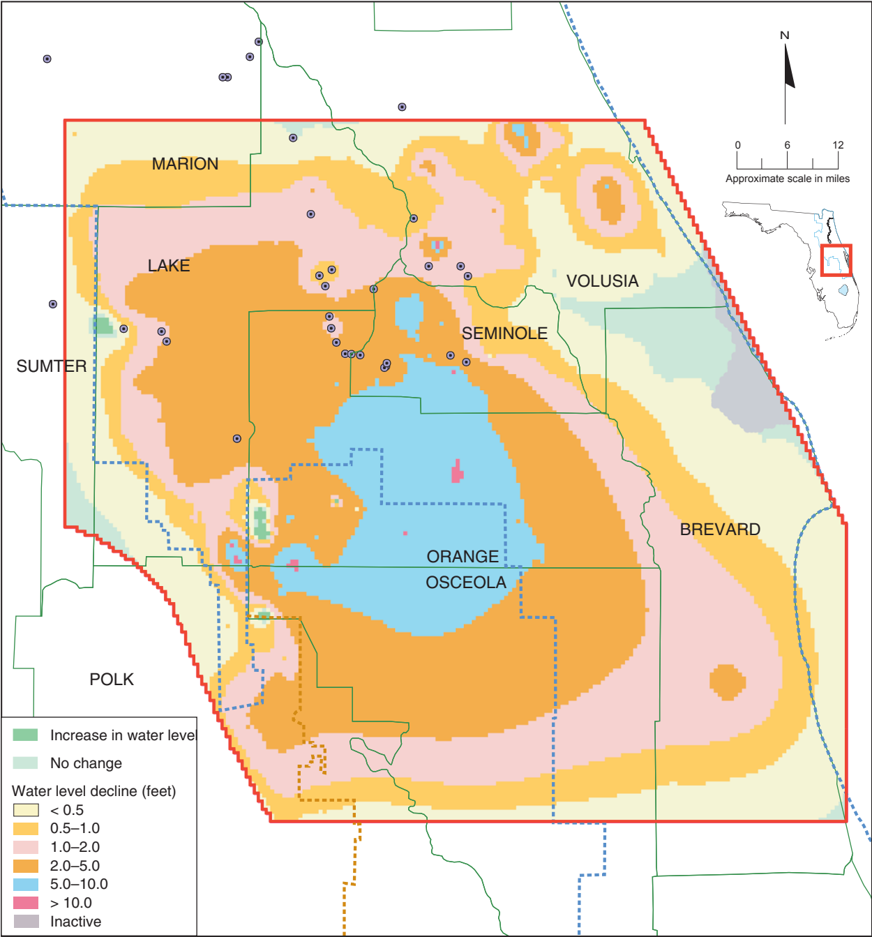
Figure 89. Predicted change in average layer 2 (Upper Floridan aquifer—upper zone) water levels, 1995–2020
