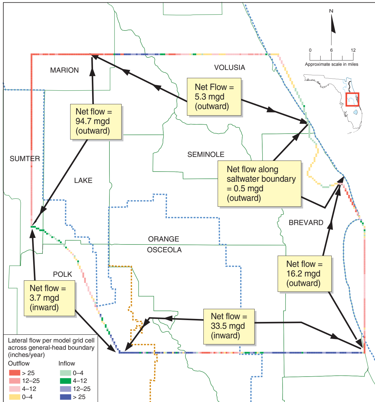
Figure 62. Simulated layer 2 (Upper Floridan aquifer—upper zone) lateral boundary flows, average 1995 conditions
