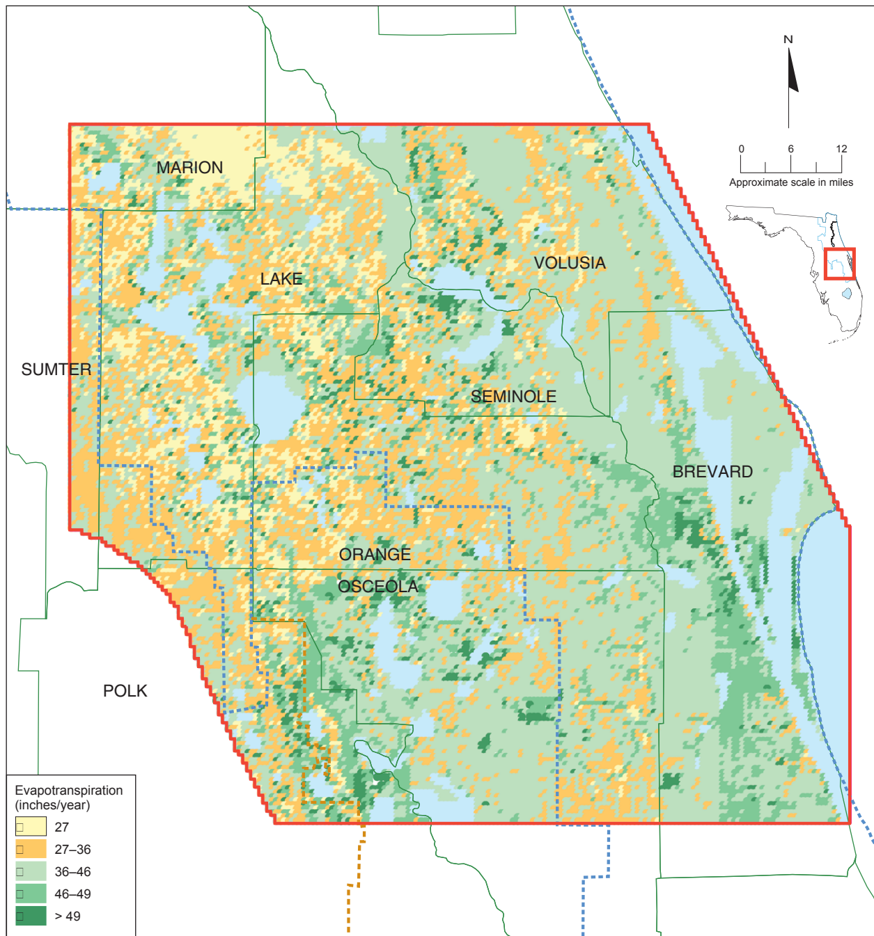
Figure 55. Estimated total evapotranspiration (ET) for average 1995 conditions (simulated ET + estimated unsaturated zone ET)
