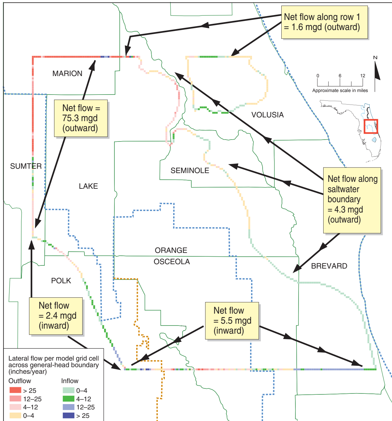
Figure 61. Simulated layer 4 (Lower Floridan aquifer) lateral boundary flows, predevelopment conditions
