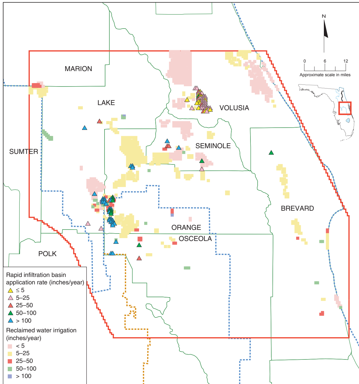
Figure 83. Average 2020 reclaimed water application rates
