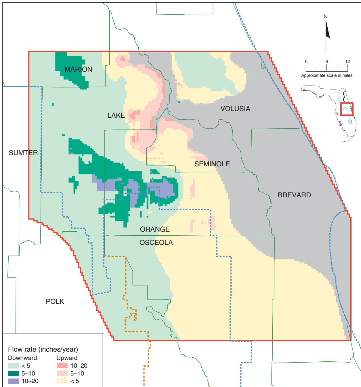
Figure 58. Simulated vertical flow between layer 3 (Upper Floridan aquifer—lower zone) and layer 4 (Lower Floridan aquifer) for average 1995 conditions
