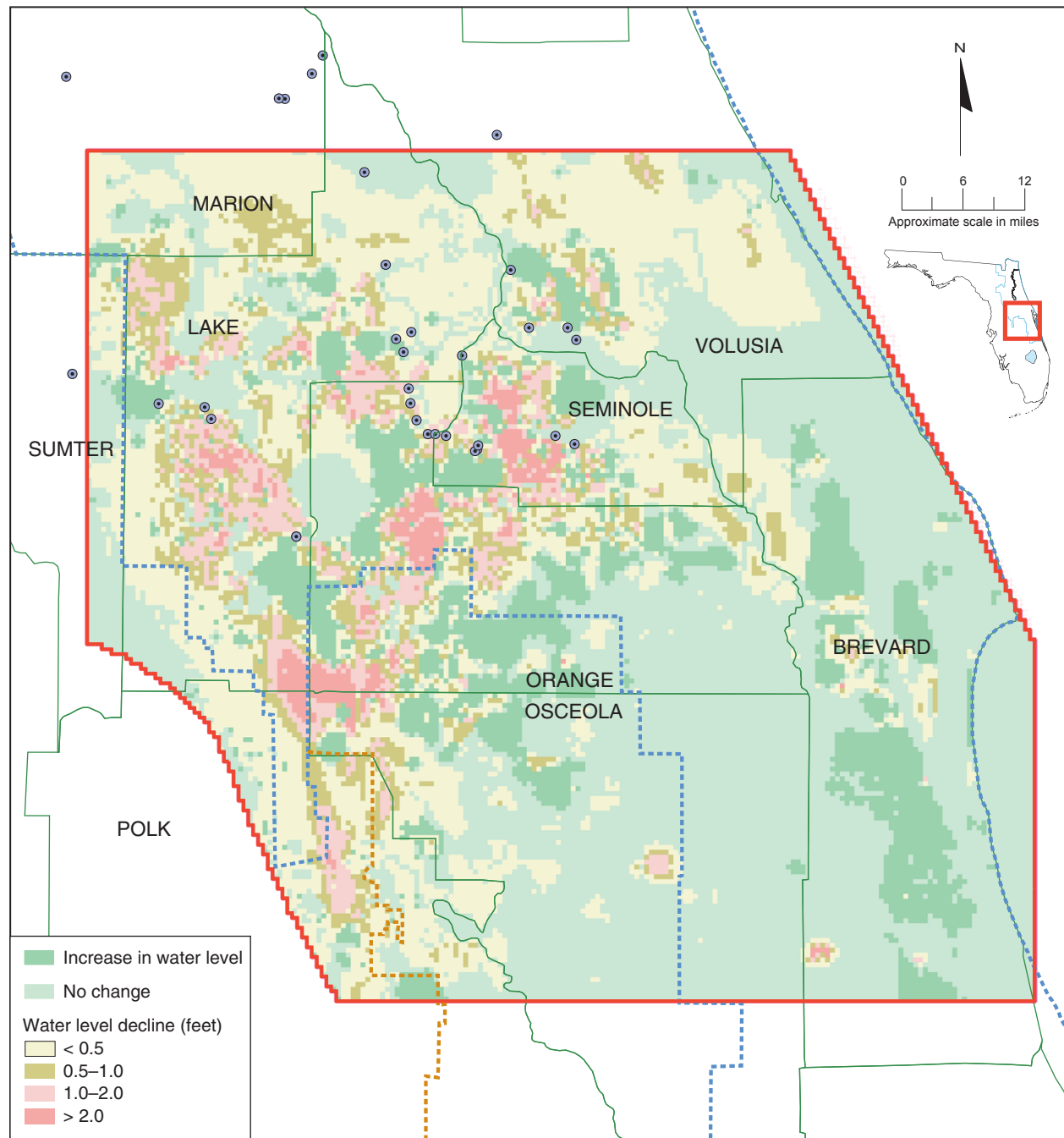
Figure 92. Predicted change in average surficial aquifer system water levels, 1995–2020, minimum drawdown simulation
