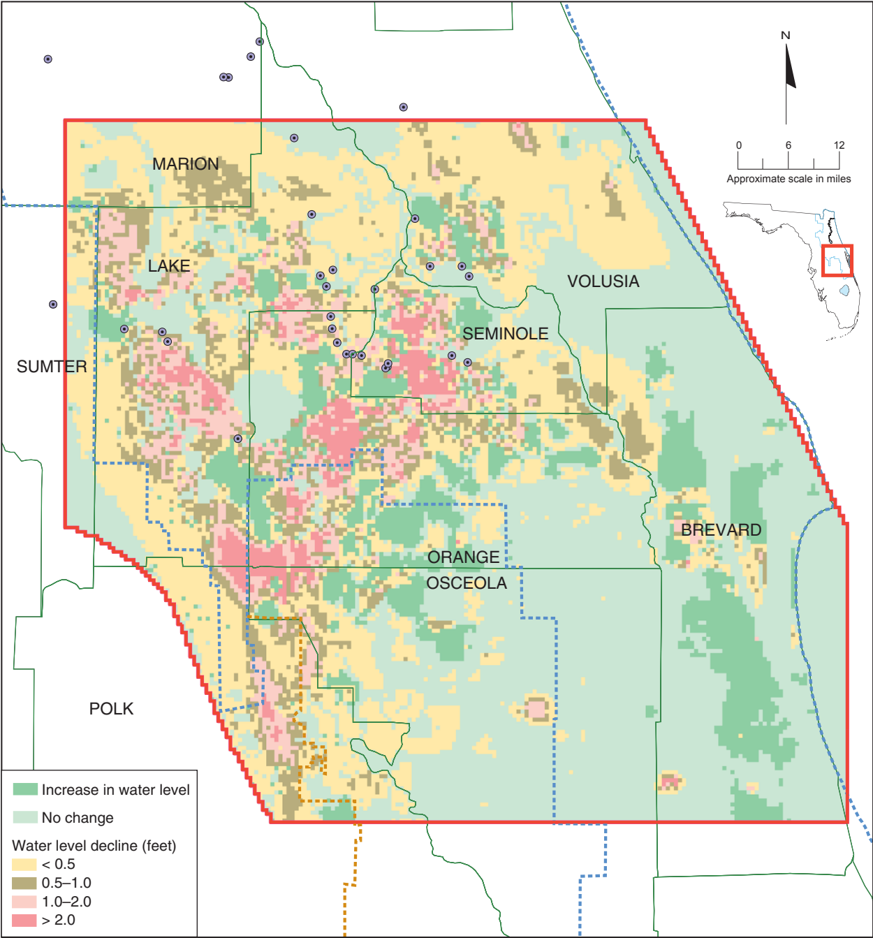
Figure 88. Predicted change in average surficial aquifer system water levels, 1995–2020
