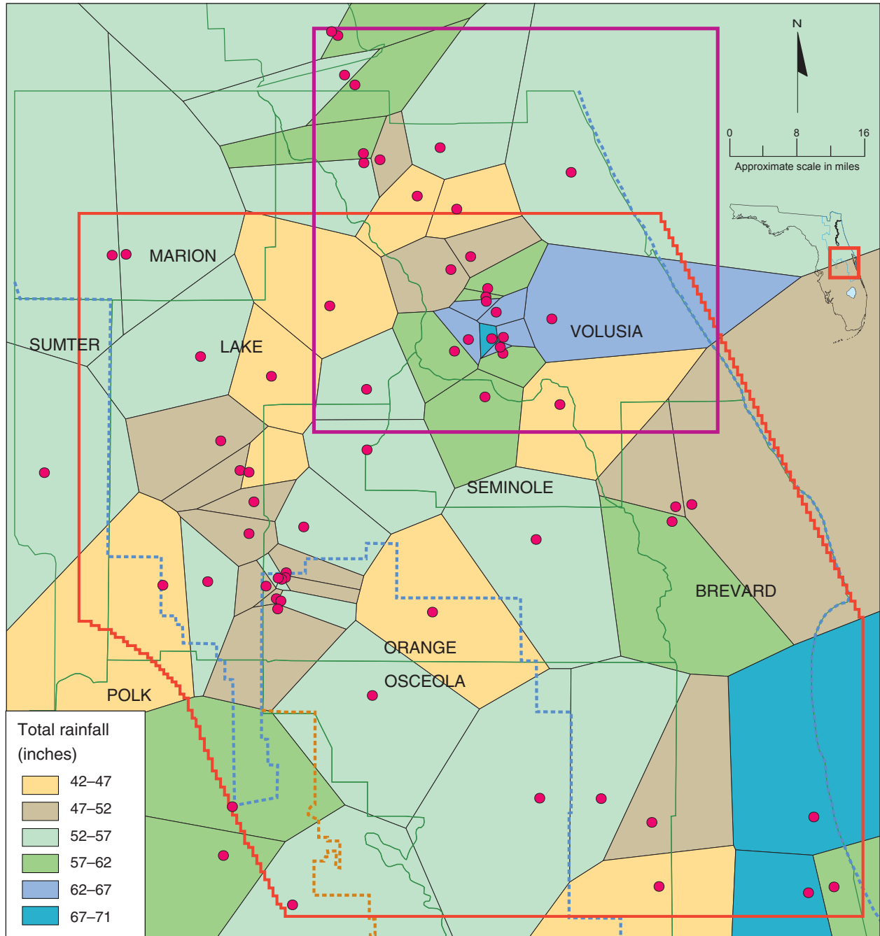
Figure 33. Theissen polygon distribution of total rainfall for 1995
