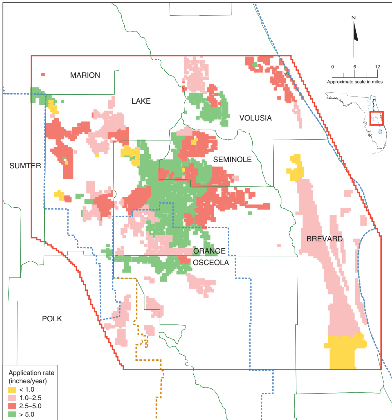
Figure 84. Average 2020 public-water supply landscape irrigation rates
