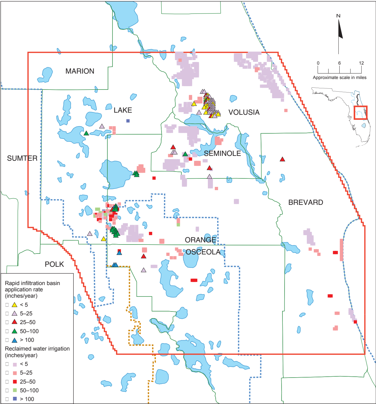
Figure 34. Average 1995 reclaimed water application rates
