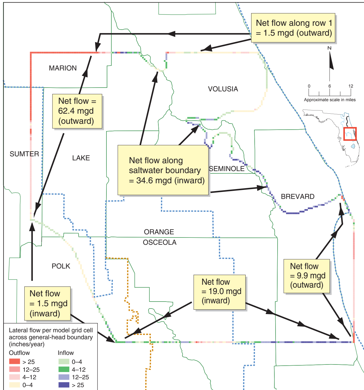
Figure 63. Simulated layer 3 (Upper Floridan aquifer—lower zone) lateral boundary flows, average 1995 conditions
