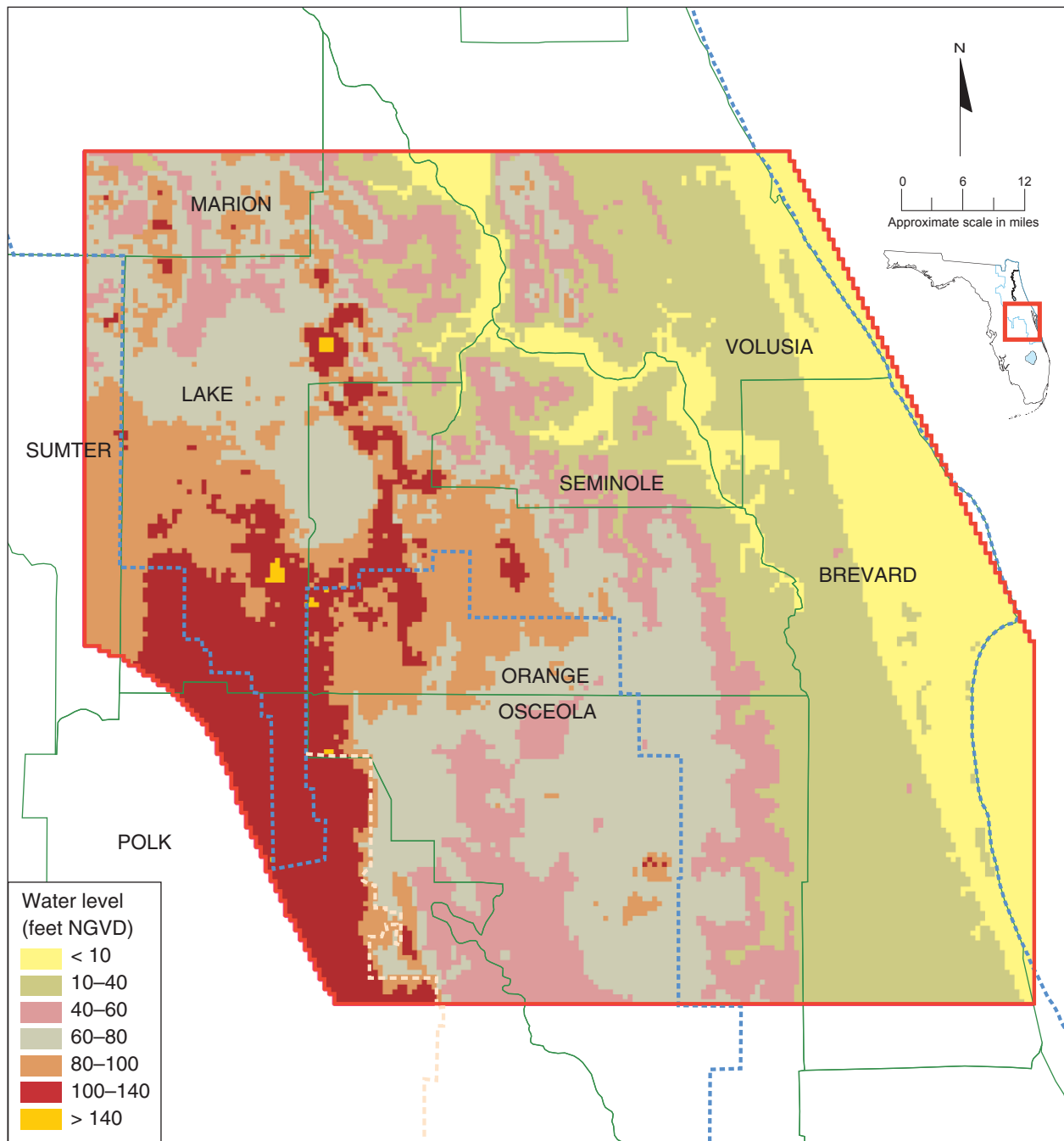
Figure 49. Simulated surficial aquifer system (layer 1) water levels for average 1995 conditions
