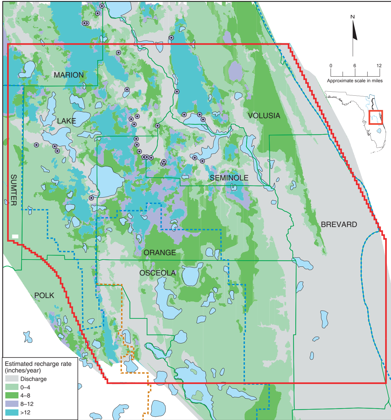
Figure 15. Areas of recharge to and discharge from the Floridan aquifer system (modified from Boniol et al. 1993)
