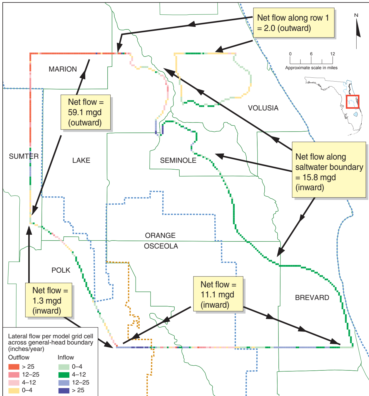
Figure 64. Simulated layer 4 (Lower Floridan aquifer) lateral boundary flows, average 1995 conditions
