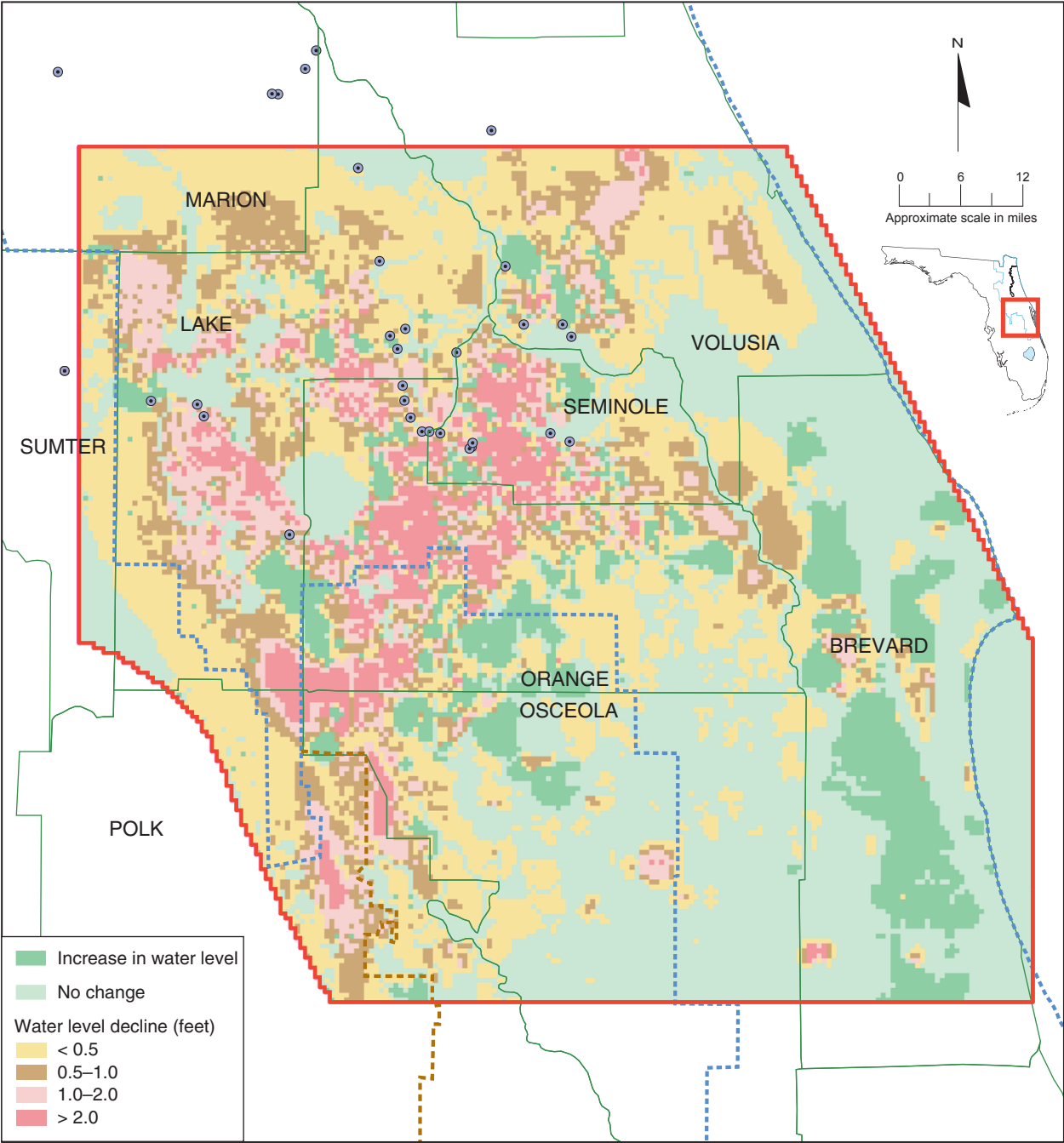
Figure 93. Predicted change in average surficial aquifer system water levels, 1995–2020, maximum drawdown simulation
