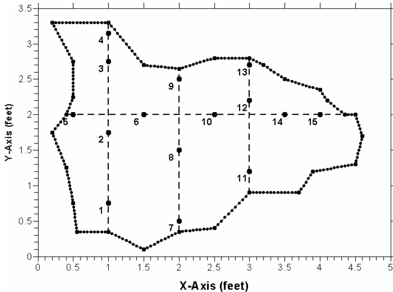
Figure 2A. Discharge measurement cross-section; Geyser Springs Group Vent A, Marion County, Florida, September 30, 2006 measurement. Cross-section is viewed to the upstream of observer, and is located at the 19 to 21-foot depth level. Velocity measurement stations are shown as numbered points. See Table 1 for station velocities. Boundary of cross section is shown as connected points. Support poles represented by dashed lines. X- and Y-axis scales are shown in feet.
