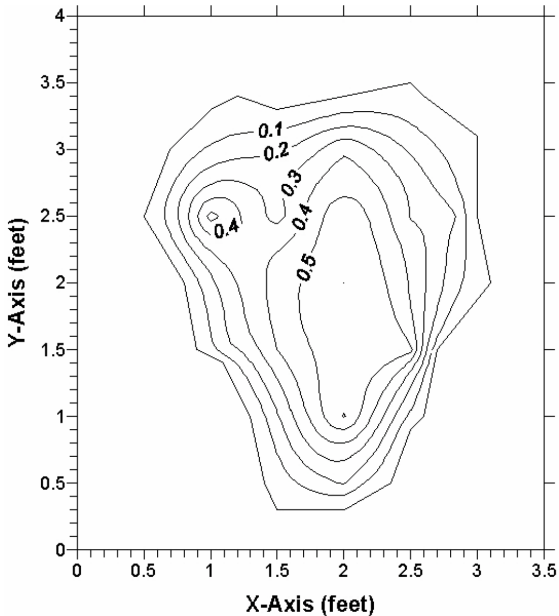
Figure 3BU. Discharge measurement cross-section; Geyser Springs Group Vent B Upper, Marion County, Florida, September 30, 2006 measurement. Flow contour velocities are shown in feet per second. Outer boundary of cross section represents the zero-value contour. X- and Y-axis scales are shown in feet.
