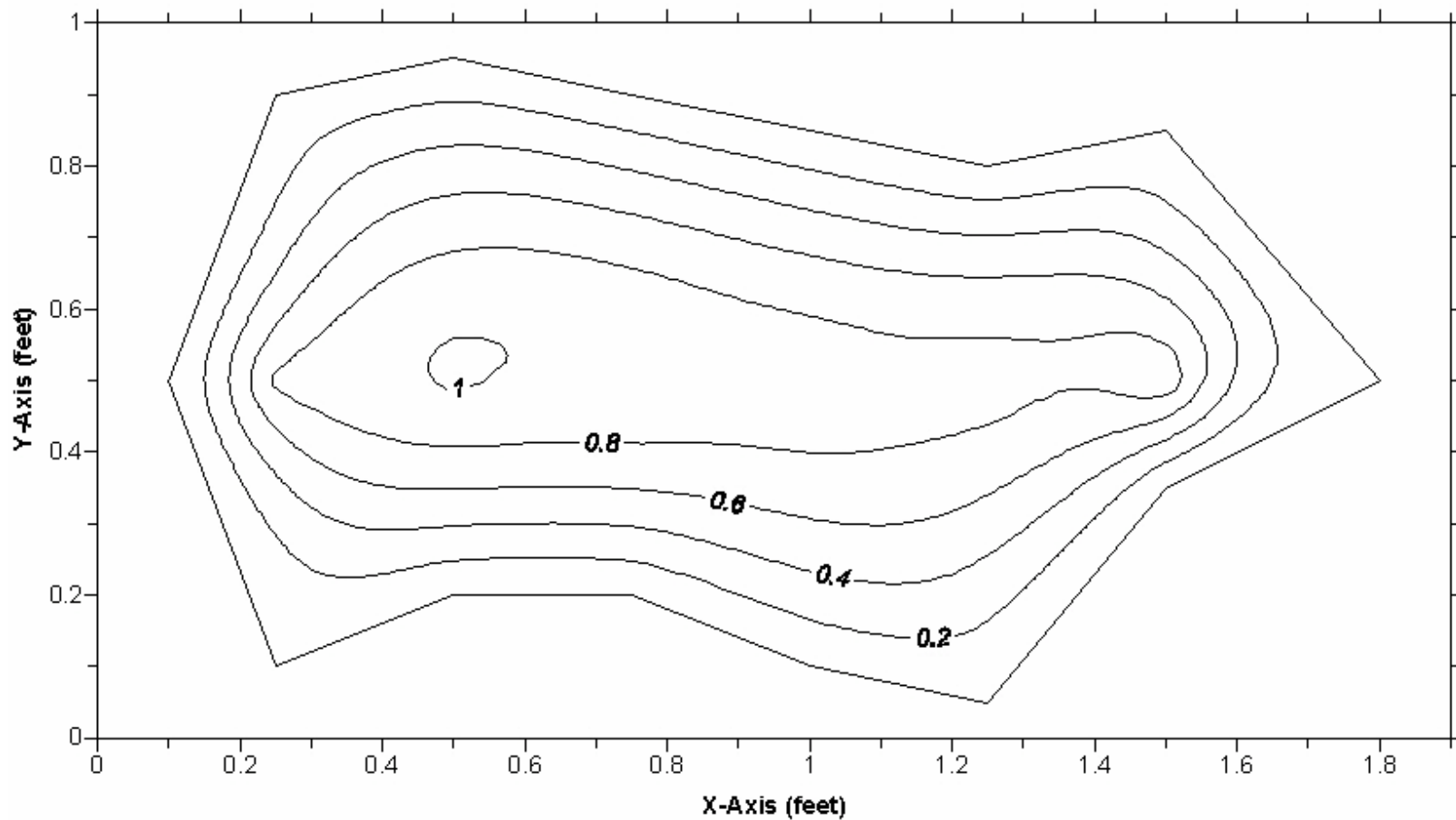
Figure 3B. Discharge measurement cross-section; Blue Grotto Spring Vent 2 (Back Vent), Marion County, Florida, September 29, 2006 measurement. Flow contour velocities are shown in feet per second. Outer boundary of cross section represents the zero-value contour. X- and Y-axis scales are shown in feet.
