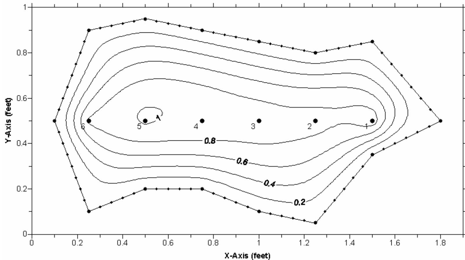
Figure 4B. Discharge measurement cross-section; Blue Grotto Spring Vent 2 (Back Vent), Marion County, Florida, September 29, 2006 measurement. Relationship of flow contours (velocities shown in feet per second) and velocity measurement stations (numbered points) are shown. Boundary of cross section is shown as connected points. X- and Y-axis scales are shown in feet.
