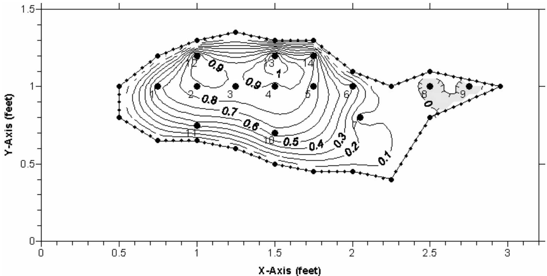
Figure 4. Discharge measurement cross-section; Second Fisherman's Paradise Spring, Marion County, Florida, September 22, 2006 measurement. Relationship of flow contours (velocities shown in feet per second) and velocity measurement stations (numbered points) are shown. Areas with negative velocities (reverse flow) are shaded and delineated by hatched lines. See Table 1 for station velocities. Boundary of cross section is shown as connected points. X- and Y-axis scales are shown in feet.
