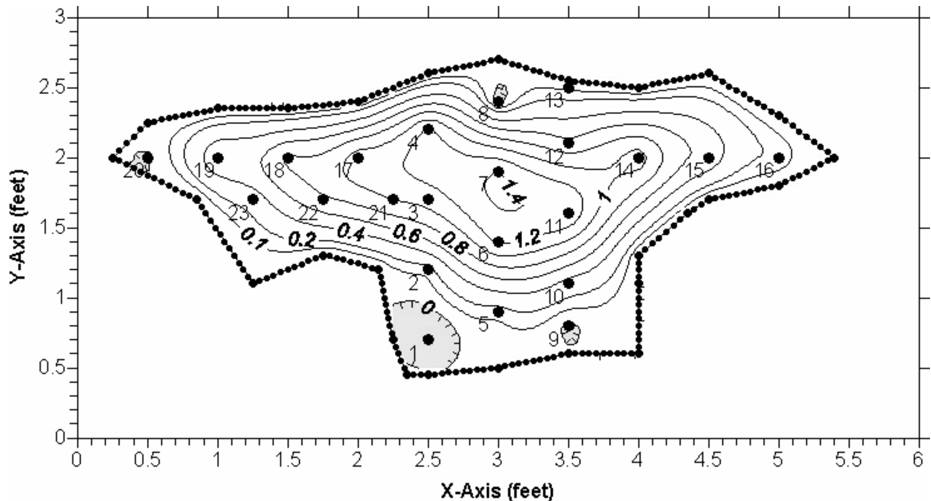
Figure 4A. Discharge measurement cross-section; Ladies Parlor Spring North Vent, Marion County, Florida, September 22, 2006 measurement. Relationship of flow contours (velocities shown in feet per second) and velocity measurement stations (numbered points) are shown. Areas with negative velocities (reverse flow) are shaded and delineated by hatched lines. See Table 1 for station velocities. Boundary of cross section is shown as connected points. X- and Y-axis scales are shown in feet.
