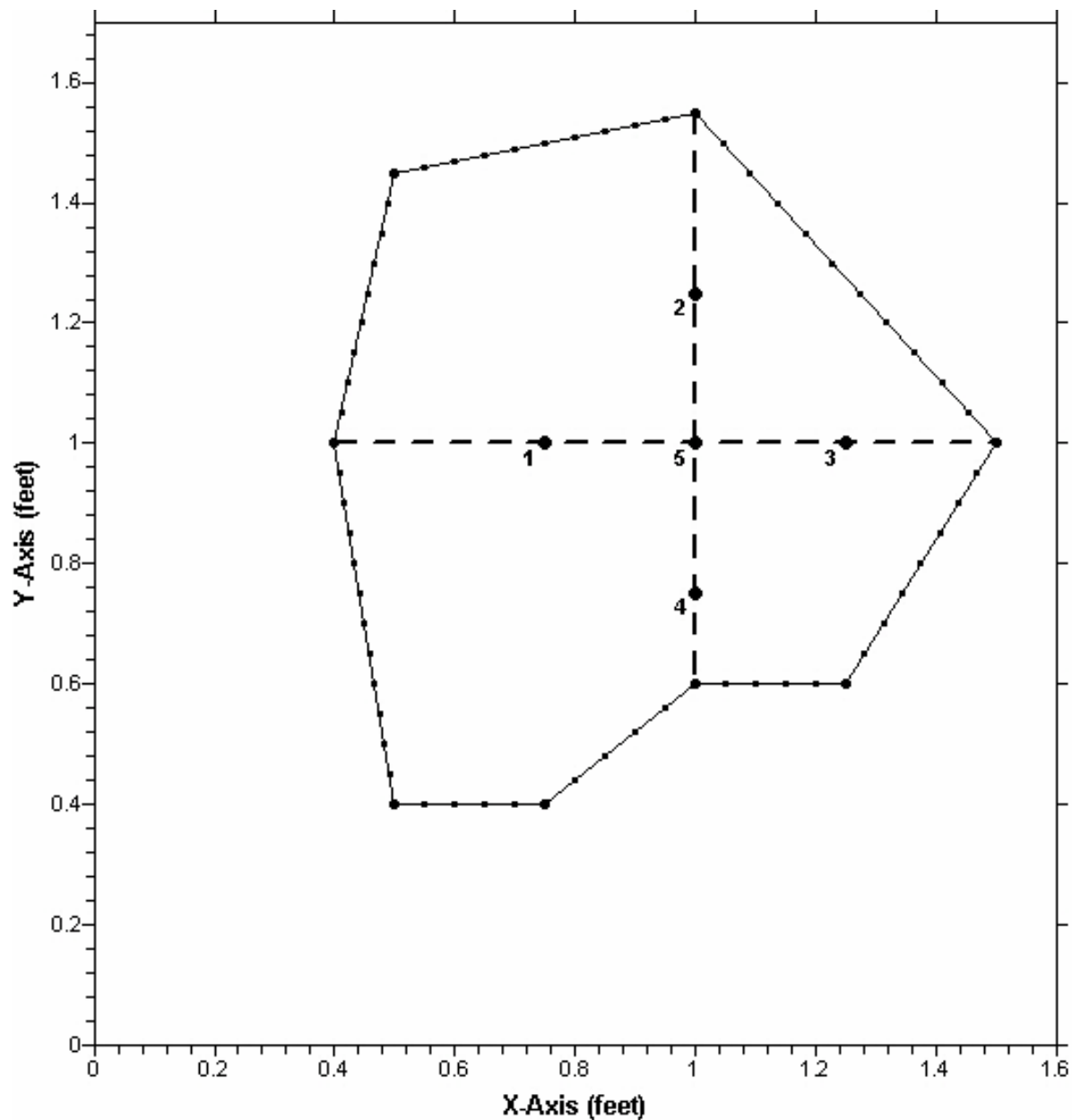
Figure 2C. Discharge measurement cross-section; Geyser Springs Group Vent C, Marion County, Florida, September 30, 2006 measurement. Cross-section is viewed to the upstream of observer, and is located at the 20-foot depth level. Velocity measurement stations are shown as numbered points. See Table 1 for station velocities. Boundary of cross section is shown as connected points. Support poles represented by dashed lines. X- and Y-axis scales are shown in feet.
