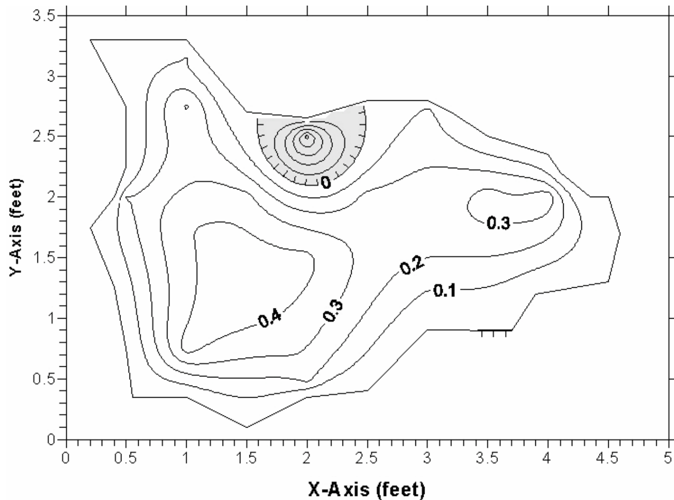
Figure 3A. Discharge measurement cross-section; Geyser Springs Group Vent A, Marion County, Florida, September 30, 2006 measurement. Flow contour velocities are shown in feet per second. Areas with negative velocities (reverse flow) are shaded and delineated by hatched lines. Outer boundary of cross section represents the zero-value contour. X- and Y-axis scales are shown in feet.
