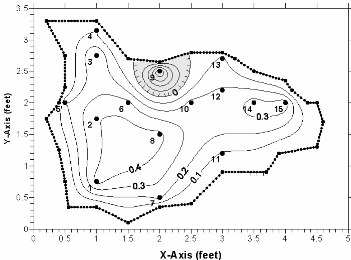
Figure 4A. Discharge measurement cross-section; Geyser Springs Group Vent A, Marion County, Florida, September 30, 2006 measurement. Relationship of flow contours (velocities shown in feet per second) and velocity measurement stations (numbered points) are shown. Areas with negative velocities (reverse flow) are shaded and delineated by hatched lines. See Table 1 for station velocities. Boundary of cross section is shown as connected points. X- and Y-axis scales are shown in feet.
