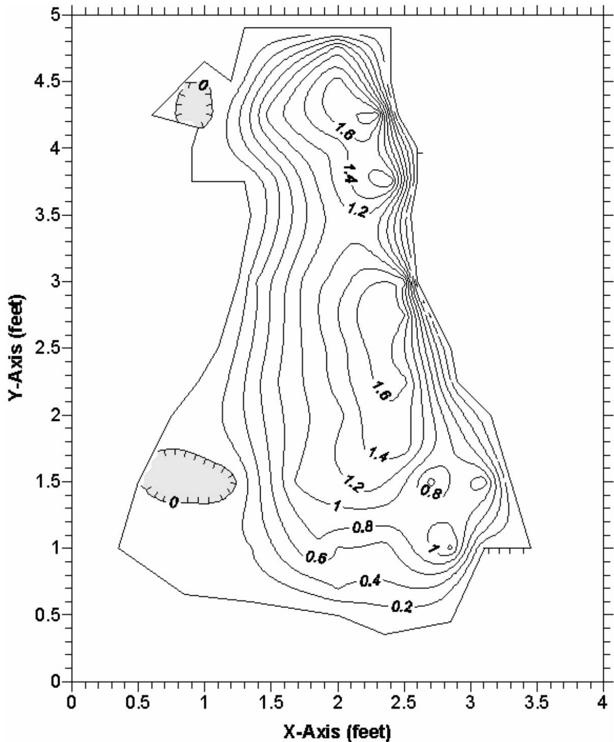
Figure 3A. Discharge measurement cross-section; Blue Grotto Spring Vent 1 (Main Vent), Marion County, Florida, September 29, 2006 measurement. Flow contour velocities are shown in feet per second. Areas with negative velocities (reverse flow) are shaded and delineated by hatched lines. Outer boundary of cross section represents the zero-value contour. X- and Y-axis scales are shown in feet.
