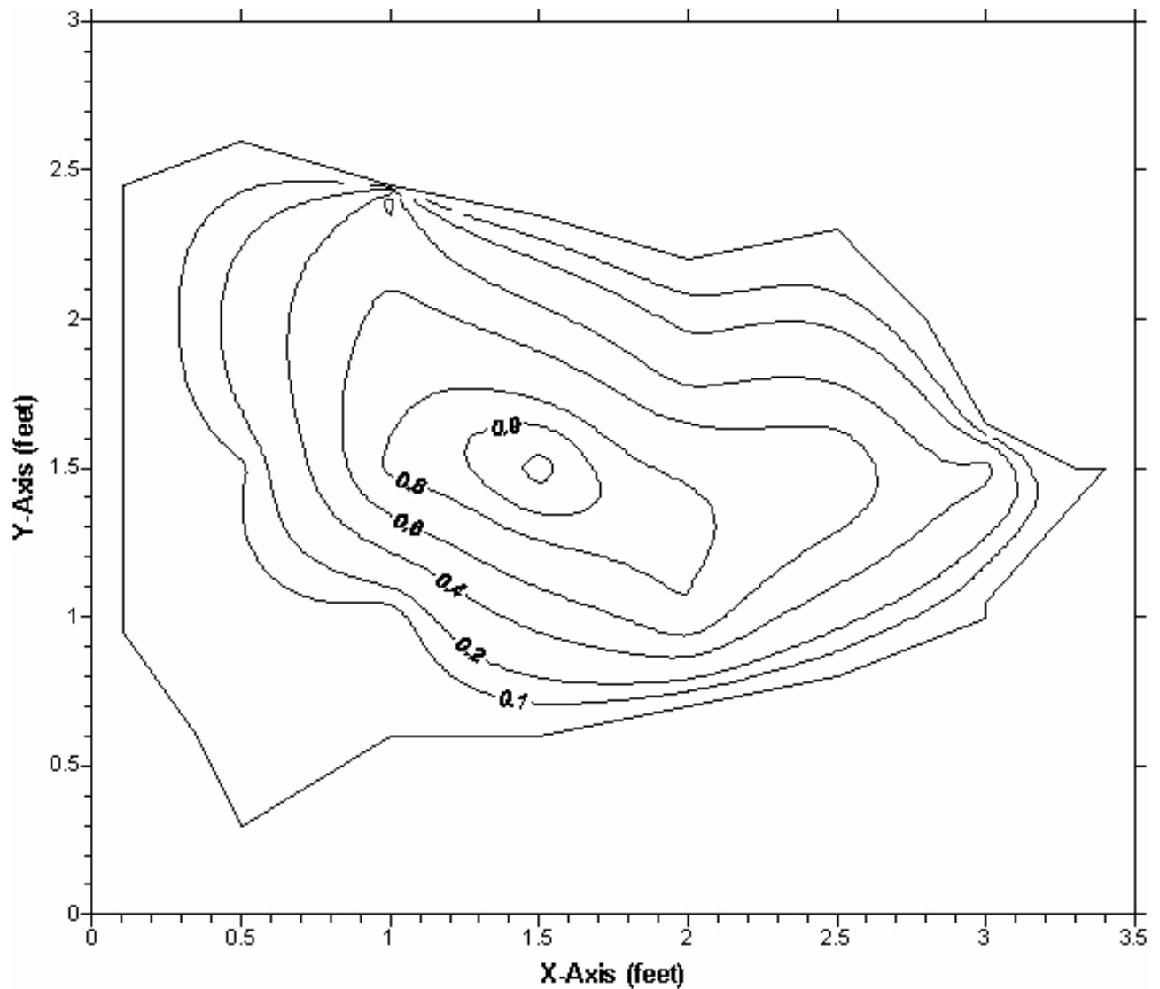
Figure 3D. Discharge measurement cross-section; Geyser Springs Group Vent D, Marion County, Florida, September 30, 2006 measurement. Flow contour velocities are shown in feet per second. Outer boundary of cross section represents the zero-value contour. X- and Y-axis scales are shown in feet.
