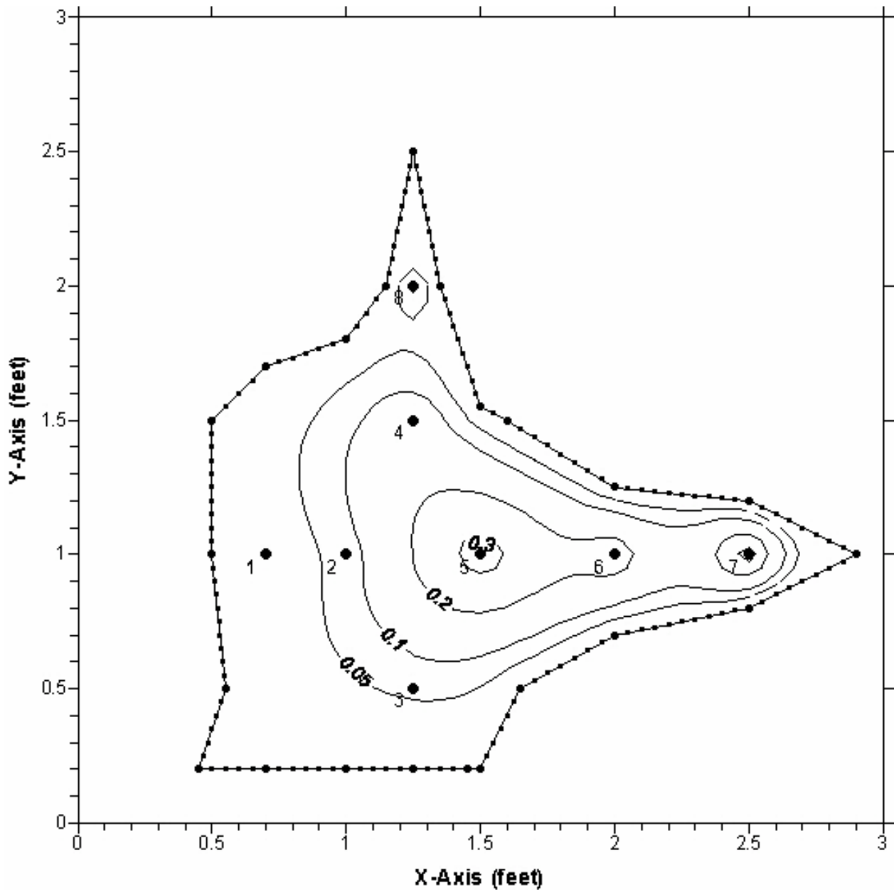
Figure 4BL. Discharge measurement cross-section; Geyser Springs Group Vent B Lower, Marion County, Florida, September 30, 2006 measurement. Relationship of flow contours (velocities shown in feet per second) and velocity measurement stations (numbered points) are shown. Boundary of cross section is shown as connected points. X- and Y-axis scales are shown in feet.
