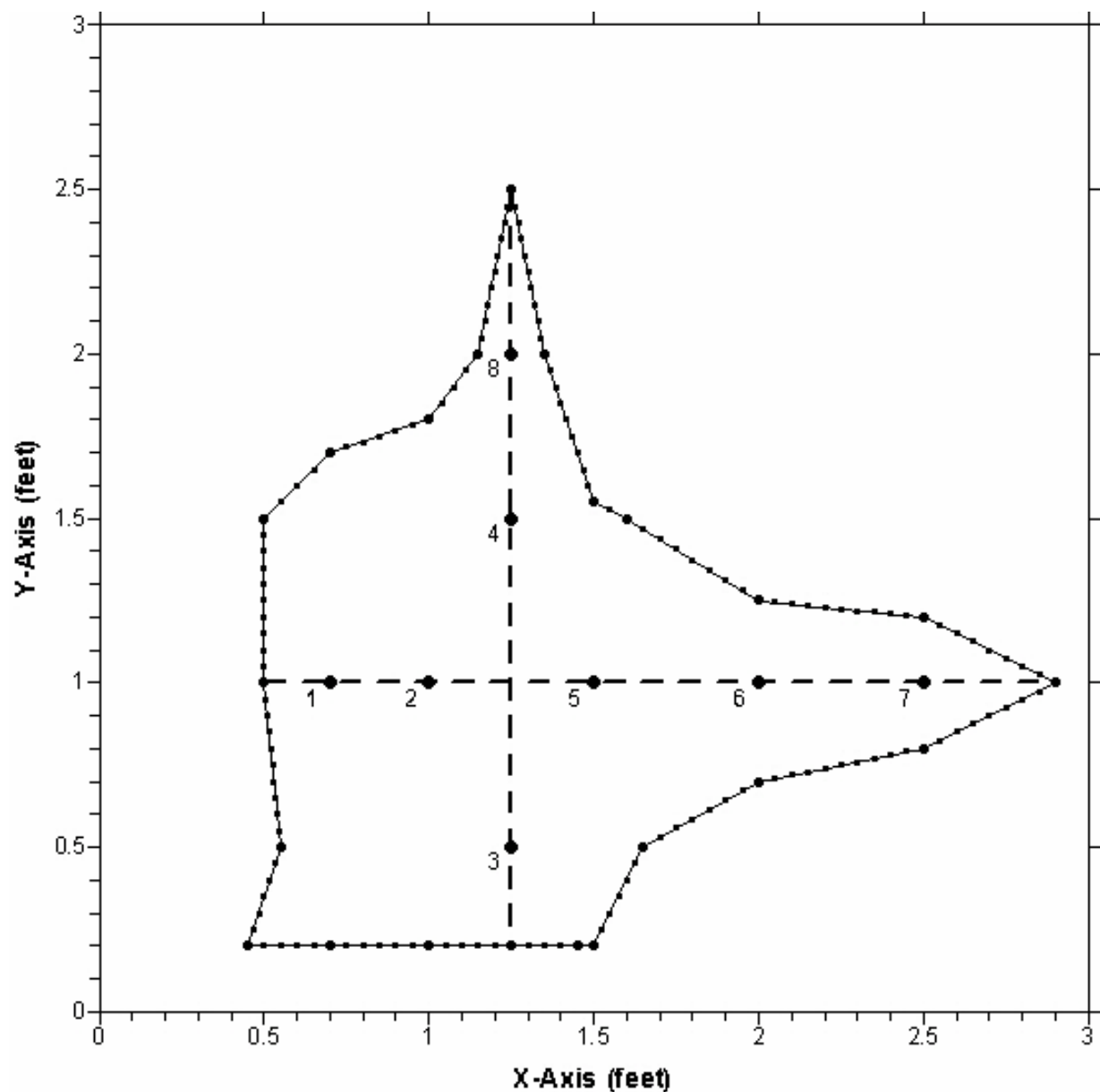
Figure 2BL. Discharge measurement cross-section; Geyser Springs Group Vent B Lower, Marion County, Florida, September 30, 2006 measurement. Cross-section is viewed to the upstream of observer, and is located at the 19-foot depth level. Velocity measurement stations are shown as numbered points. See Table 1 for station velocities. Boundary of cross section is shown as connected points. Support poles represented by dashed lines. X- and Y-axis scales are shown in feet.
