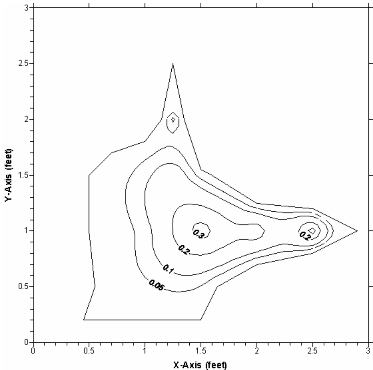
Figure 3BL. Discharge measurement cross-section; Geyser Springs Group Vent B Lower, Marion County, Florida, September 30, 2006 measurement. Flow contour velocities are shown in feet per second. Outer boundary of cross section represents the zero-value contour. X- and Y-axis scales are shown in feet.
