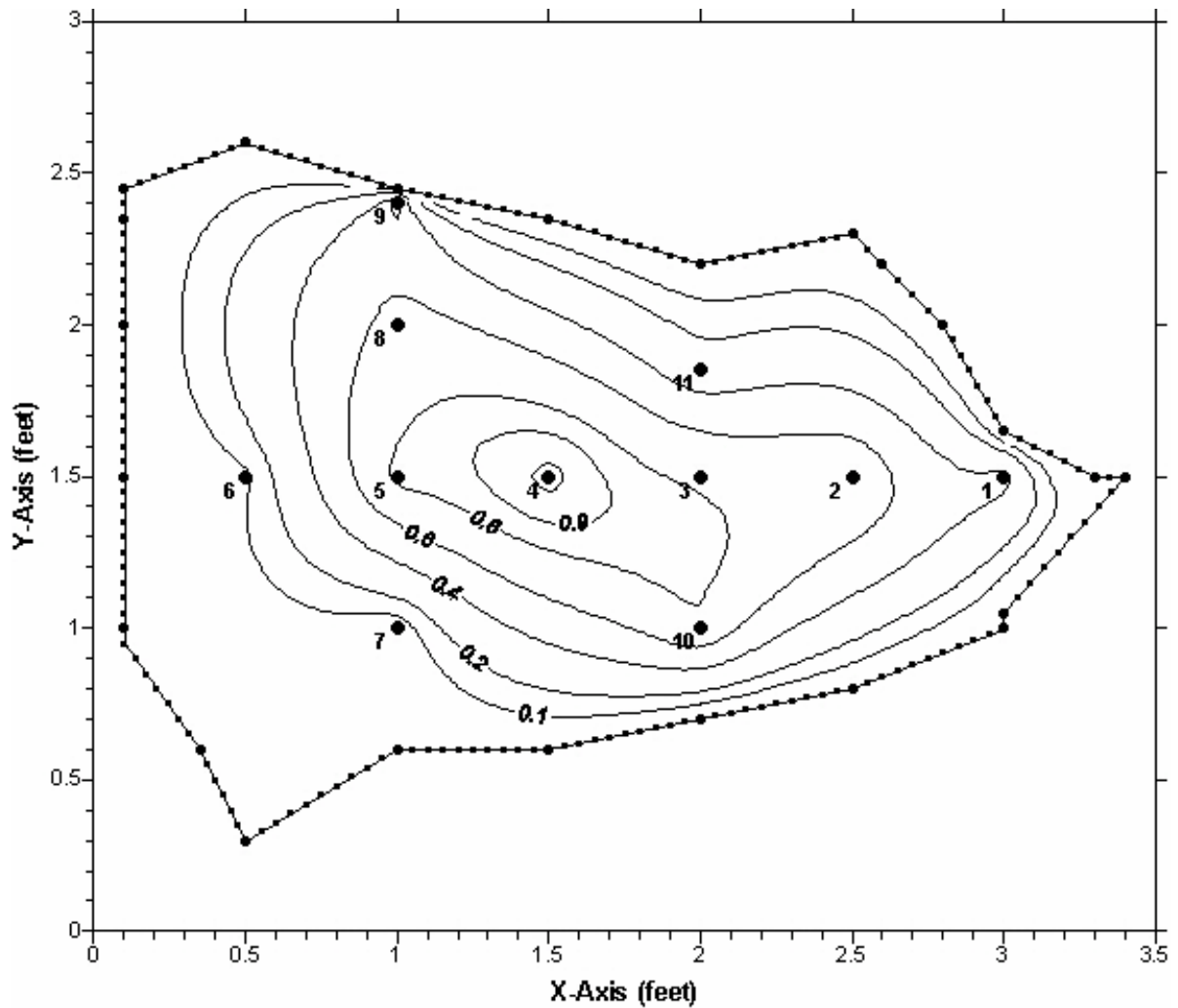
Figure 4D. Discharge measurement cross-section; Geyser Springs Group Vent D, Marion County, Florida, September 30, 2006 measurement. Relationship of flow contours (velocities shown in feet per second) and velocity measurement stations (numbered points) are shown. Boundary of cross section is shown as connected points. X- and Y-axis scales are shown in feet.
