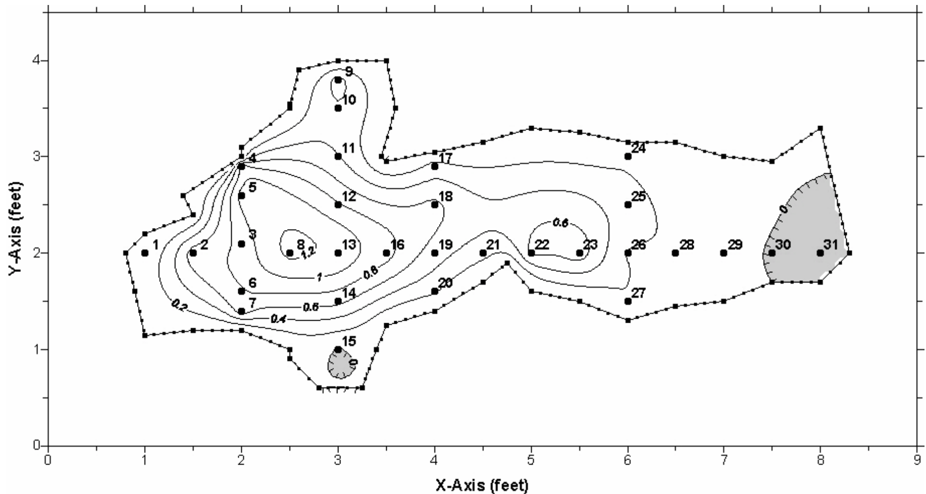
Figure 4. Discharge measurement cross-section; Bridal Chamber Spring, Marion County, Florida, September 22, 2006 measurement. Relationship of flow contours (velocities shown in feet per second) and velocity measurement stations (numbered points) are shown. Areas with negative velocities (reverse flow) are shaded and delineated by hatched lines. See Table 1 for station velocities. Boundary of cross section is shown as connected points. X- and Y-axis scales are shown in feet.
