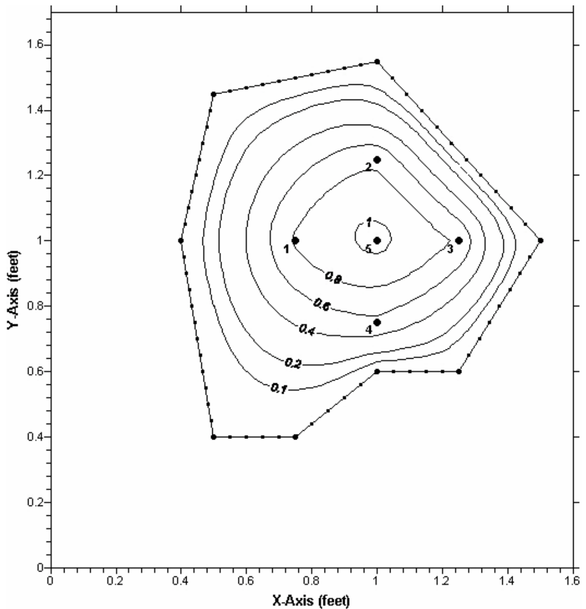
Figure 4C. Discharge measurement cross-section; Geyser Springs Group Vent C, Marion County, Florida, September 30, 2006 measurement. Relationship of flow contours (velocities shown in feet per second) and velocity measurement stations (numbered points) are shown. Boundary of cross section is shown as connected points. X- and Y-axis scales are shown in feet.
