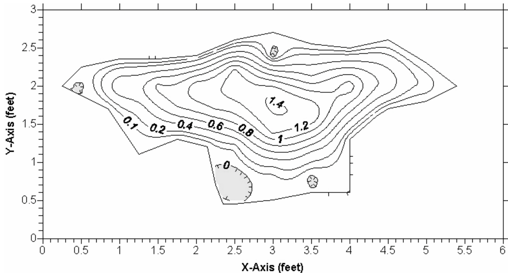
Figure 3A. Discharge measurement cross-section; Ladies Parlor Spring North Vent, Marion County, Florida, September 22, 2006 measurement. Flow contour velocities are shown in feet per second. Areas with negative velocities (reverse flow) are shaded and delineated by hatched lines. Outer boundary of cross section represents the zero-value contour. X- and Y-axis scales are shown in feet.
