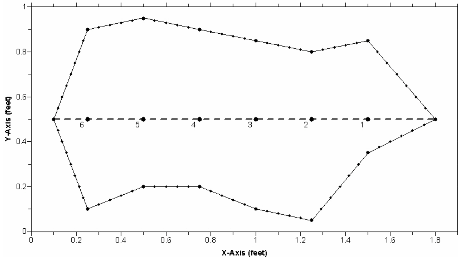
Figure 2B. Discharge measurement cross-section; Blue Grotto Spring Vent 2 (Back Vent), Marion County, Florida, September 29, 2006 measurement. Cross-section is viewed to the upstream of observer, and is located at the 21-foot depth level. Velocity measurement stations are shown as numbered points. See Table 1 for station velocities. Boundary of cross section is shown as connected points. Support poles represented by dashed lines. X- and Y-axis scales are shown in feet.
