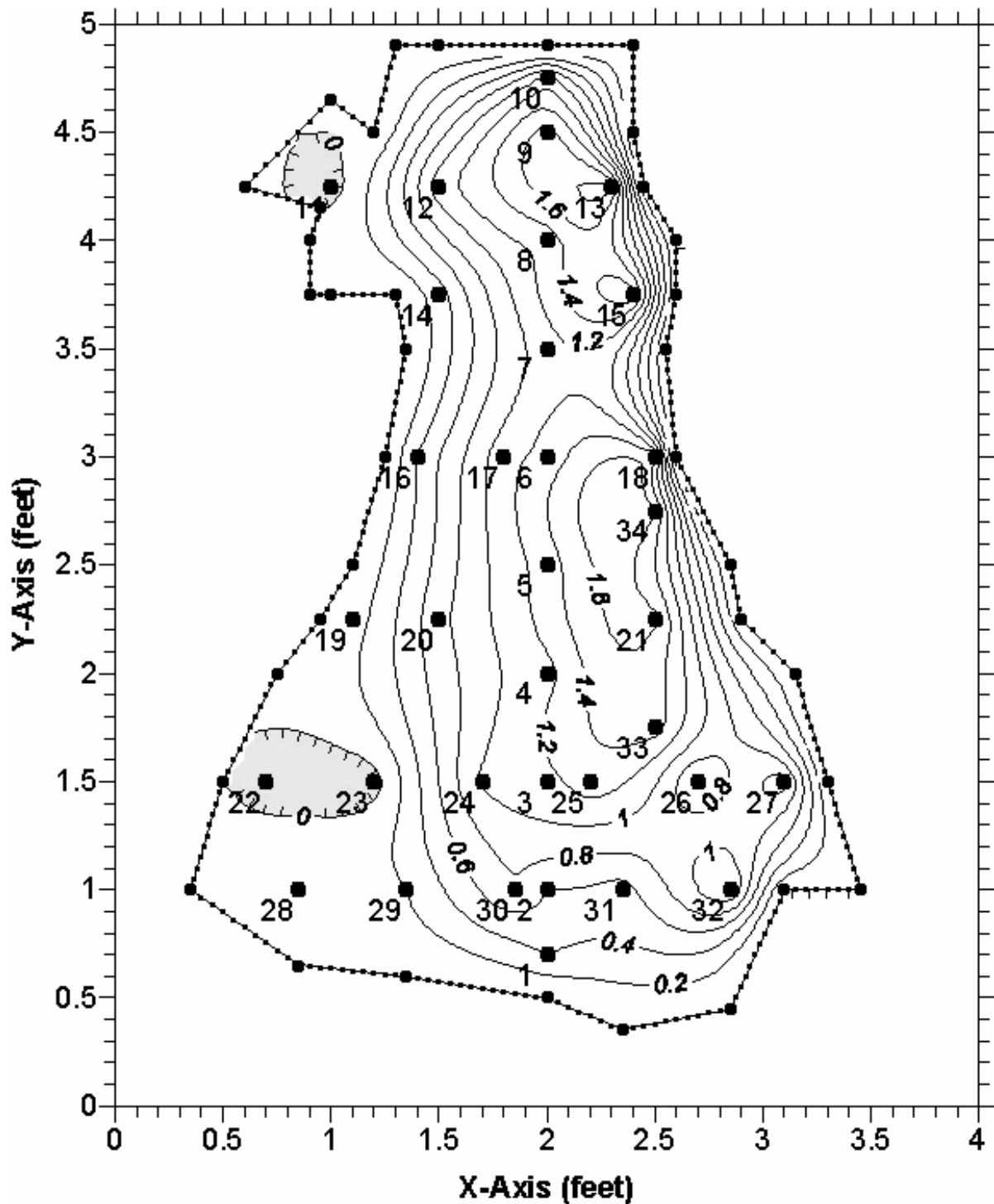
Figure 4A. Discharge measurement cross-section; Blue Grotto Spring Vent 1 (Main Vent), Marion County, Florida, September 29, 2006 measurement. Relationship of flow contours (velocities shown in feet per second) and velocity measurement stations (numbered points) are shown. Areas with negative velocities (reverse flow) are shaded and delineated by hatched lines. See Table 1 for station velocities. Boundary of cross section is shown as connected points. X- and Y-axis scales are shown in feet.
