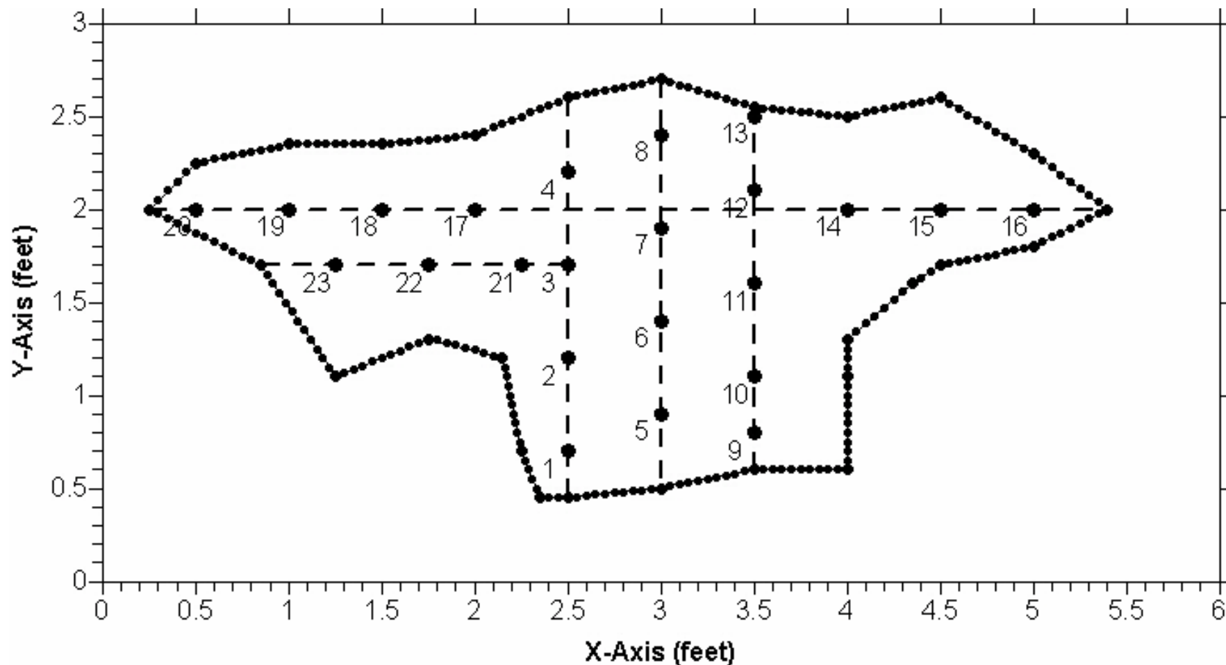
Figure 2A. Discharge measurement cross-section; Ladies Parlor Spring North Vent, Marion County, Florida, September 22, 2006 measurement. Cross-section is viewed to the upstream of observer, and is located at the 20 to 22-foot depth level. Velocity measurement stations are shown as numbered points. See Table 1 for station velocities. Boundary of cross section is shown as connected points. Support poles represented by dashed lines. X- and Y-axis scales are shown in feet.
