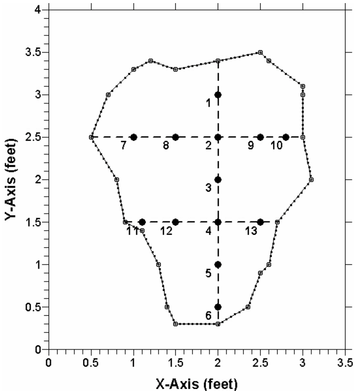
Figure 2BU. Discharge measurement cross-section; Geyser Springs Group Vent B Upper, Marion County, Florida, September 30, 2006 measurement. Cross-section is viewed to the upstream of observer, and is located at the 18 to 20-foot depth level. Velocity measurement stations are shown as numbered points. See Table 1 for station velocities. Boundary of cross section is shown as connected points. Support poles represented by dashed lines. X- and Y-axis scales are shown in feet.
