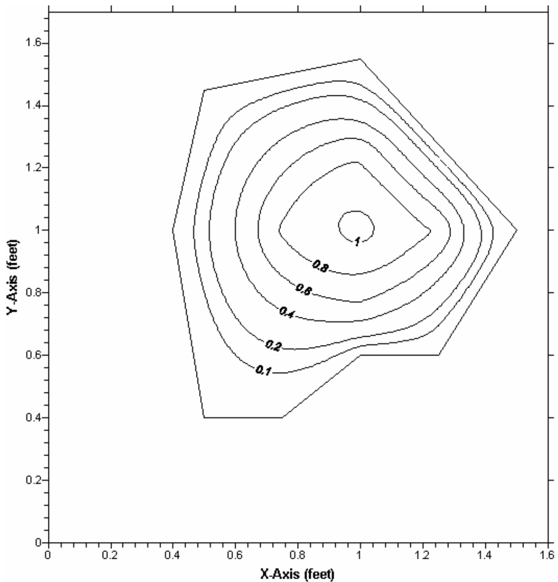
Figure 3C. Discharge measurement cross-section; Geyser Springs Group Vent C, Marion County, Florida, September 30, 2006 measurement. Flow contour velocities are shown in feet per second. Outer boundary of cross section represents the zero-value contour. X- and Y-axis scales are shown in feet.
