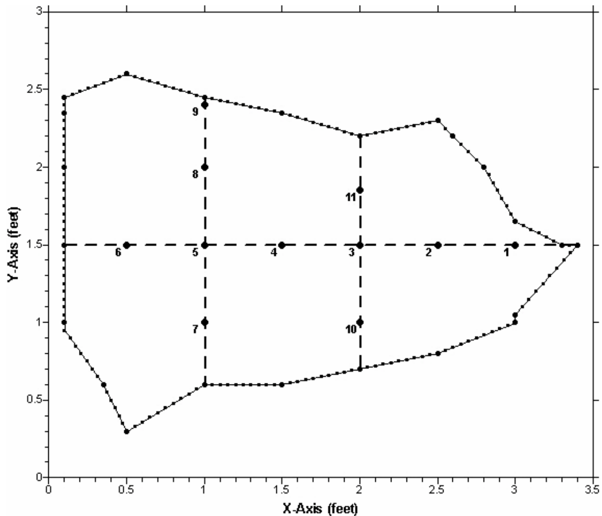
Figure 2D. Discharge measurement cross-section; Geyser Springs Group Vent D, Marion County, Florida, September 30, 2006 measurement. Cross-section is viewed to the upstream of observer, and is located at the 20 to 21-foot depth level. Velocity measurement stations are shown as numbered points. See Table 1 for station velocities. Boundary of cross section is shown as connected points. Support poles represented by dashed lines. X- and Y-axis scales are shown in feet.
