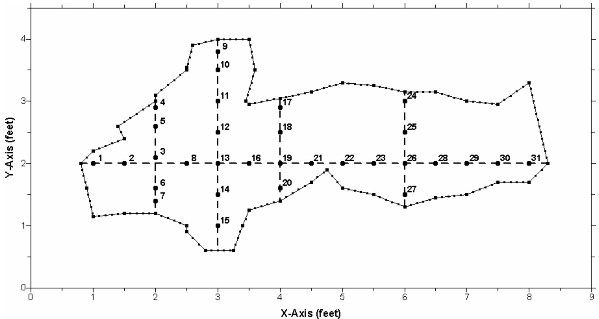
Figure 2. Discharge measurement cross-section; Bridal Chamber Spring, Marion County, Florida, September 22, 2006 measurement. Cross-section is viewed to the upstream of observer, and is located at the 25-foot depth level. Velocity measurement stations are shown as numbered points. See Table 1 for station velocities. Boundary of cross section is shown as connected points. Support poles represented by dashed lines. X- and Y-axis scales are shown in feet.
