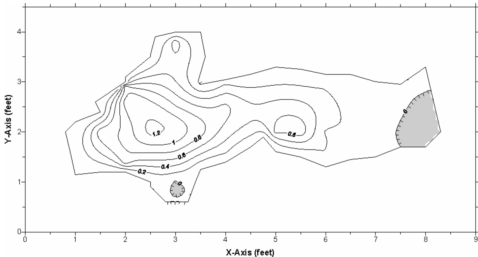
Figure 3. Discharge measurement cross-section; Bridal Chamber Spring, Marion County, Florida, September 22, 2006 measurement. Flow contour velocities are shown in feet per second. Areas with negative velocities (reverse flow) are shaded and delineated by hatched lines. Outer boundary of cross section represents the zero-value contour. X- and Y-axis scales are shown in feet.
