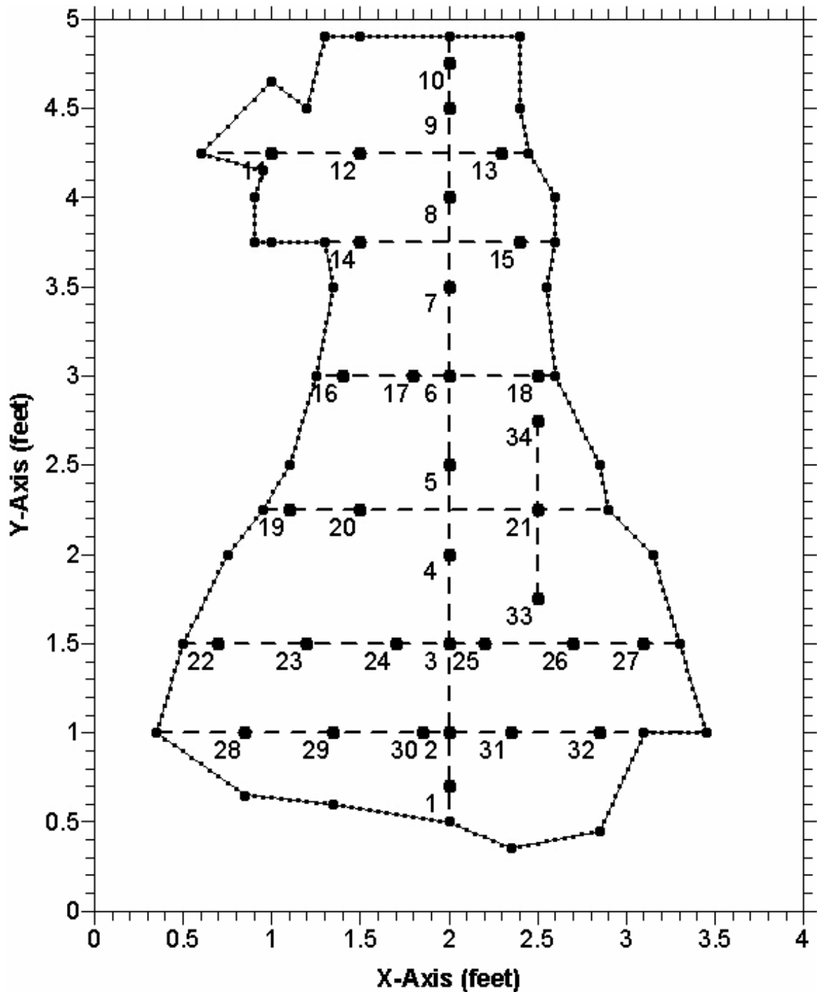
Figure 2A. Discharge measurement cross-section; Blue Grotto Spring Vent 1 (Main Vent), Marion County, Florida, September 29, 2006 measurement. Cross-section is viewed to the upstream of observer, and is located at the 24 to 26-foot depth level. Velocity measurement stations are shown as numbered points. See Table 1 for station velocities. Boundary of cross section is shown as connected points. Support poles represented by dashed lines. X- and Y-axis scales are shown in feet.
