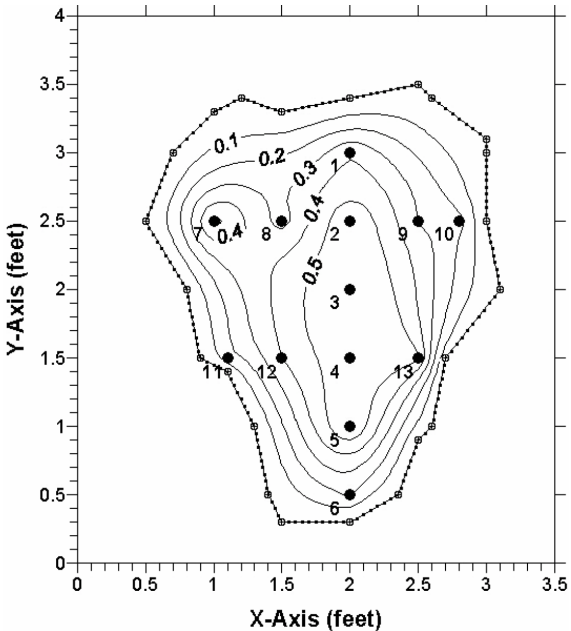
Figure 4BU. Discharge measurement cross-section; Geyser Springs Group Vent B Upper, Marion County, Florida, September 30, 2006 measurement. Relationship of flow contours (velocities shown in feet per second) and velocity measurement stations (numbered points) are shown. Boundary of cross section is shown as connected points. X- and Y-axis scales are shown in feet.
