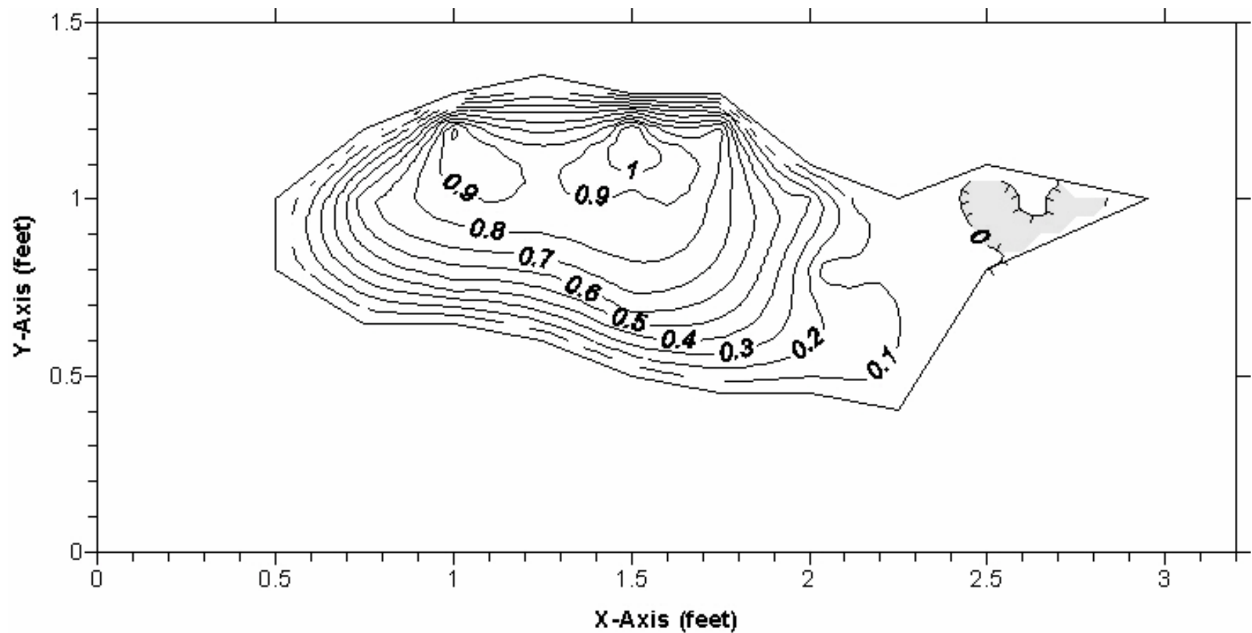
Figure 3. Discharge measurement cross-section; Second Fisherman's Paradise Spring, Marion County, Florida, September 22, 2006 measurement. Flow contour velocities are shown in feet per second. Areas with negative velocities (reverse flow) are shaded and delineated by hatched lines. Outer boundary of cross section represents the zero-value contour. X- and Y-axis scales are shown in feet.
