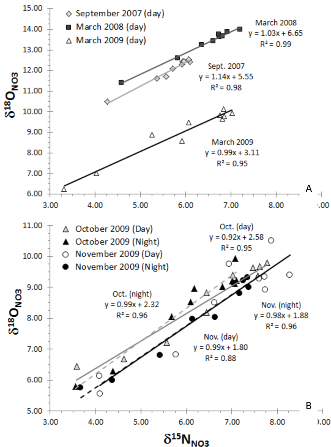
Fig. 5-4. Dual isotope coupling (slope of \delta^{15}\text{N} vs. \delta^{18}\text{O} ) from longitudinal transects (5 day – solid lines and 2 night – dashed lines).
