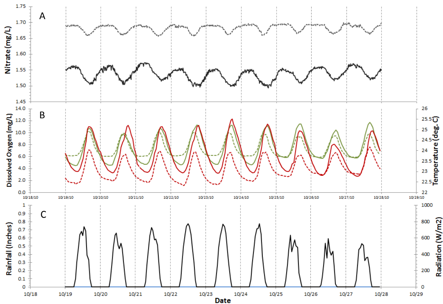
Fig. 2-33 - Diel variation in nitrate (solid grey line – downstream, dashed grey line - upstream), dissolved oxygen (solid green line – downstream, dashed green line – upstream), water temperature (solid red line – downstream, dashed red line – upstream), radiation (black line) and rainfall (blue line) for Rainbow River during an October 2010 deployment. Vertical dashed lines are at midnight every 24 hours.
