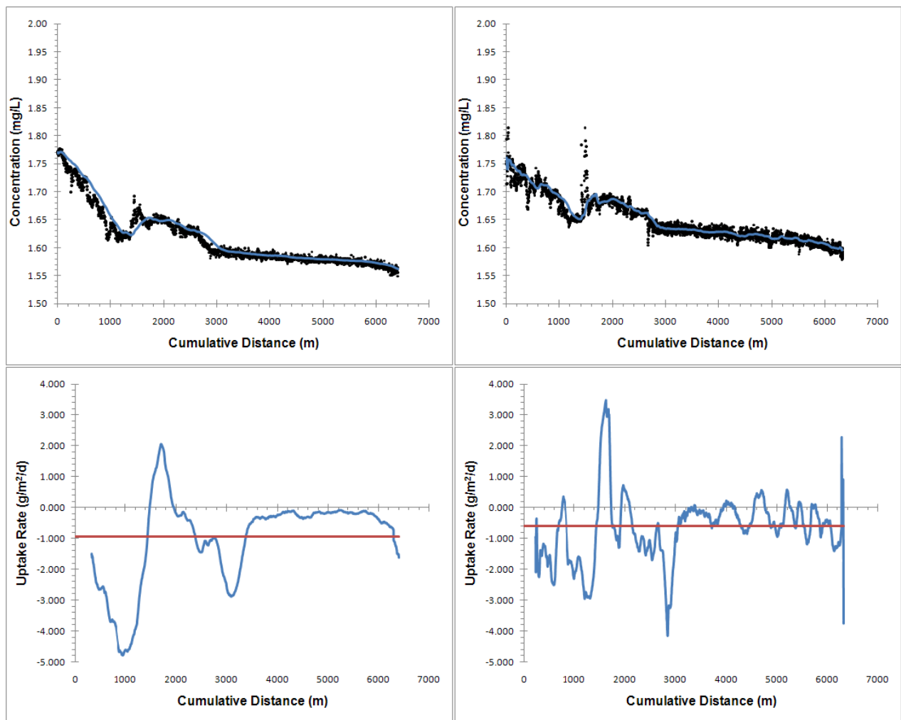
Figure 3-15. Longitudinal nitrate concentration profile (Top) and loss rate profile (Bottom) for Rainbow River on October 18, 2010 (Left) and October 28, 2010 (Right).
