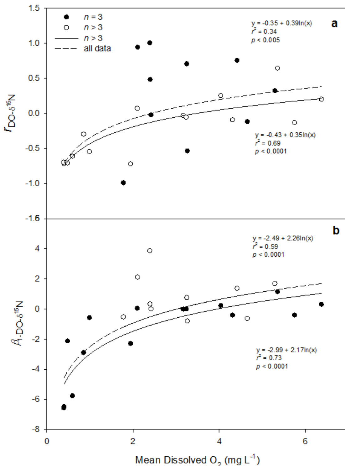
Figure 6-6. Parameters of within-spring relationships between dissolved \text{O}_2 and \delta^{15}\text{N}_{\text{NO}_3} as a function of spring mean dissolved oxygen. Large negative values of both (a) correlation coefficient and (b) slope in low- \text{O}_2 springs, and their absence in higher- \text{O}_2 systems, suggest that isotopically-enriched nitrate pools are associated with old, deeply anoxic flowpaths where denitrification would be most likely to occur. Open symbols indicate springs with 3 observations of \text{O}_2 and \delta^{15}\text{N}_{\text{NO}_3} . Closed symbols indicated springs with 4 or more observations.
