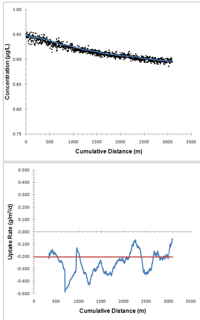
Figure 3-20. Longitudinal nitrate concentration profile (Top) and loss rate profile (Bottom) for Weeki Wachee River on January 27, 2011.
