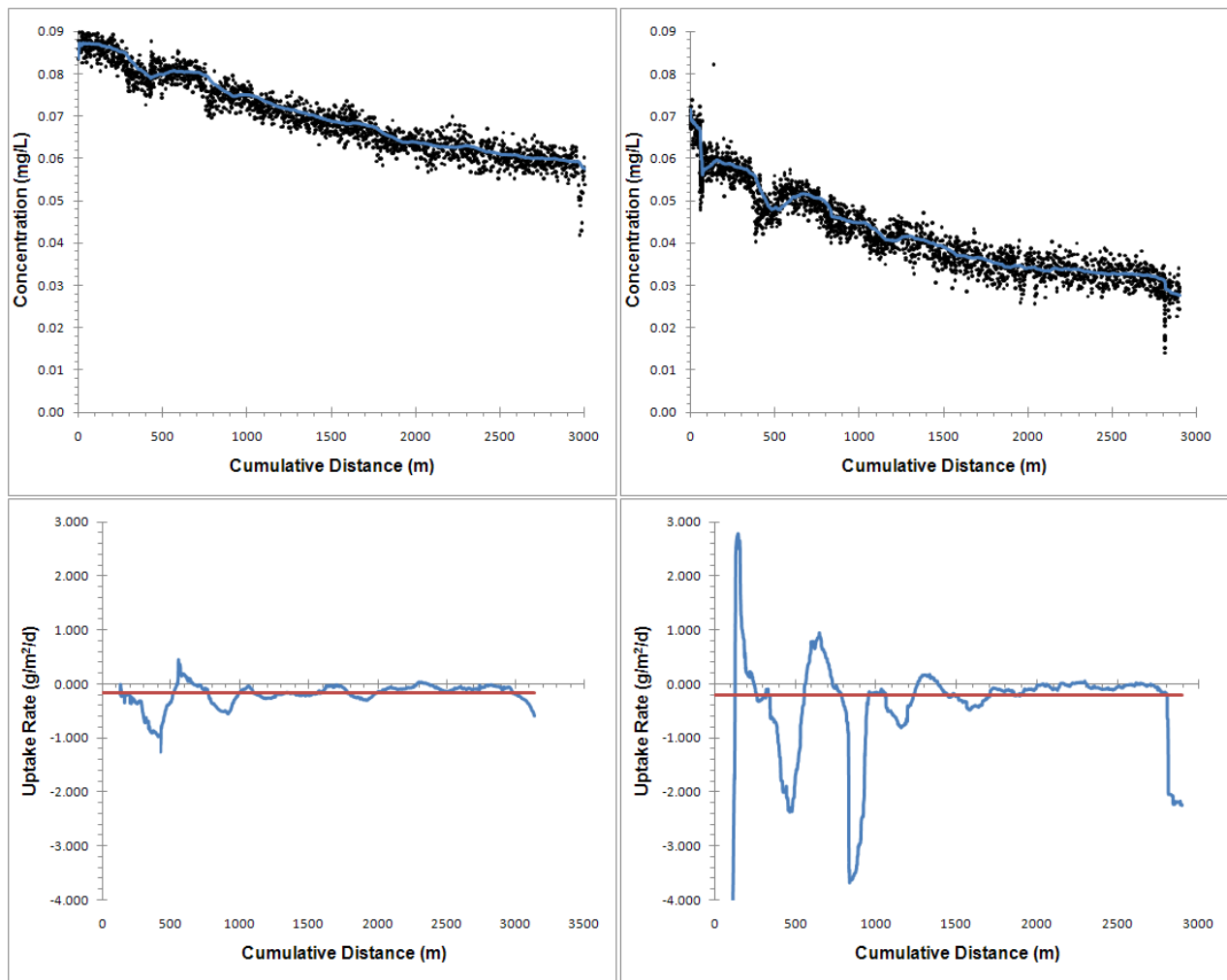
Figure 3-14. Longitudinal nitrate concentration profile (Top) and loss rate profile (Bottom) for Juniper Creek on November 10, 2010 (Left) and November 22, 2010 (Right).
