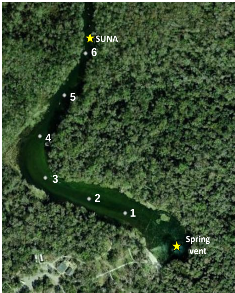
Fig. 7-1. Location of the spring vent, sampling sites (1 through 6) and the continuous nitrate sensor (SUNA) at Alexander Springs Creek.
