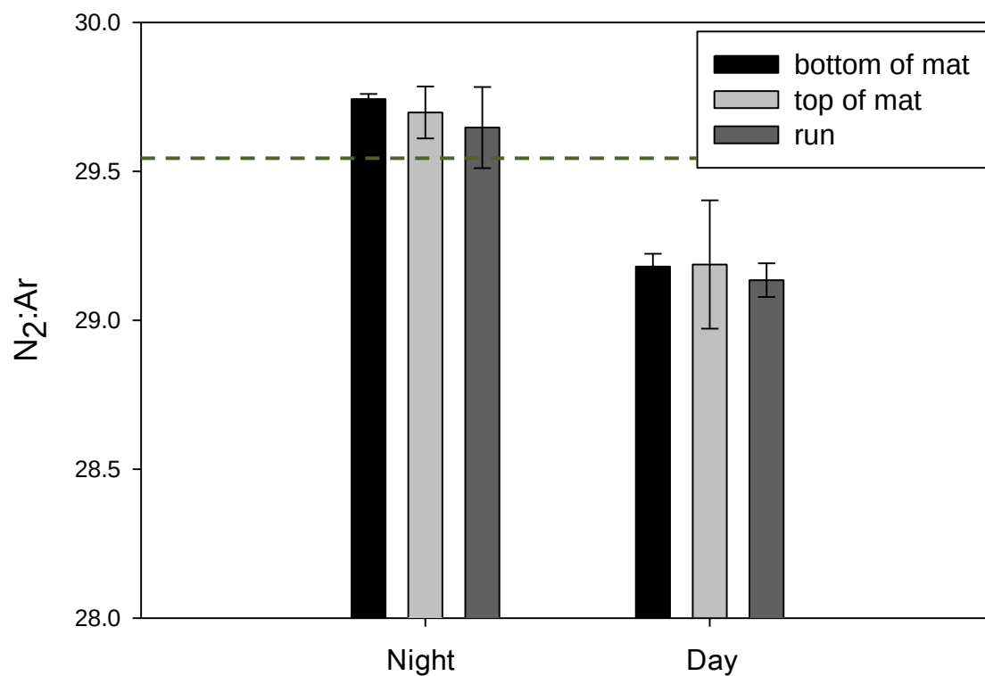
Fig. 7-12. Differences in the mean N_2:Ar ratio due to time of day and location in the river run. The dashed line represents the mean N_2:Ar ratio of the spring vent (29.57). Error bars are \pm one standard error.
