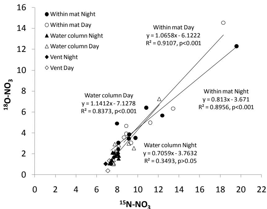
Fig. 7-8. Relationship between \delta^{15}\text{N} and \delta^{18}\text{O}-\text{NO}_3 of water from the spring vent, the water column and within the algal mat (both the top and bottom of the mat) at the spring vent and Sites 1 through 6 along Alexander Springs Creek .
