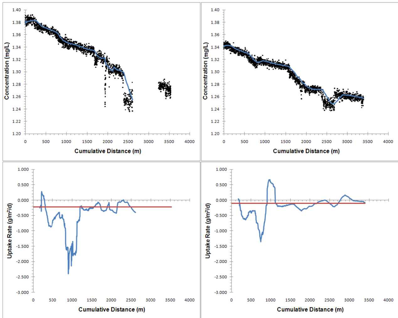
Figure 3-16. Longitudinal nitrate concentration (Top) and loss rate (Bottom) for Rock Springs Run on Dec. 1, 2010 (Left) and Dec. 16, 2010 (Right). The data break on the left is due to equipment malfunction.
