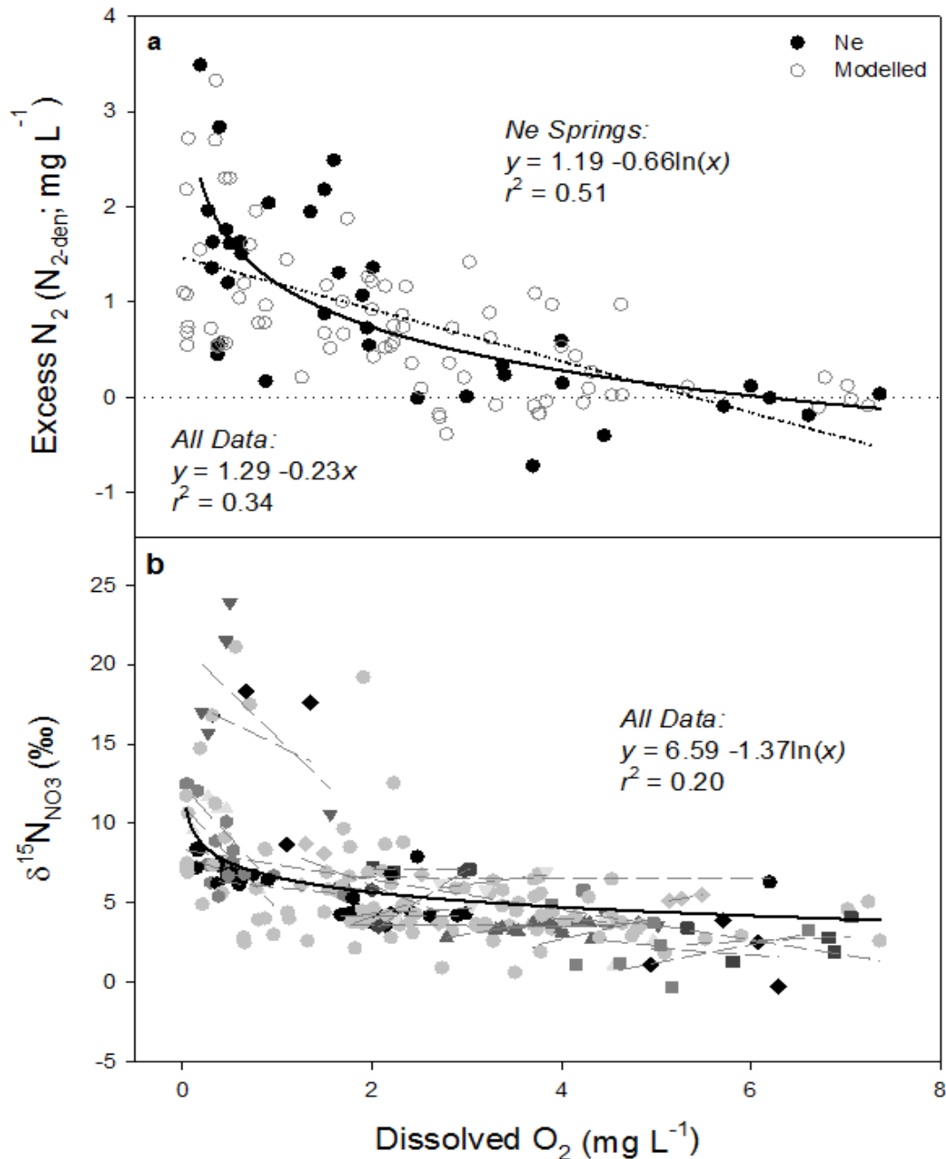
Fig. 6-4. Dissolved oxygen as a predictor of (a) excess N_2 and (b) \delta^{15}N_{NO_3} in Florida springs. In (a), closed symbols indicate measurements of denitrification-derived N_2 ( [N_{2\text{-den}}] ) based on direct estimation of excess air and recharge temperature via Ne and Ar; best fit for Ne springs is given by the solid line. Open symbols in (a) indicate [N_{2\text{-den}}] measurements based on modeled excess air and estimation of recharge temperature from Ar; best fit for all [N_{2\text{-den}}] data are shown by the dashed line. In (b), light symbols indicate data from springs with 3 or fewer observations; dark symbols indicate data from springs with 4 or more observations. Lines in (b) are best-fit linear regressions for individual springs with four or more observations of O_2 and \delta^{15}N_{NO_3} . Springs with high O_2 exhibit little variation in \delta^{15}N_{NO_3} , but low O_2 springs exhibit higher variability in \delta^{15}N_{NO_3} that is linked to variation in oxygen concentrations. Best-fit parameters for individual springs are given in Table 6-3 and their relationship to mean dissolved O_2 is shown in Figure 6-6.
