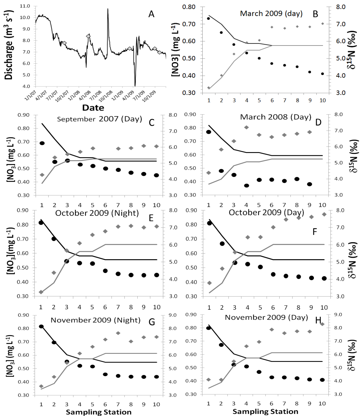
Fig. 5-2. Measured downstream discharge (A, black line) showing longitudinal sampling events (grey diamonds); hourly sampling was done in March and November 2009. Longitudinal changes in [NO_3^-] (black circles) and \delta^{15}N (grey diamonds) are shown from 7 events (5 day, 2 night, B - H). Springs inputs assuming mixing only are shown for [NO_3^-] (black line) and \delta^{15}N (grey line); deviation between observations and this line indicate biological processing.
