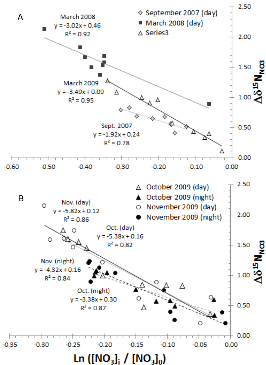
Fig. 5-3. Isotope enrichment ( \Delta\delta^{15}N between observations and flux-weighted springs inputs) of residual NO_3^- from 7 longitudinal sampling events (5 day – solid lines, 2 night – dashed lines); fitted slopes are enrichment factors ( \epsilon^{15} in ‰).
