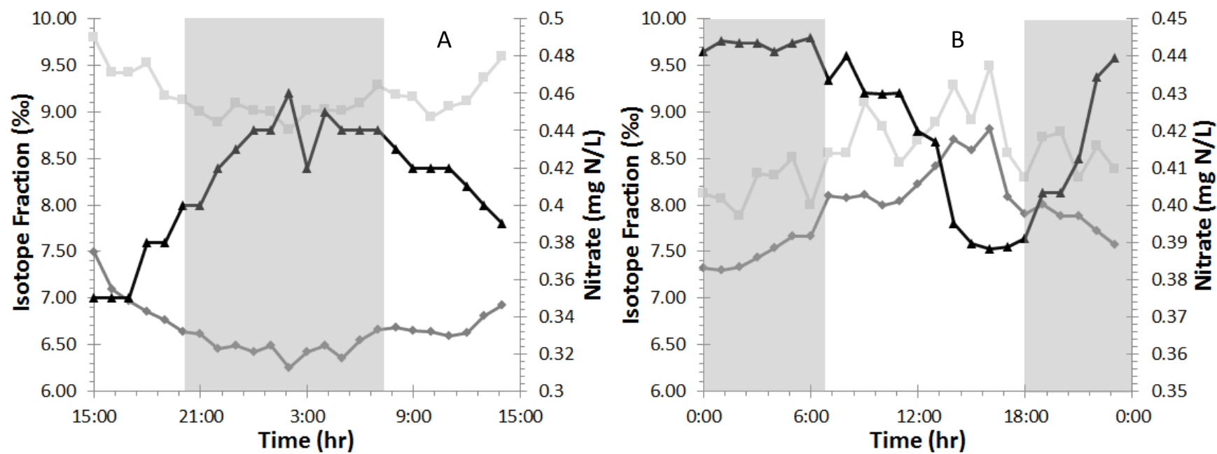
Fig. 5-6. Diel variation in [NO_3] (black line), \delta^{15}N (dark grey line) and \delta^{18}O (light grey line) for a) March and b) November 2009. Shaded areas denote night-time.
