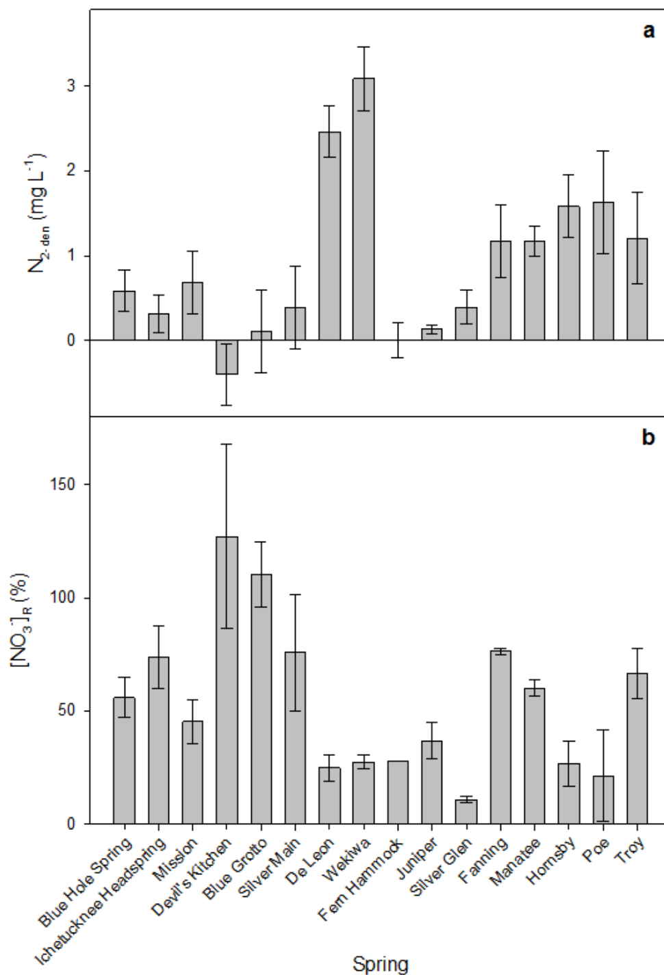
Figure 6-9. Variation in the magnitude of denitrification ( [N_2]_{den} ; panel A) and residual nitrate pools ( [NO_3]_R ; panel B) within and among springs of the Upper Floridan Aquifer. Variation among springs accounts for more than 90% of total variation in [N_2]_{den} . Full results of analysis of variance are given in Table S2. Data shown are from all springs with 3 or more estimates of [N_2]_{den} .
