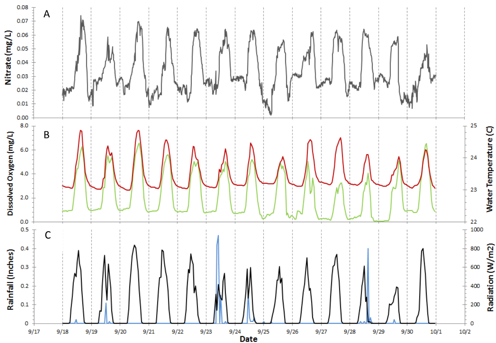
Fig. 2-38 - Diel variation in nitrate (grey line), dissolved oxygen (green line), water temperature (red line), radiation (black line) and rainfall (blue line) for the Alexander Springs Creek during September 2010 deployment. Vertical dashed lines are at midnight every 24 hours.
