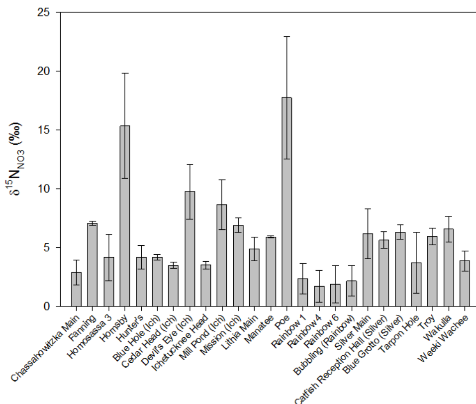
Figure 6-5. Variation in nitrate isotopic composition ( \delta^{15}N_{NO_3} ) within and among springs of the Upper Floridan Aquifer. Variation among springs accounts for more than 90% of total variation in \delta^{15}N_{NO_3} . Full results of analysis of variance are given in Table S2. Data shown are from all springs with 3 or more measurements of \delta^{15}N_{NO_3} .
