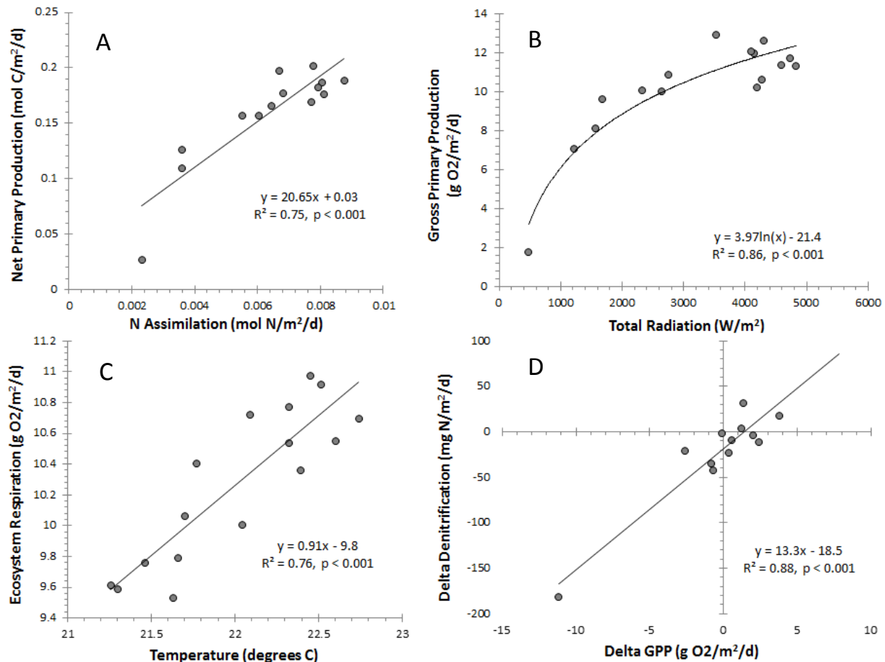
Fig. 2-9 – Summary of interrelated elements of ecosystem C and N metabolism. A) Relationship between N assimilation and C assimilation (assuming net primary production = 0.5 \times gross primary production) on a molar basis. The fitted slope indicates the C:N stoichiometry of ecosystem metabolism is ca. 20:1. B) Relationship between GPP (in g O 2 /m 2 /d) and incoming solar radiation (W/m 2 ), with a natural log best fit line. C) Relationship between ecosystem respiration (g O 2 /m 2 /d) and minimum daily water temperature (degrees C). D) Strong inter-day coupling of gross primary production and heterotrophic N removal (denitrification), showing that day-to-day changes in GPP (in g O 2 /m 2 /d) explain almost 90% of the observed day-to-day changes in estimated denitrification (mg N/m 2 /d).
