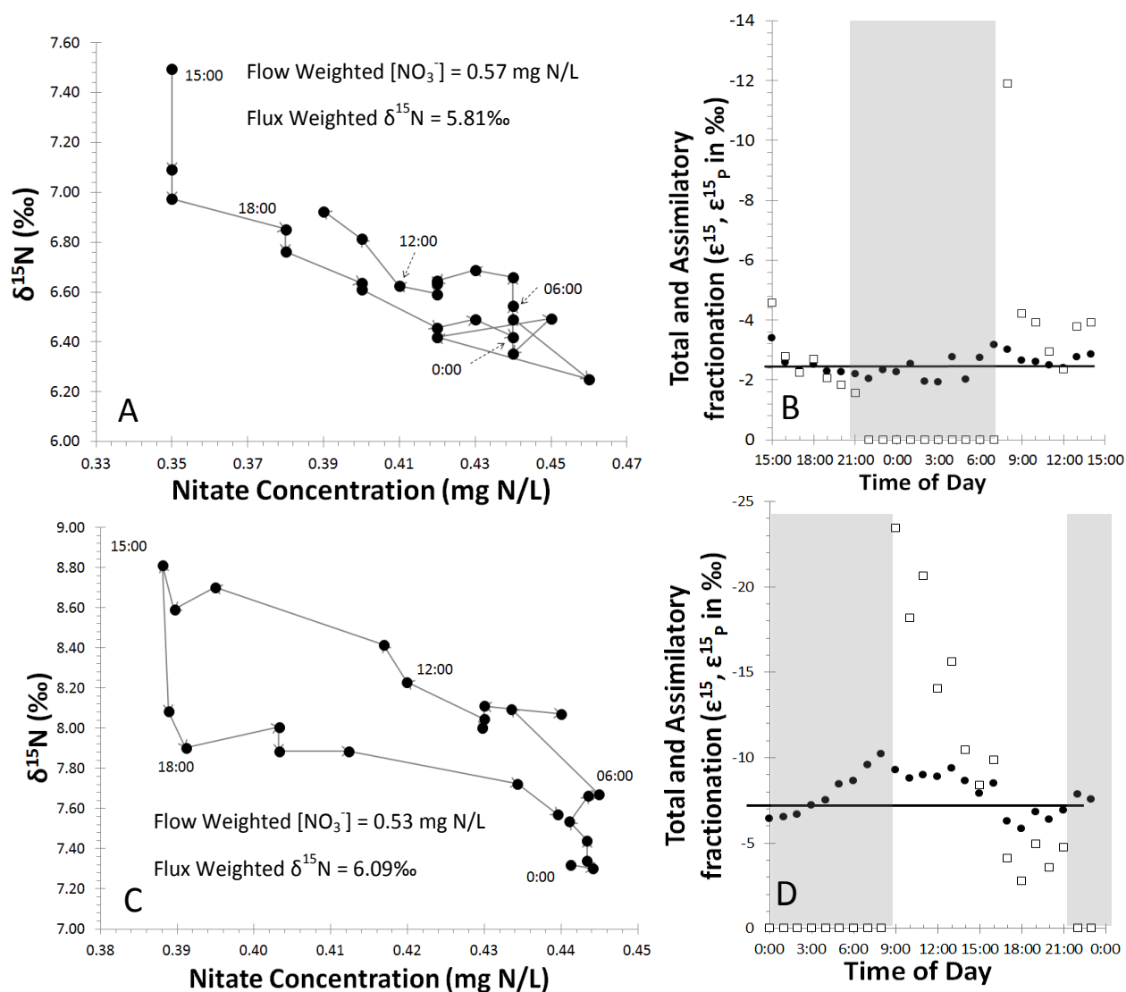
Fig. 5-8. Diel variation in isotope values and [\text{NO}_3^-] (A and C, for March and November 2009, respectively). Springs inputs (flow-weighted [\text{NO}_3^-] and flux-weighted \delta^{15}\text{N} ) are shown for each date. Total fractionation (black dots, in B and D, from March and November 2009, respectively) at night (grey areas) was used to estimate denitrification fractionation (horizontal black lines). Assuming constant denitrification fractionation implies significant variation in assimilatory fractionation (white squares) that drops over the course of the day.
