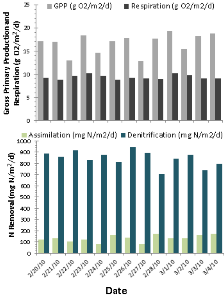
Fig. 2-12 – Summary of February 2010 deployment at Rainbow River showing estimates of gross primary production and respiration (top panel) and assimilatory and dissimilatory N removal (bottom panel).
