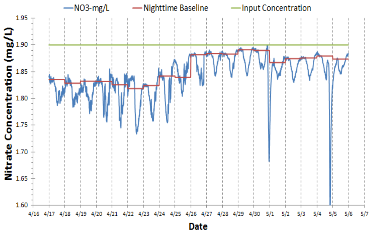
Fig. 2-25 – Summary of N removal mechanism inference. Assimilatory removal is estimated based on diel variation in nitrate (blue line) referenced to a nighttime baseline value (red line). Dissimilatory removal is estimated as the mass loss between upstream input concentrations (green line) and the nighttime baseline; that is, denitrification is assumed constant over the course of each 24-hour period. Day-to-day variation in the nitrate baseline is explored below.
