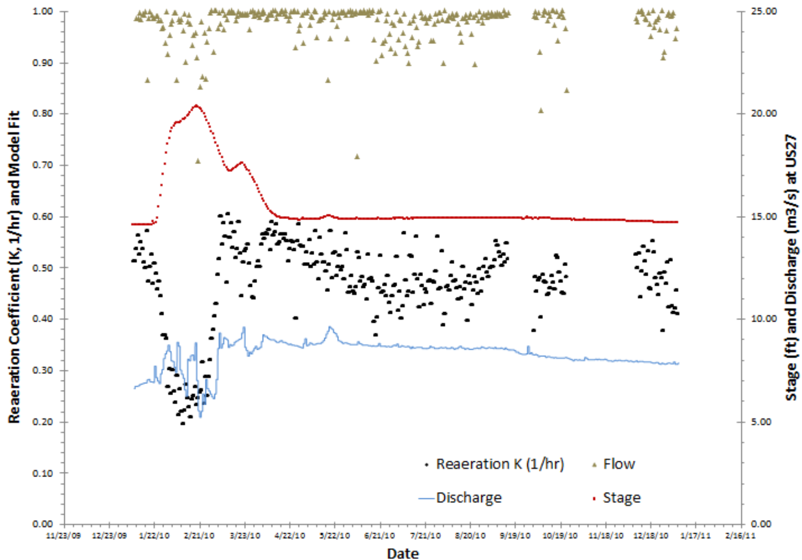
Fig. 2-19 – Results from the Ichetucknee River long term deployment showing the estimated reaeration constant ( K , \text{hr}^{-1} ) for each day (black dots). Also shown are river discharge ( \text{m}^3/\text{s} ) and stage (ft) at the US 27 bridge, as well as an estimate of goodness of fit ( r^2 ) for estimating K from nighttime DO dynamics.
