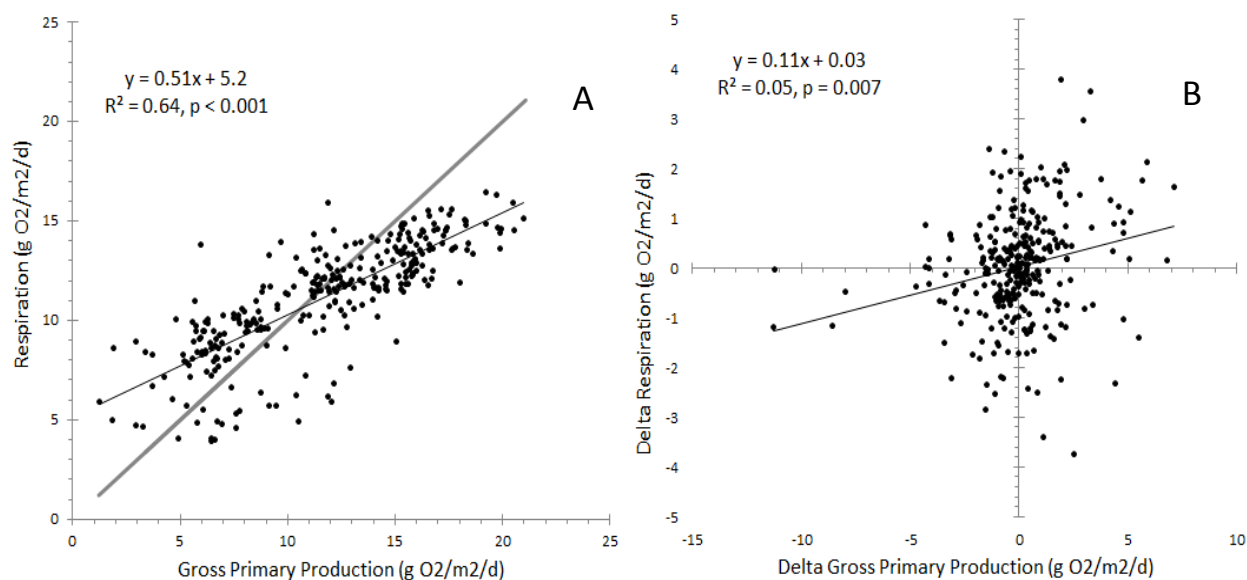
Fig. 2-22 – a) Association between GPP and R in the Ichetucknee River. Shown are instantaneous values of P and R, the best fit line, and the 1:1 line. Over the entire period, P:R is 1.1:1, but varies substantially. During periods of low GPP, baseline R remains high (intercept = 5.2 g O 2 /m 2 /d), and R varies less annually (mean ± SD: 11.1 ± 2.77 g O 2 /m 2 /d) than GPP (11.7 ± 4.3 g O 2 /m 2 /d). b) Inter-day coupling of P and R, showing weak but statistically significant positive coupling between day-to-day changes in GPP and associated changes in R.
