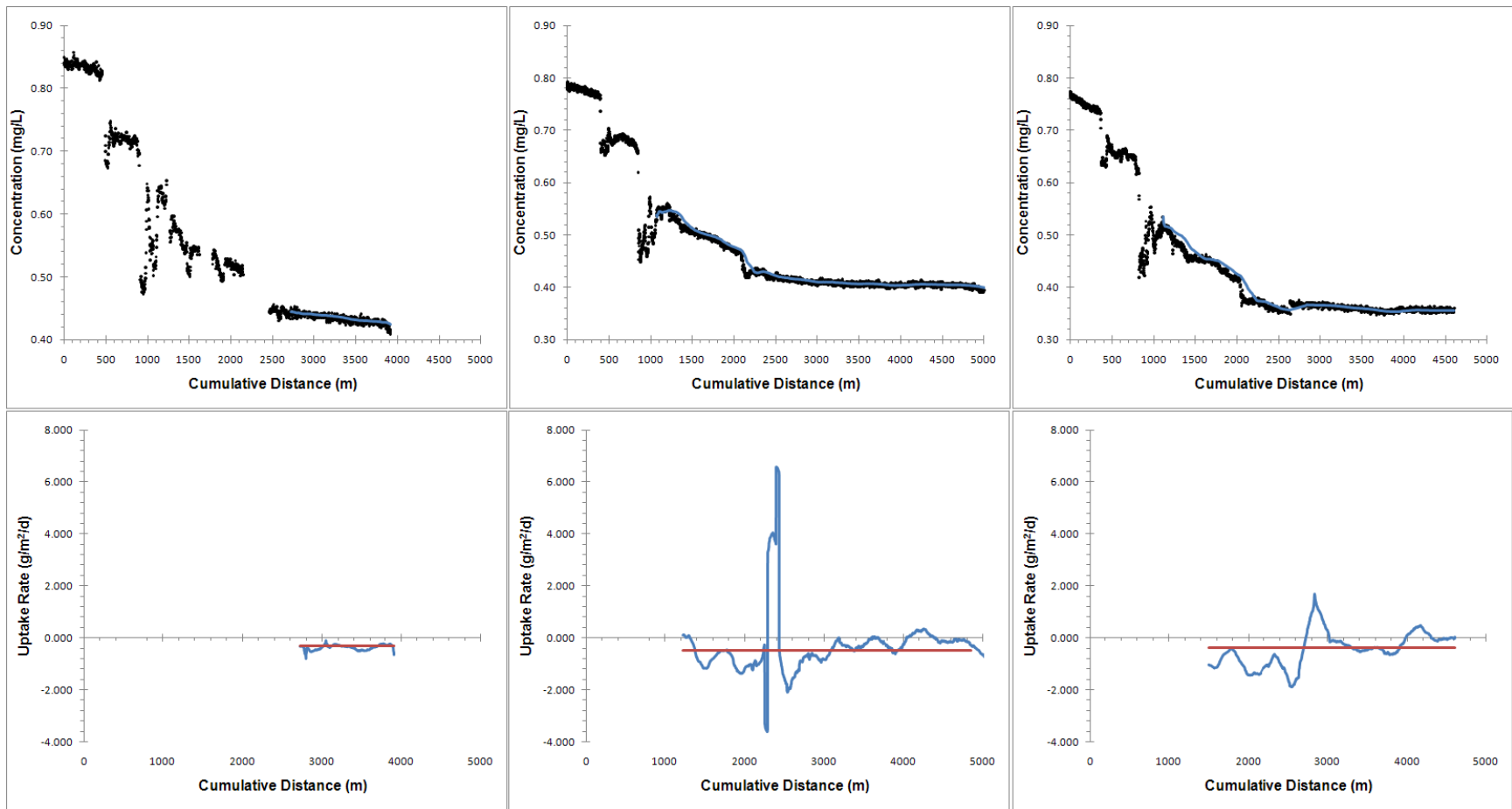
Figure 3-13. Longitudinal nitrate concentration profile (Top) and loss rate profile (Bottom) for Ichetucknee River on March 18, 2010 (Left), March 21, 2011 morning (Center) and March 21, 2011 afternoon (Right) . The large drops in the data are the result of spring inputs. The large break in the March 18, 2010 data is due to equipment malfunction. Note the loss rate has only been calculated for the downstream reach which has continuous data (last 1,500 m).
