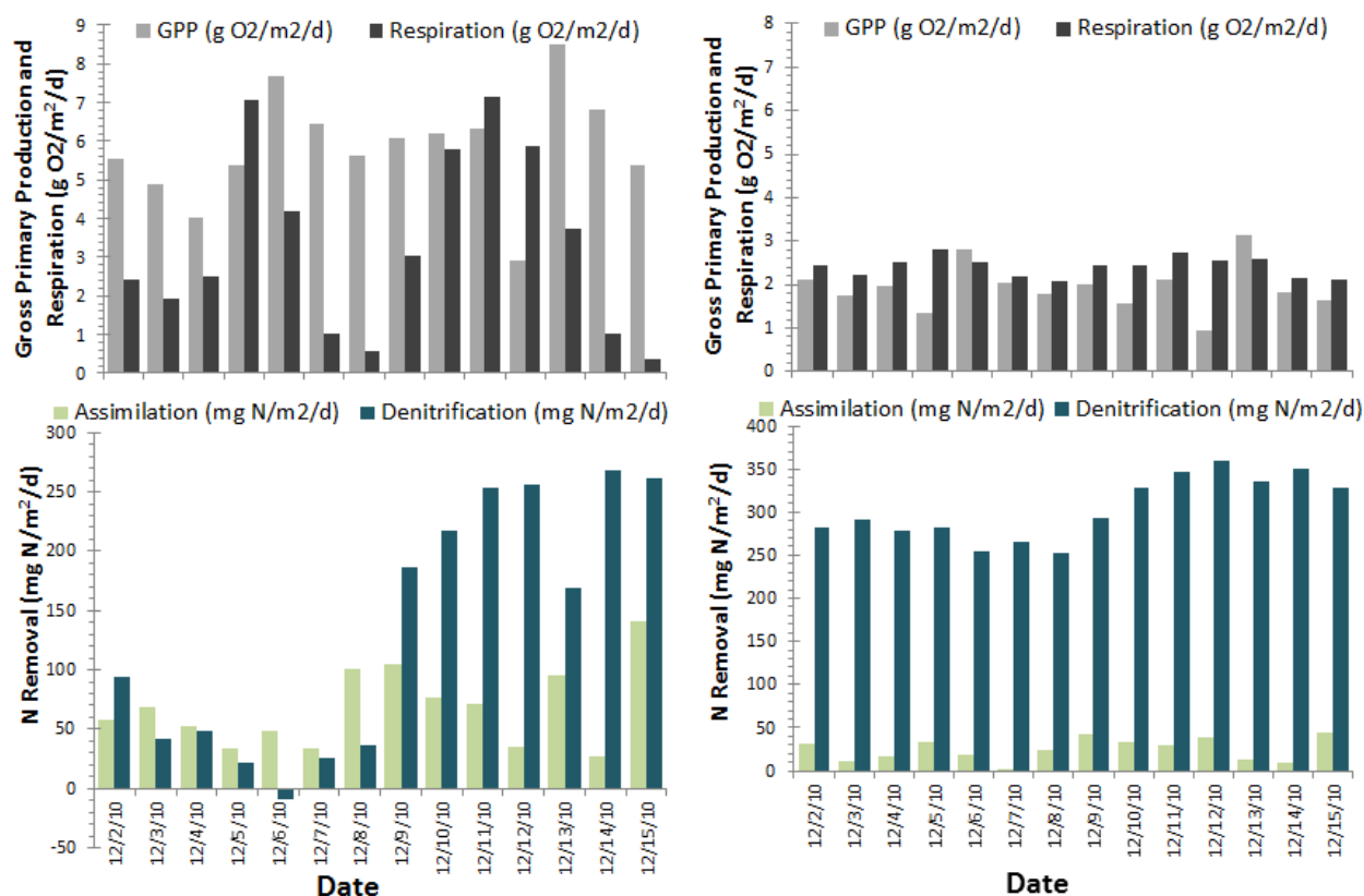
Fig. 2-53 – Summary of December 2010 deployment at Rock Springs Run showing estimates of gross primary production and respiration (top panels) and assimilatory and dissimilatory N removal (bottom panels) for both upstream (left panels) and downstream (right panels) reaches.
