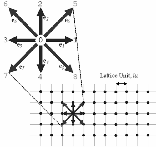
Figure 1. D2Q9 grid (Sukop and Thorne, 2006), e_{1-8} are unit velocity vectors
