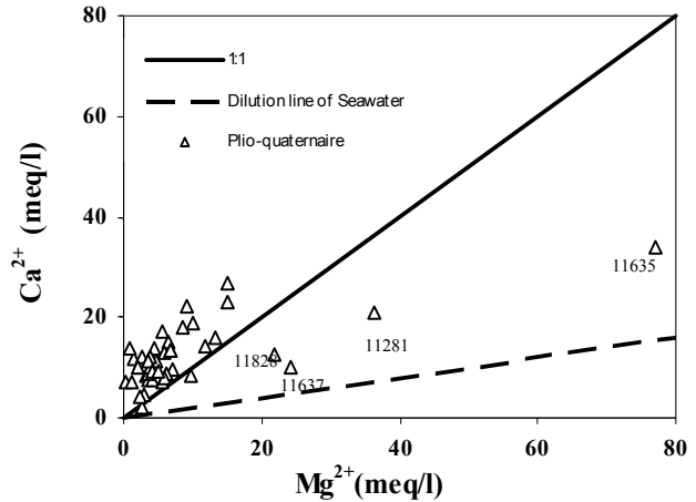
Figure 2. [\text{Ca}^{2+}]/[\text{Mg}^{2+}] correlation
