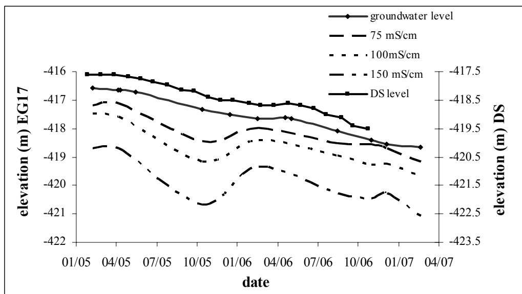
Figure 2. The transition zone between the fresh and saline water in a borehole located 200 m from the Dead Sea shore (values are of electrical conductivity which represent salinity up to about half of that of the Dead Sea). The transition zone moves downward during the Dead Sea level drop. Seasonal rises in the Dead Sea level cause an upward movement of the transition zone.
