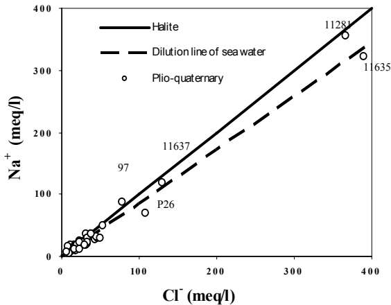
Figure 1. [\text{Na}^+]/[\text{Cl}^-] correlation
