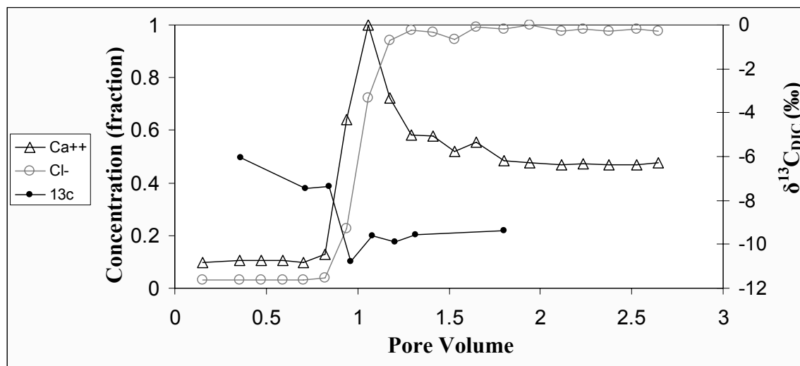
Figure 2. Seawater intrusion experiment results ( 200 \text{ m}\cdot\text{y}^{-1} ).
