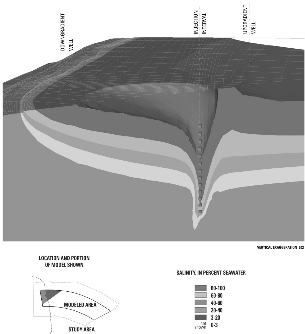
Figure 2. Cutaway block diagram showing simulated wastewater injection plume at Kihei, Maui, Hawaii. Effluent of 1 percent salinity is injected deep into brackish saline water but rises buoyantly, spreads laterally, and flows toward the coast at left. [Grayscale version of color original in Hunt, 2007.]
