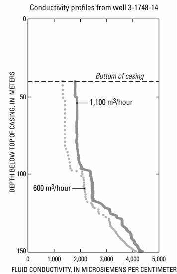
Figure 3. Fluid-conductivity profiles for nearby withdrawal of 600 m 3 /hour and 1,100 m 3 /hour, southern Oahu, Hawaii.
