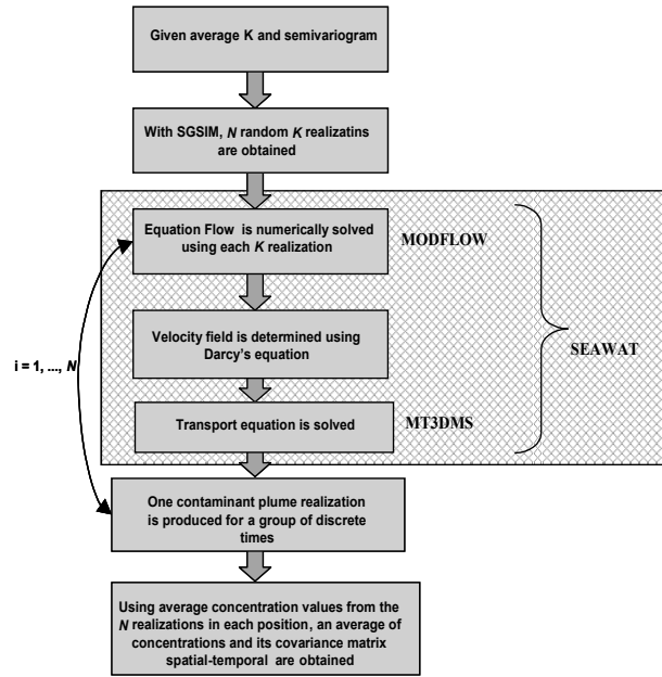
Figure 1. Flow chart of Variable density groundwater flow and transport solute simulation, used to obtain input files for GWQMonitor program.
