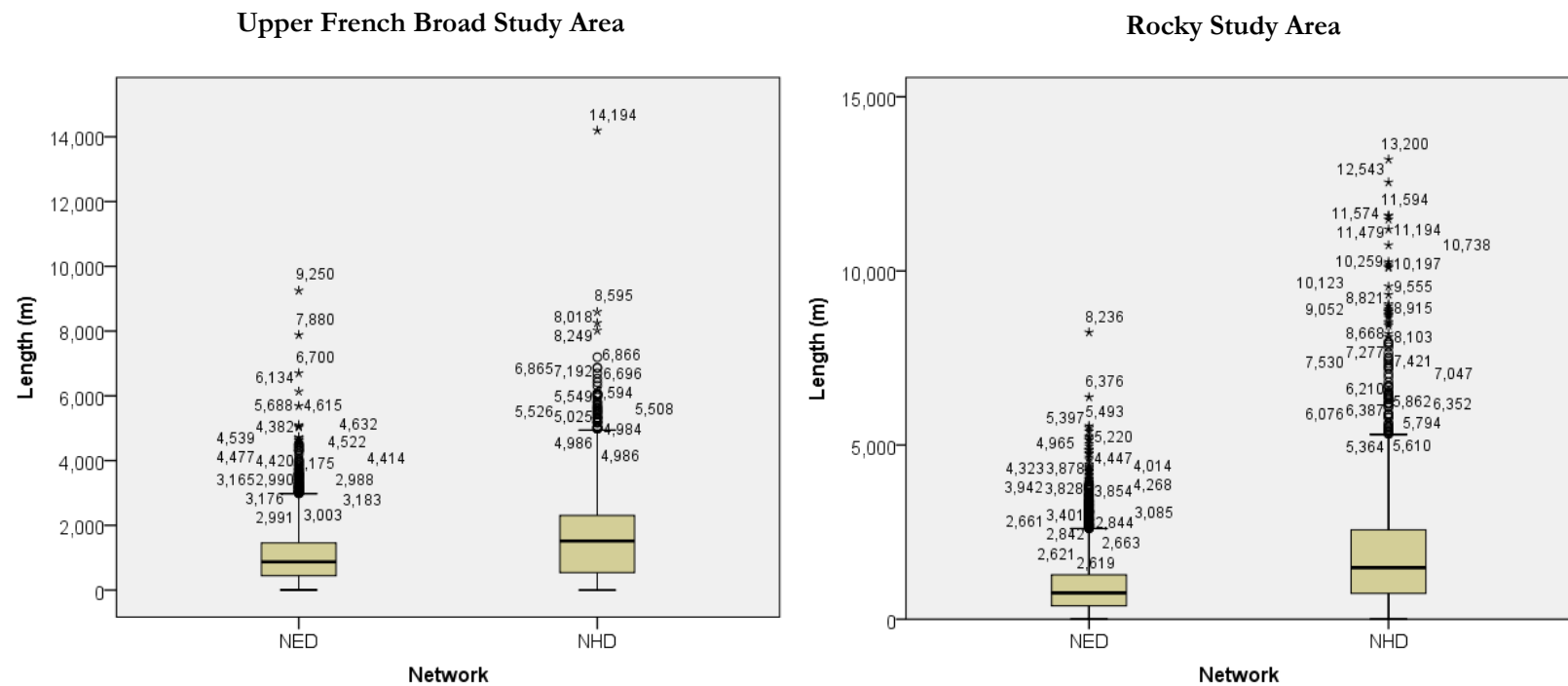
Figure 5.4. Reach Lengths of LIDAR-derived and NHDPlus Stream Networks
