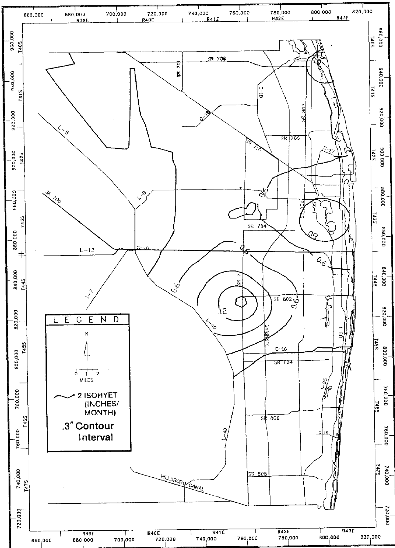
Figure D-16 KRIGED RAINFALL DISTRIBUTION IN EASTERN PALM BEACH COUNTY FOR FEBRUARY 1985
