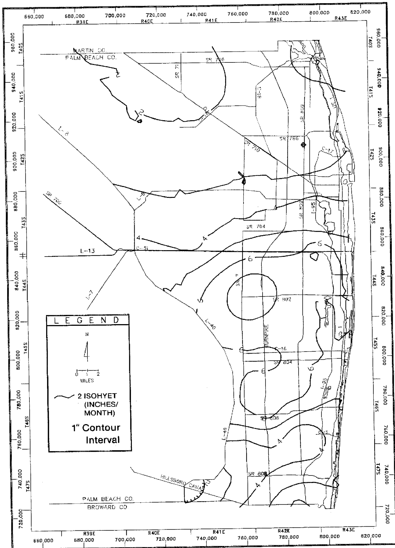
Figure D-6 KRIGED RAINFALL DISTRIBUTION IN EASTERN PALM BEACH COUNTY FOR APRIL 1984
