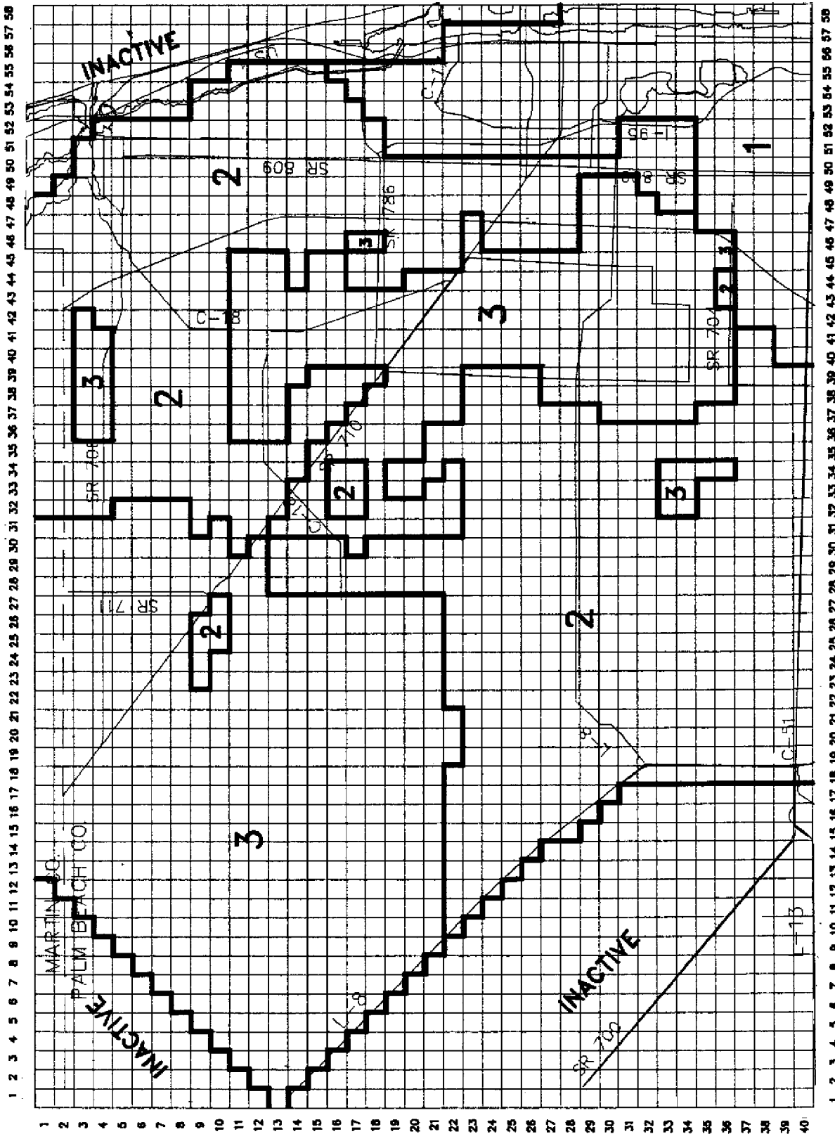
Figure 13 NORTH PALM BEACH COUNTY MODEL RECHARGE ZONES
