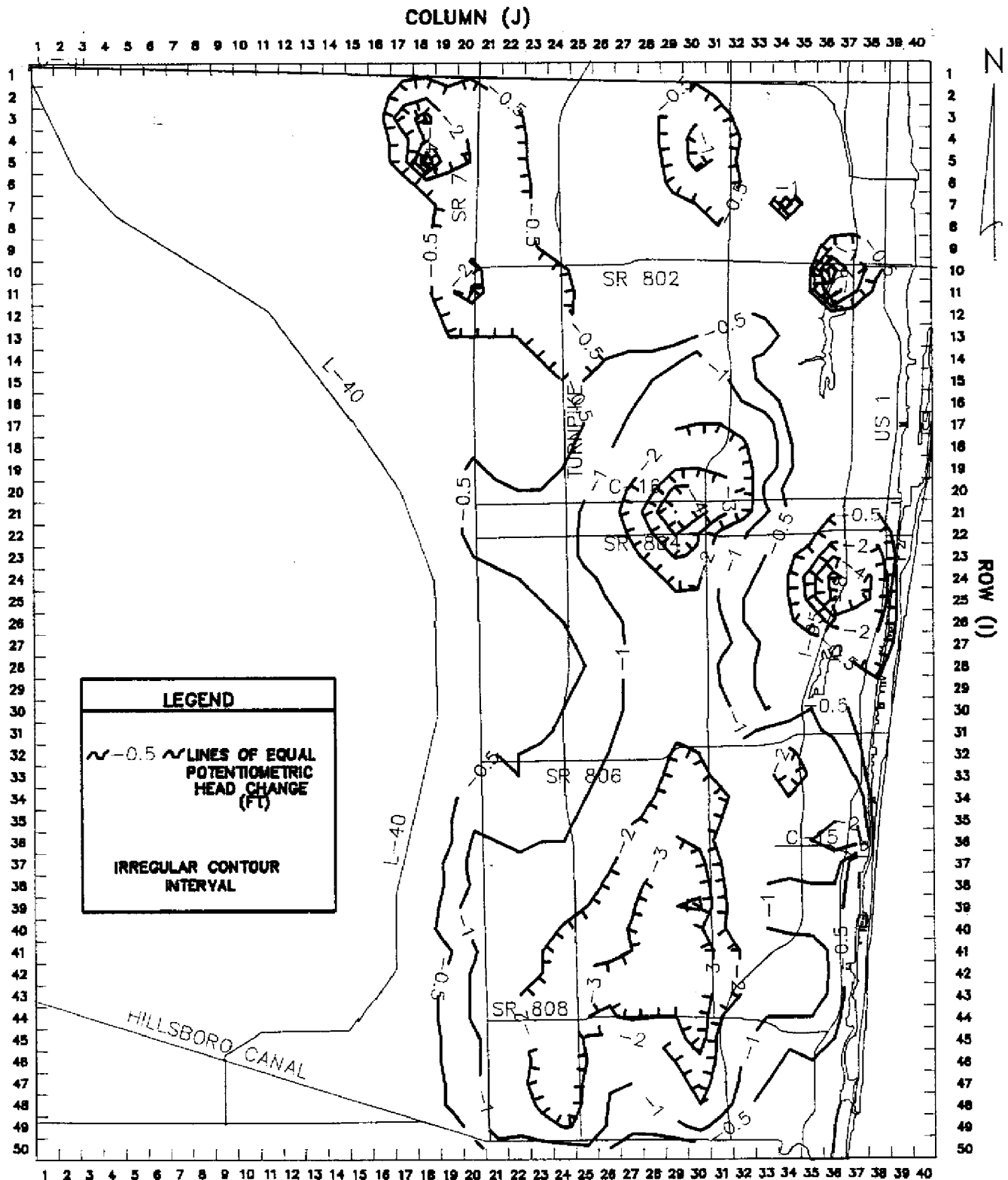
Figure 74 SIMULATED DECLINE IN GROUND WATER LEVELS IN SOUTHEASTERN PALM BEACH COUNTY (MODEL LAYER 1) AS A RESULT OF ELIMINATING RECHARGE FROM SURFACE WATER SYSTEMS UNDER AVERAGE CONDITIONS
