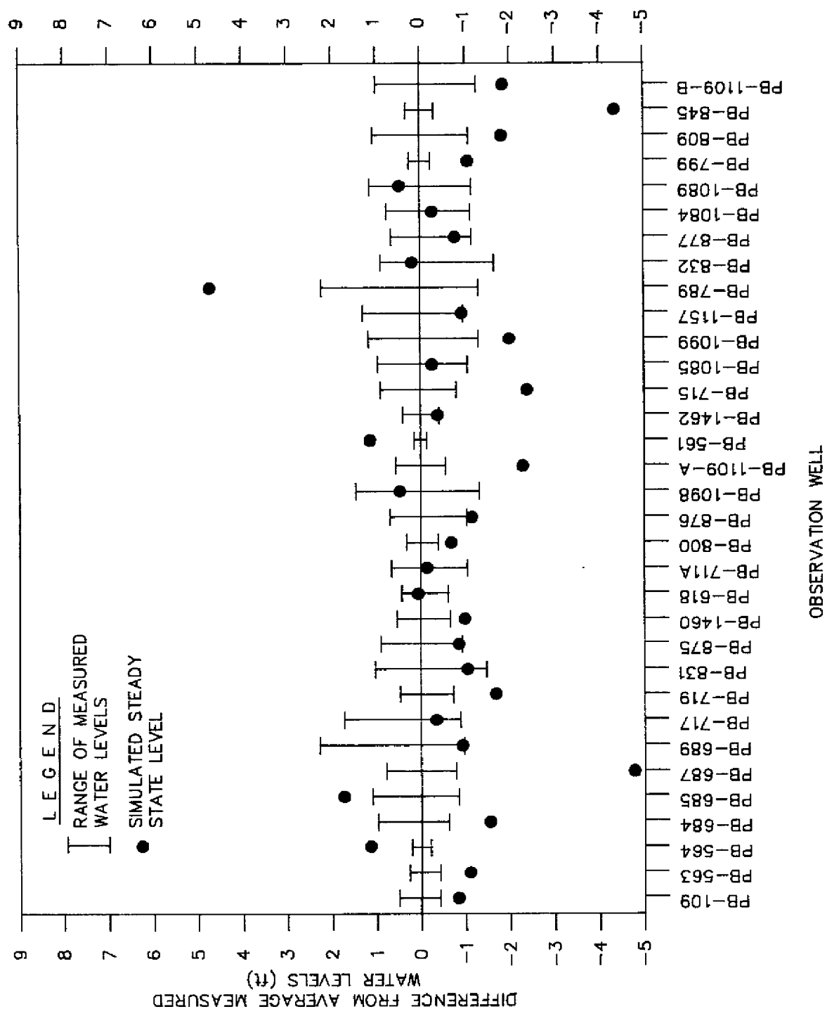
Figure 39 NORTH PALM BEACH COUNTY MODEL STEADY STATE CALIBRATION RESIDUALS FROM AVERAGE MEASURED WATER LEVELS
