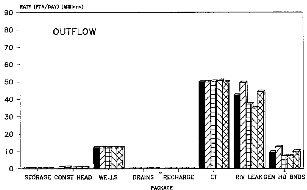
Figure 52 SOUTH MODEL INFLOW AND OUTFLOW MASS BALANCES FOR BASE RUN AND HYDRAULIC CONDUCTIVITY, VERTICAL CONDUCTANCE, AND VERTICAL TO HORIZONTAL ANISOTROPY RATIO SENSITIVITY SIMULATIONS
