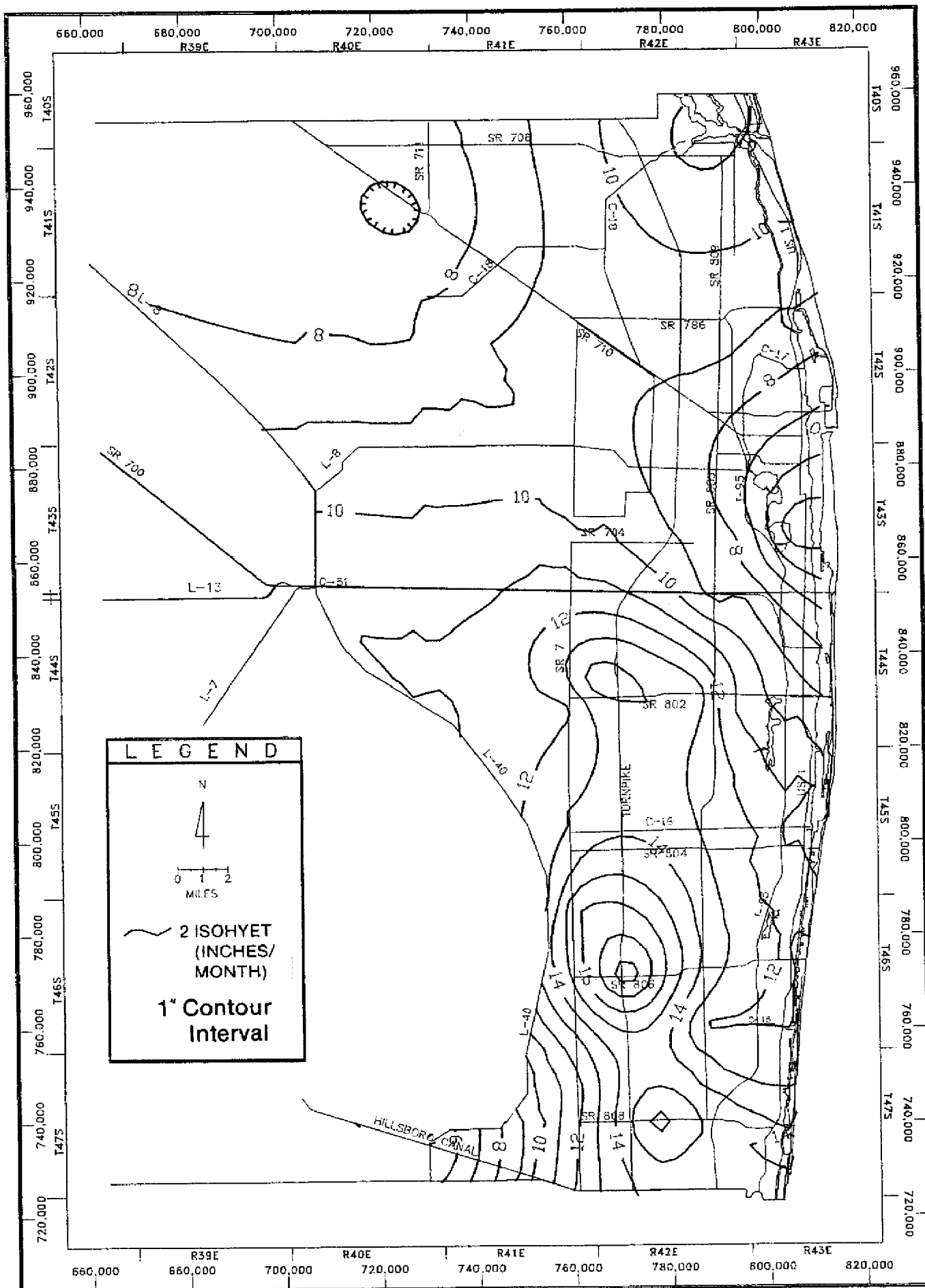
Figure D-7 KRIGED RAINFALL DISTRIBUTION IN EASTERN PALM BEACH COUNTY FOR MAY 1984
