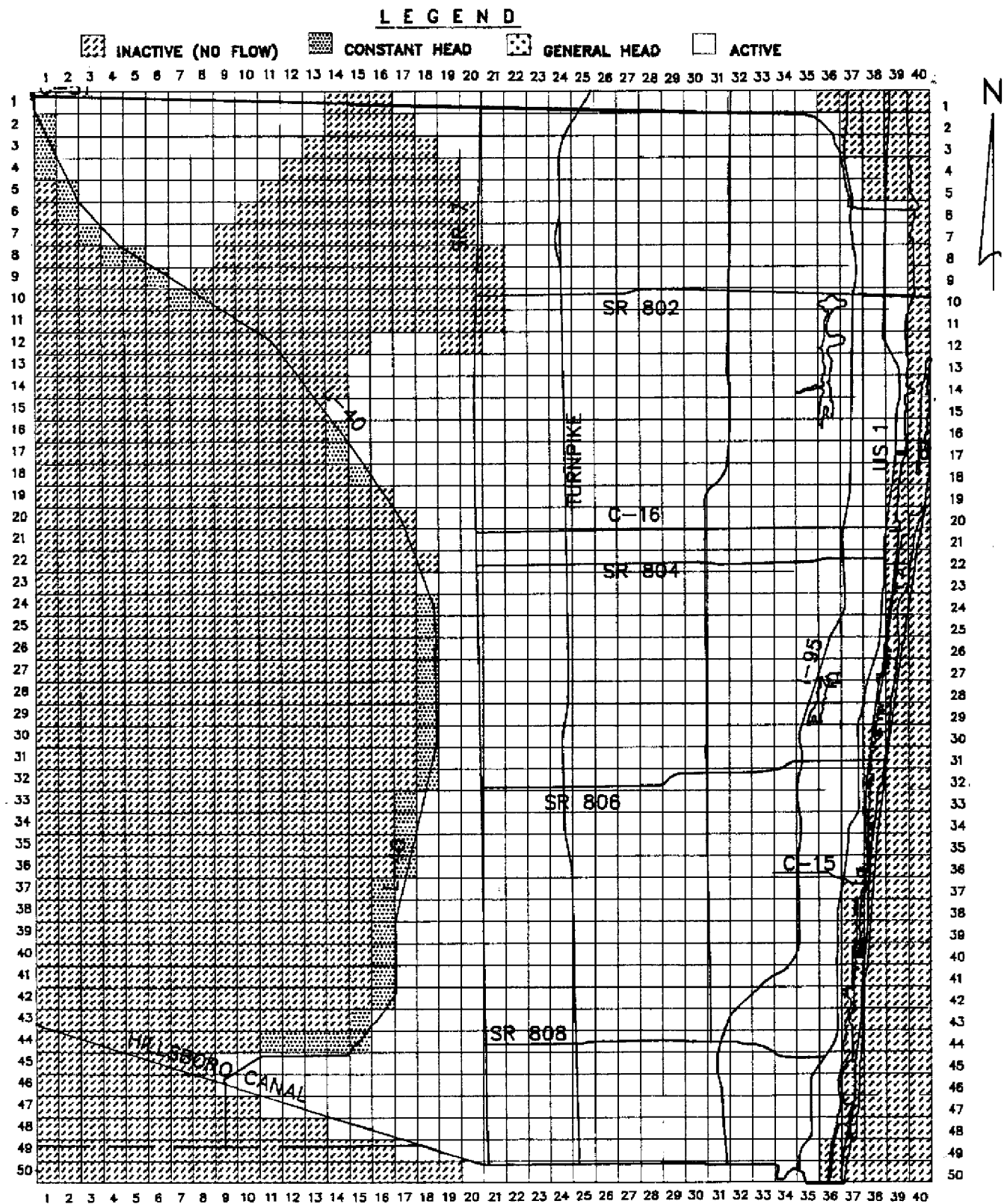
Figure 22 SOUTH PALM BEACH COUNTY MODEL LAYER 5 CELL TYPES
