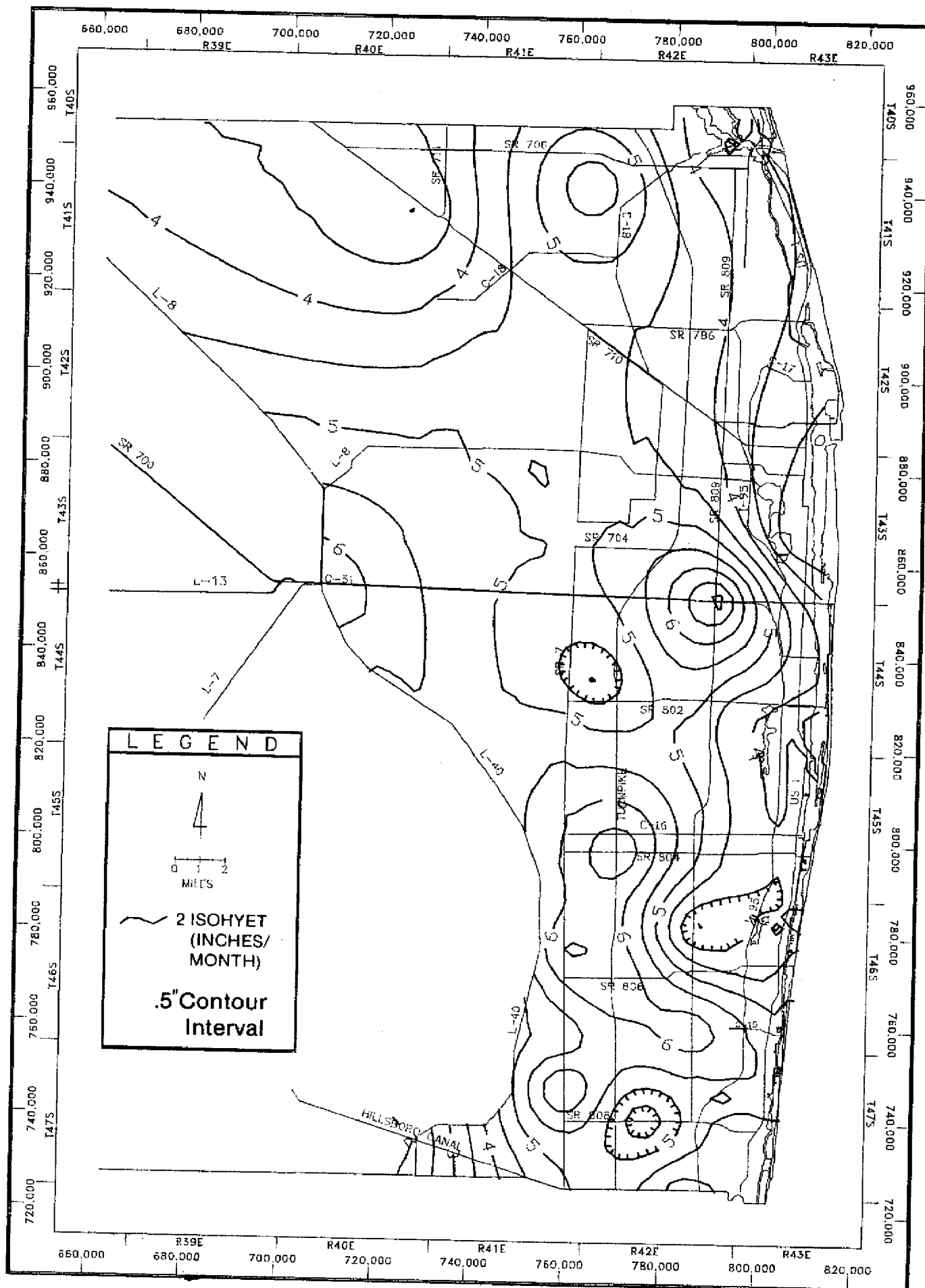
Figure D-9 KRIGED RAINFALL DISTRIBUTION IN EASTERN PALM BEACH COUNTY FOR JULY 1984
