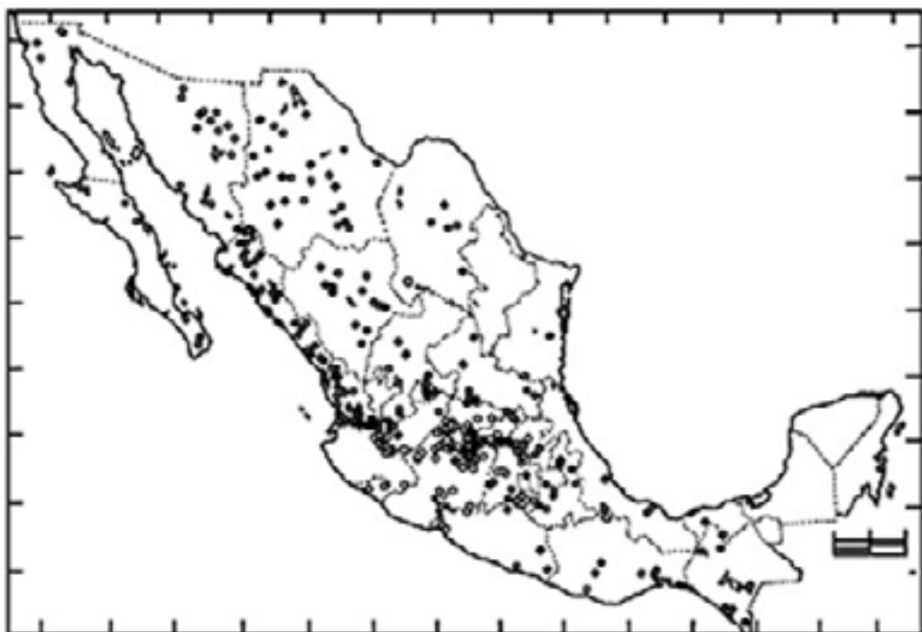
Figure 9-110. Distribution of thermal springs mapped by the Federal Comisión of Electricity of Mexico.
