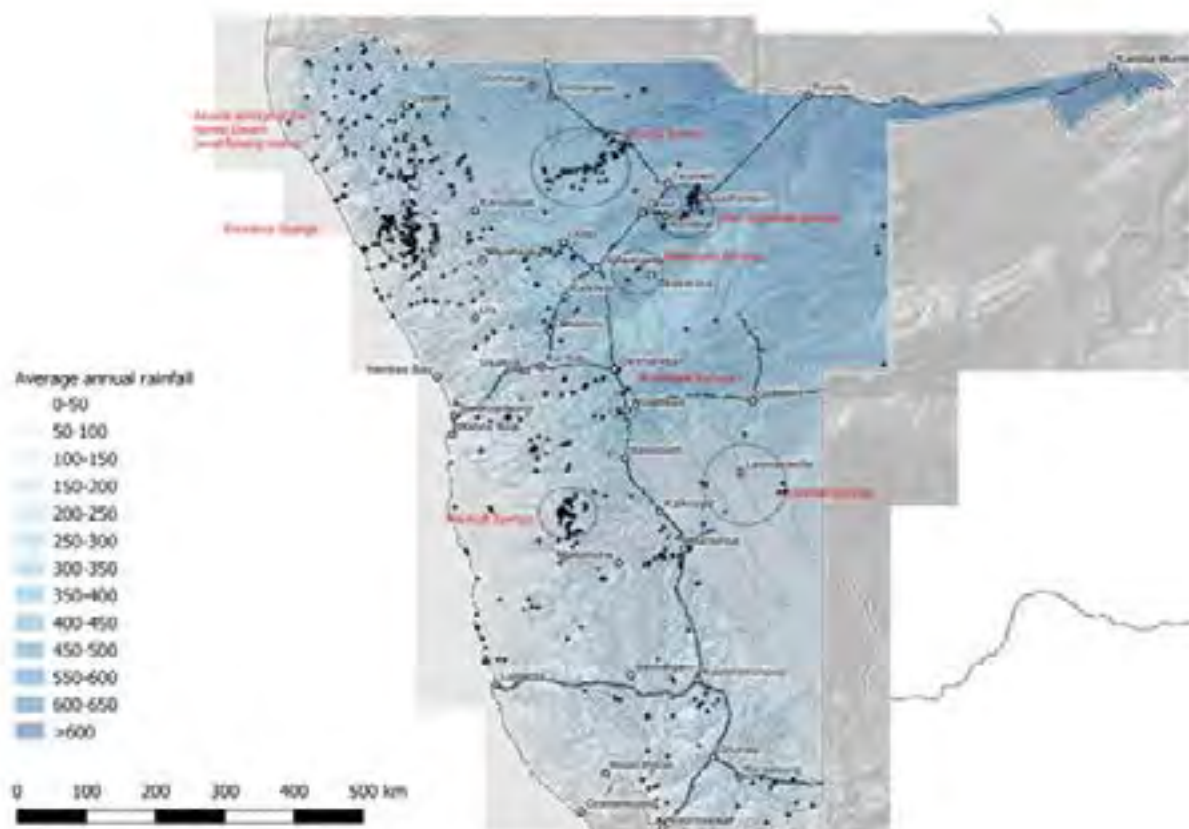
Figure 4-50. Distribution of Namibia's springs and average rainfall
