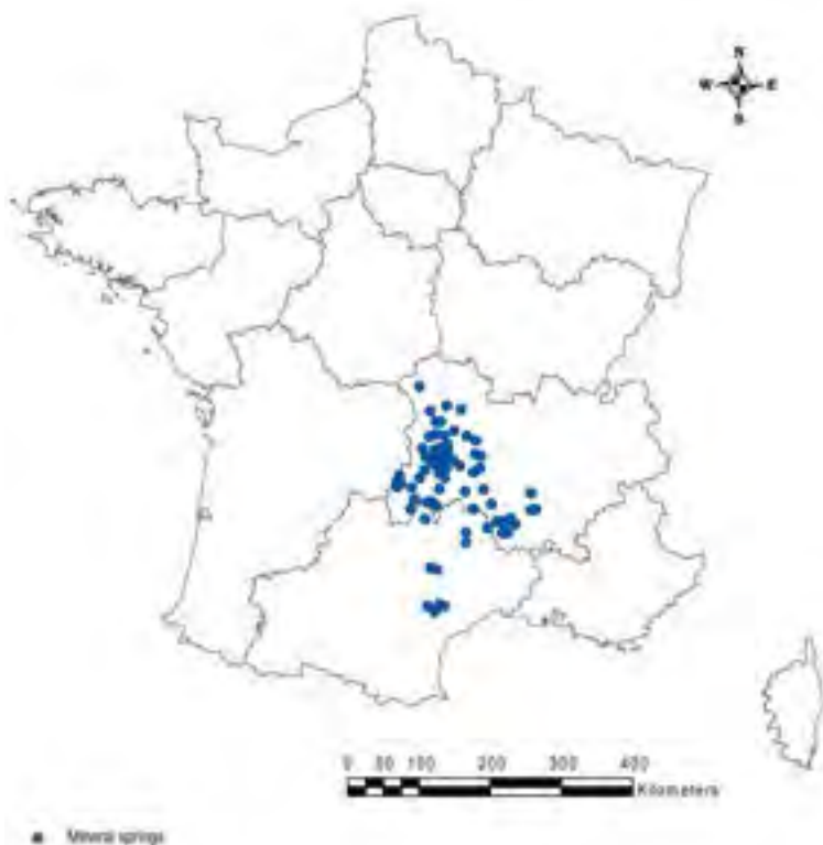
Figure 3-17. Map of the mineral springs of the French Massif Central (prepared by Olivier Voldoire).
