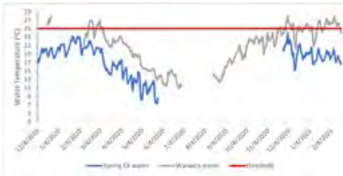
Figure 8-81. Plot of average daily water temperature in groundwater-fed South Spring Creek and in a more typical upper Condamine River site at nearby Warwick (Queensland Government stream gauge 422310C). Even during the extreme heatwave conditions of late 2019 Spring Creek water temperature remained below the thermal threshold of 25°C required to sustain its specialist cold water species, whereas water in the general region exceeded that limit (Queensland Government, unpublished data).
