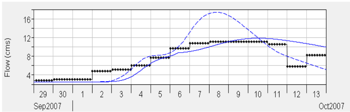
Figure 2-31. Jane Green Reservoir Validation Results USGS Gauge 02231600
