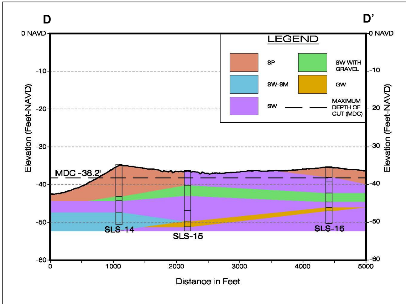
Figure 5.13: St. Lucie Shoal: Area D – Interpreted Fence Diagram
