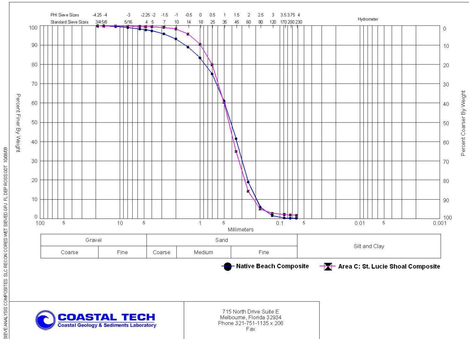
Figure 5.11: Native Beach and St. Lucie Shoal: Area C Composite Grain-size Distribution Curves
