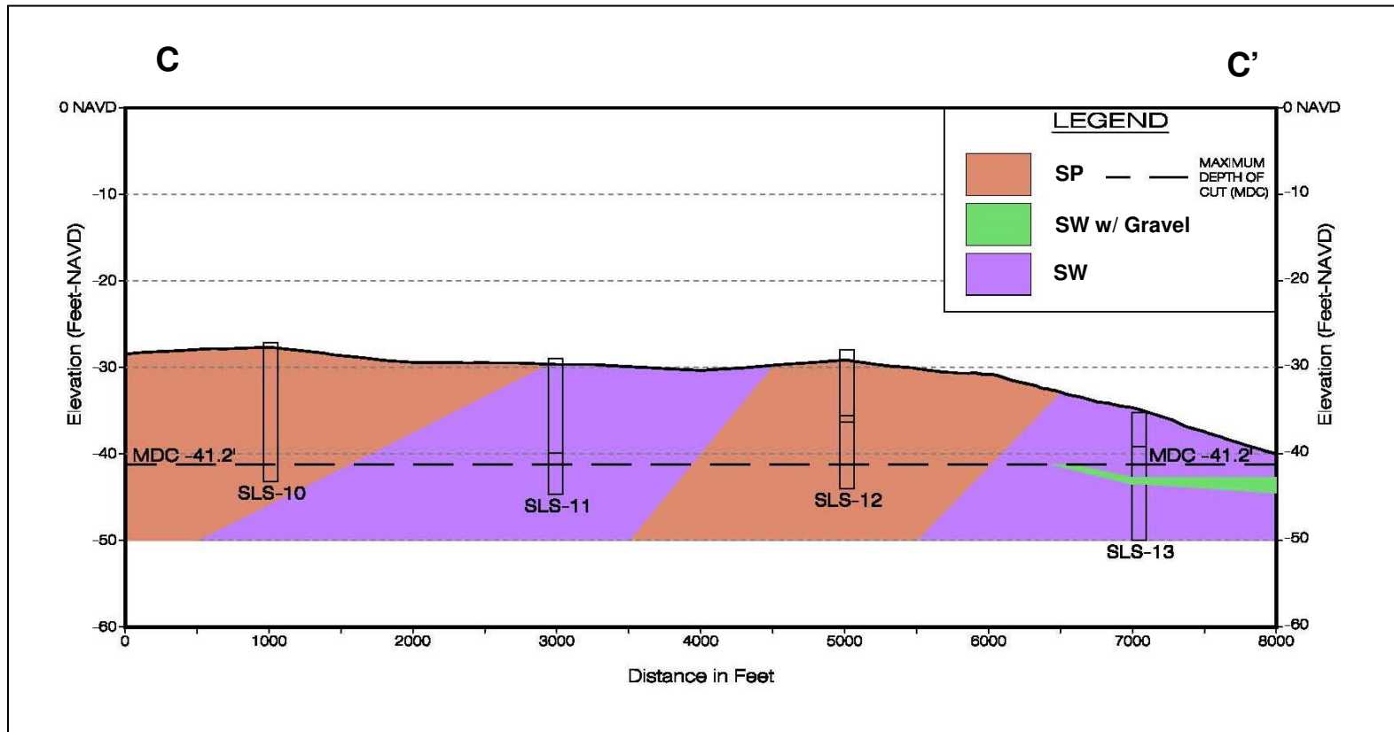
Figure 5.10: St. Lucie Shoal: Area C – Interpreted Fence Diagram
