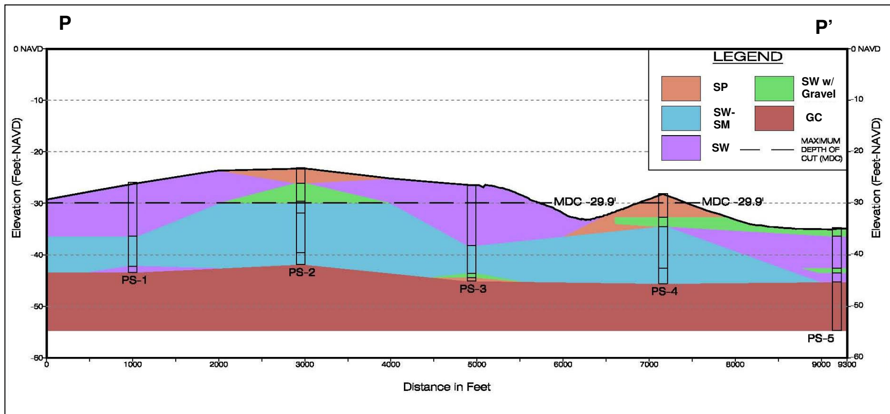
Figure 5.4: Pierce Shoal – Interpreted Fence Diagram
