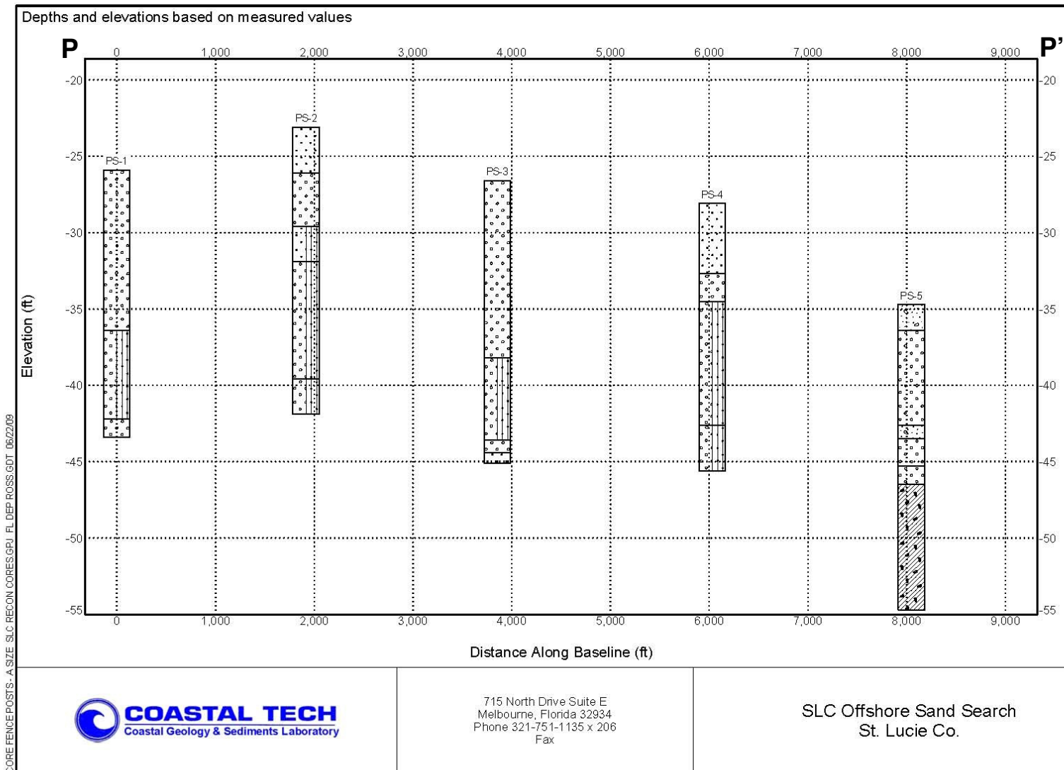
Figure 5.3: Pierce Shoal Geologic Cross-Section
