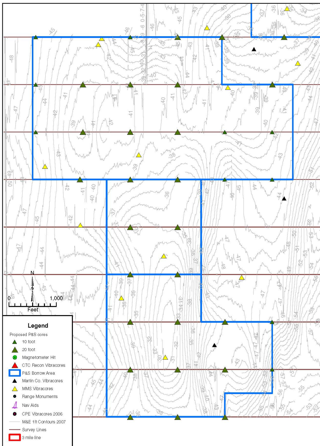
Figure 6.3: Proposed Plans and Specs Vibracoring Plan: Area B
