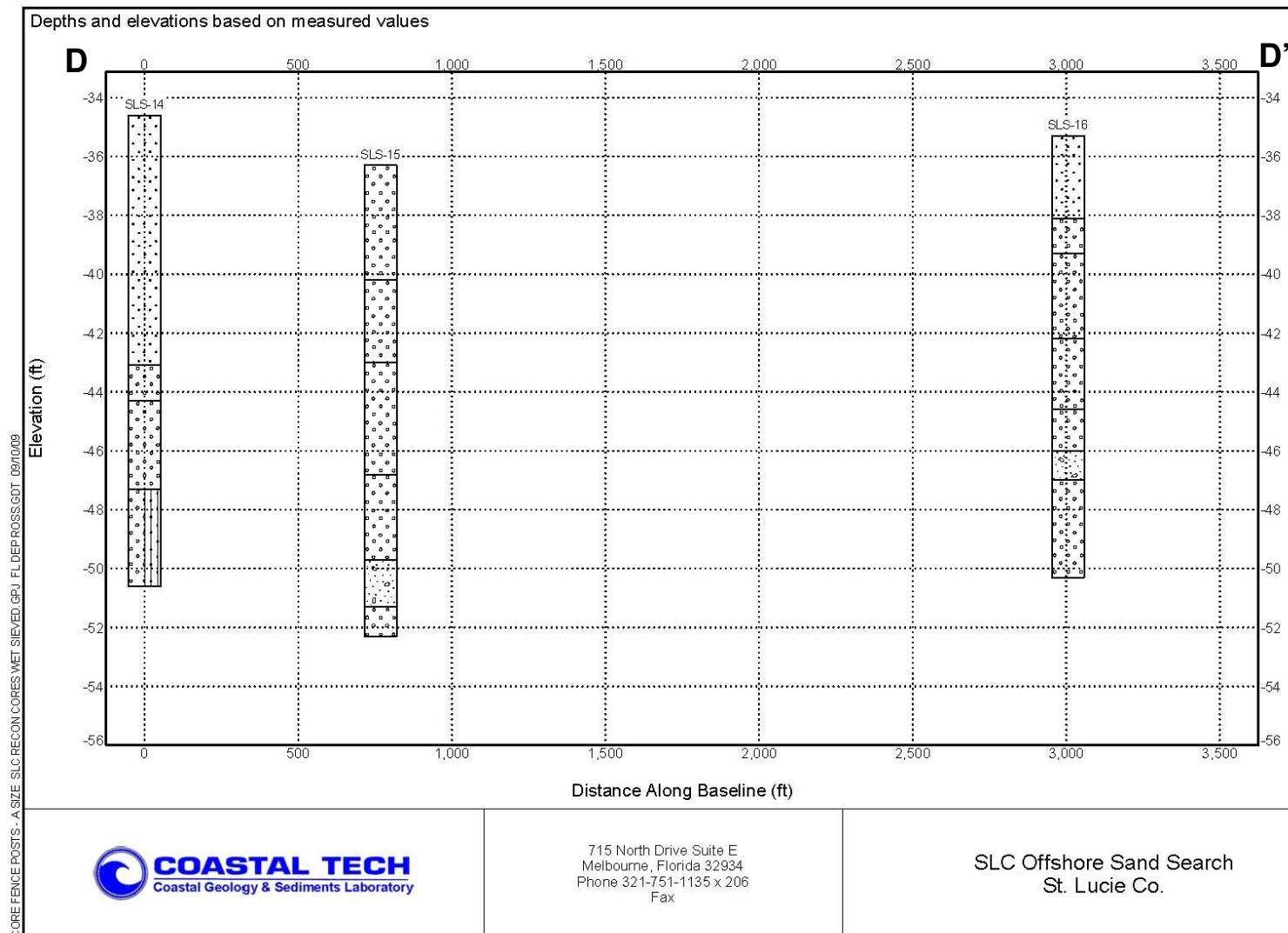
Figure 5.12: St. Lucie Shoal: Area D – Geologic Cross-Section
