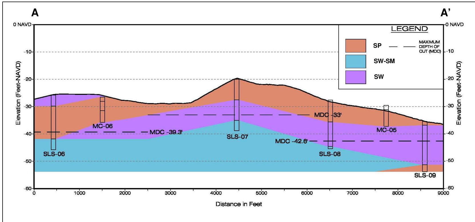
Figure 5.7: St. Lucie Shoal: Area A – Interpreted Fence Diagram
