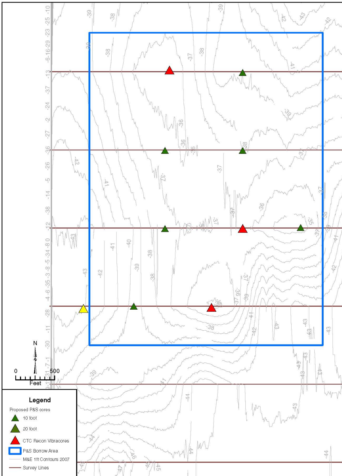
Figure 6.5: Proposed Plans and Specs Vibracoring Plan: Area D
