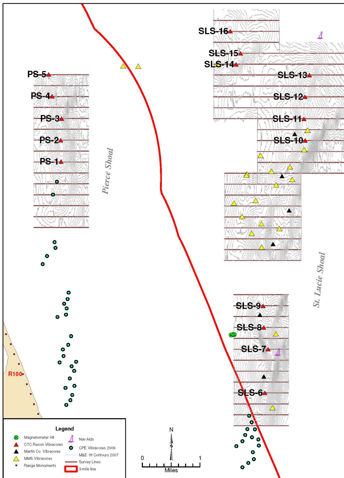
Figure 2.1: Location Map - Reconnaissance & Existing Vibracores
