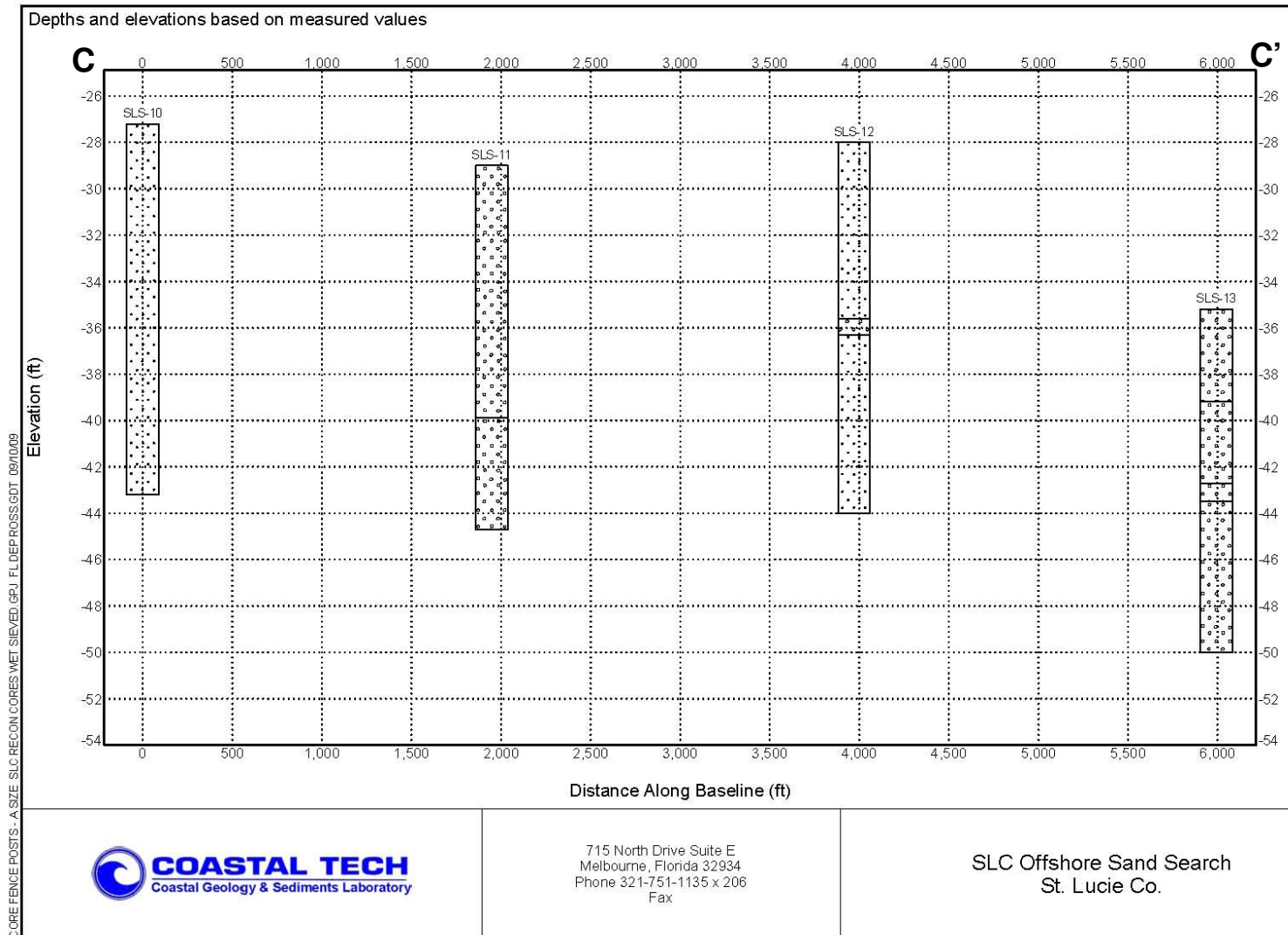
Figure 5.9: St. Lucie Shoal: Area C – Geologic Cross-Section
