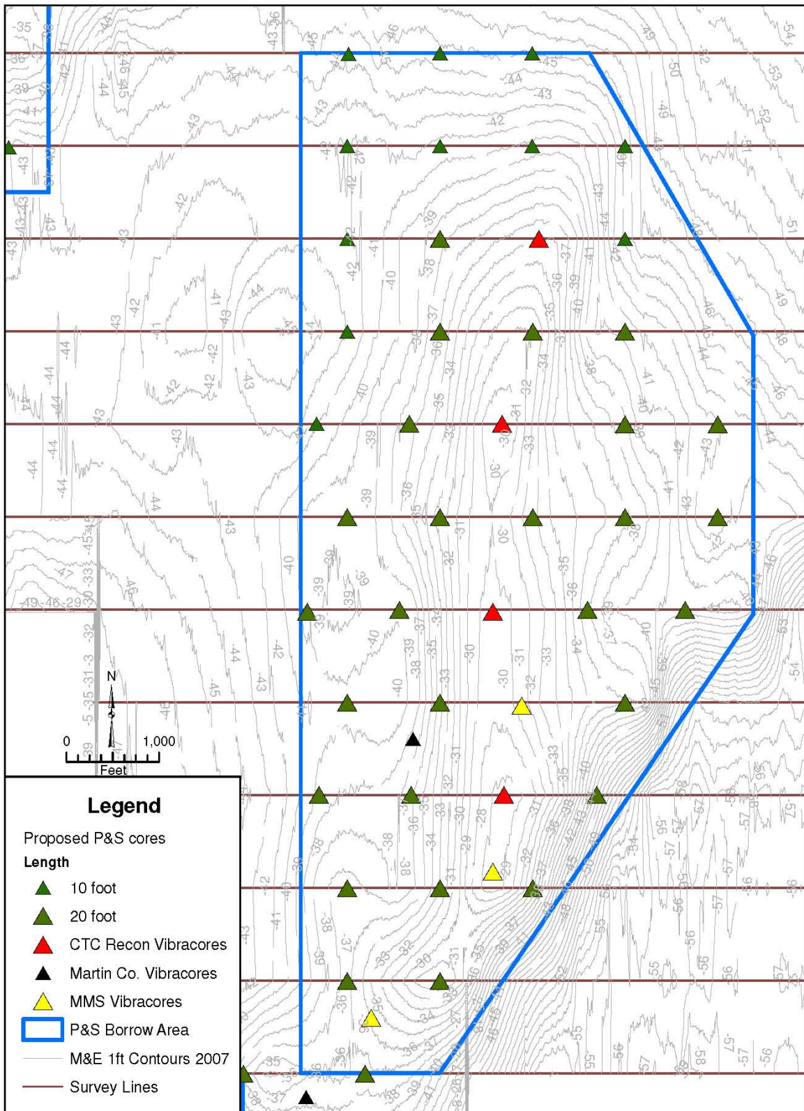
Figure 6.4: Proposed Plans and Specs Vibracoring Plan: Area C
