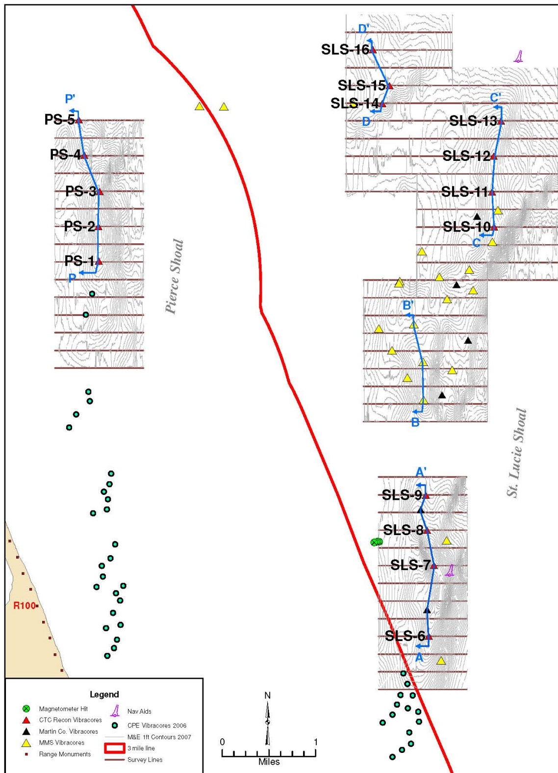
Figure 5.2: Potential Borrow Areas with Cross-Section Lines
