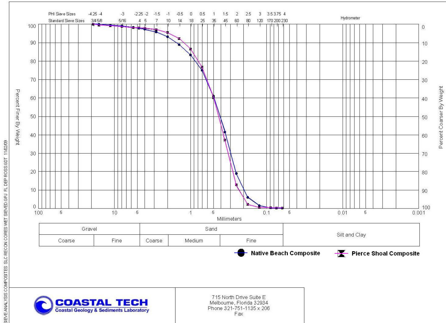
Figure 5.5: Native Beach and Pierce Shoal: Composite Grain-size Distribution Curves
