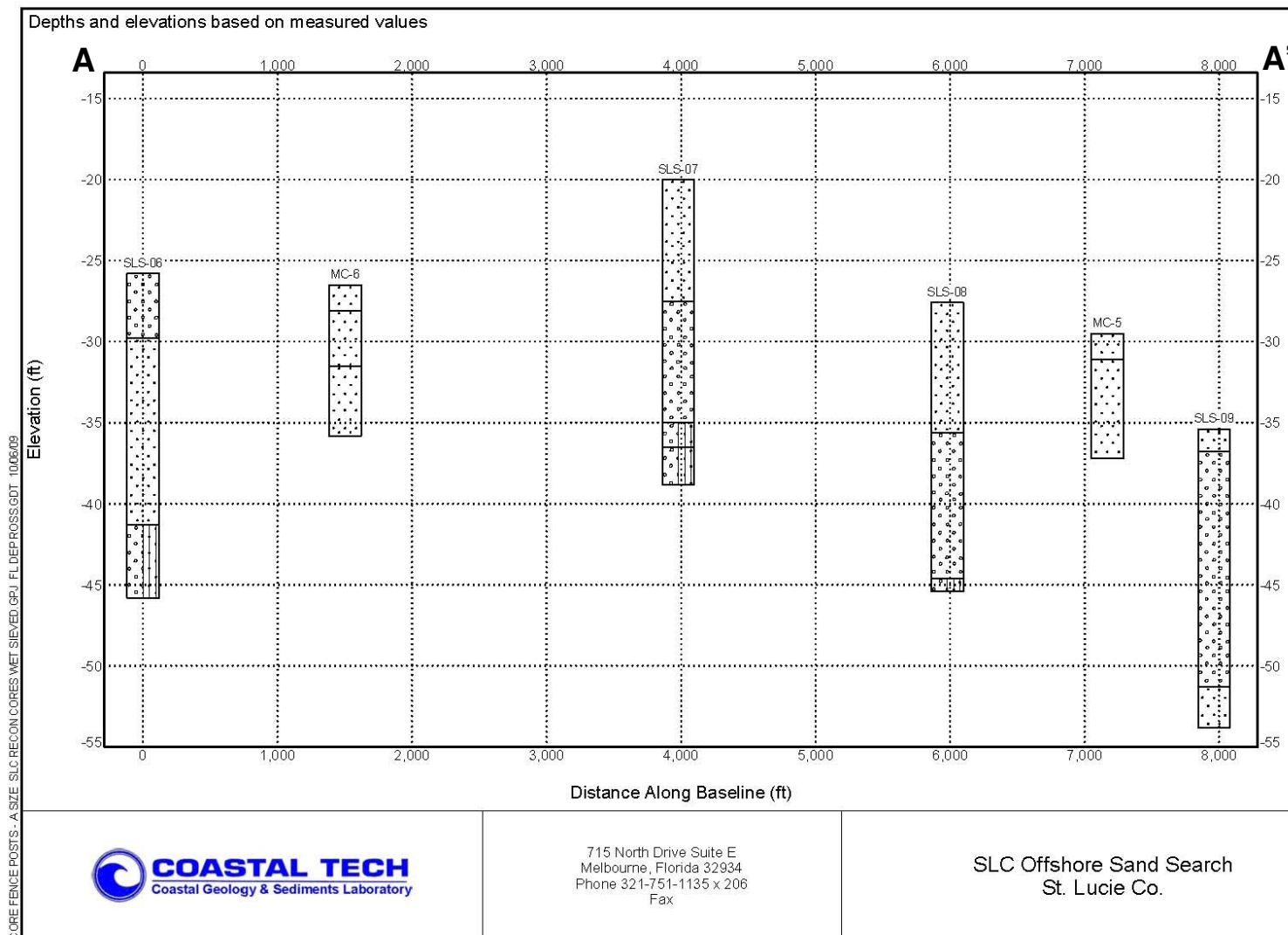
Figure 5.6: St. Lucie Shoal: Area A – Geologic Cross-Section
