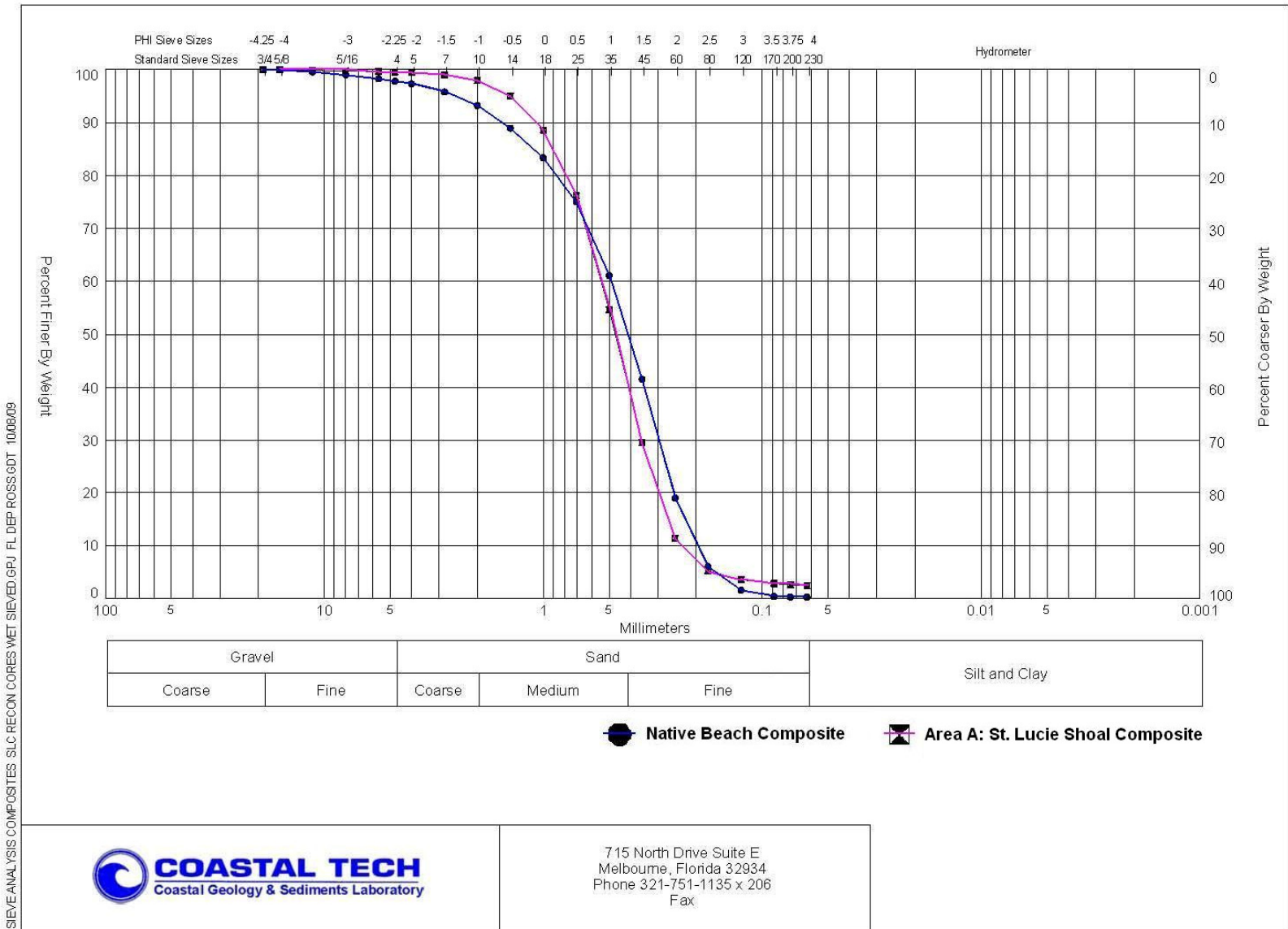
Figure 5.8: Native Beach and St. Lucie Shoal: Area A Composite Grain-size Distribution Curves
