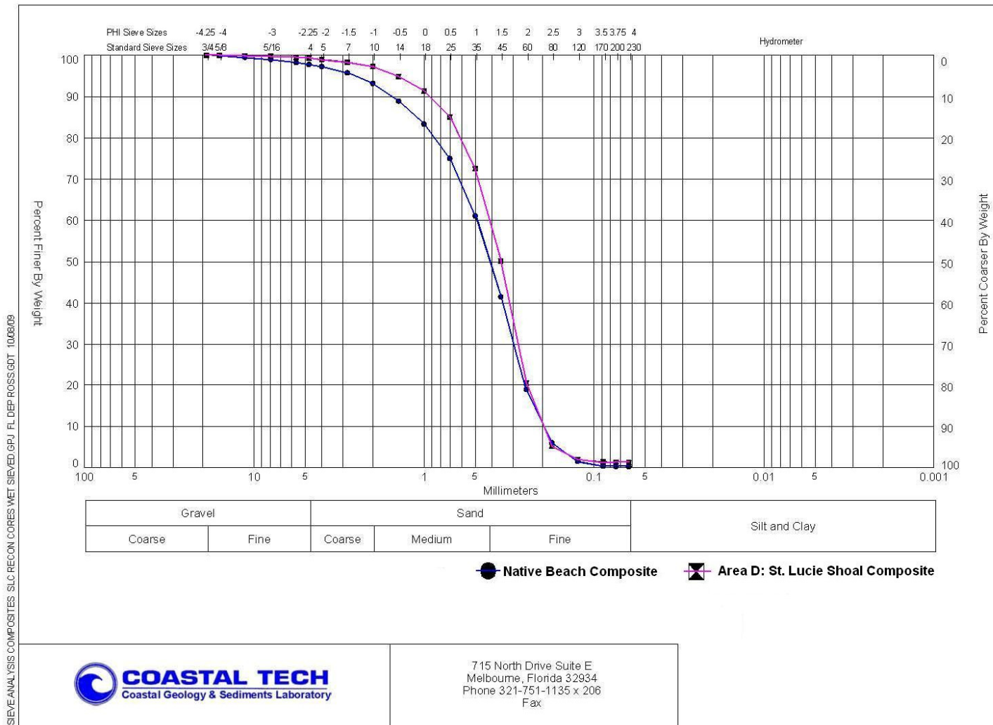
Figure 5.14: Native Beach and St. Lucie Shoal: Area D Composite Grain-size Distribution Curves
