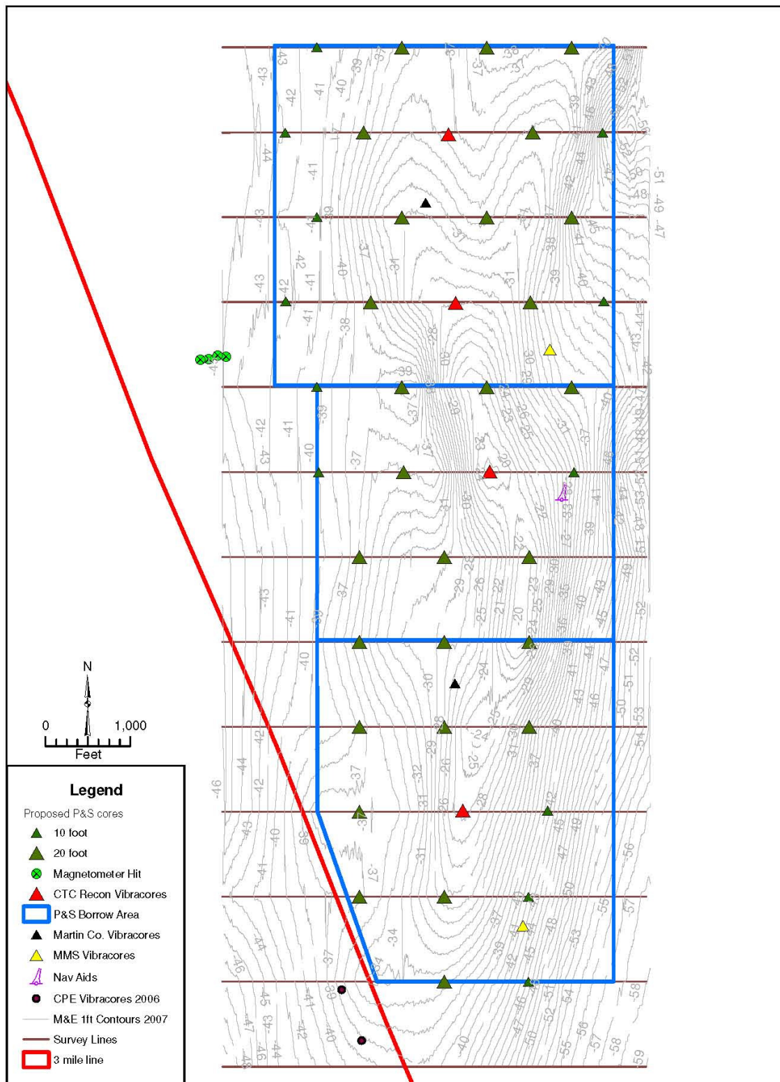
Figure 6.2: Proposed Plans and Specs Vibracoring Plan: Area A
