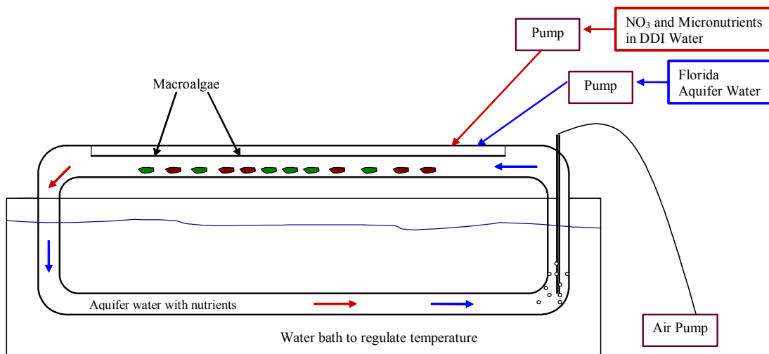
Figure 5.1. Cross-sectional view of a single stream channel. Water is lifted by air bubbles at one end of stream and flows over substrata in top of pipe, which has been cut out to expose open channel.
