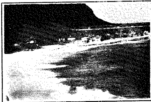
SURGING BREAKER
