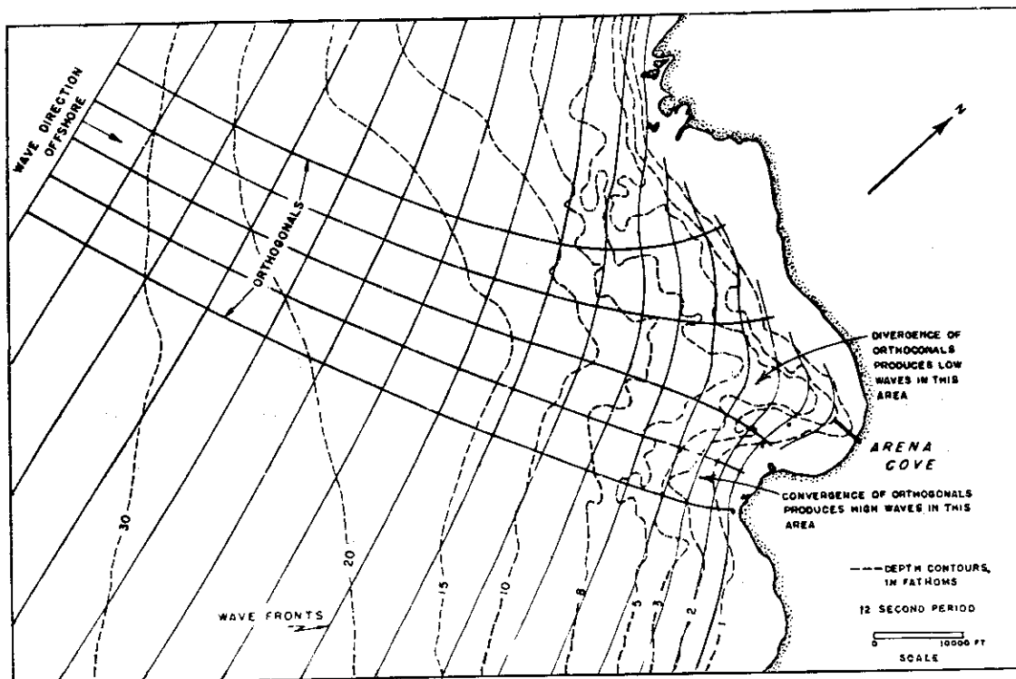
Figure A-6. Refraction Diagram.
