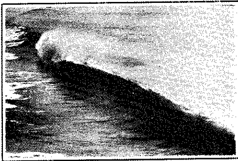
PLUNGING BREAKER
