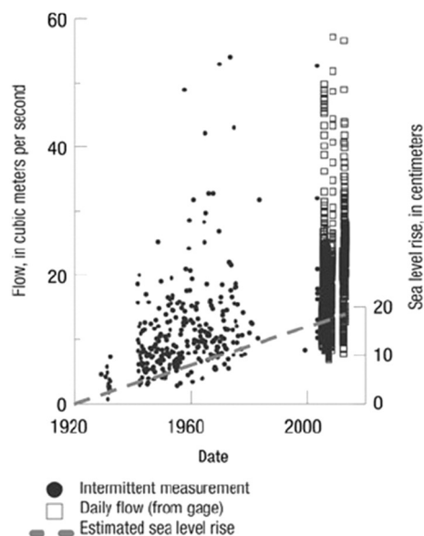
Fig. 8. Flow at Wakulla Springs from 1930 to 2010 and estimated sea level rise from 1920 to 2020, modified from Davis and Verdi (2014).
