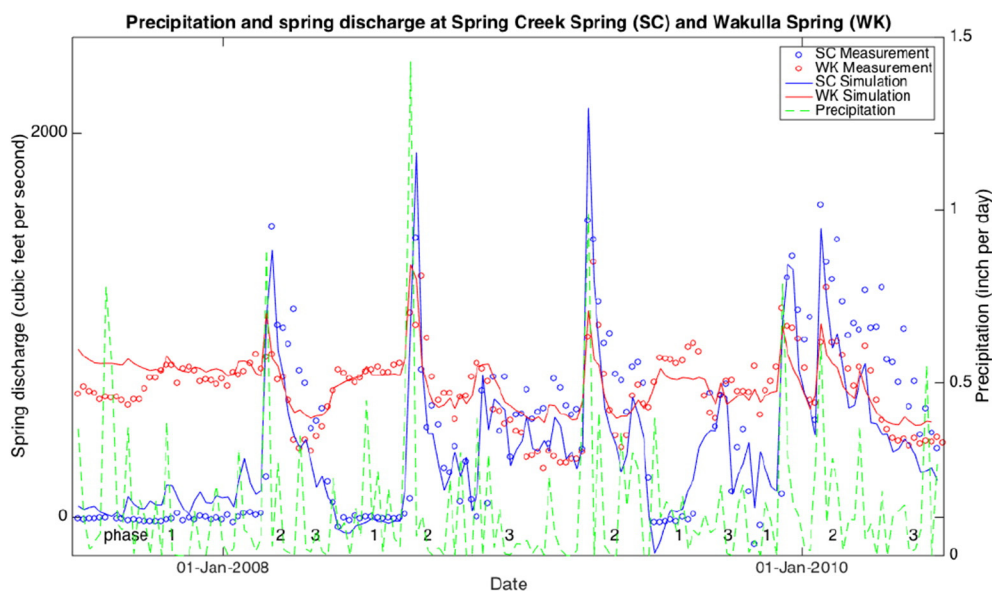
Fig. 6. Measured and simulated results of discharges at Wakulla Springs and Spring Creek Springs, from June 2007 to June 2010, as well as precipitation.
