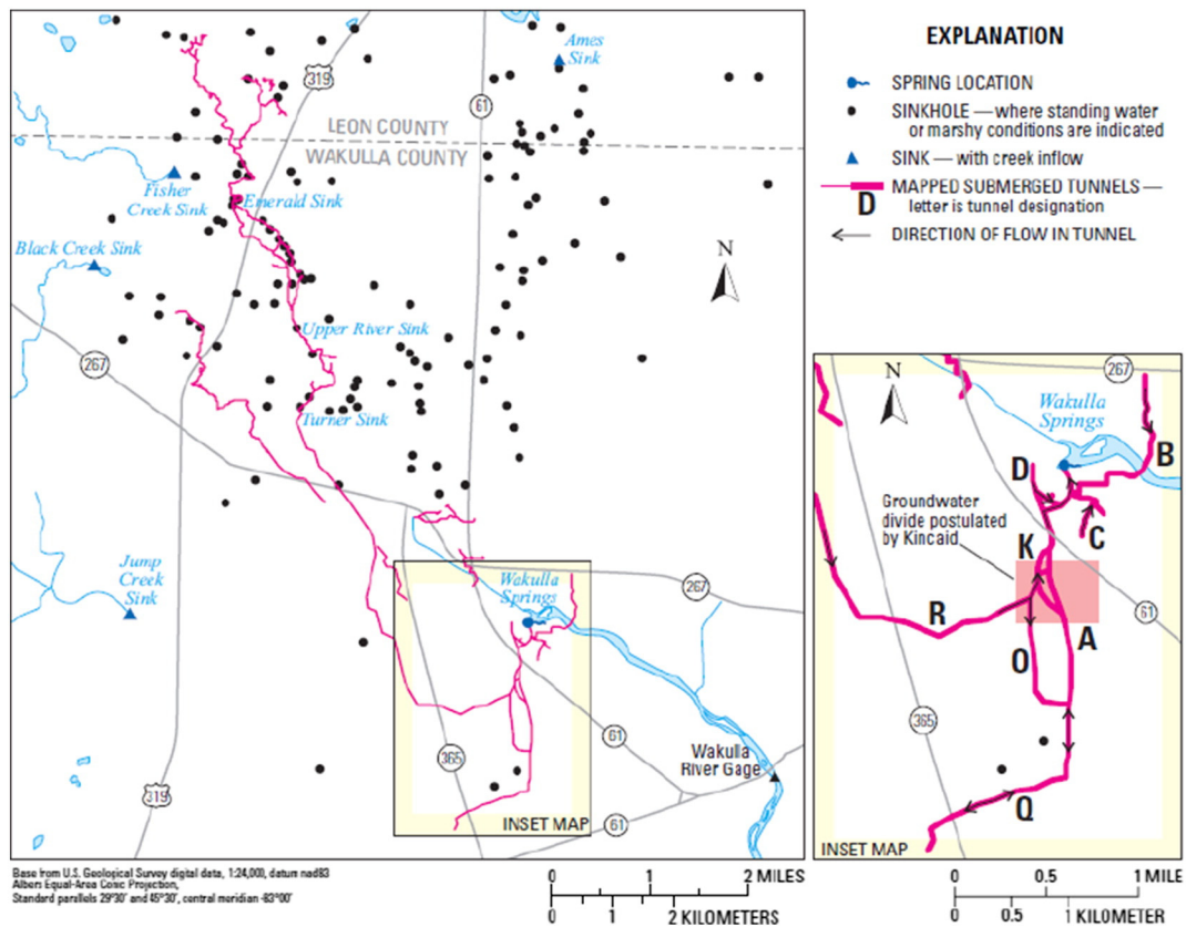
Fig. 3. Locations of subground conduit network systems in the area of Wakulla Spring, modified from Davis et al. (2010).
