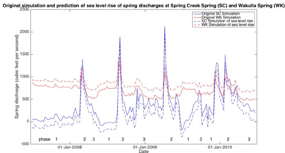
Fig. 7. Original (calibrated) simulation results and the prediction of rising sea level of the discharges at Wakulla Springs and Spring Creek Springs, from June 2007 to June 2010.
