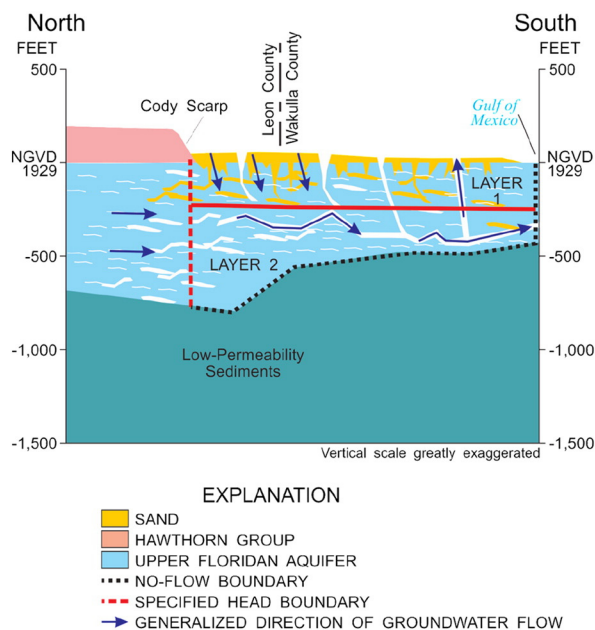
Fig. 2. Generalized geological cross section in Woodville Karst Plain and model layers, modified from Davis et al. (2010).
