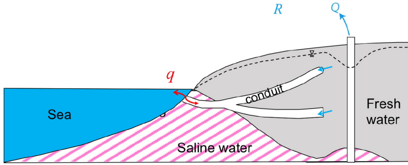
Fig. 4. Schematic cross-section of a coastal karst aquifer with conduit networks and submarine spring (Spring Creek Springs). Flow direction q would be seaward when precipitation recharge R is large; however, reversal occurs when sea level rises, pumping rate Q is high or precipitation recharge R is small.
